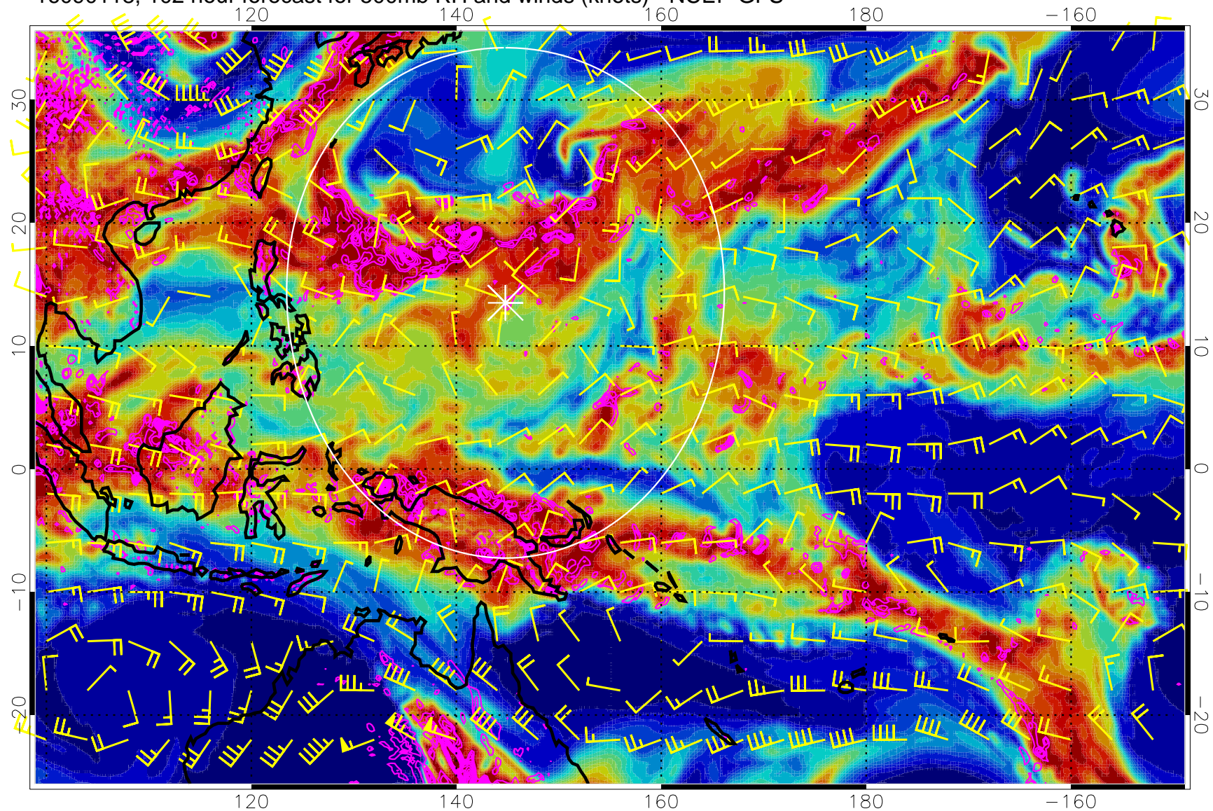
16090118, 102 hour forecast for 500mb RH and winds (knots) - NCEP GFS
