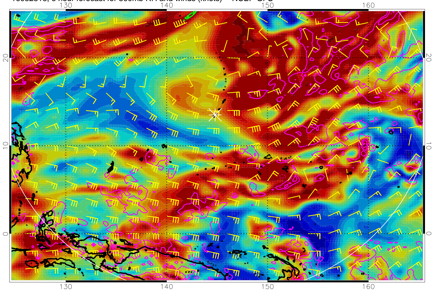
16082818, 6 hour forecast for 300mb RH and winds (knots) -- NCEP GFS
