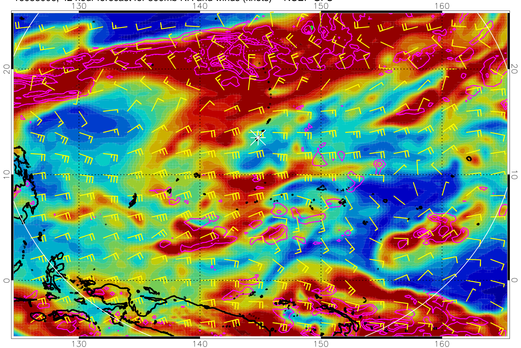
16083006, 42 hour forecast for 300mb RH and winds (knots) -- NCEP GFS
