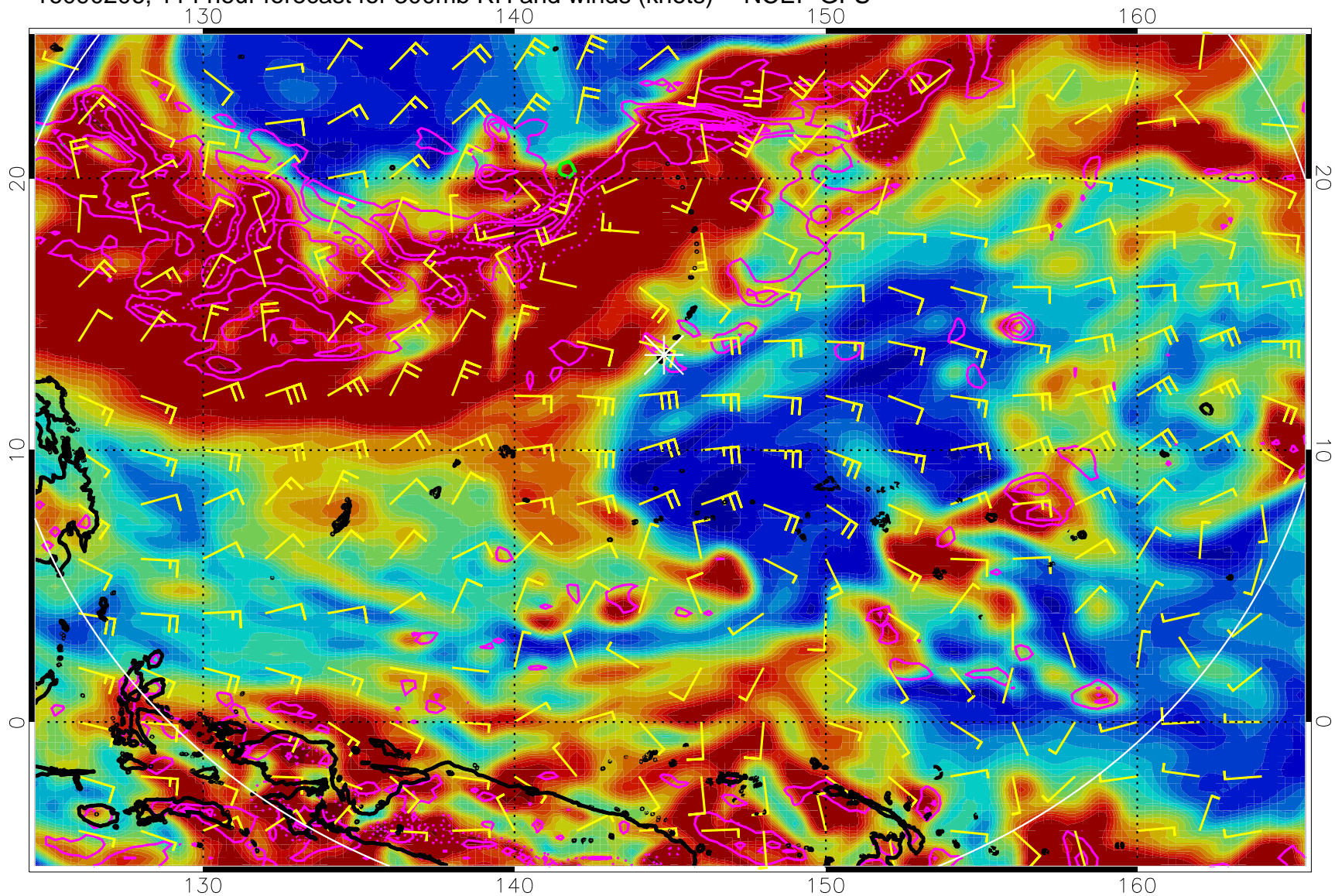
16090206, 114 hour forecast for 300mb RH and winds (knots) -- NCEP GFS
