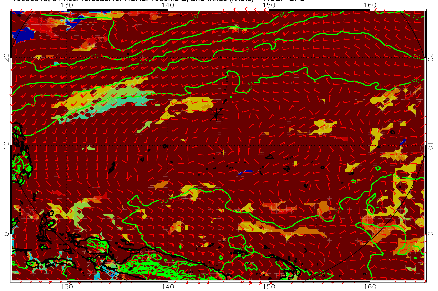
16083018, 54 hour forecast for HCAL, 1000mb Z, and winds (knots) -- NCEP GFS
