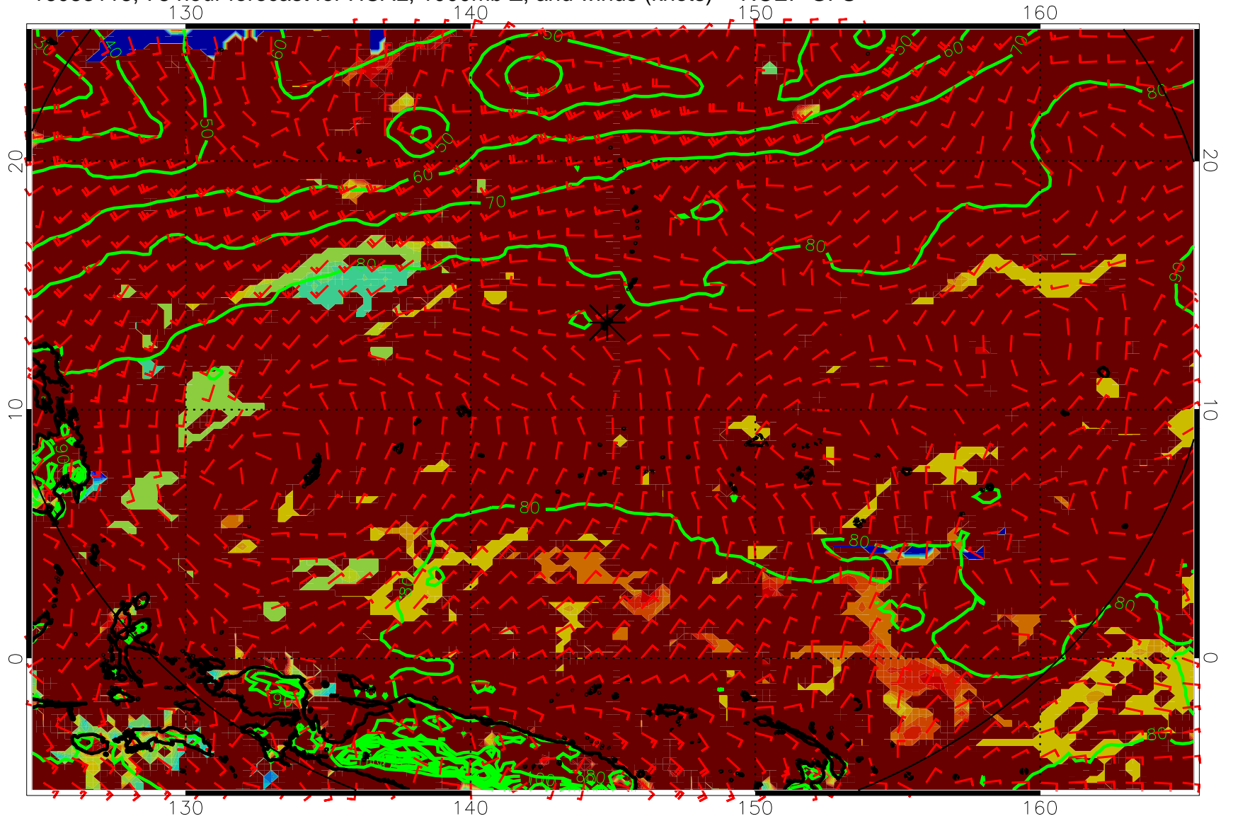
16083118, 78 hour forecast for HCAL, 1000mb Z, and winds (knots) -- NCEP GFS
