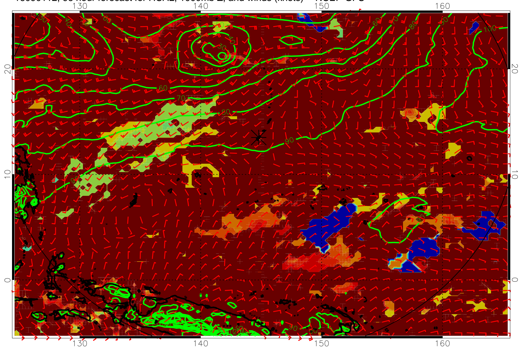
16090112, 96 hour forecast for HCAL, 1000mb Z, and winds (knots) -- NCEP GFS
