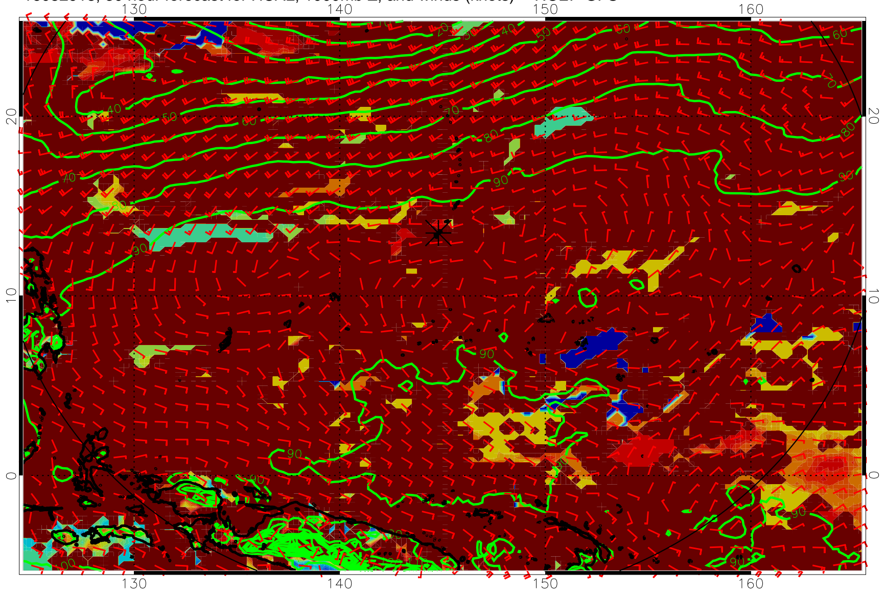
16082918, 30 hour forecast for HCAL, 1000mb Z, and winds (knots) -- NCEP GFS
