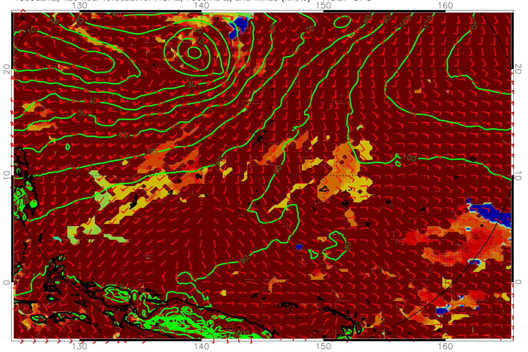
16090212, 120 hour forecast for HCAL, 1000mb Z, and winds (knots) -- NCEP GFS
