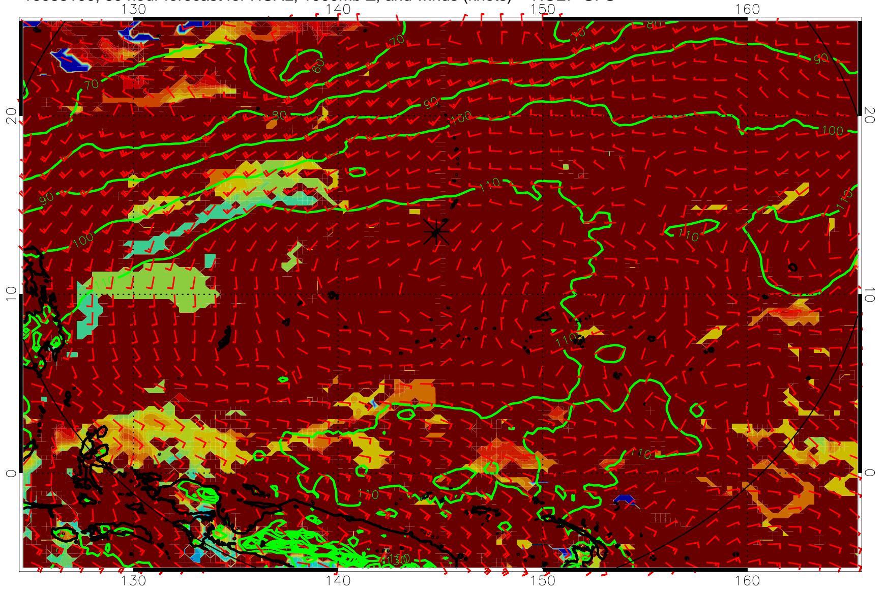
16083100, 60 hour forecast for HCAL, 1000mb Z, and winds (knots) -- NCEP GFS
