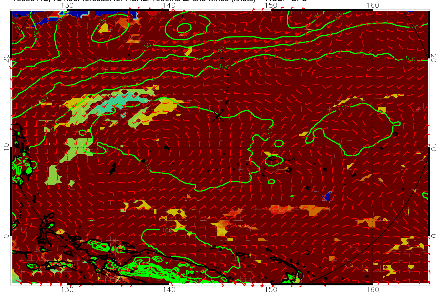
16083112, 72 hour forecast for HCAL, 1000mb Z, and winds (knots) -- NCEP GFS
