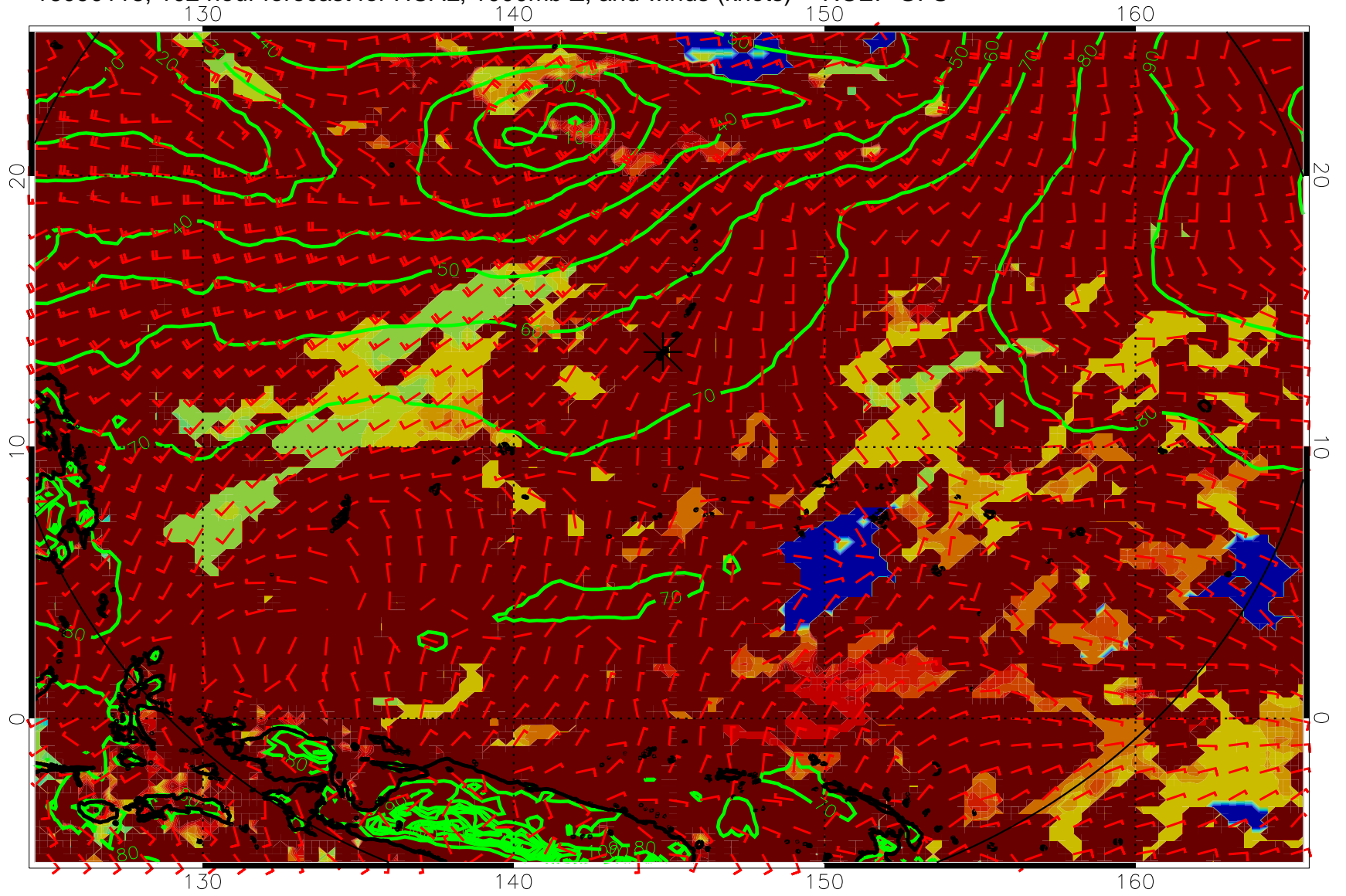
16090118, 102 hour forecast for HCAL, 1000mb Z, and winds (knots) -- NCEP GFS
