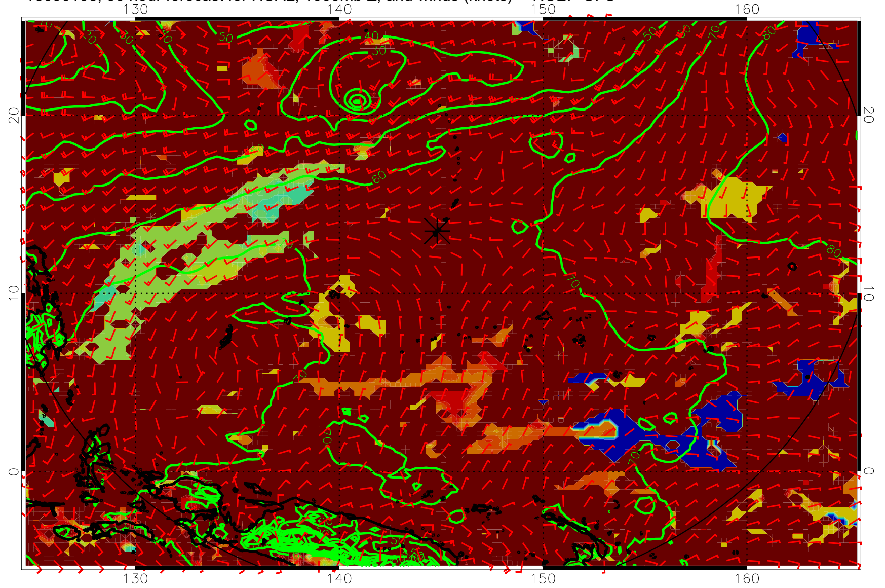
16090106, 90 hour forecast for HCAL, 1000mb Z, and winds (knots) -- NCEP GFS
