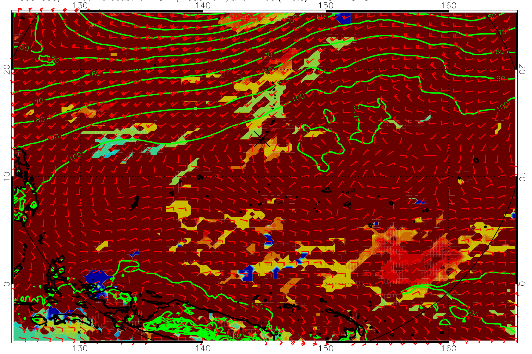
16082900, 12 hour forecast for HCAL, 1000mb Z, and winds (knots) -- NCEP GFS
