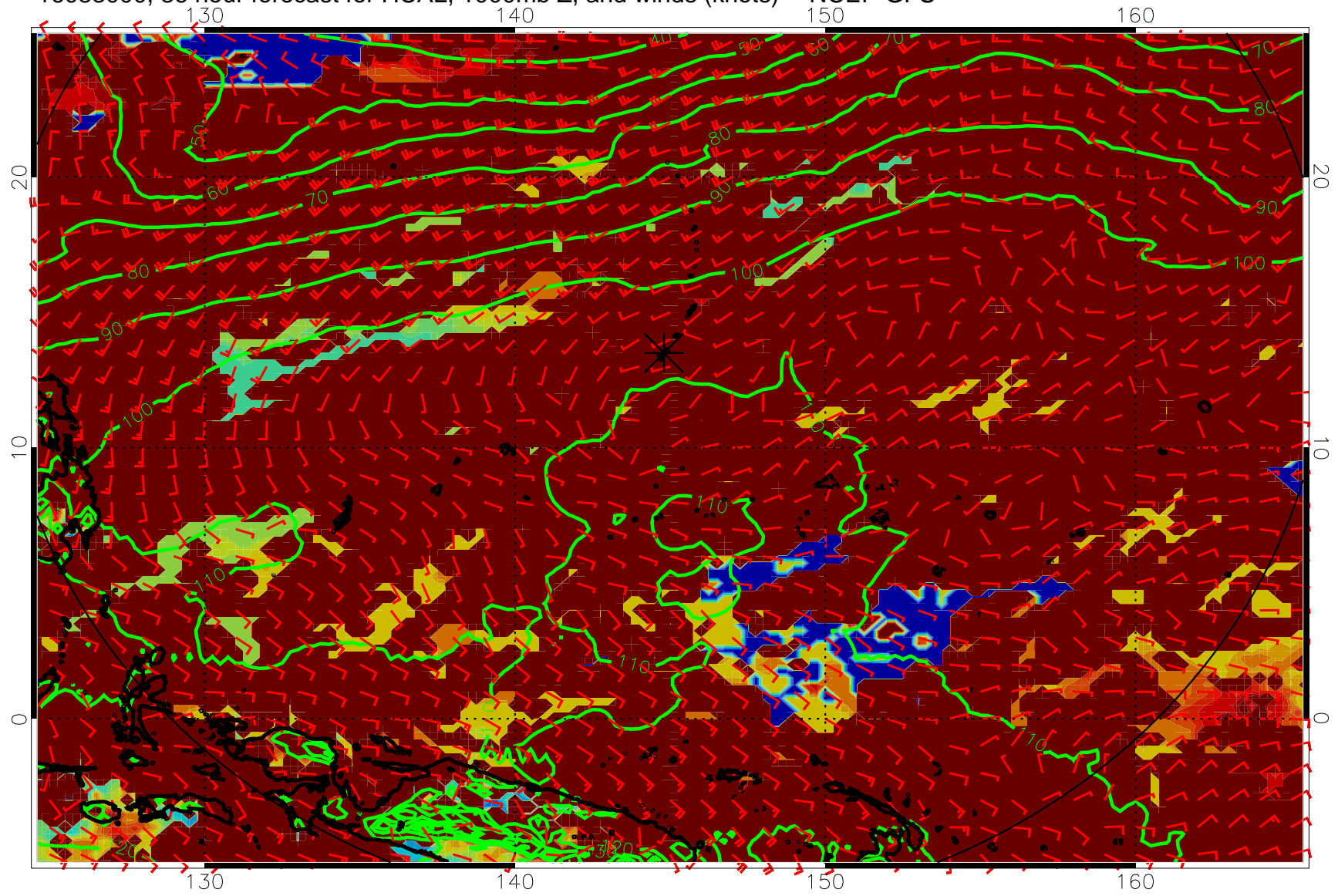
16083000, 36 hour forecast for HCAL, 1000mb Z, and winds (knots) -- NCEP GFS
