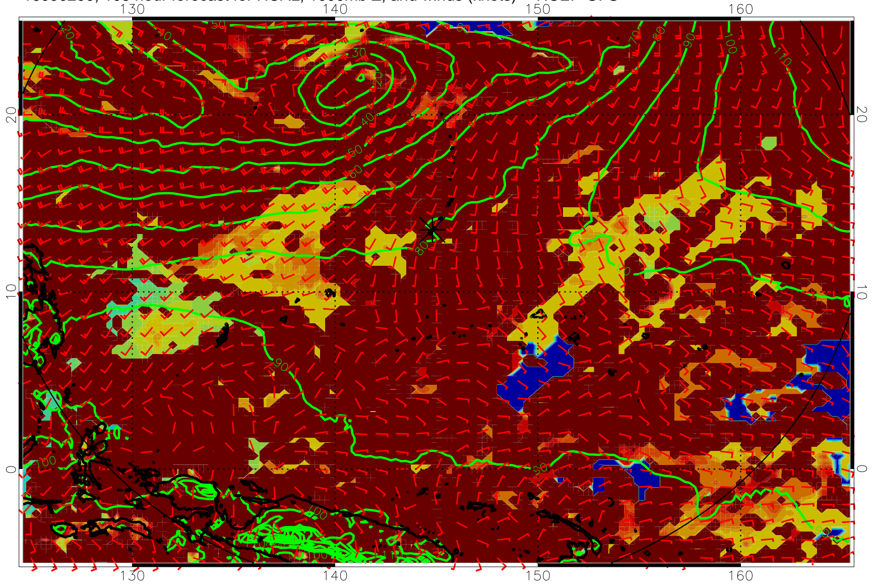
16090200, 108 hour forecast for HCAL, 1000mb Z, and winds (knots) -- NCEP GFS
