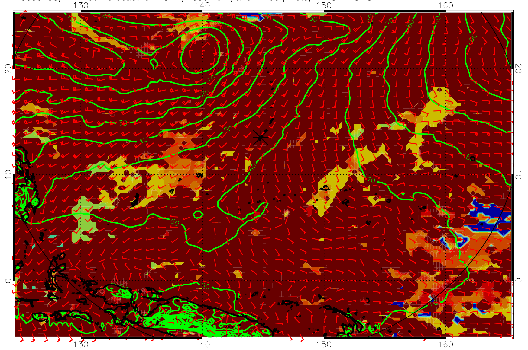
16090206, 114 hour forecast for HCAL, 1000mb Z, and winds (knots) -- NCEP GFS
