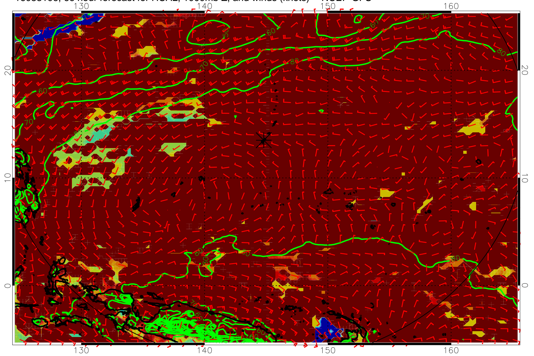
16083106, 66 hour forecast for HCAL, 1000mb Z, and winds (knots) -- NCEP GFS
