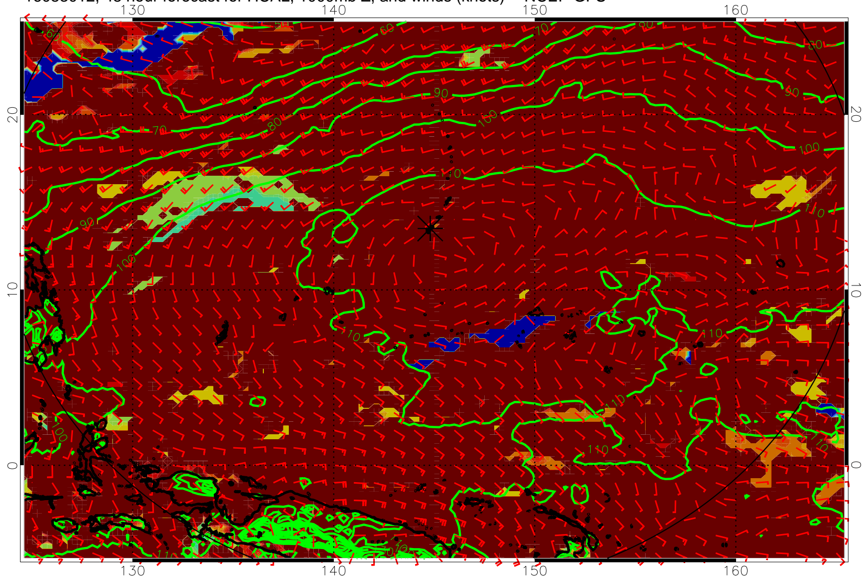
16083012, 48 hour forecast for HCAL, 1000mb Z, and winds (knots) -- NCEP GFS
