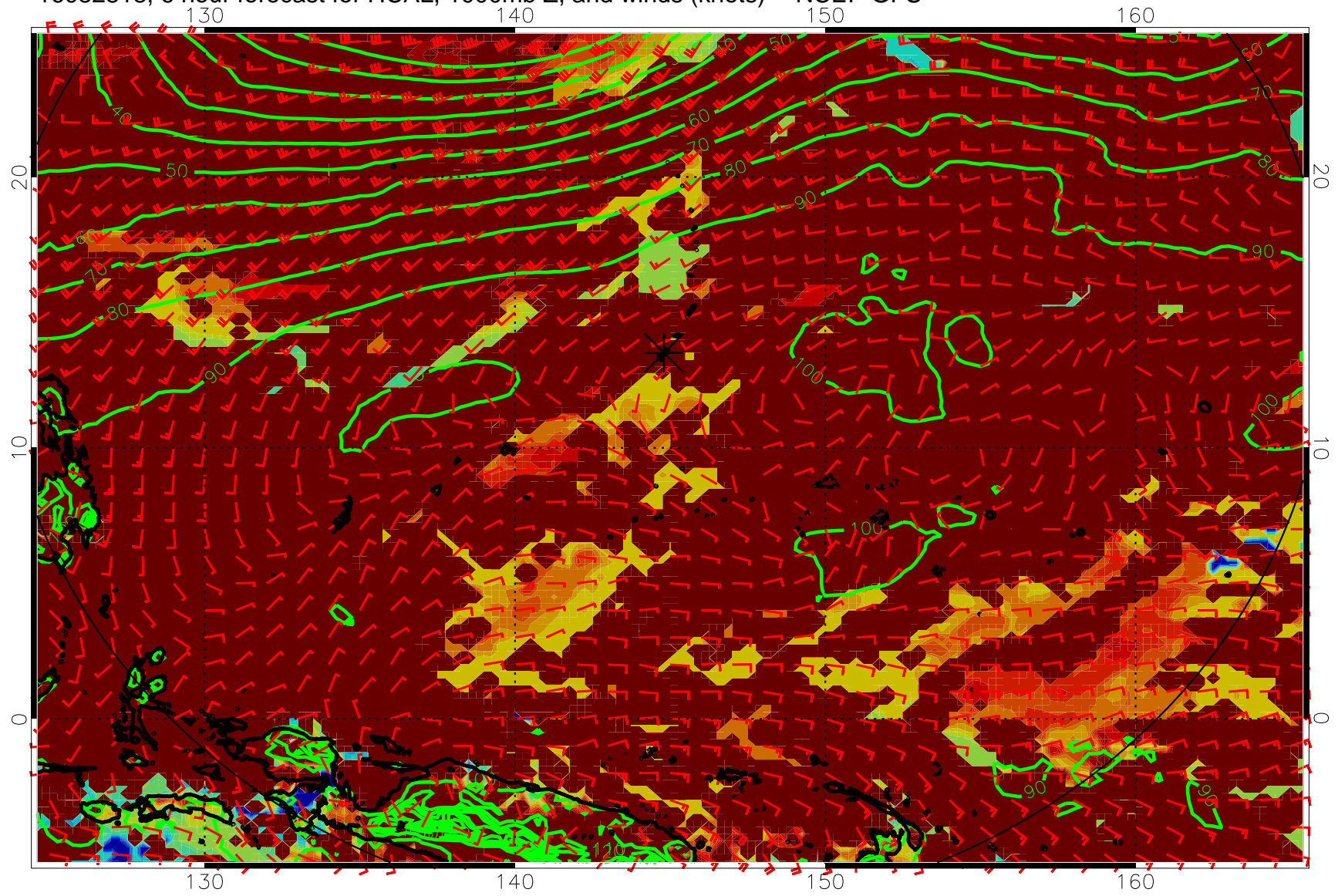
16082818, 6 hour forecast for HCAL, 1000mb Z, and winds (knots) -- NCEP GFS
