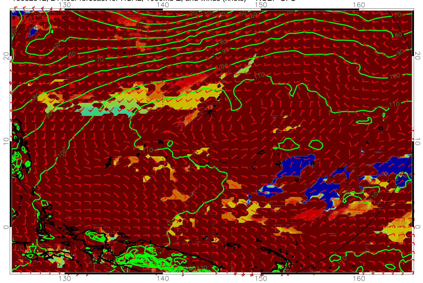
16082912, 24 hour forecast for HCAL, 1000mb Z, and winds (knots) -- NCEP GFS
