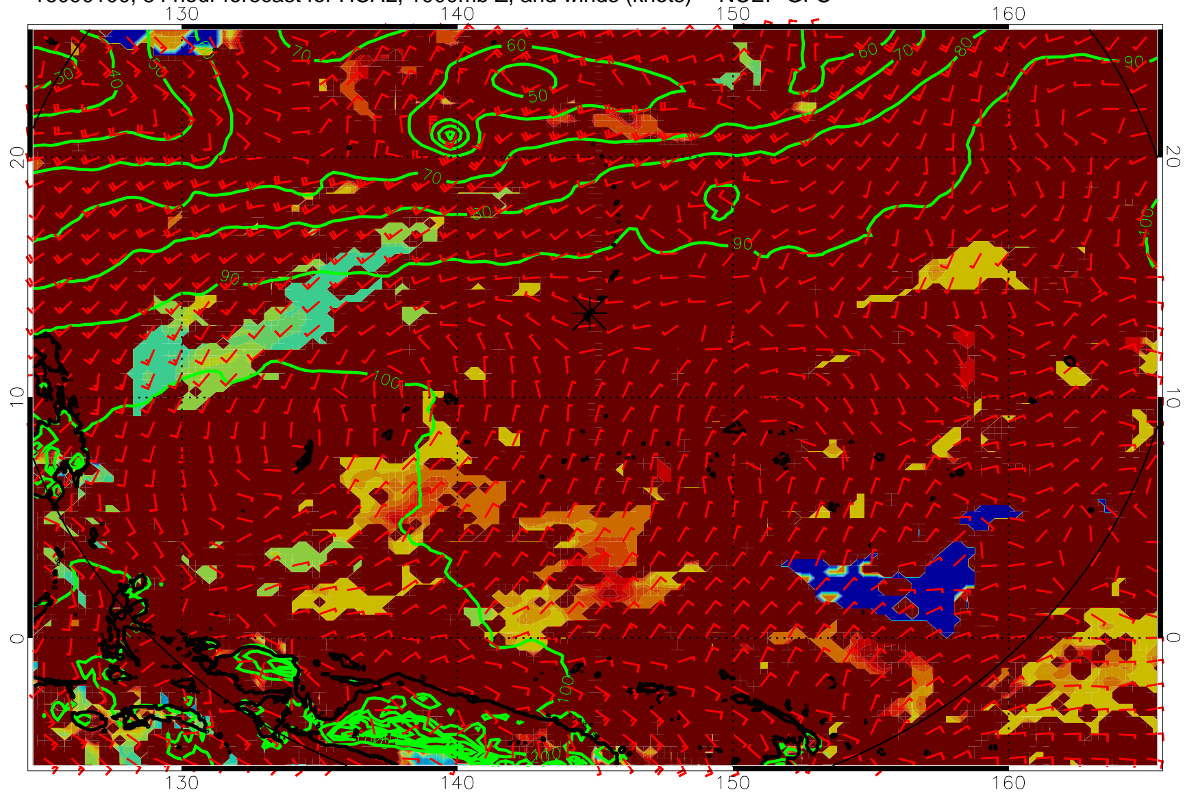
16090100, 84 hour forecast for HCAL, 1000mb Z, and winds (knots) -- NCEP GFS
