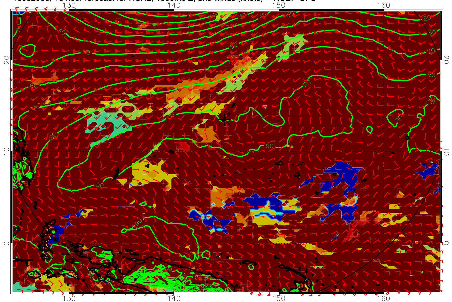
16082906, 18 hour forecast for HCAL, 1000mb Z, and winds (knots) -- NCEP GFS
