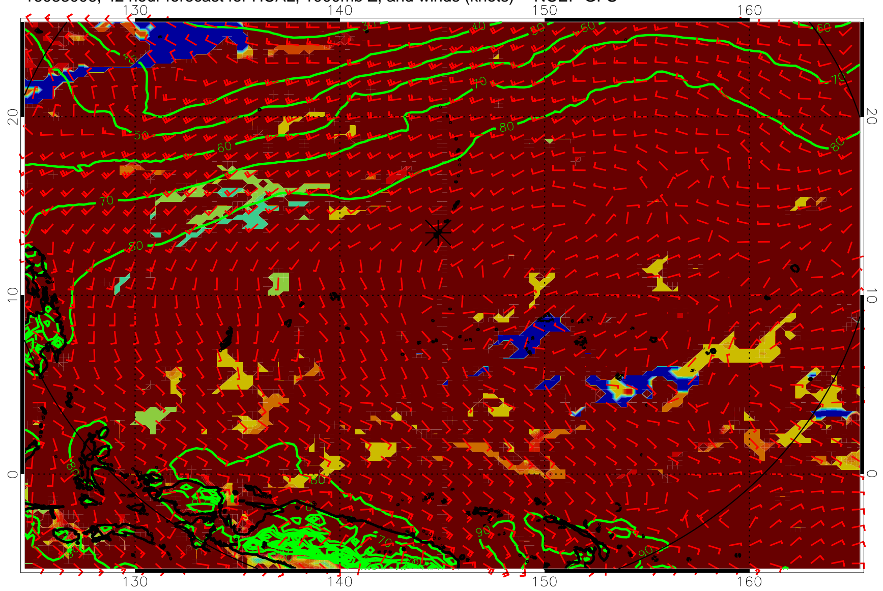
16083006, 42 hour forecast for HCAL, 1000mb Z, and winds (knots) -- NCEP GFS
