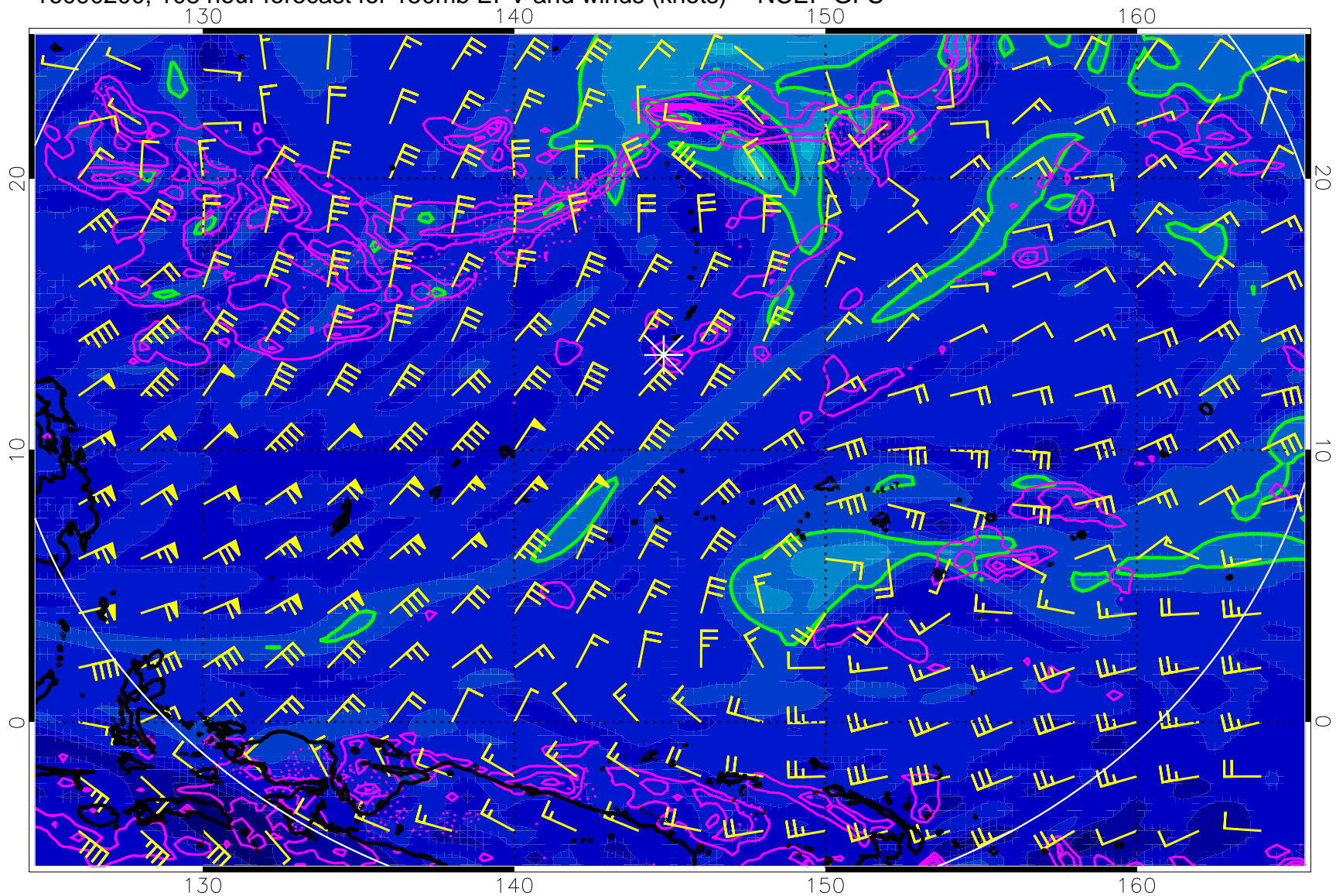
16090200, 108 hour forecast for 150mb EPV and winds (knots) -- NCEP GFS
