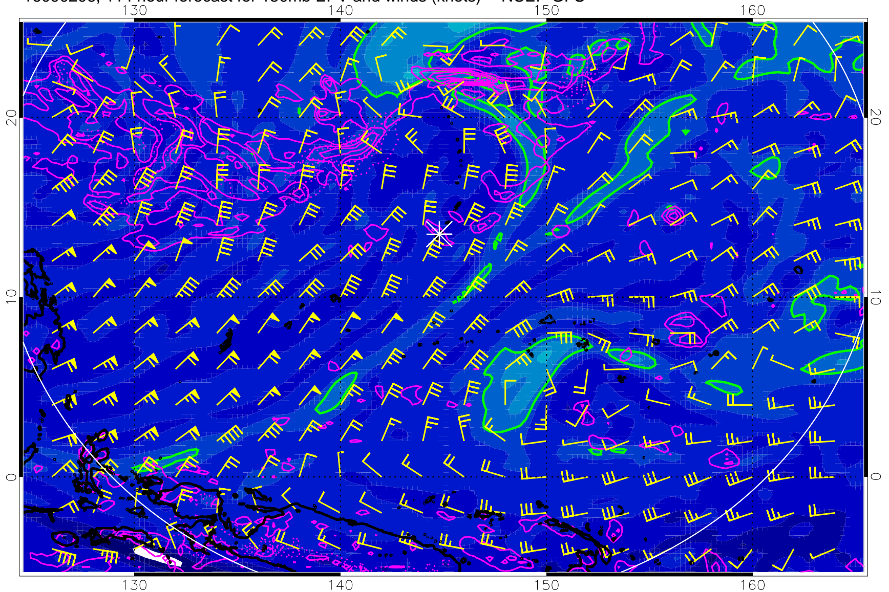
16090206, 114 hour forecast for 150mb EPV and winds (knots) -- NCEP GFS
