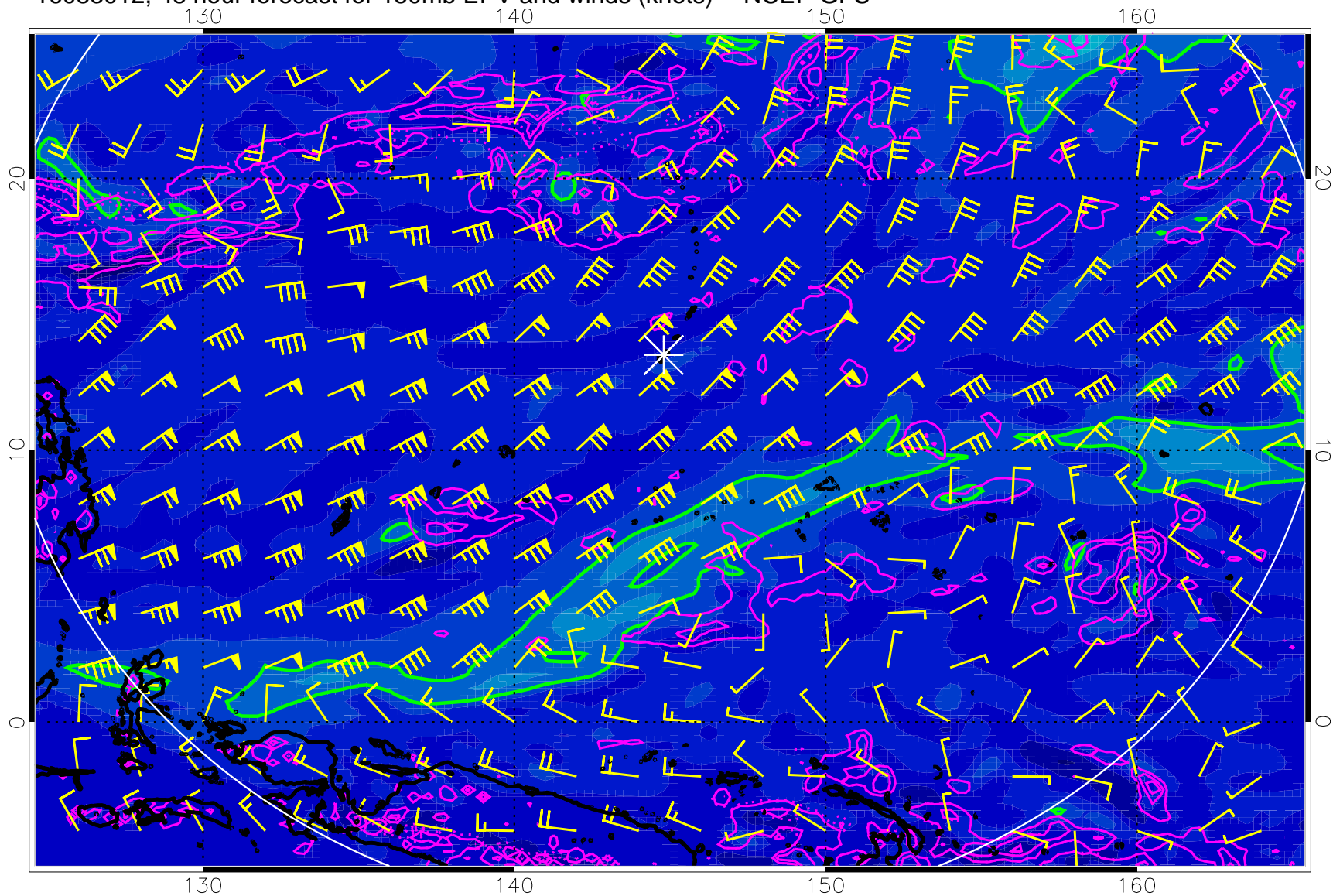
16083012, 48 hour forecast for 150mb EPV and winds (knots) -- NCEP GFS
