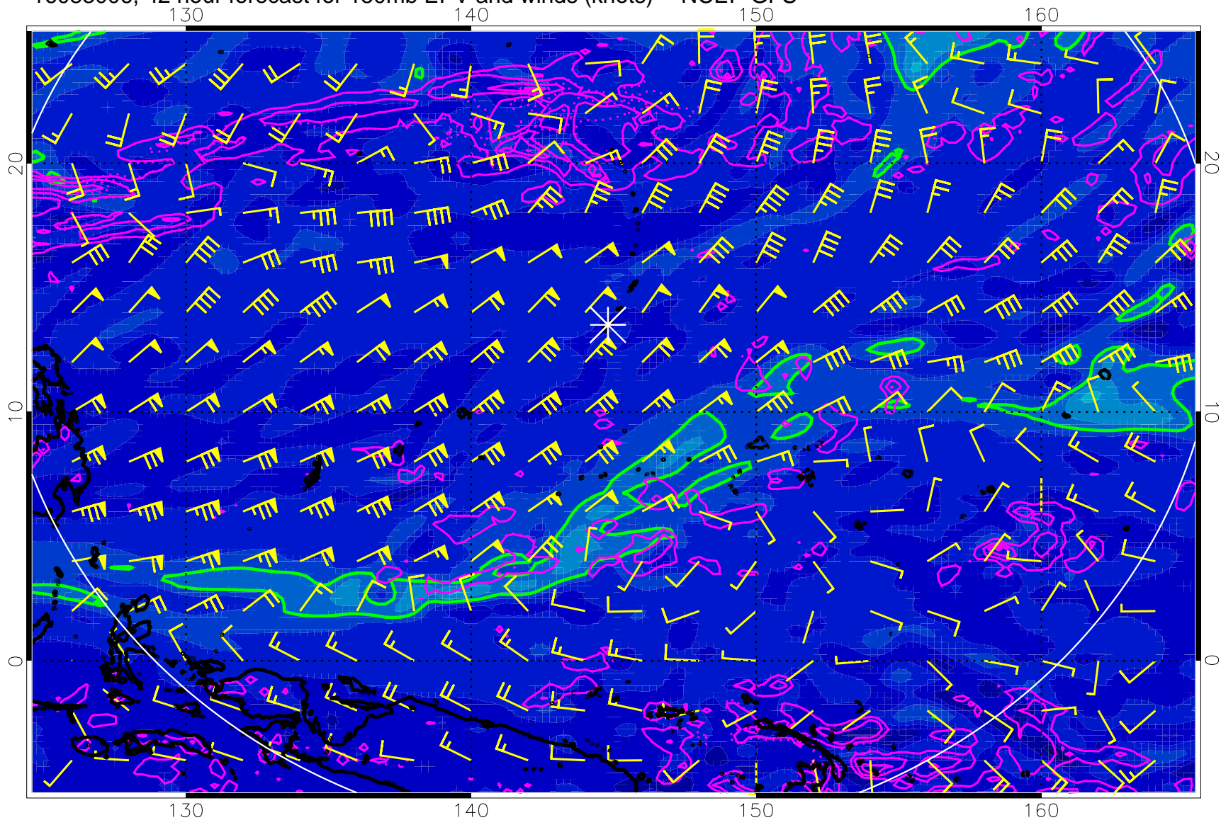
16083006, 42 hour forecast for 150mb EPV and winds (knots) -- NCEP GFS
