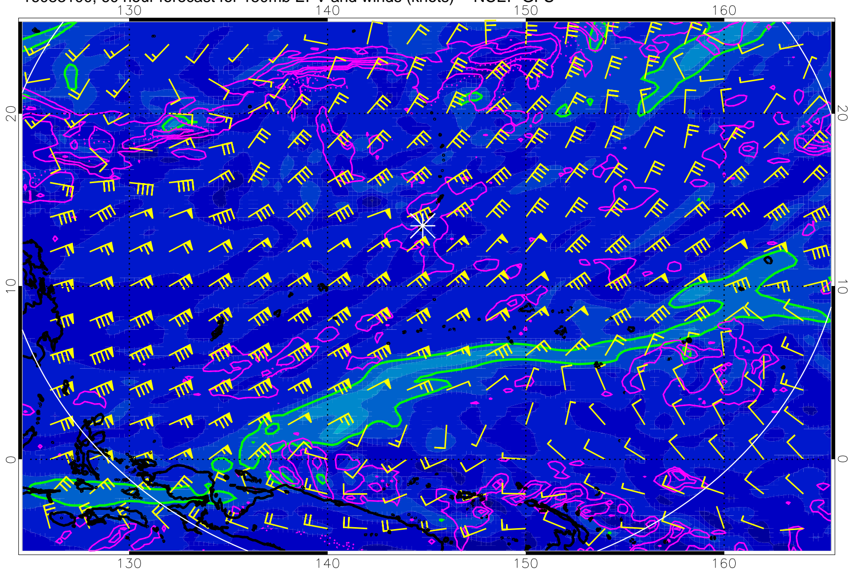
16083100, 60 hour forecast for 150mb EPV and winds (knots) -- NCEP GFS
