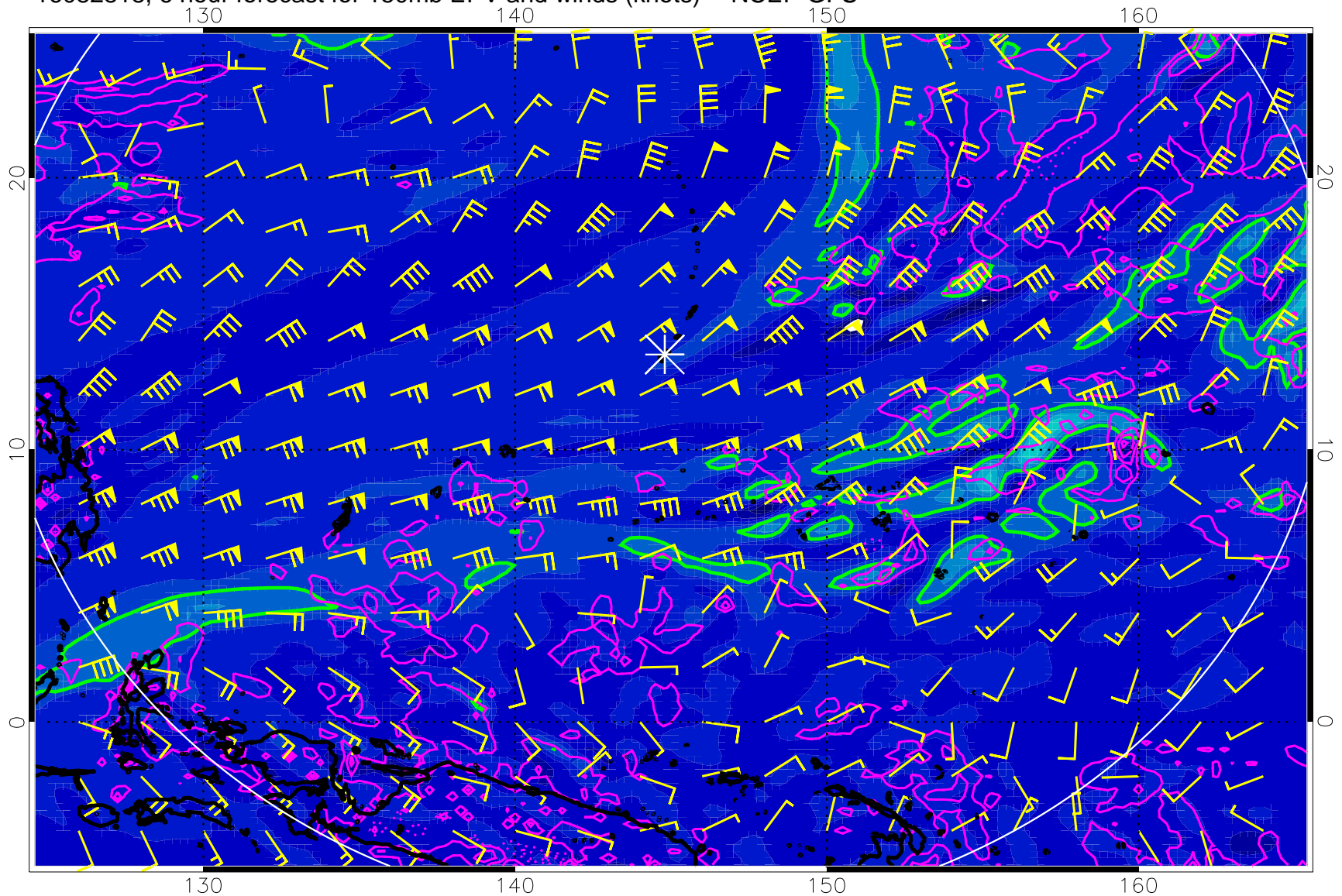
16082818, 6 hour forecast for 150mb EPV and winds (knots) -- NCEP GFS
