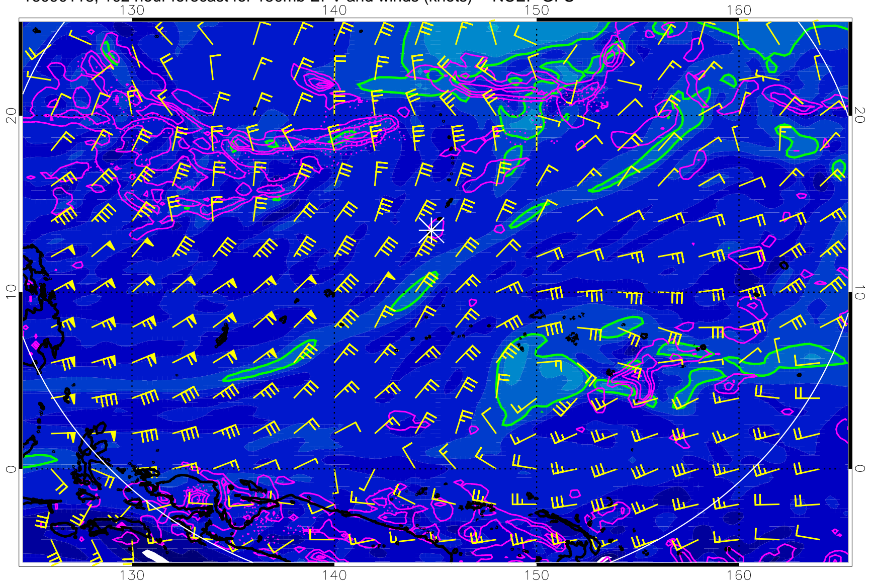
16090118, 102 hour forecast for 150mb EPV and winds (knots) -- NCEP GFS
