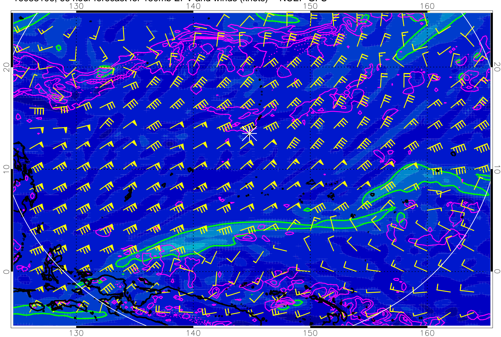
16083106, 66 hour forecast for 150mb EPV and winds (knots) -- NCEP GFS
