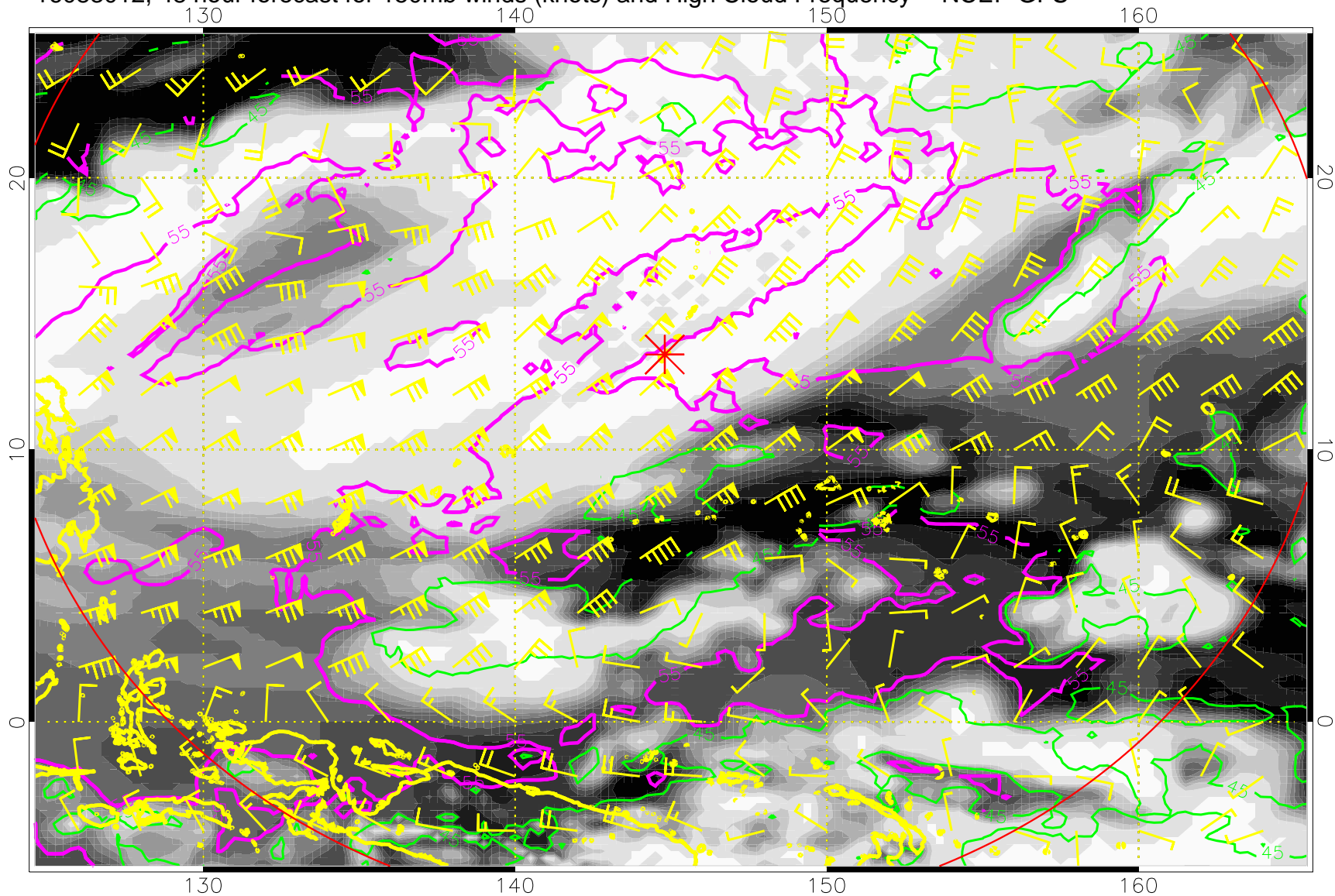
16083012, 48 hour forecast for 150mb winds (knots) and High Cloud Frequency -- NCEP GFS
