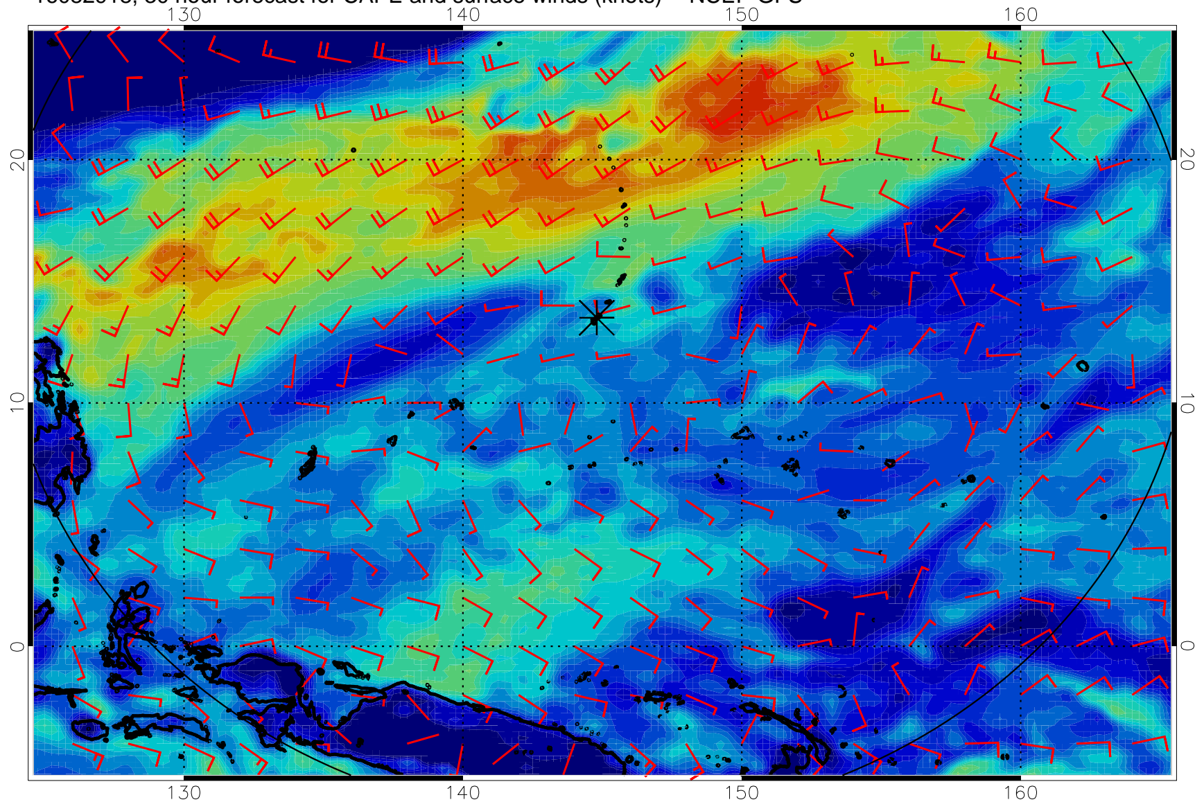
16082918, 30 hour forecast for CAPE and surface winds (knots) -- NCEP GFS
