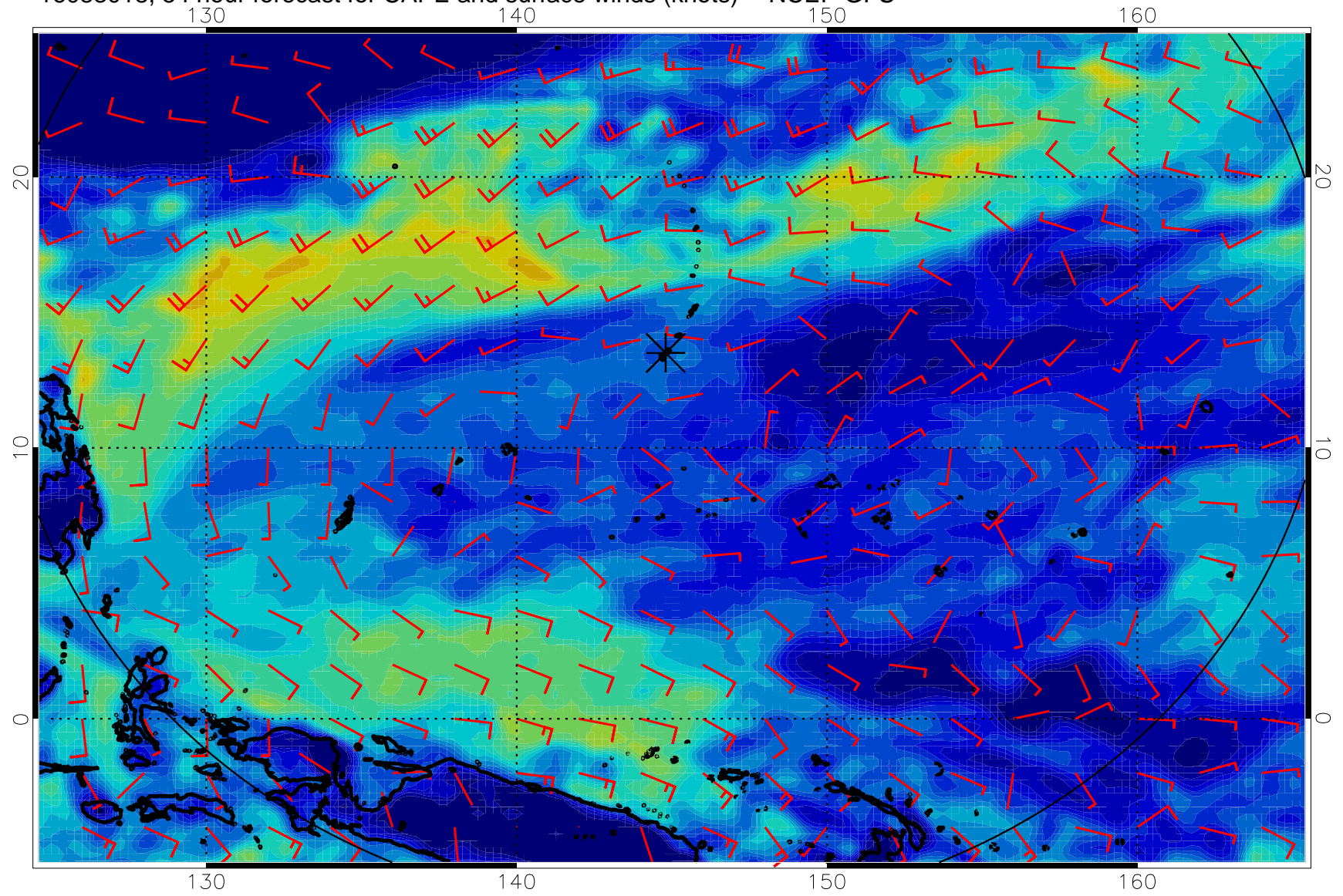
16083018, 54 hour forecast for CAPE and surface winds (knots) -- NCEP GFS
