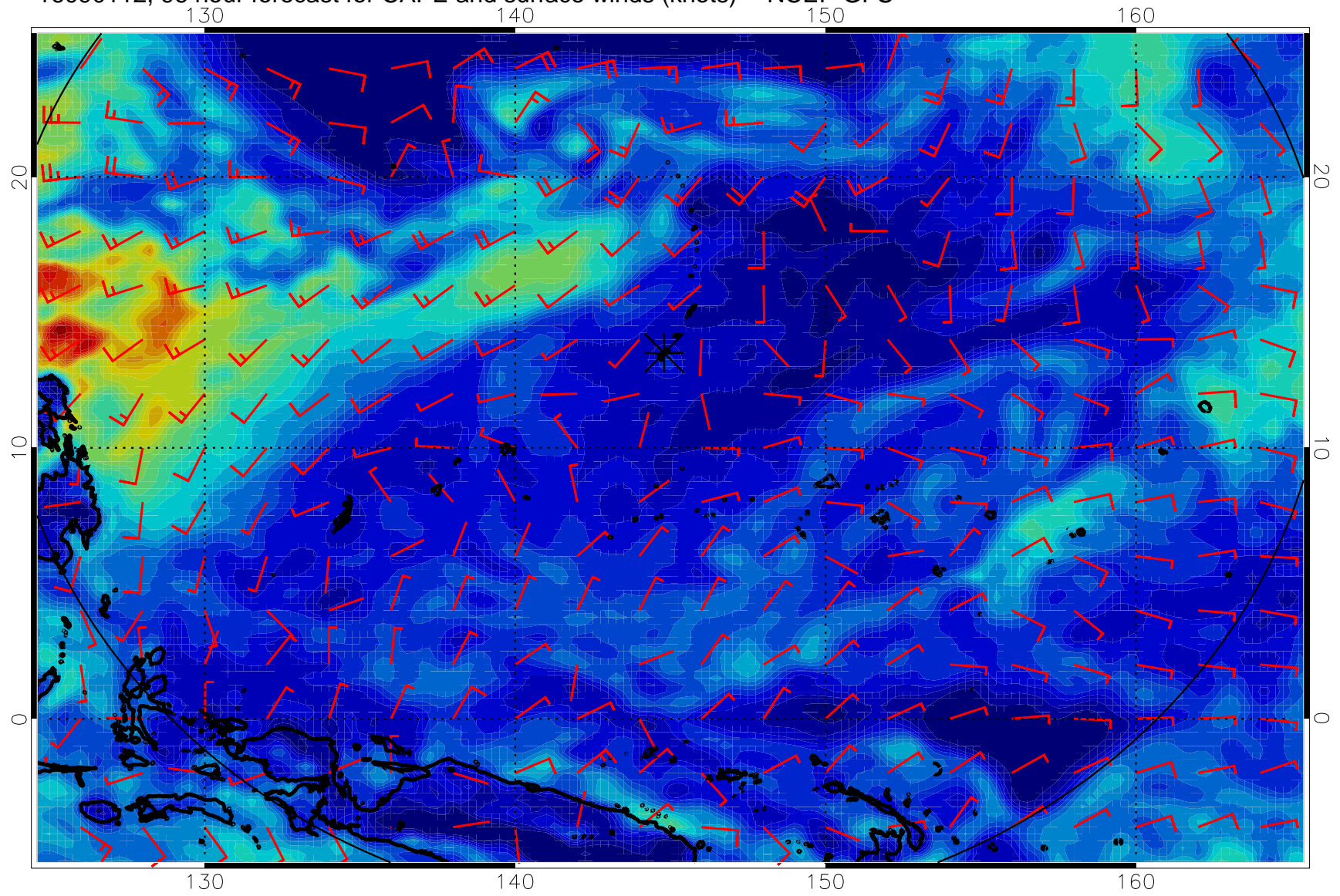
16090112, 96 hour forecast for CAPE and surface winds (knots) -- NCEP GFS
