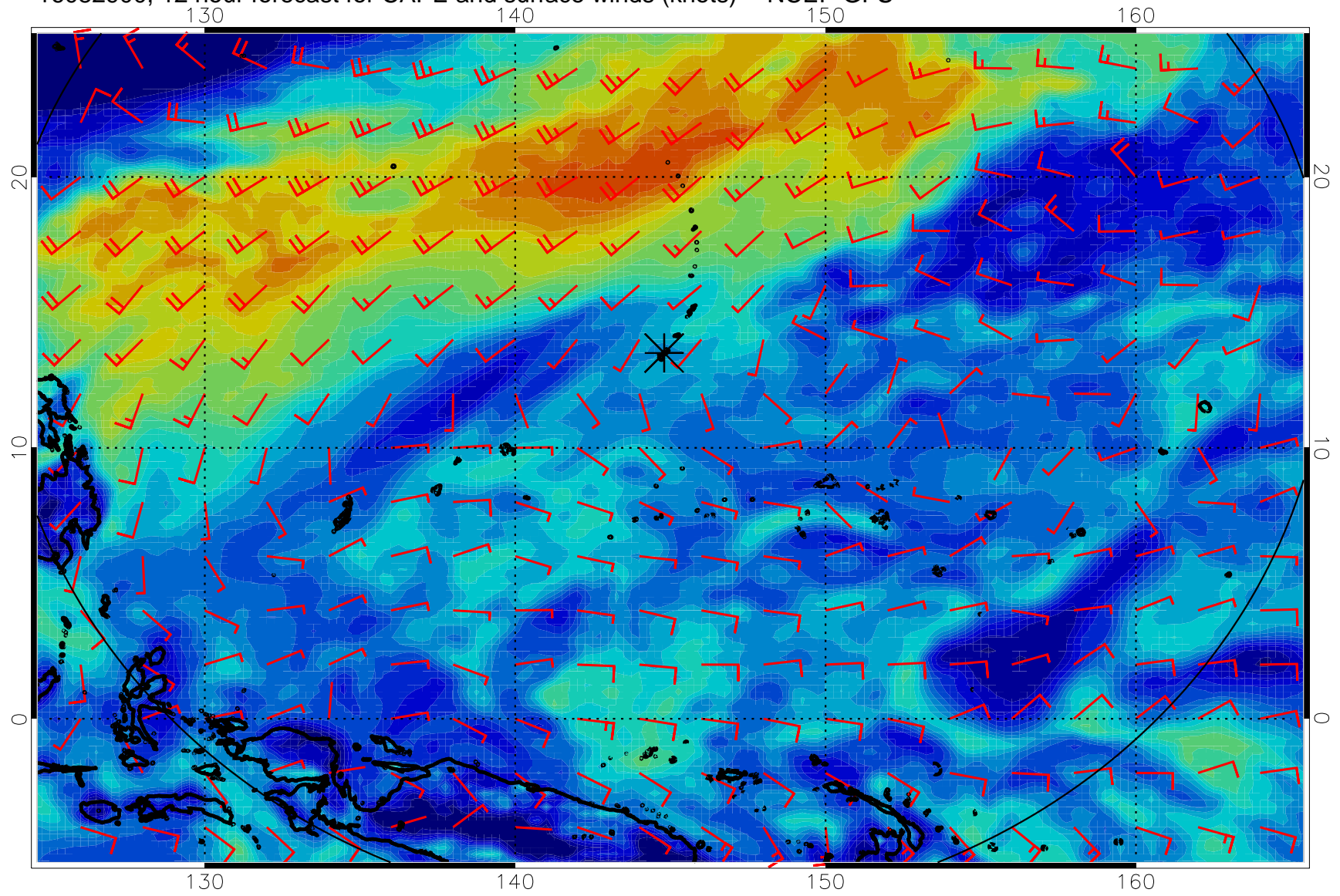
16082900, 12 hour forecast for CAPE and surface winds (knots) -- NCEP GFS
