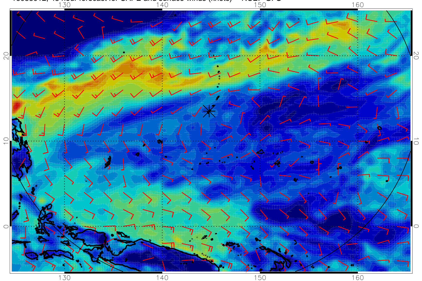
16083012, 48 hour forecast for CAPE and surface winds (knots) -- NCEP GFS
