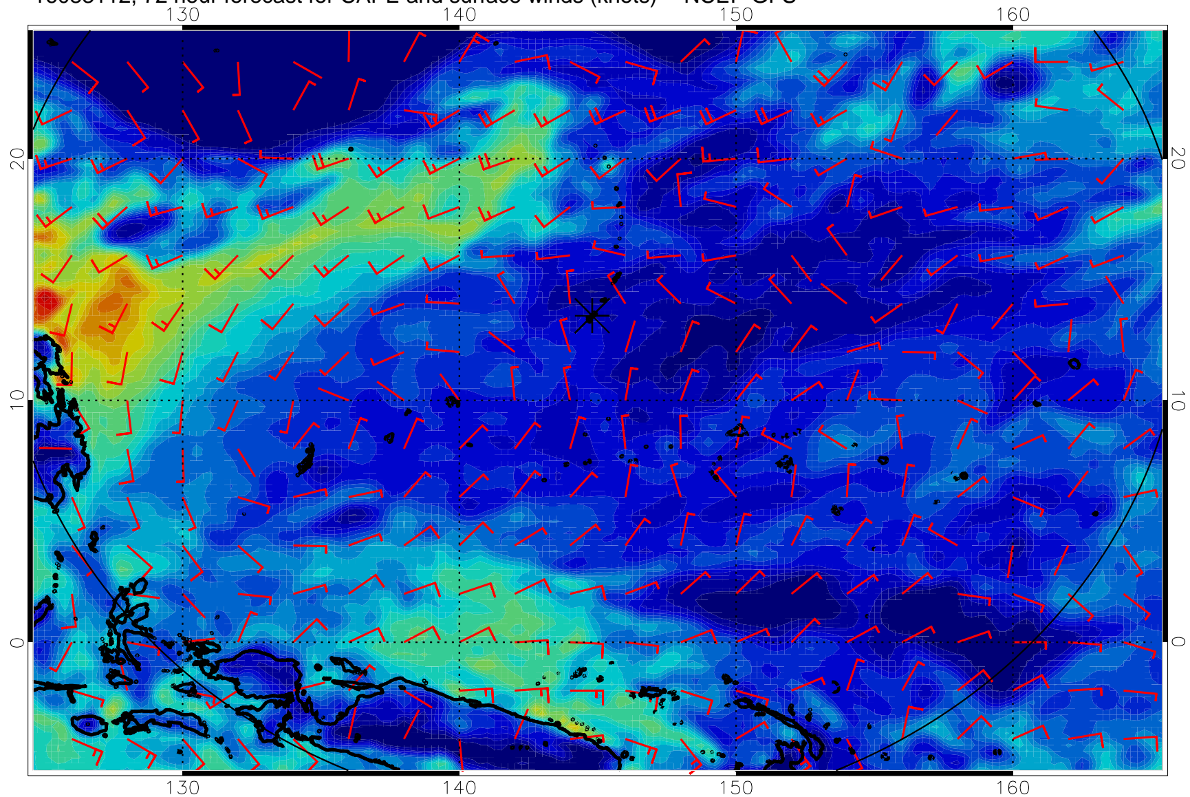
16083112, 72 hour forecast for CAPE and surface winds (knots) -- NCEP GFS
