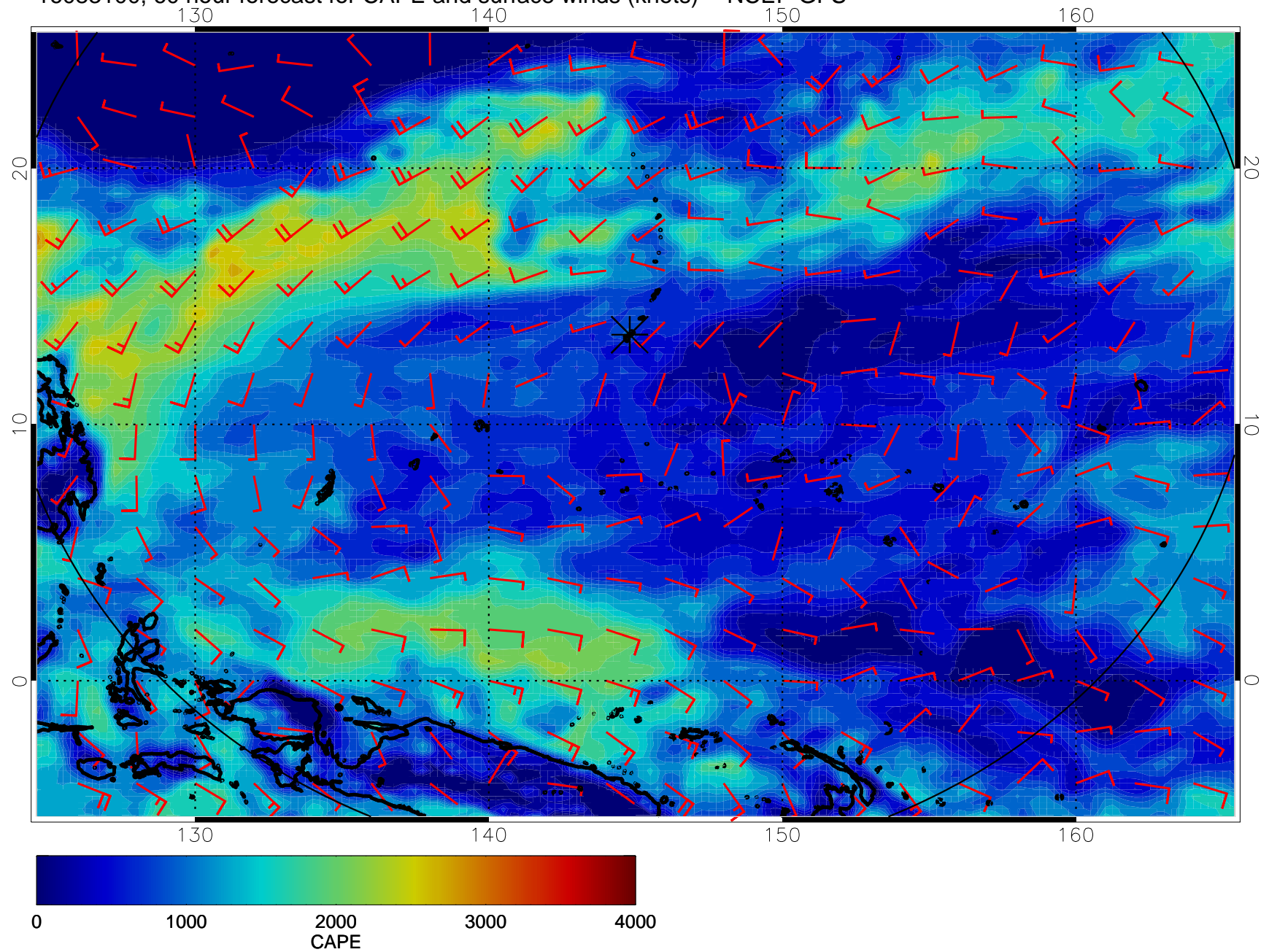
16083100, 60 hour forecast for CAPE and surface winds (knots) -- NCEP GFS
