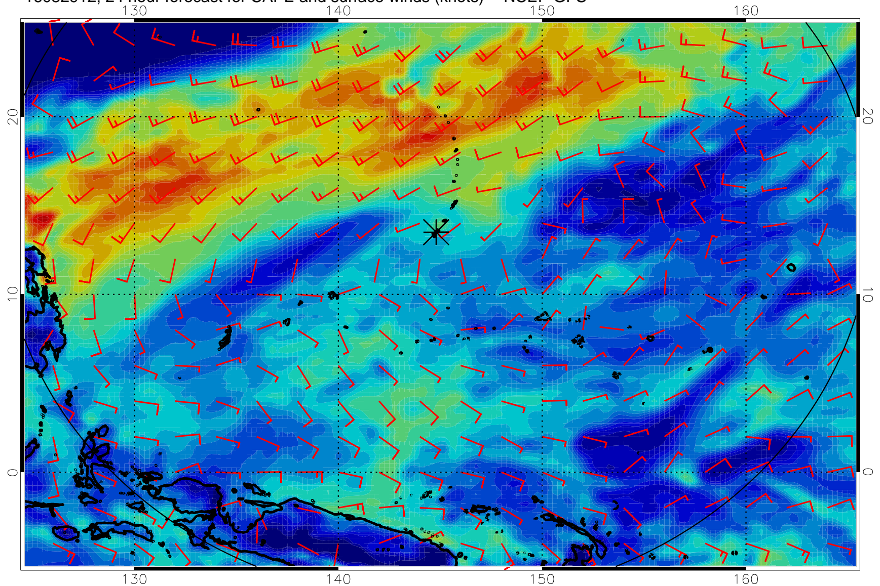
16082912, 24 hour forecast for CAPE and surface winds (knots) -- NCEP GFS
