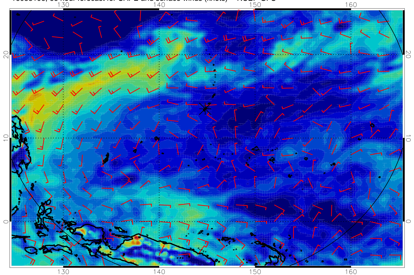
16083106, 66 hour forecast for CAPE and surface winds (knots) -- NCEP GFS
