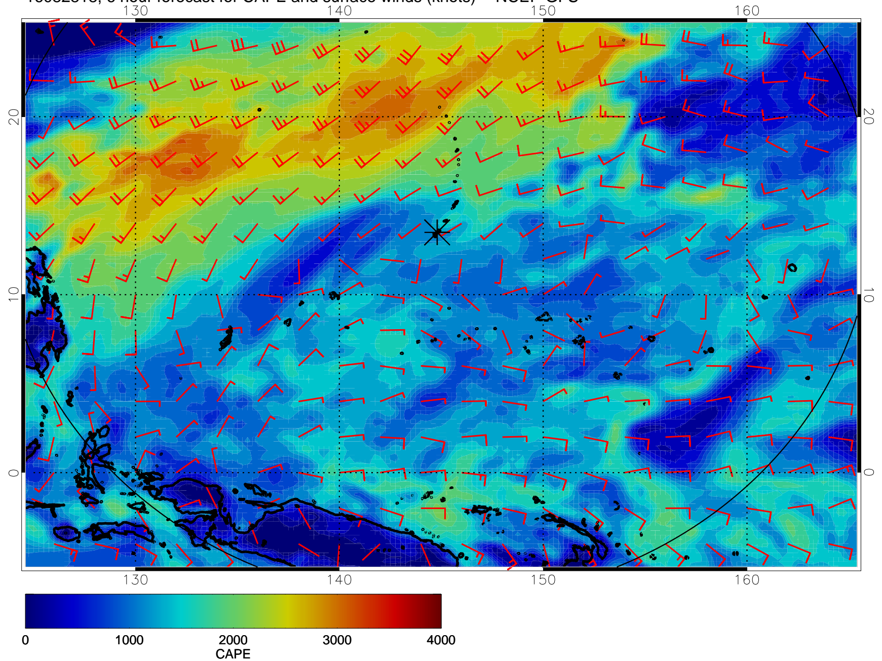
16082818, 6 hour forecast for CAPE and surface winds (knots) -- NCEP GFS
