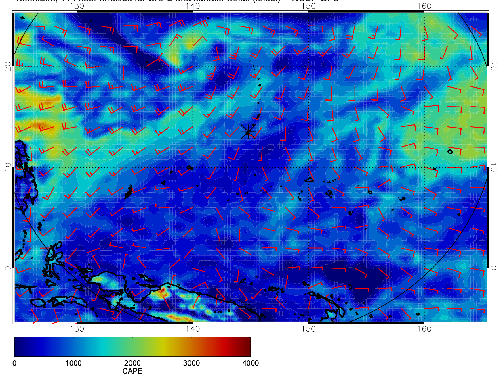
16090206, 114 hour forecast for CAPE and surface winds (knots) -- NCEP GFS
