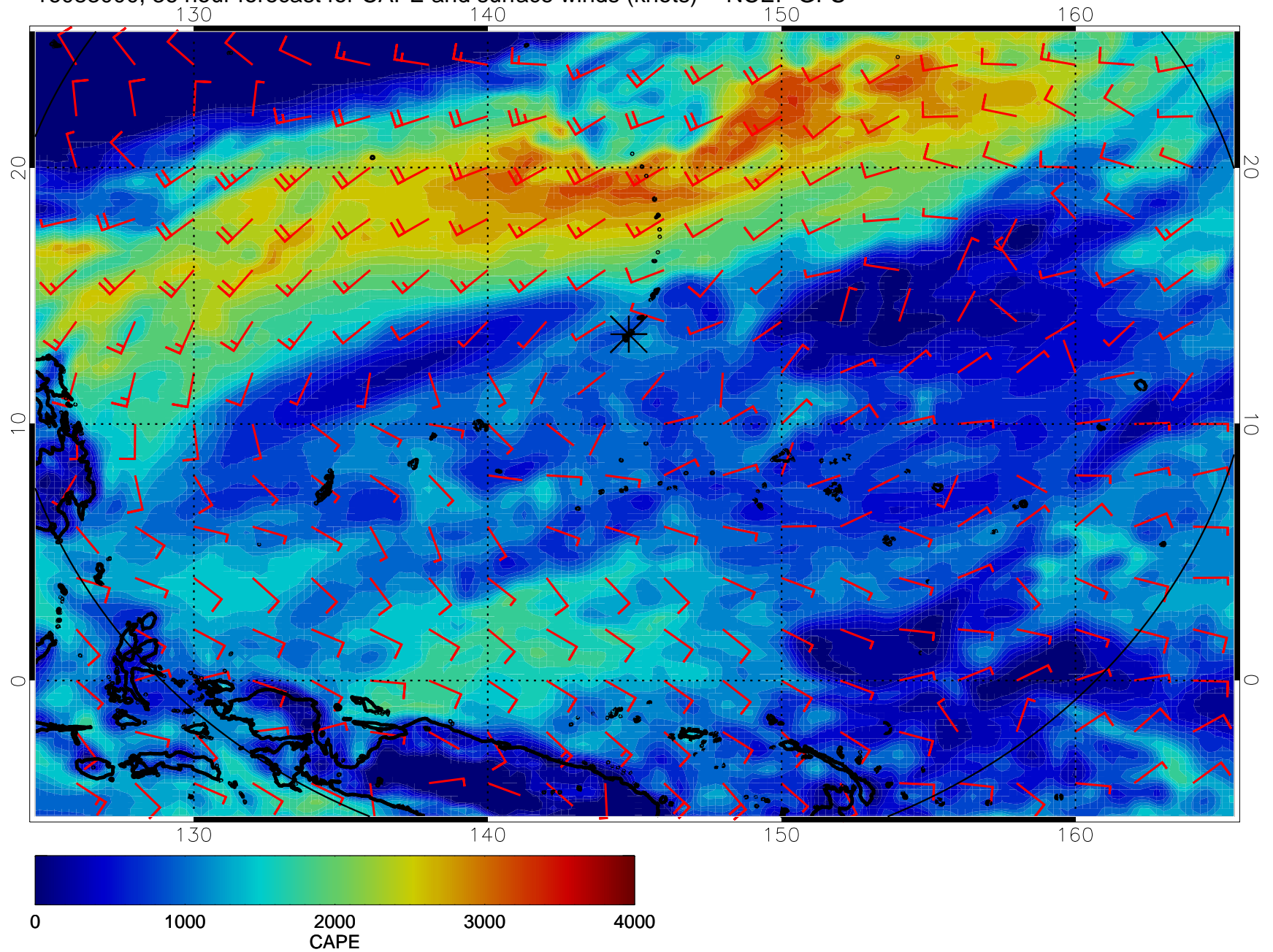
16083000, 36 hour forecast for CAPE and surface winds (knots) -- NCEP GFS
