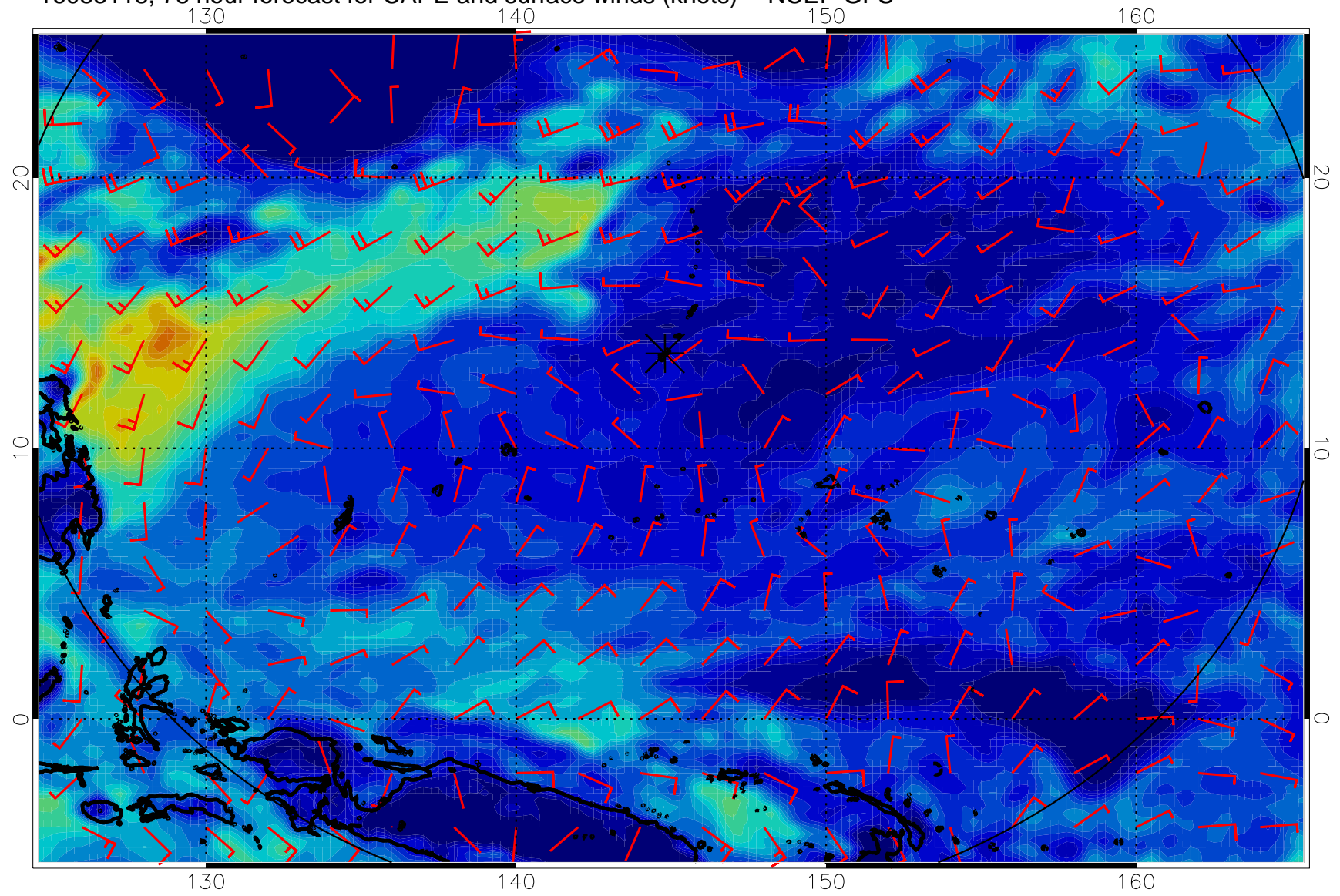
16083118, 78 hour forecast for CAPE and surface winds (knots) -- NCEP GFS
