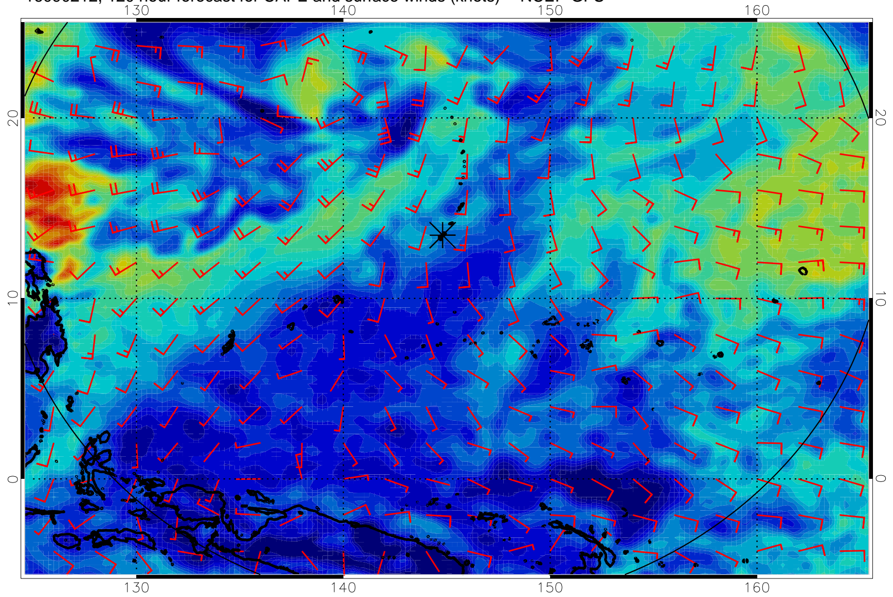
16090212, 120 hour forecast for CAPE and surface winds (knots) -- NCEP GFS
