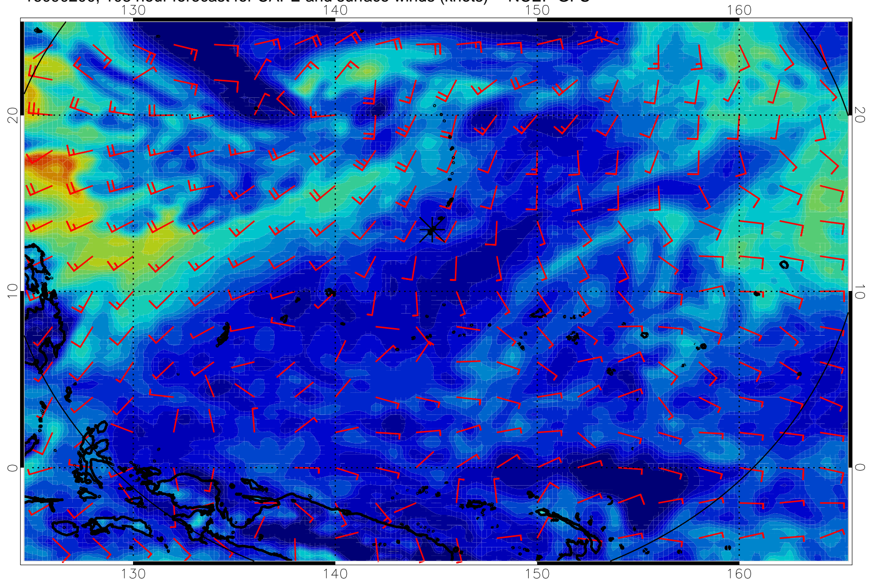
16090200, 108 hour forecast for CAPE and surface winds (knots) -- NCEP GFS
