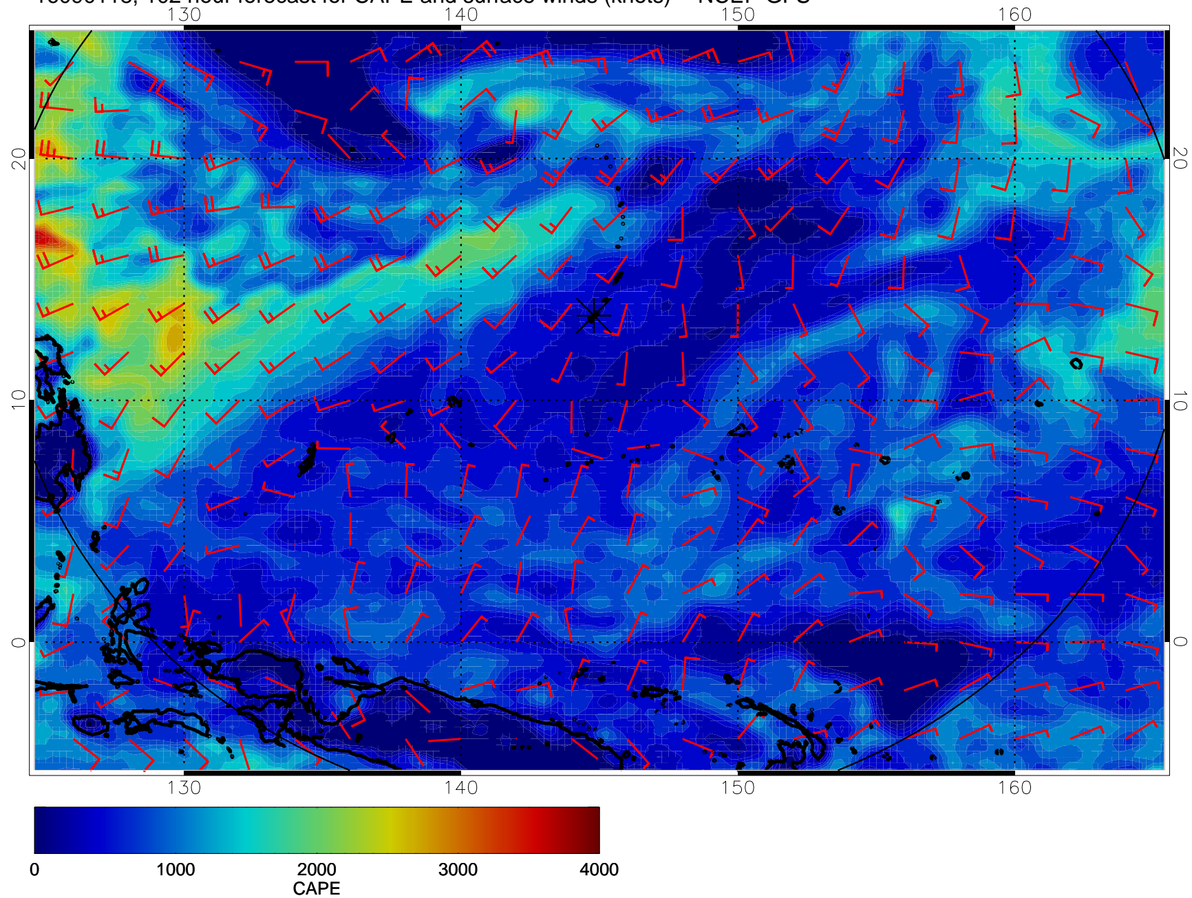
16090118, 102 hour forecast for CAPE and surface winds (knots) -- NCEP GFS
