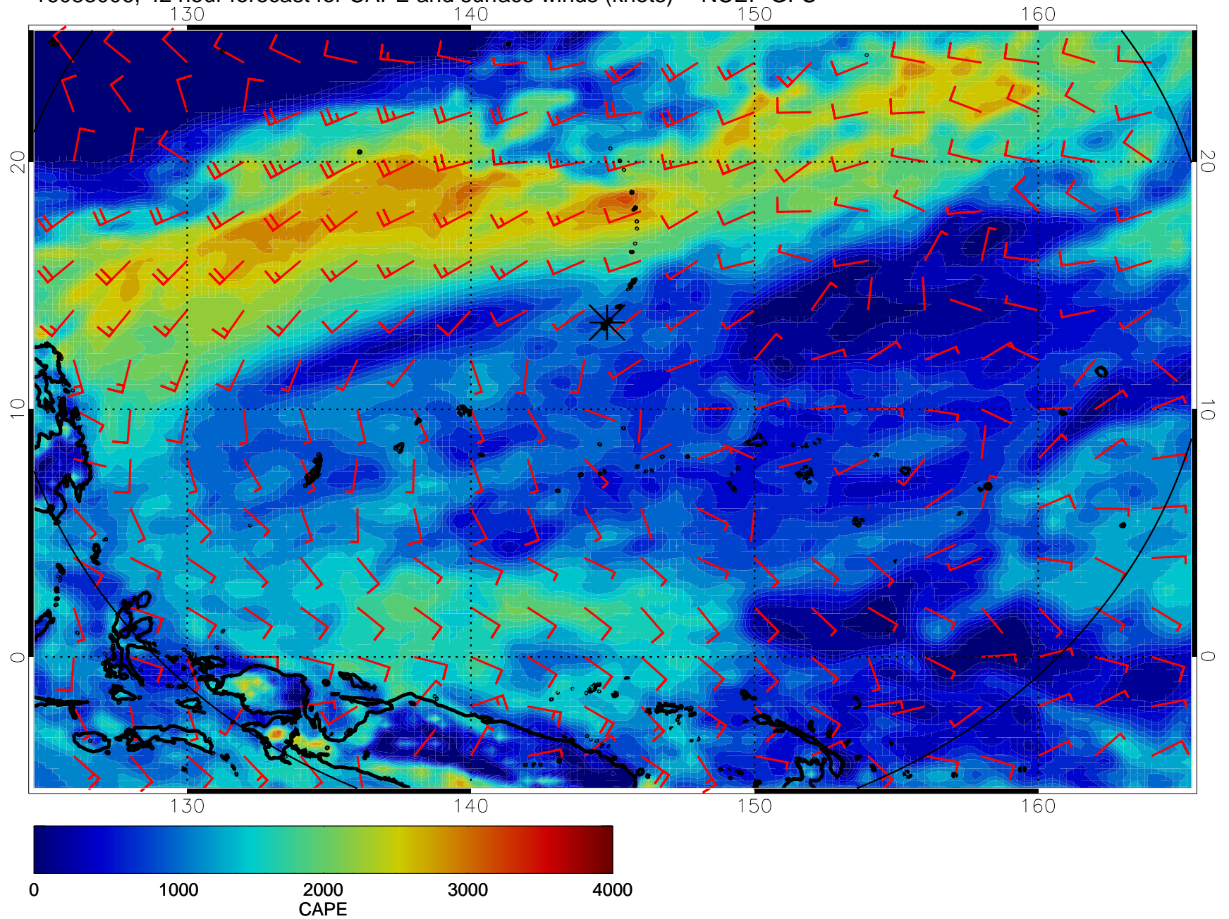
16083006, 42 hour forecast for CAPE and surface winds (knots) -- NCEP GFS
