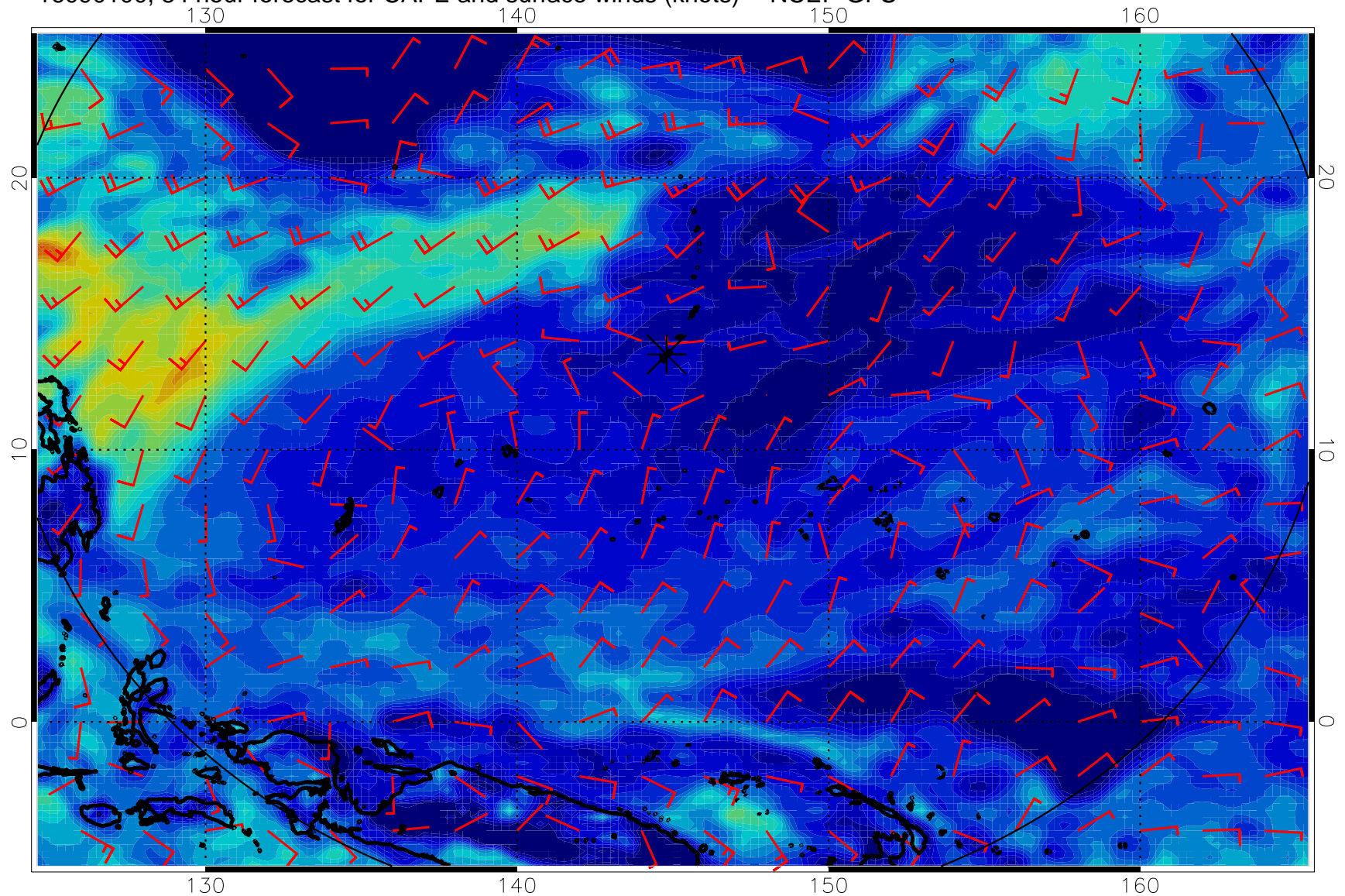
16090100, 84 hour forecast for CAPE and surface winds (knots) -- NCEP GFS
