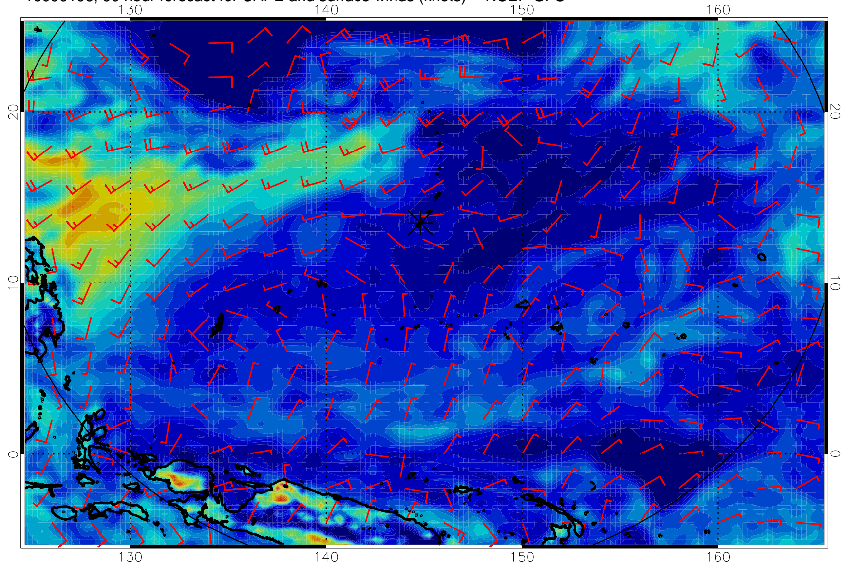
16090106, 90 hour forecast for CAPE and surface winds (knots) -- NCEP GFS
