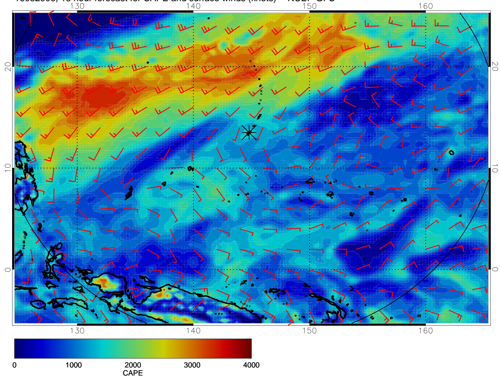
16082906, 18 hour forecast for CAPE and surface winds (knots) -- NCEP GFS
