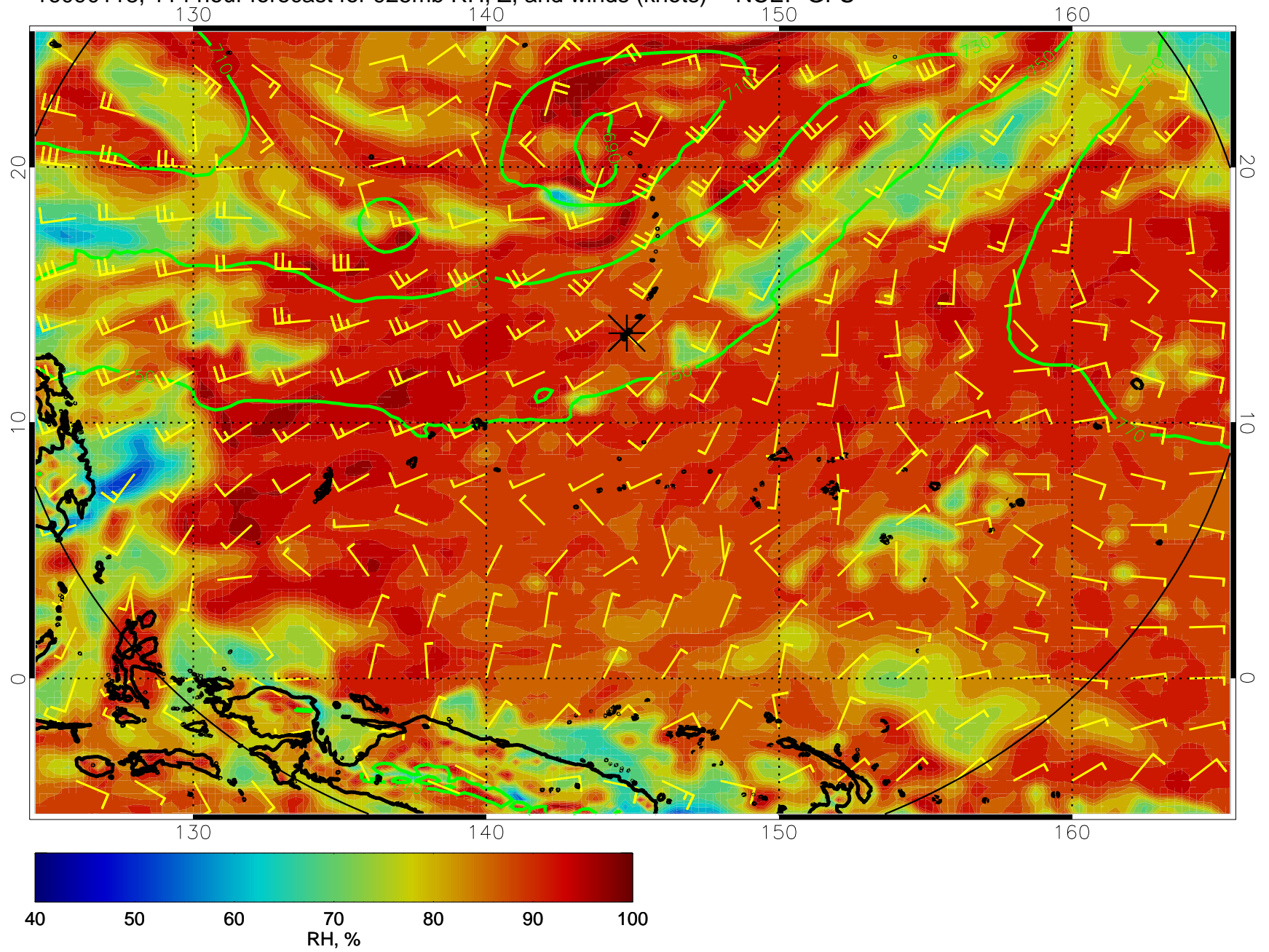
16090118, 114 hour forecast for 925mb RH, Z, and winds (knots) -- NCEP GFS
