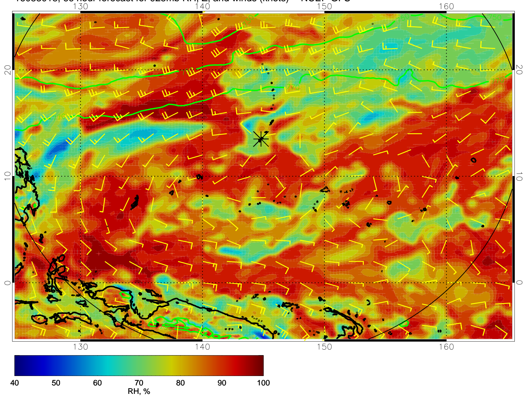
16083018, 66 hour forecast for 925mb RH, Z, and winds (knots) -- NCEP GFS
