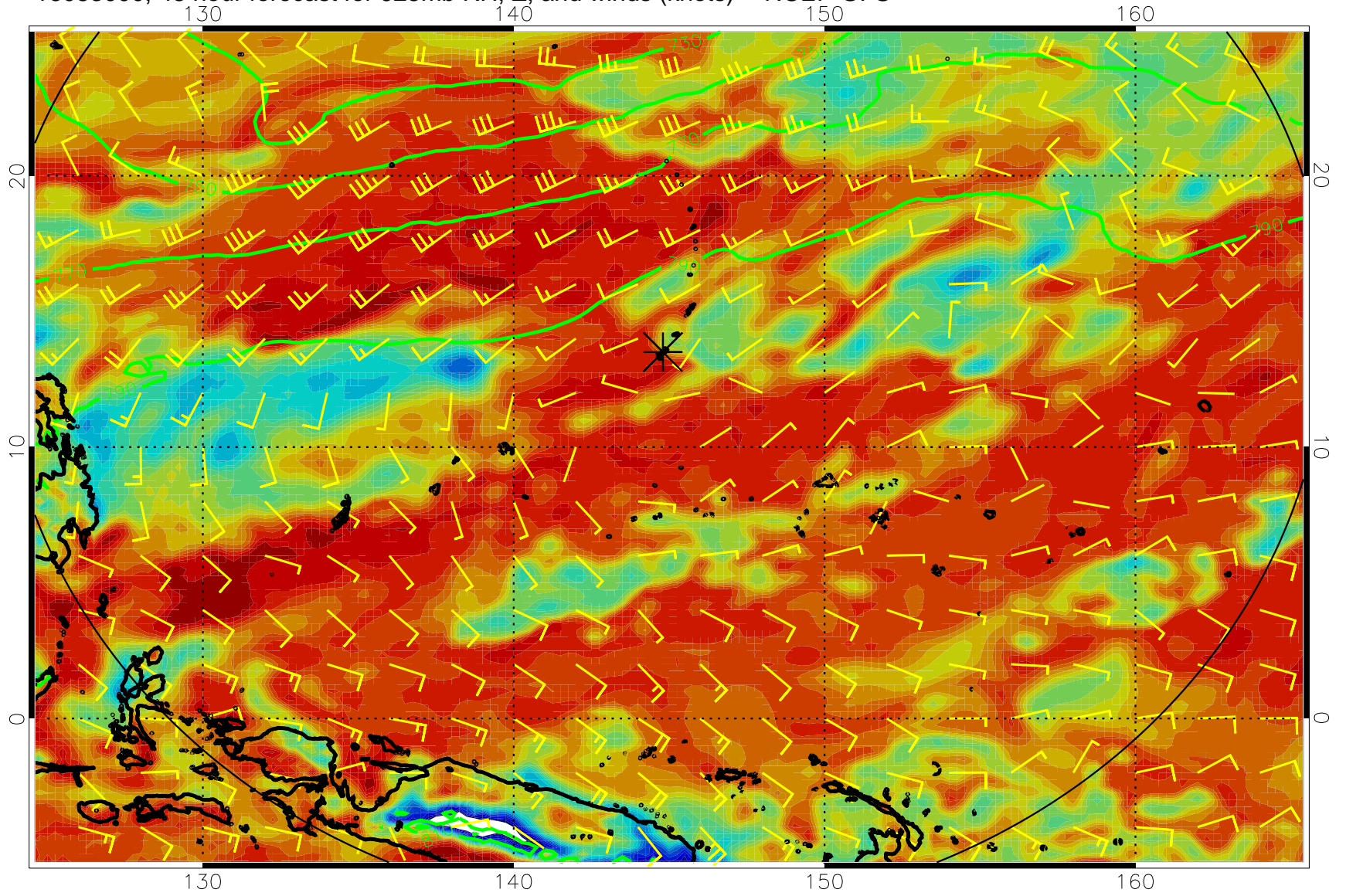
16083000, 48 hour forecast for 925mb RH, Z, and winds (knots) -- NCEP GFS
