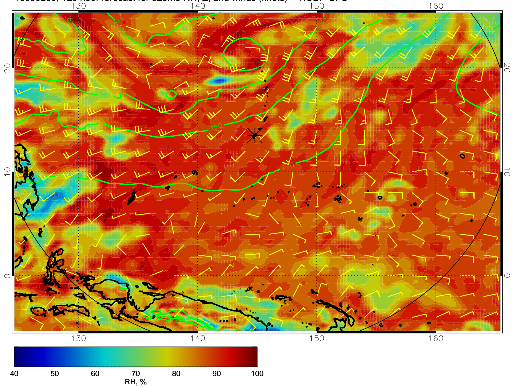
16090200, 120 hour forecast for 925mb RH, Z, and winds (knots) -- NCEP GFS
