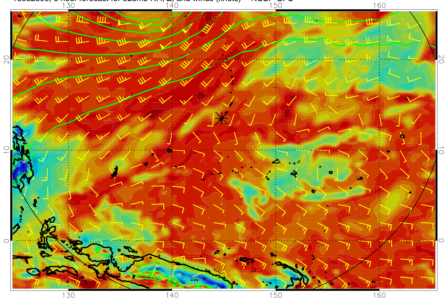
16082806, 6 hour forecast for 925mb RH, Z, and winds (knots) -- NCEP GFS
