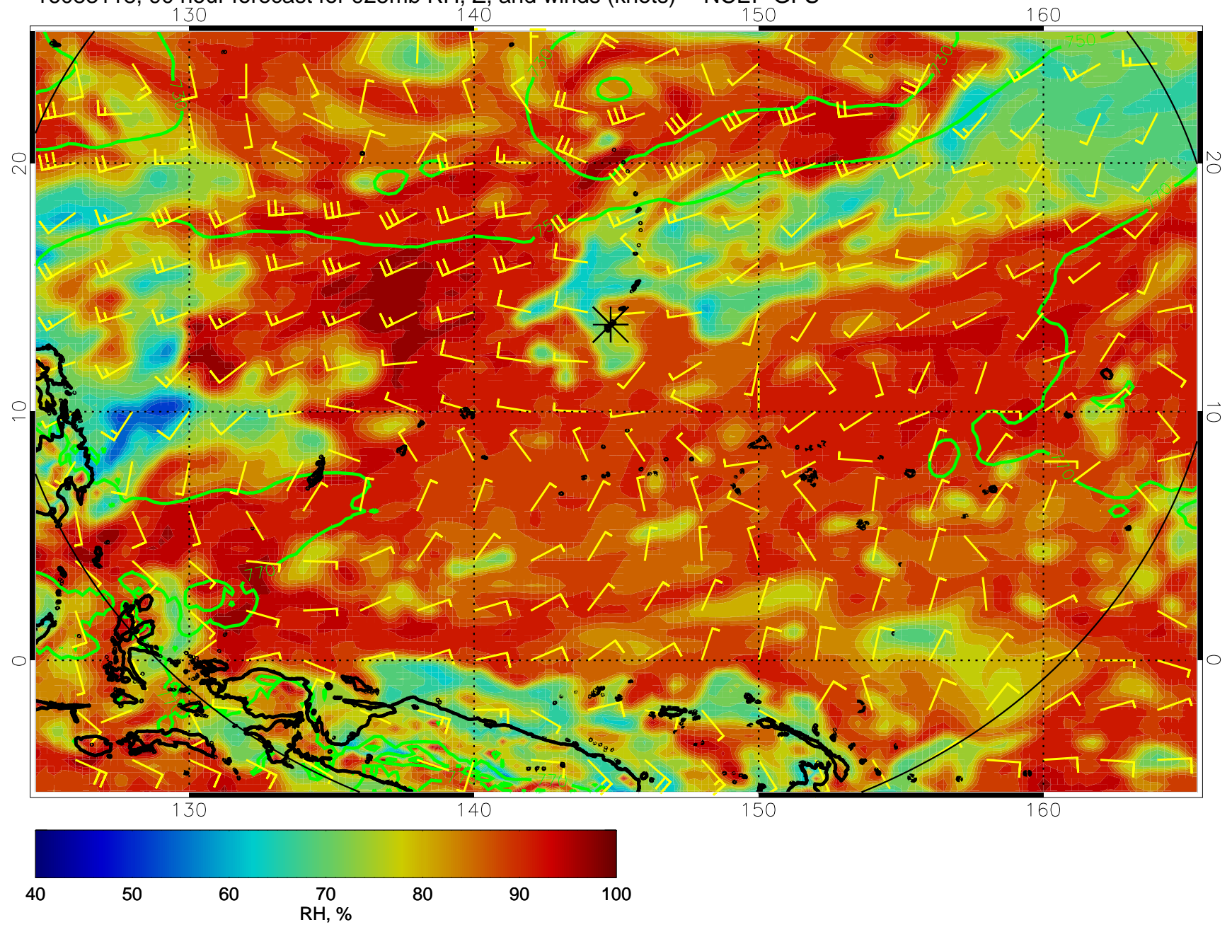
16083118, 90 hour forecast for 925mb RH, Z, and winds (knots) -- NCEP GFS
