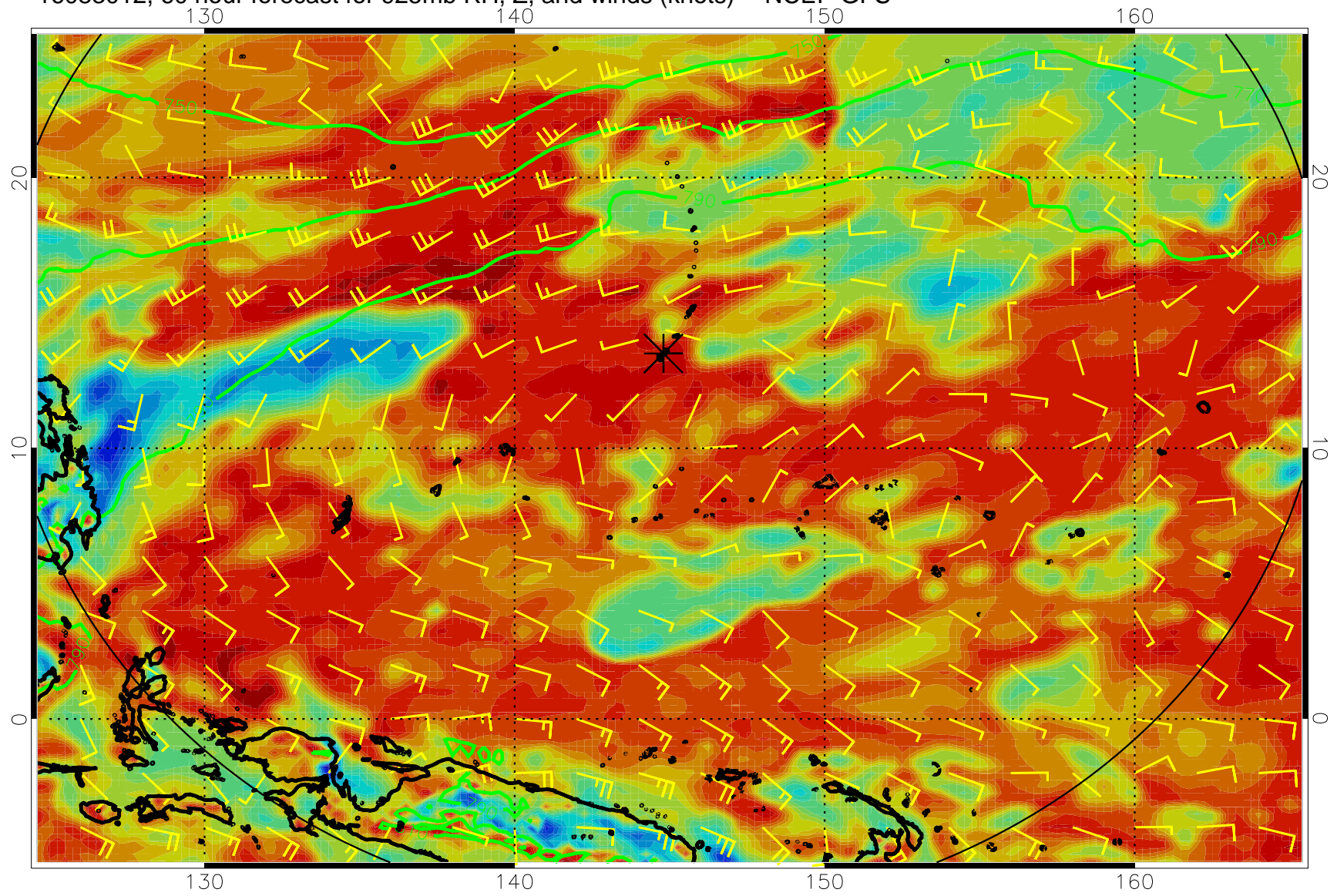
16083012, 60 hour forecast for 925mb RH, Z, and winds (knots) -- NCEP GFS
