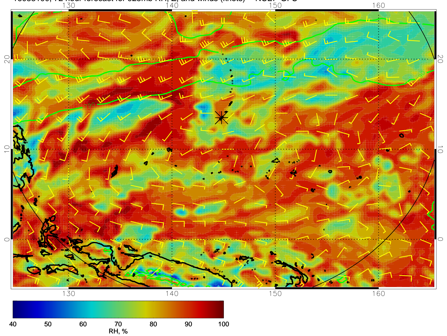
16083100, 72 hour forecast for 925mb RH, Z, and winds (knots) -- NCEP GFS
