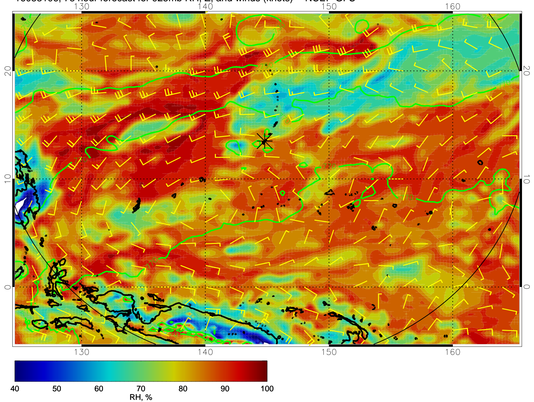
16083106, 78 hour forecast for 925mb RH, Z, and winds (knots) -- NCEP GFS
