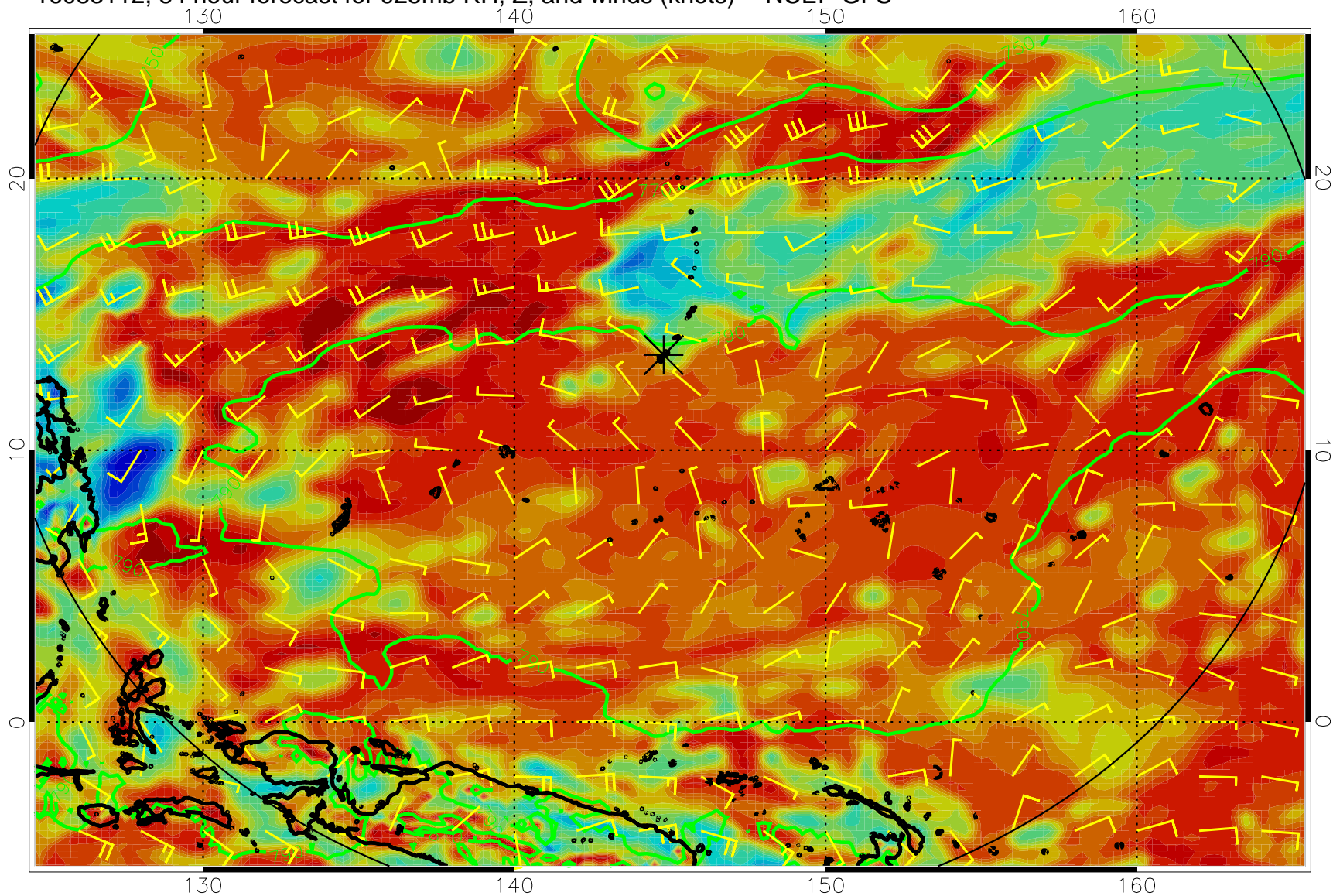
16083112, 84 hour forecast for 925mb RH, Z, and winds (knots) -- NCEP GFS
