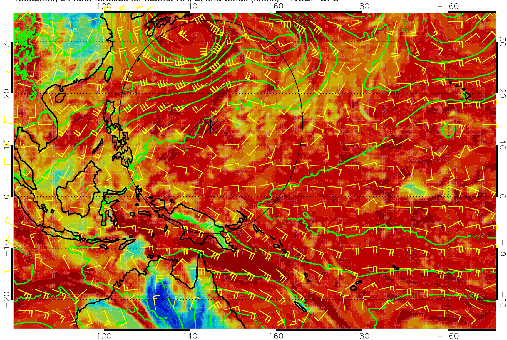
16082900, 24 hour forecast for 925mb RH, Z, and winds (knots) -- NCEP GFS
