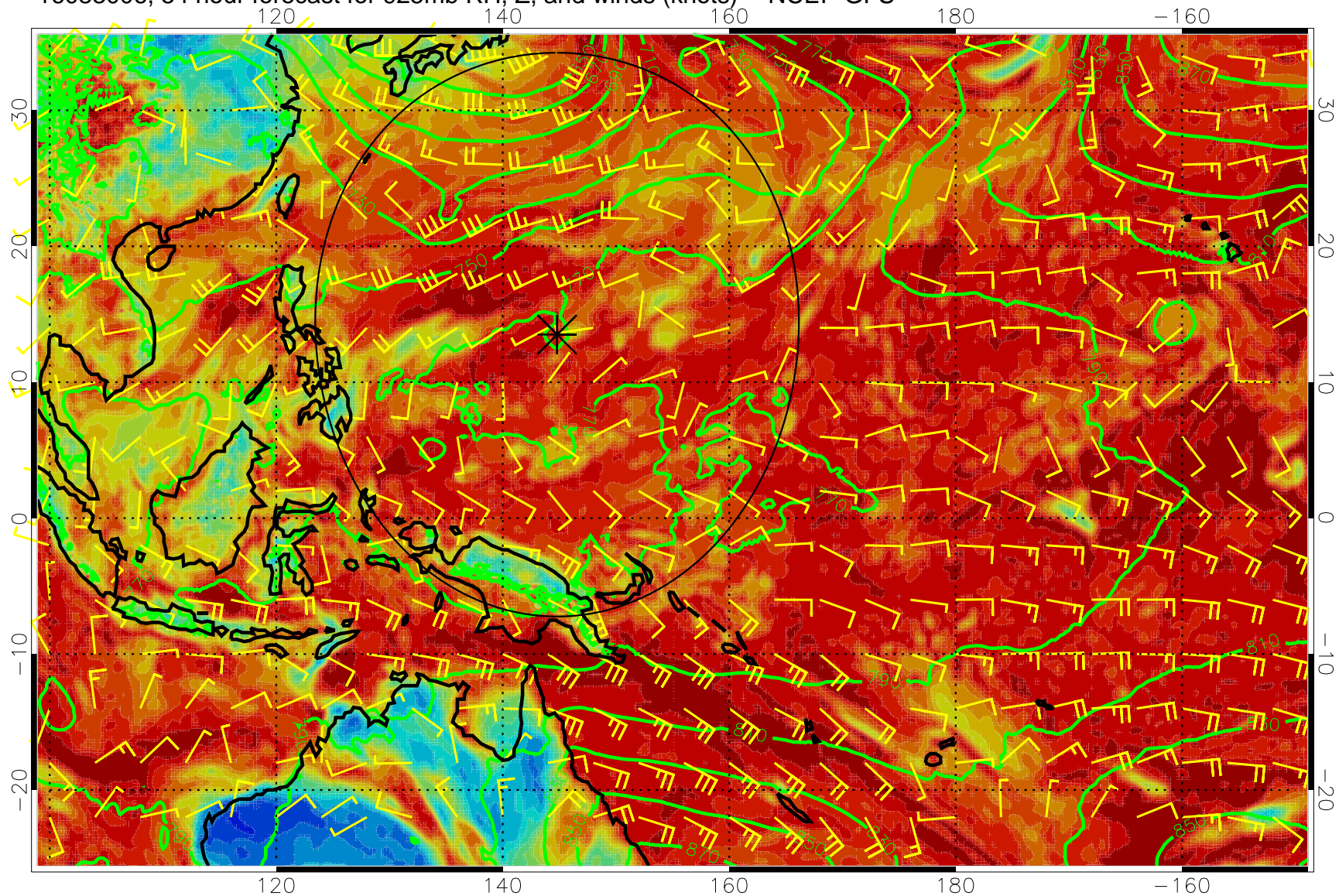
16083006, 54 hour forecast for 925mb RH, Z, and winds (knots) -- NCEP GFS
