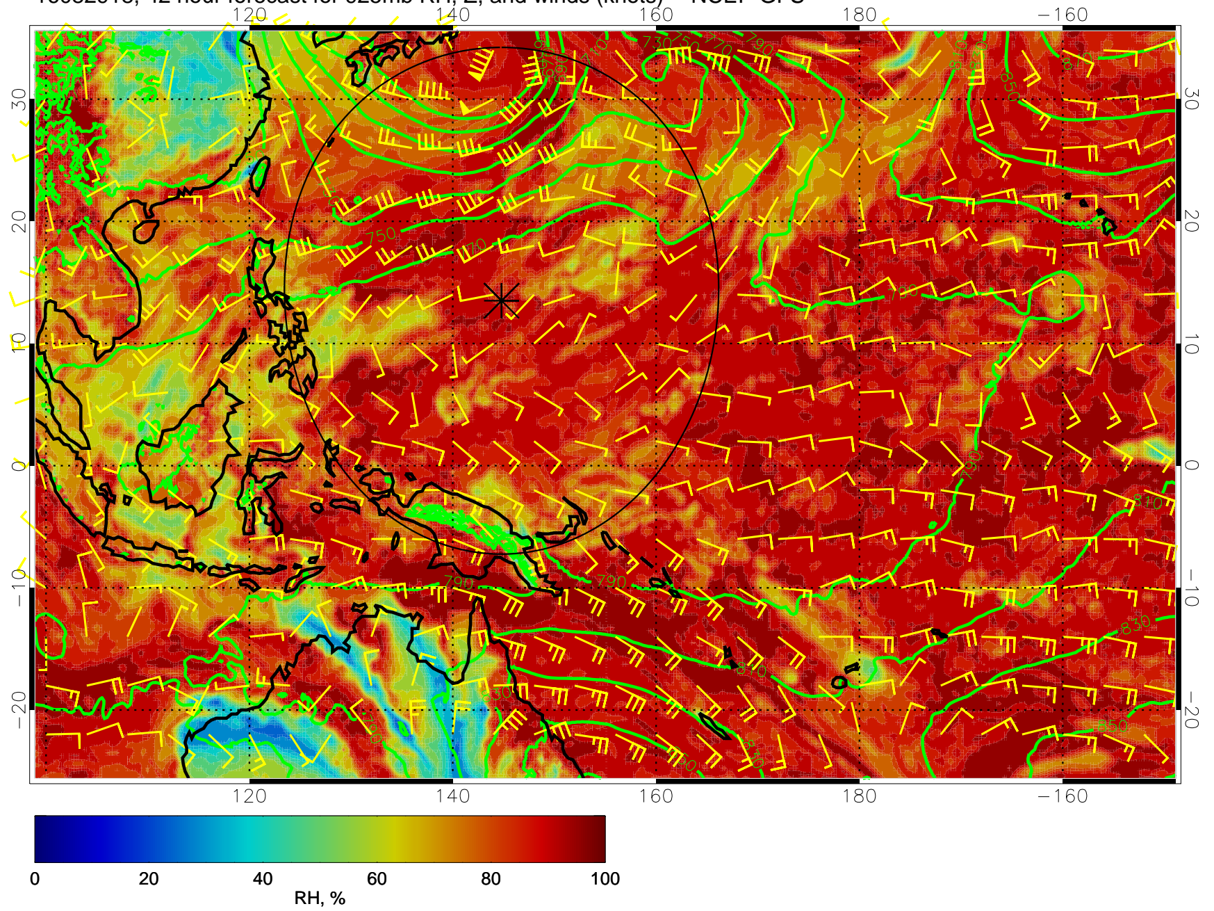
16082918, 42 hour forecast for 925mb RH, Z, and winds (knots) -- NCEP GFS
