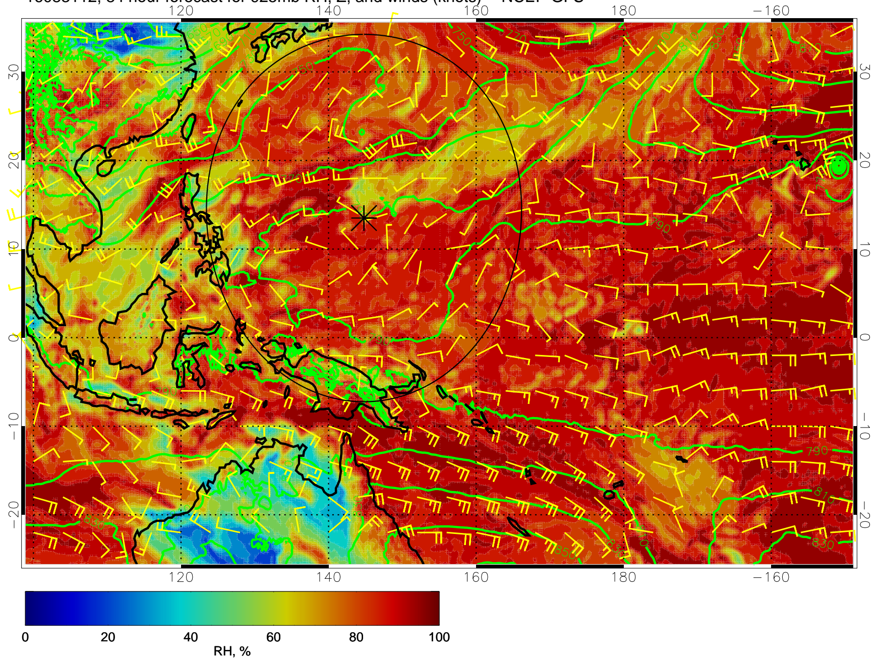
16083112, 84 hour forecast for 925mb RH, Z, and winds (knots) -- NCEP GFS
