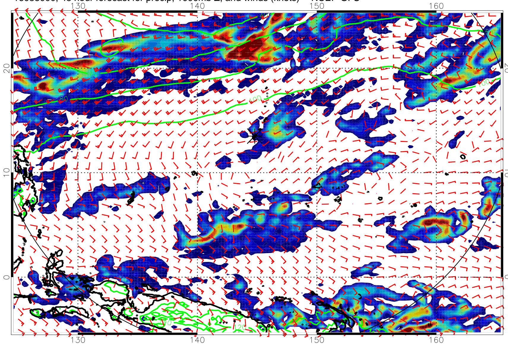
16083000, 48 hour forecast for precip, 1000mb Z, and winds (knots) -- NCEP GFS
