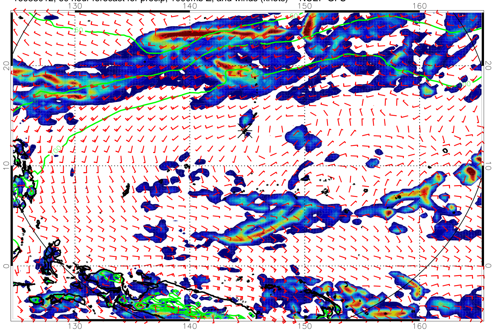
16083012, 60 hour forecast for precip, 1000mb Z, and winds (knots) -- NCEP GFS
