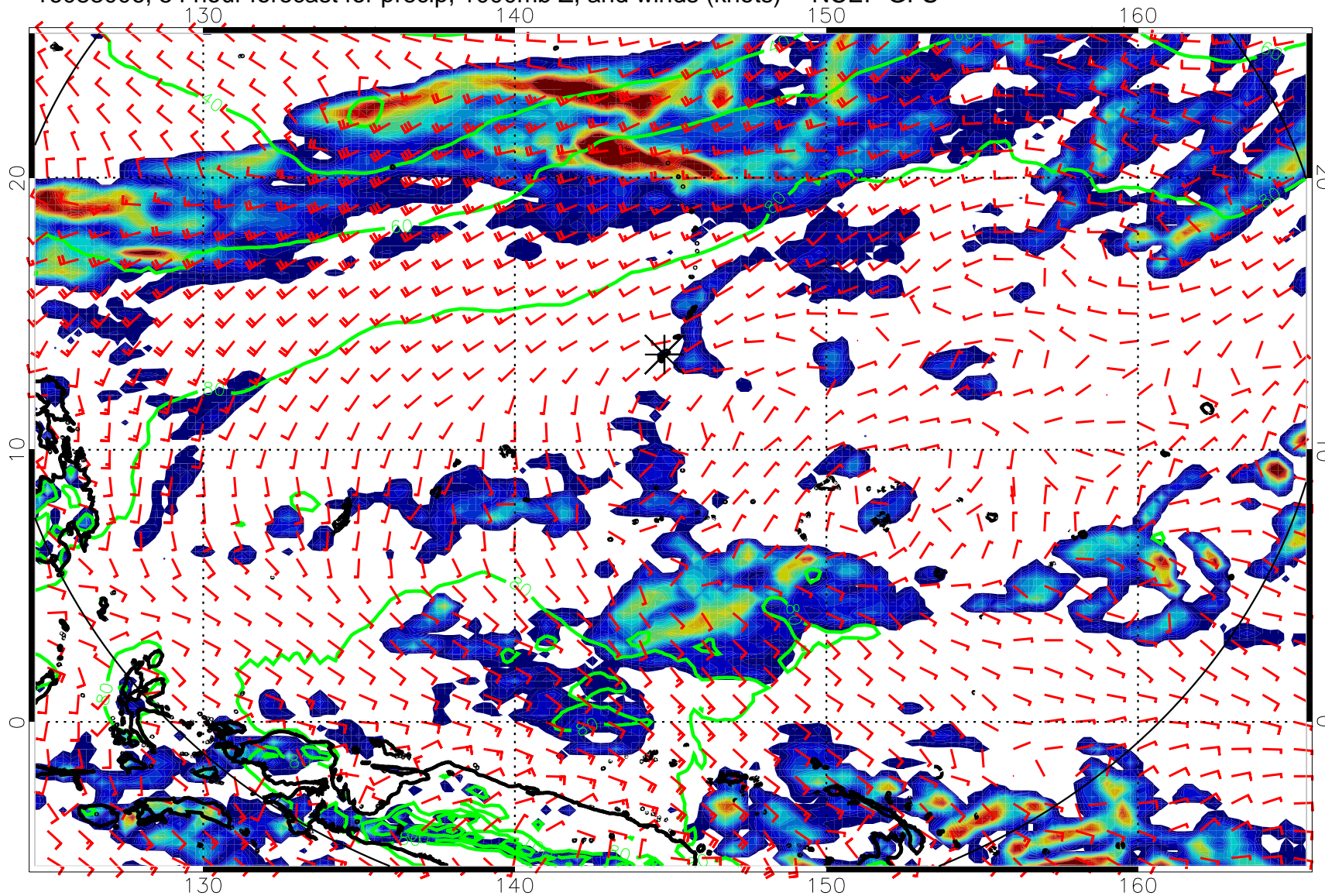
16083006, 54 hour forecast for precip, 1000mb Z, and winds (knots) -- NCEP GFS
