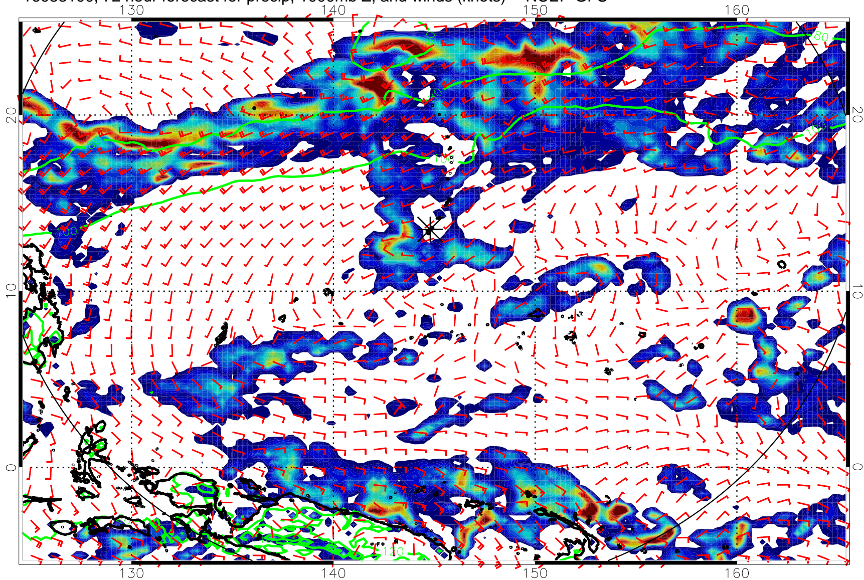
16083100, 72 hour forecast for precip, 1000mb Z, and winds (knots) -- NCEP GFS
