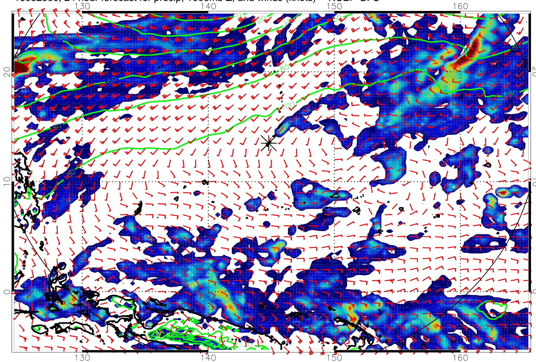
16082900, 24 hour forecast for precip, 1000mb Z, and winds (knots) -- NCEP GFS
