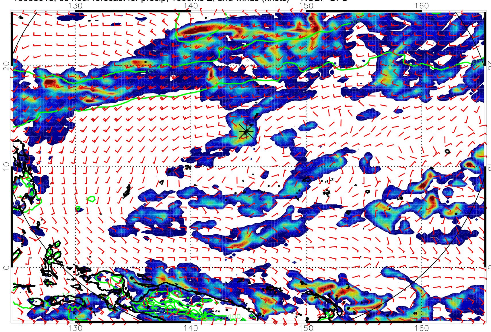
16083018, 66 hour forecast for precip, 1000mb Z, and winds (knots) -- NCEP GFS
