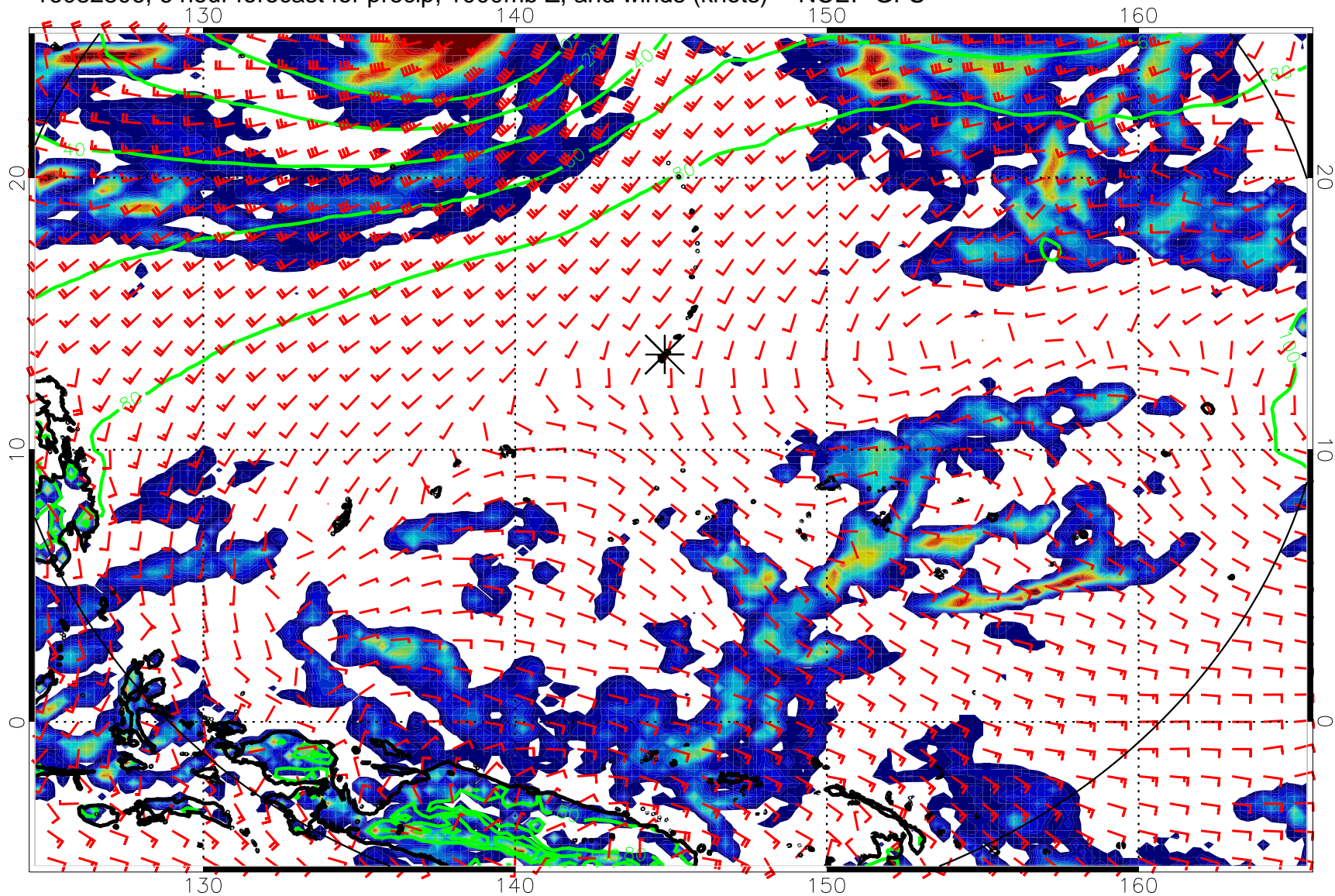
16082806, 6 hour forecast for precip, 1000mb Z, and winds (knots) -- NCEP GFS
