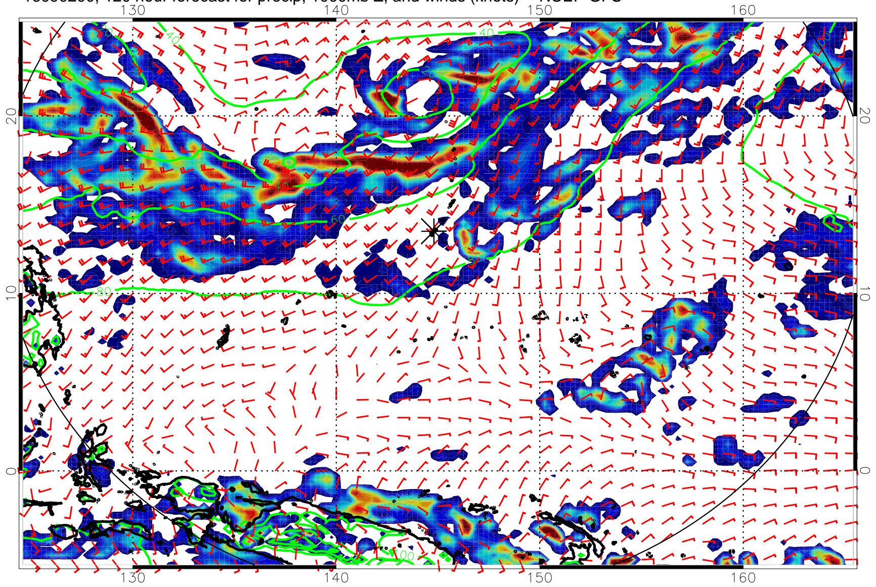
16090200, 120 hour forecast for precip, 1000mb Z, and winds (knots) -- NCEP GFS
