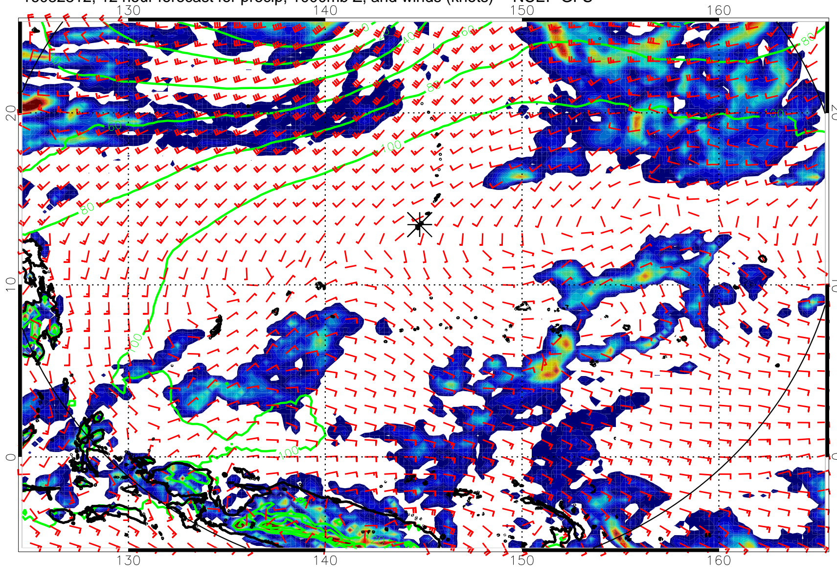
16082812, 12 hour forecast for precip, 1000mb Z, and winds (knots) -- NCEP GFS
