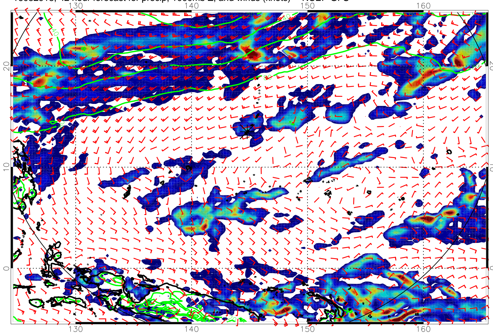
16082918, 42 hour forecast for precip, 1000mb Z, and winds (knots) -- NCEP GFS
