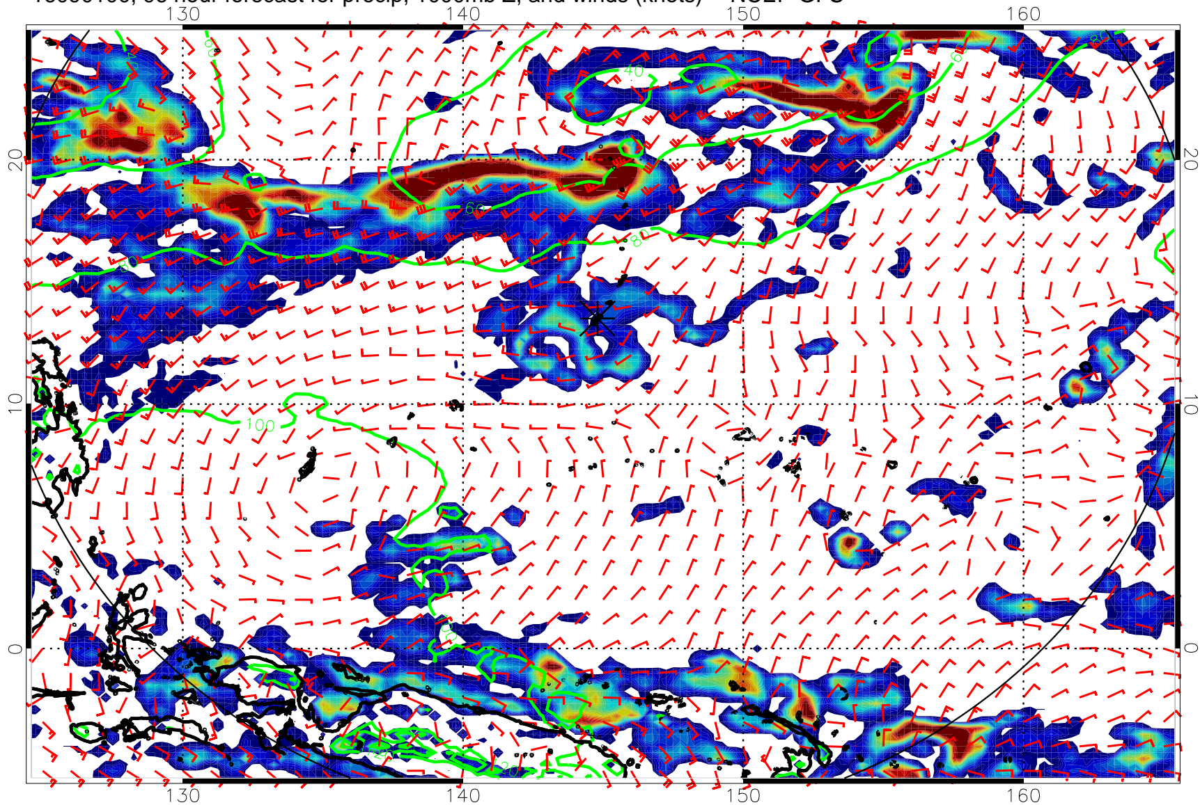
16090100, 96 hour forecast for precip, 1000mb Z, and winds (knots) -- NCEP GFS
