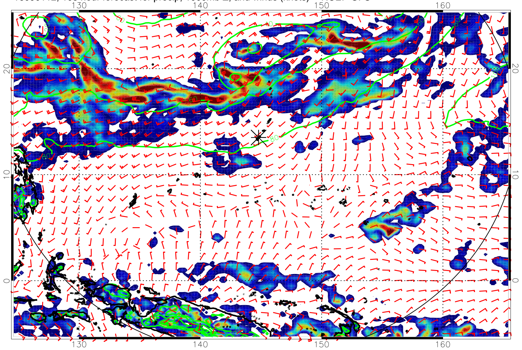
16090112, 108 hour forecast for precip, 1000mb Z, and winds (knots) -- NCEP GFS
