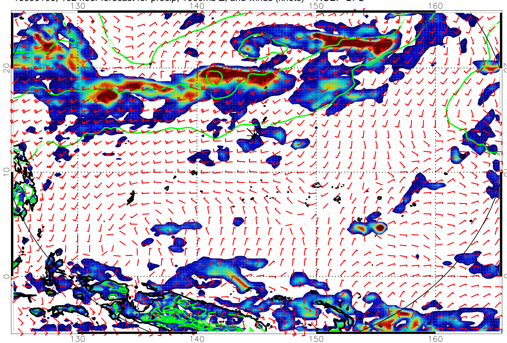
16090106, 102 hour forecast for precip, 1000mb Z, and winds (knots) -- NCEP GFS
