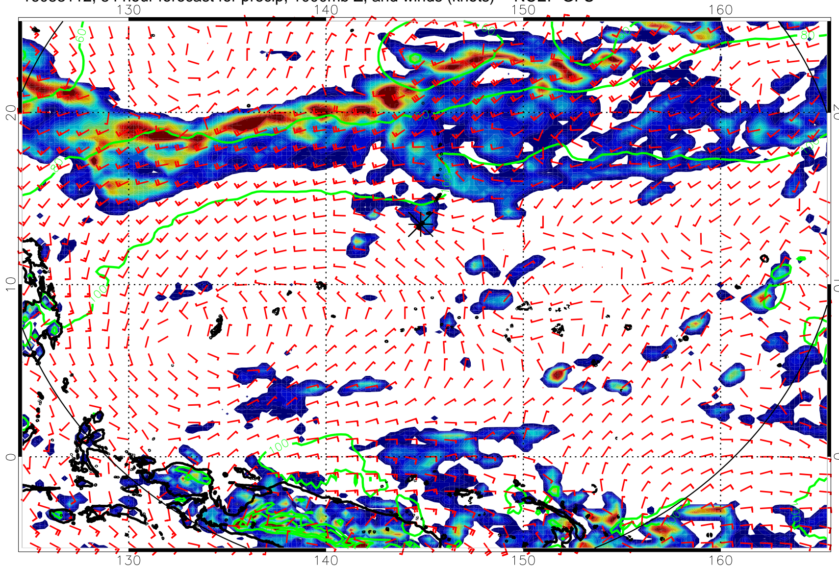
16083112, 84 hour forecast for precip, 1000mb Z, and winds (knots) -- NCEP GFS
