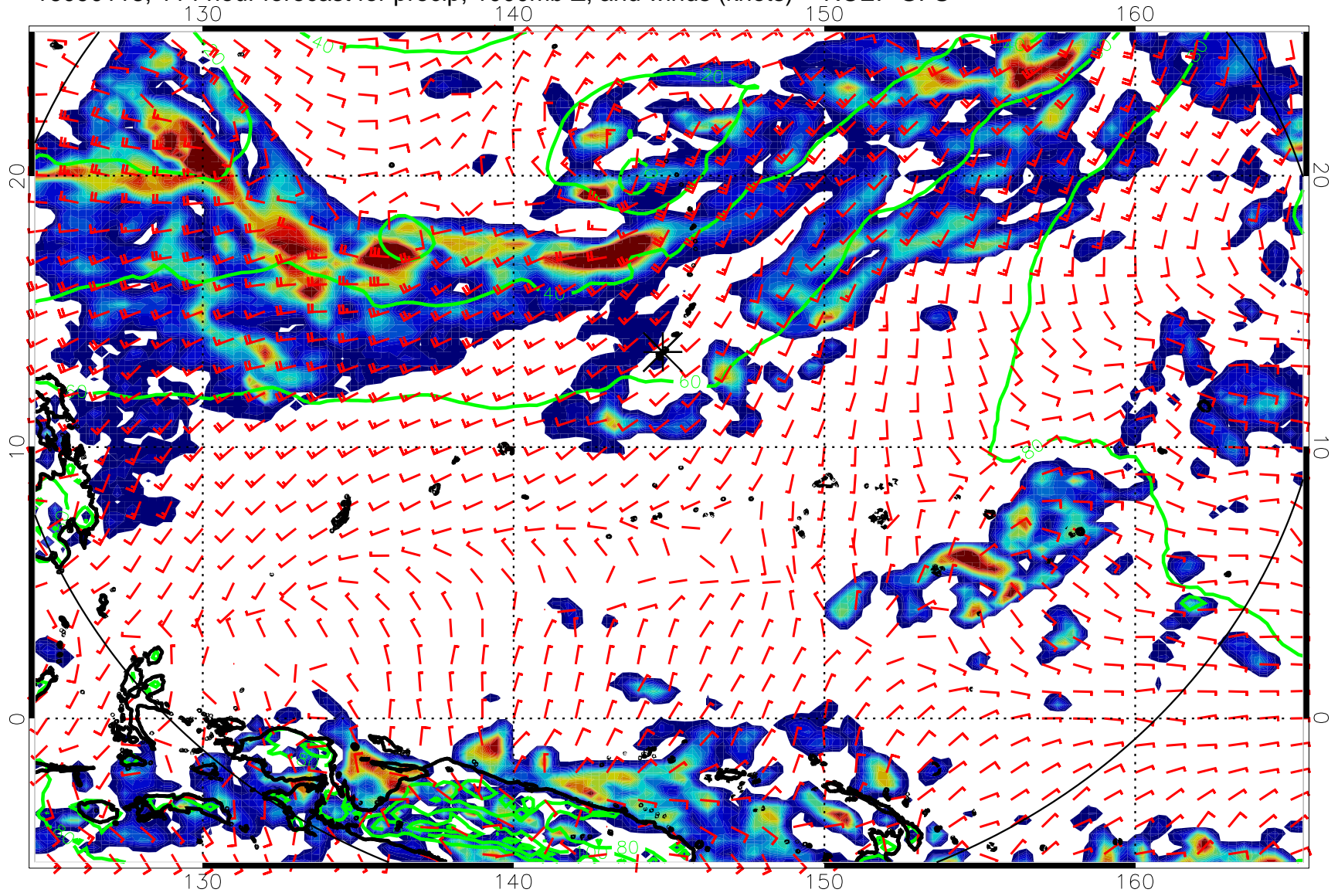
16090118, 114 hour forecast for precip, 1000mb Z, and winds (knots) -- NCEP GFS
