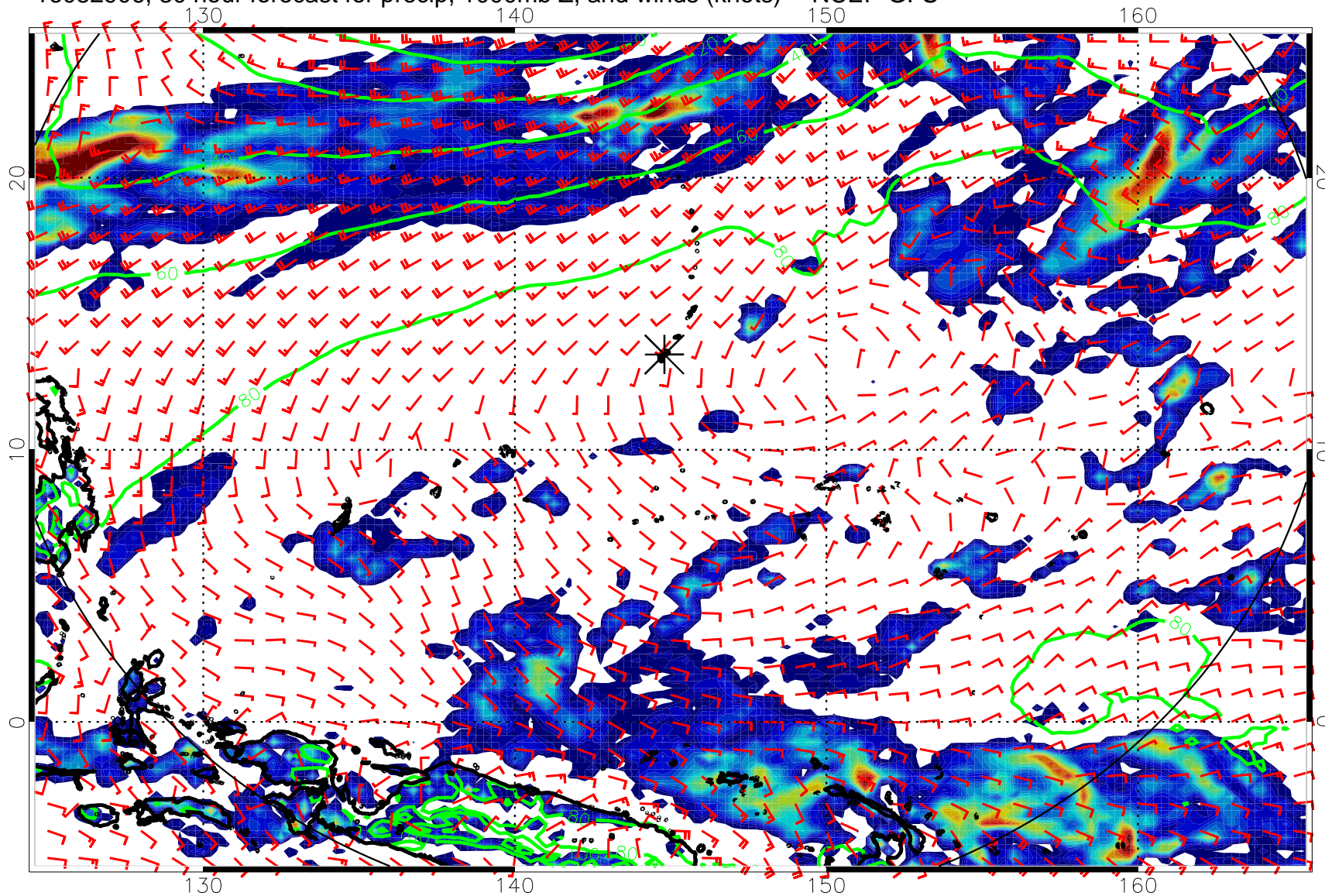
16082906, 30 hour forecast for precip, 1000mb Z, and winds (knots) -- NCEP GFS
