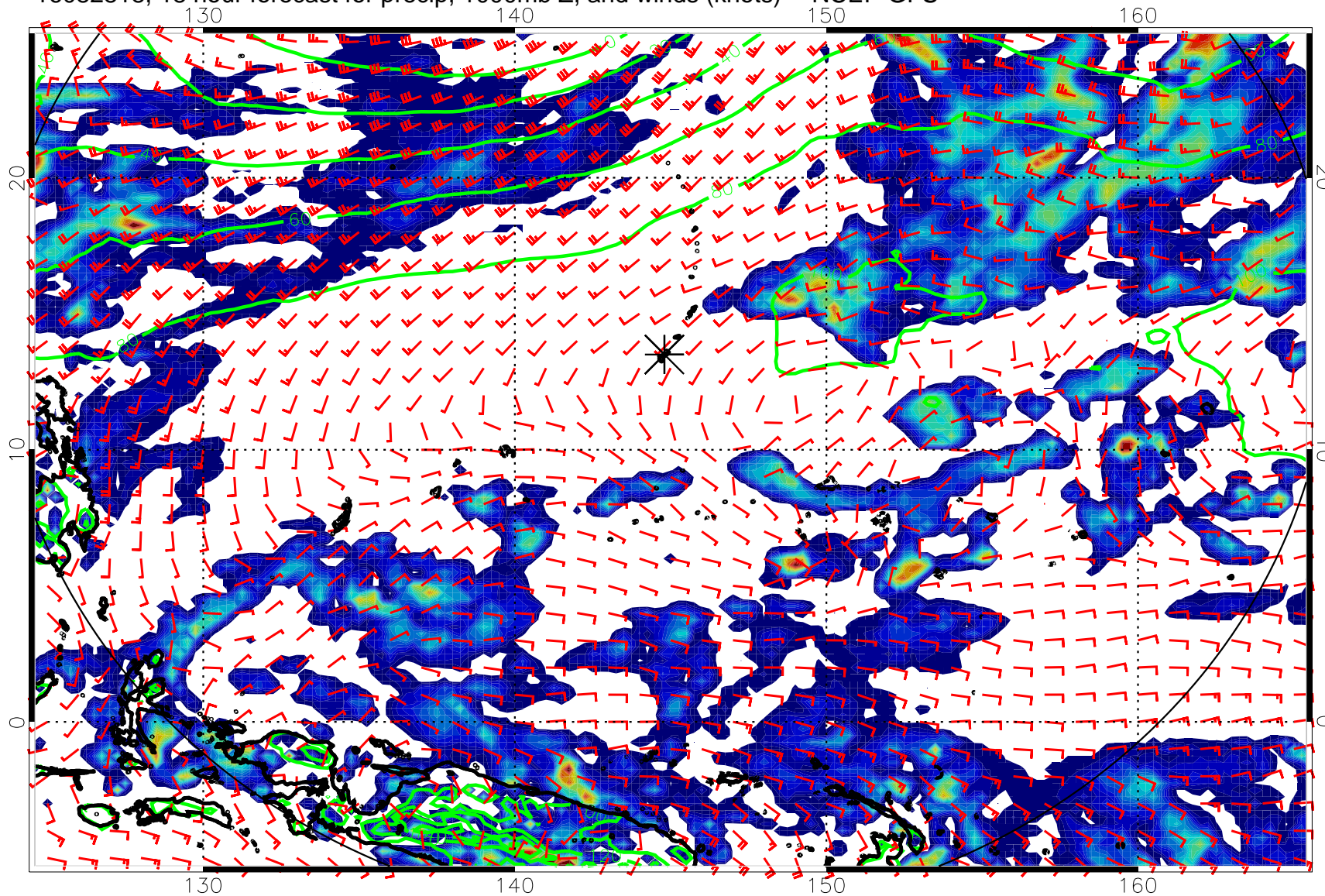
16082818, 18 hour forecast for precip, 1000mb Z, and winds (knots) -- NCEP GFS
