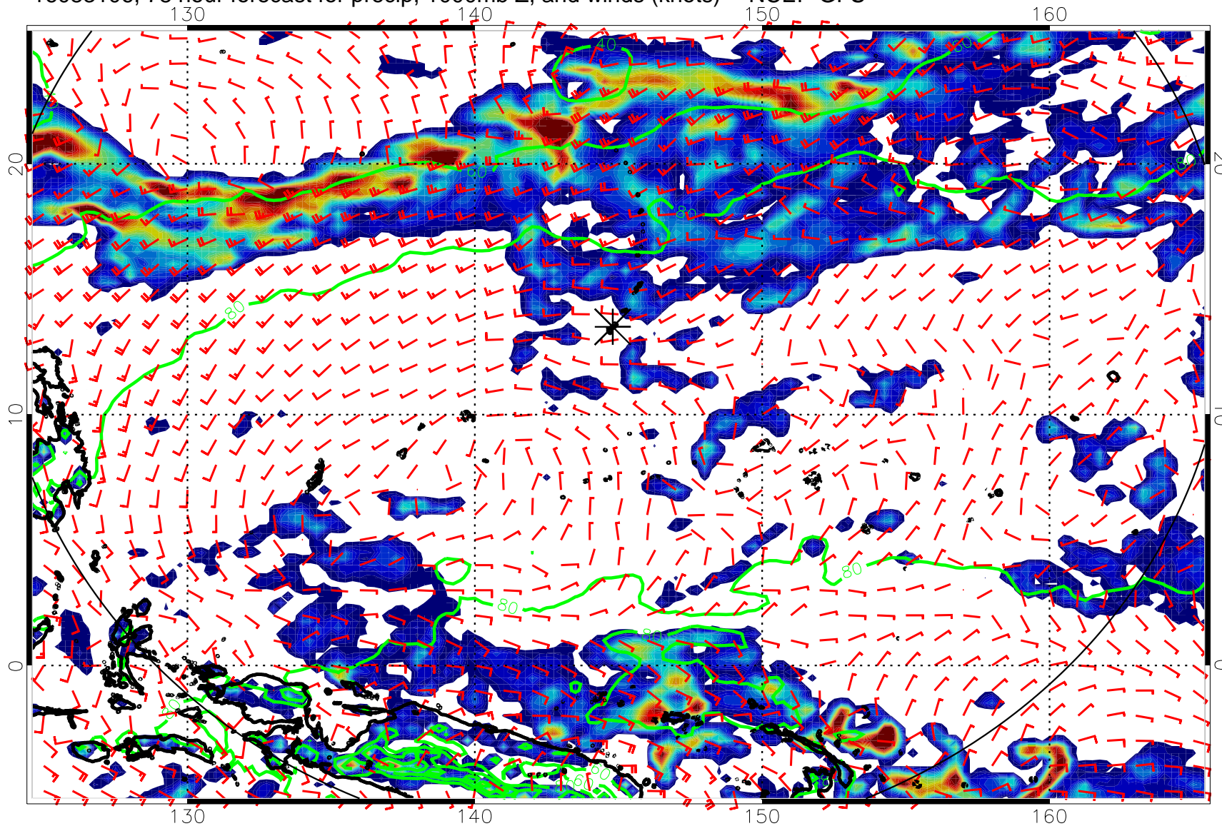
16083106, 78 hour forecast for precip, 1000mb Z, and winds (knots) -- NCEP GFS
