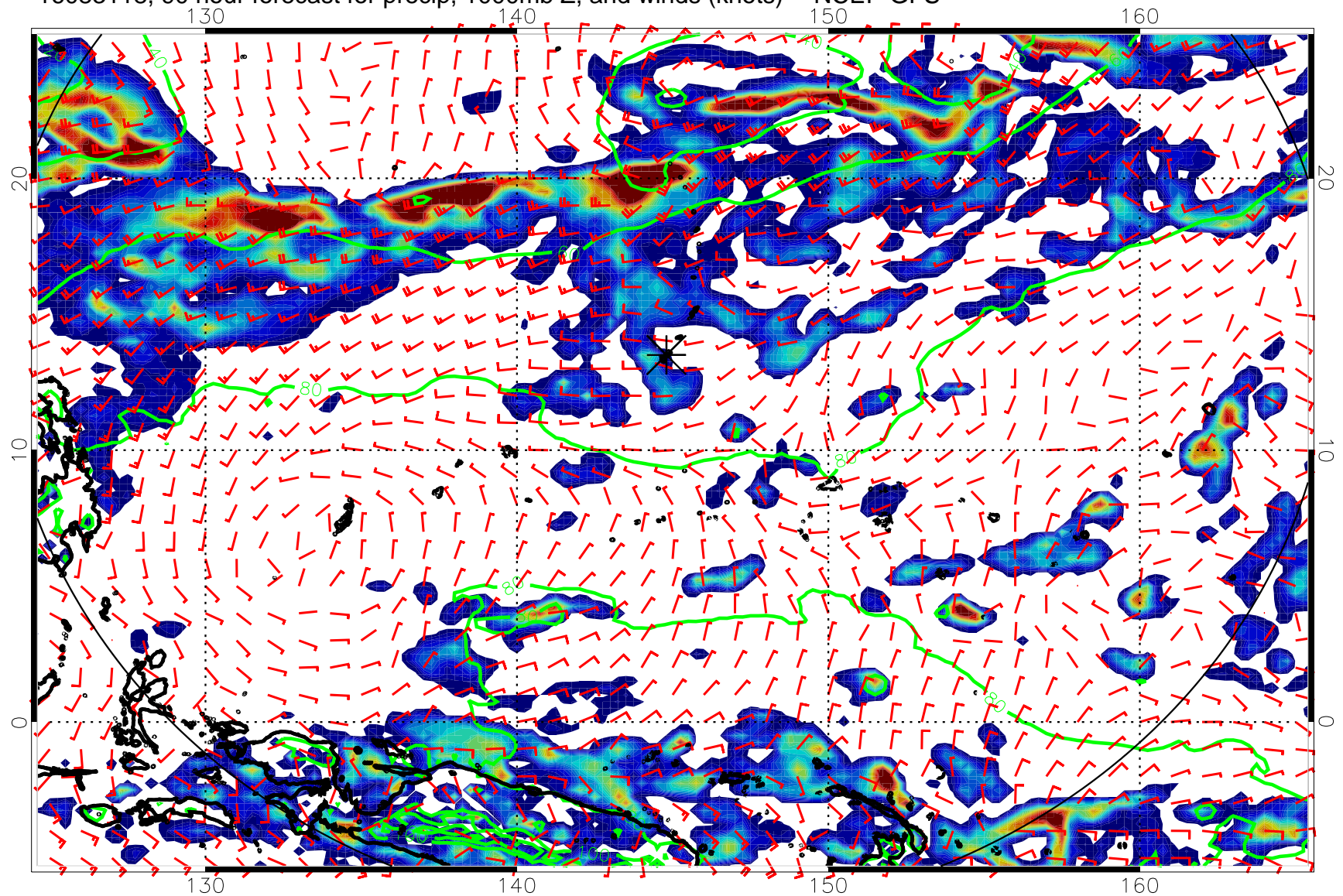
16083118, 90 hour forecast for precip, 1000mb Z, and winds (knots) -- NCEP GFS
