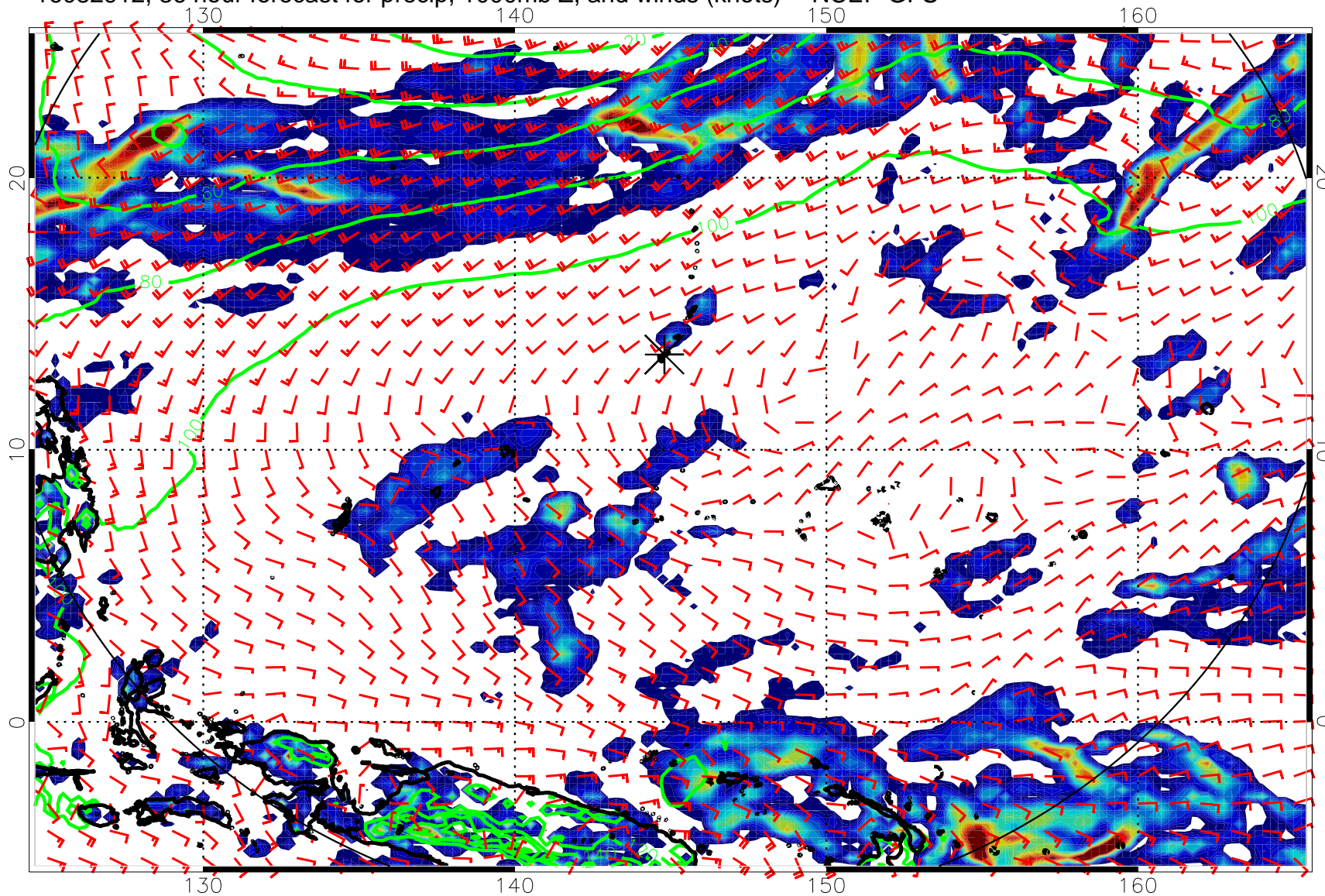
16082912, 36 hour forecast for precip, 1000mb Z, and winds (knots) -- NCEP GFS
