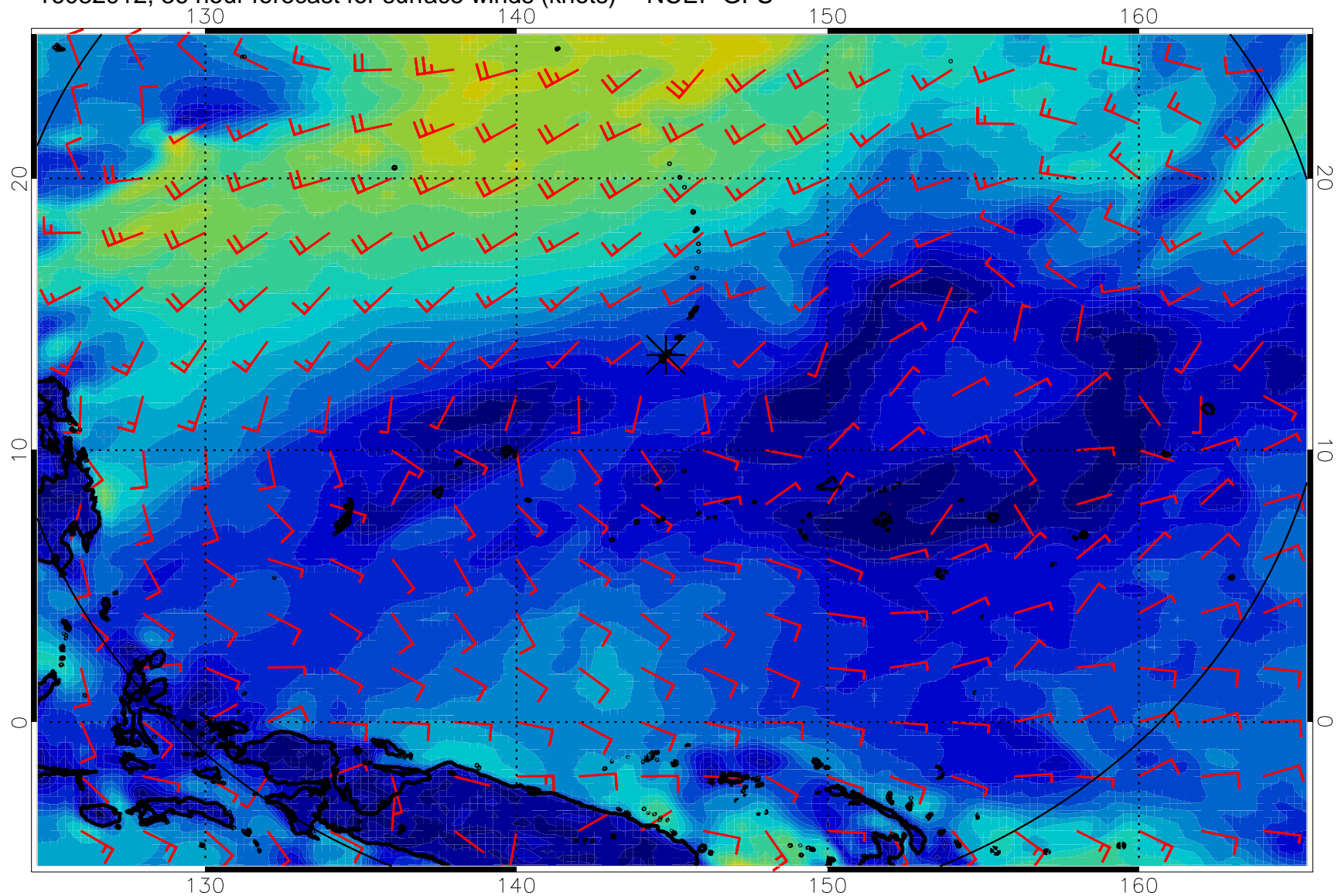
16082912, 36 hour forecast for surface winds (knots) -- NCEP GFS
