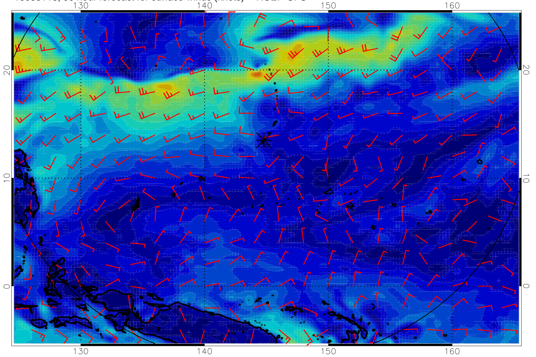
16083118, 90 hour forecast for surface winds (knots) -- NCEP GFS
