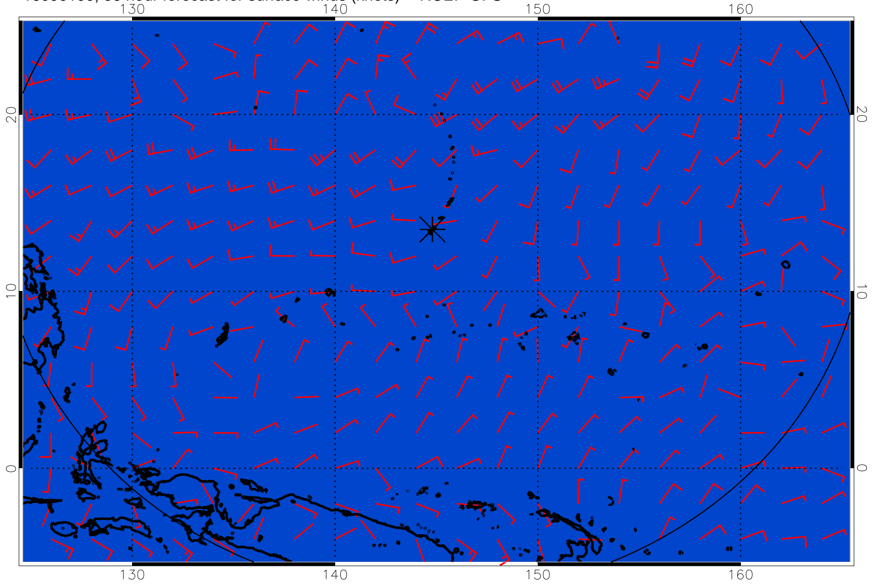
16090100, 96 hour forecast for surface winds (knots) -- NCEP GFS
