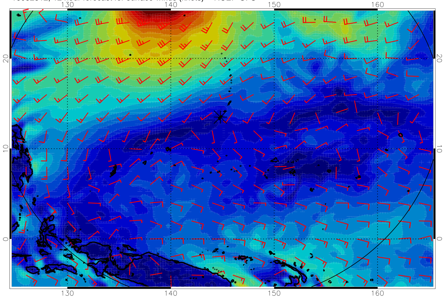
16082812, 12 hour forecast for surface winds (knots) -- NCEP GFS
