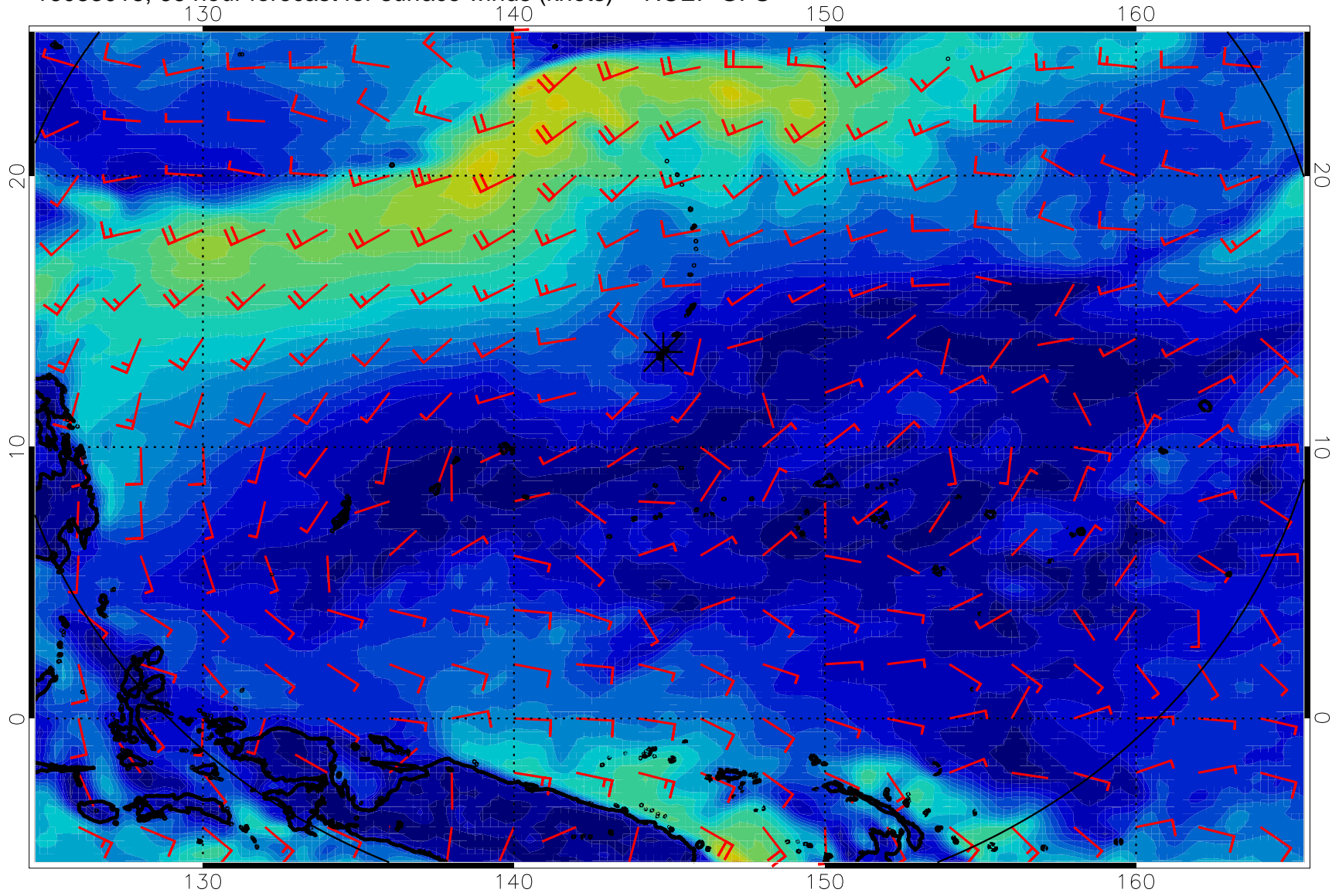
16083018, 66 hour forecast for surface winds (knots) -- NCEP GFS
