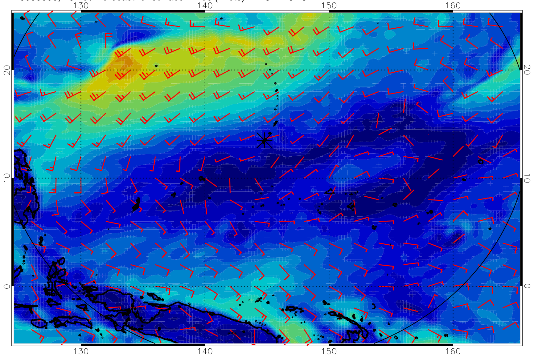
16083000, 48 hour forecast for surface winds (knots) -- NCEP GFS
