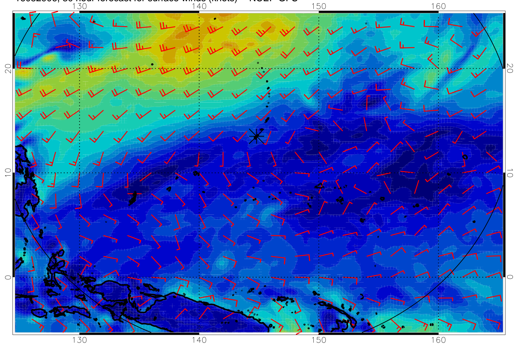
16082906, 30 hour forecast for surface winds (knots) -- NCEP GFS
