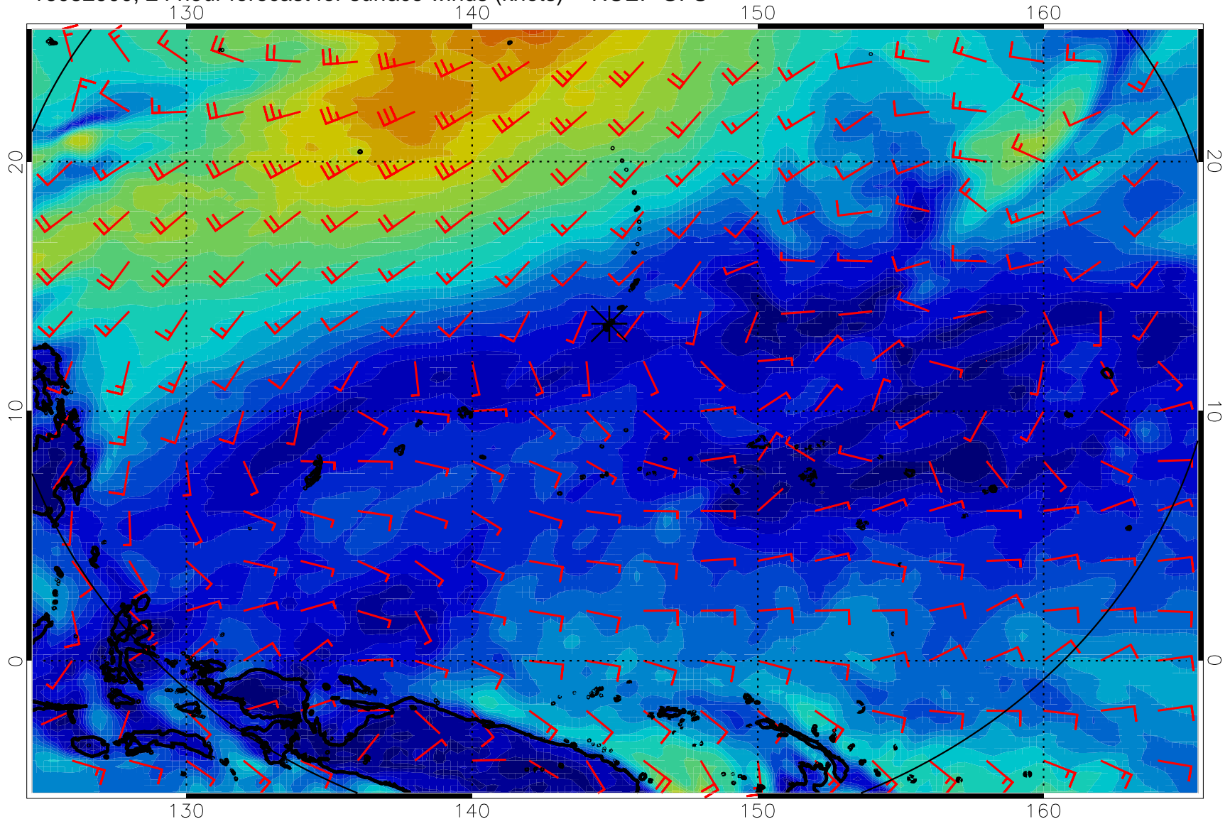
16082900, 24 hour forecast for surface winds (knots) -- NCEP GFS
