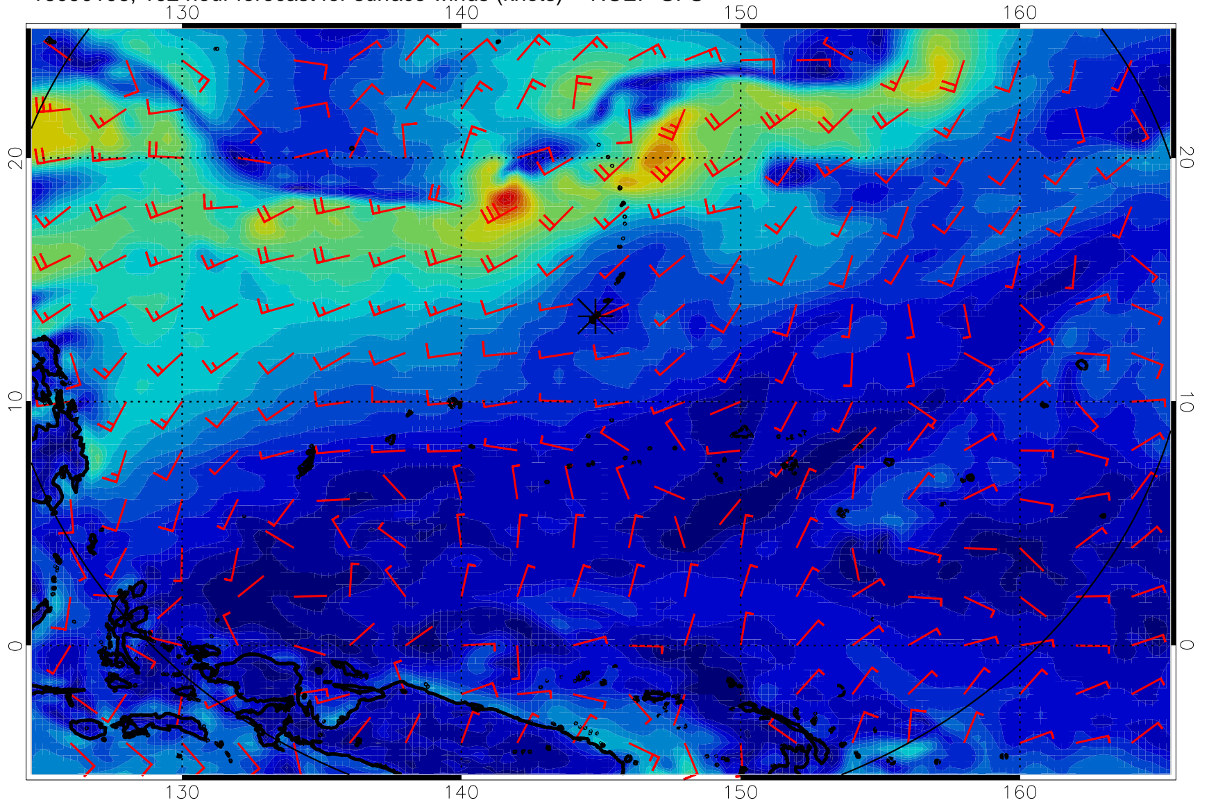
16090106, 102 hour forecast for surface winds (knots) -- NCEP GFS
