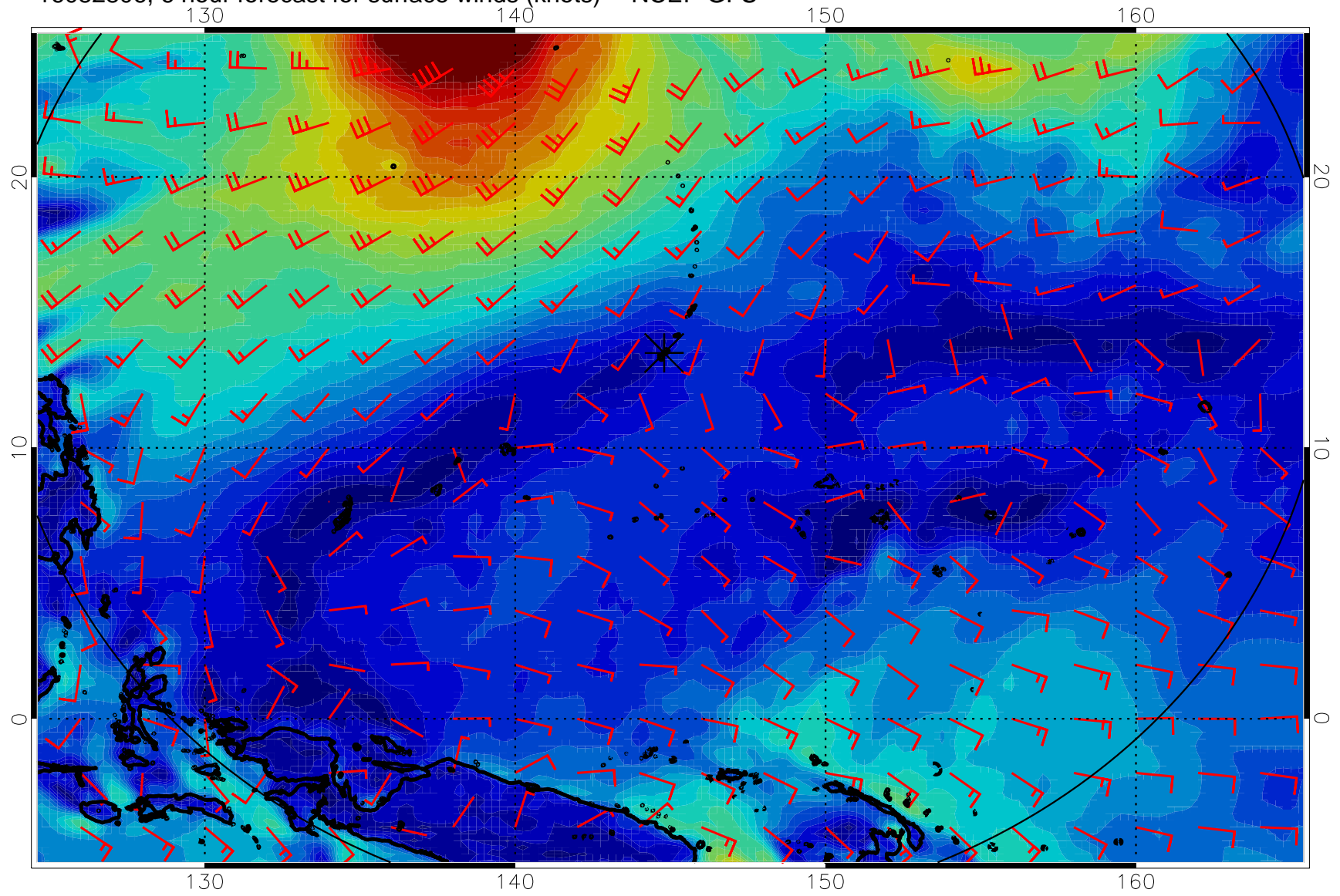
16082806, 6 hour forecast for surface winds (knots) -- NCEP GFS
