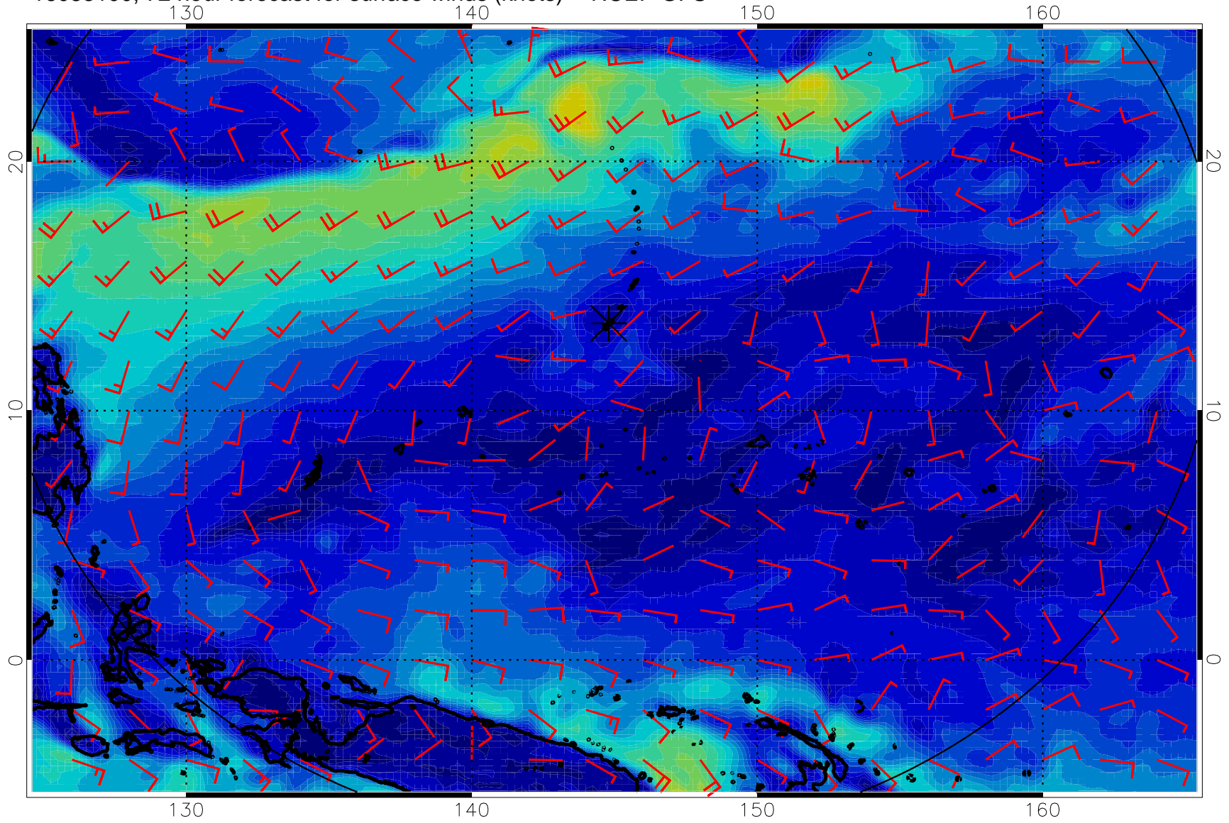
16083100, 72 hour forecast for surface winds (knots) -- NCEP GFS
