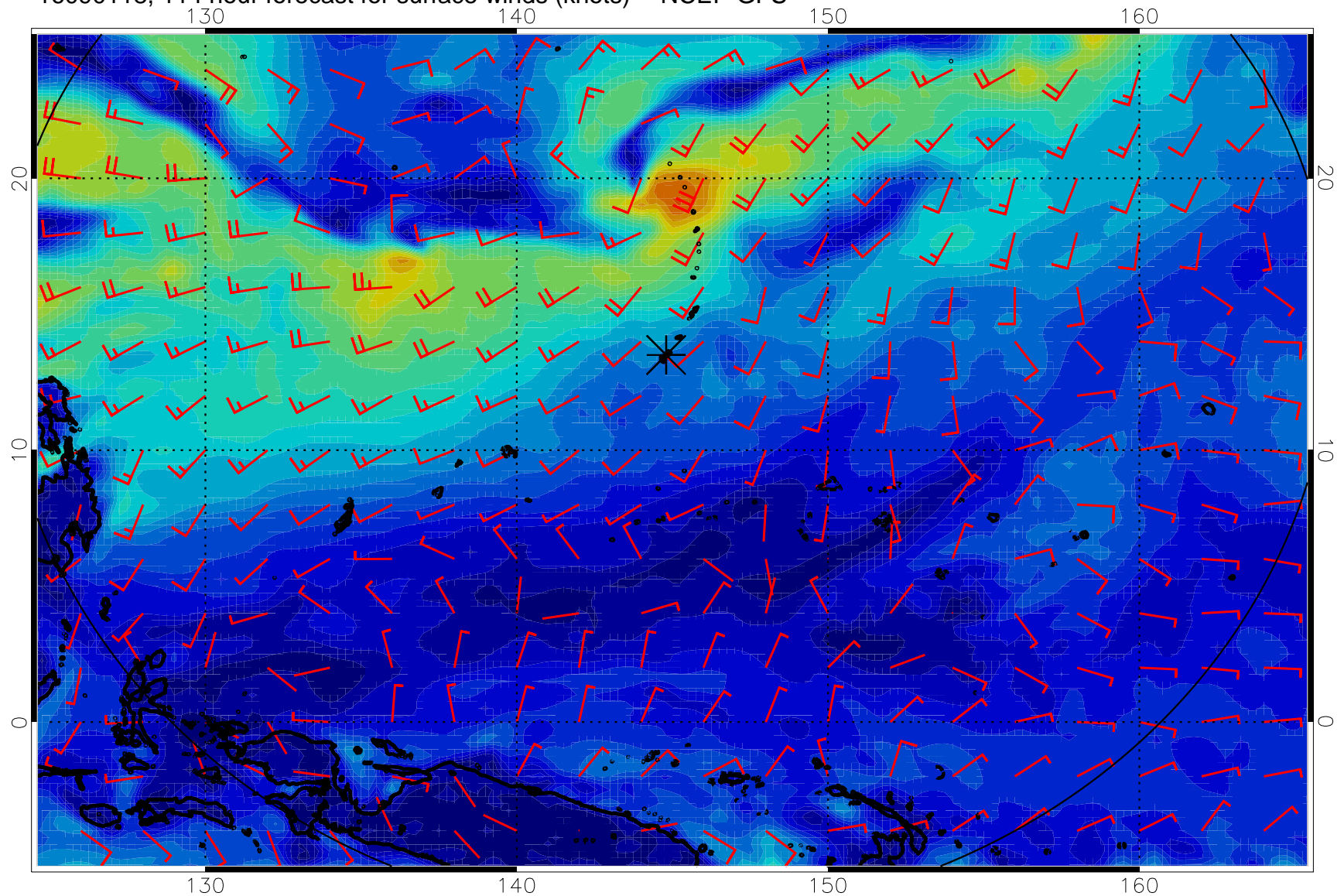
16090118, 114 hour forecast for surface winds (knots) -- NCEP GFS
