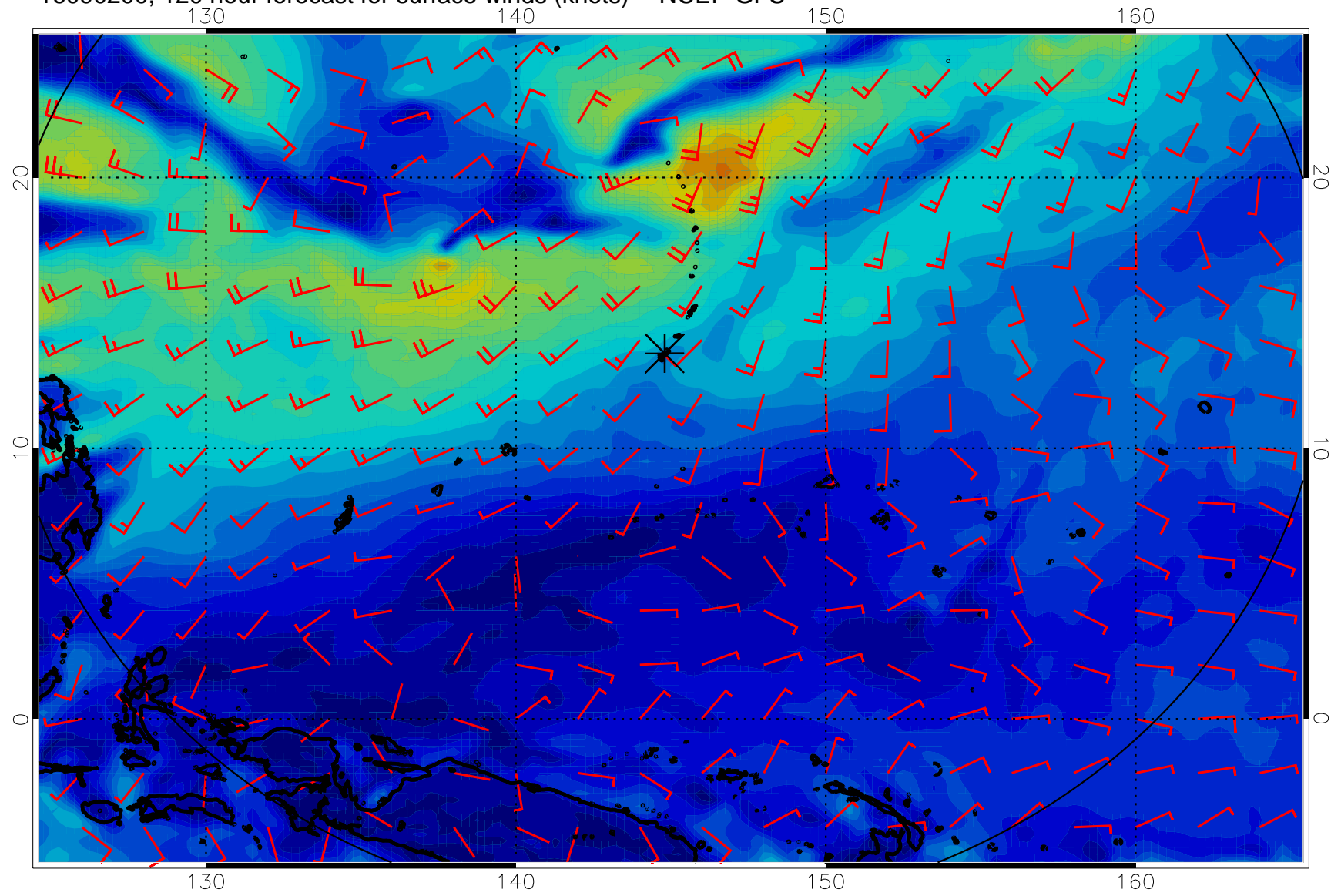
16090200, 120 hour forecast for surface winds (knots) -- NCEP GFS
