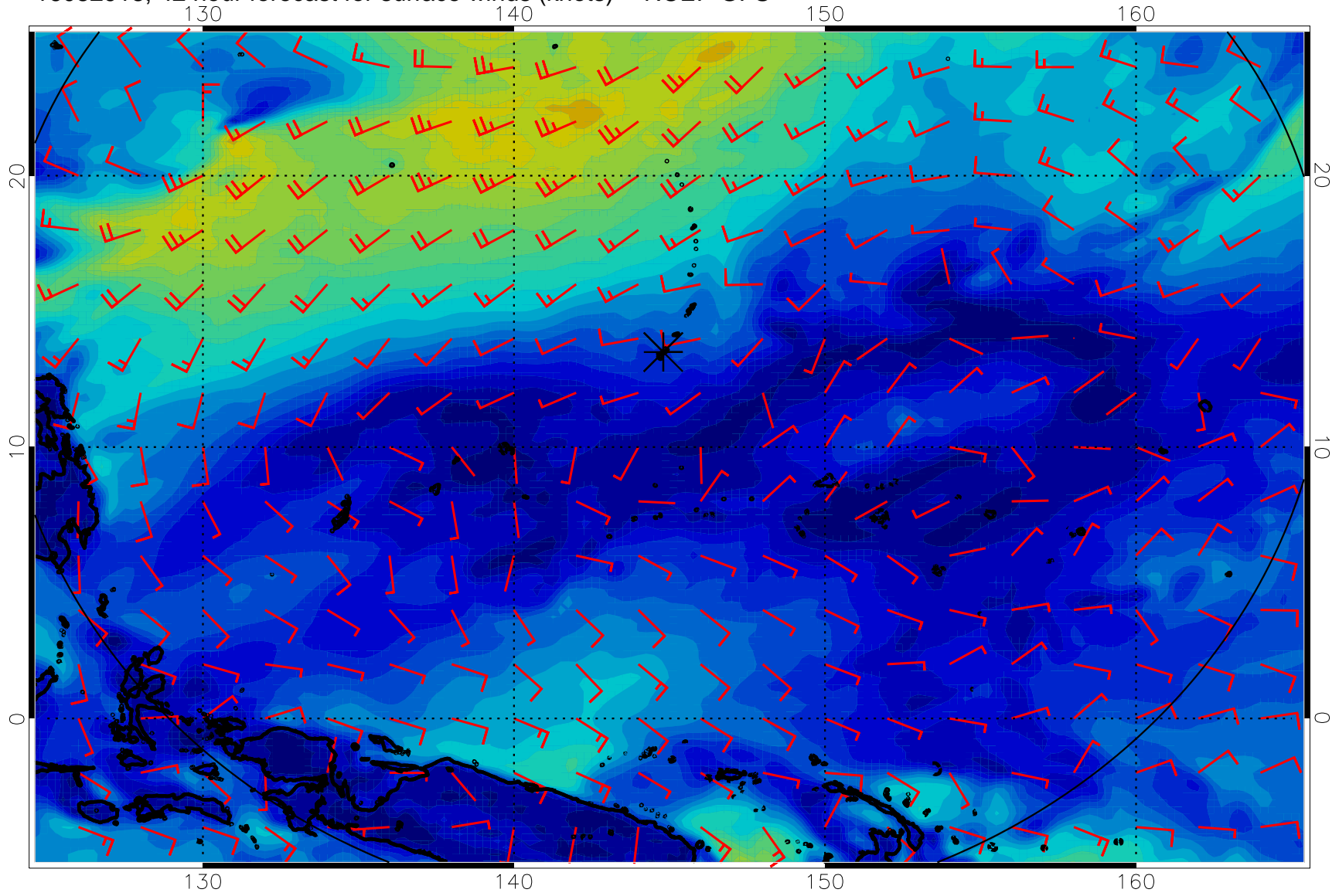
16082918, 42 hour forecast for surface winds (knots) -- NCEP GFS
