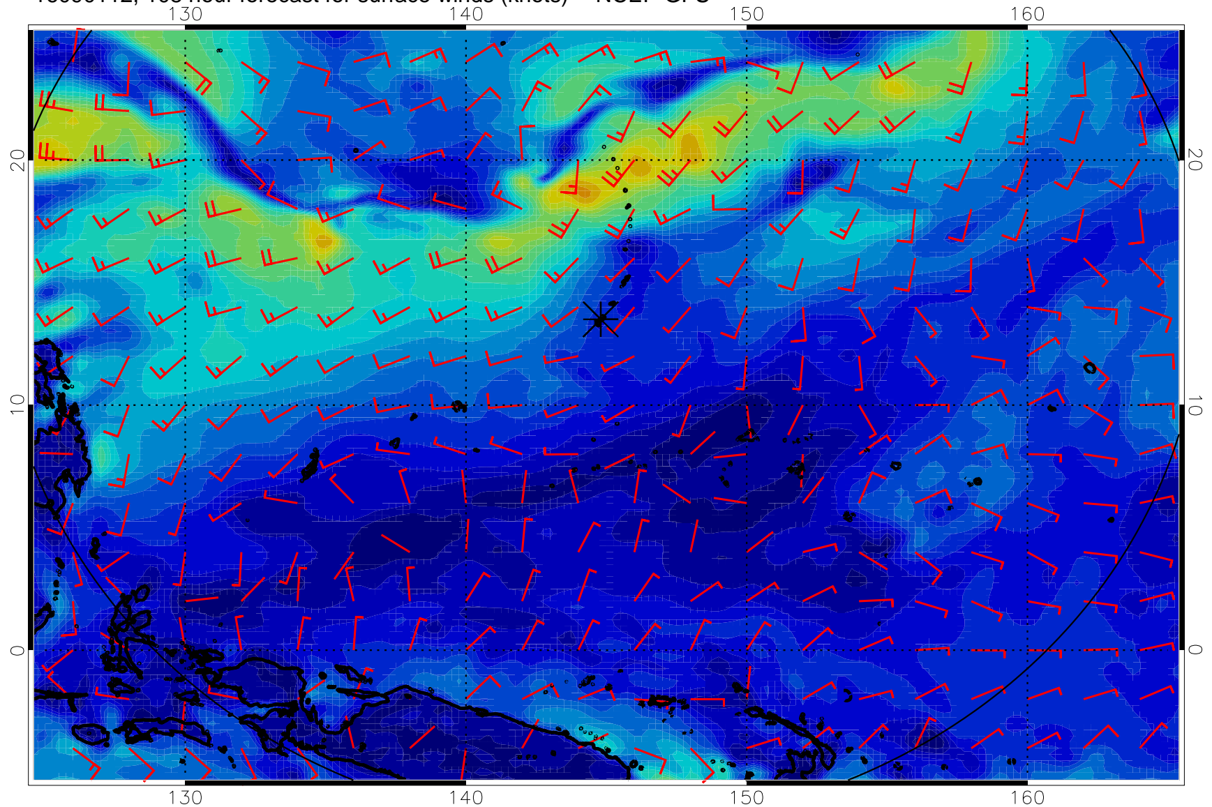
16090112, 108 hour forecast for surface winds (knots) -- NCEP GFS
