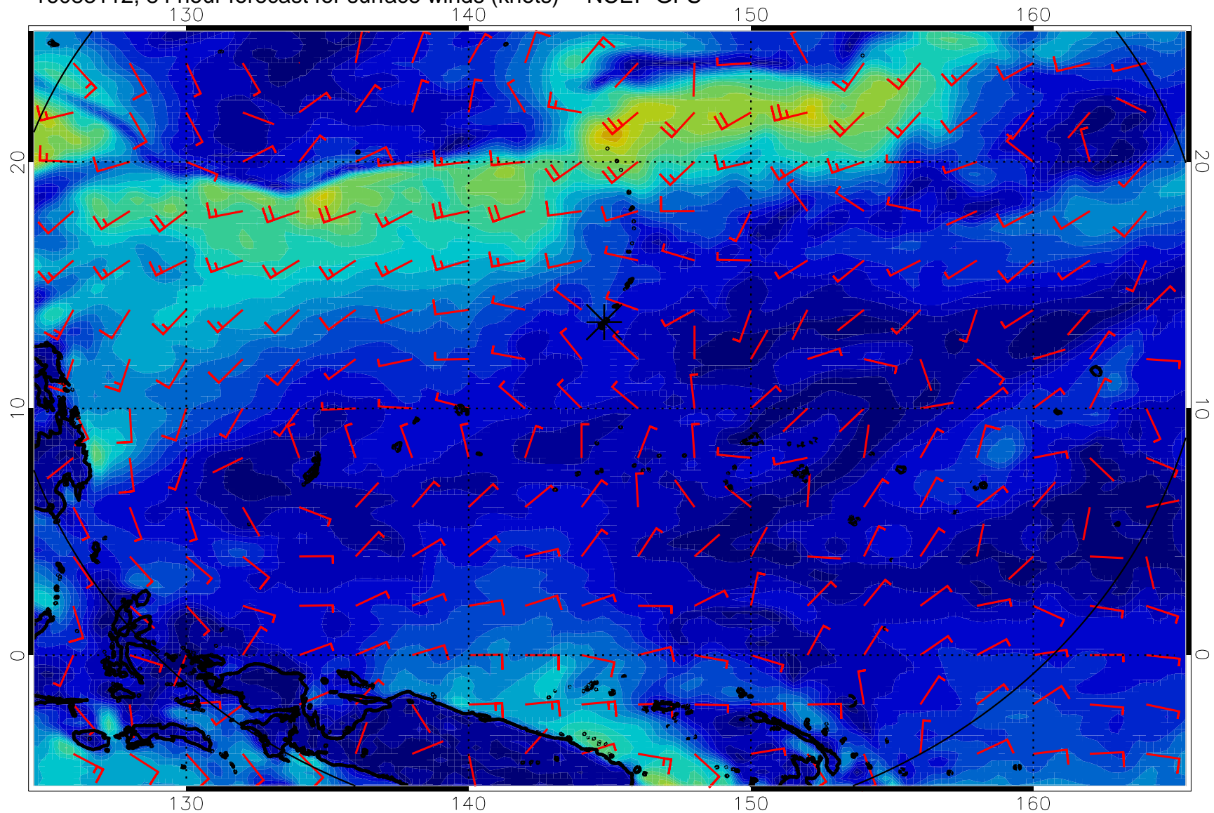
16083112, 84 hour forecast for surface winds (knots) -- NCEP GFS
