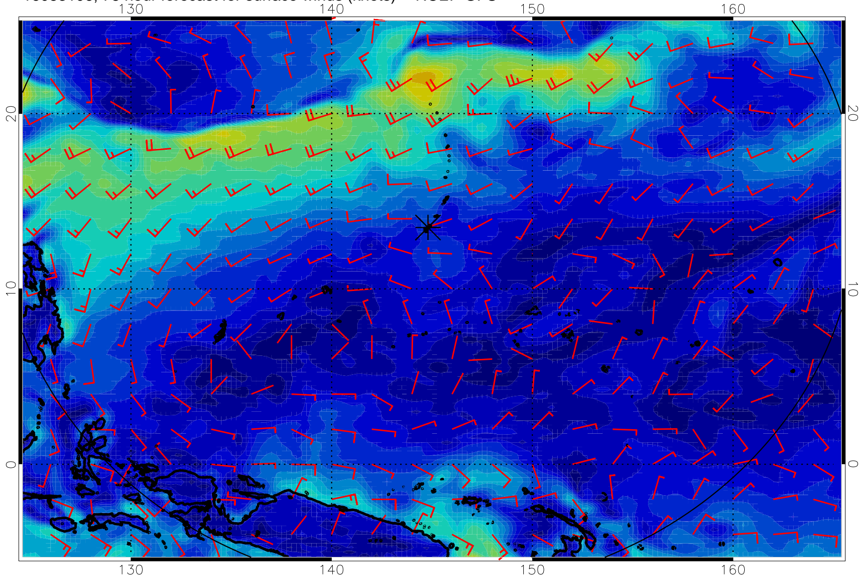
16083106, 78 hour forecast for surface winds (knots) -- NCEP GFS
