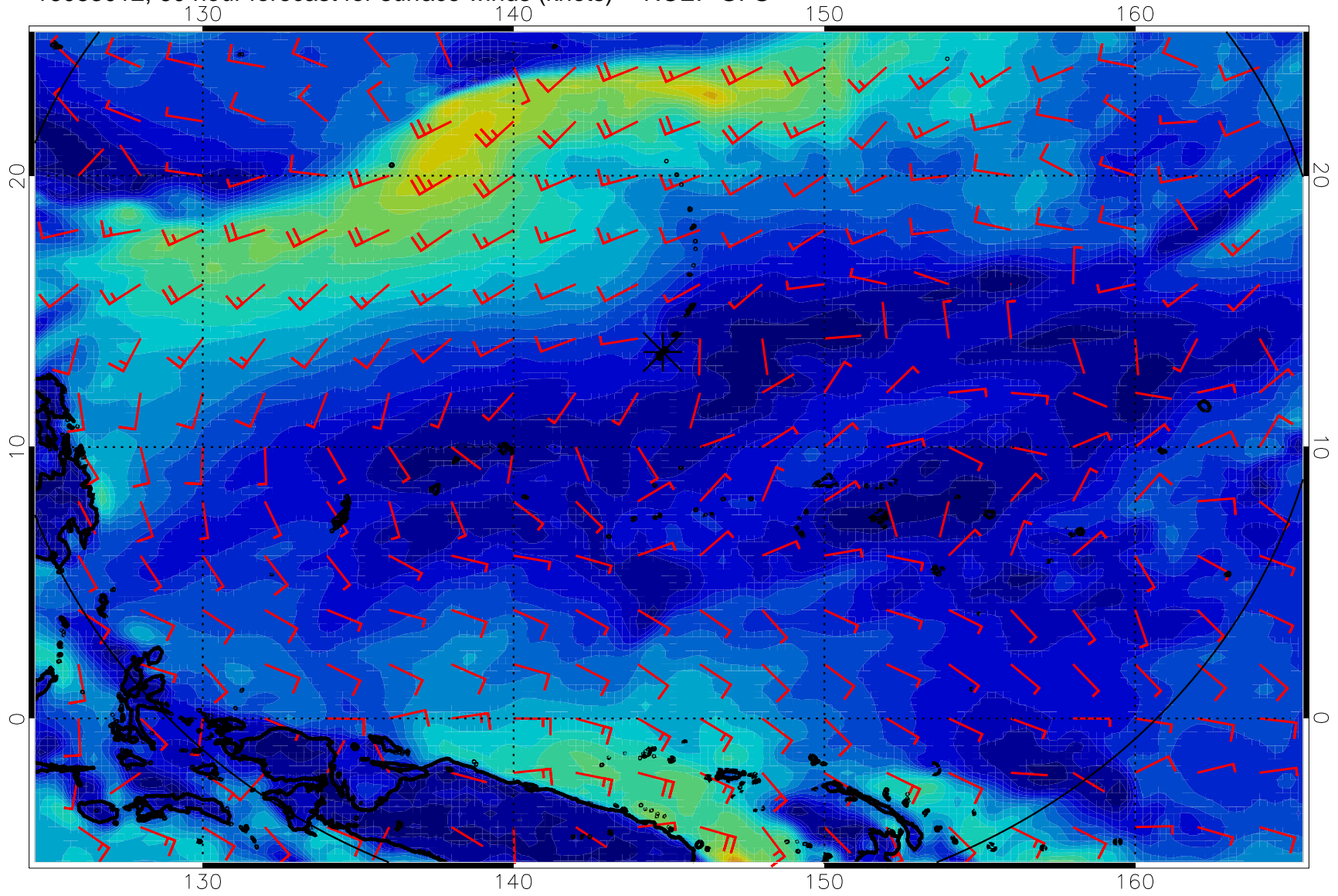
16083012, 60 hour forecast for surface winds (knots) -- NCEP GFS
