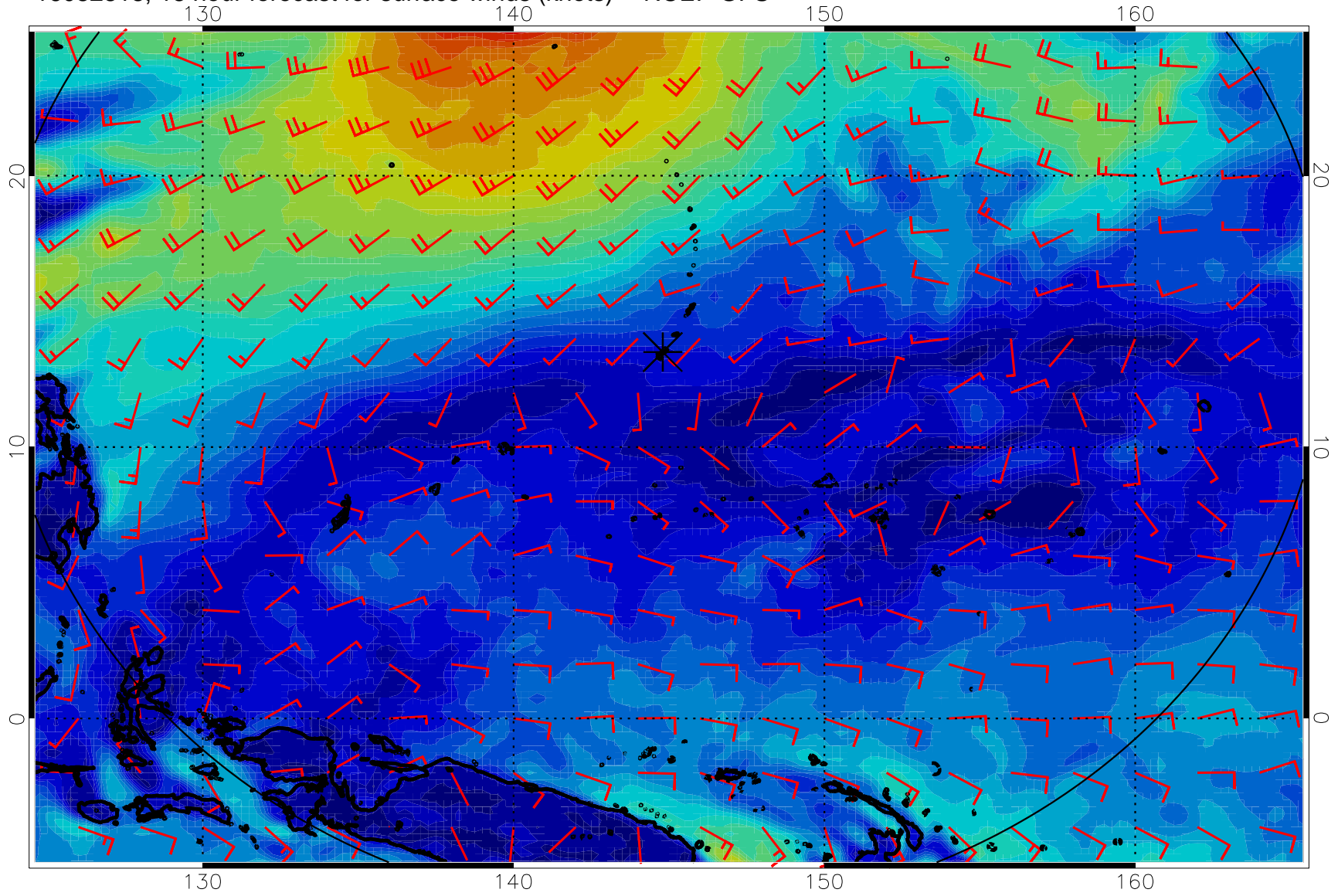
16082818, 18 hour forecast for surface winds (knots) -- NCEP GFS
