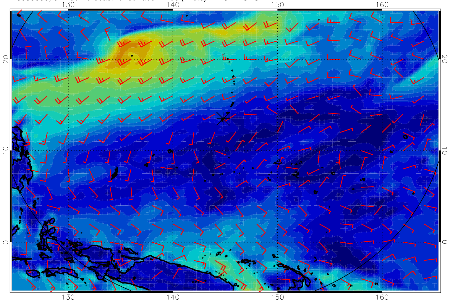
16083006, 54 hour forecast for surface winds (knots) -- NCEP GFS
