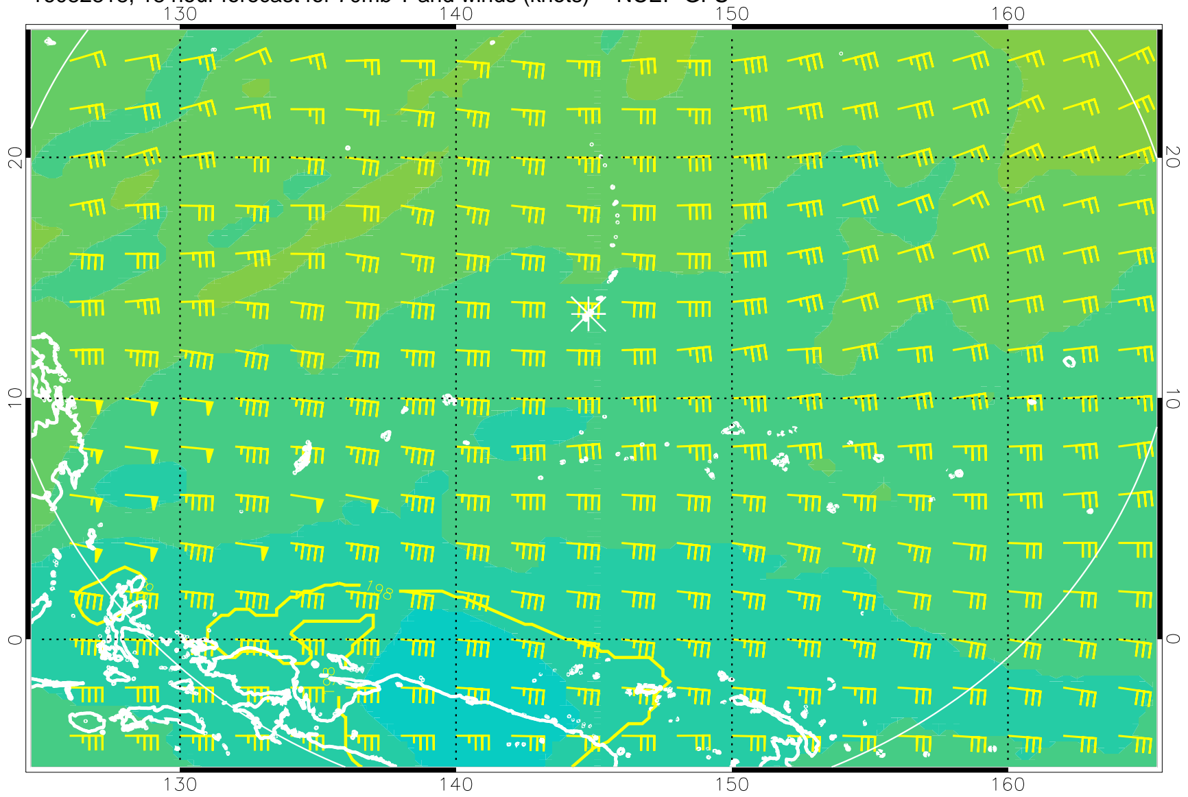
16082818, 18 hour forecast for 70mb T and winds (knots) -- NCEP GFS
