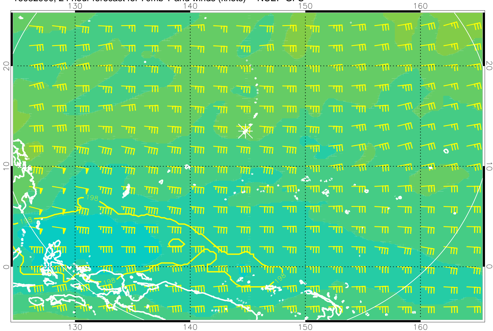
16082900, 24 hour forecast for 70mb T and winds (knots) -- NCEP GFS
