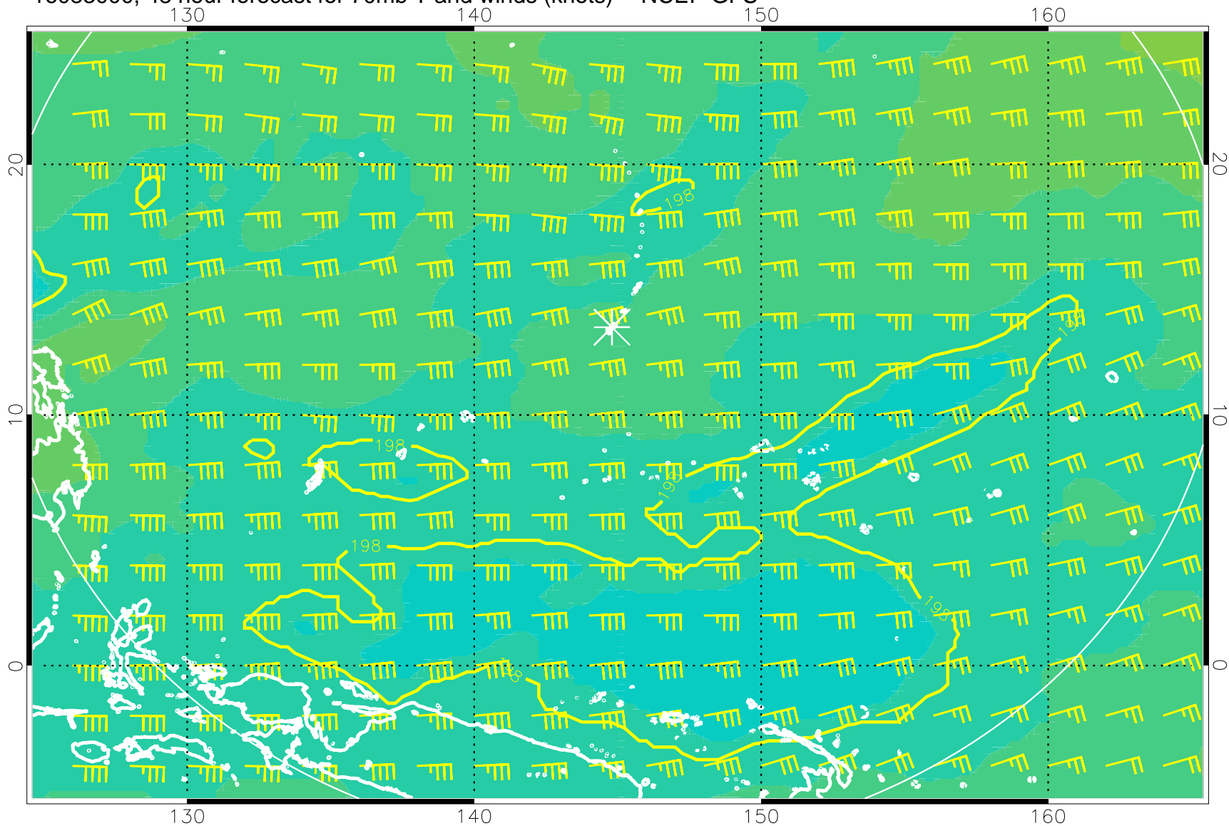
16083000, 48 hour forecast for 70mb T and winds (knots) -- NCEP GFS
