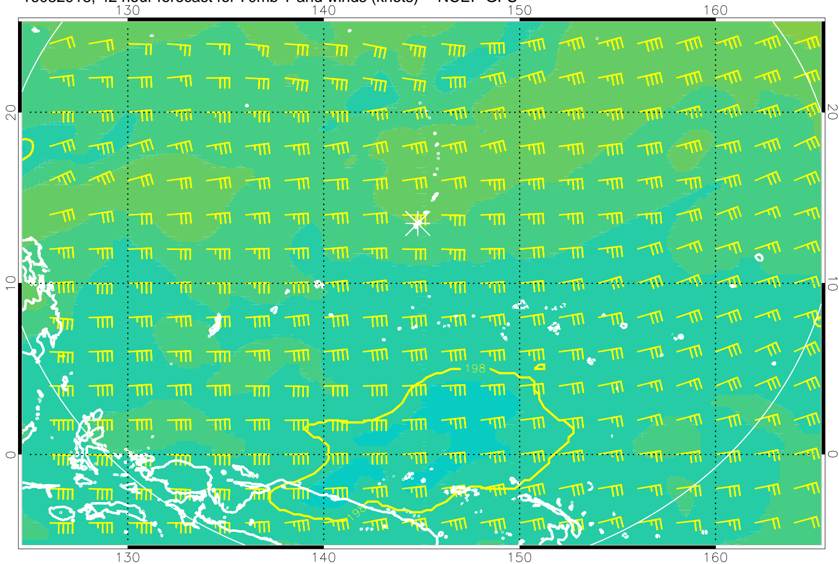
16082918, 42 hour forecast for 70mb T and winds (knots) -- NCEP GFS
