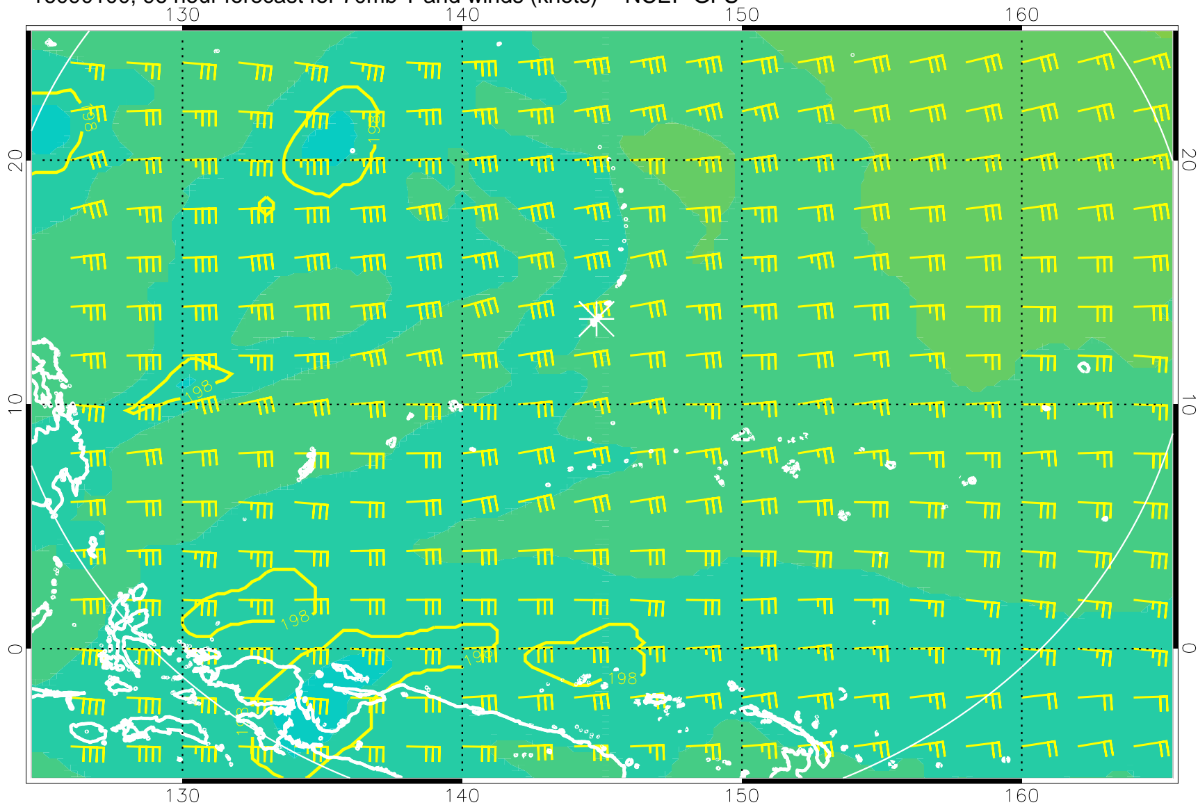
16090100, 96 hour forecast for 70mb T and winds (knots) -- NCEP GFS
