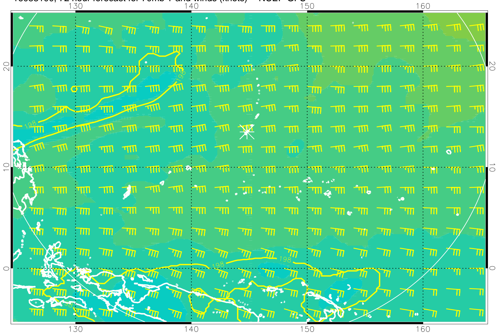
16083100, 72 hour forecast for 70mb T and winds (knots) -- NCEP GFS
