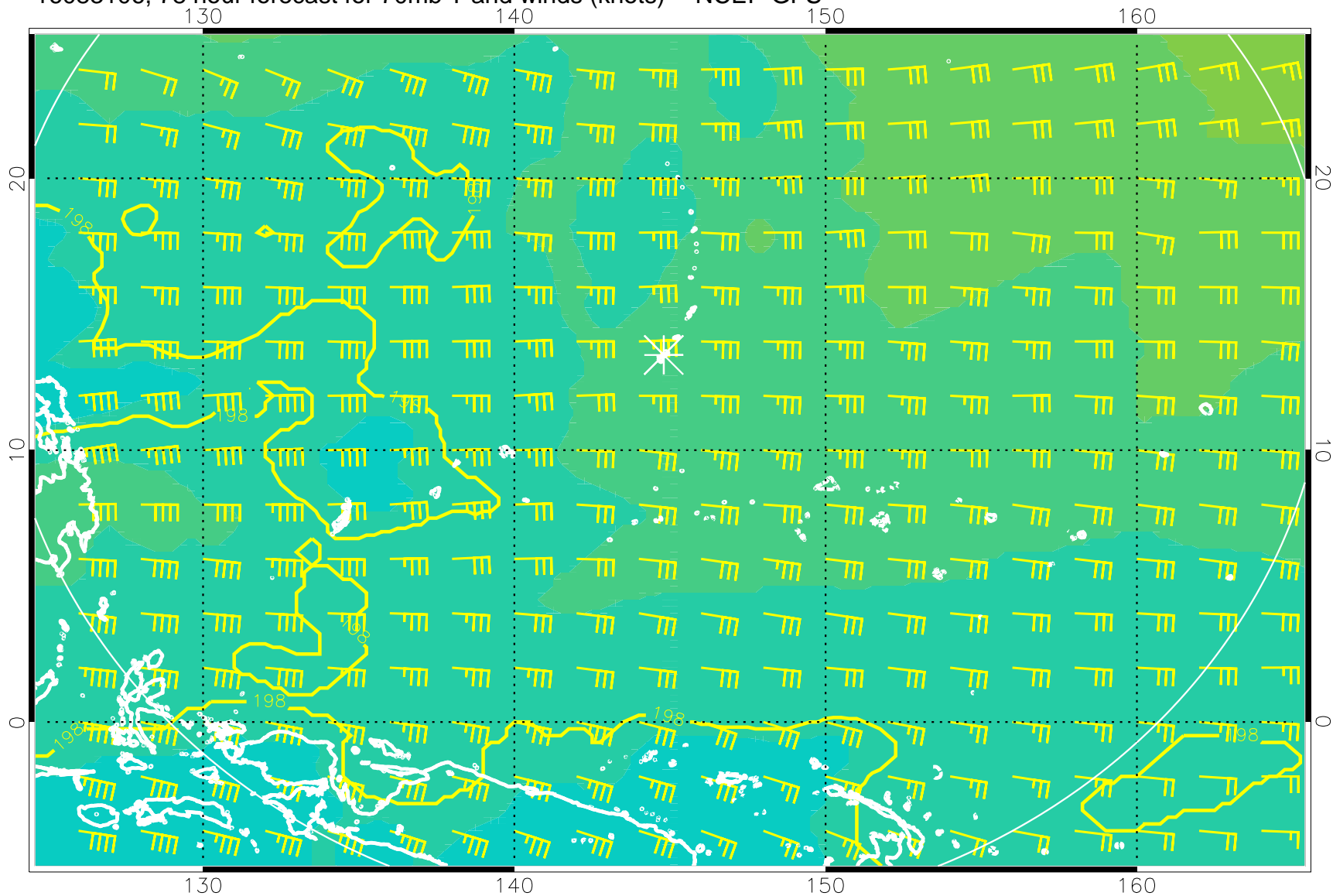
16083106, 78 hour forecast for 70mb T and winds (knots) -- NCEP GFS
