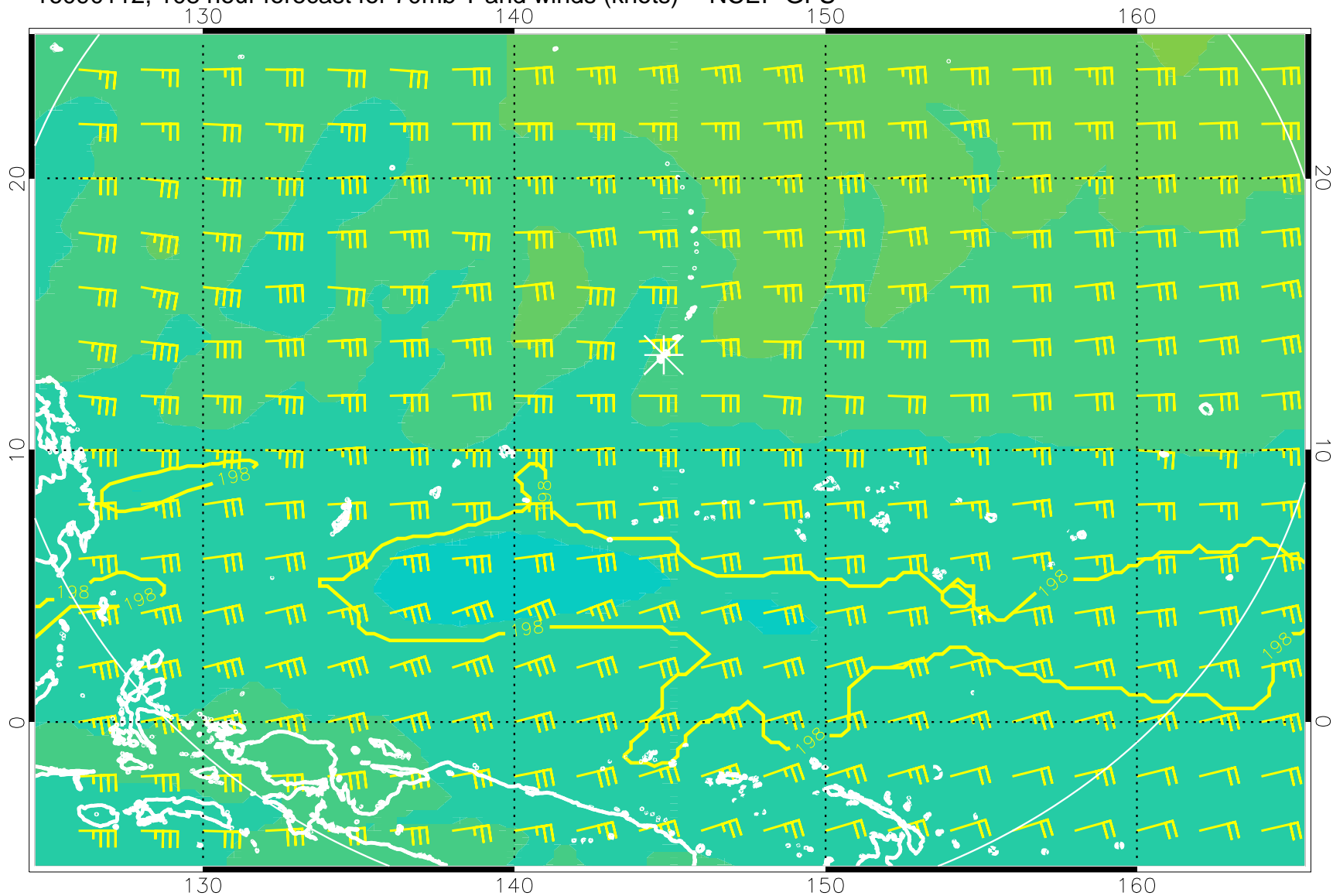
16090112, 108 hour forecast for 70mb T and winds (knots) -- NCEP GFS
