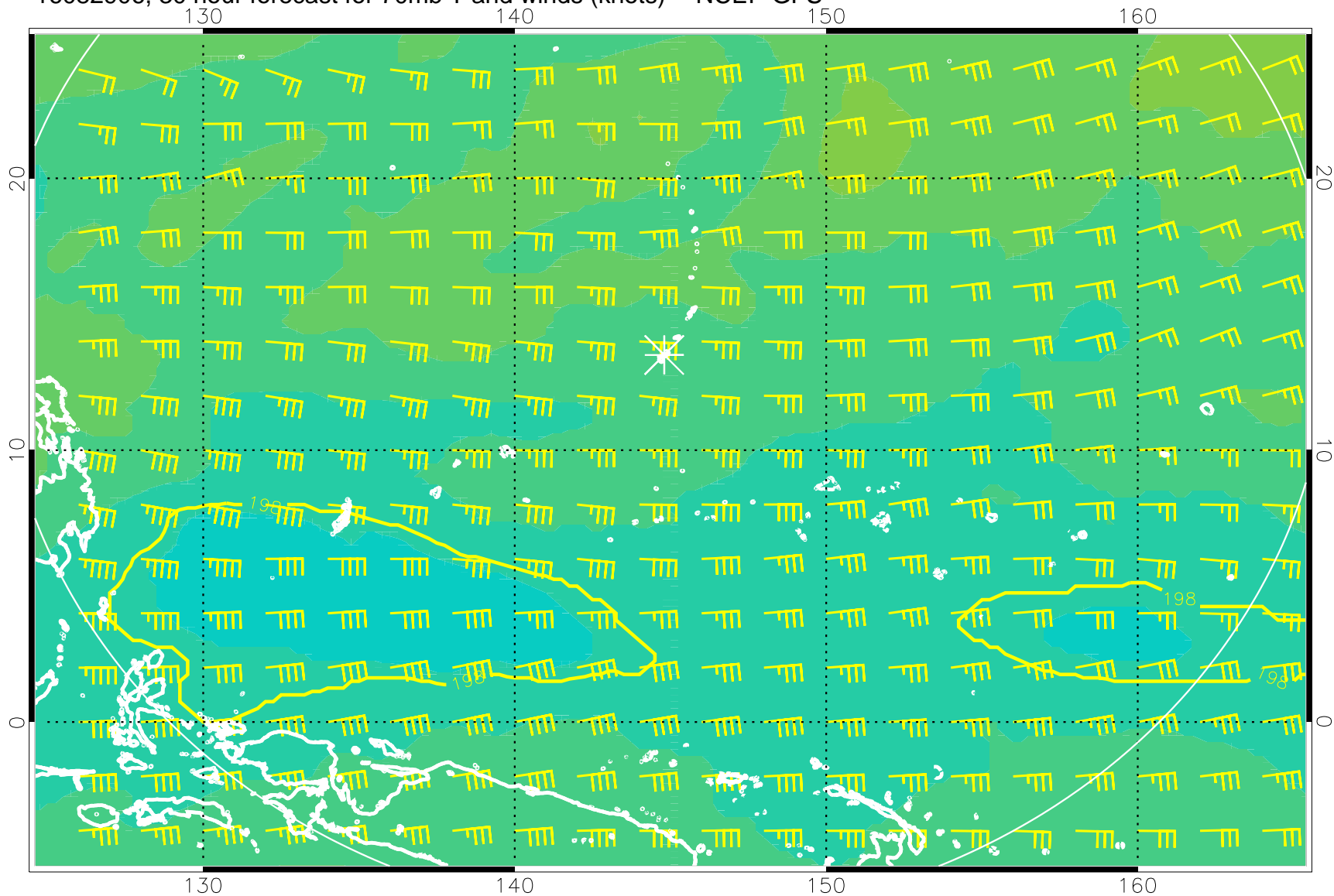
16082906, 30 hour forecast for 70mb T and winds (knots) -- NCEP GFS
