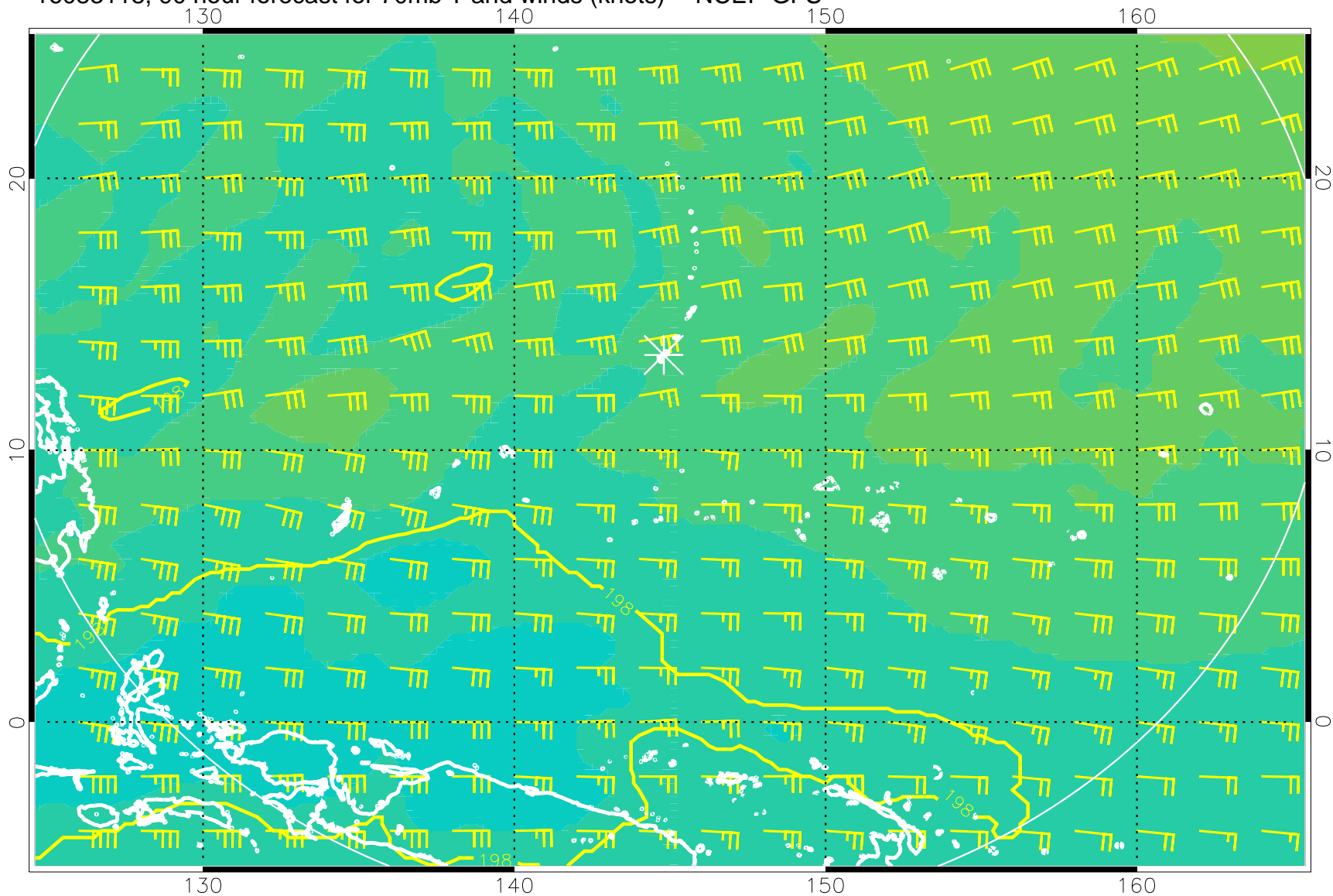
16083118, 90 hour forecast for 70mb T and winds (knots) -- NCEP GFS
