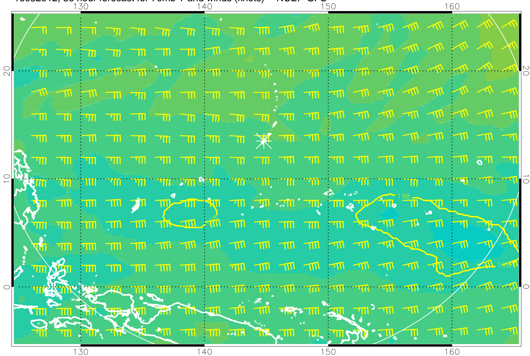
16082912, 36 hour forecast for 70mb T and winds (knots) -- NCEP GFS
