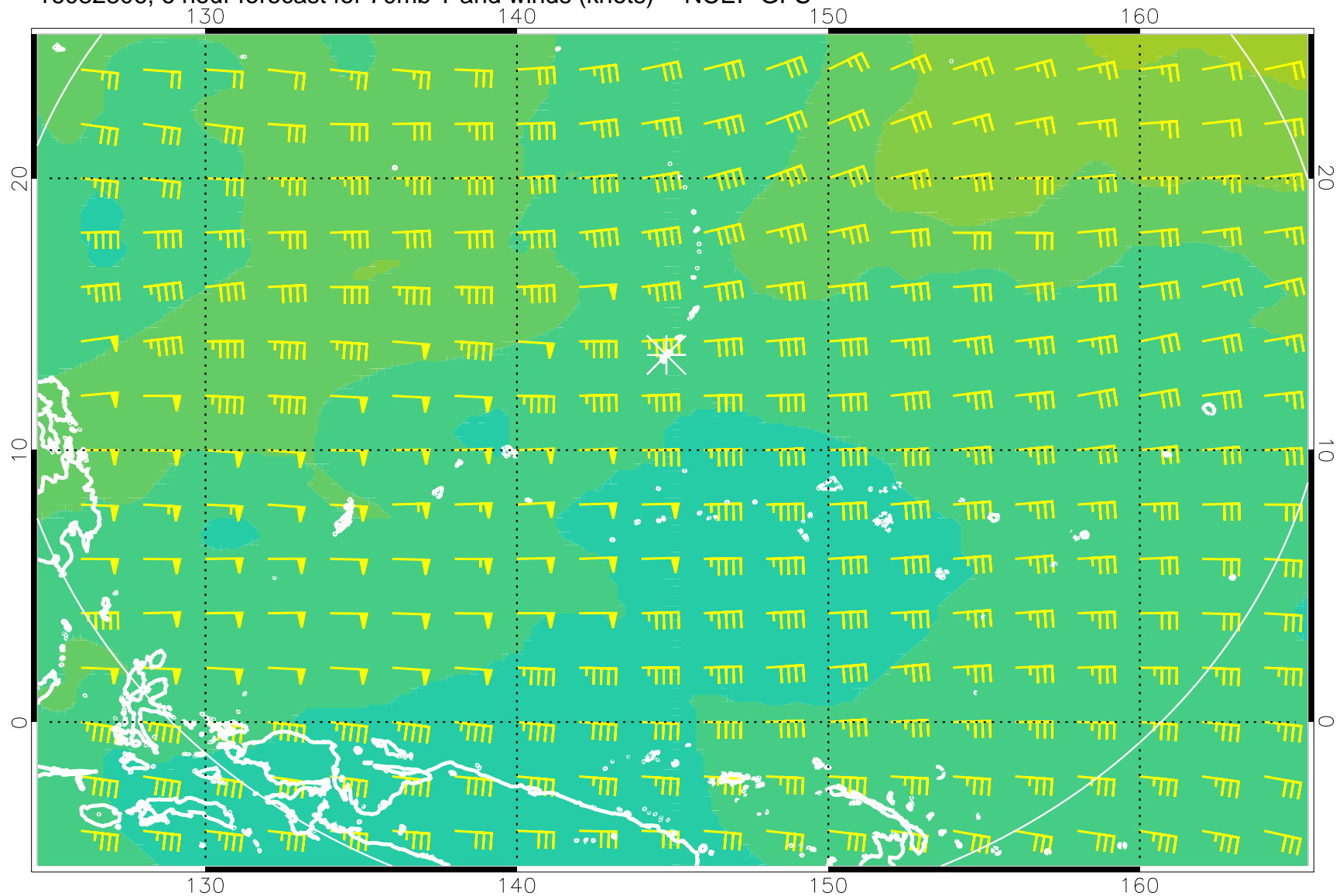
16082806, 6 hour forecast for 70mb T and winds (knots) -- NCEP GFS
