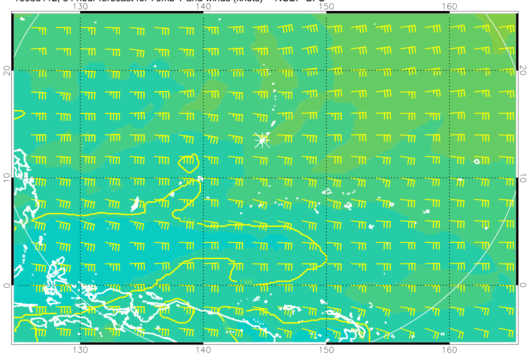
16083112, 84 hour forecast for 70mb T and winds (knots) -- NCEP GFS
