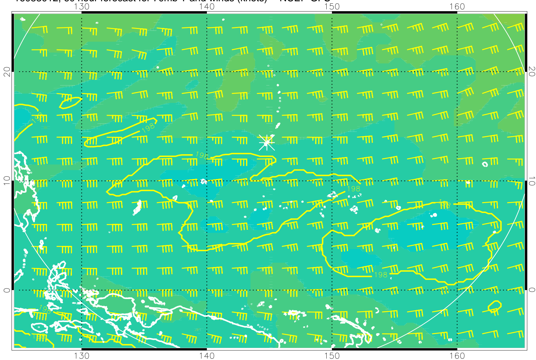
16083012, 60 hour forecast for 70mb T and winds (knots) -- NCEP GFS
