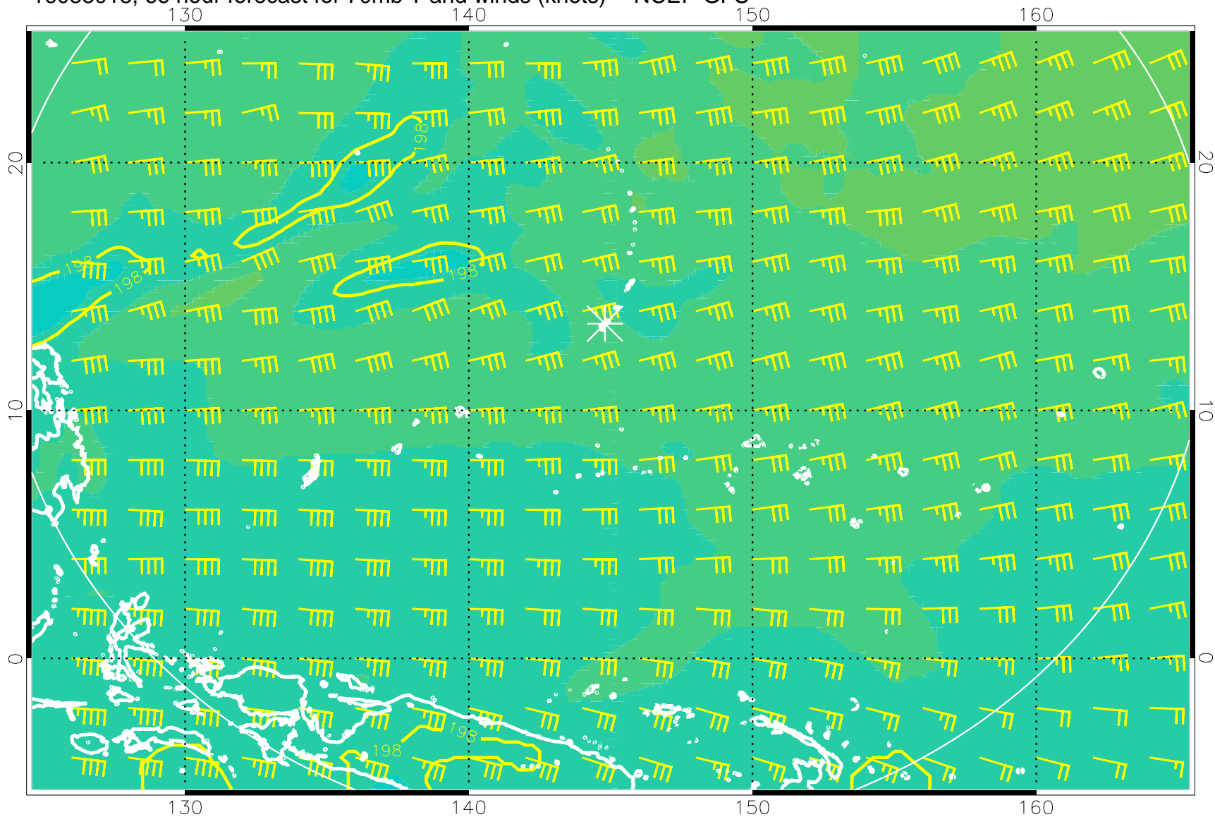
16083018, 66 hour forecast for 70mb T and winds (knots) -- NCEP GFS
