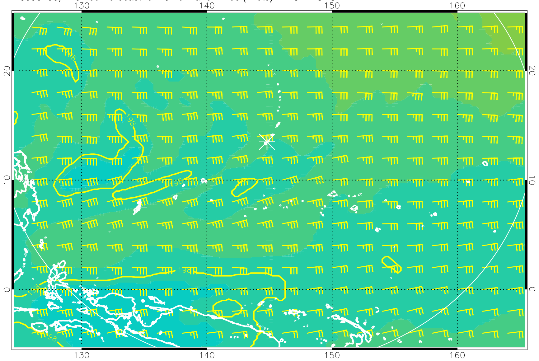
16090200, 120 hour forecast for 70mb T and winds (knots) -- NCEP GFS
