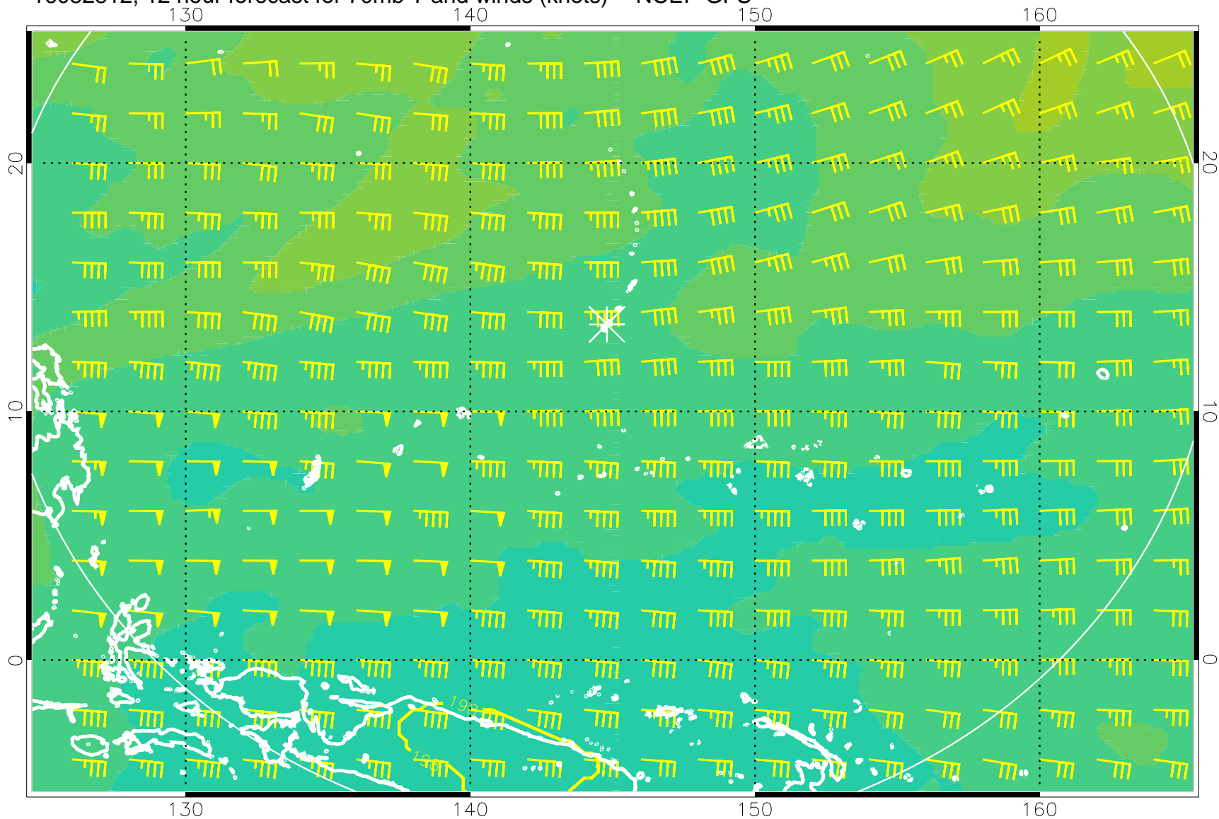
16082812, 12 hour forecast for 70mb T and winds (knots) -- NCEP GFS
