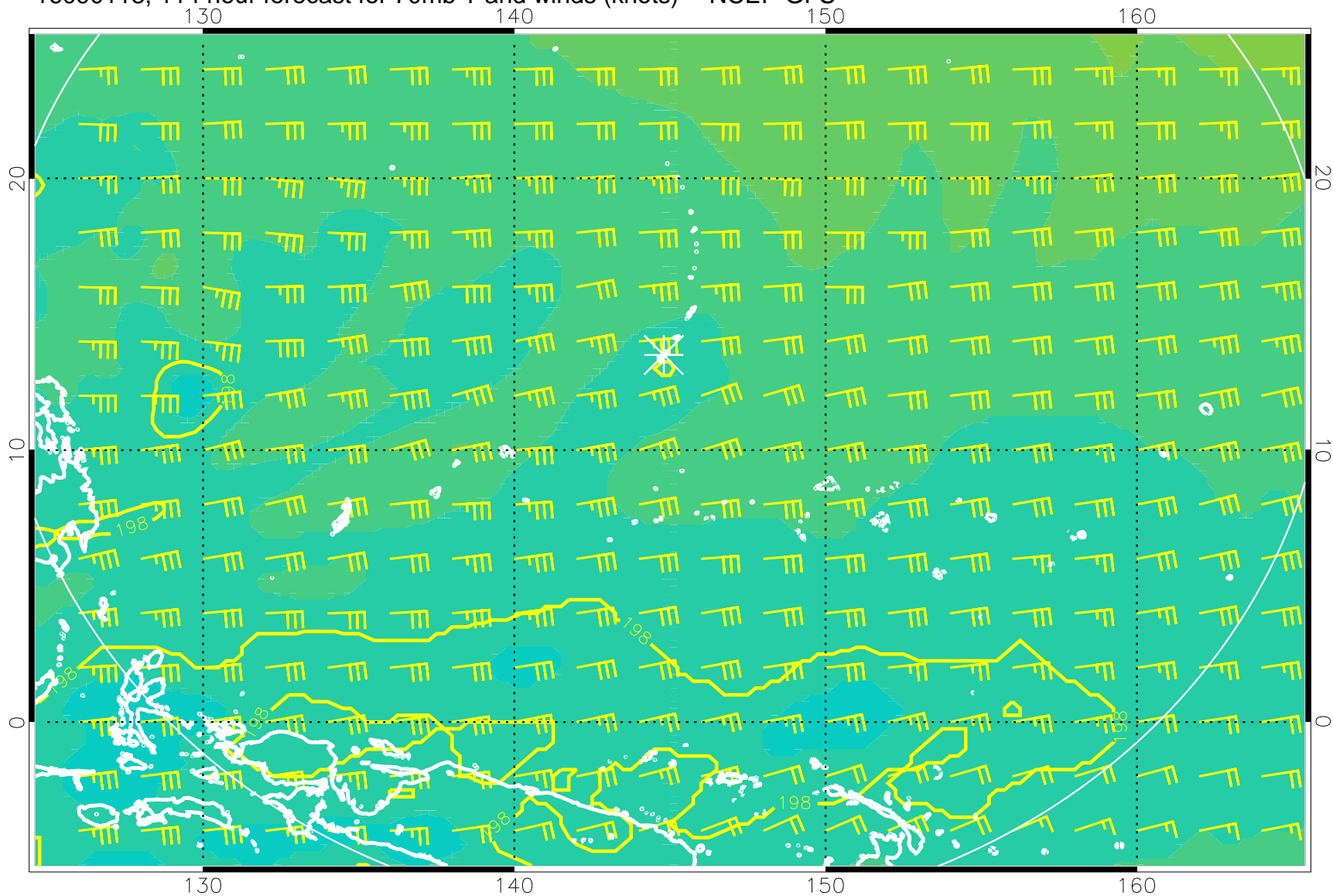
16090118, 114 hour forecast for 70mb T and winds (knots) -- NCEP GFS
