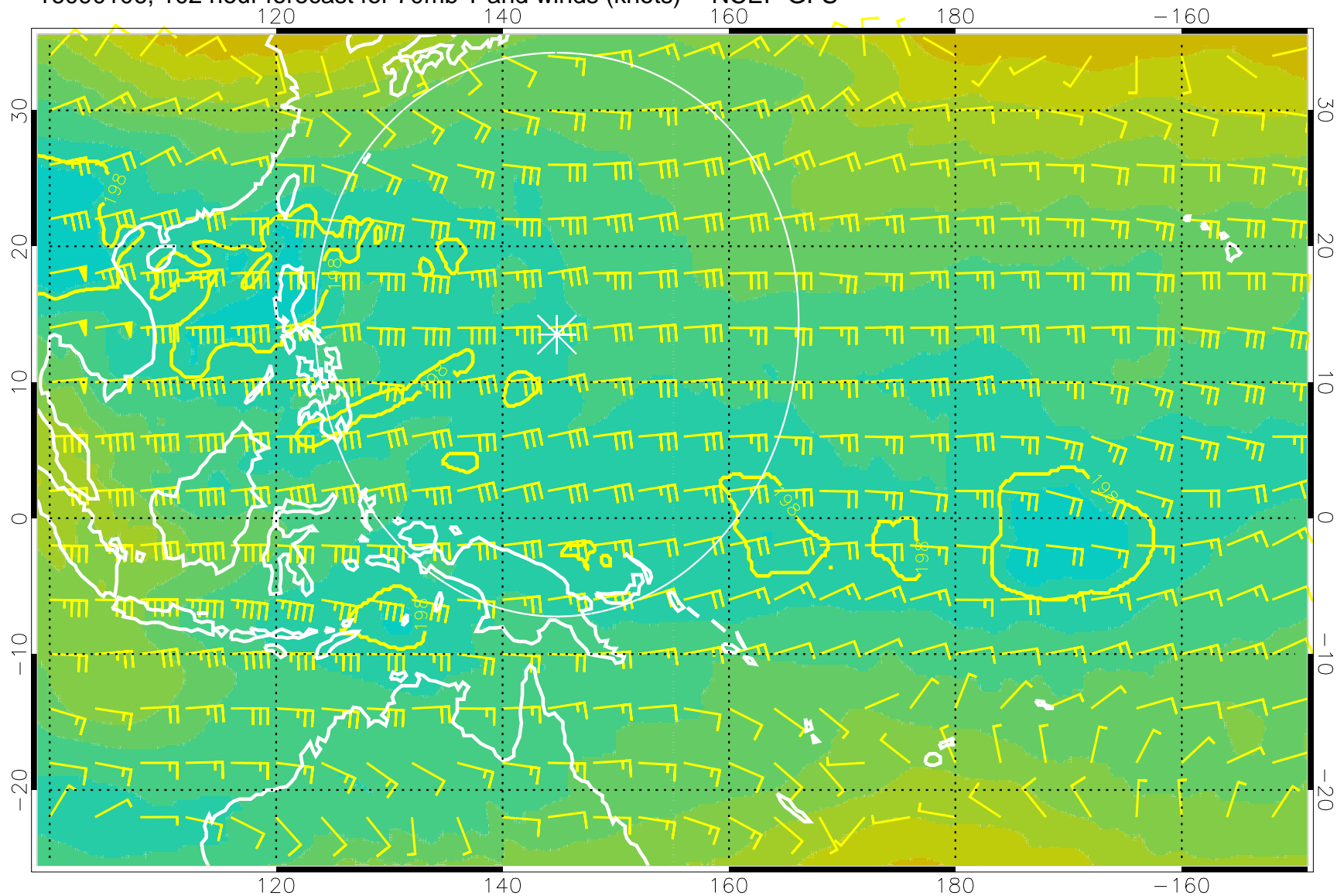
16090106, 102 hour forecast for 70mb T and winds (knots) -- NCEP GFS
