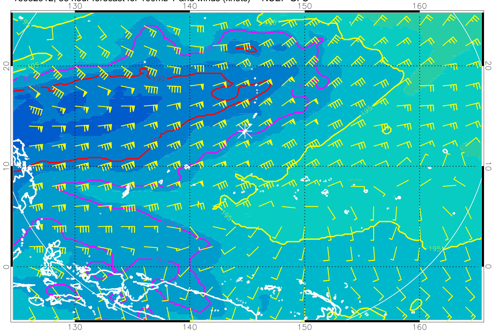
16082912, 36 hour forecast for 100mb T and winds (knots) -- NCEP GFS
