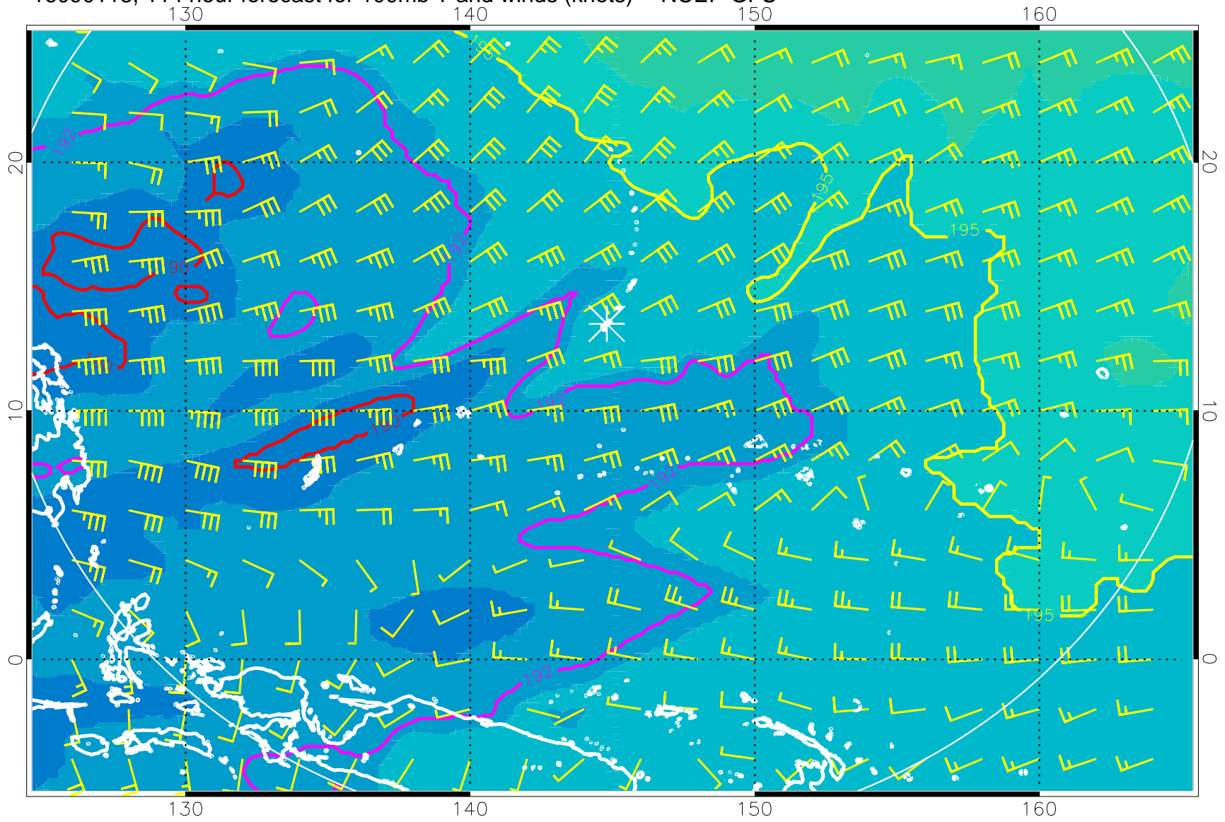
16090118, 114 hour forecast for 100mb T and winds (knots) -- NCEP GFS
