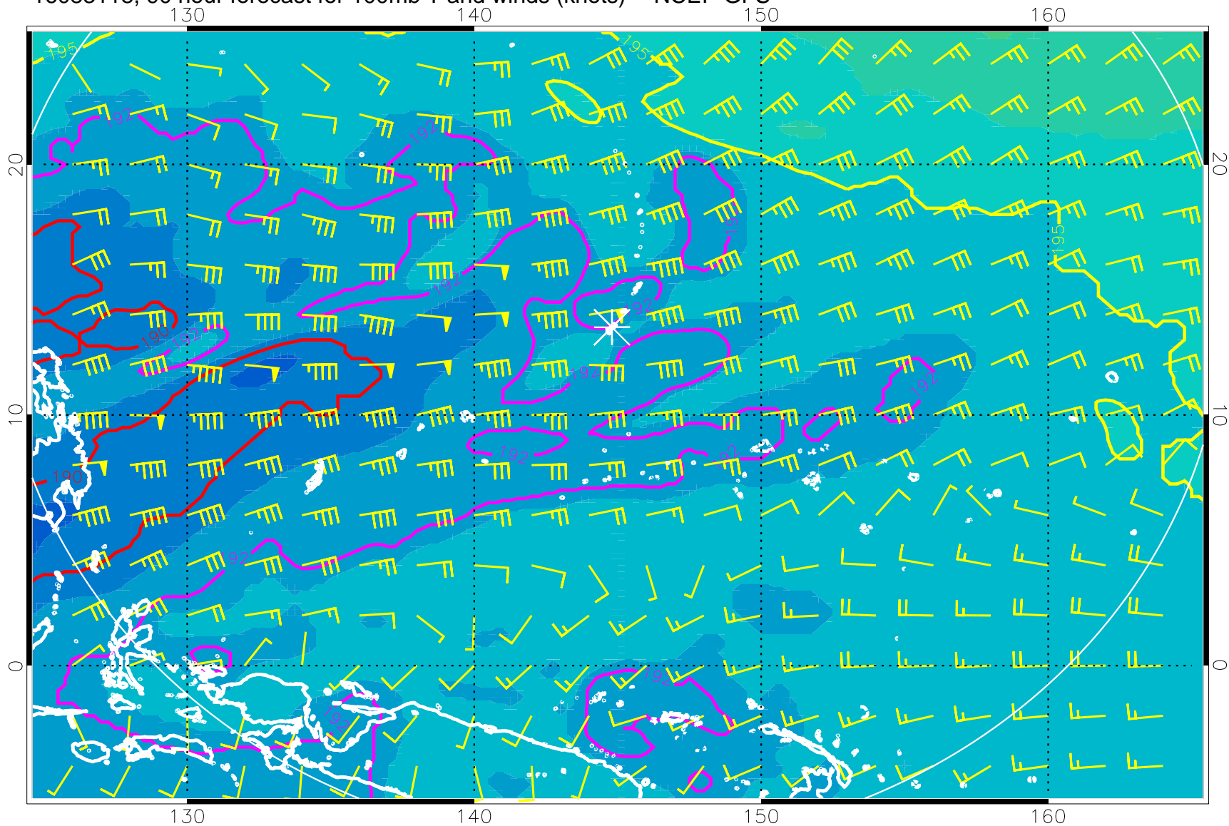
16083118, 90 hour forecast for 100mb T and winds (knots) -- NCEP GFS
