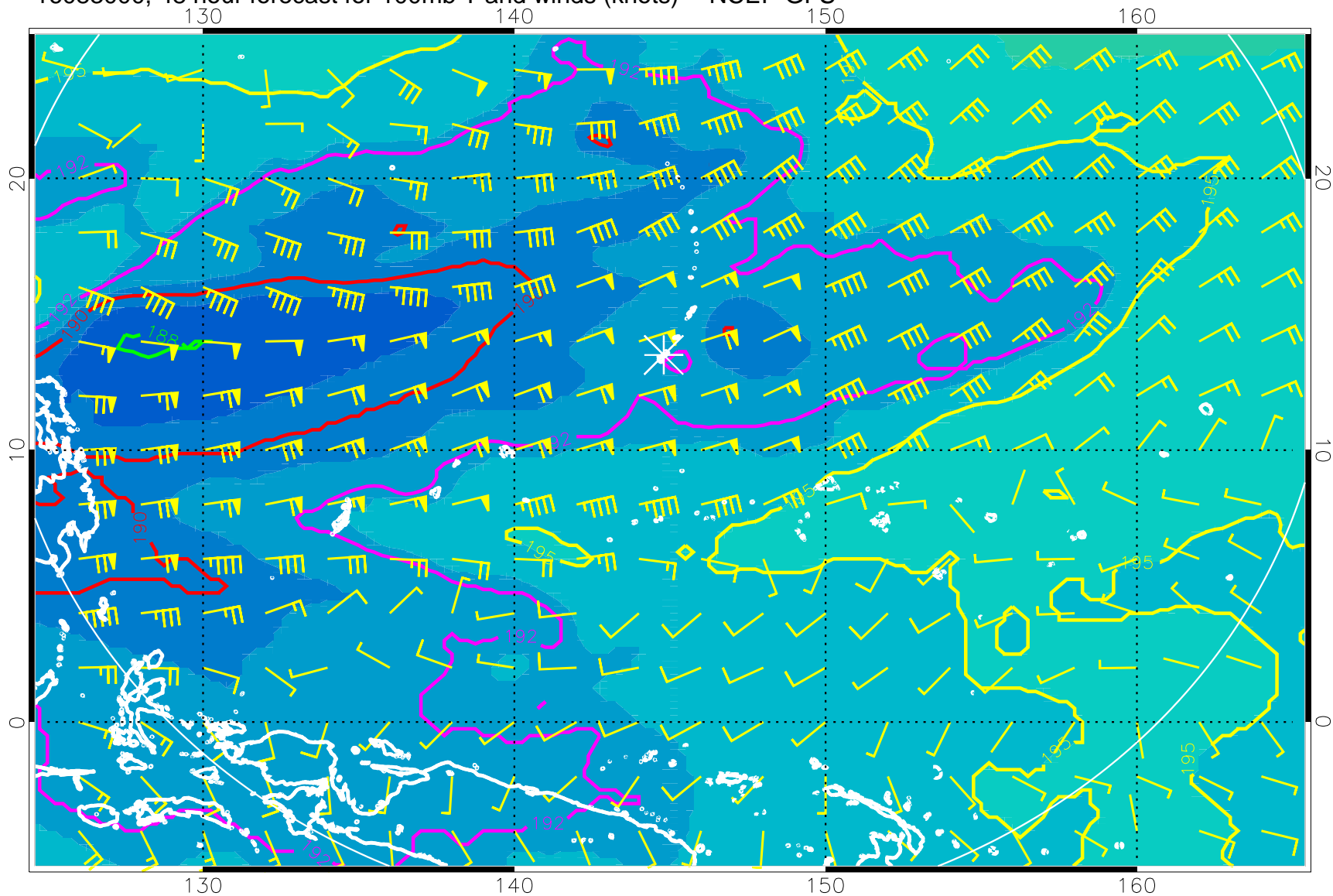
16083000, 48 hour forecast for 100mb T and winds (knots) -- NCEP GFS
