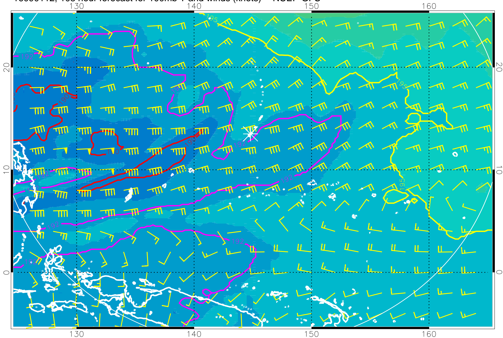
16090112, 108 hour forecast for 100mb T and winds (knots) -- NCEP GFS
