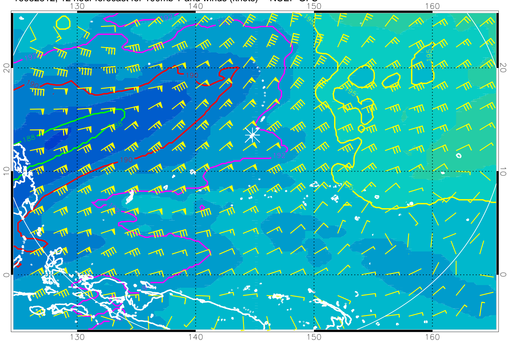
16082812, 12 hour forecast for 100mb T and winds (knots) -- NCEP GFS
