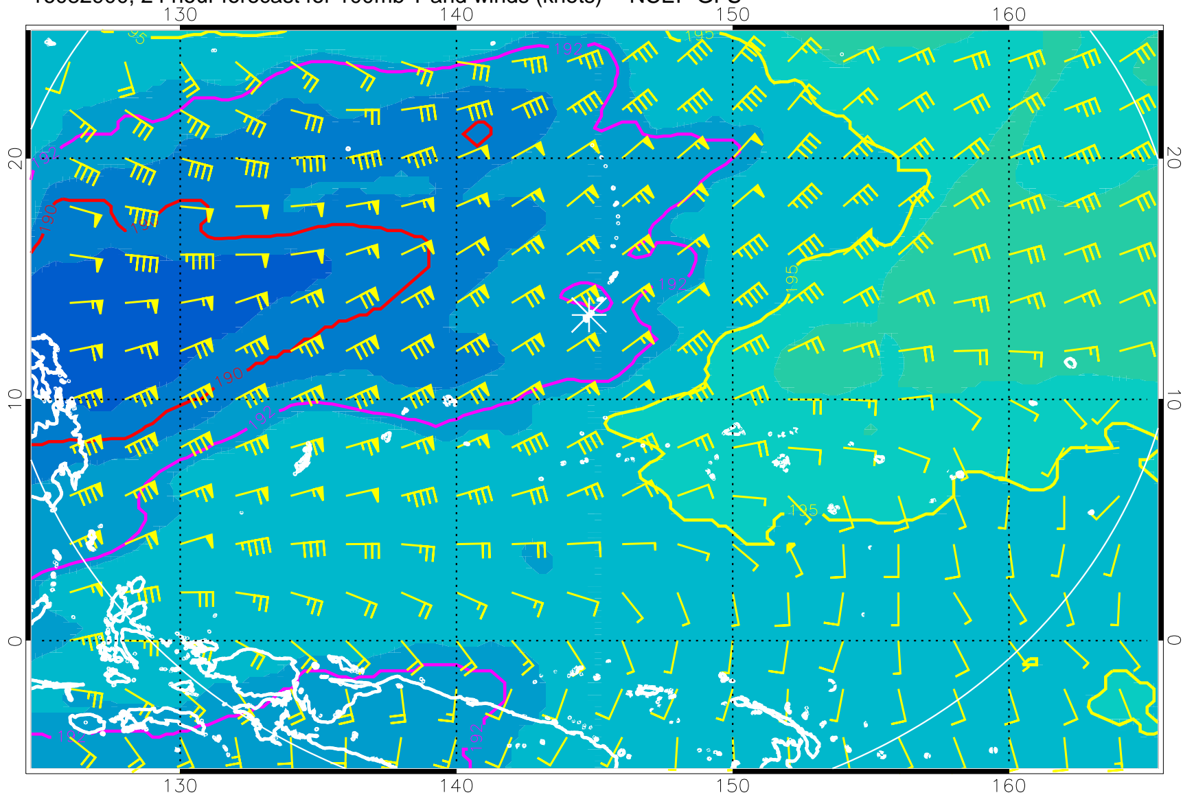
16082900, 24 hour forecast for 100mb T and winds (knots) -- NCEP GFS
