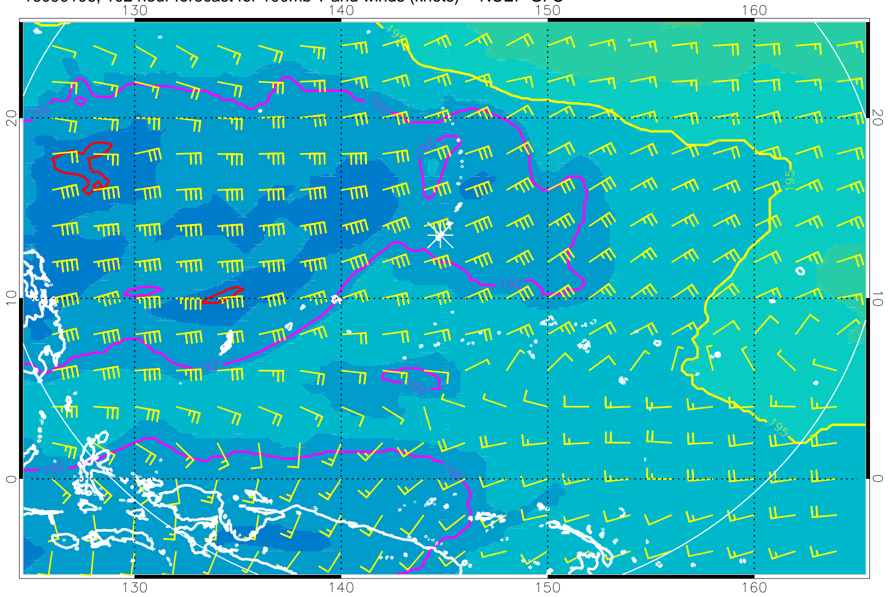
16090106, 102 hour forecast for 100mb T and winds (knots) -- NCEP GFS
