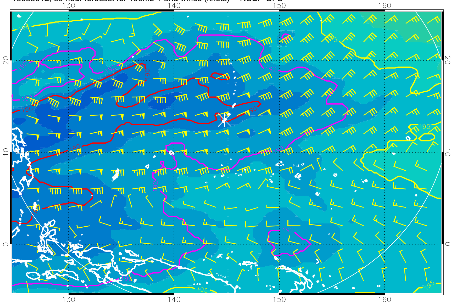
16083012, 60 hour forecast for 100mb T and winds (knots) -- NCEP GFS
