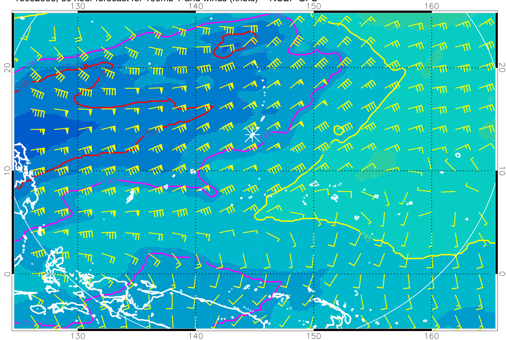
16082906, 30 hour forecast for 100mb T and winds (knots) -- NCEP GFS
