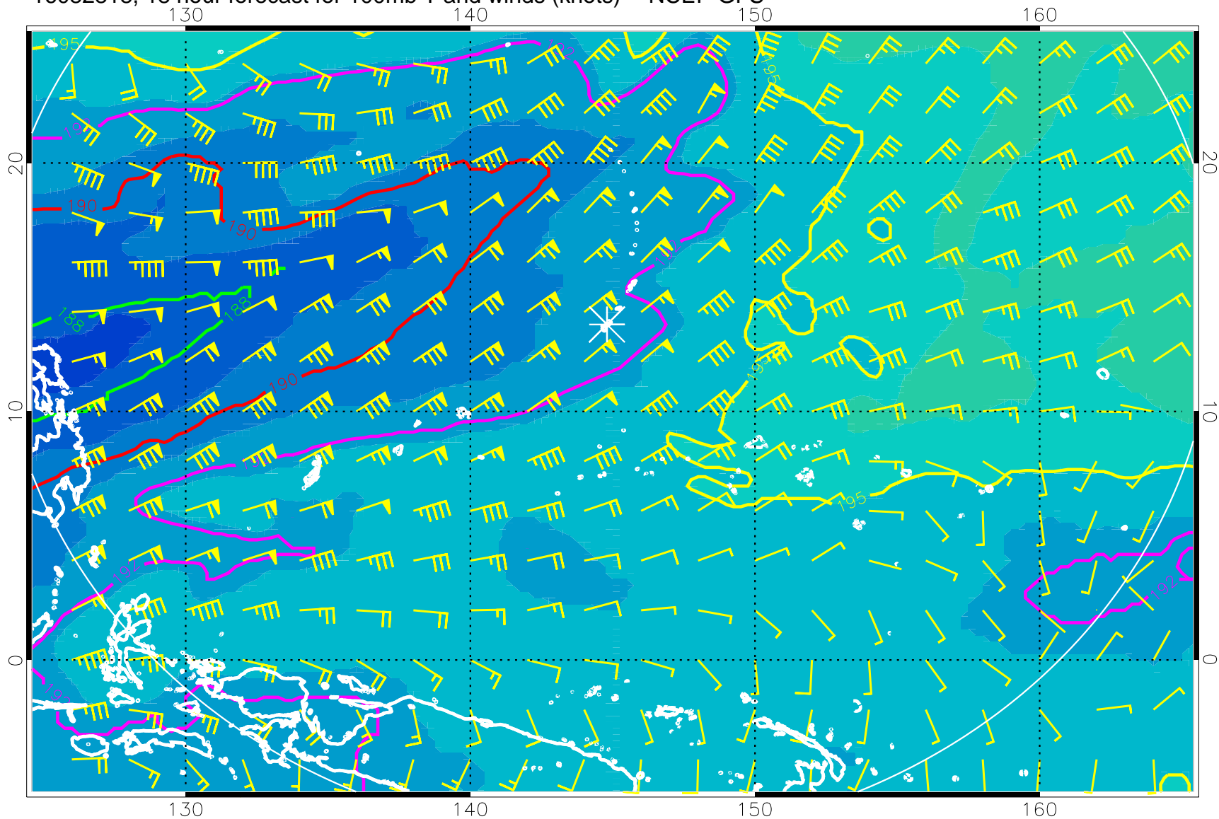
16082818, 18 hour forecast for 100mb T and winds (knots) -- NCEP GFS
