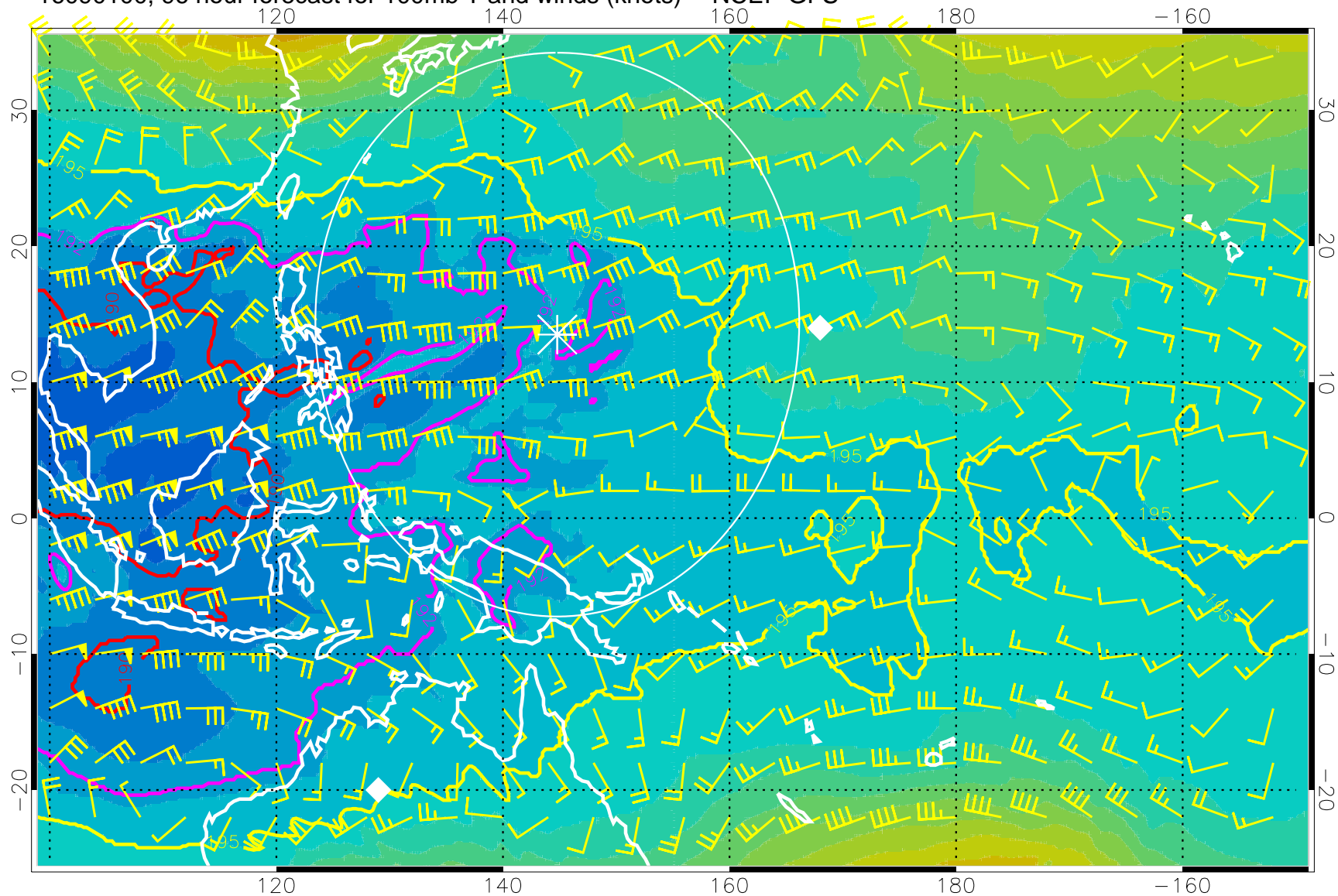
16090100, 96 hour forecast for 100mb T and winds (knots) -- NCEP GFS
