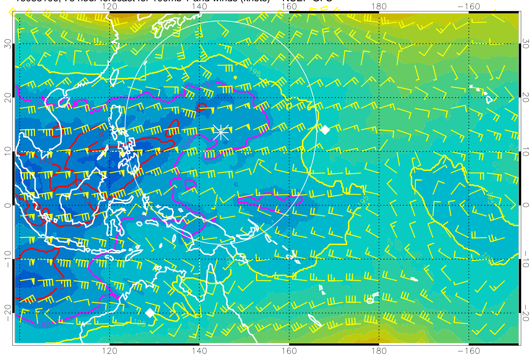
16083106, 78 hour forecast for 100mb T and winds (knots) -- NCEP GFS
