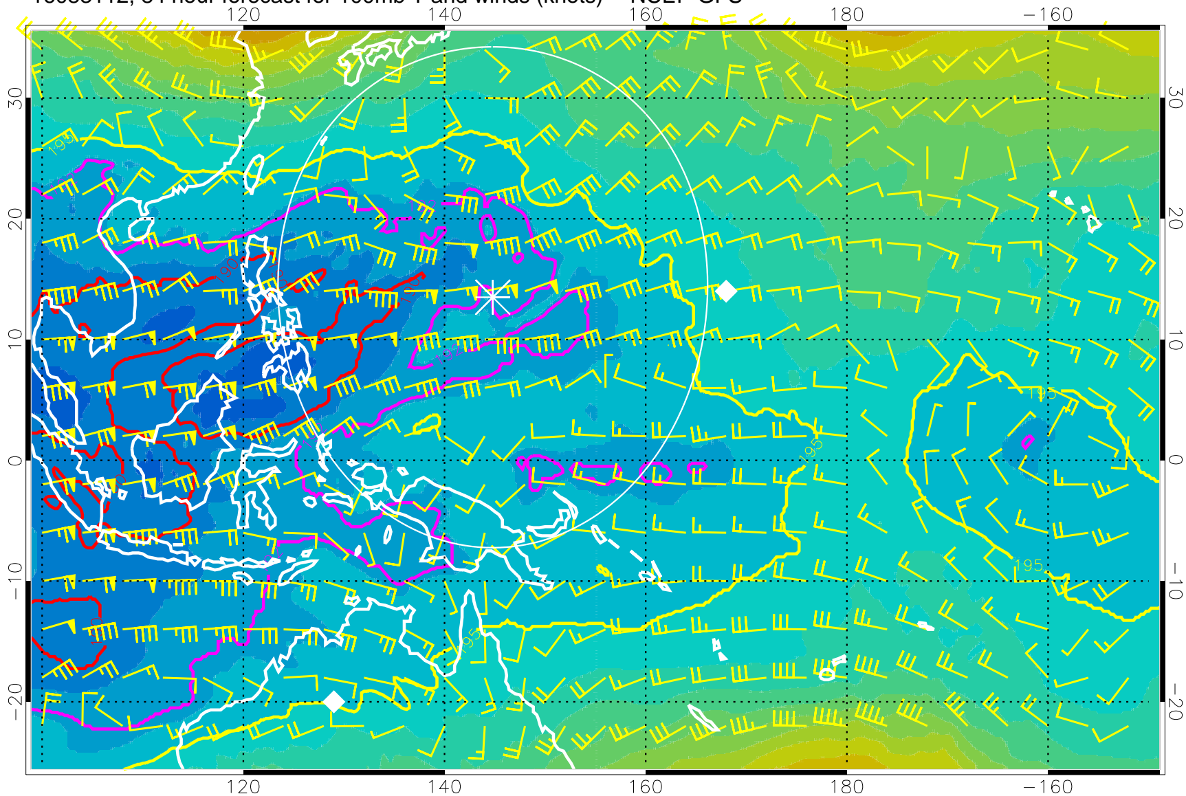
16083112, 84 hour forecast for 100mb T and winds (knots) -- NCEP GFS
