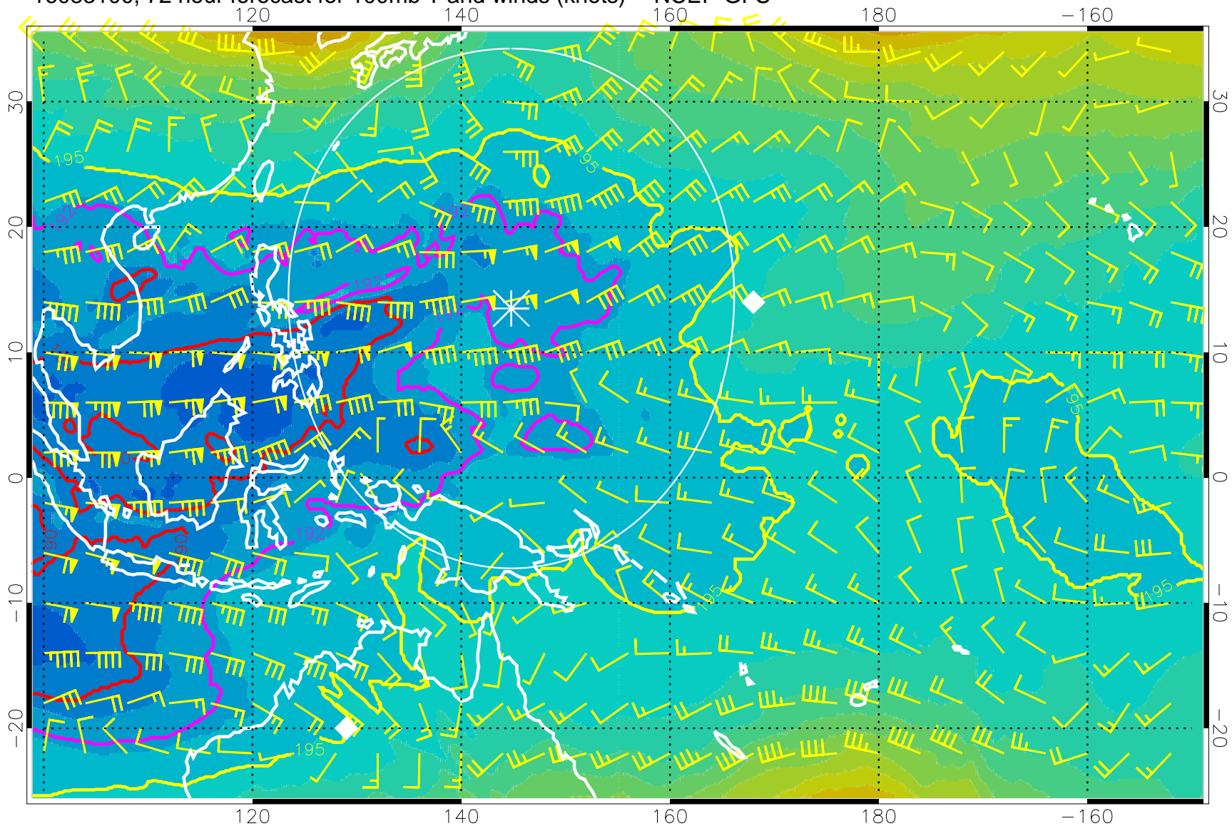
16083100, 72 hour forecast for 100mb T and winds (knots) -- NCEP GFS
