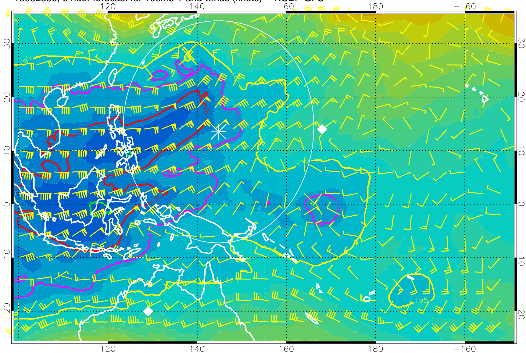
16082806, 6 hour forecast for 100mb T and winds (knots) -- NCEP GFS
