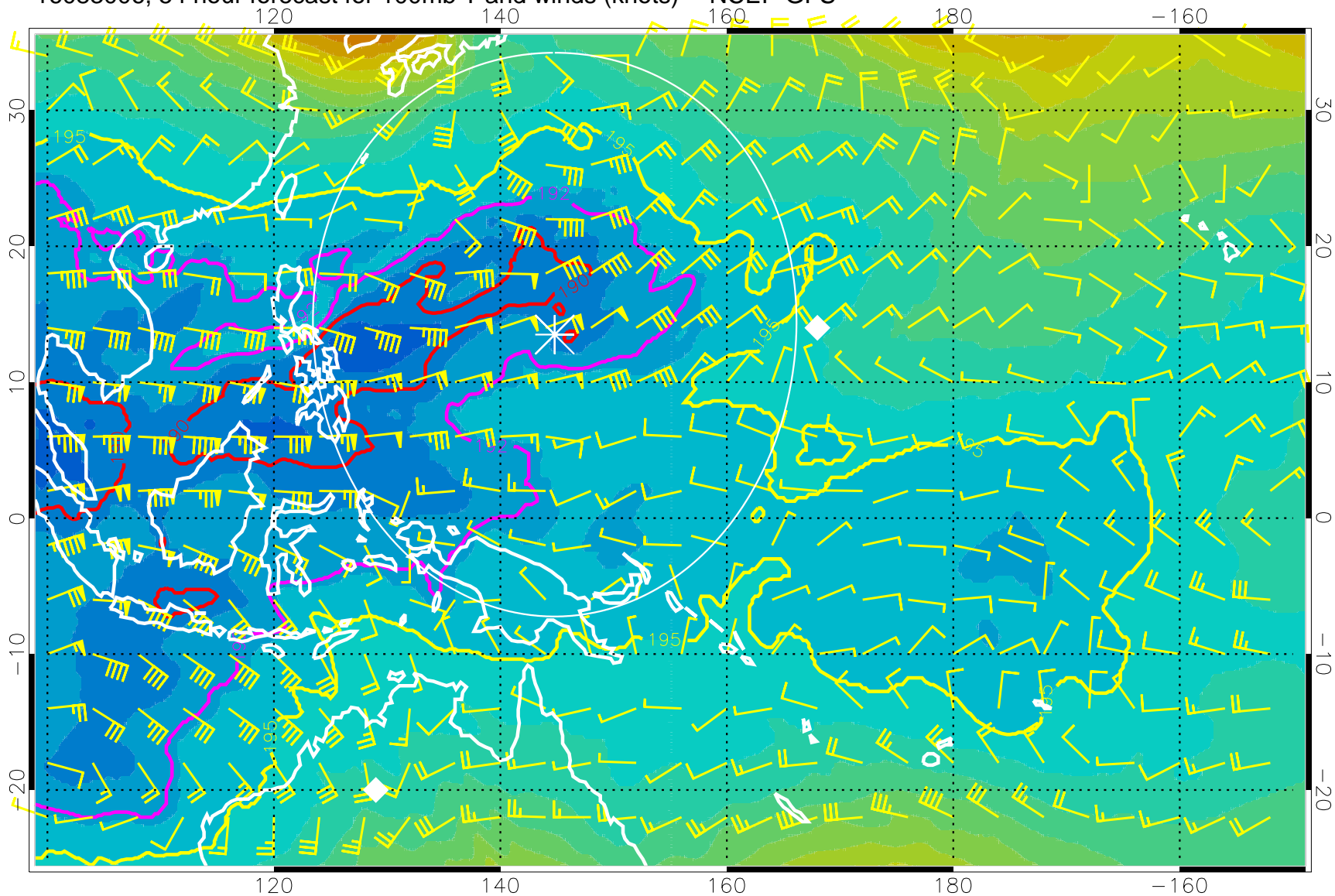
16083006, 54 hour forecast for 100mb T and winds (knots) -- NCEP GFS
