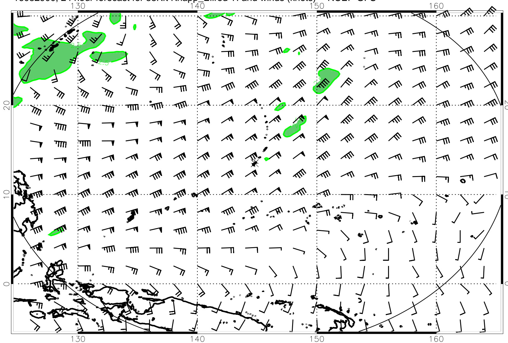
16082900, 24 hour forecast for 53Kft Knapp_Ellrod TI and winds (knots) -- NCEP GFS
