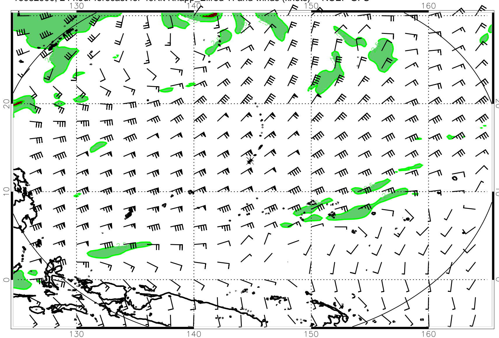
16082900, 24 hour forecast for 49Kft Knapp_Ellrod TI and winds (knots) -- NCEP GFS
