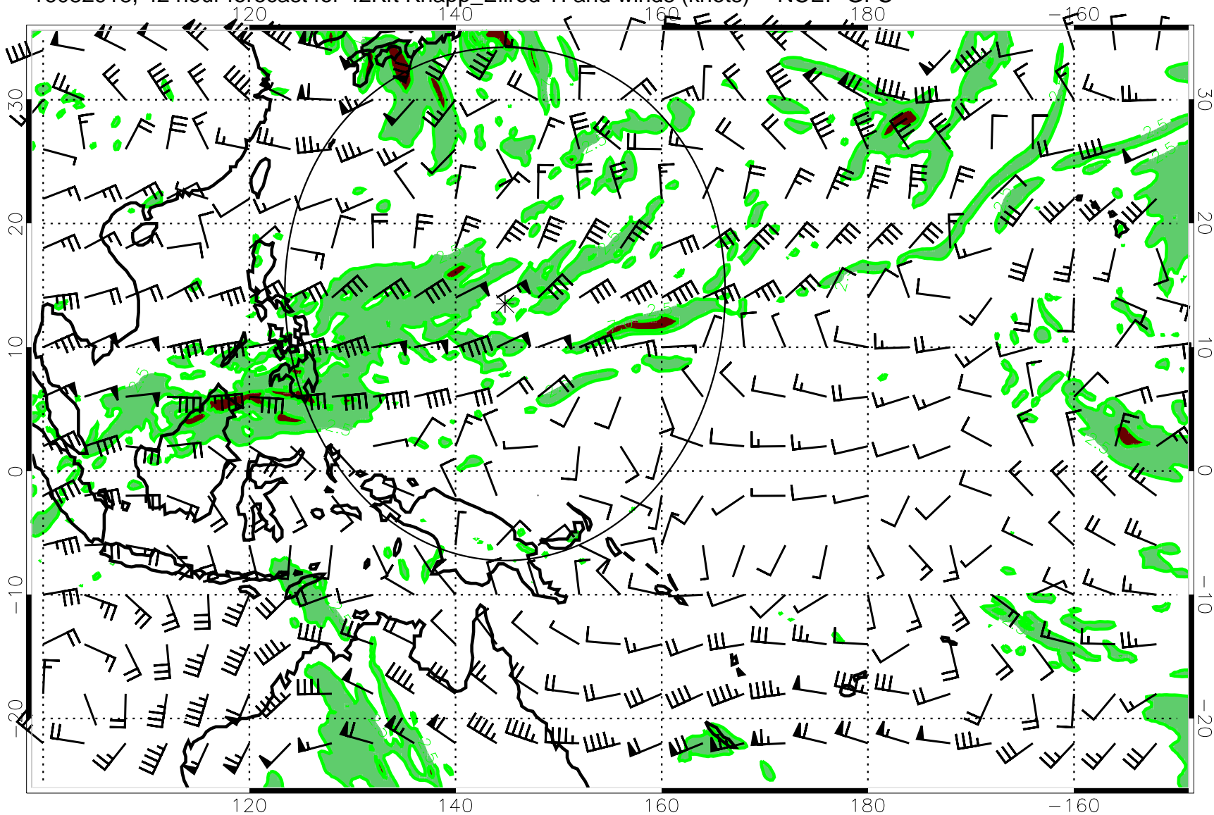
16082918, 42 hour forecast for 42Kft Knapp_Ellrod TI and winds (knots) -- NCEP GFS
