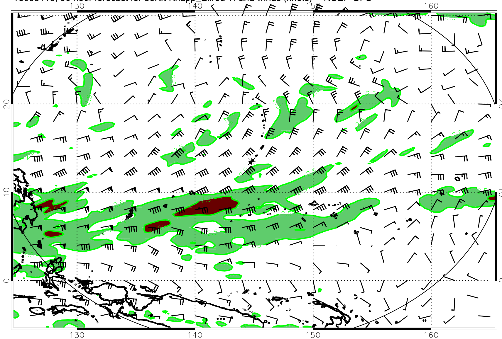
16083118, 90 hour forecast for 36Kft Knapp_Ellrod TI and winds (knots) -- NCEP GFS
