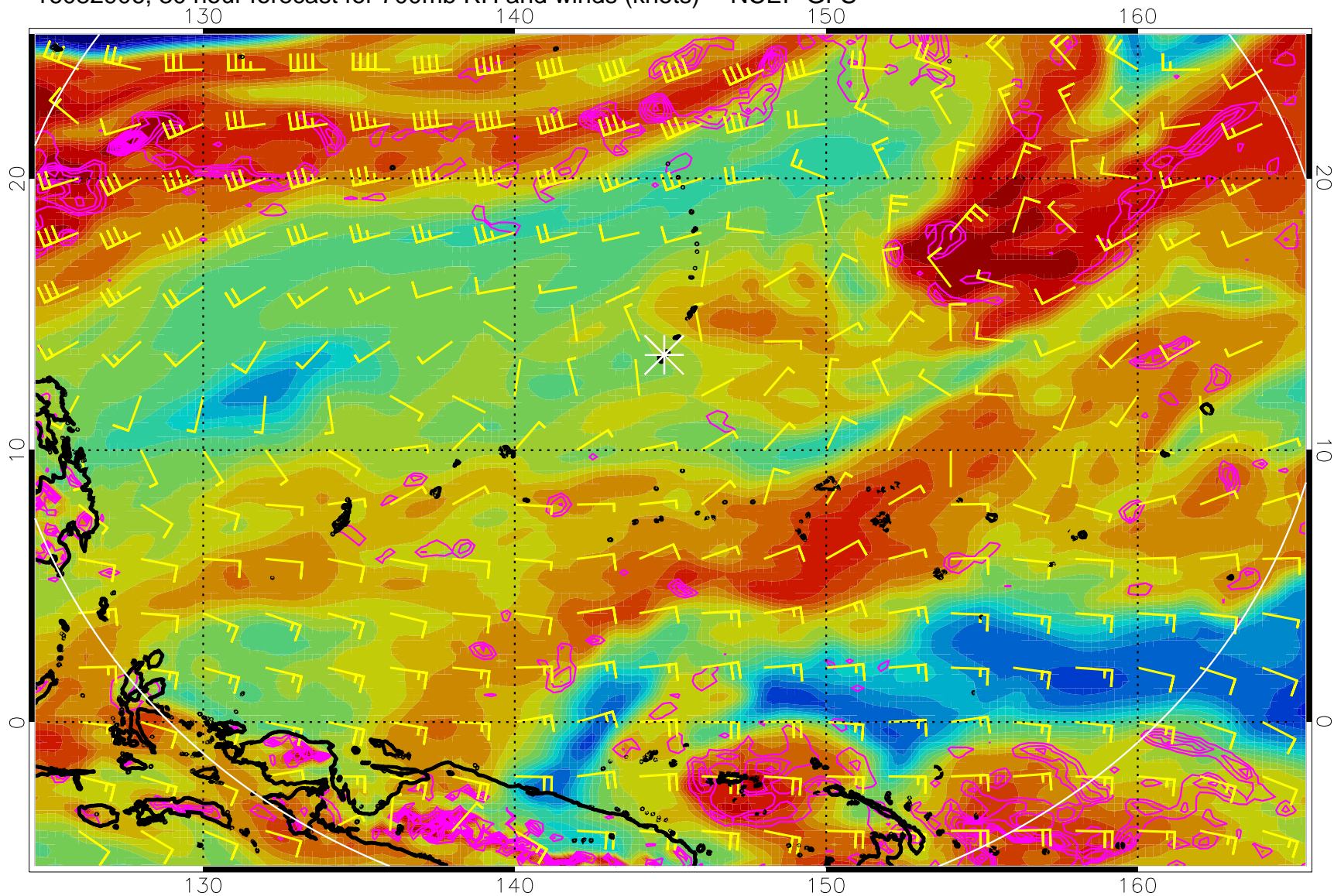
16082906, 30 hour forecast for 700mb RH and winds (knots) -- NCEP GFS
