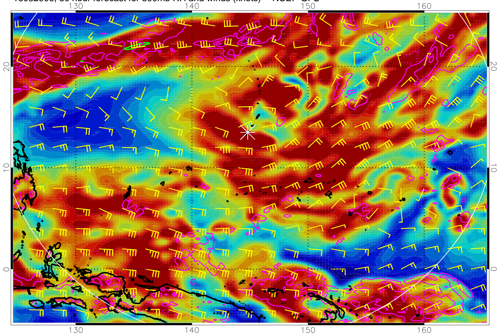
16082906, 30 hour forecast for 300mb RH and winds (knots) -- NCEP GFS
