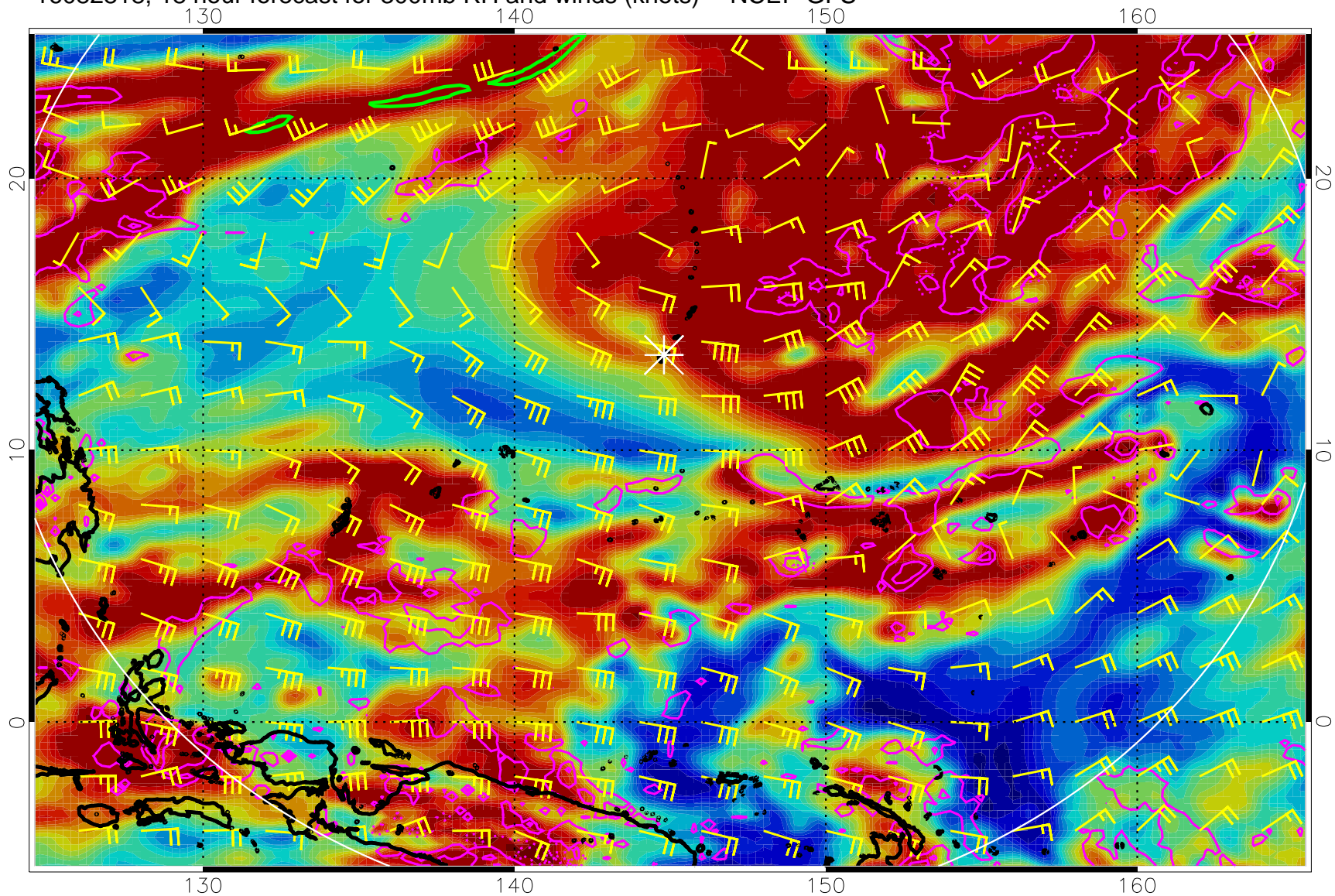
16082818, 18 hour forecast for 300mb RH and winds (knots) -- NCEP GFS
