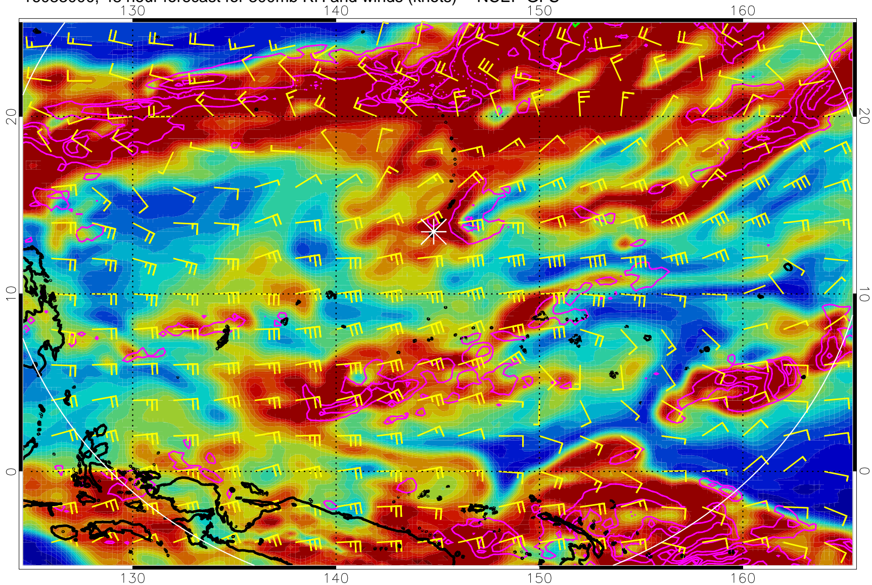
16083000, 48 hour forecast for 300mb RH and winds (knots) -- NCEP GFS
