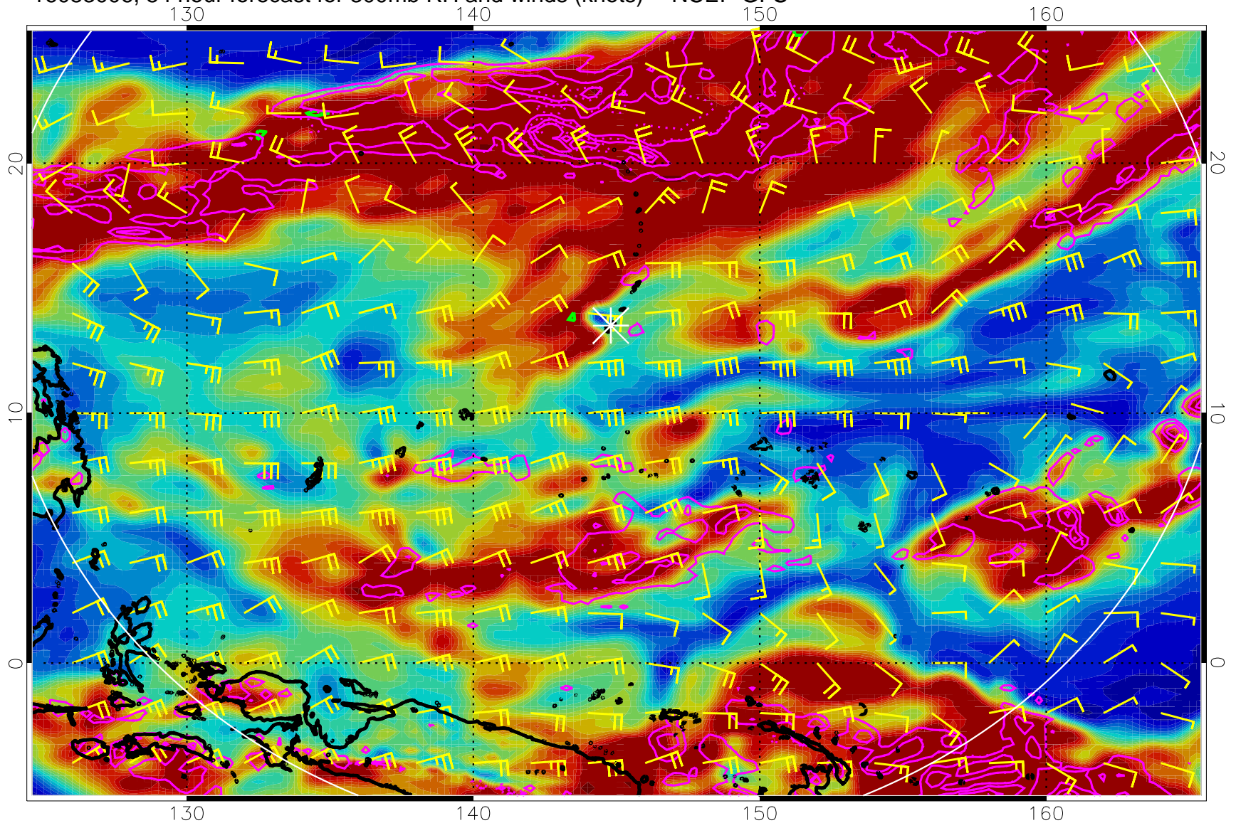
16083006, 54 hour forecast for 300mb RH and winds (knots) -- NCEP GFS
