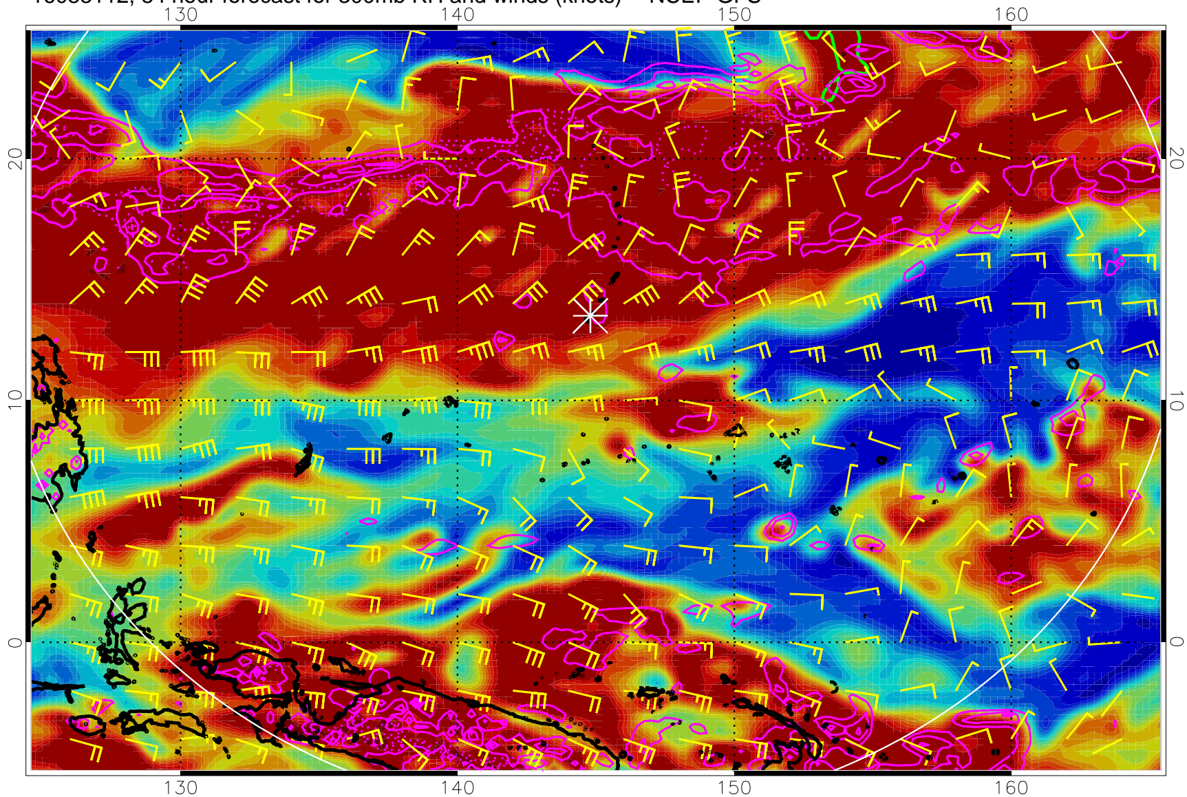
16083112, 84 hour forecast for 300mb RH and winds (knots) -- NCEP GFS
