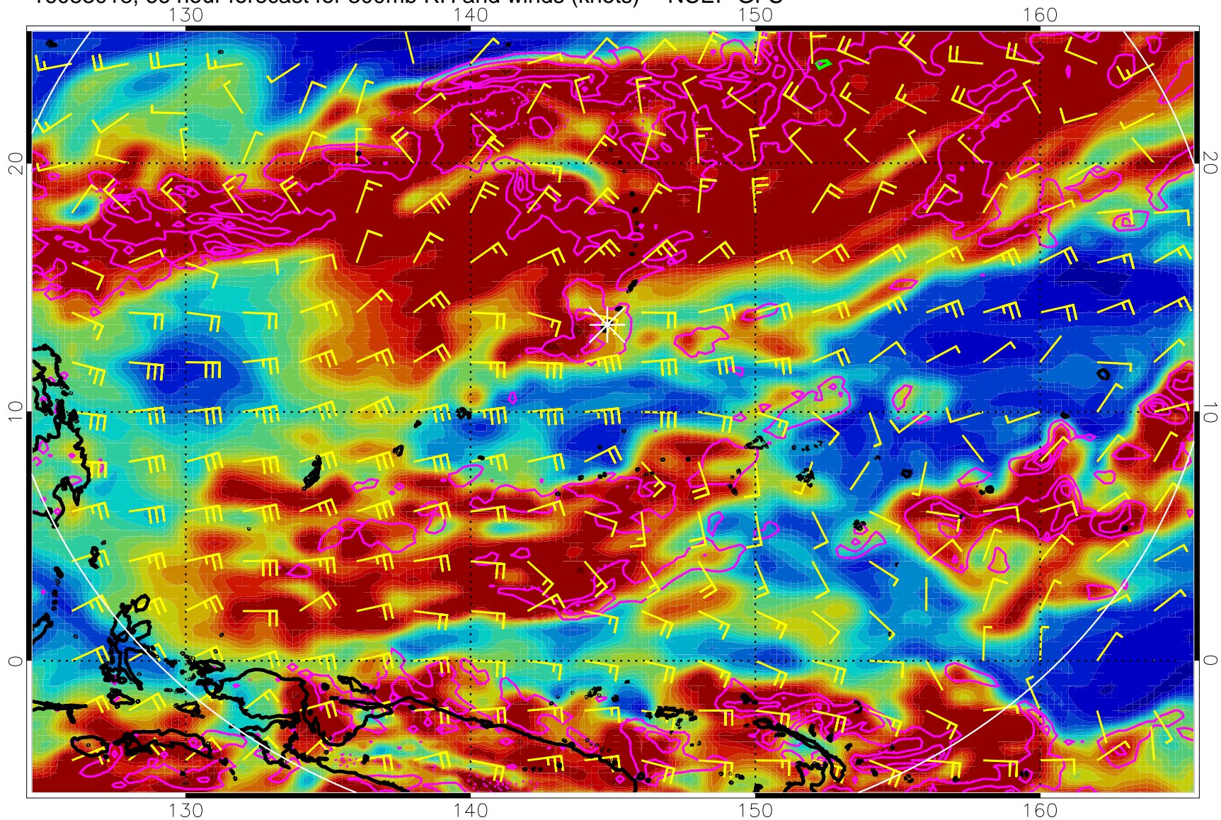
16083018, 66 hour forecast for 300mb RH and winds (knots) -- NCEP GFS
