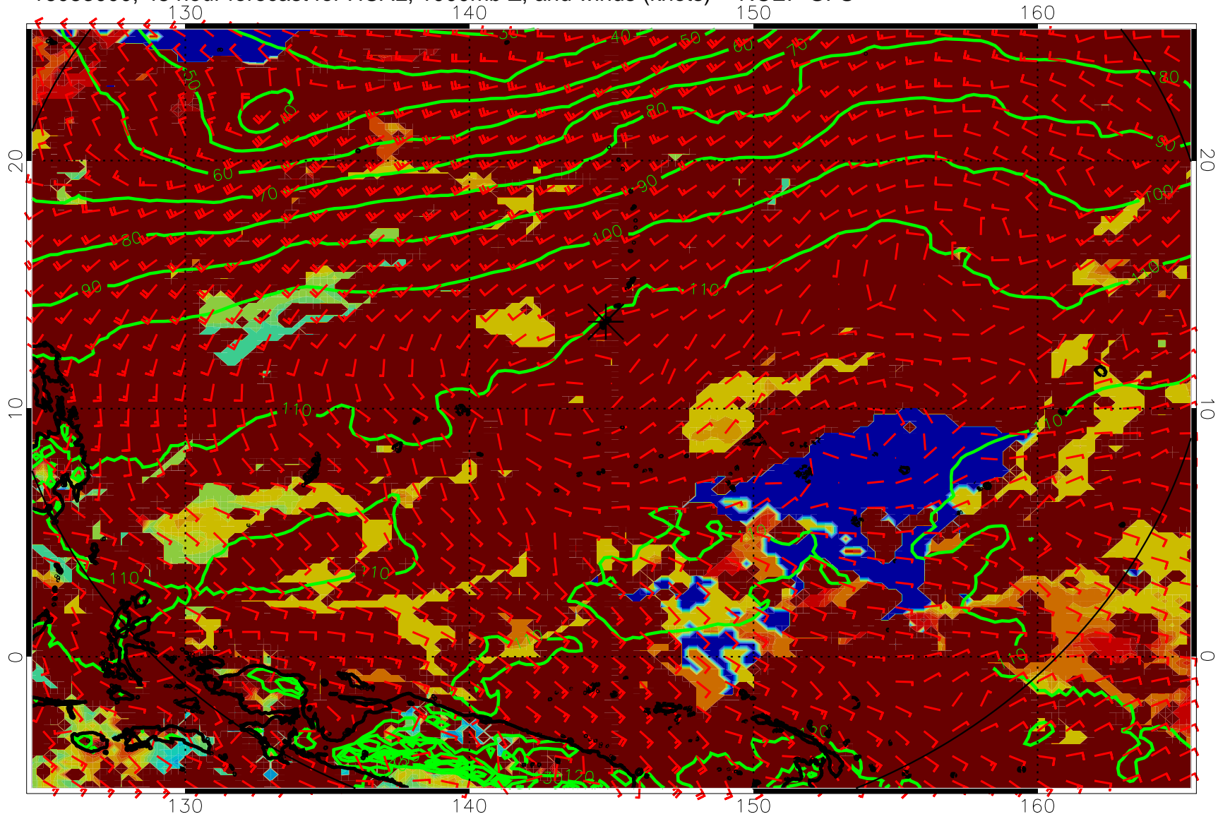
16083000, 48 hour forecast for HCAL, 1000mb Z, and winds (knots) -- NCEP GFS
