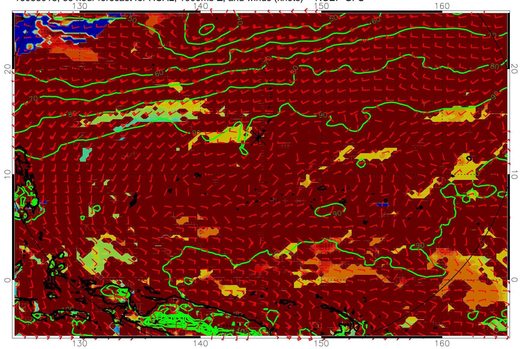
16083018, 66 hour forecast for HCAL, 1000mb Z, and winds (knots) -- NCEP GFS
