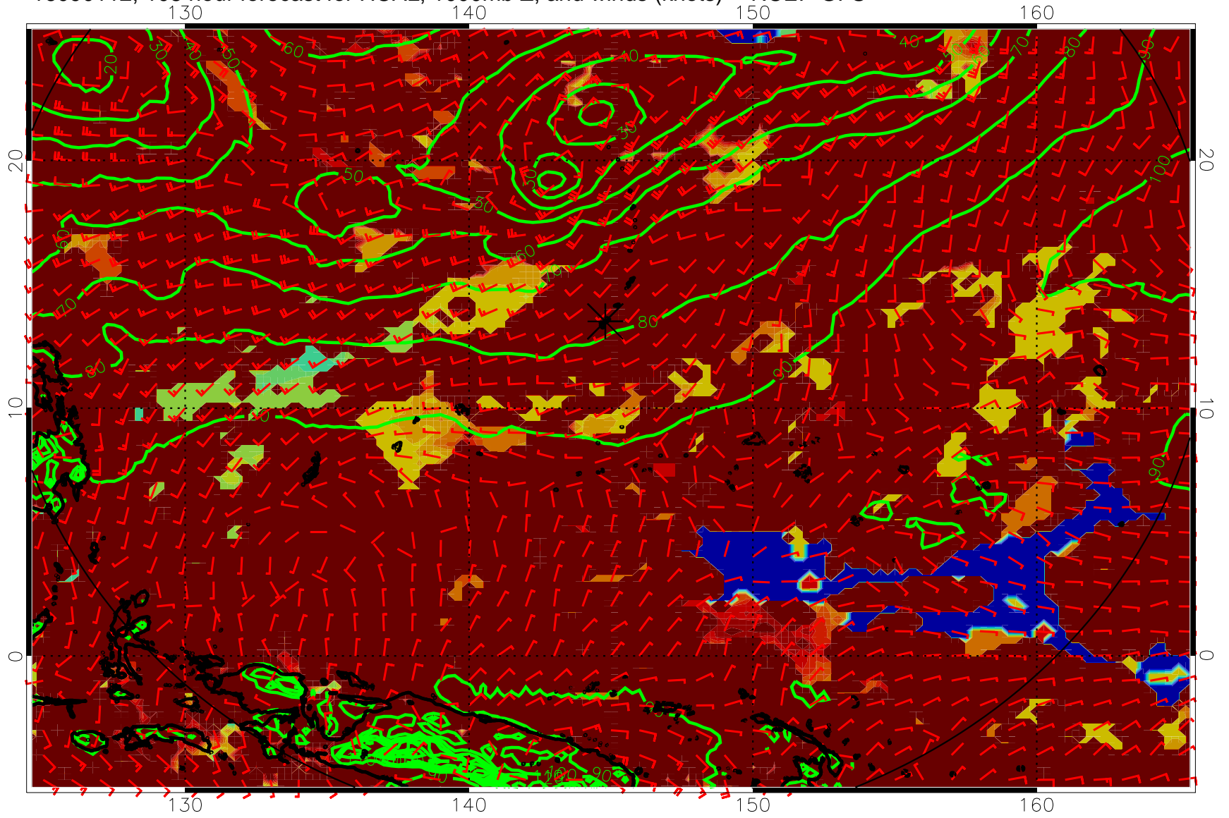
16090112, 108 hour forecast for HCAL, 1000mb Z, and winds (knots) -- NCEP GFS
