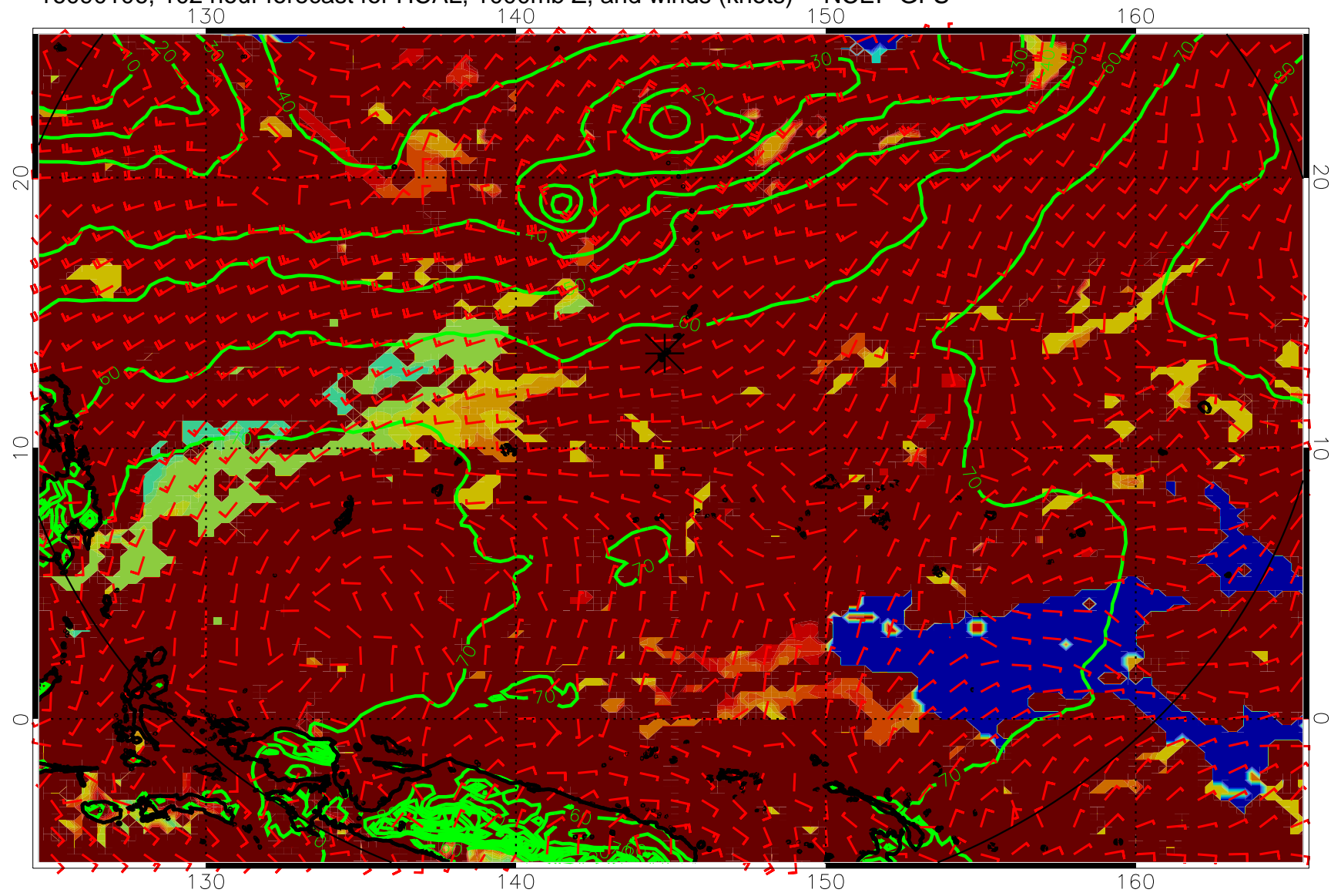
16090106, 102 hour forecast for HCAL, 1000mb Z, and winds (knots) -- NCEP GFS
