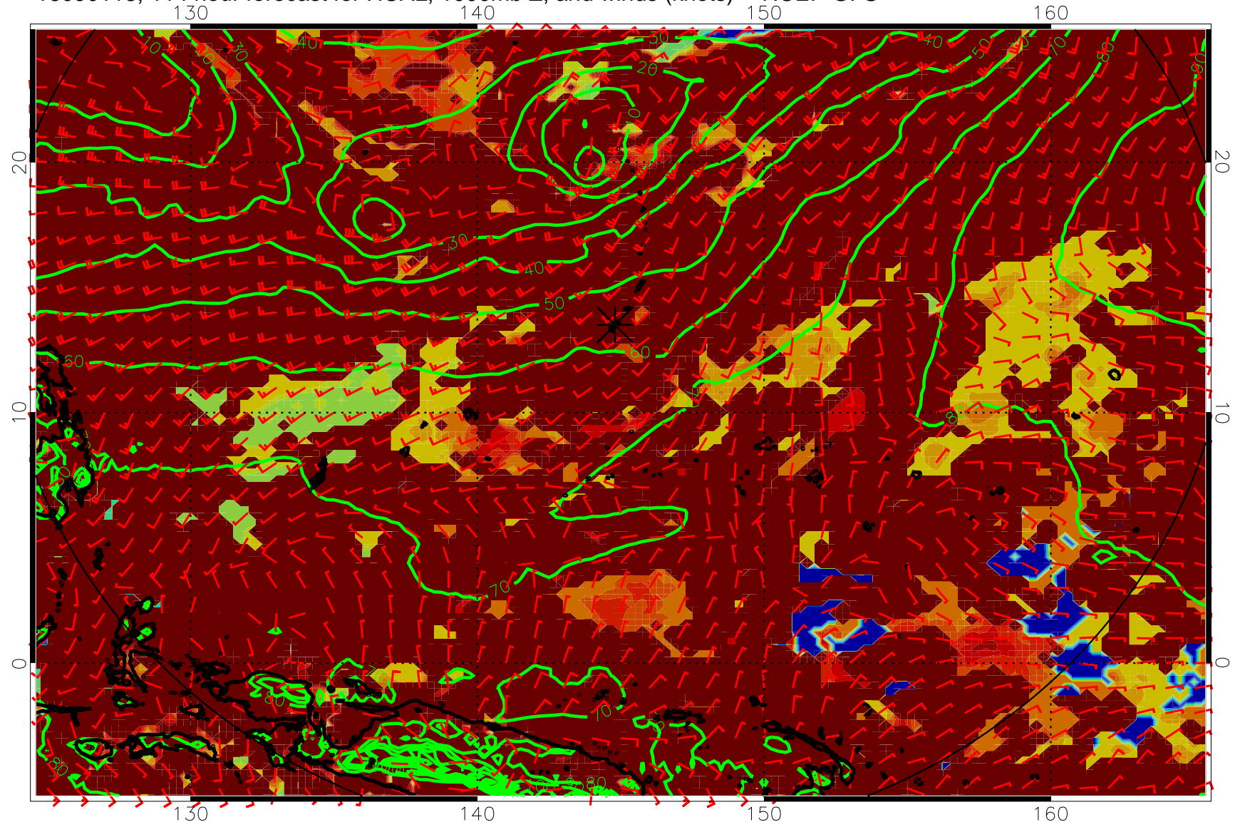
16090118, 114 hour forecast for HCAL, 1000mb Z, and winds (knots) -- NCEP GFS
