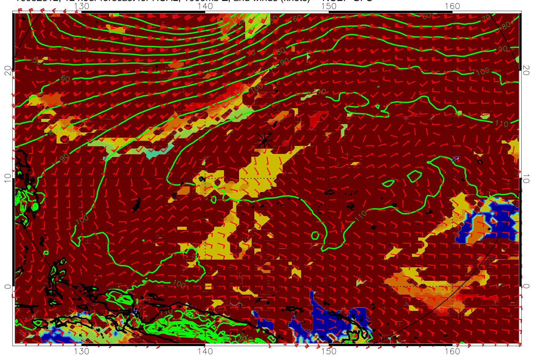
16082812, 12 hour forecast for HCAL, 1000mb Z, and winds (knots) -- NCEP GFS
