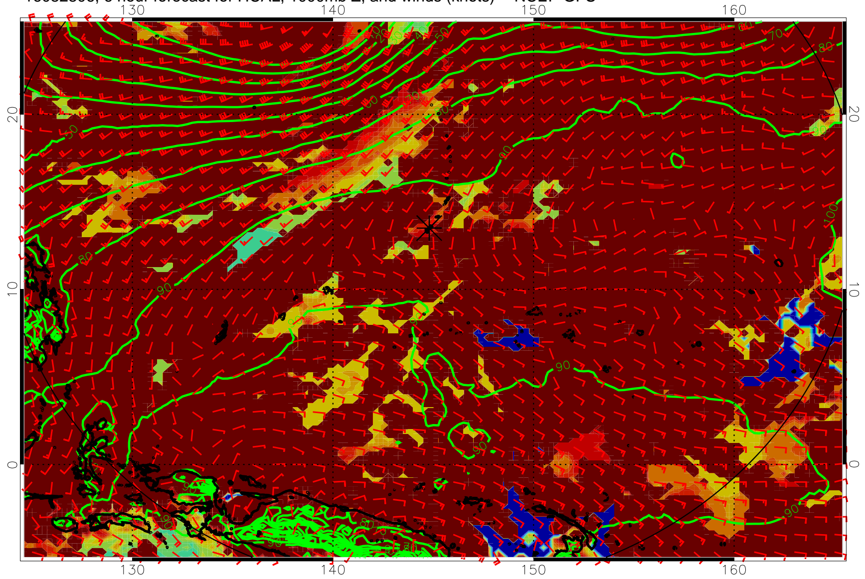
16082806, 6 hour forecast for HCAL, 1000mb Z, and winds (knots) -- NCEP GFS
