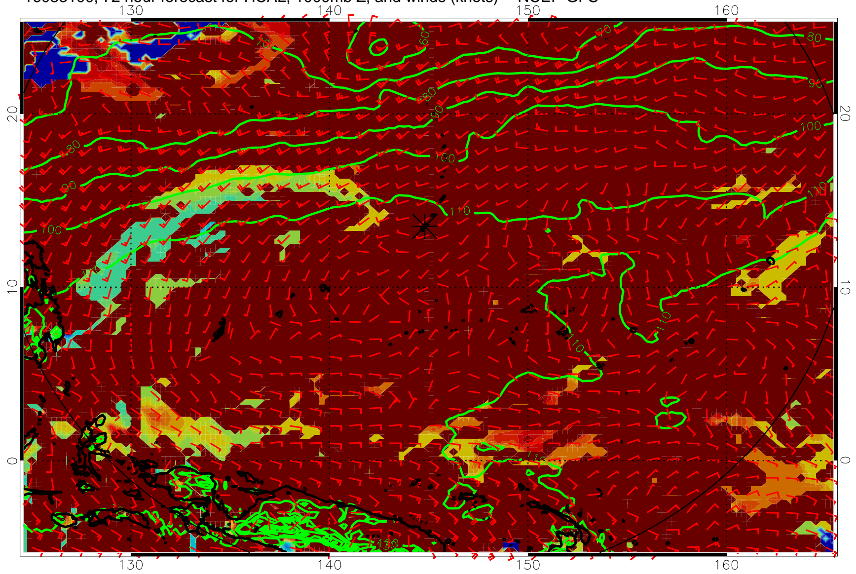
16083100, 72 hour forecast for HCAL, 1000mb Z, and winds (knots) -- NCEP GFS
