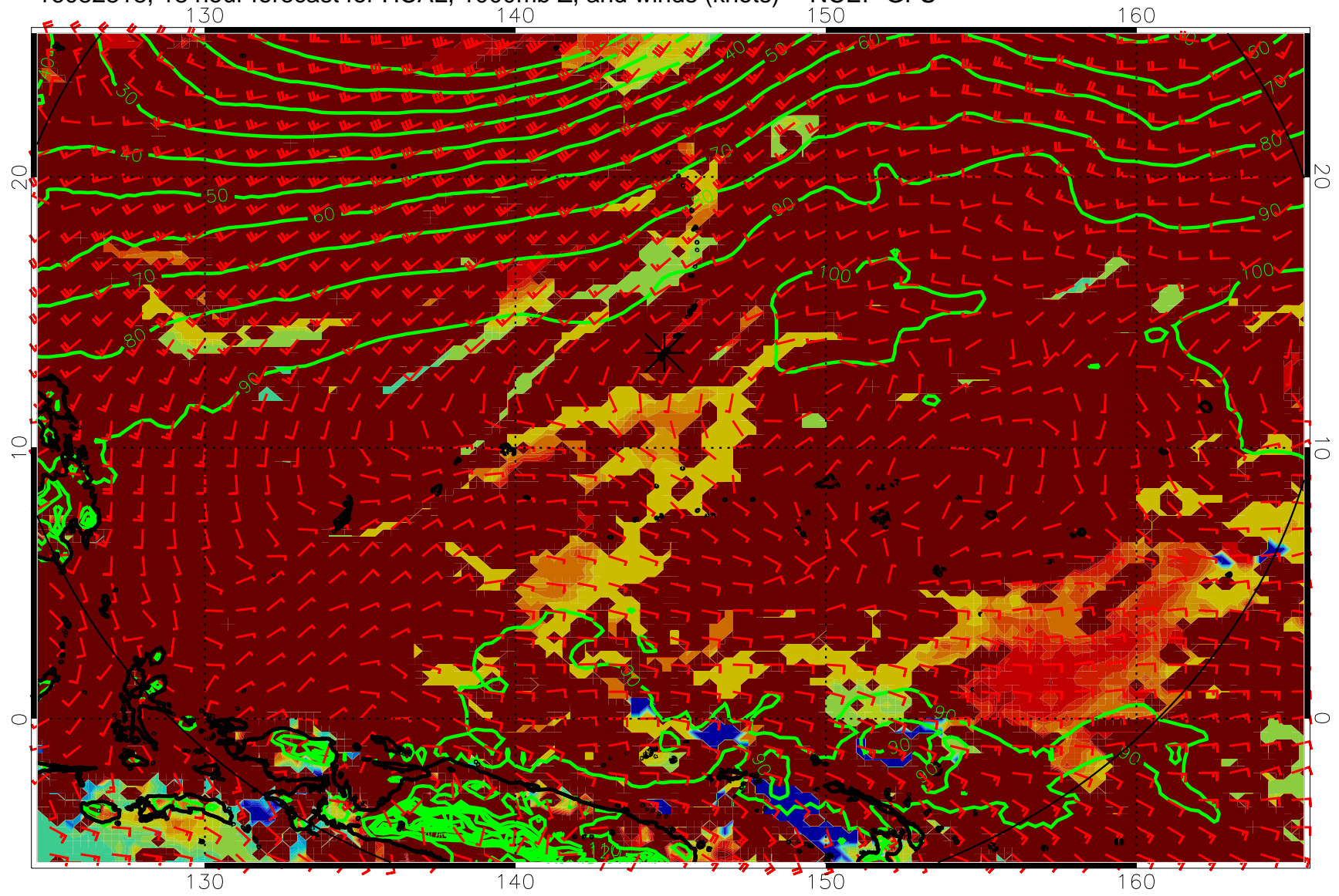
16082818, 18 hour forecast for HCAL, 1000mb Z, and winds (knots) -- NCEP GFS
