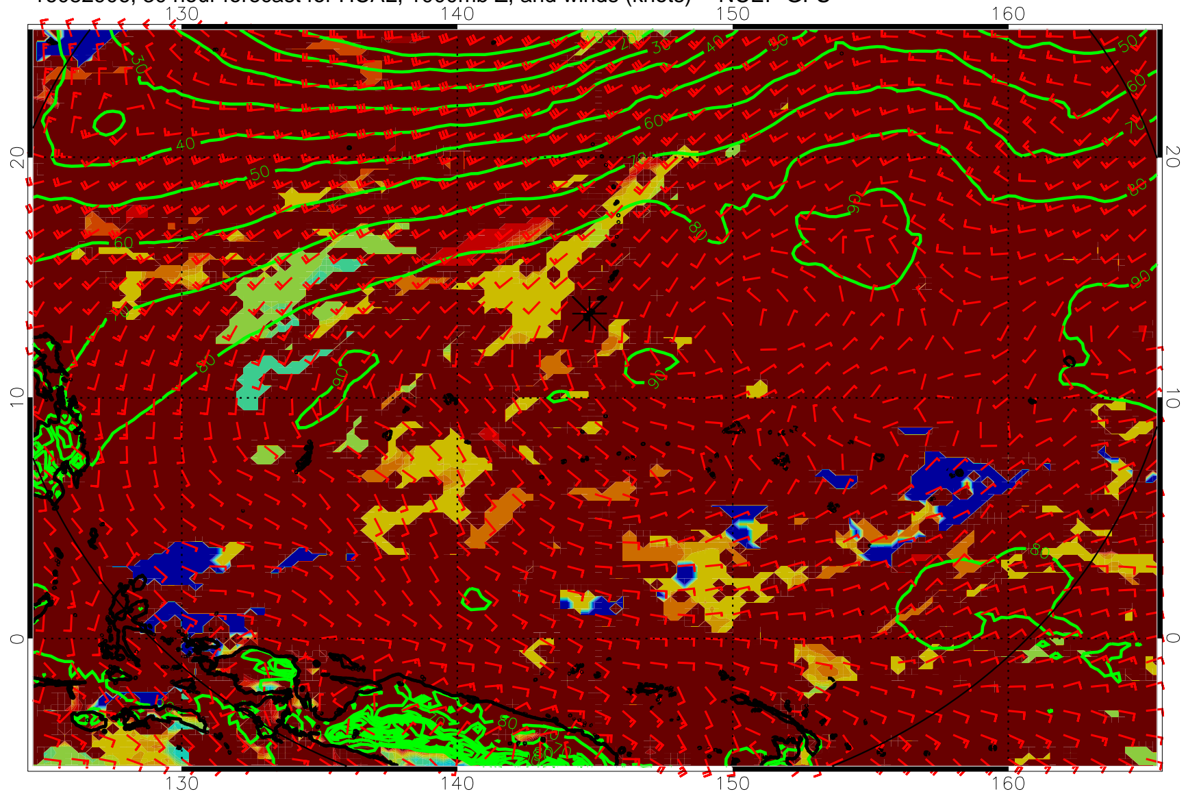
16082906, 30 hour forecast for HCAL, 1000mb Z, and winds (knots) -- NCEP GFS
