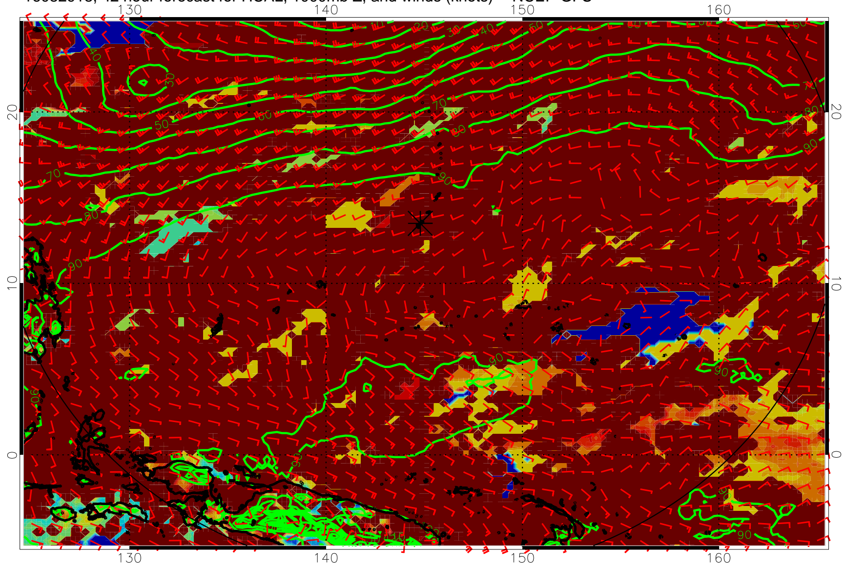
16082918, 42 hour forecast for HCAL, 1000mb Z, and winds (knots) -- NCEP GFS
