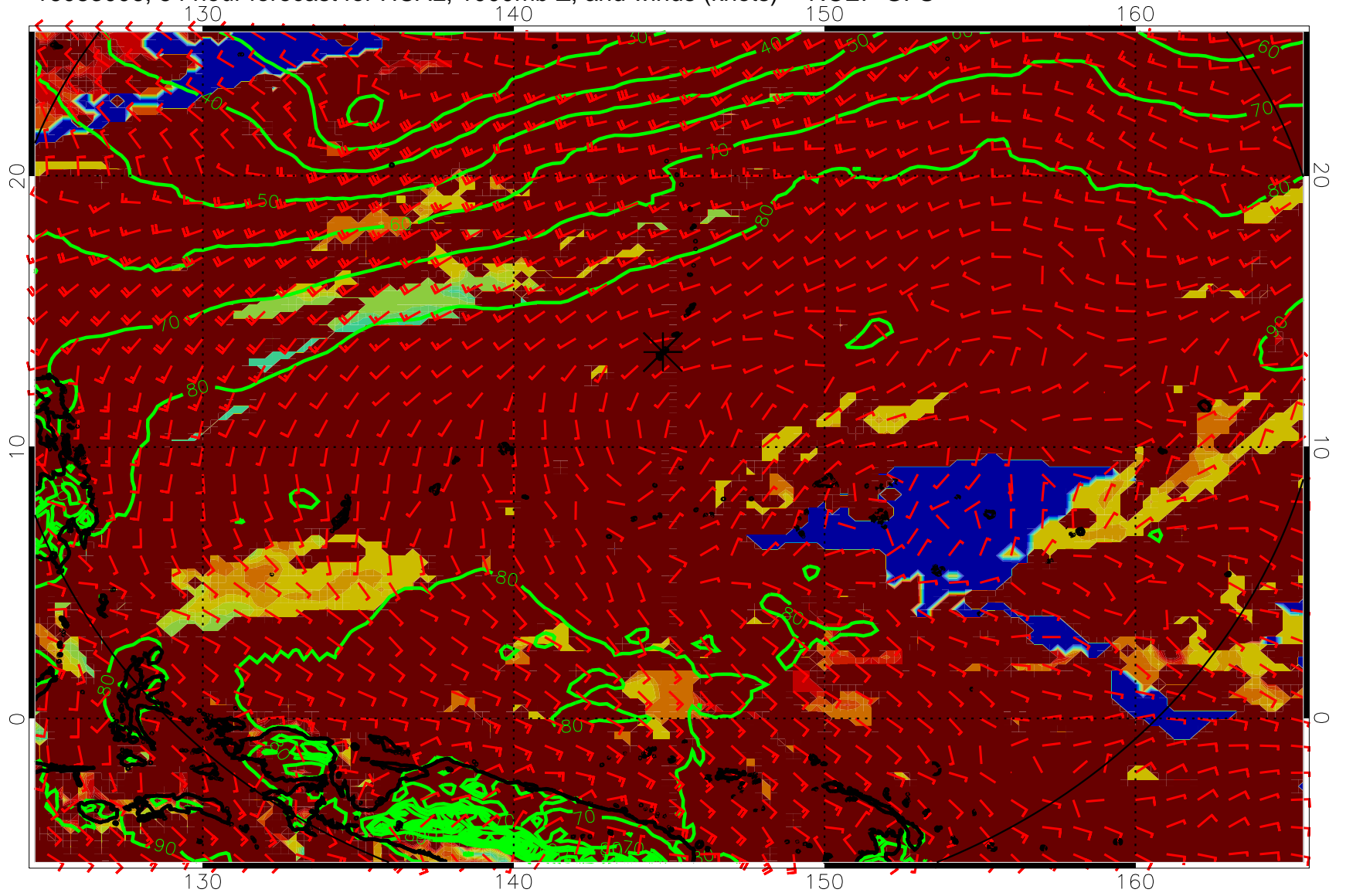
16083006, 54 hour forecast for HCAL, 1000mb Z, and winds (knots) -- NCEP GFS
