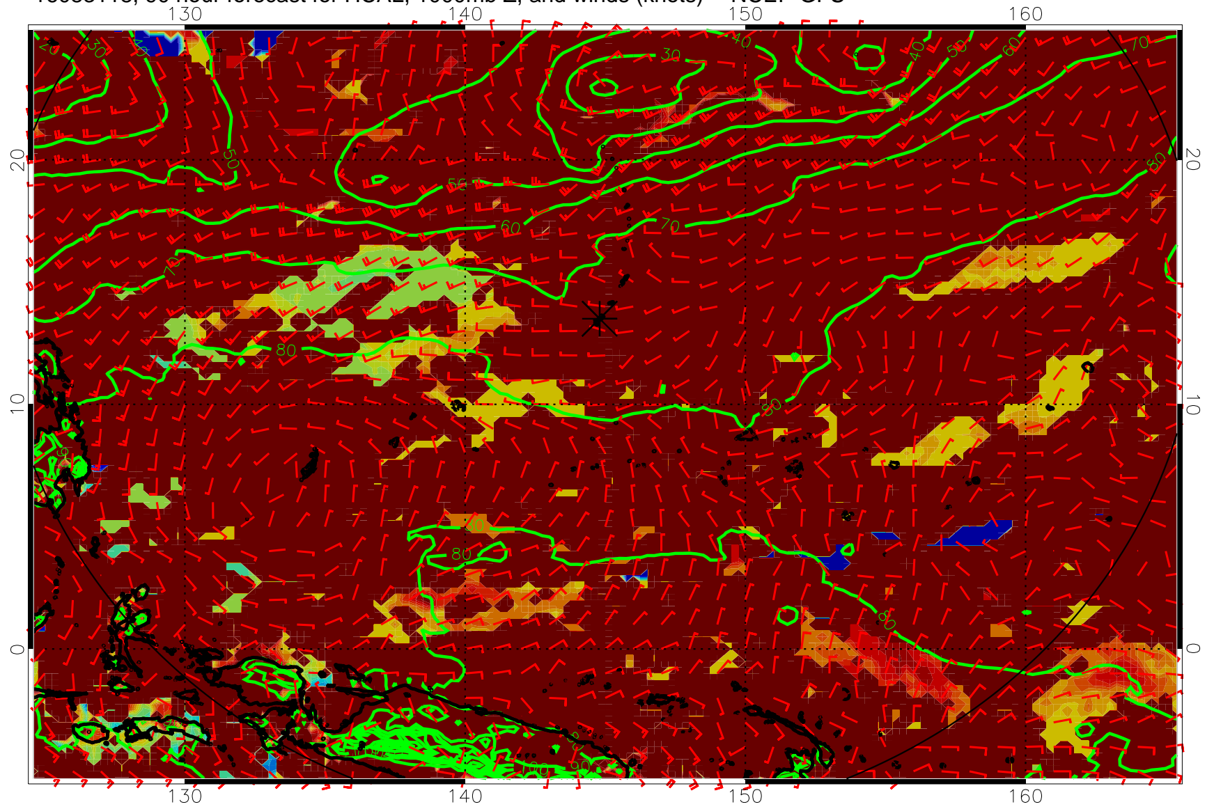
16083118, 90 hour forecast for HCAL, 1000mb Z, and winds (knots) -- NCEP GFS
