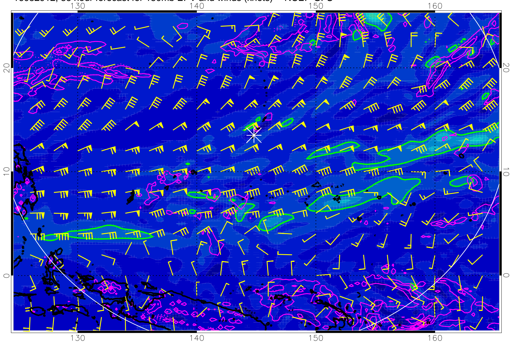
16082912, 36 hour forecast for 150mb EPV and winds (knots) -- NCEP GFS
