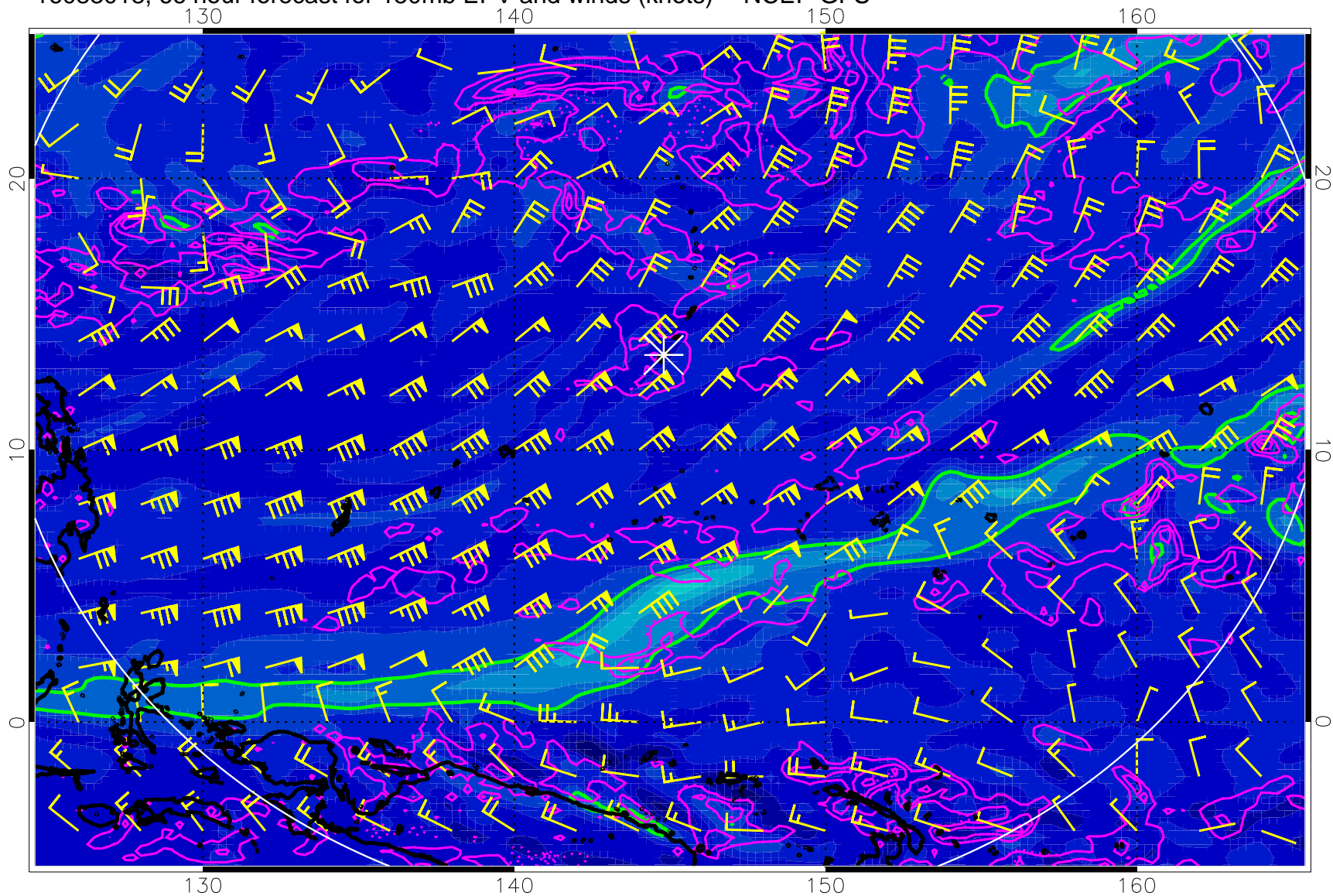
16083018, 66 hour forecast for 150mb EPV and winds (knots) -- NCEP GFS
