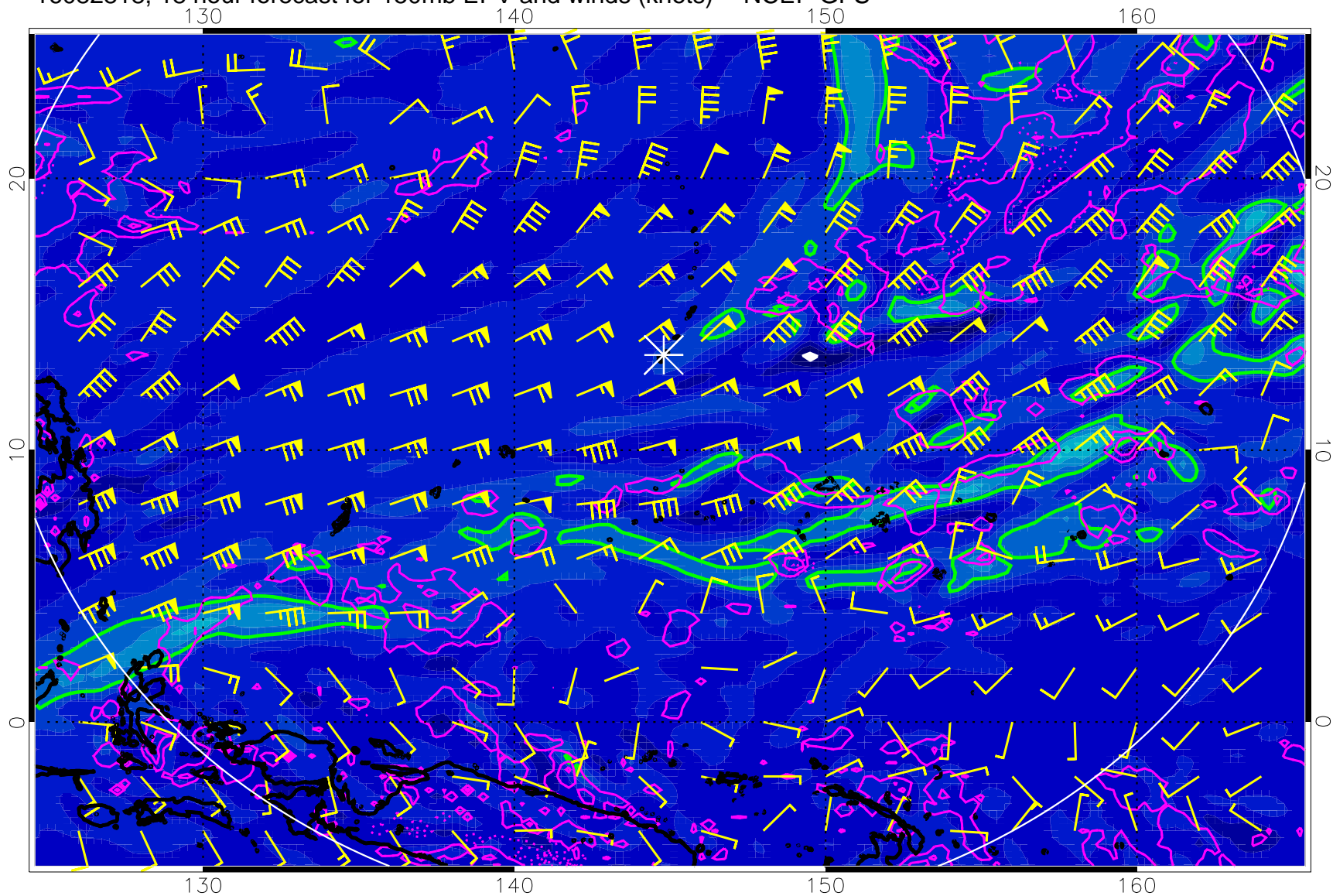
16082818, 18 hour forecast for 150mb EPV and winds (knots) -- NCEP GFS
