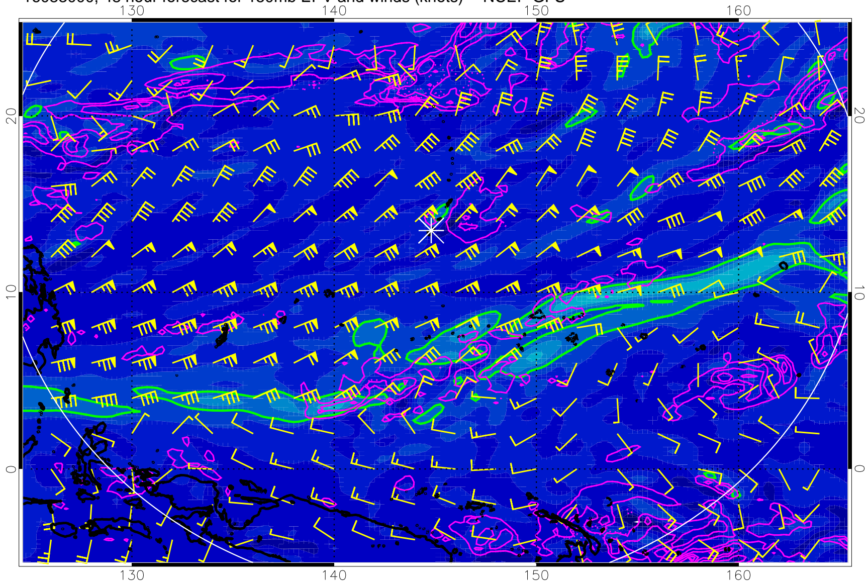
16083000, 48 hour forecast for 150mb EPV and winds (knots) -- NCEP GFS
