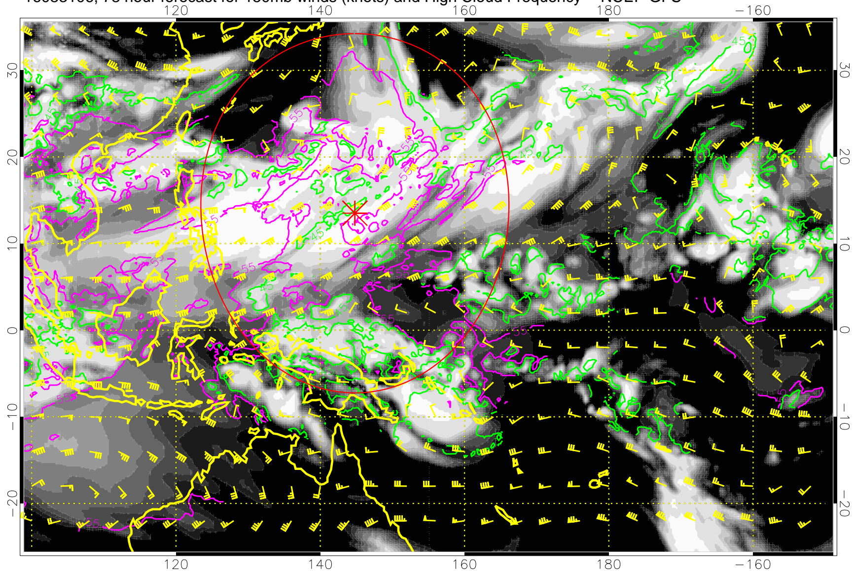
16083106, 78 hour forecast for 150mb winds (knots) and High Cloud Frequency -- NCEP GFS
