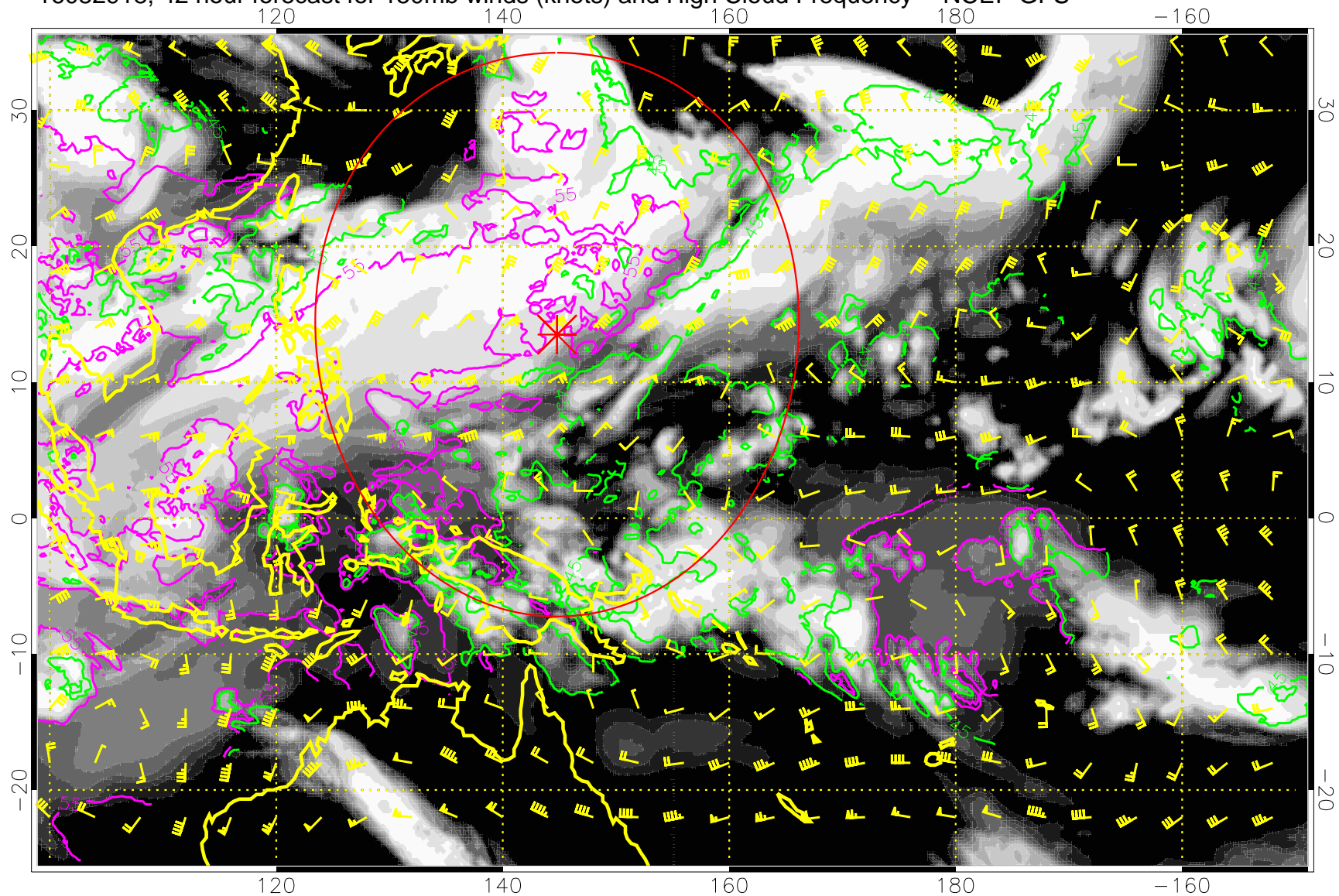
16082918, 42 hour forecast for 150mb winds (knots) and High Cloud Frequency -- NCEP GFS
