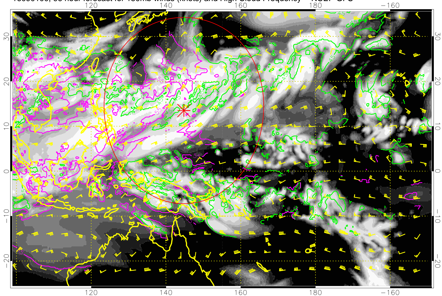
16090100, 96 hour forecast for 150mb winds (knots) and High Cloud Frequency -- NCEP GFS
