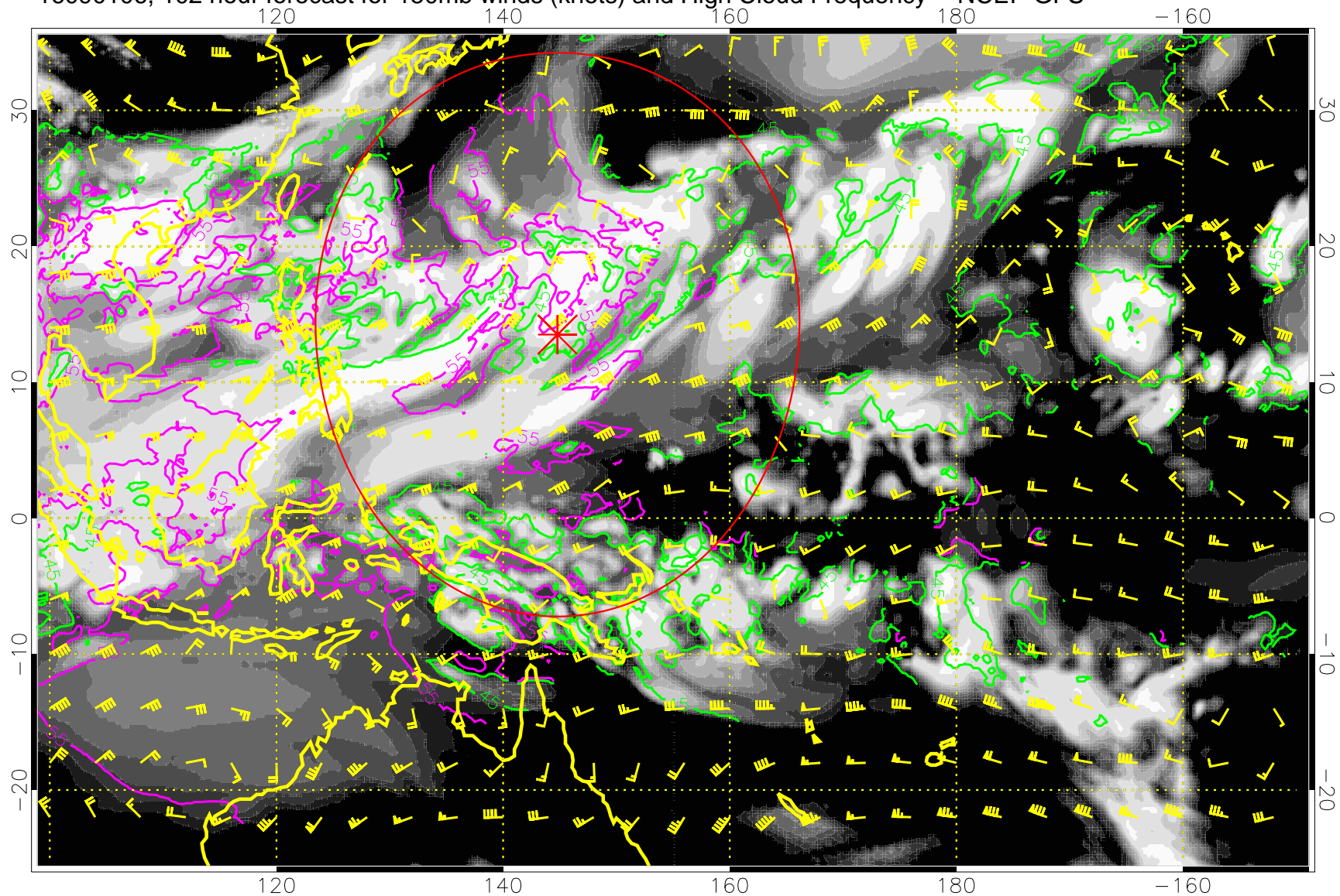
16090106, 102 hour forecast for 150mb winds (knots) and High Cloud Frequency -- NCEP GFS
