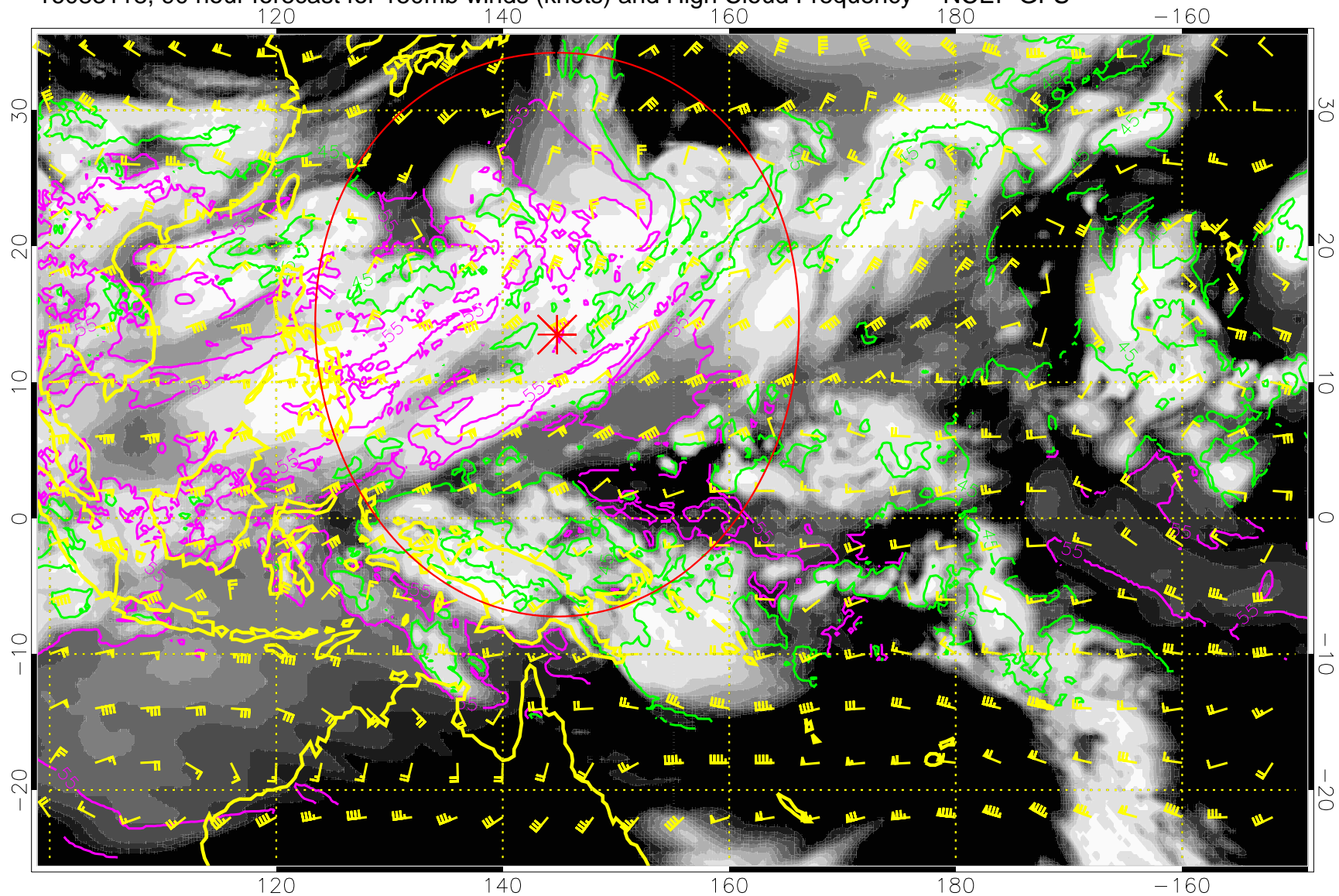
16083118, 90 hour forecast for 150mb winds (knots) and High Cloud Frequency -- NCEP GFS
