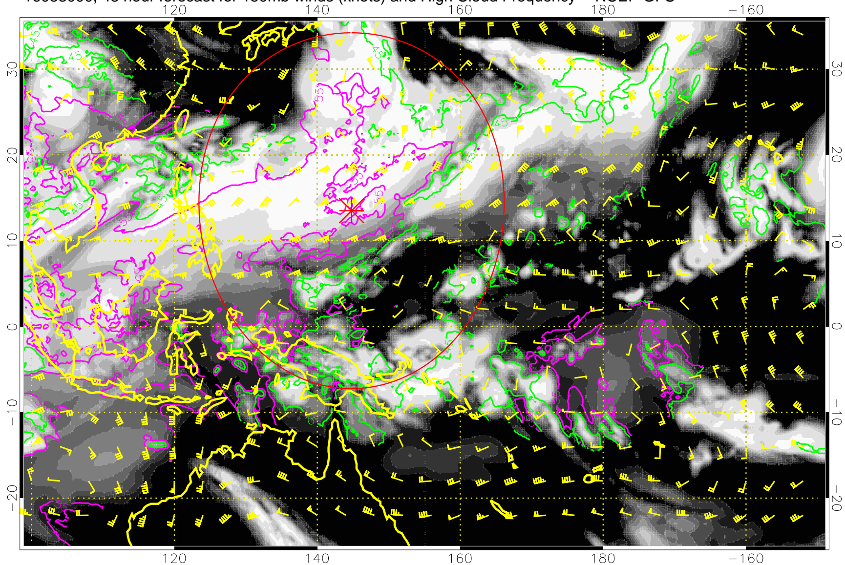
16083000, 48 hour forecast for 150mb winds (knots) and High Cloud Frequency -- NCEP GFS
