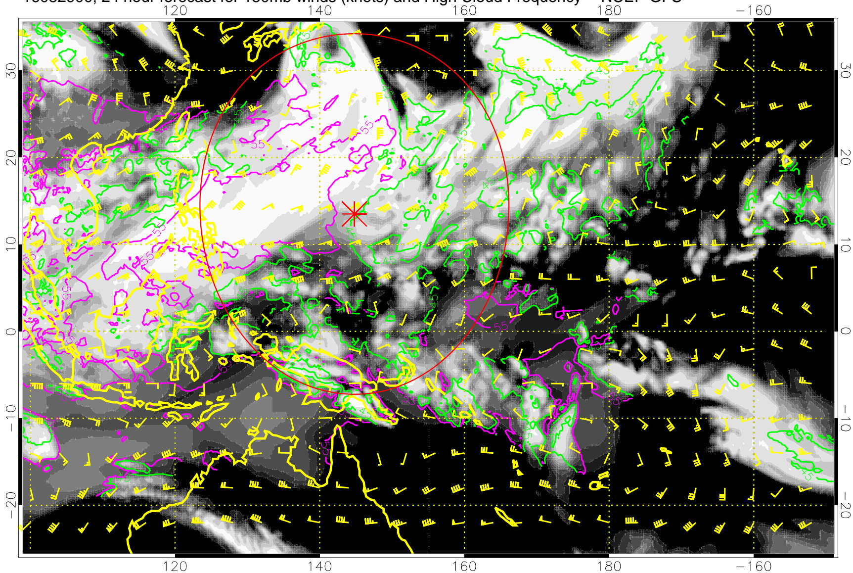
16082900, 24 hour forecast for 150mb winds (knots) and High Cloud Frequency -- NCEP GFS
