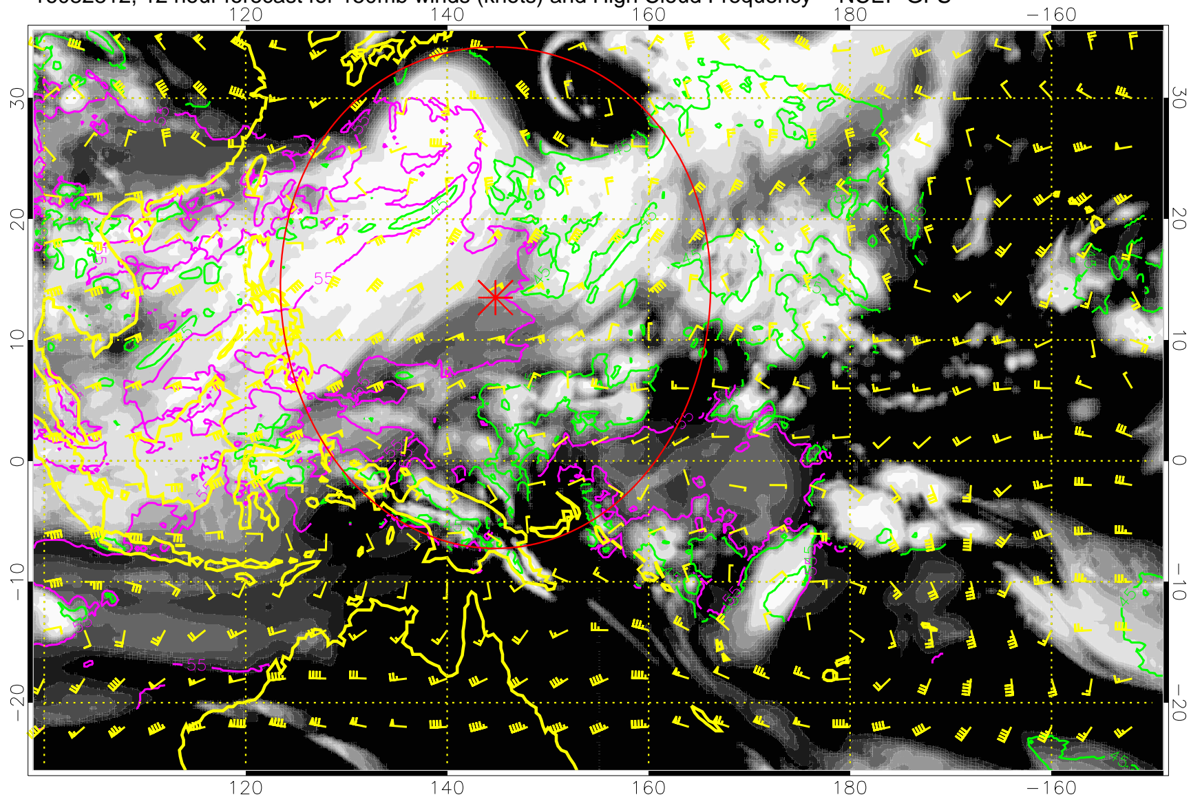
16082812, 12 hour forecast for 150mb winds (knots) and High Cloud Frequency -- NCEP GFS
