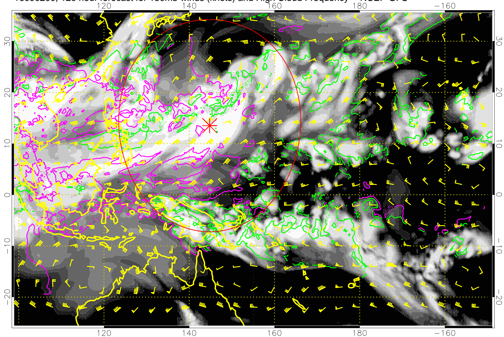
16090200, 120 hour forecast for 150mb winds (knots) and High Cloud Frequency -- NCEP GFS
