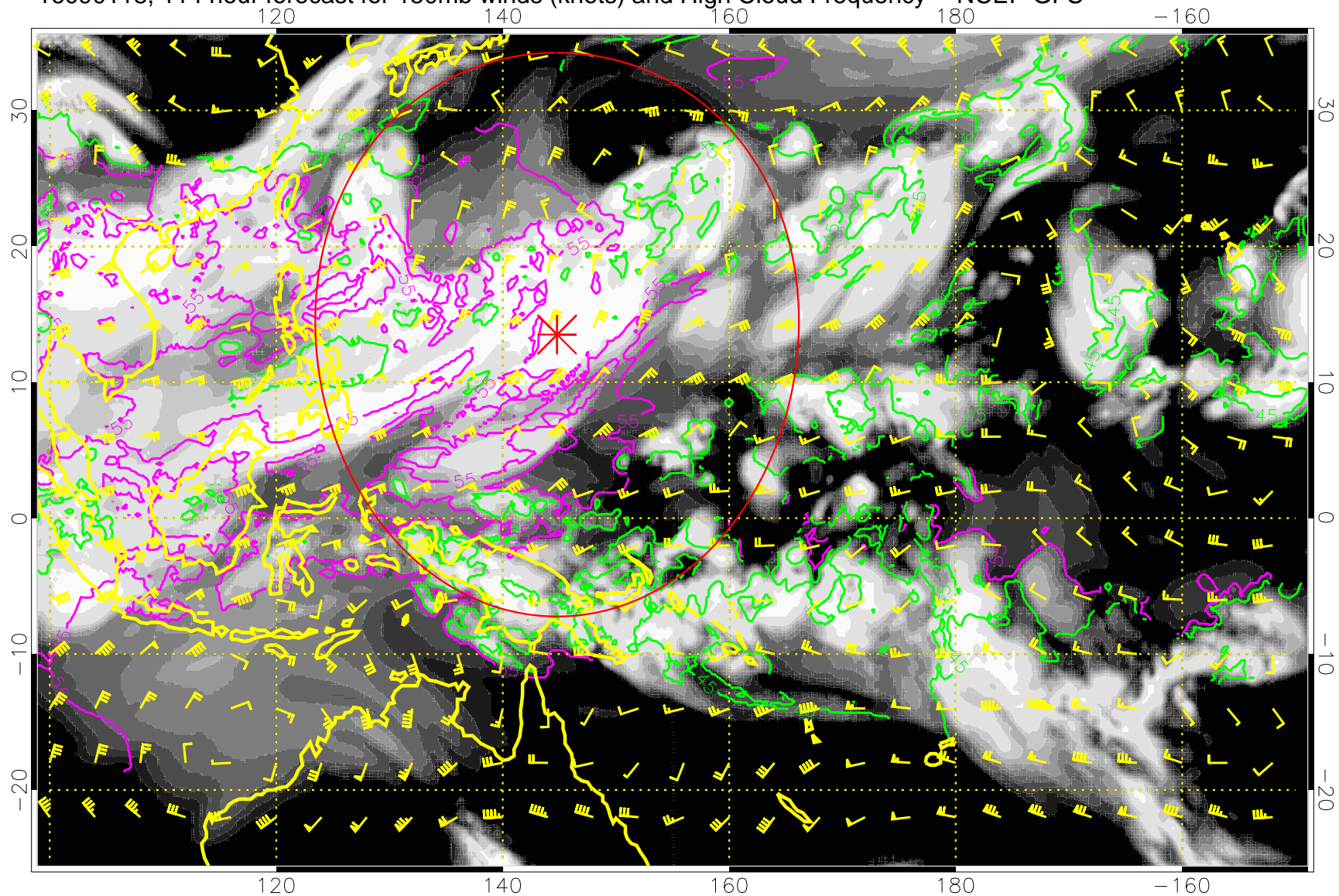
16090118, 114 hour forecast for 150mb winds (knots) and High Cloud Frequency -- NCEP GFS
