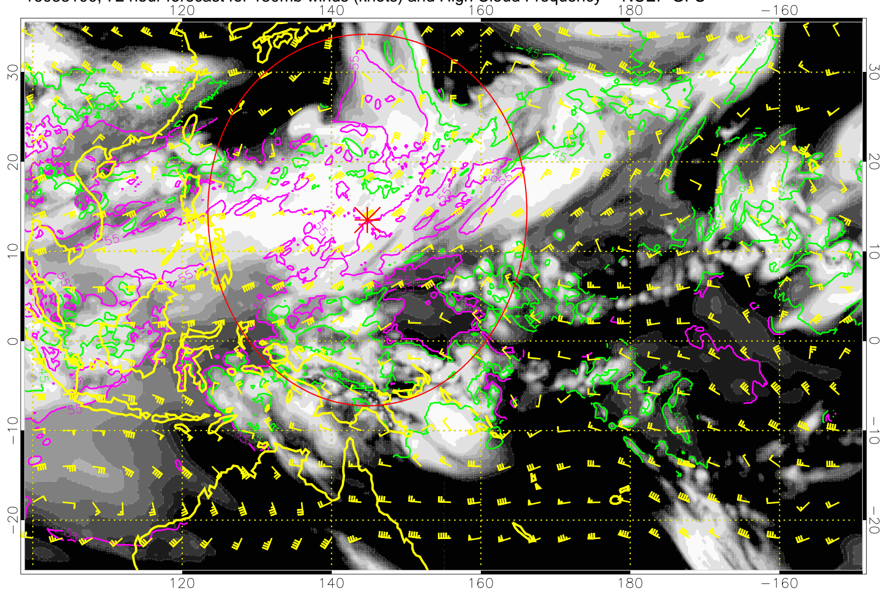
16083100, 72 hour forecast for 150mb winds (knots) and High Cloud Frequency -- NCEP GFS
