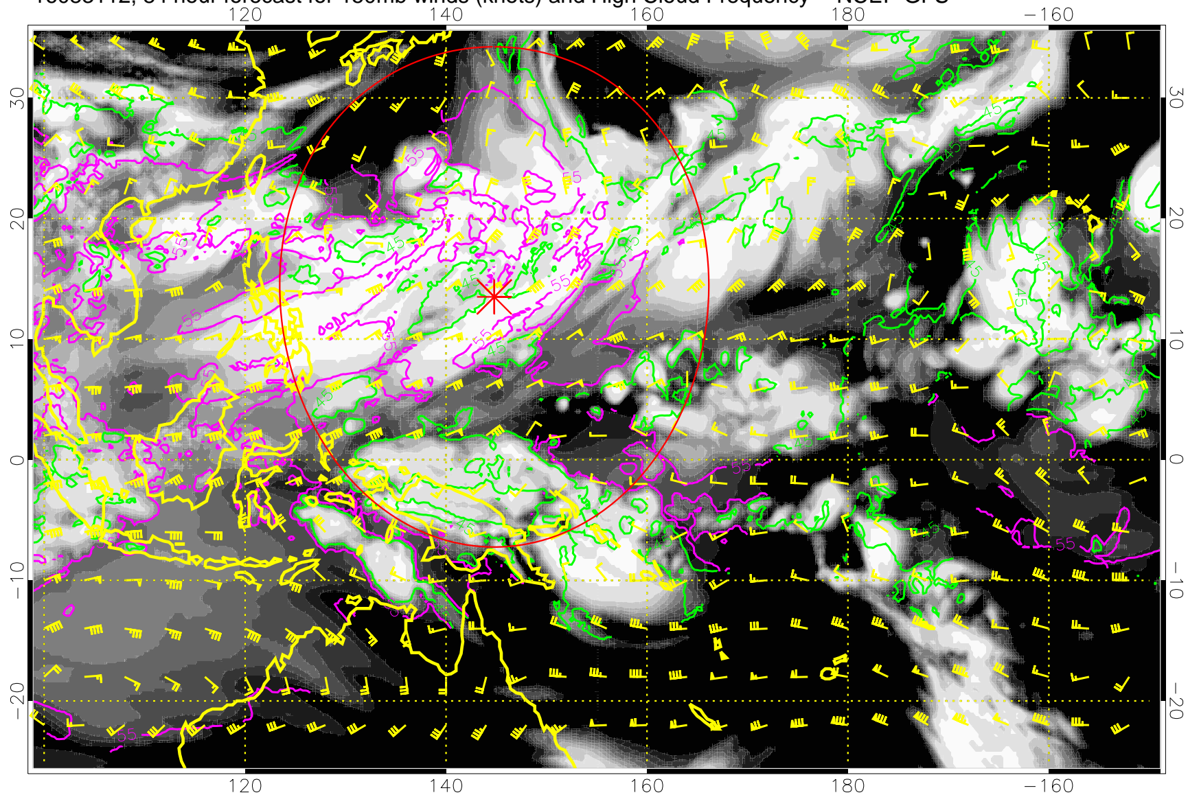
16083112, 84 hour forecast for 150mb winds (knots) and High Cloud Frequency -- NCEP GFS
