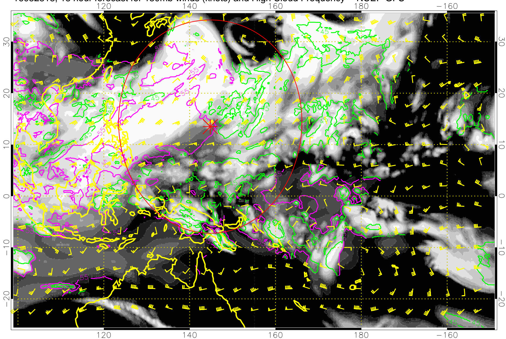
16082818, 18 hour forecast for 150mb winds (knots) and High Cloud Frequency -- NCEP GFS
