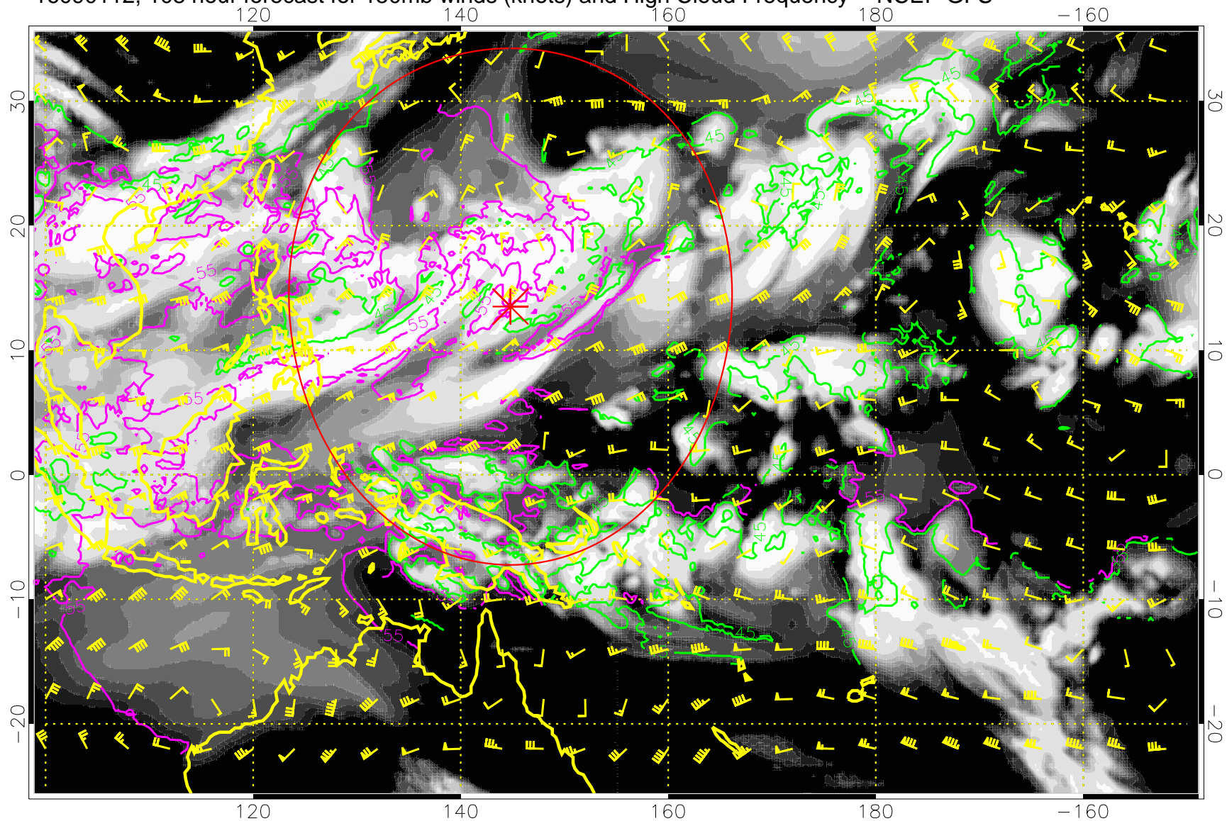
16090112, 108 hour forecast for 150mb winds (knots) and High Cloud Frequency -- NCEP GFS
