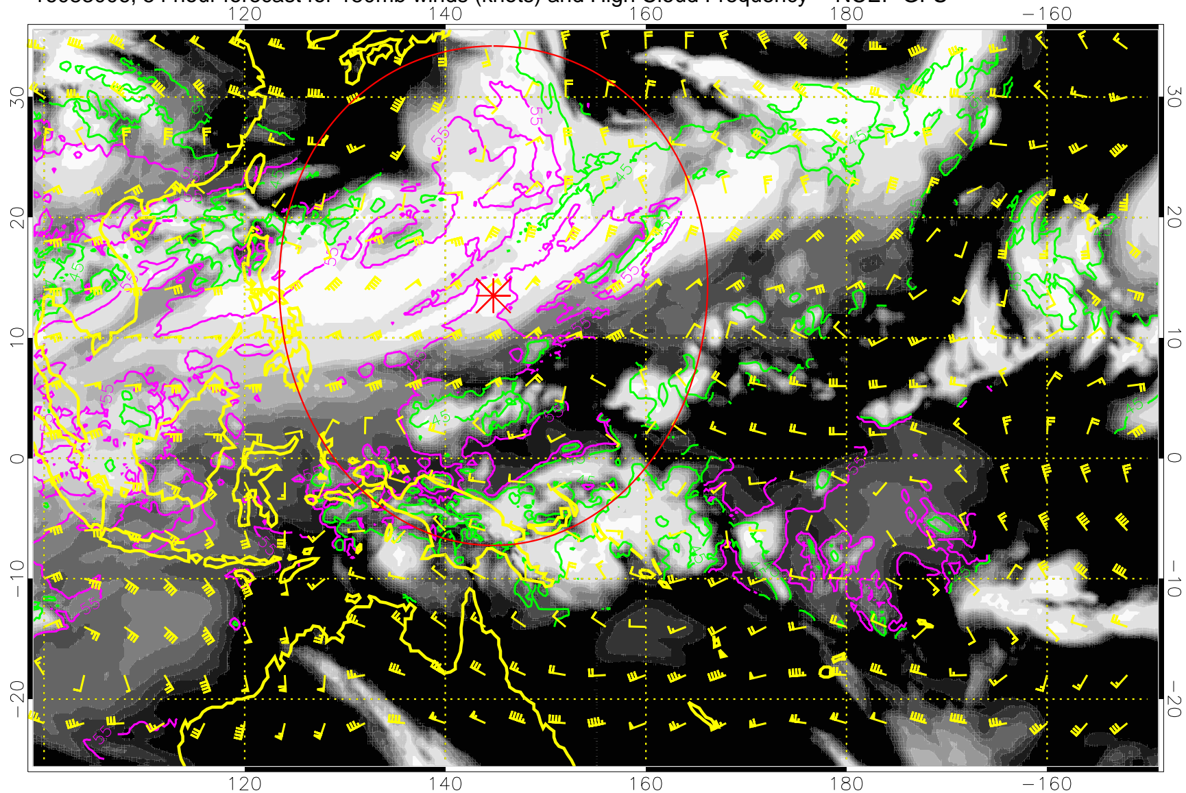
16083006, 54 hour forecast for 150mb winds (knots) and High Cloud Frequency -- NCEP GFS
