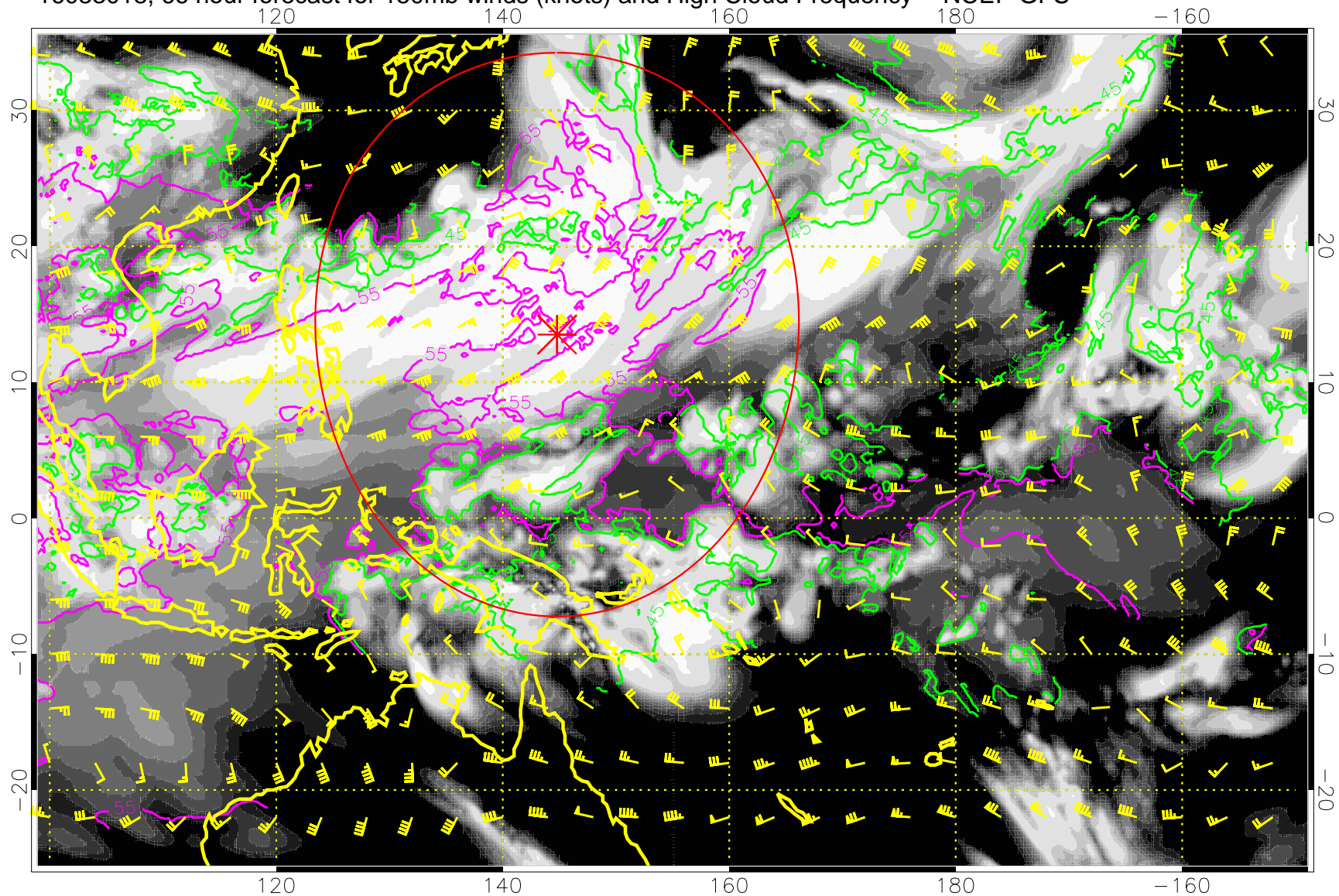
16083018, 66 hour forecast for 150mb winds (knots) and High Cloud Frequency -- NCEP GFS
