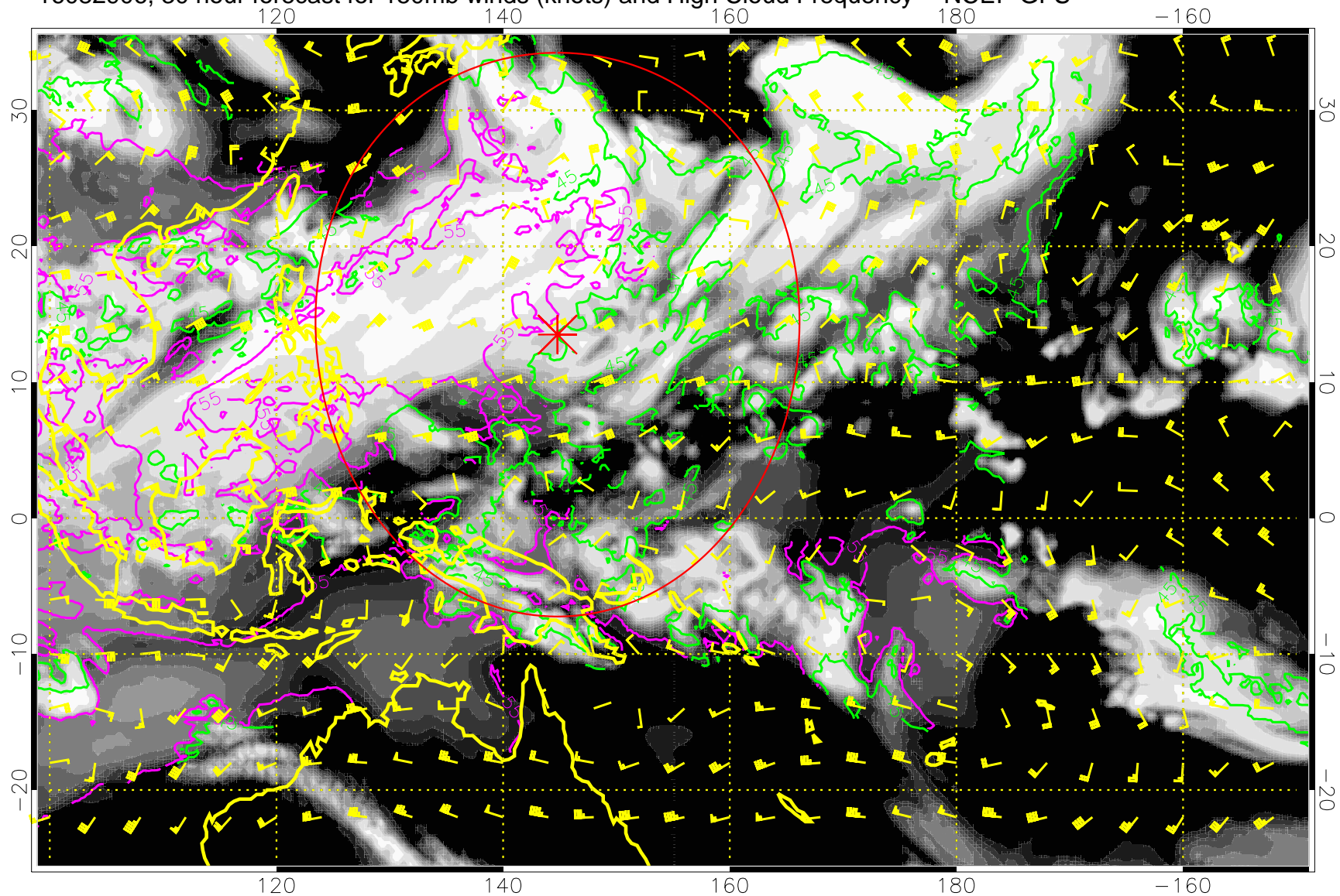
16082906, 30 hour forecast for 150mb winds (knots) and High Cloud Frequency -- NCEP GFS
