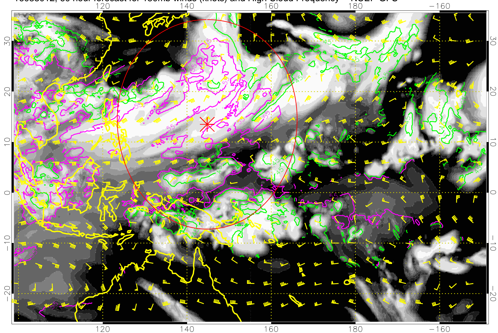
16083012, 60 hour forecast for 150mb winds (knots) and High Cloud Frequency -- NCEP GFS
