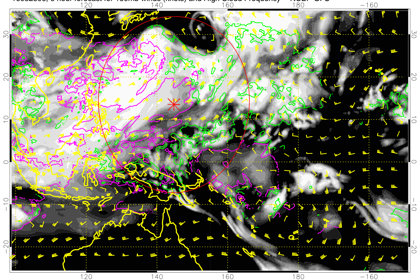
16082806, 6 hour forecast for 150mb winds (knots) and High Cloud Frequency -- NCEP GFS
