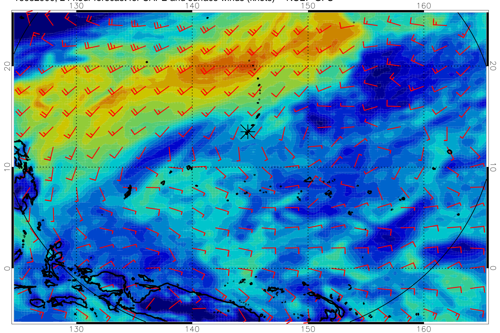
16082900, 24 hour forecast for CAPE and surface winds (knots) -- NCEP GFS
