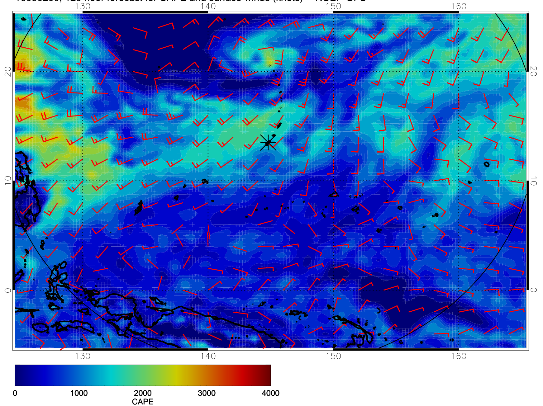
16090200, 120 hour forecast for CAPE and surface winds (knots) -- NCEP GFS
