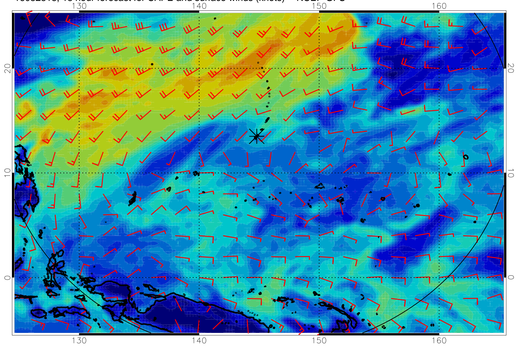
16082818, 18 hour forecast for CAPE and surface winds (knots) -- NCEP GFS
