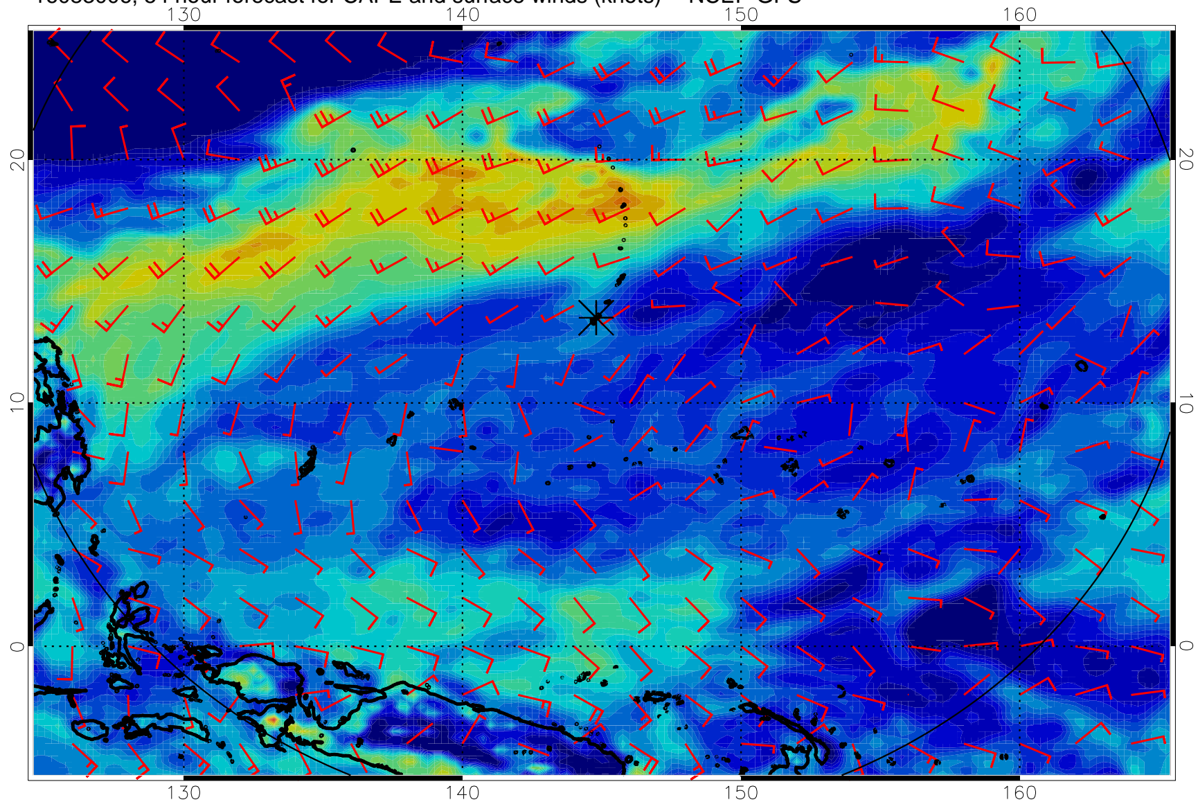
16083006, 54 hour forecast for CAPE and surface winds (knots) -- NCEP GFS
