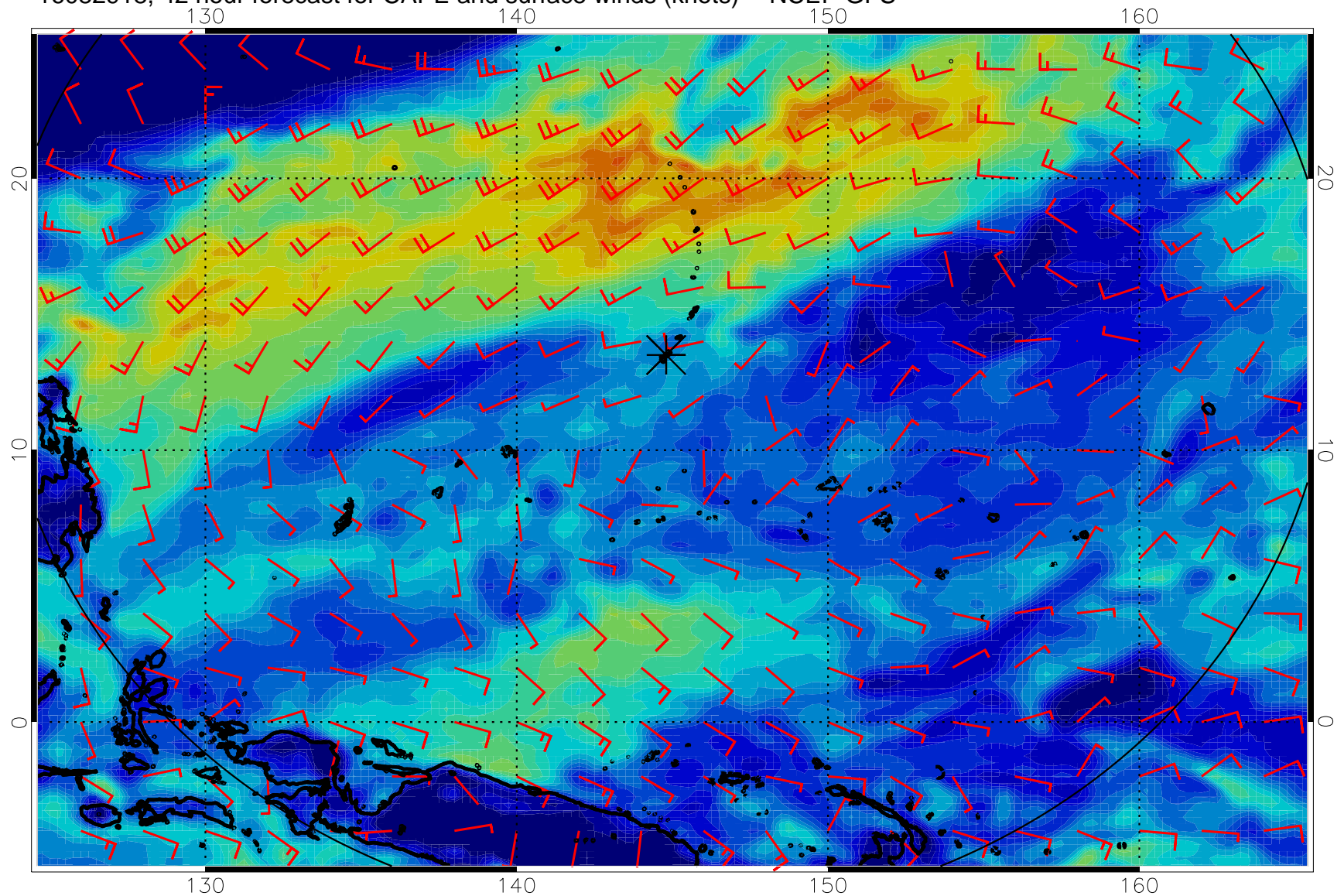
16082918, 42 hour forecast for CAPE and surface winds (knots) -- NCEP GFS
