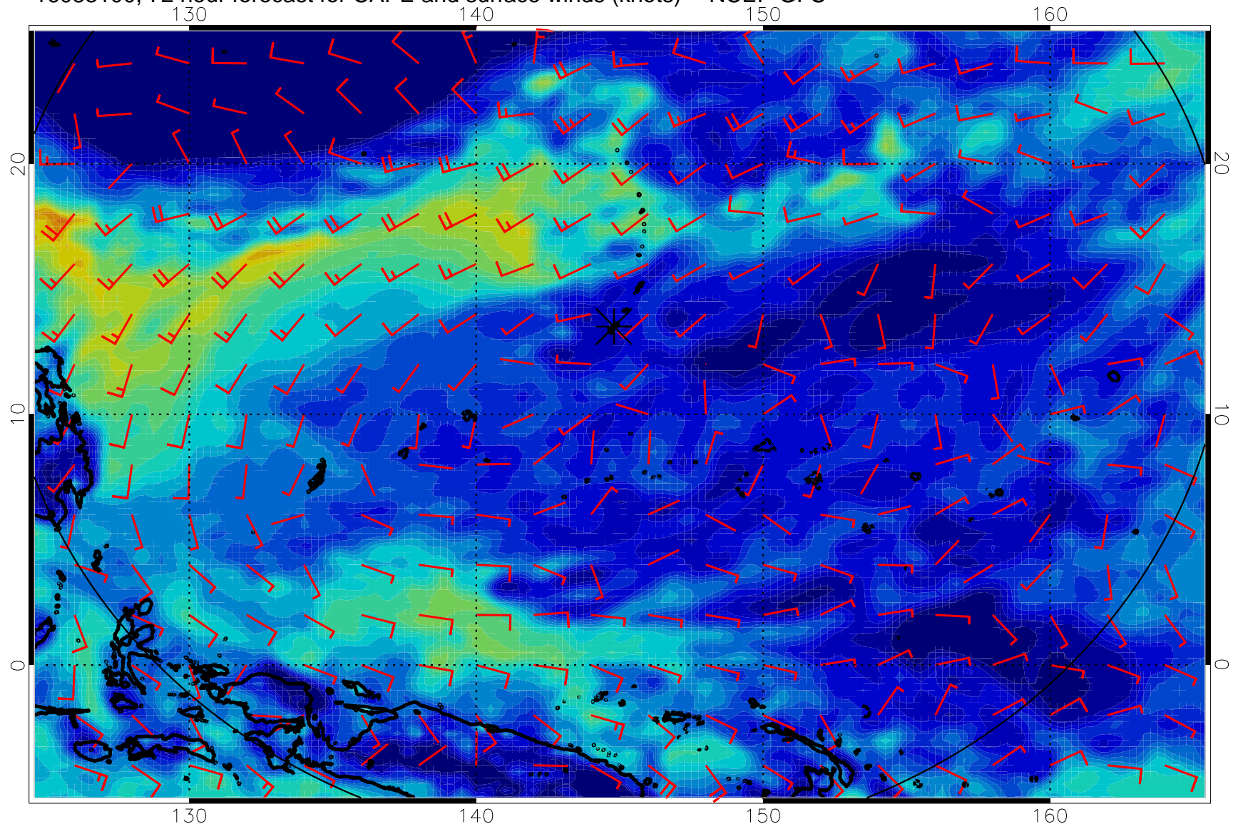
16083100, 72 hour forecast for CAPE and surface winds (knots) -- NCEP GFS
