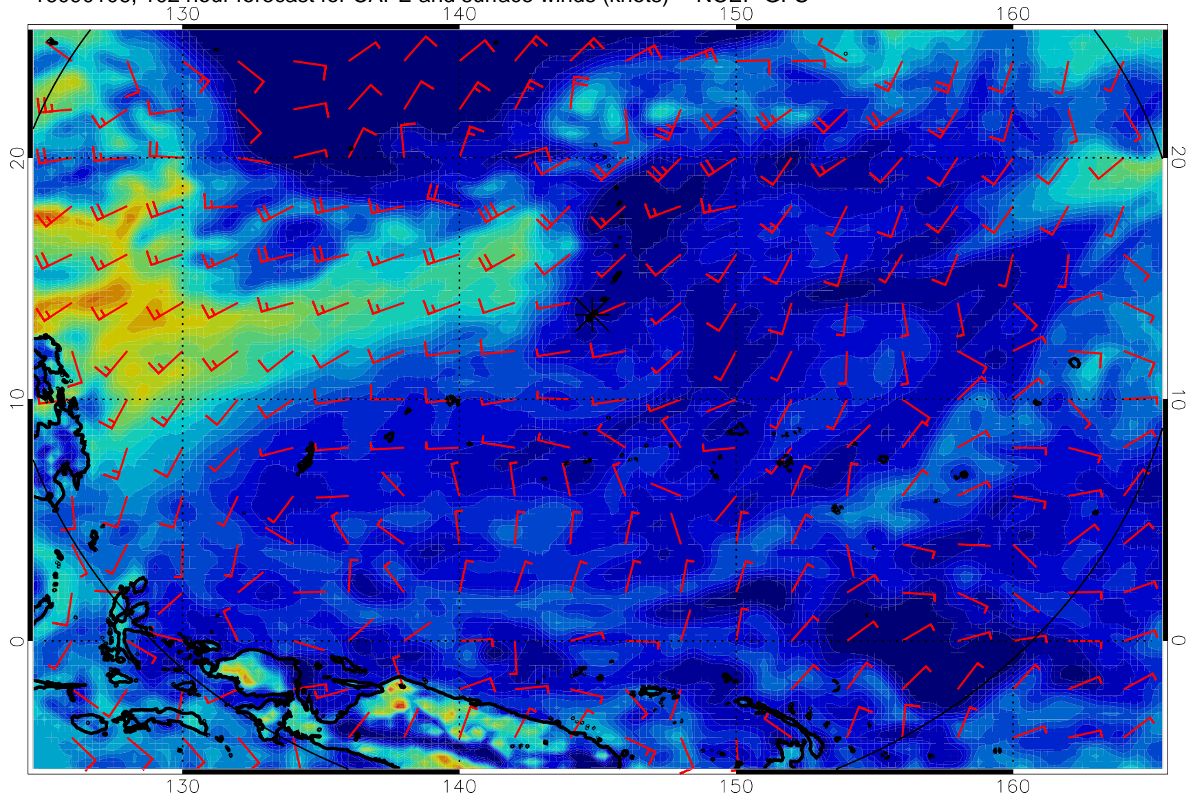
16090106, 102 hour forecast for CAPE and surface winds (knots) -- NCEP GFS
