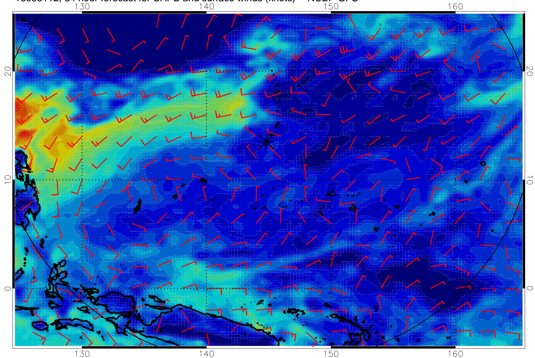
16083112, 84 hour forecast for CAPE and surface winds (knots) -- NCEP GFS
