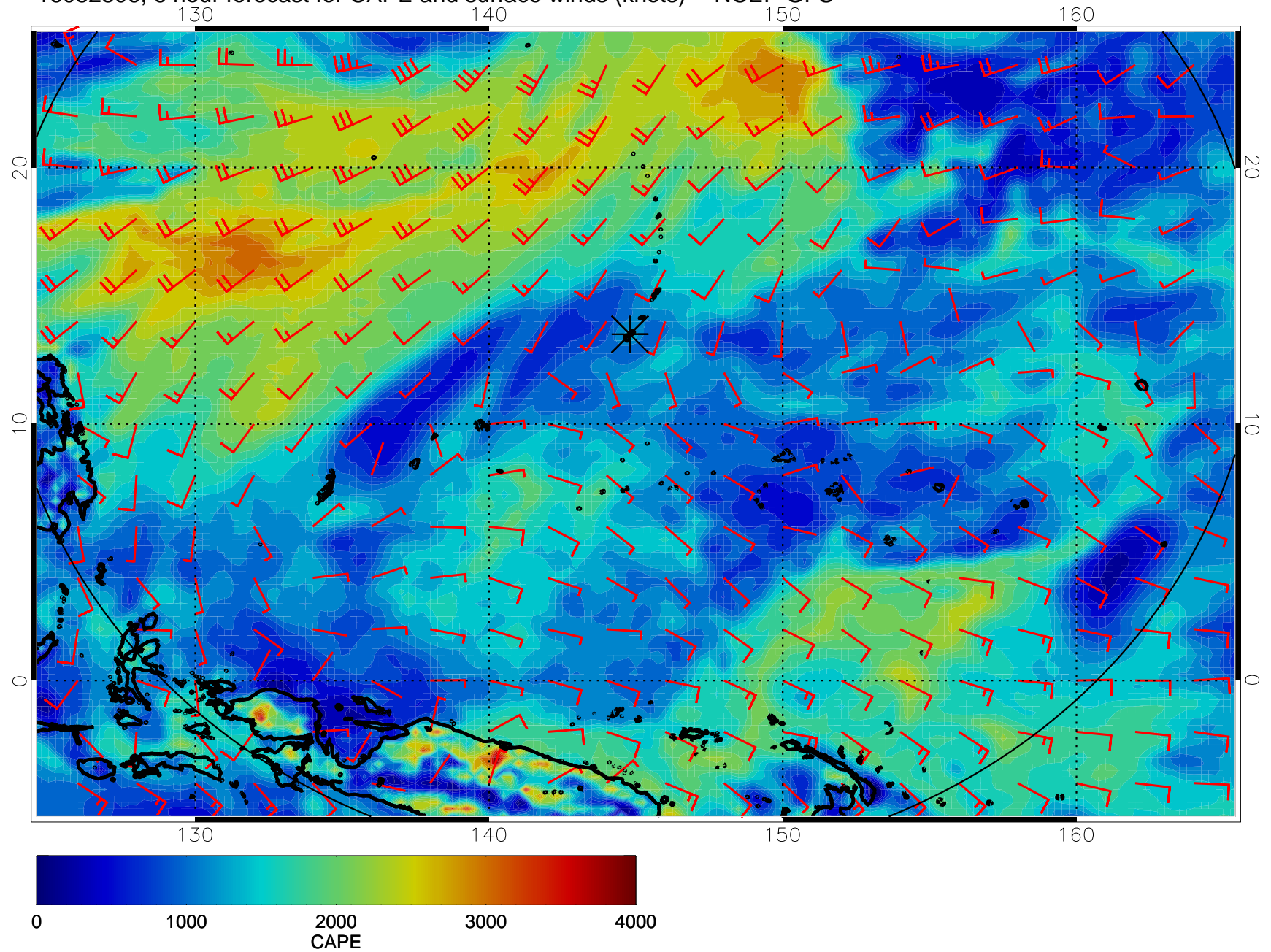
16082806, 6 hour forecast for CAPE and surface winds (knots) -- NCEP GFS
