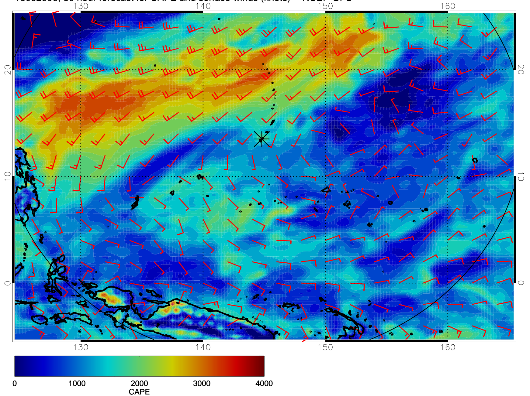
16082906, 30 hour forecast for CAPE and surface winds (knots) -- NCEP GFS
