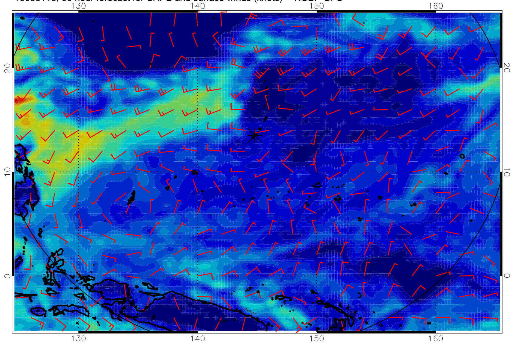
16083118, 90 hour forecast for CAPE and surface winds (knots) -- NCEP GFS
