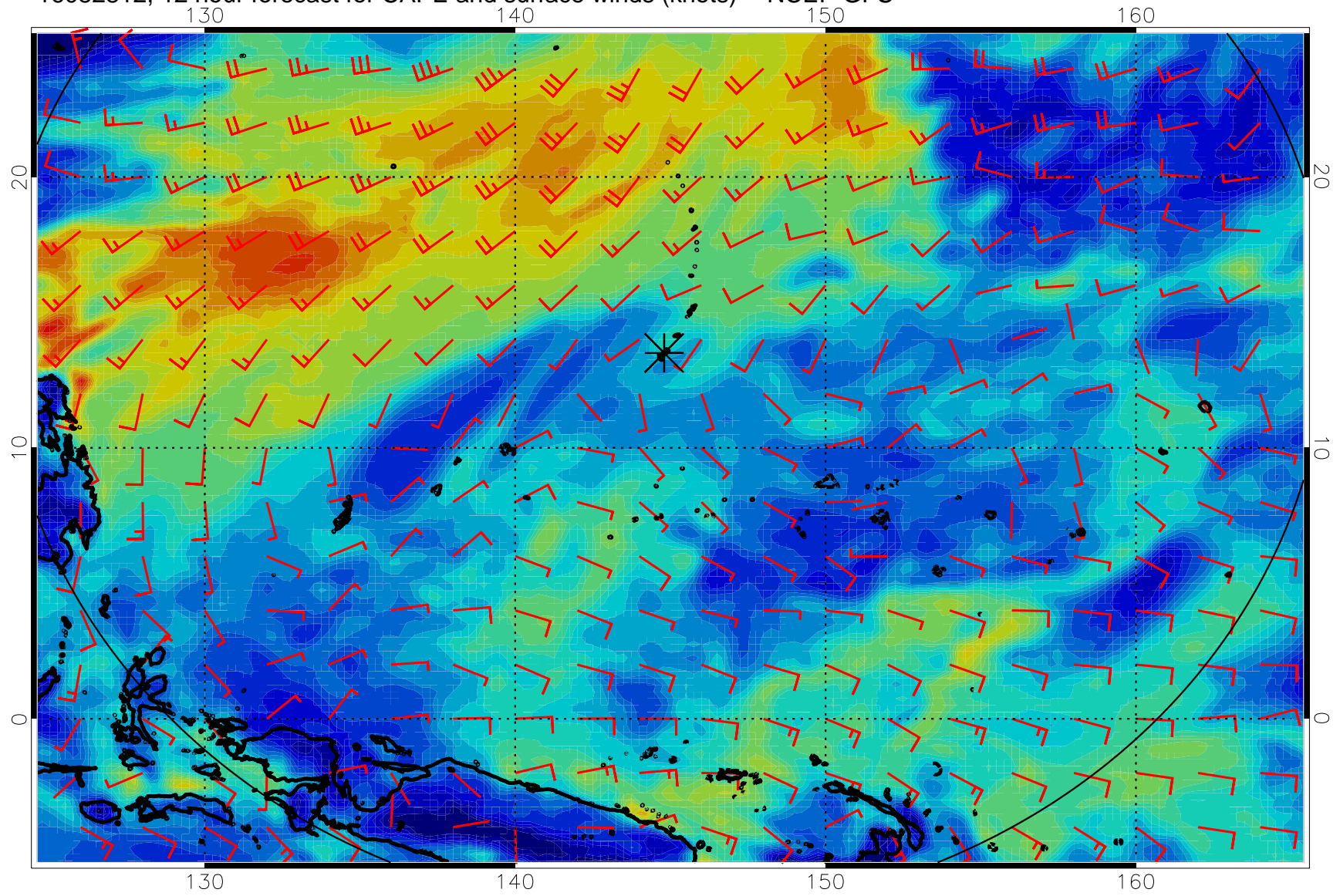
16082812, 12 hour forecast for CAPE and surface winds (knots) -- NCEP GFS
