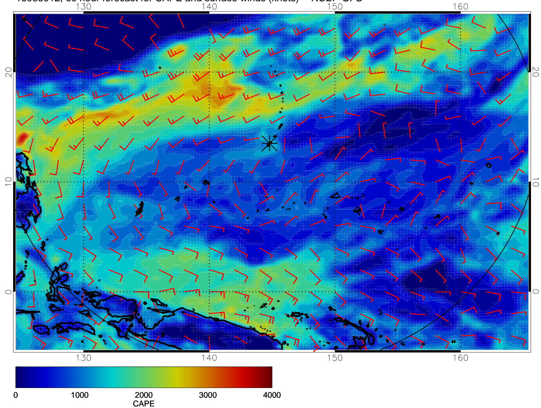
16083012, 60 hour forecast for CAPE and surface winds (knots) -- NCEP GFS
