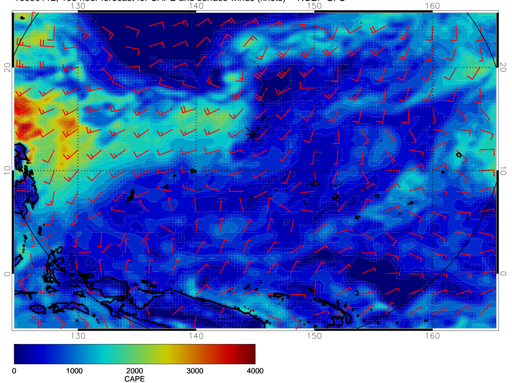
16090112, 108 hour forecast for CAPE and surface winds (knots) -- NCEP GFS
