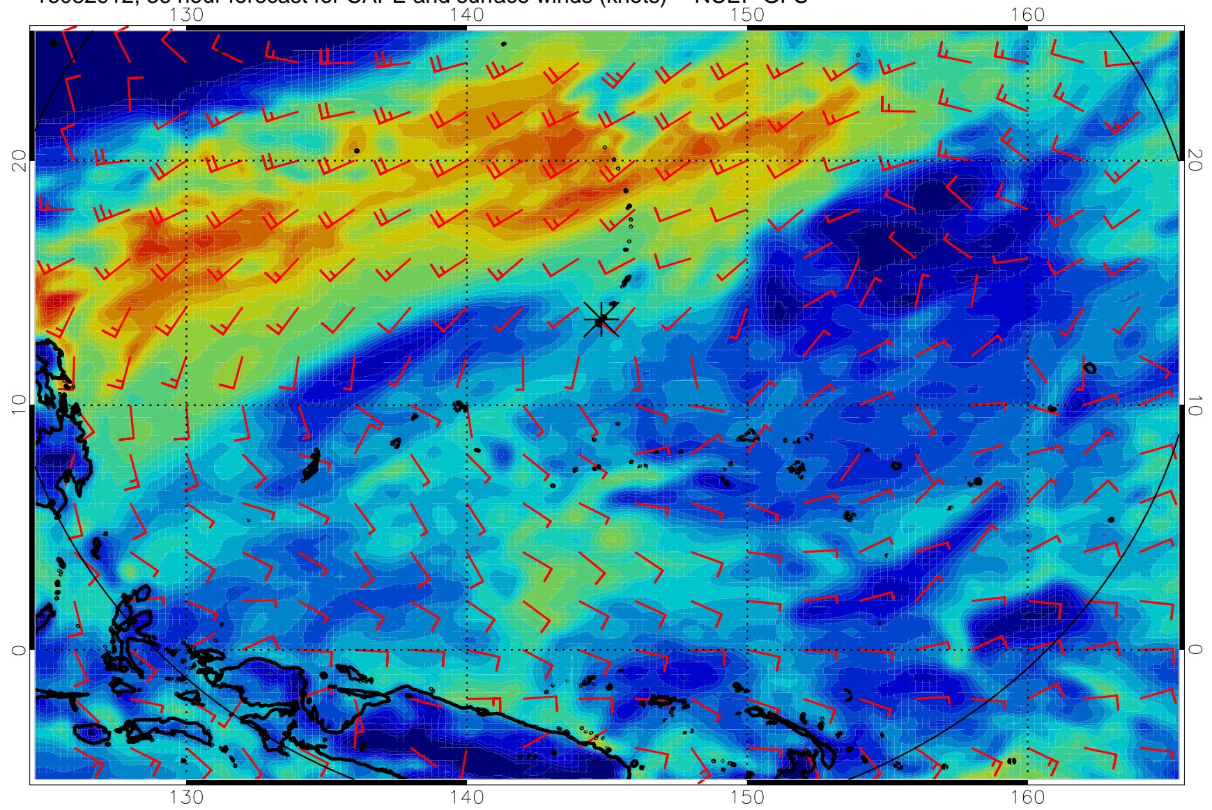
16082912, 36 hour forecast for CAPE and surface winds (knots) -- NCEP GFS
