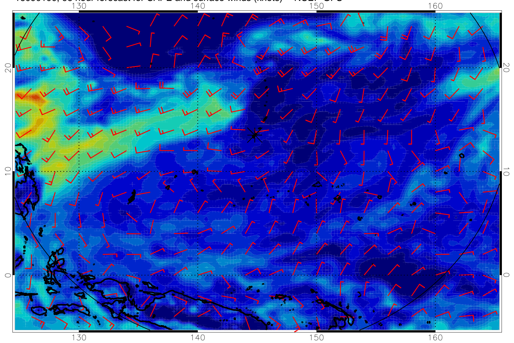
16090100, 96 hour forecast for CAPE and surface winds (knots) -- NCEP GFS
