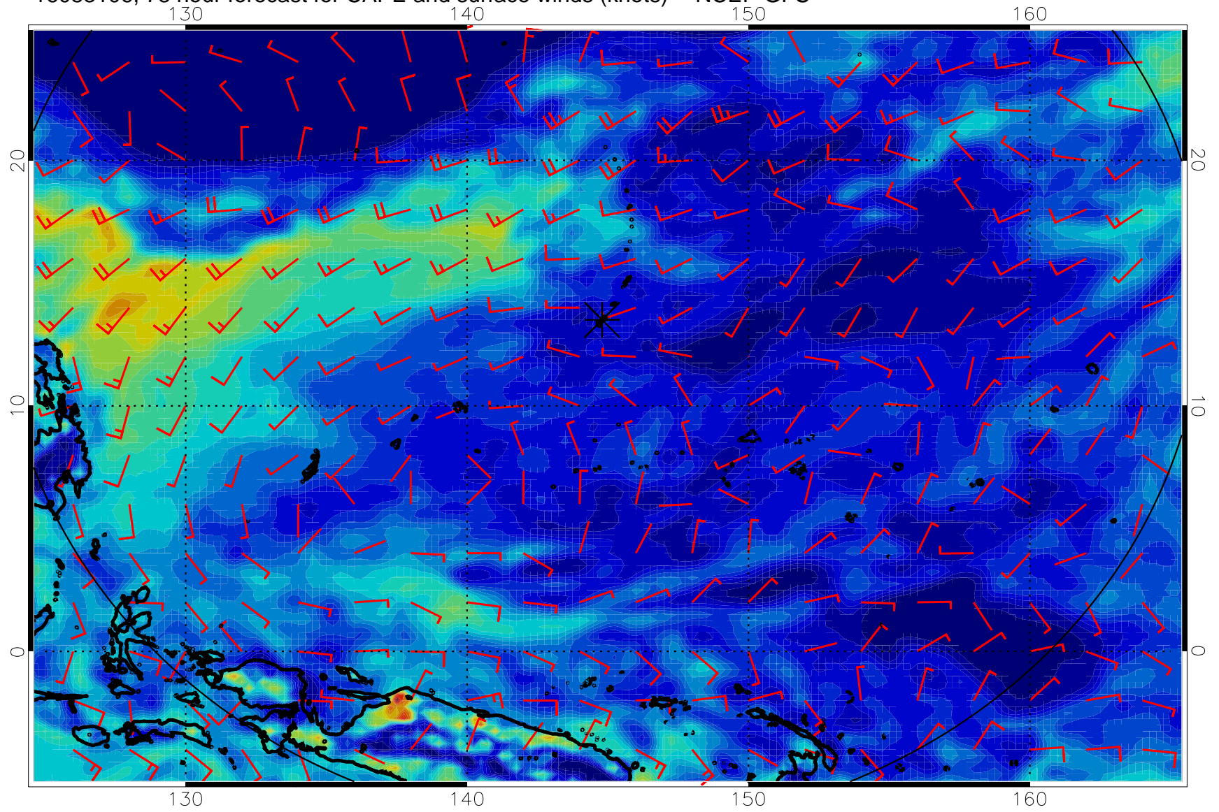
16083106, 78 hour forecast for CAPE and surface winds (knots) -- NCEP GFS
