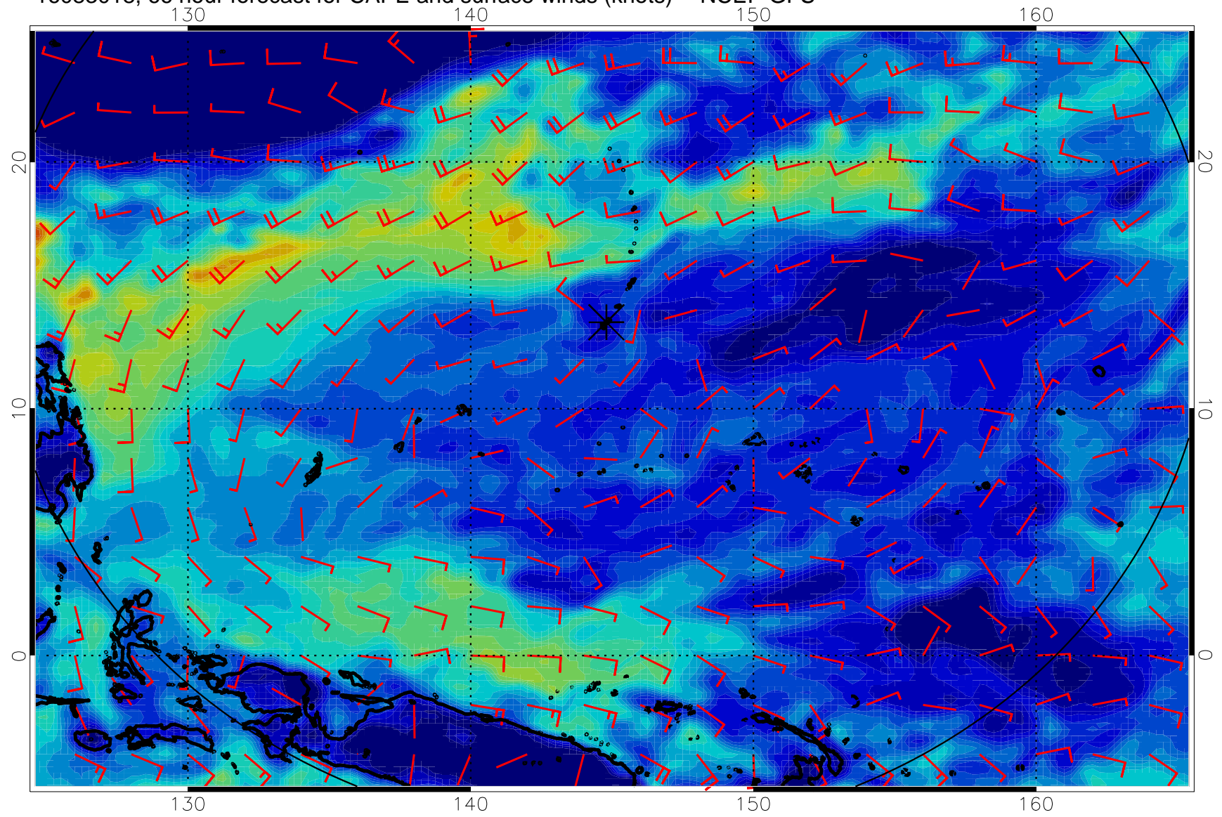
16083018, 66 hour forecast for CAPE and surface winds (knots) -- NCEP GFS
