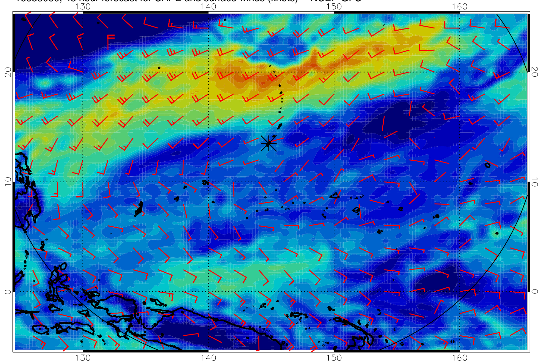
16083000, 48 hour forecast for CAPE and surface winds (knots) -- NCEP GFS
