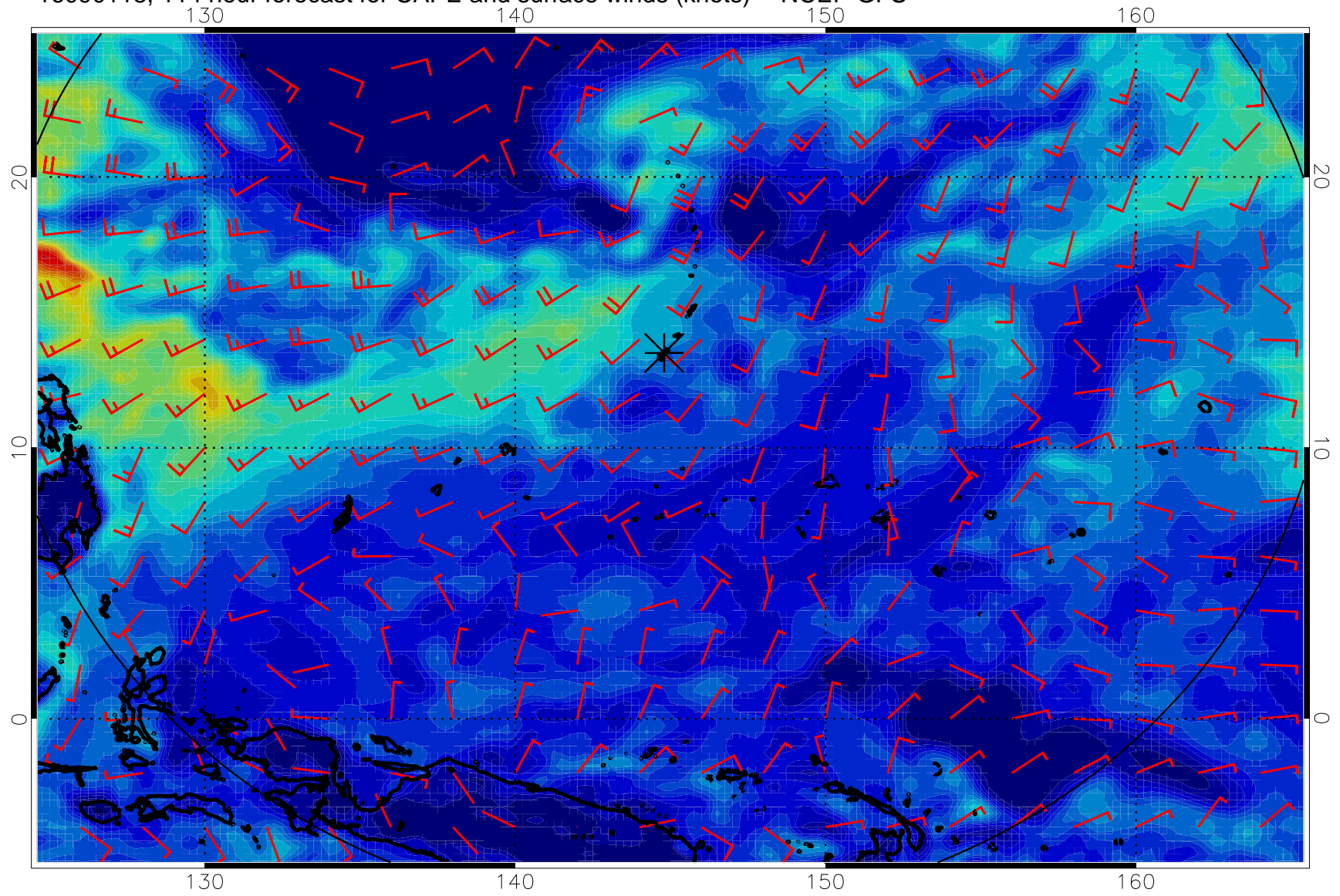
16090118, 114 hour forecast for CAPE and surface winds (knots) -- NCEP GFS
