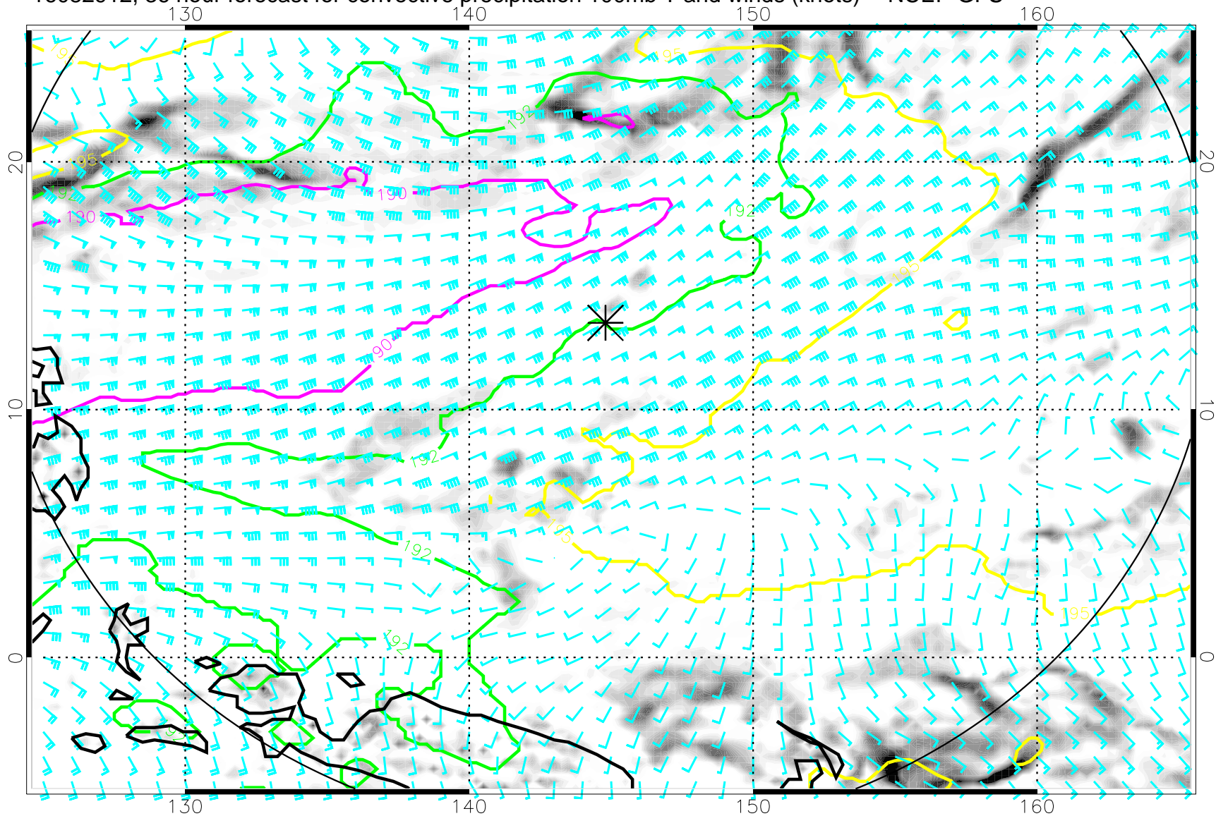
16082912, 36 hour forecast for convective precipitation 100mb T and winds (knots) -- NCEP GFS
