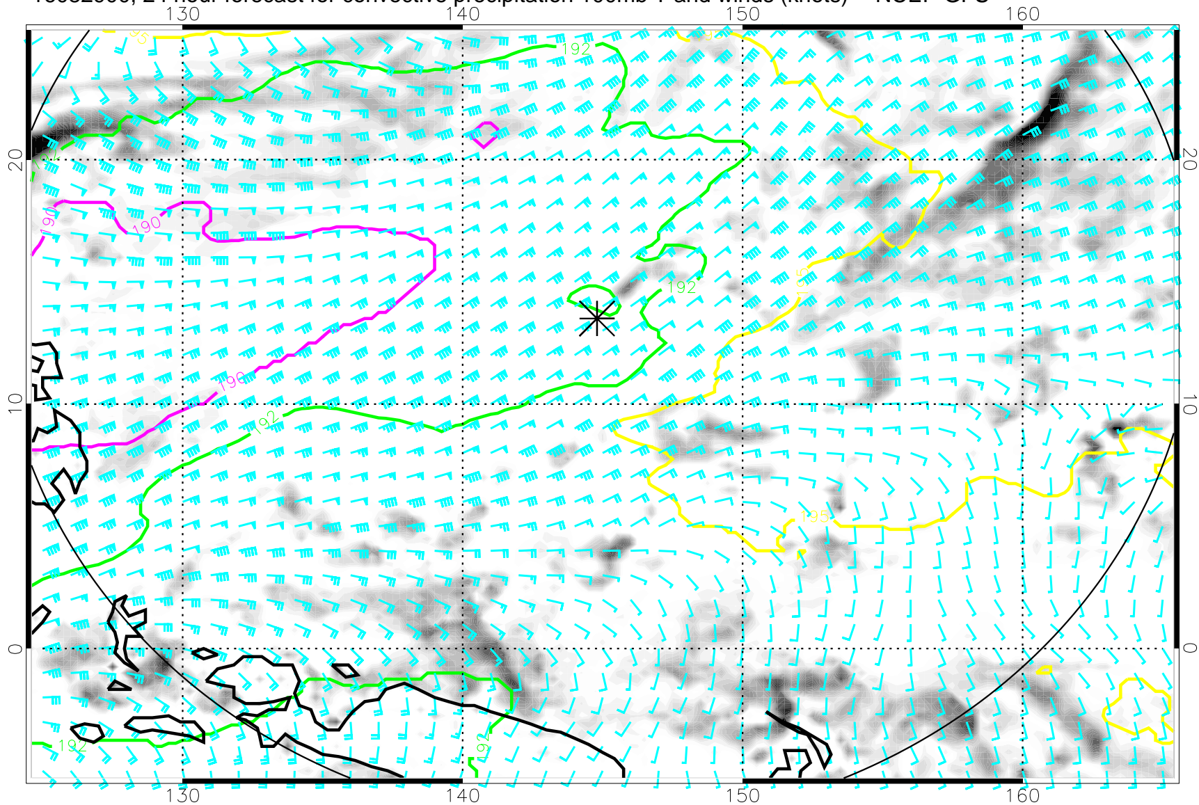
16082900, 24 hour forecast for convective precipitation 100mb T and winds (knots) -- NCEP GFS
