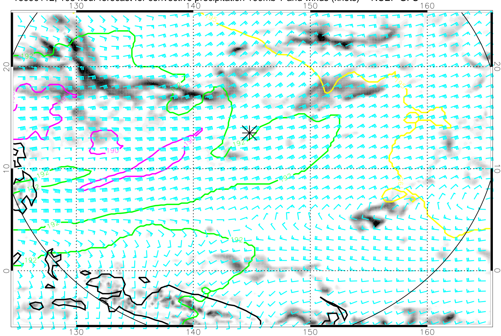
16090112, 108 hour forecast for convective precipitation 100mb T and winds (knots) -- NCEP GFS
