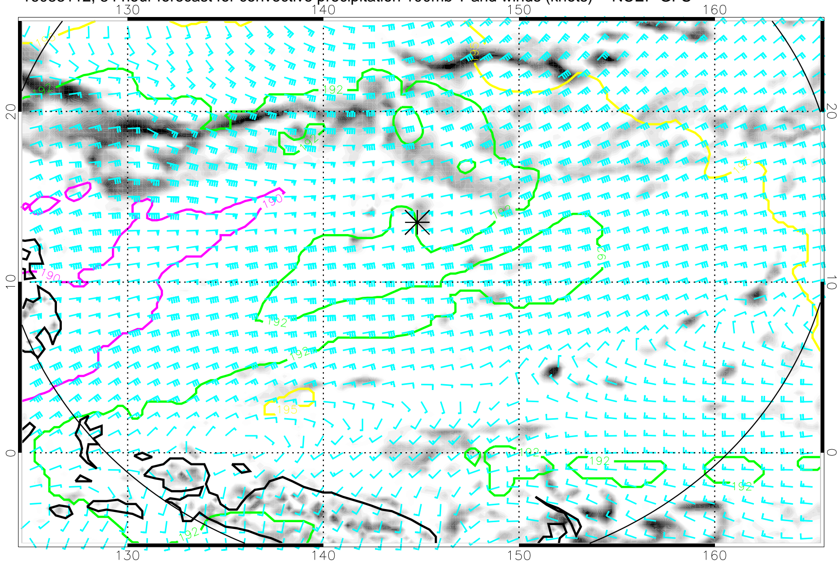
16083112, 84 hour forecast for convective precipitation 100mb T and winds (knots) -- NCEP GFS
