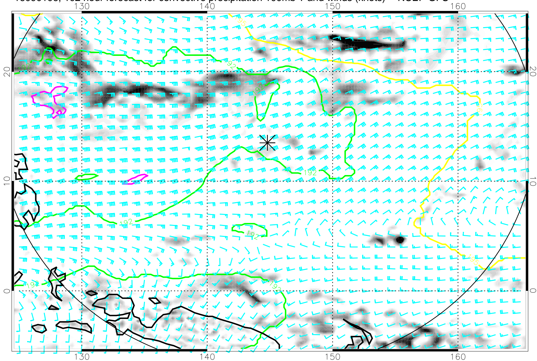
16090106, 102 hour forecast for convective precipitation 100mb T and winds (knots) -- NCEP GFS
