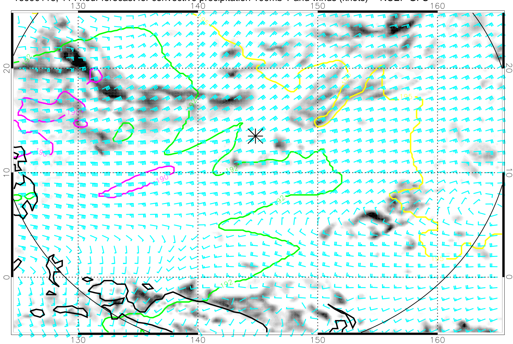
16090118, 114 hour forecast for convective precipitation 100mb T and winds (knots) -- NCEP GFS
