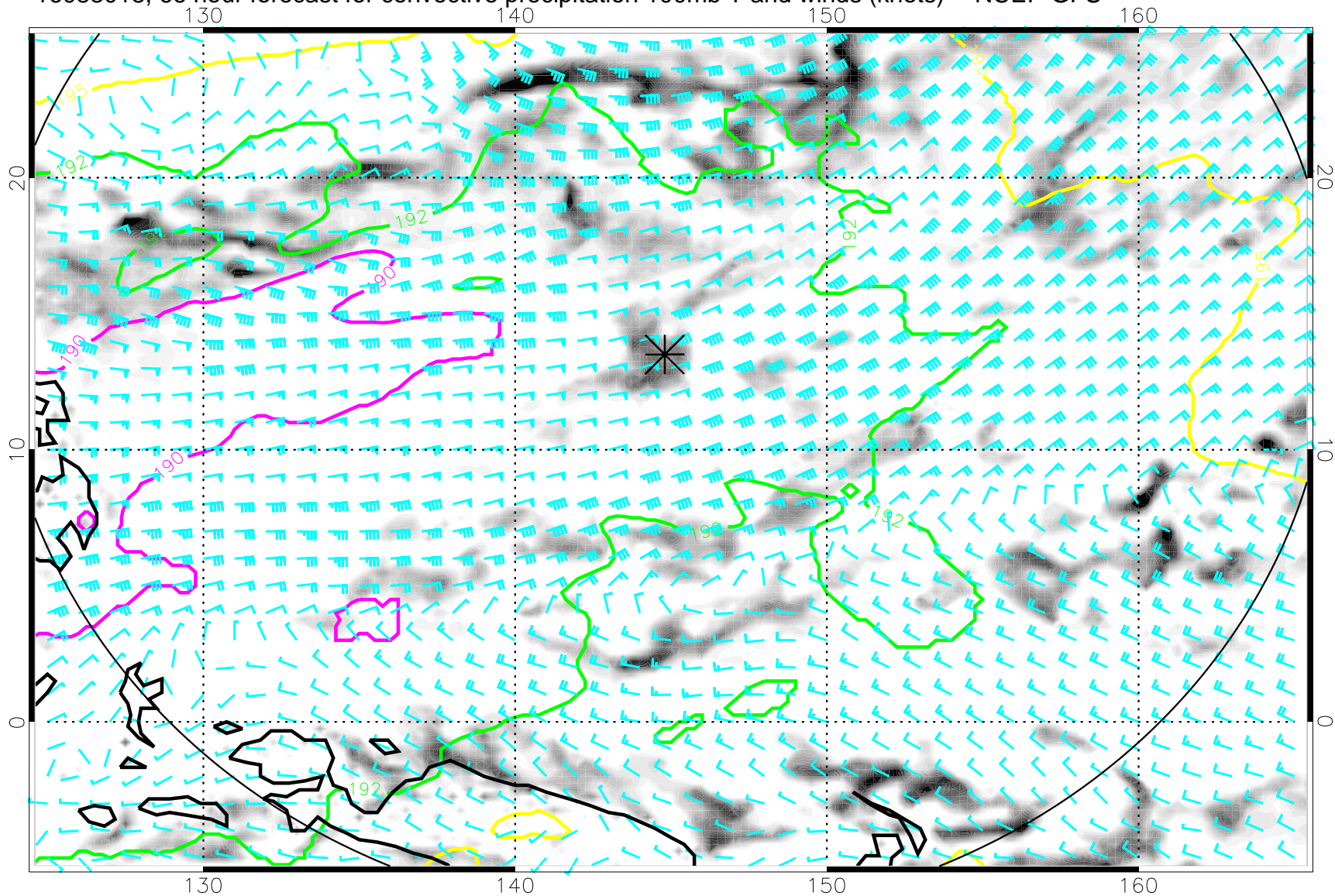
16083018, 66 hour forecast for convective precipitation 100mb T and winds (knots) -- NCEP GFS
