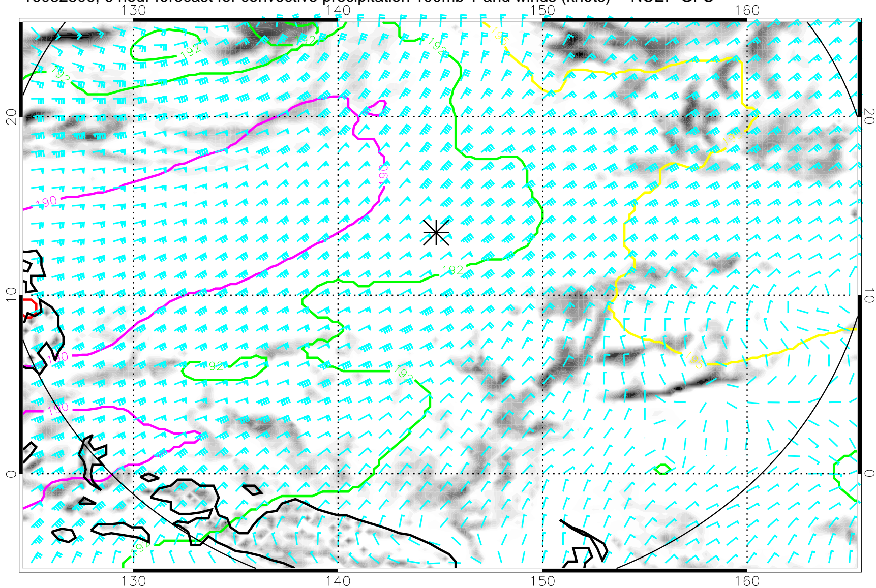
16082806, 6 hour forecast for convective precipitation 100mb T and winds (knots) -- NCEP GFS
