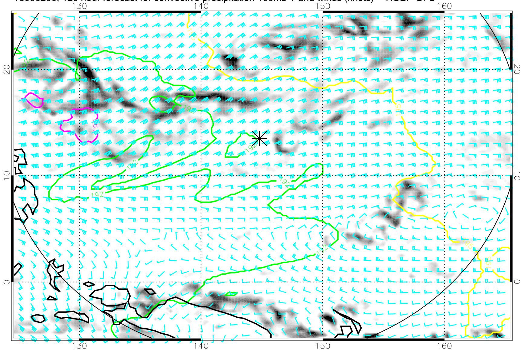
16090200, 120 hour forecast for convective precipitation 100mb T and winds (knots) -- NCEP GFS
