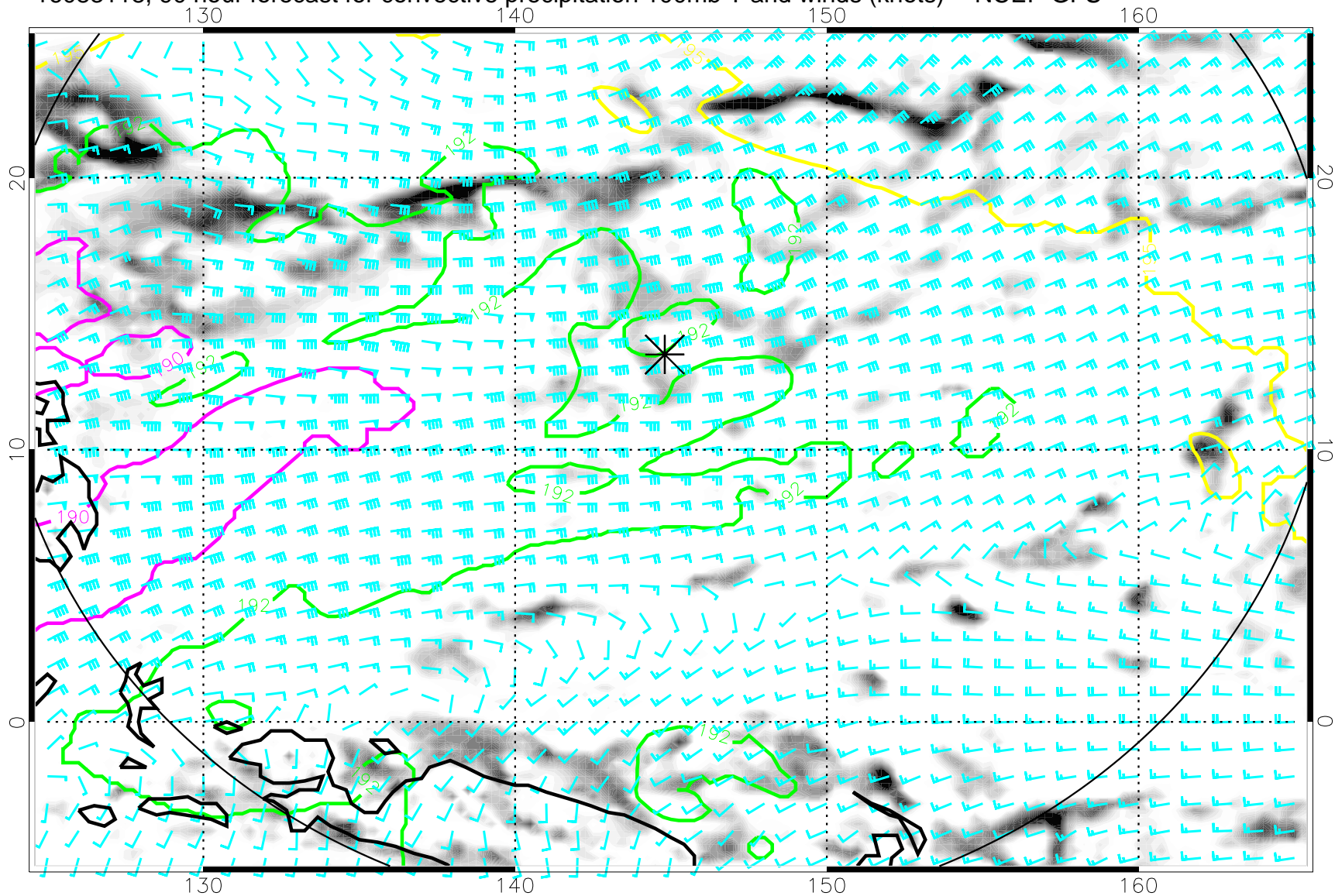
16083118, 90 hour forecast for convective precipitation 100mb T and winds (knots) -- NCEP GFS
