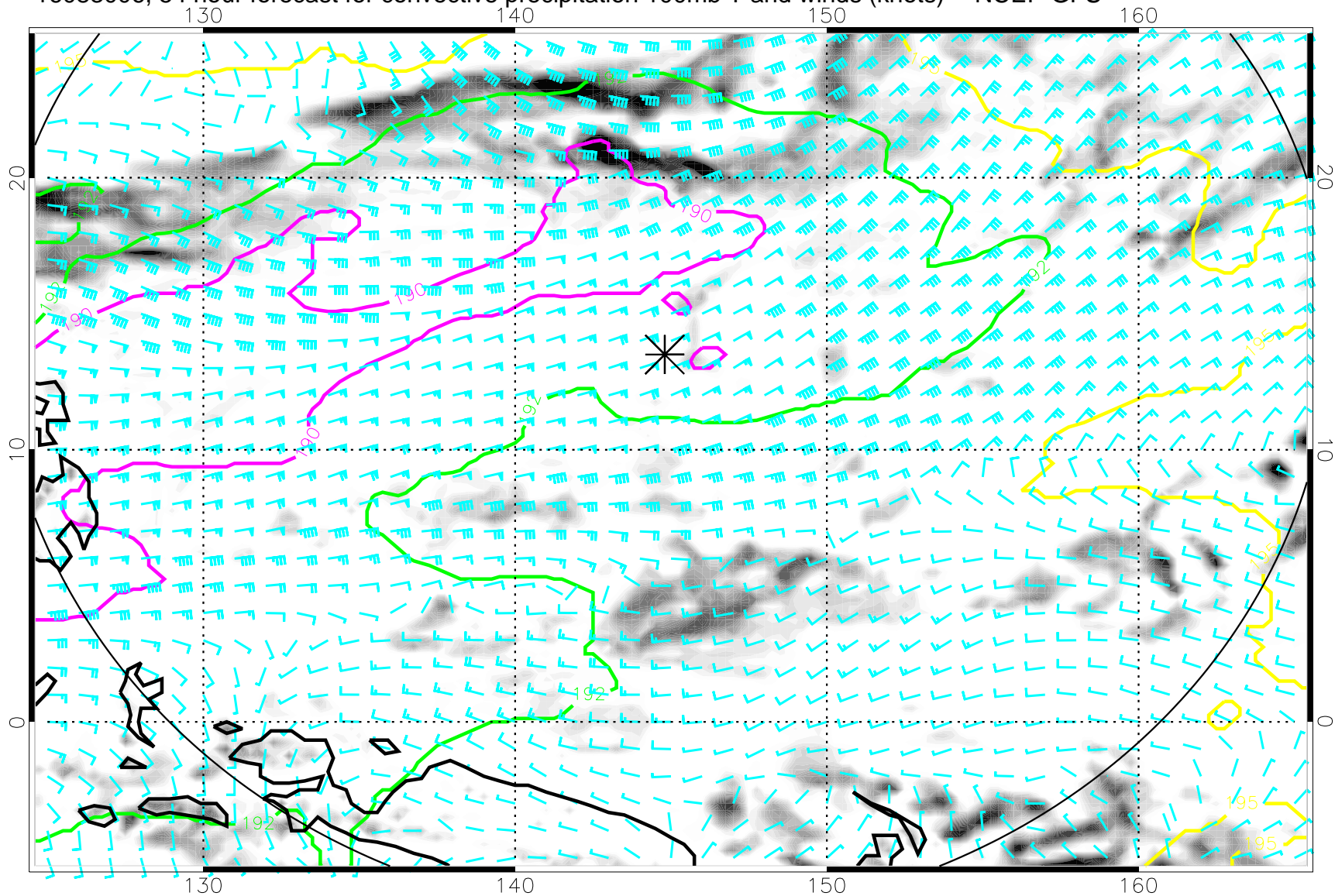
16083006, 54 hour forecast for convective precipitation 100mb T and winds (knots) -- NCEP GFS
