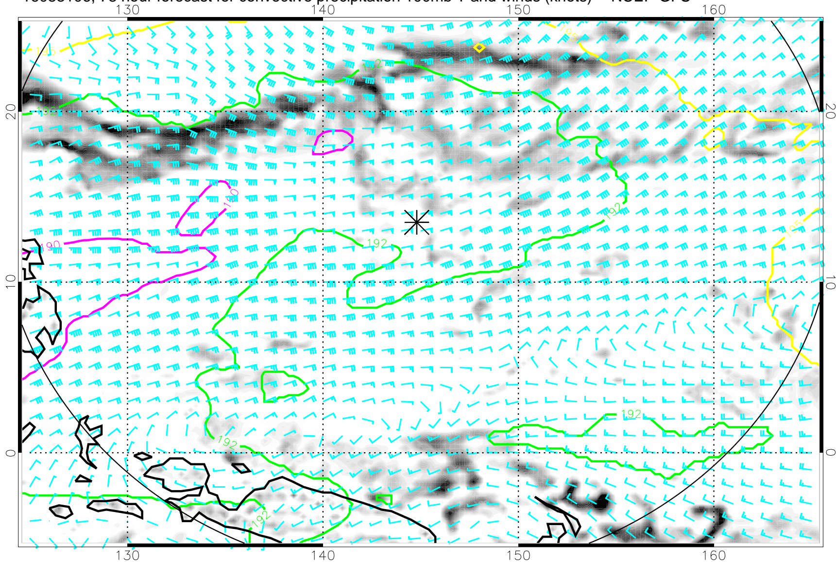
16083106, 78 hour forecast for convective precipitation 100mb T and winds (knots) -- NCEP GFS
