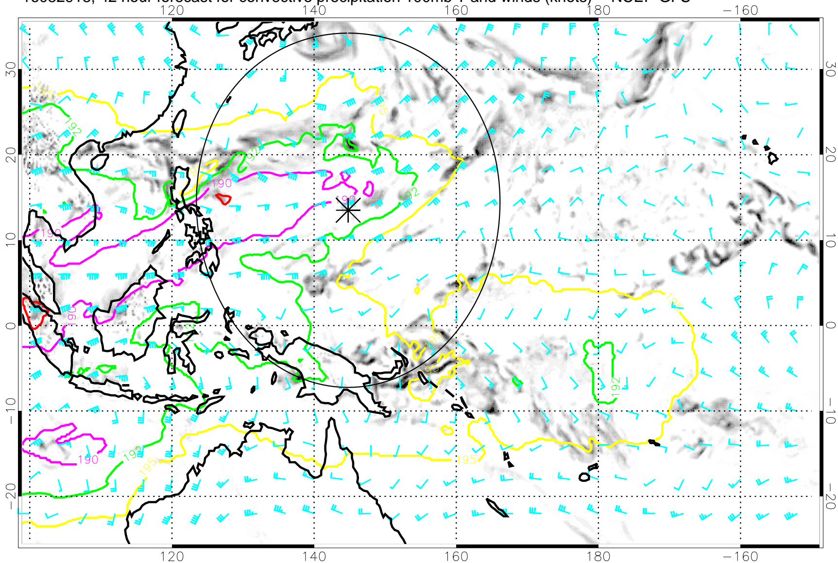
16082918, 42 hour forecast for convective precipitation 100mb T and winds (knots) -- NCEP GFS
