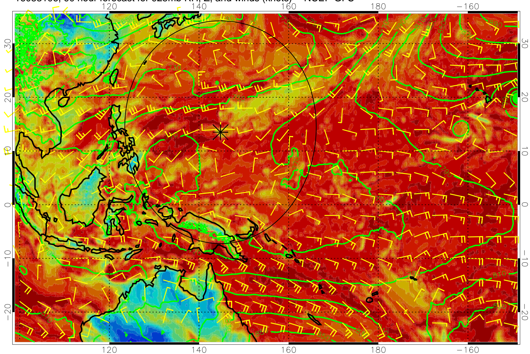
16083106, 90 hour forecast for 925mb RH, Z, and winds (knots) -- NCEP GFS
