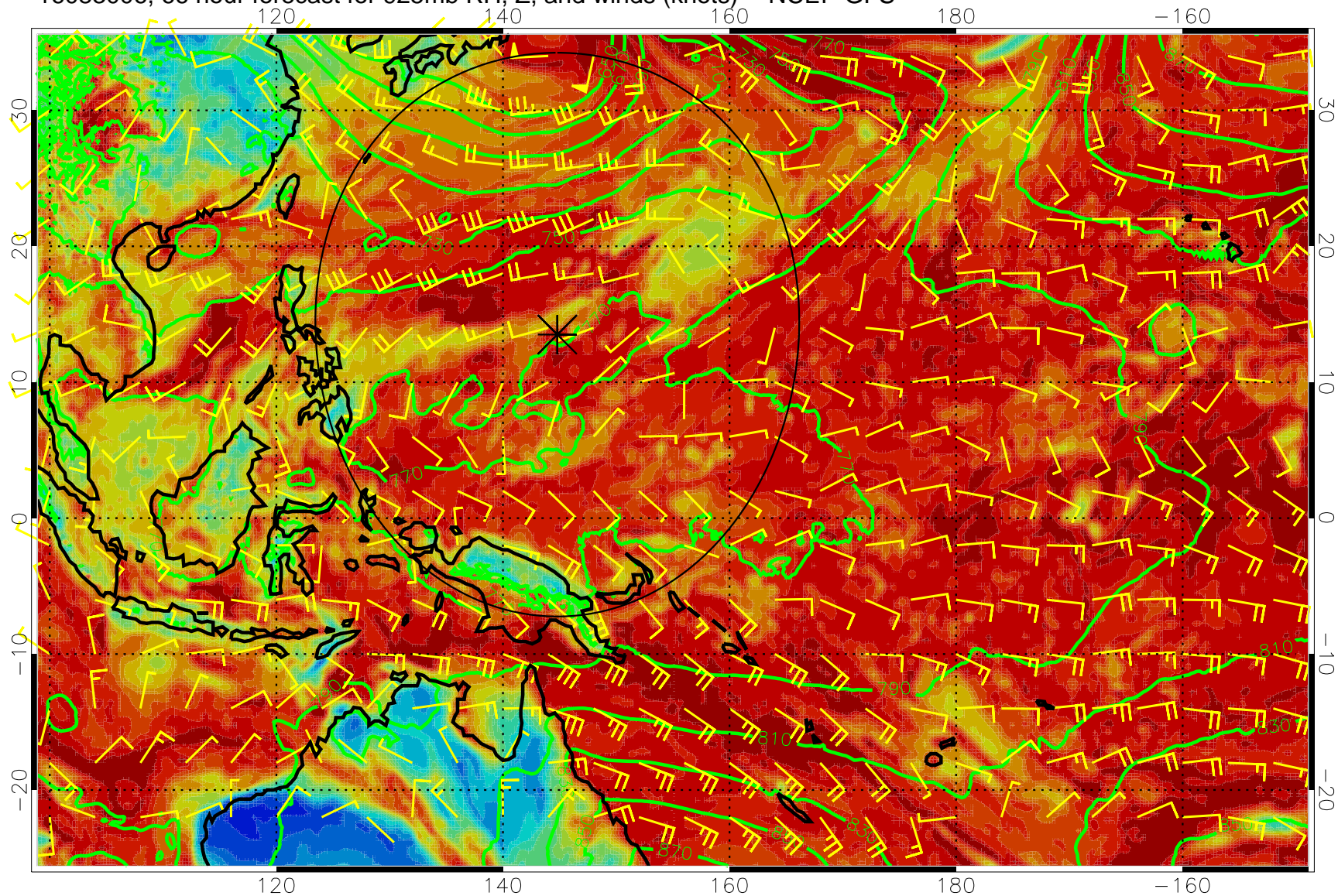
16083006, 66 hour forecast for 925mb RH, Z, and winds (knots) -- NCEP GFS
