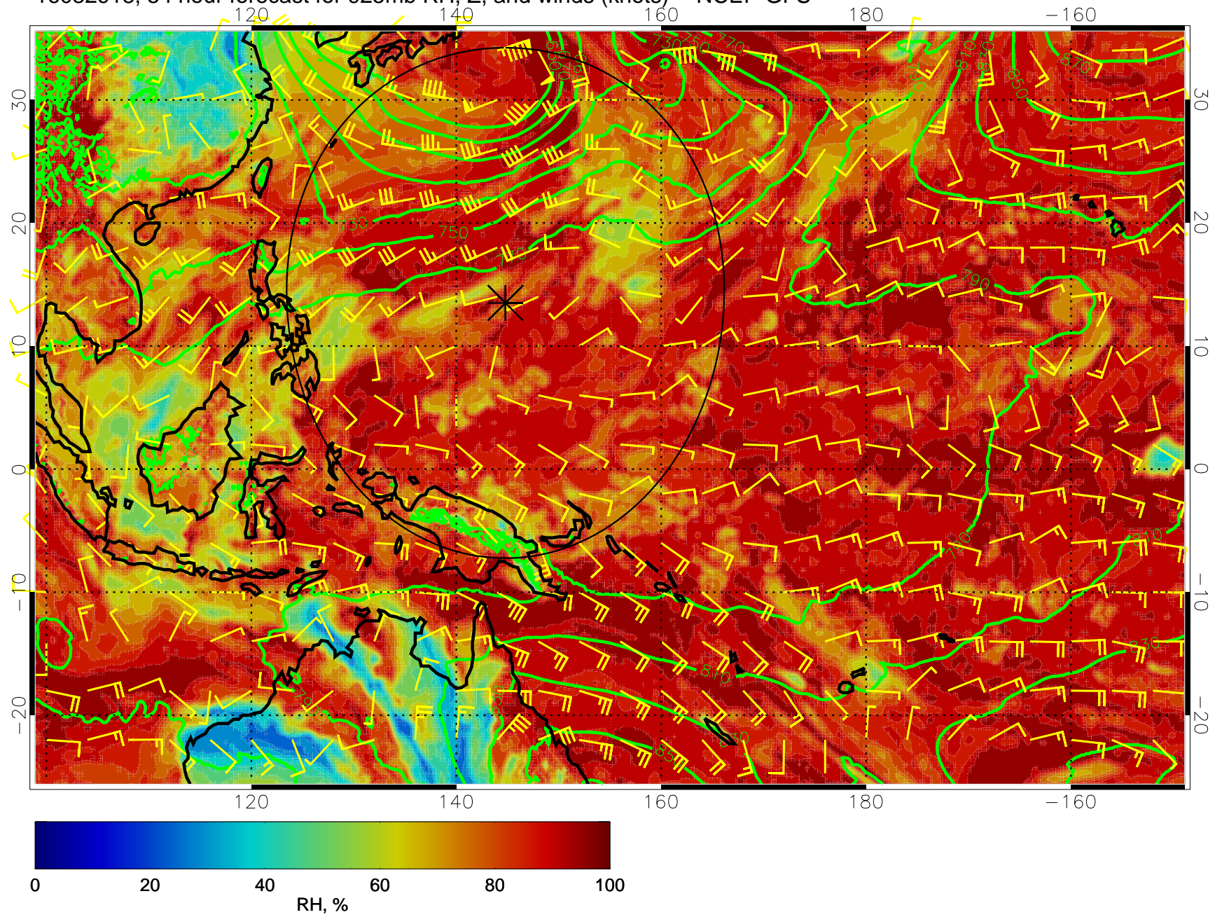
16082918, 54 hour forecast for 925mb RH, Z, and winds (knots) -- NCEP GFS
