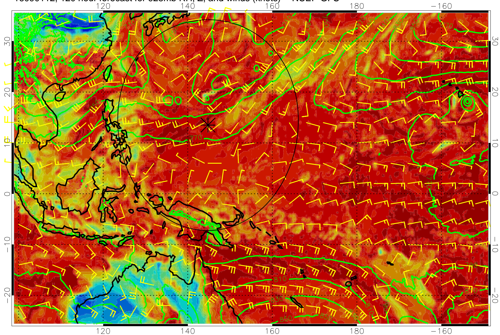
16090112, 120 hour forecast for 925mb RH, Z, and winds (knots) -- NCEP GFS
