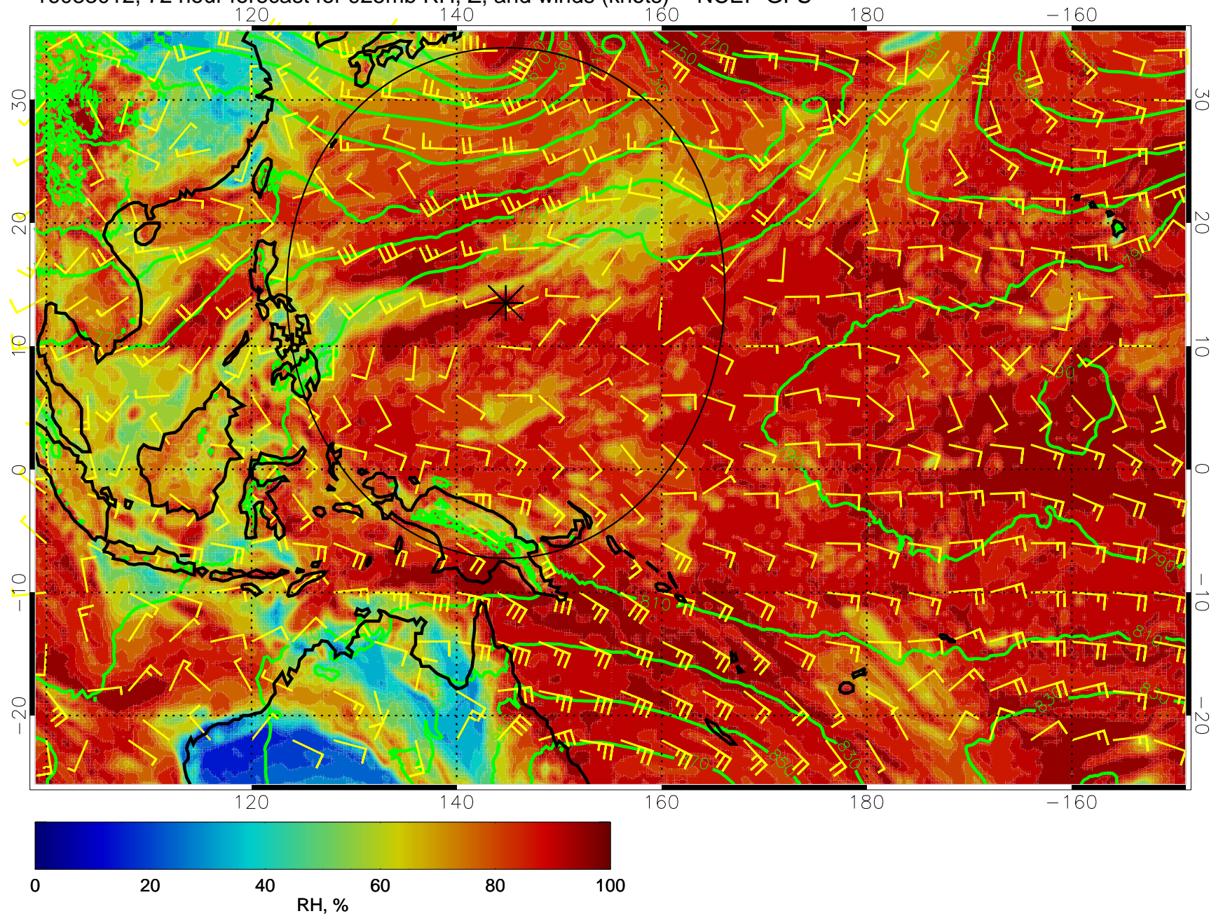
16083012, 72 hour forecast for 925mb RH, Z, and winds (knots) -- NCEP GFS
