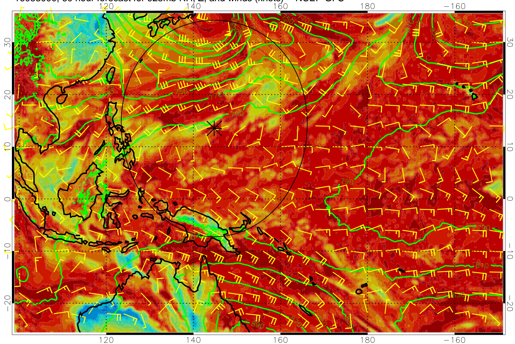
16083000, 60 hour forecast for 925mb RH, Z, and winds (knots) -- NCEP GFS
