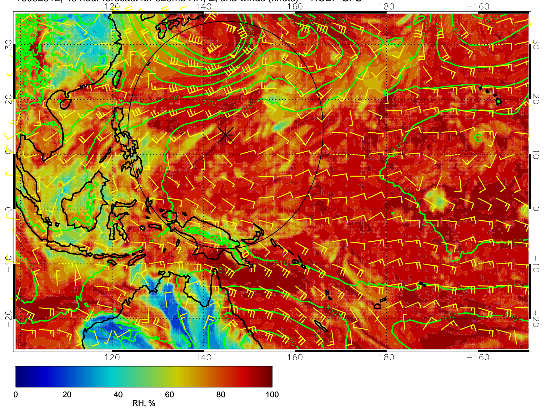
16082912, 48 hour forecast for 925mb RH, Z, and winds (knots) -- NCEP GFS
