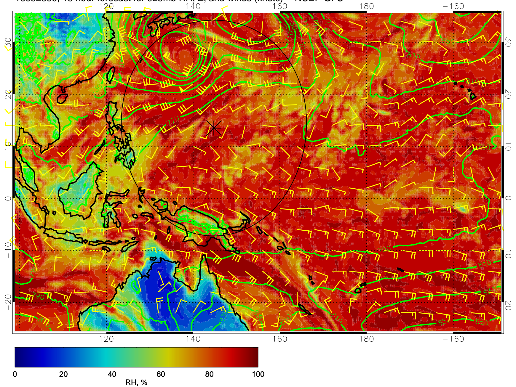
16082806, 18 hour forecast for 925mb RH, Z, and winds (knots) -- NCEP GFS
