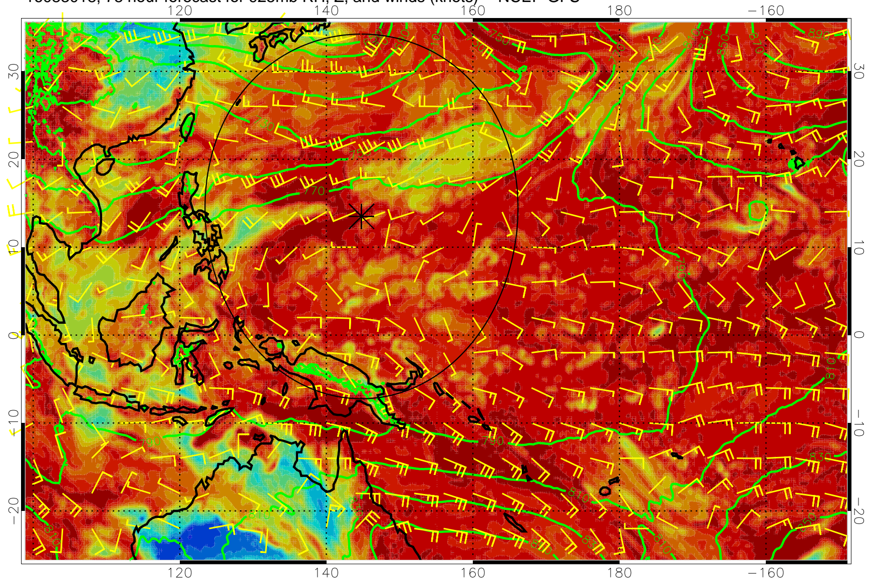
16083018, 78 hour forecast for 925mb RH, Z, and winds (knots) -- NCEP GFS
