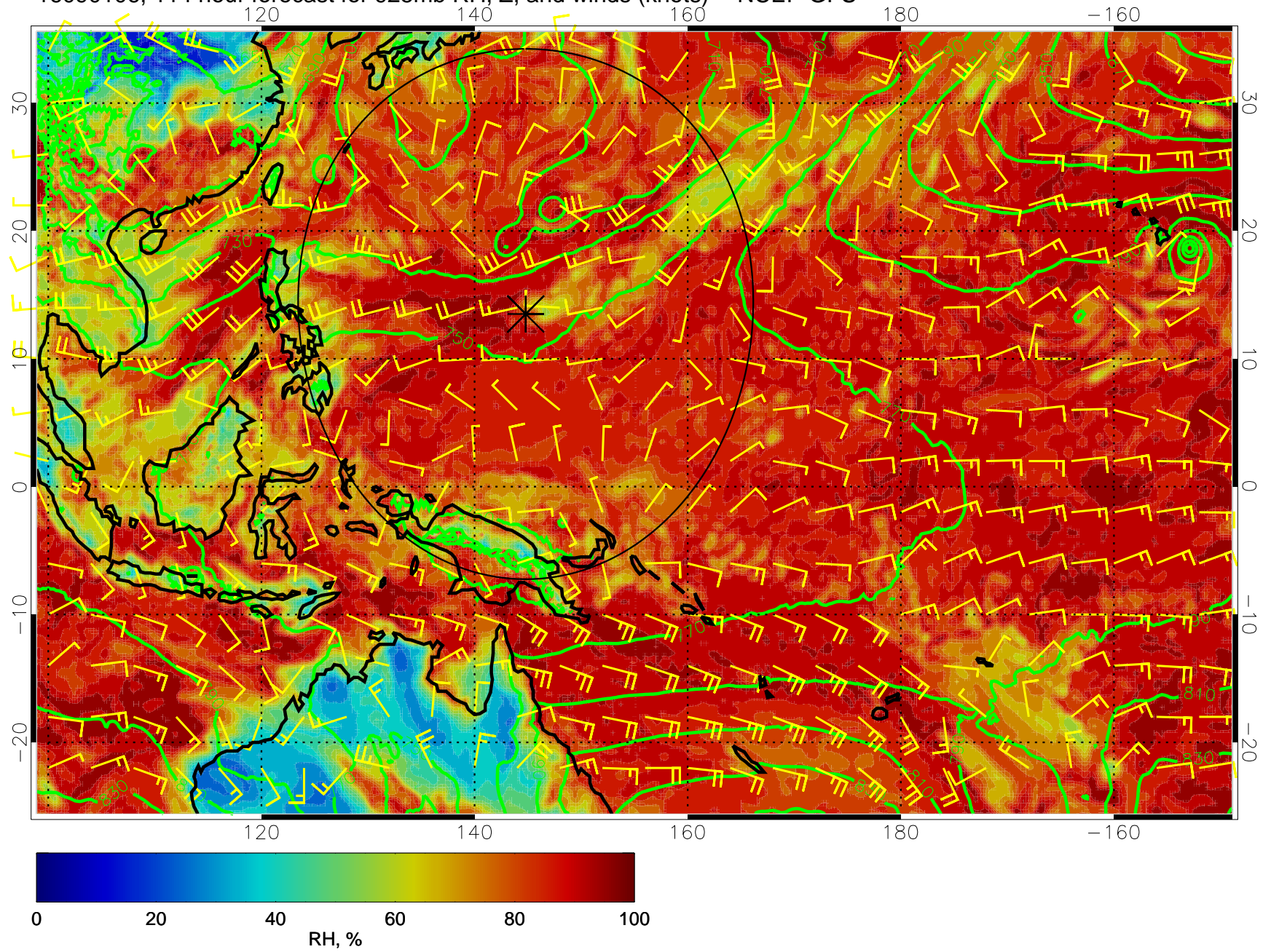
16090106, 114 hour forecast for 925mb RH, Z, and winds (knots) -- NCEP GFS
