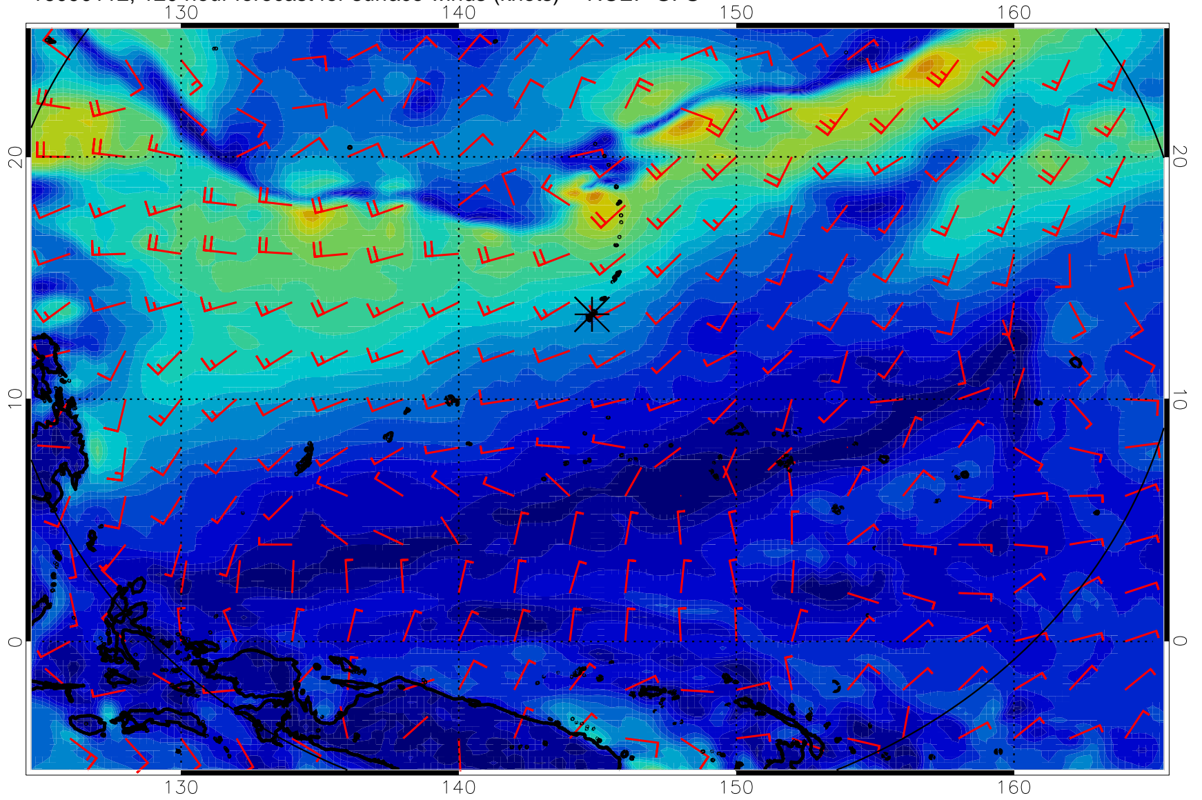
16090112, 120 hour forecast for surface winds (knots) -- NCEP GFS
