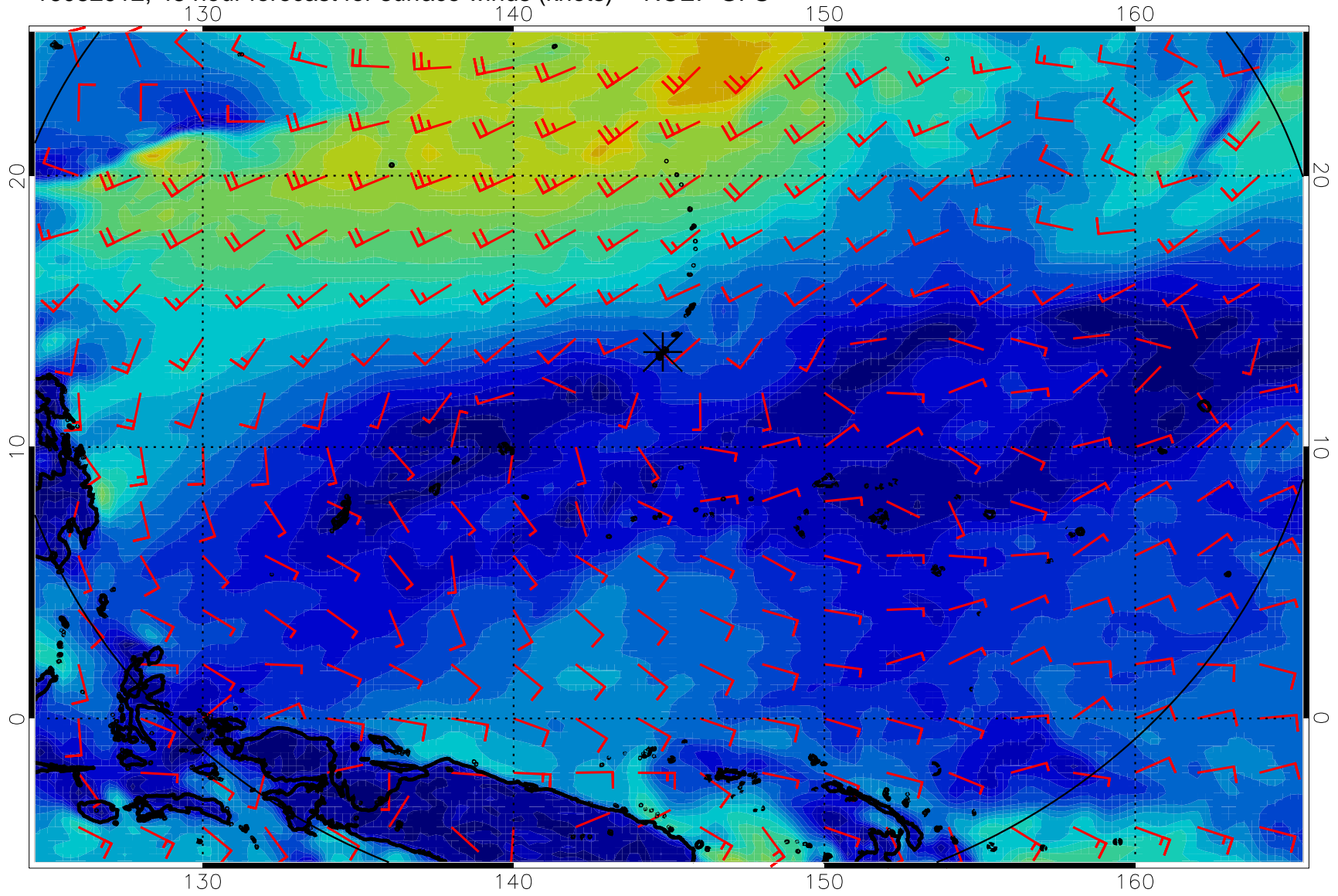
16082912, 48 hour forecast for surface winds (knots) -- NCEP GFS
