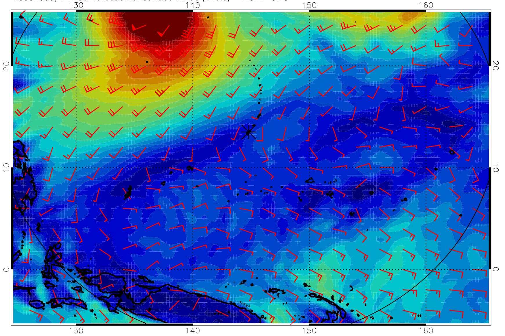
16082800, 12 hour forecast for surface winds (knots) -- NCEP GFS
