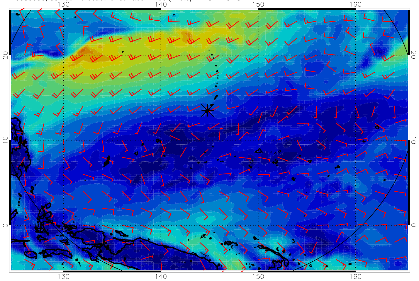
16083000, 60 hour forecast for surface winds (knots) -- NCEP GFS
