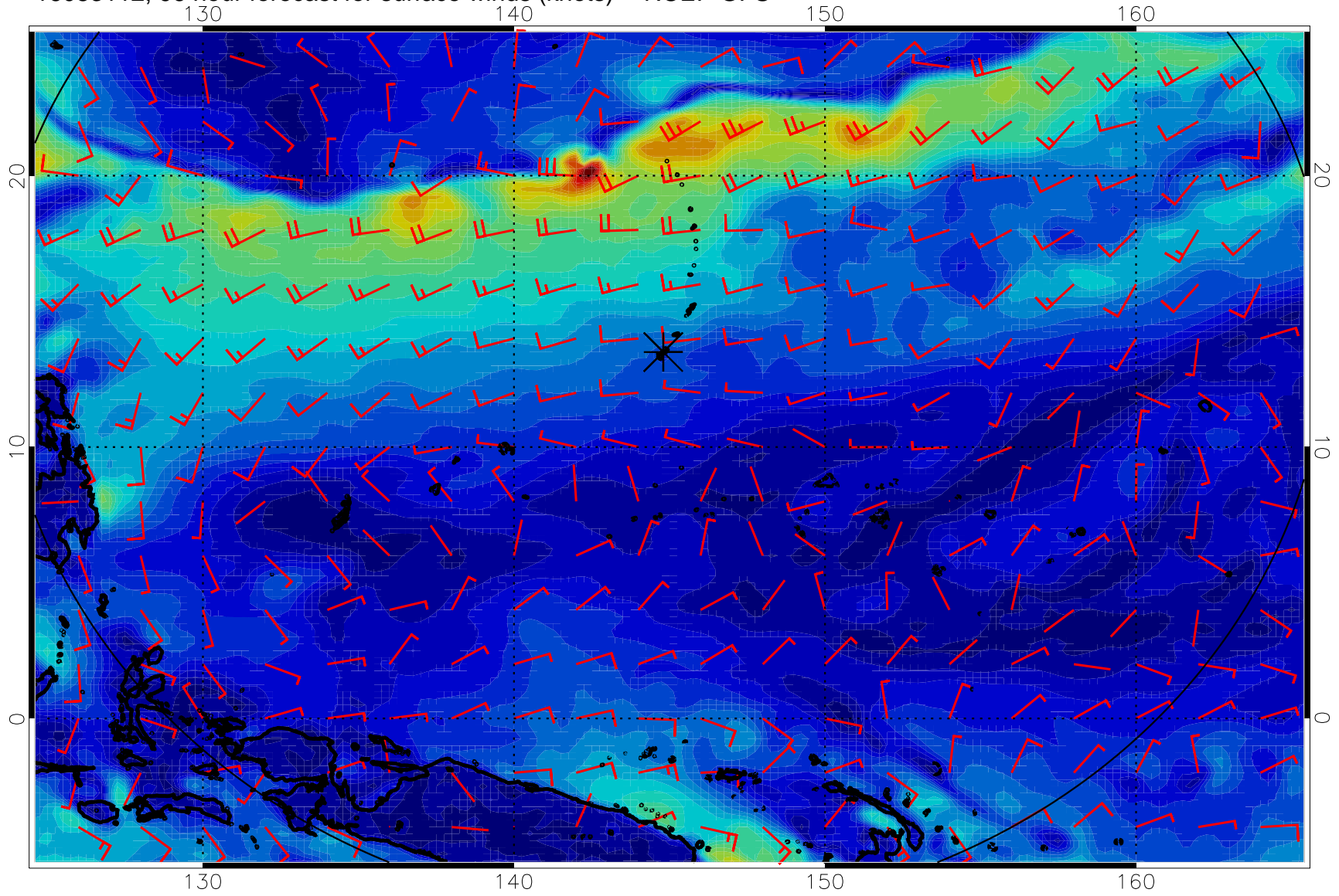
16083112, 96 hour forecast for surface winds (knots) -- NCEP GFS
