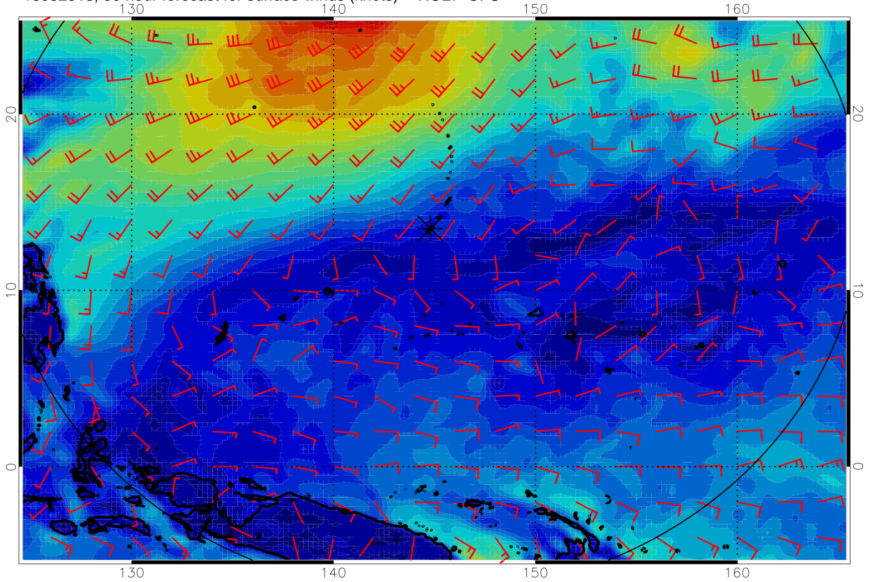
16082818, 30 hour forecast for surface winds (knots) -- NCEP GFS
