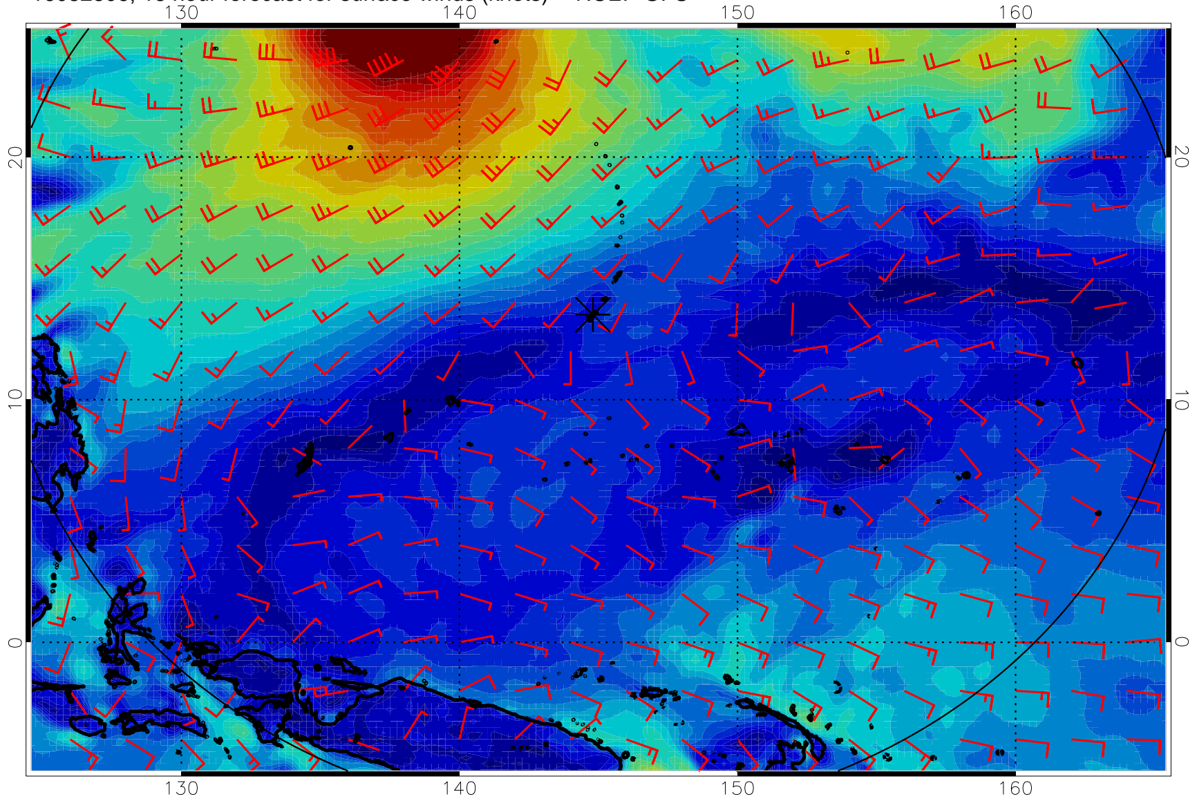
16082806, 18 hour forecast for surface winds (knots) -- NCEP GFS
