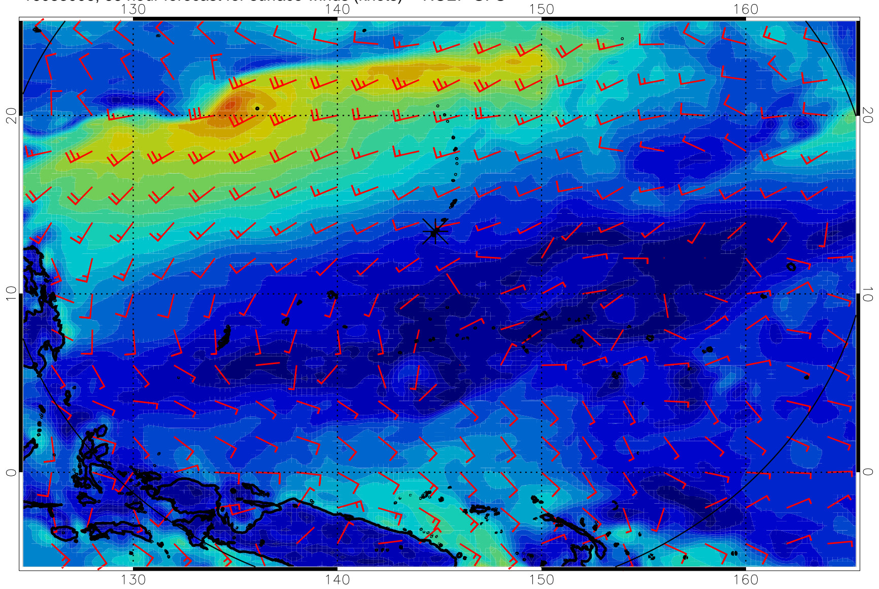
16083006, 66 hour forecast for surface winds (knots) -- NCEP GFS
