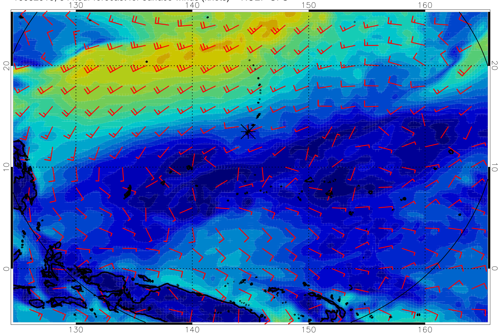
16082918, 54 hour forecast for surface winds (knots) -- NCEP GFS
