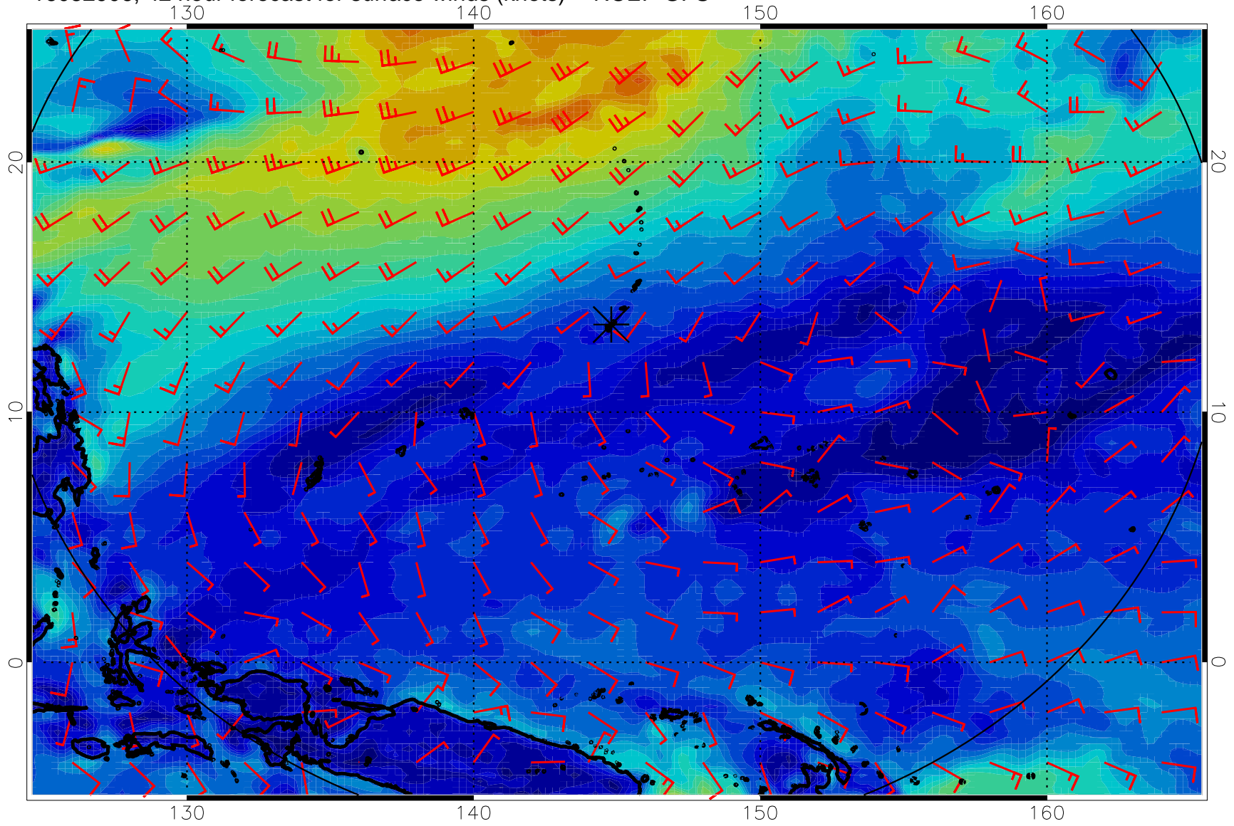
16082906, 42 hour forecast for surface winds (knots) -- NCEP GFS
