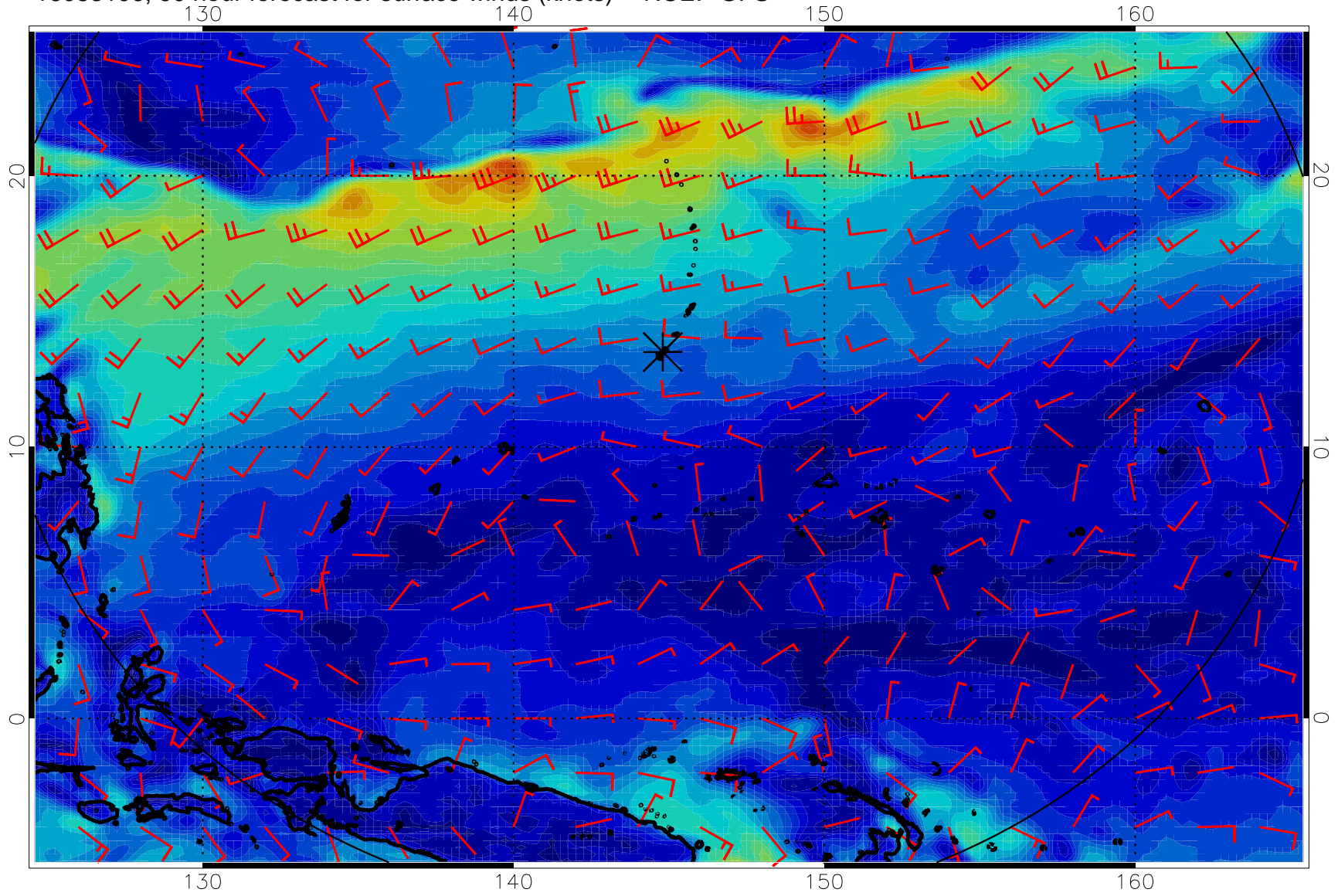
16083106, 90 hour forecast for surface winds (knots) -- NCEP GFS
