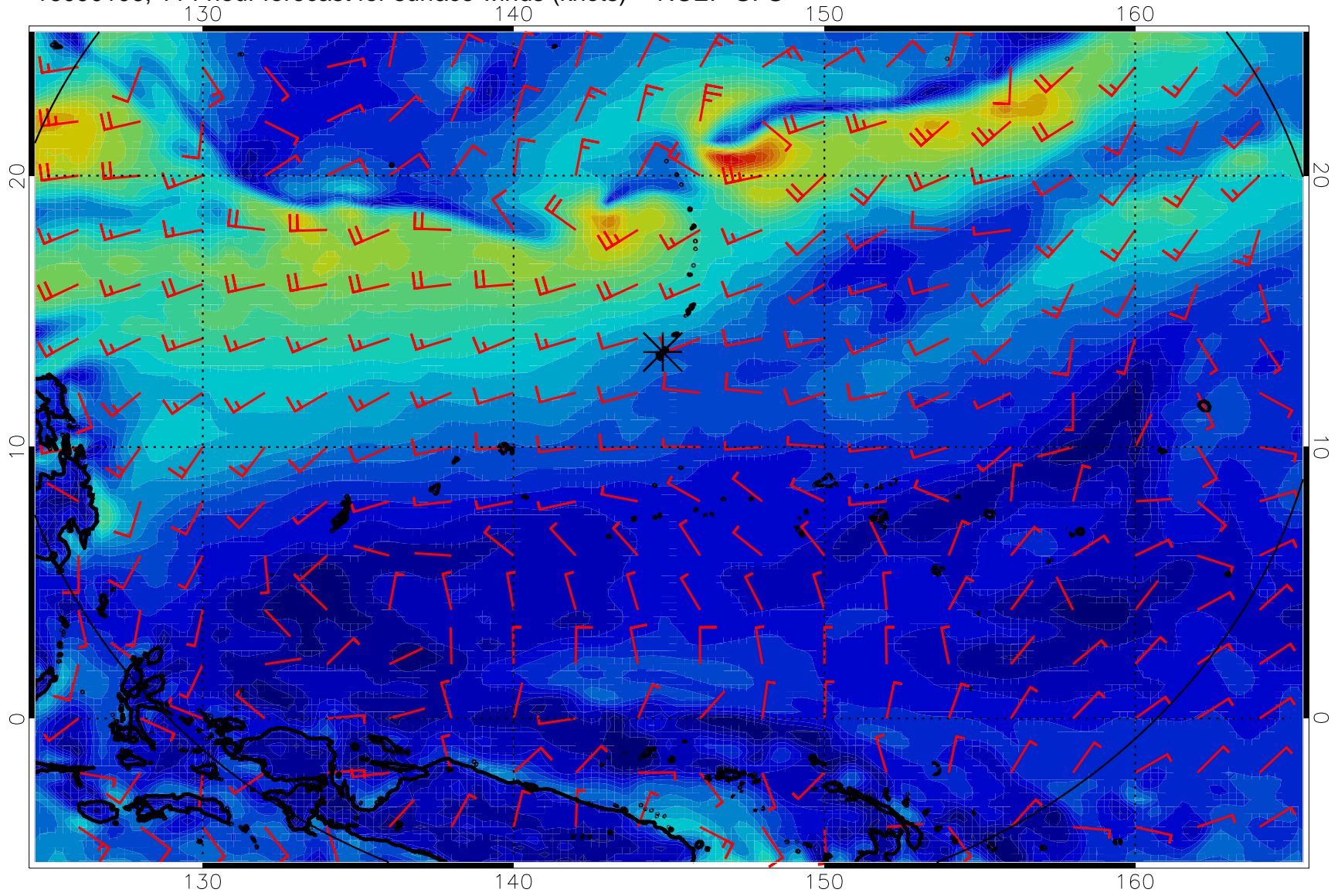
16090106, 114 hour forecast for surface winds (knots) -- NCEP GFS
