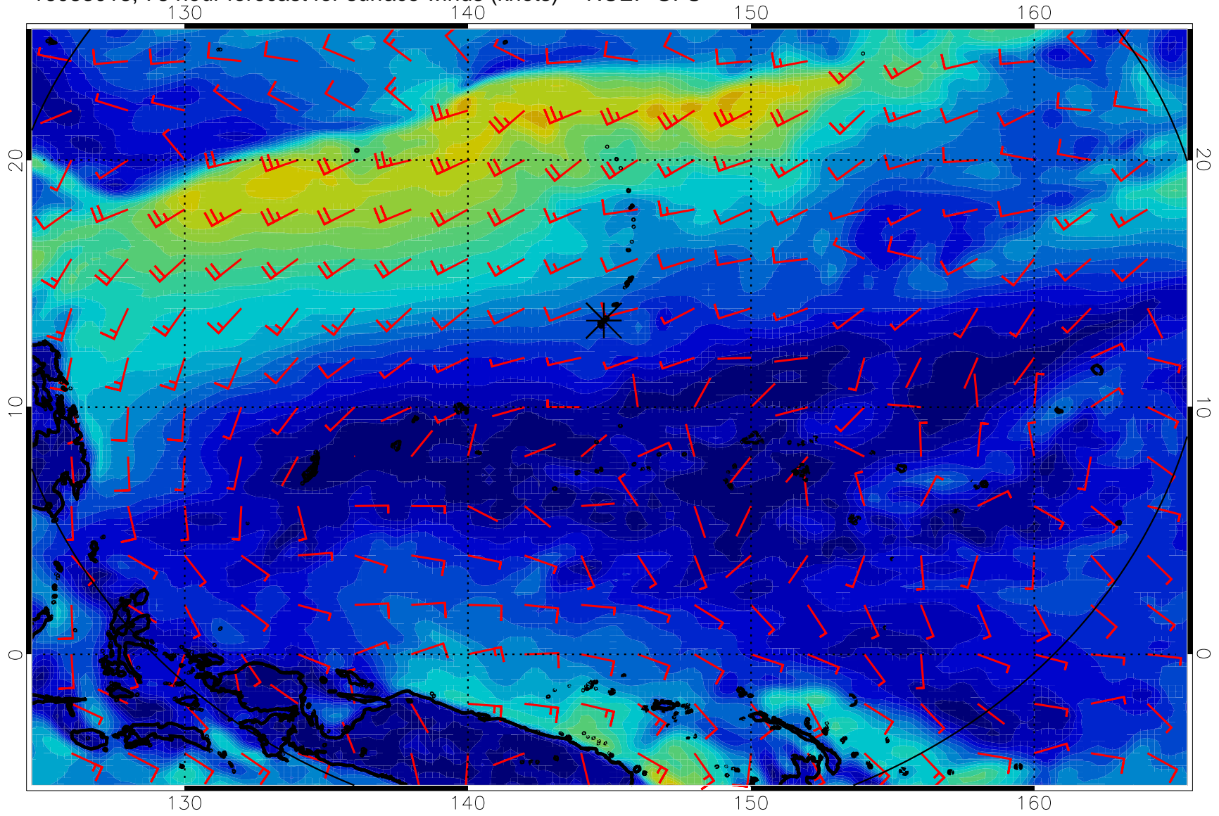
16083018, 78 hour forecast for surface winds (knots) -- NCEP GFS
