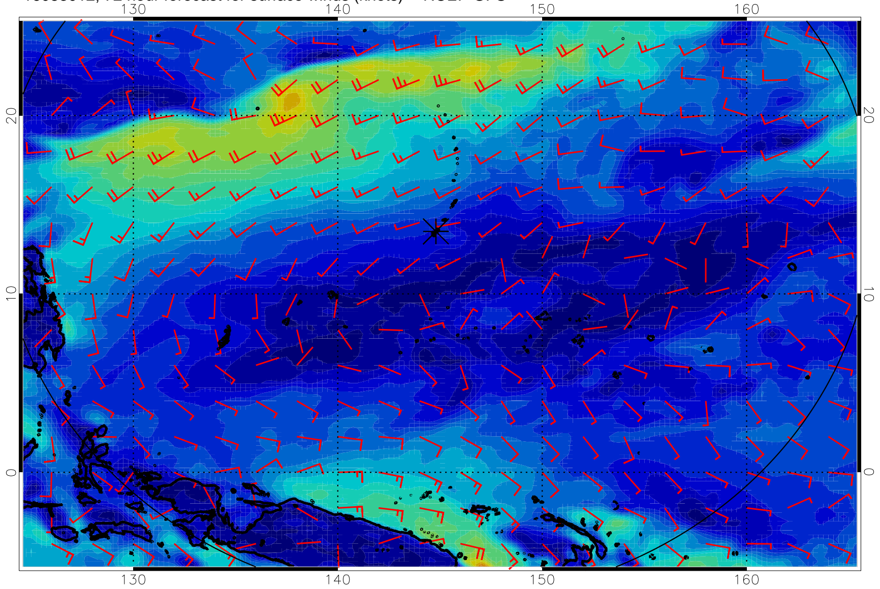
16083012, 72 hour forecast for surface winds (knots) -- NCEP GFS
