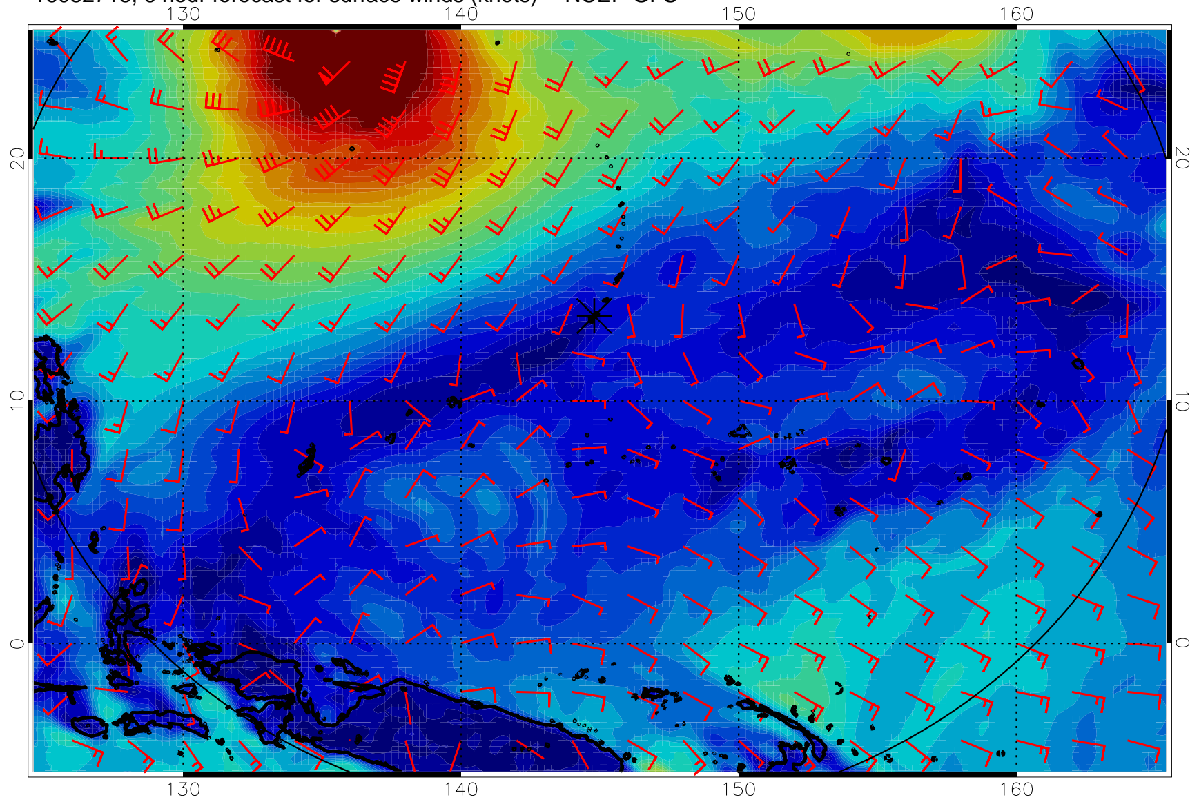
16082718, 6 hour forecast for surface winds (knots) -- NCEP GFS
