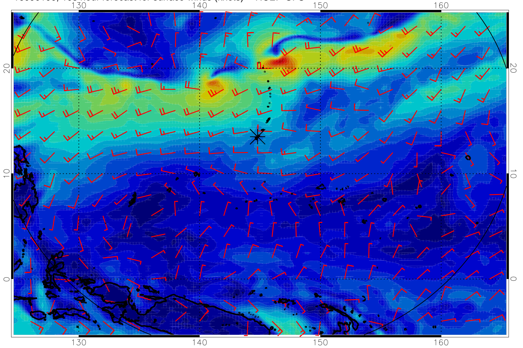
16090100, 108 hour forecast for surface winds (knots) -- NCEP GFS
