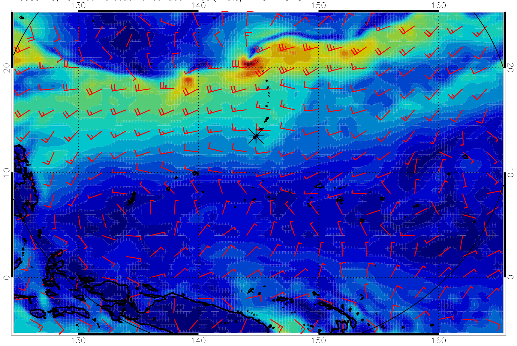
16083118, 102 hour forecast for surface winds (knots) -- NCEP GFS
