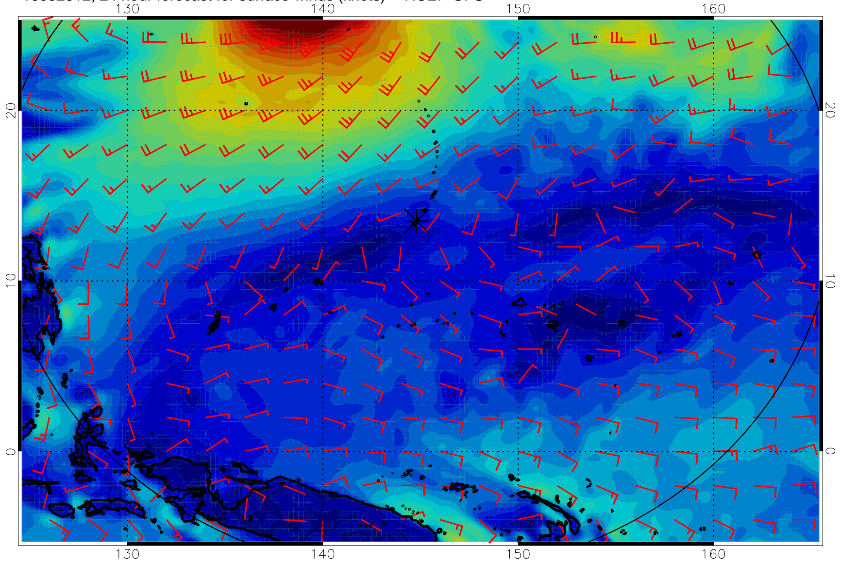
16082812, 24 hour forecast for surface winds (knots) -- NCEP GFS
