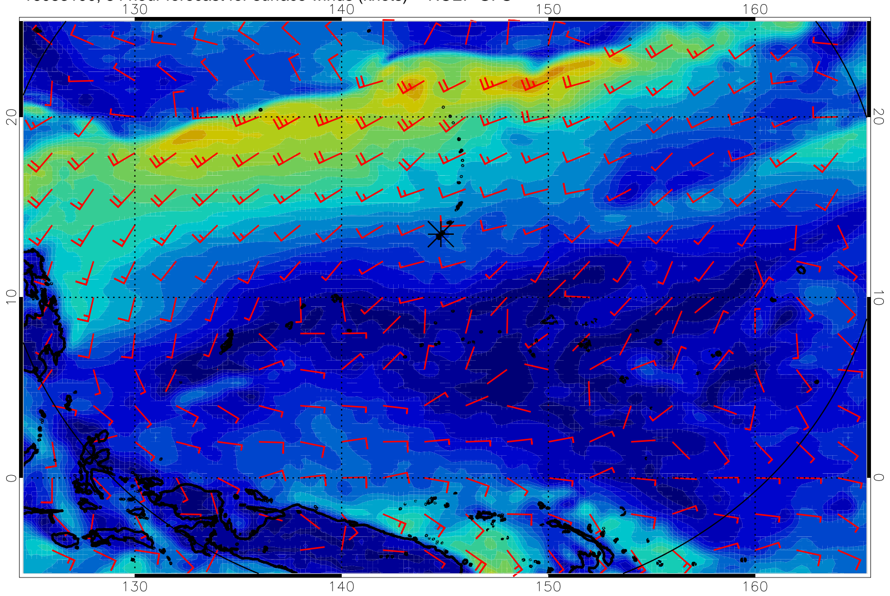
16083100, 84 hour forecast for surface winds (knots) -- NCEP GFS
