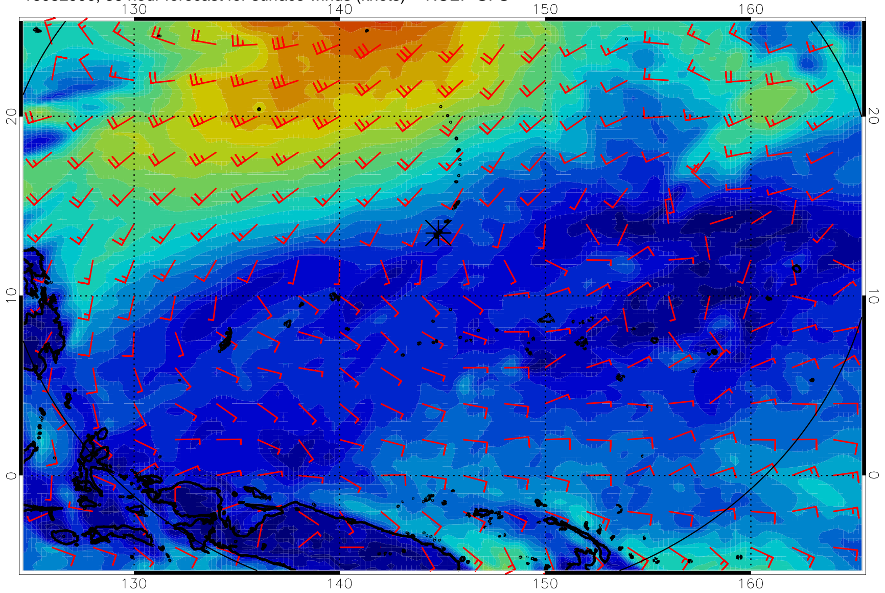
16082900, 36 hour forecast for surface winds (knots) -- NCEP GFS
