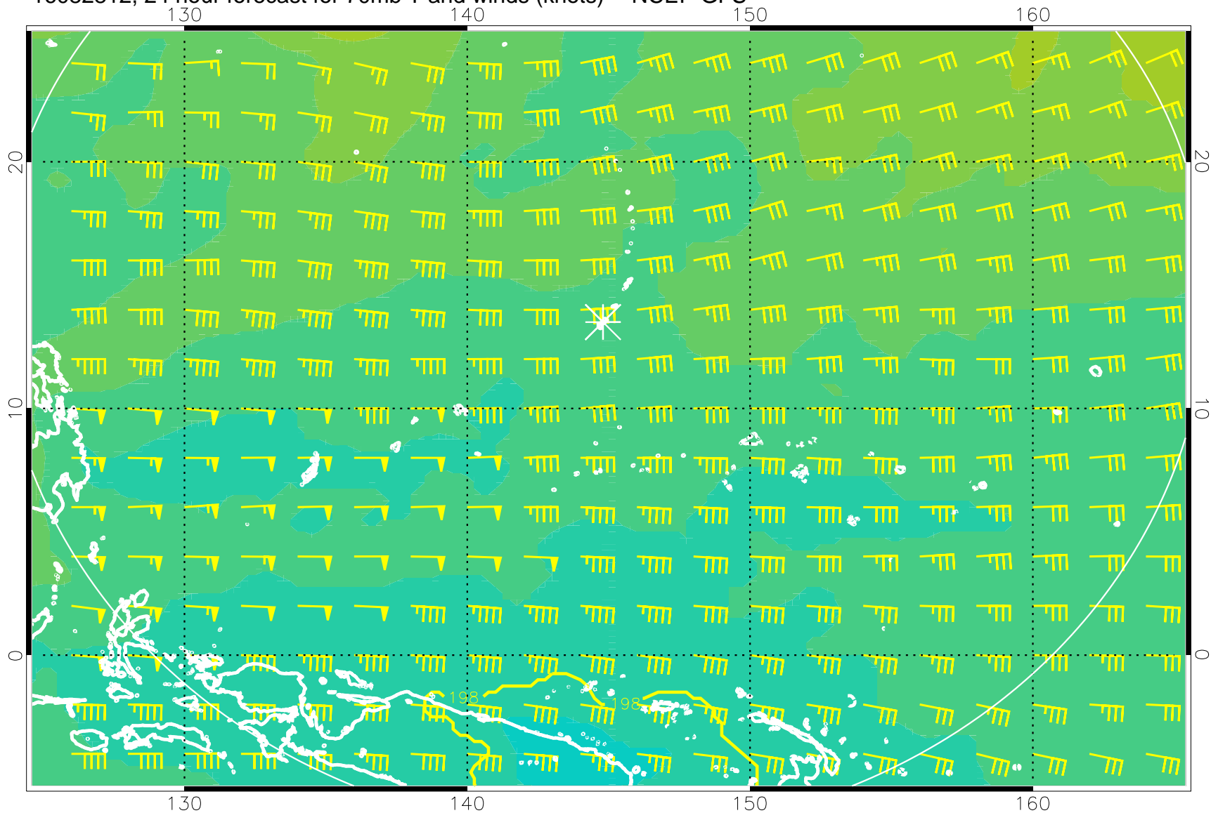
16082812, 24 hour forecast for 70mb T and winds (knots) -- NCEP GFS
