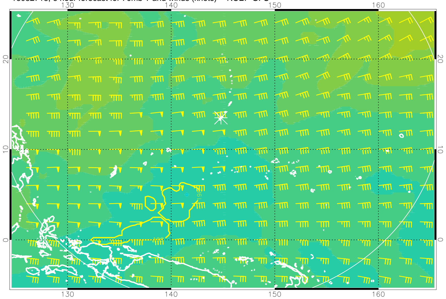
16082718, 6 hour forecast for 70mb T and winds (knots) -- NCEP GFS
