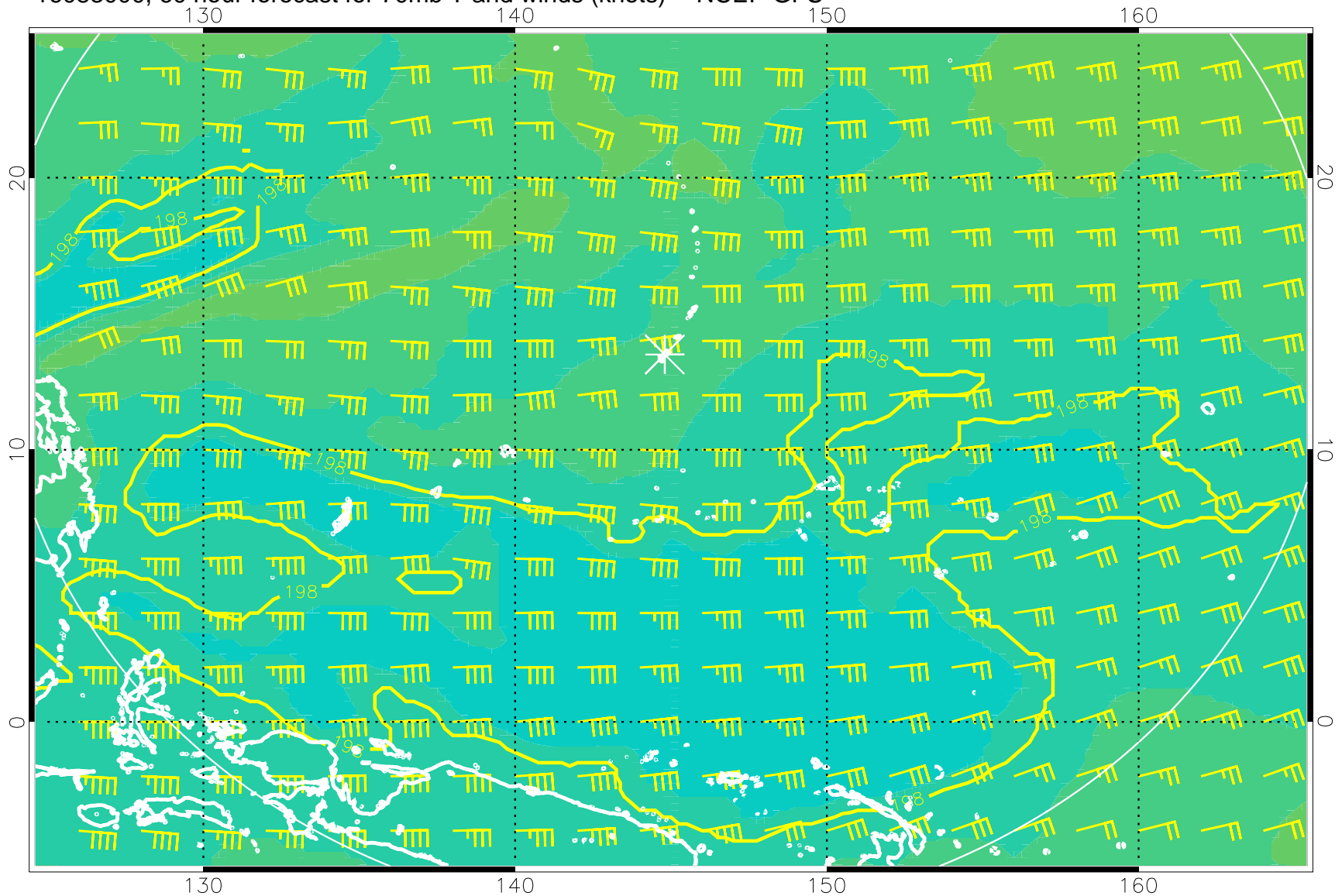
16083000, 60 hour forecast for 70mb T and winds (knots) -- NCEP GFS
