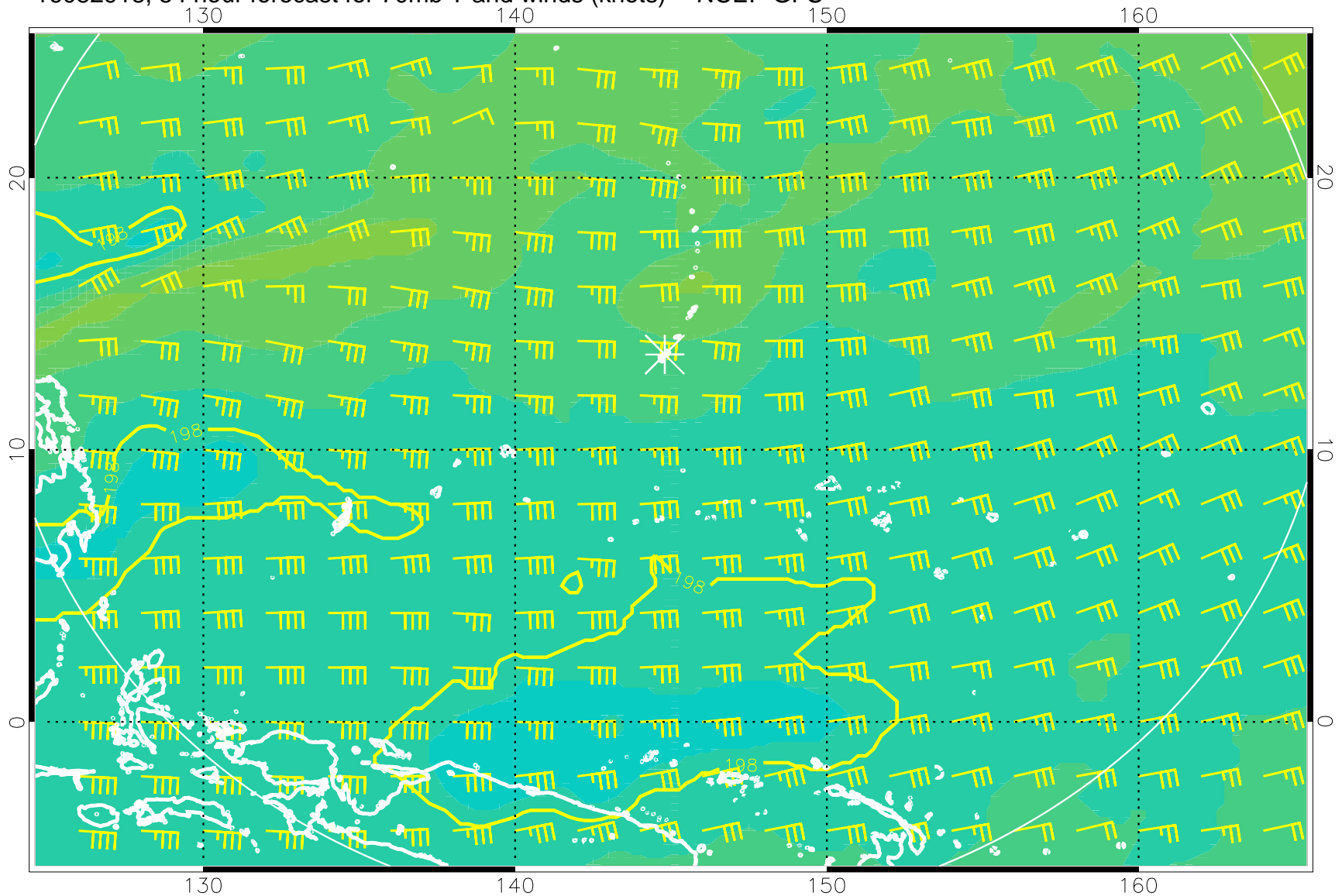
16082918, 54 hour forecast for 70mb T and winds (knots) -- NCEP GFS
