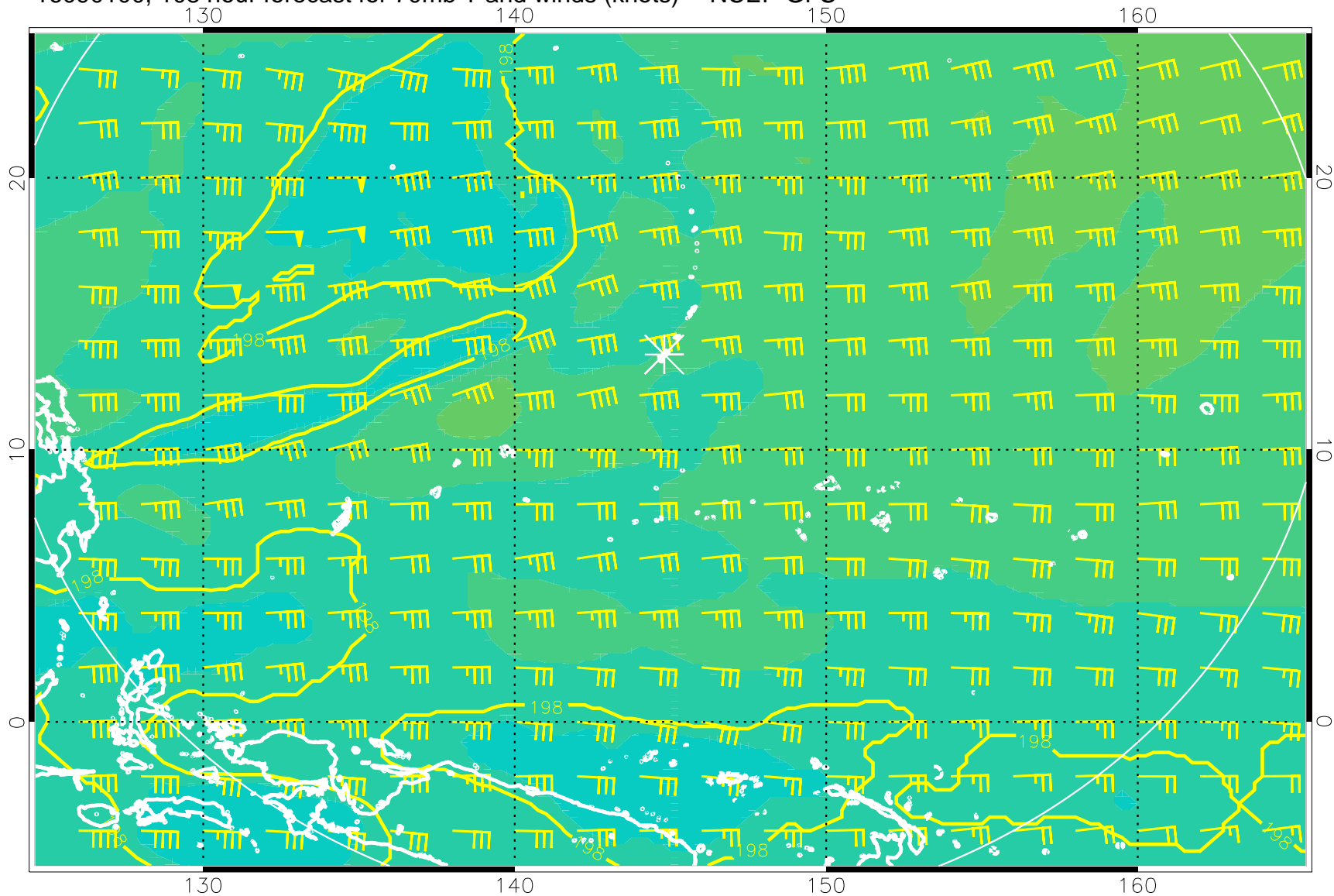
16090100, 108 hour forecast for 70mb T and winds (knots) -- NCEP GFS
