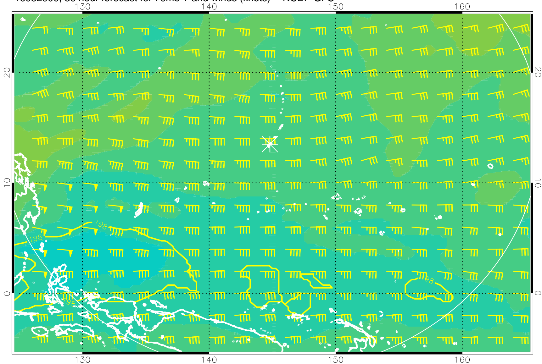
16082900, 36 hour forecast for 70mb T and winds (knots) -- NCEP GFS
