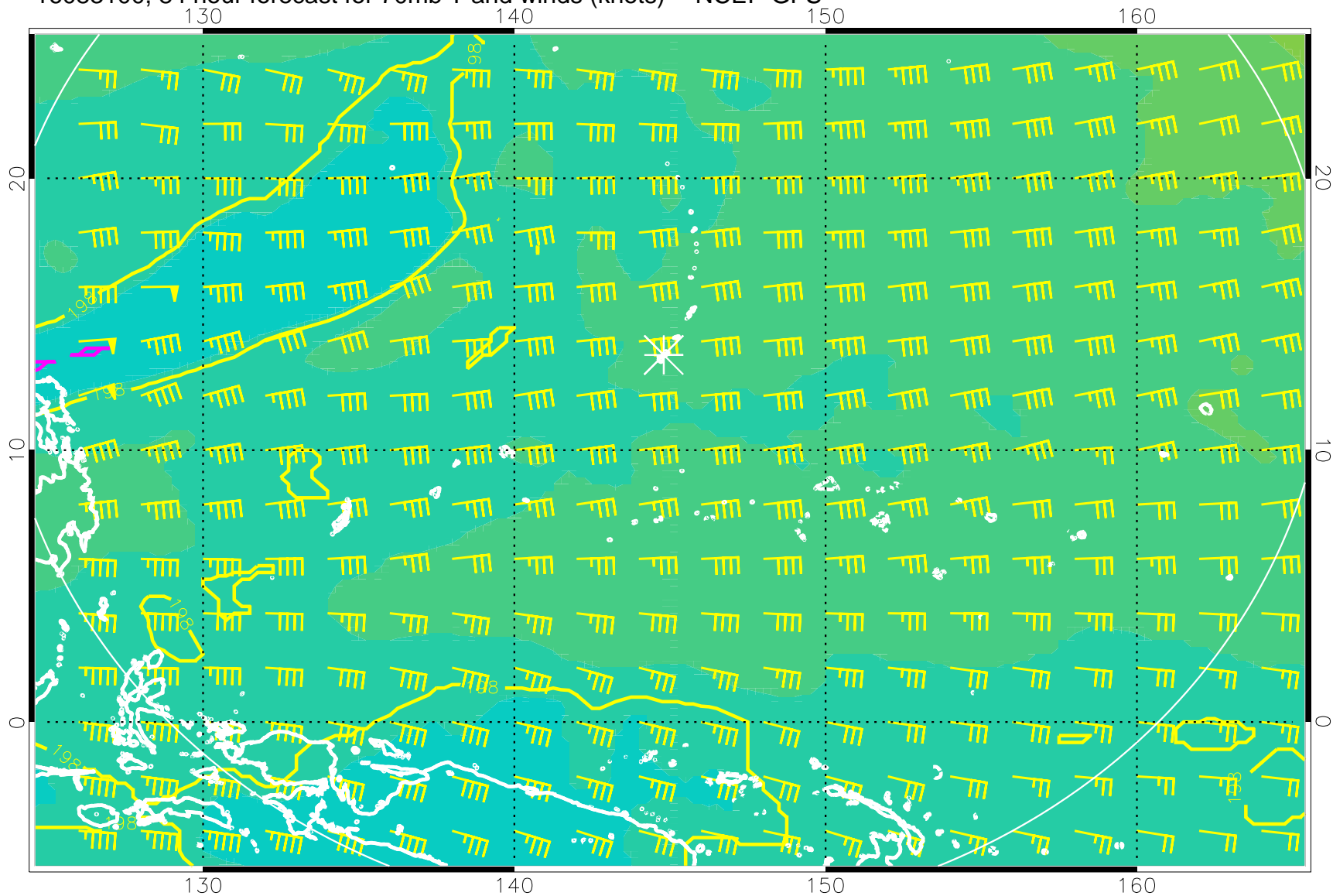
16083100, 84 hour forecast for 70mb T and winds (knots) -- NCEP GFS
