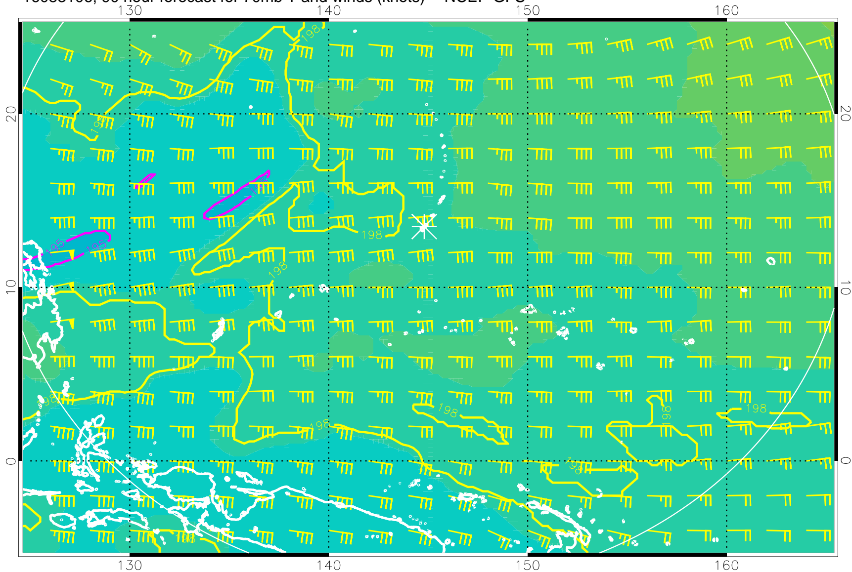
16083106, 90 hour forecast for 70mb T and winds (knots) -- NCEP GFS
