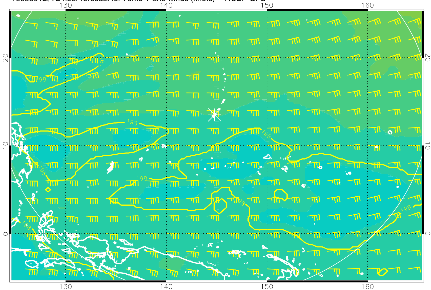
16083012, 72 hour forecast for 70mb T and winds (knots) -- NCEP GFS
