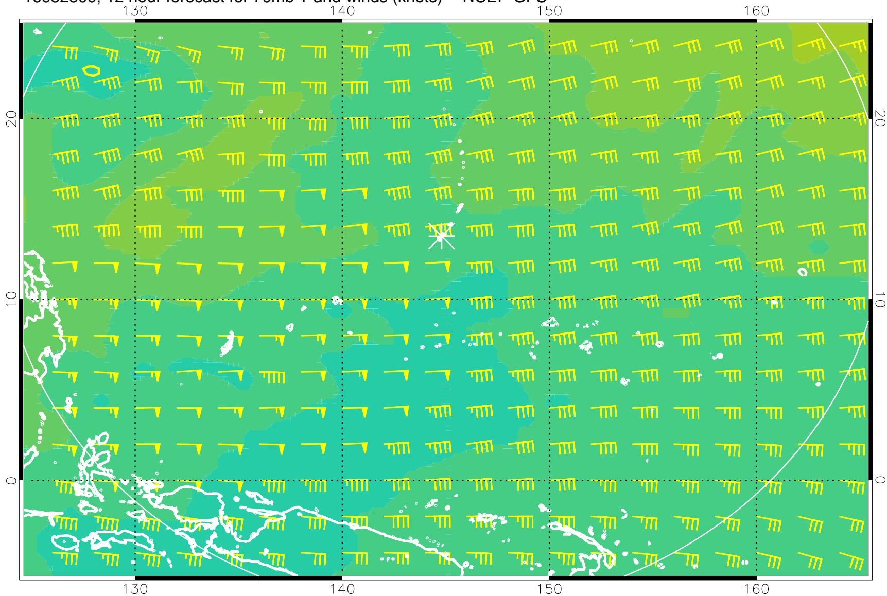
16082800, 12 hour forecast for 70mb T and winds (knots) -- NCEP GFS
