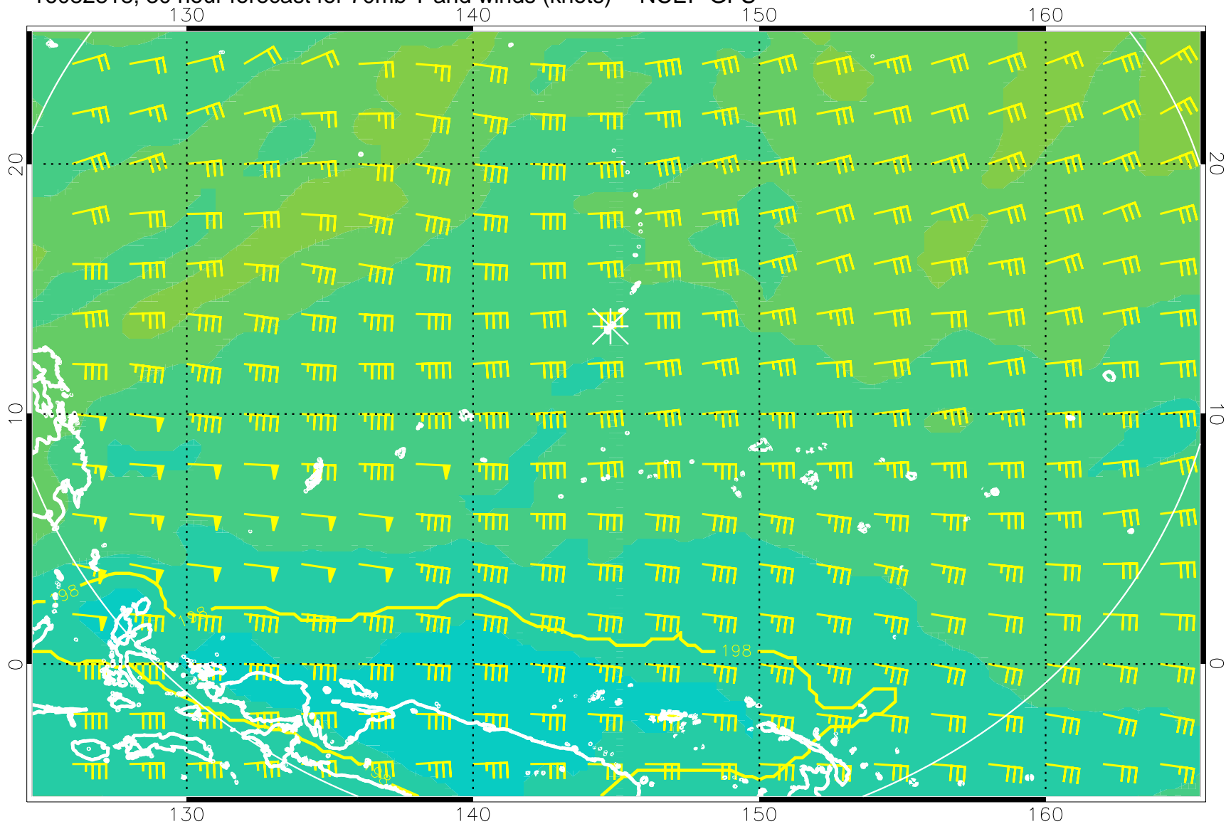
16082818, 30 hour forecast for 70mb T and winds (knots) -- NCEP GFS
