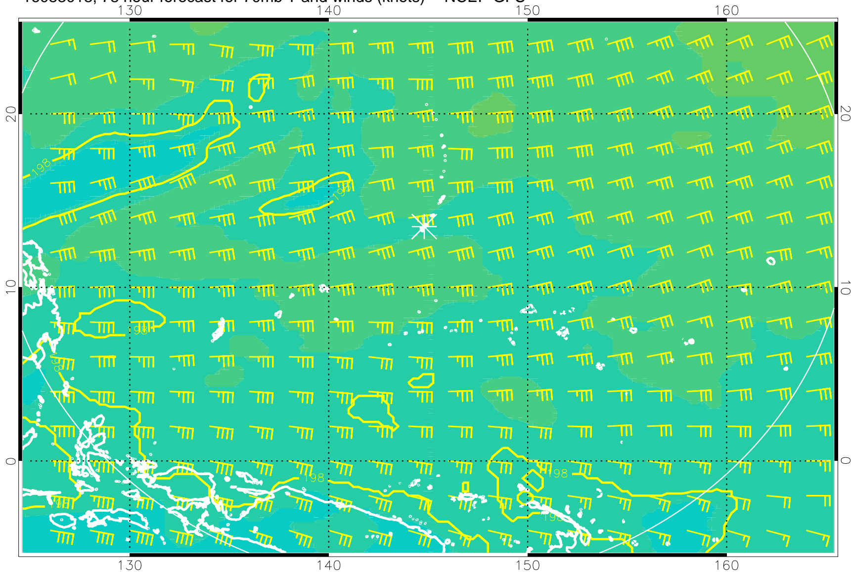
16083018, 78 hour forecast for 70mb T and winds (knots) -- NCEP GFS
