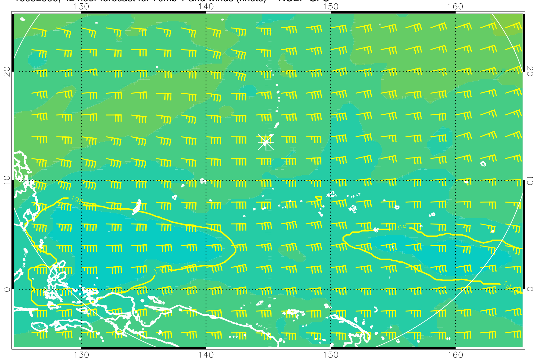
16082906, 42 hour forecast for 70mb T and winds (knots) -- NCEP GFS
