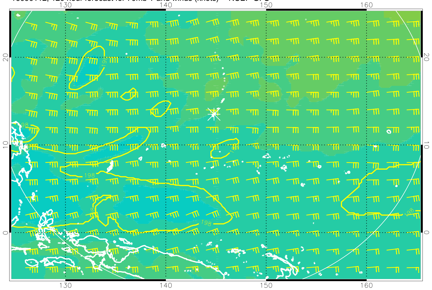
16090112, 120 hour forecast for 70mb T and winds (knots) -- NCEP GFS
