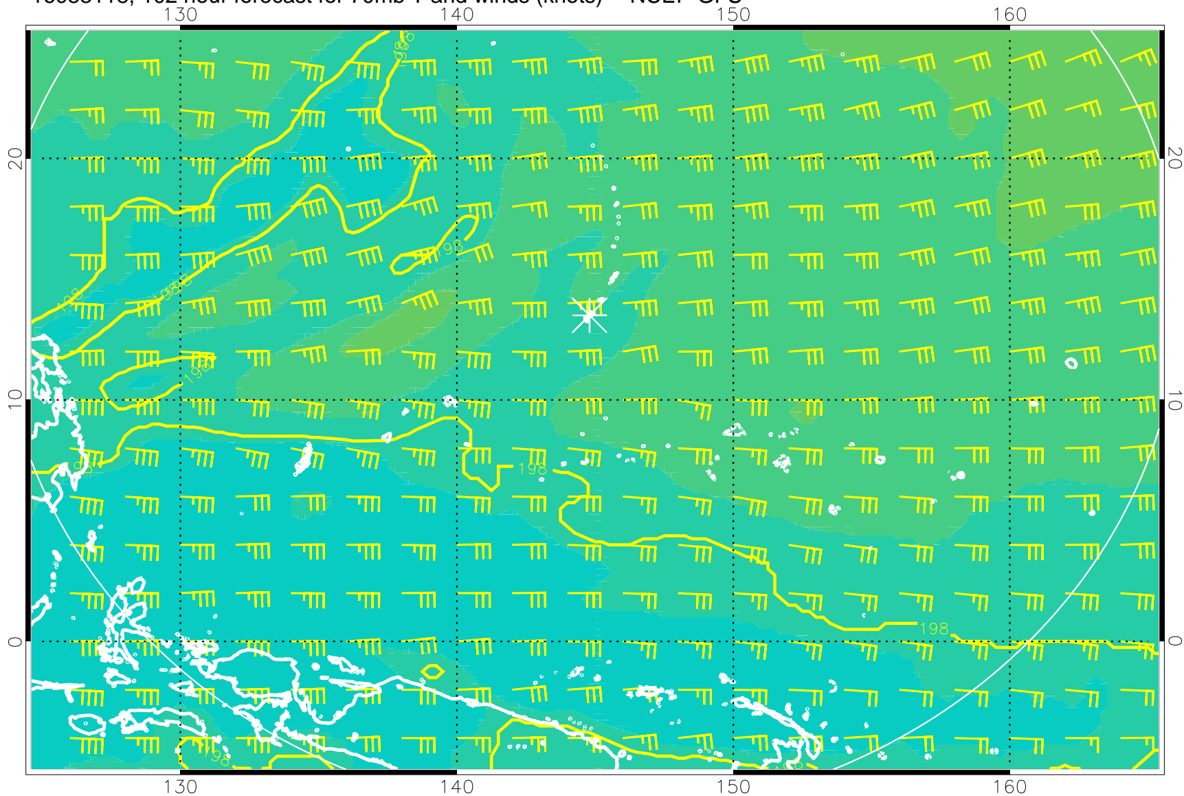
16083118, 102 hour forecast for 70mb T and winds (knots) -- NCEP GFS
