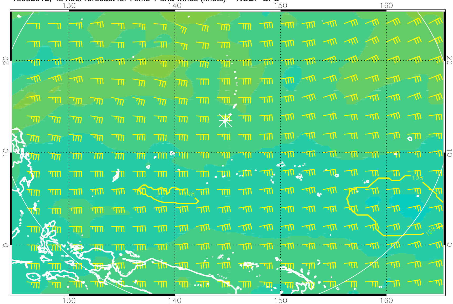
16082912, 48 hour forecast for 70mb T and winds (knots) -- NCEP GFS
