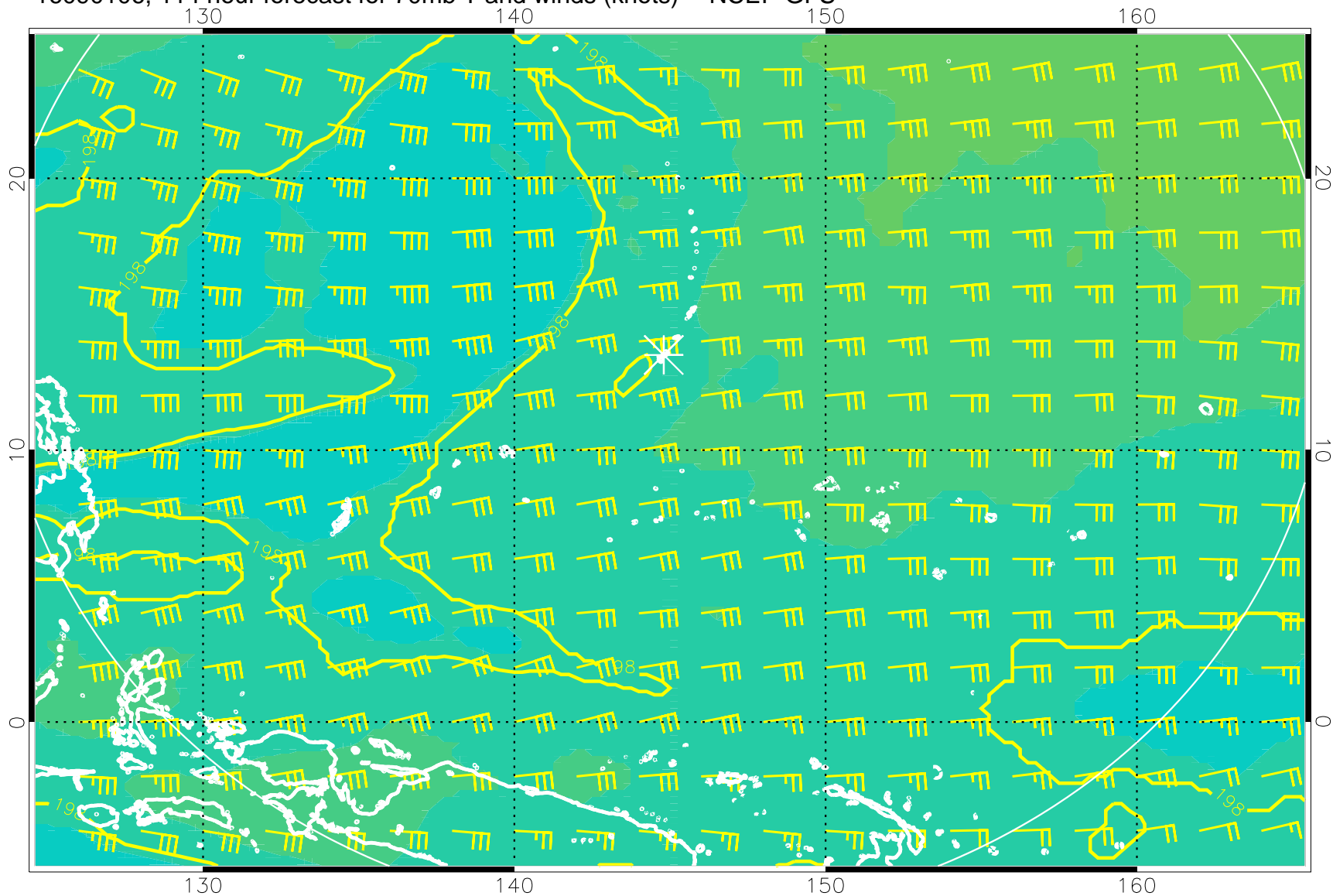
16090106, 114 hour forecast for 70mb T and winds (knots) -- NCEP GFS
