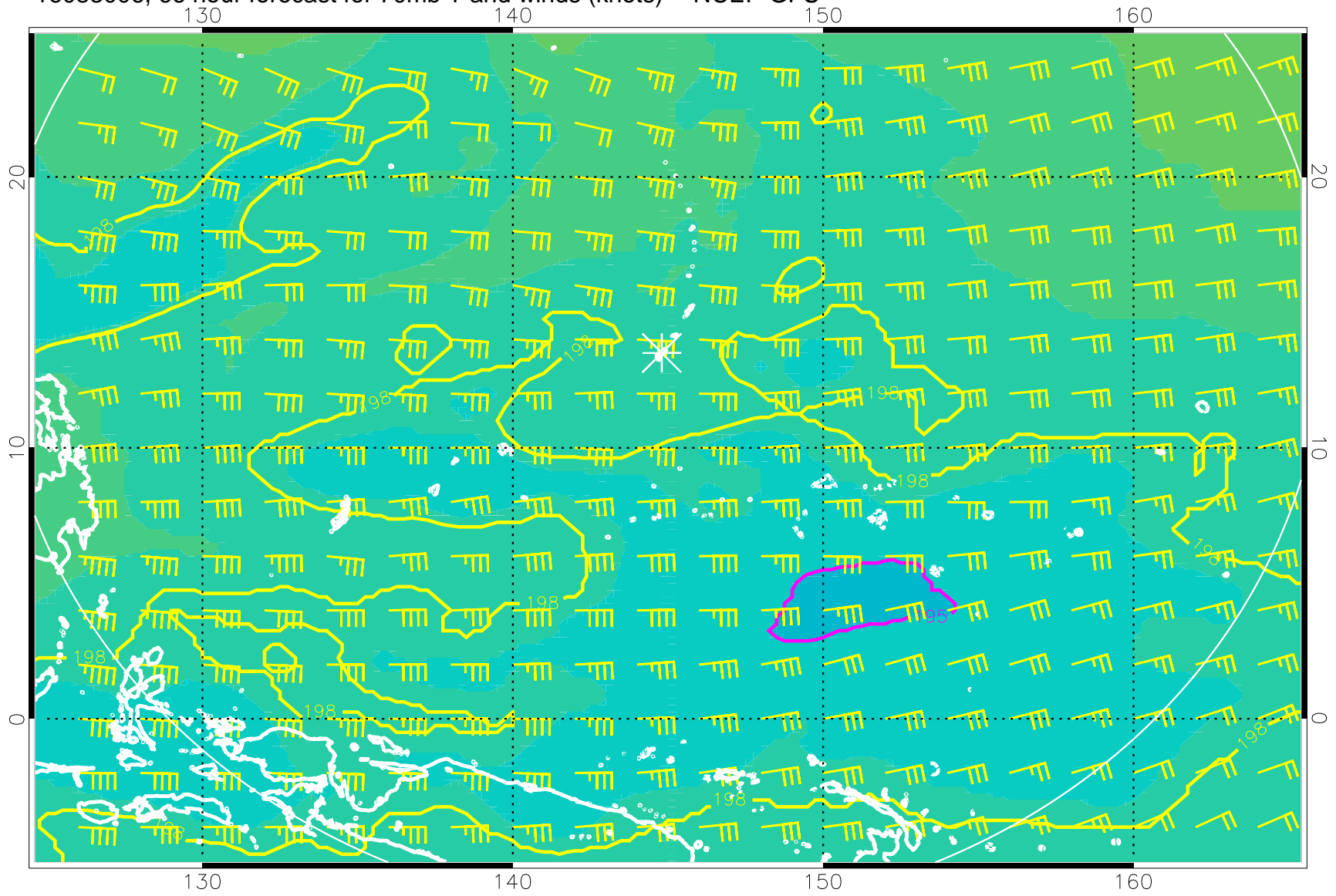
16083006, 66 hour forecast for 70mb T and winds (knots) -- NCEP GFS
