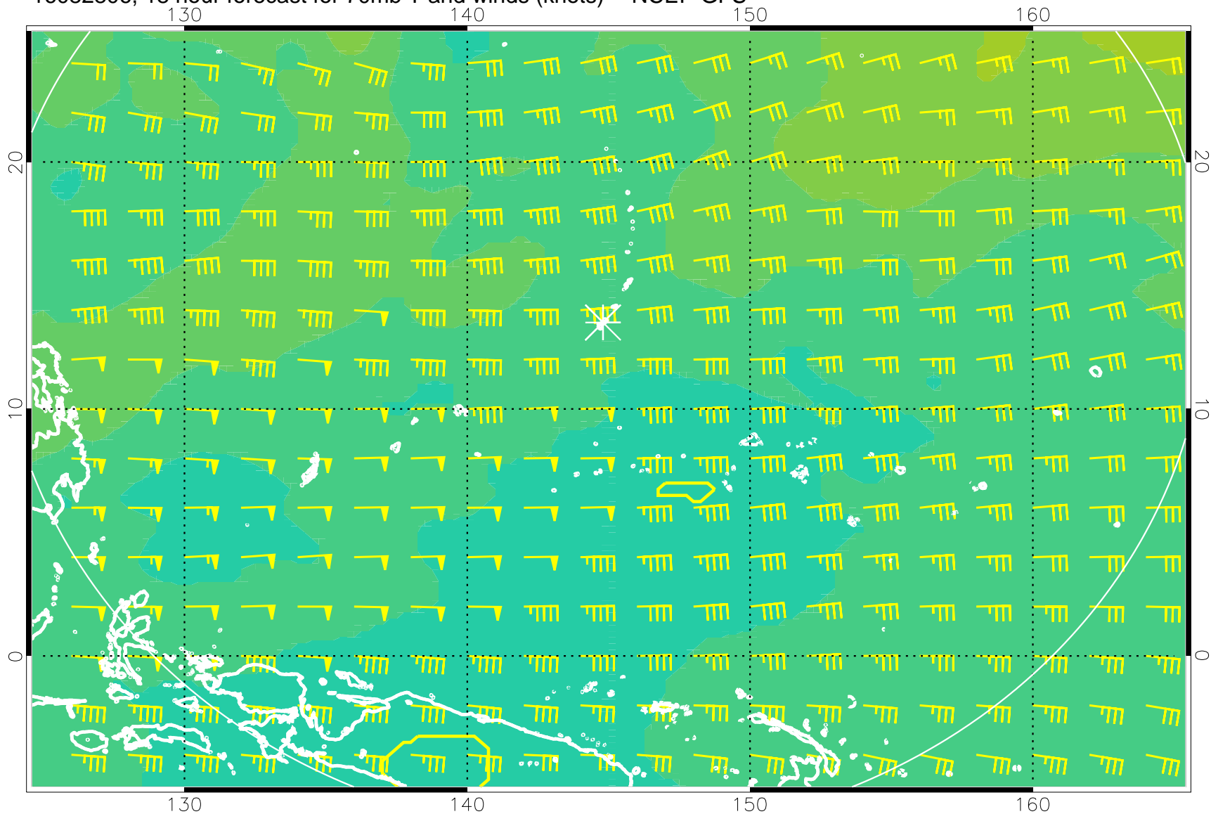
16082806, 18 hour forecast for 70mb T and winds (knots) -- NCEP GFS
