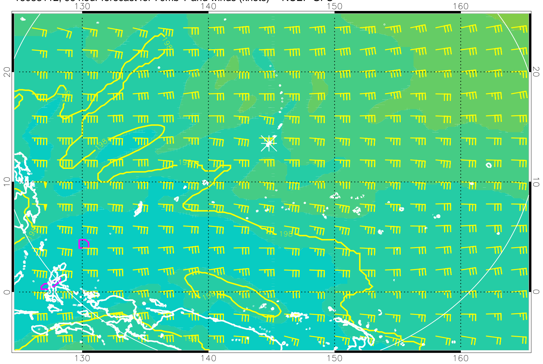
16083112, 96 hour forecast for 70mb T and winds (knots) -- NCEP GFS
