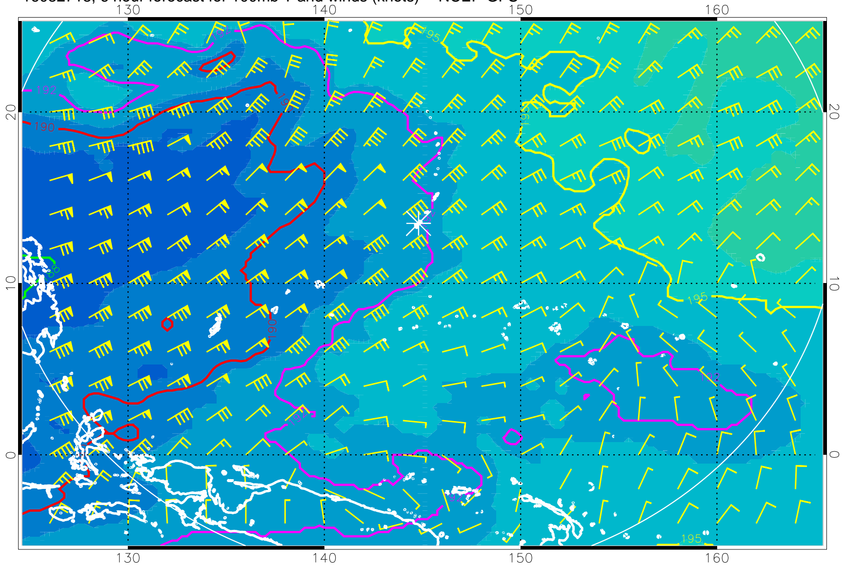
16082718, 6 hour forecast for 100mb T and winds (knots) -- NCEP GFS
