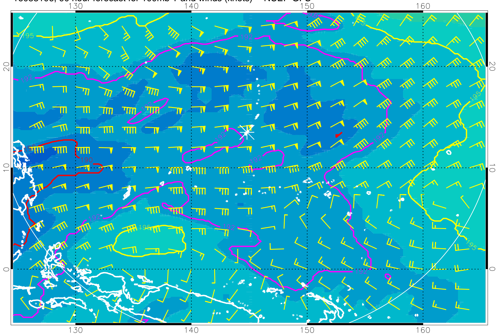
16083106, 90 hour forecast for 100mb T and winds (knots) -- NCEP GFS
