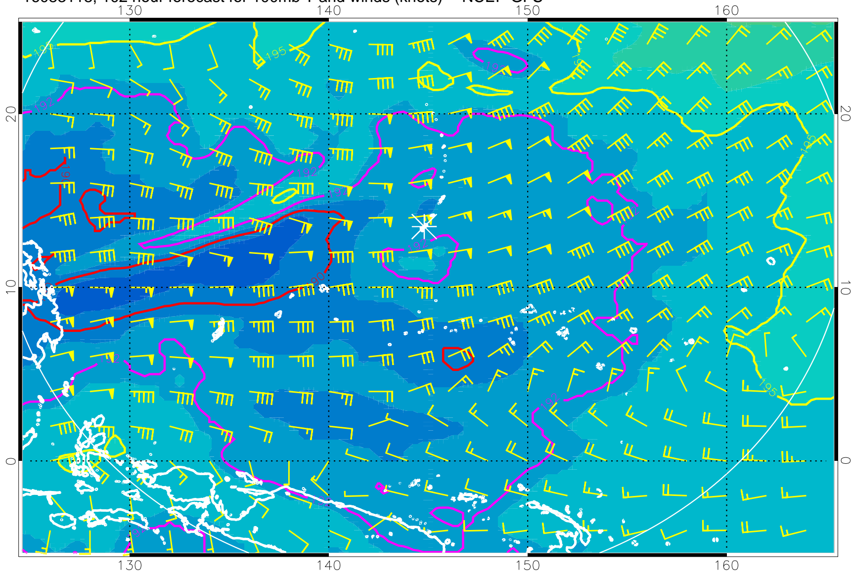
16083118, 102 hour forecast for 100mb T and winds (knots) -- NCEP GFS
