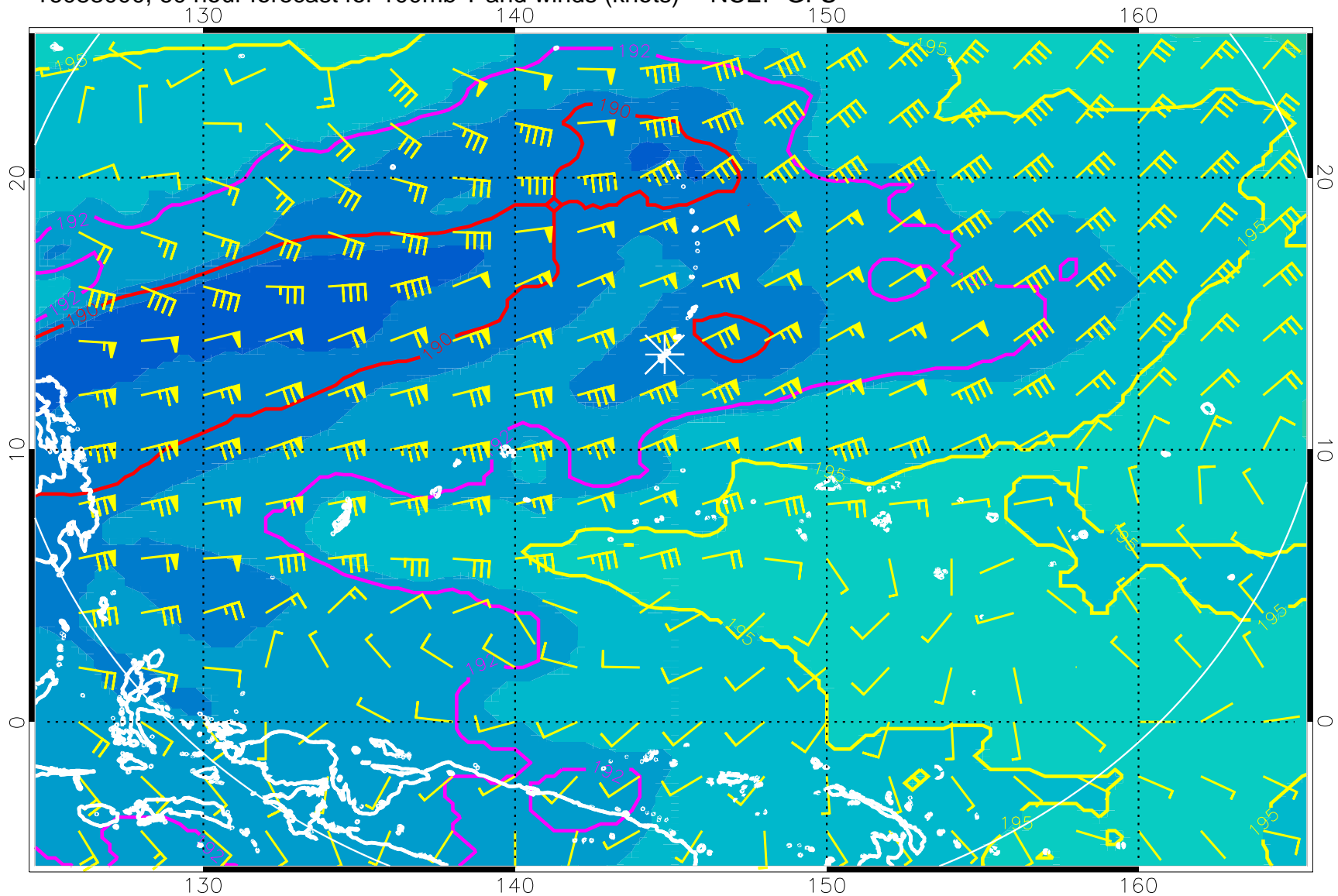
16083000, 60 hour forecast for 100mb T and winds (knots) -- NCEP GFS
