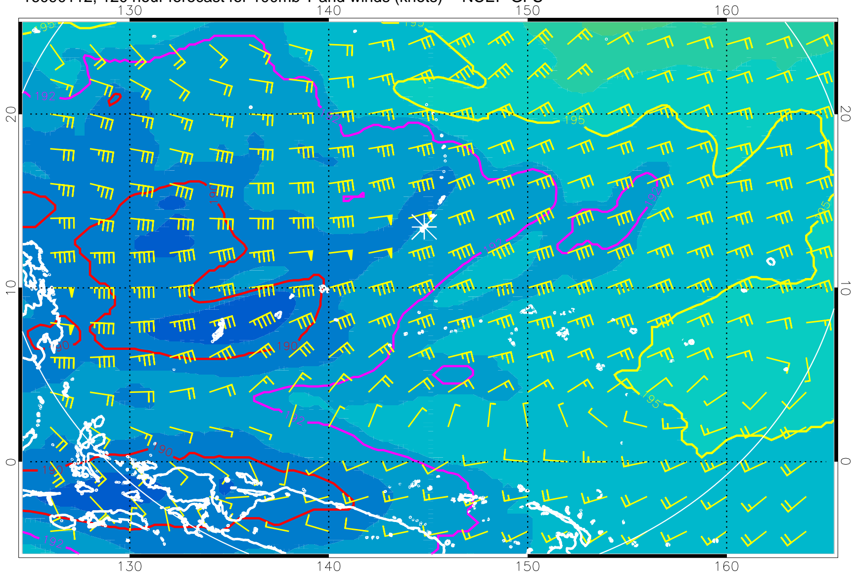
16090112, 120 hour forecast for 100mb T and winds (knots) -- NCEP GFS
