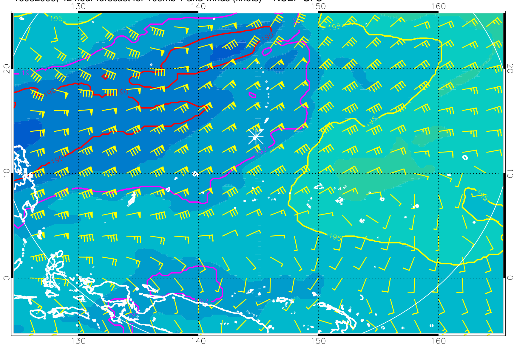
16082906, 42 hour forecast for 100mb T and winds (knots) -- NCEP GFS
