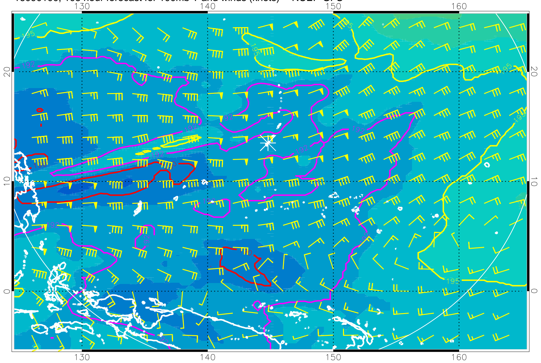
16090100, 108 hour forecast for 100mb T and winds (knots) -- NCEP GFS
