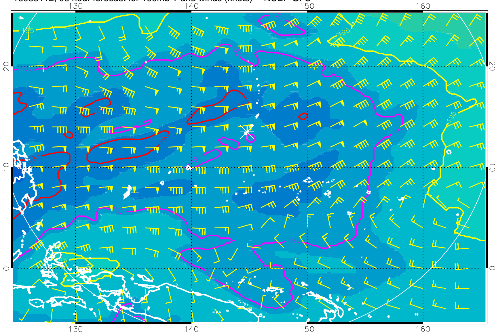
16083112, 96 hour forecast for 100mb T and winds (knots) -- NCEP GFS
