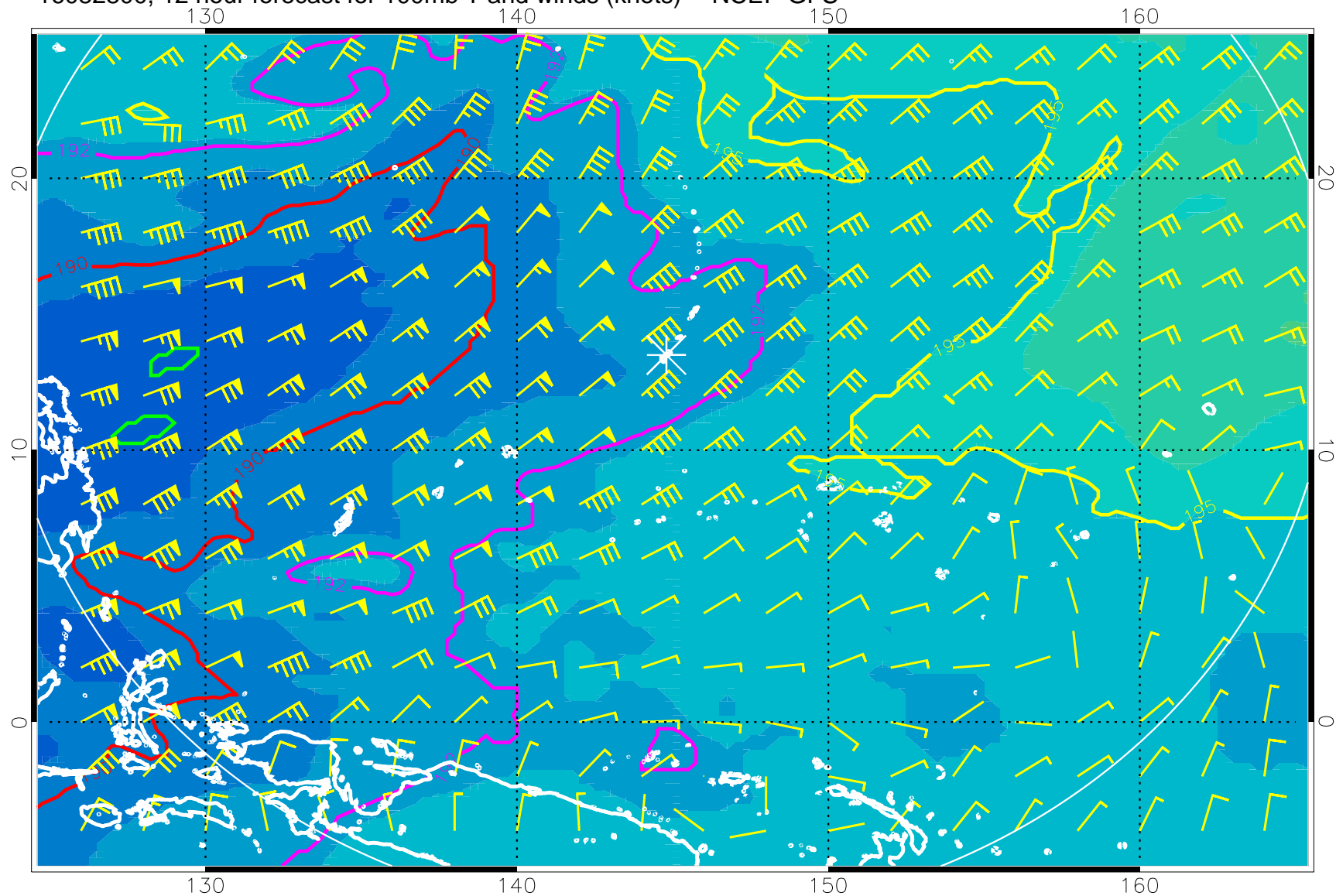
16082800, 12 hour forecast for 100mb T and winds (knots) -- NCEP GFS
