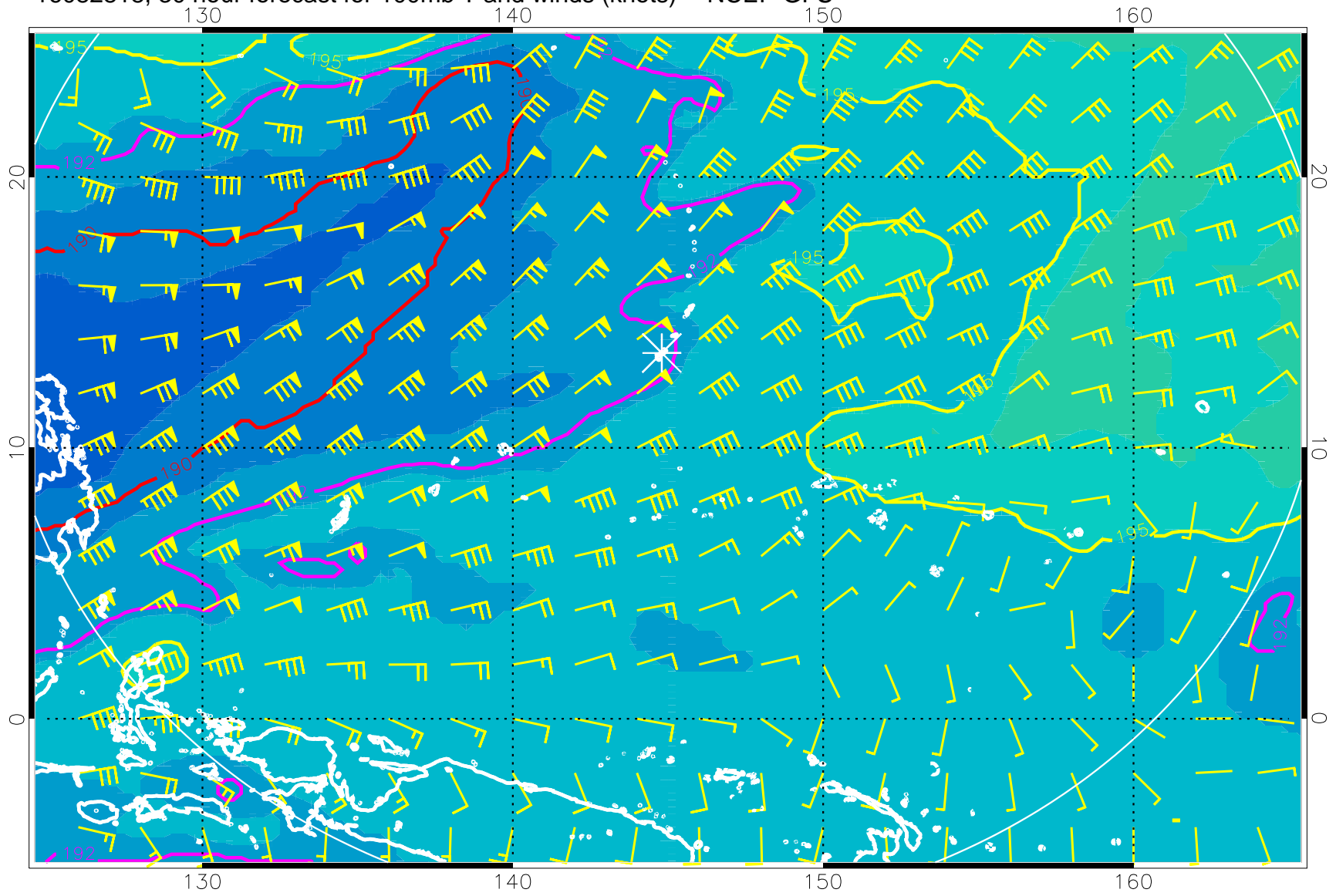
16082818, 30 hour forecast for 100mb T and winds (knots) -- NCEP GFS
