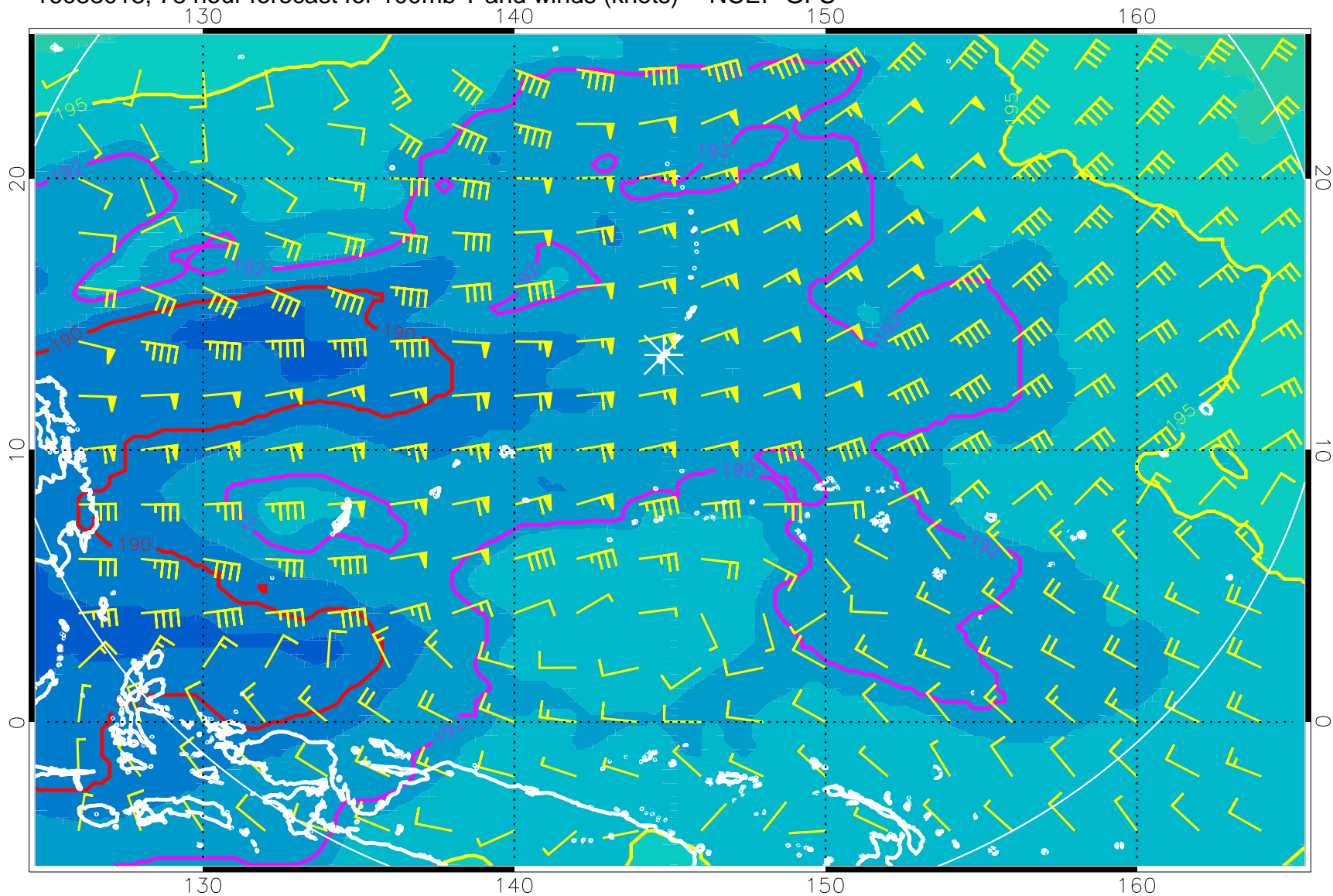
16083018, 78 hour forecast for 100mb T and winds (knots) -- NCEP GFS
