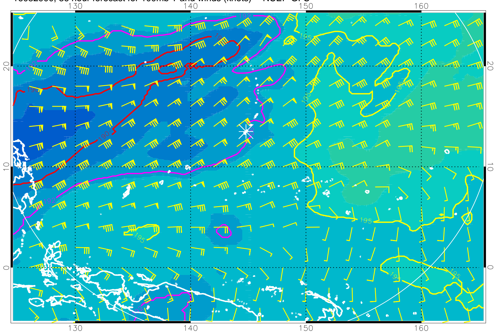
16082900, 36 hour forecast for 100mb T and winds (knots) -- NCEP GFS
