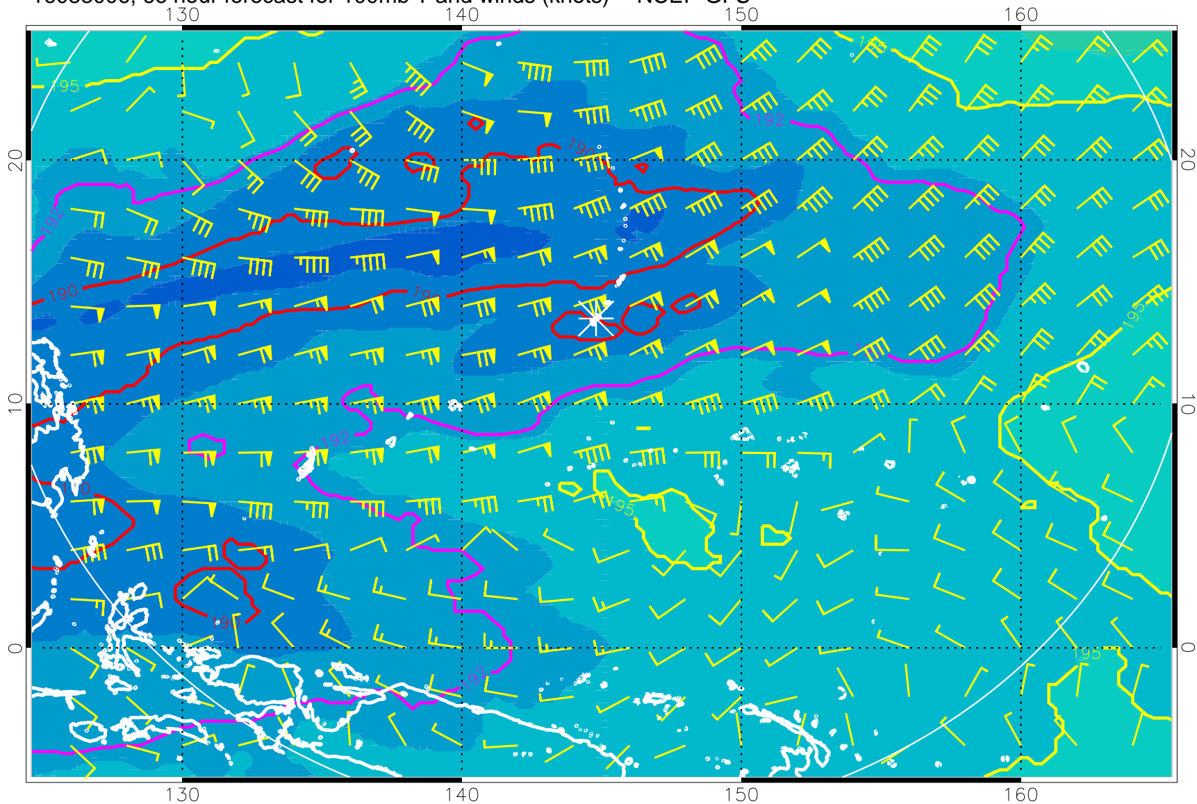
16083006, 66 hour forecast for 100mb T and winds (knots) -- NCEP GFS
