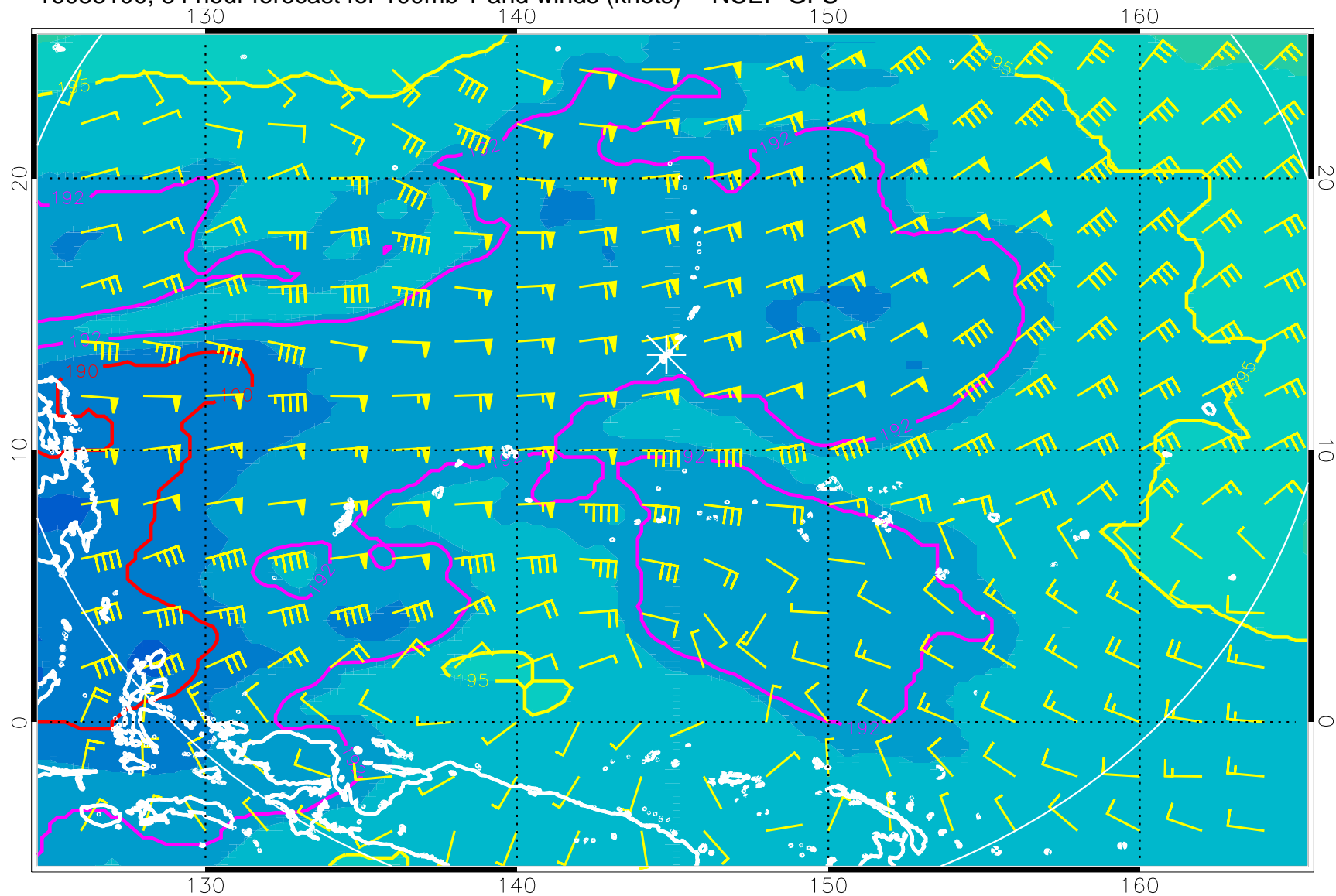
16083100, 84 hour forecast for 100mb T and winds (knots) -- NCEP GFS
