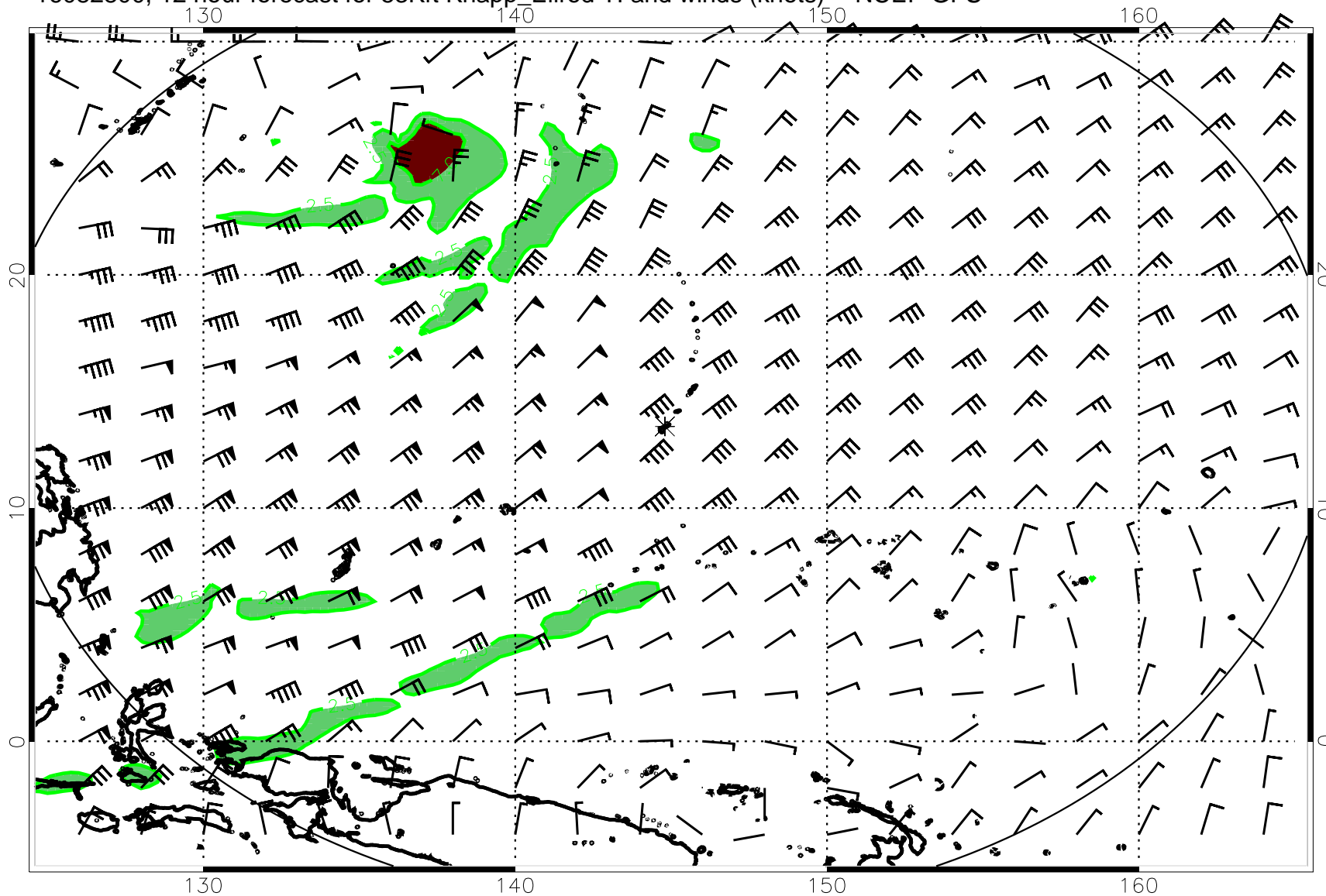
16082800, 12 hour forecast for 53Kft Knapp_Ellrod TI and winds (knots) -- NCEP GFS
