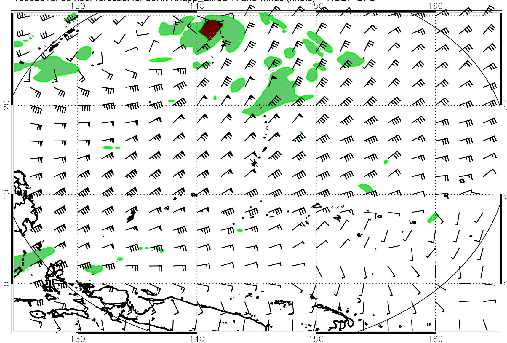
16082818, 30 hour forecast for 53Kft Knapp_Ellrod TI and winds (knots) -- NCEP GFS
