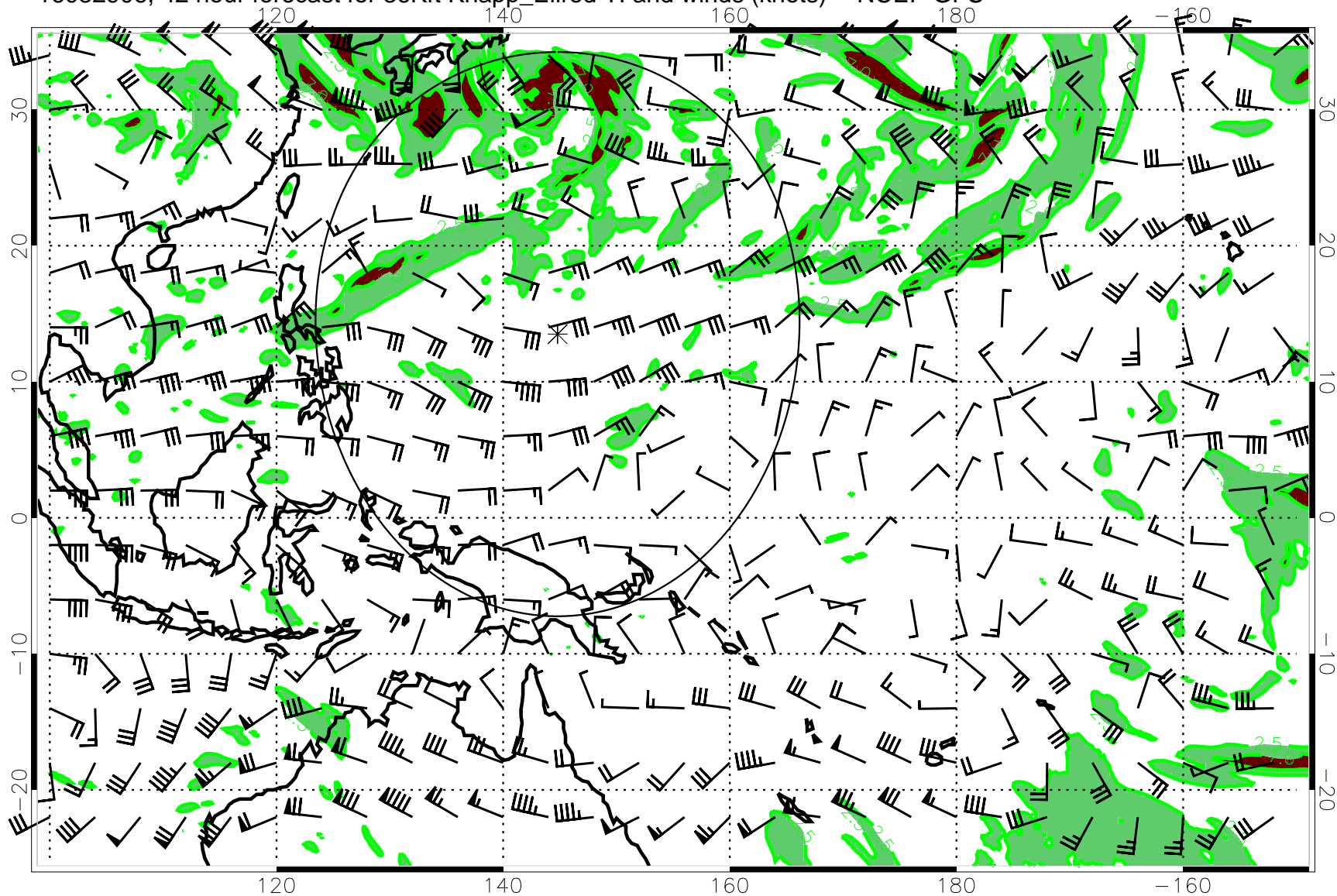
16082906, 42 hour forecast for 36Kft Knapp_Ellrod TI and winds (knots) -- NCEP GFS
