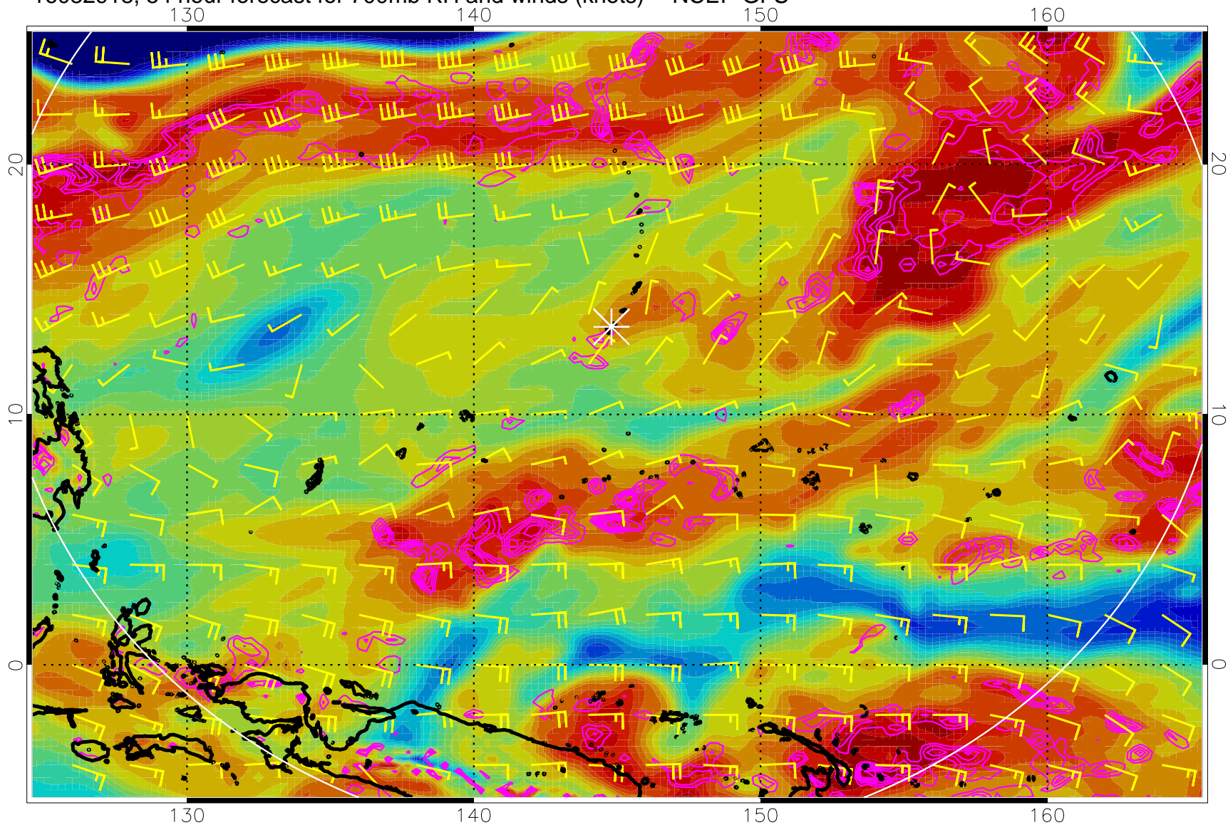
16082918, 54 hour forecast for 700mb RH and winds (knots) -- NCEP GFS
