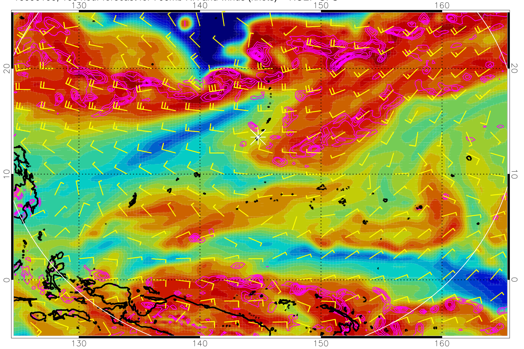
16090100, 108 hour forecast for 700mb RH and winds (knots) -- NCEP GFS
