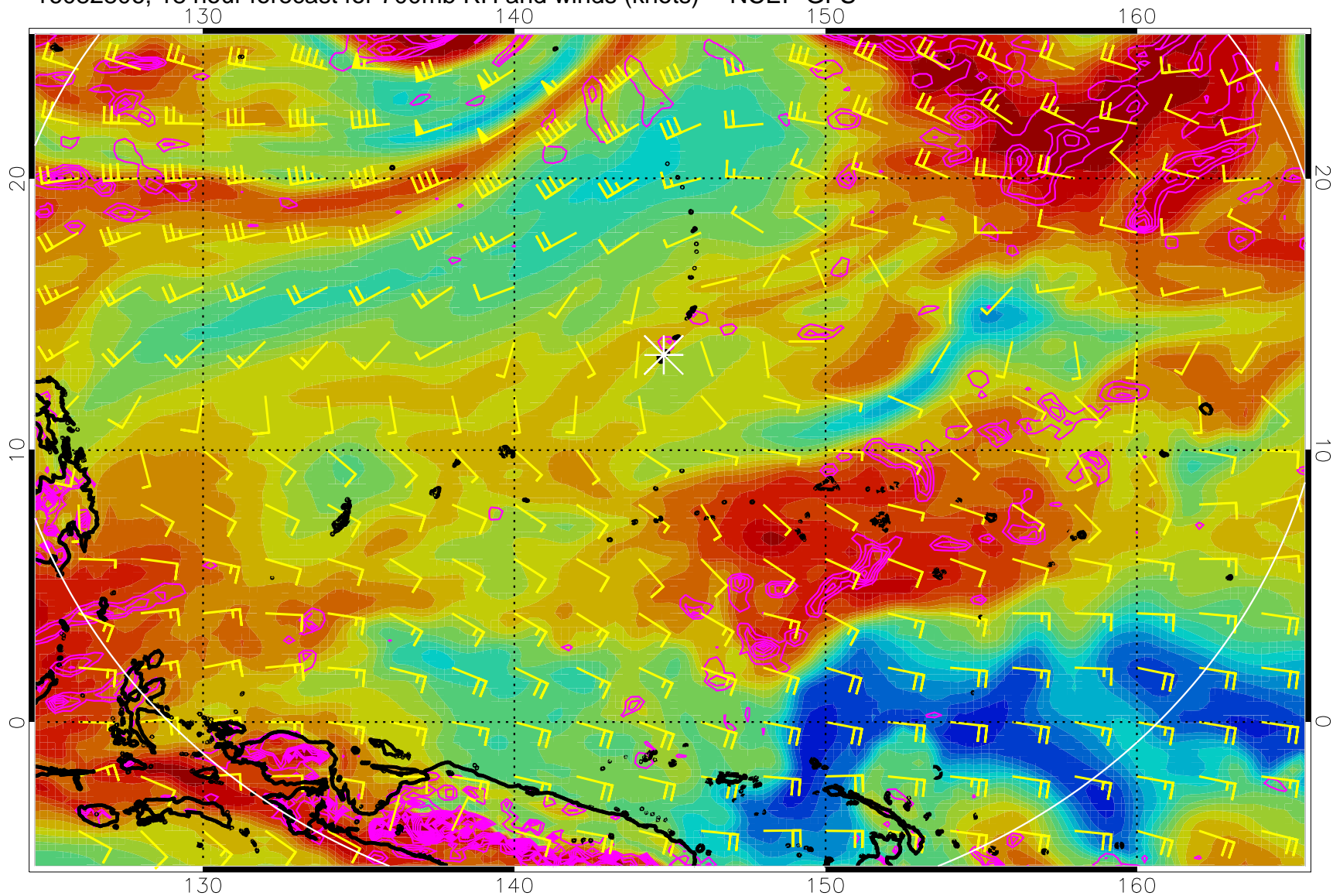
16082806, 18 hour forecast for 700mb RH and winds (knots) -- NCEP GFS
