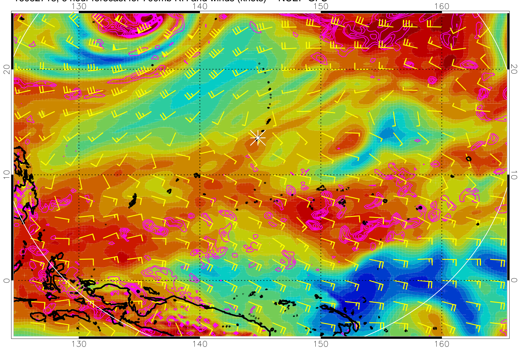
16082718, 6 hour forecast for 700mb RH and winds (knots) -- NCEP GFS
