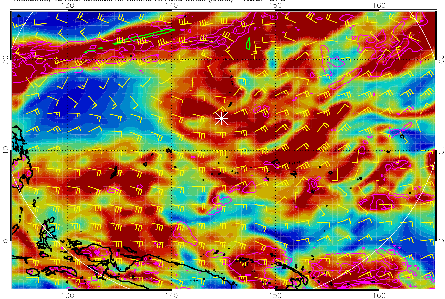
16082906, 42 hour forecast for 300mb RH and winds (knots) -- NCEP GFS
