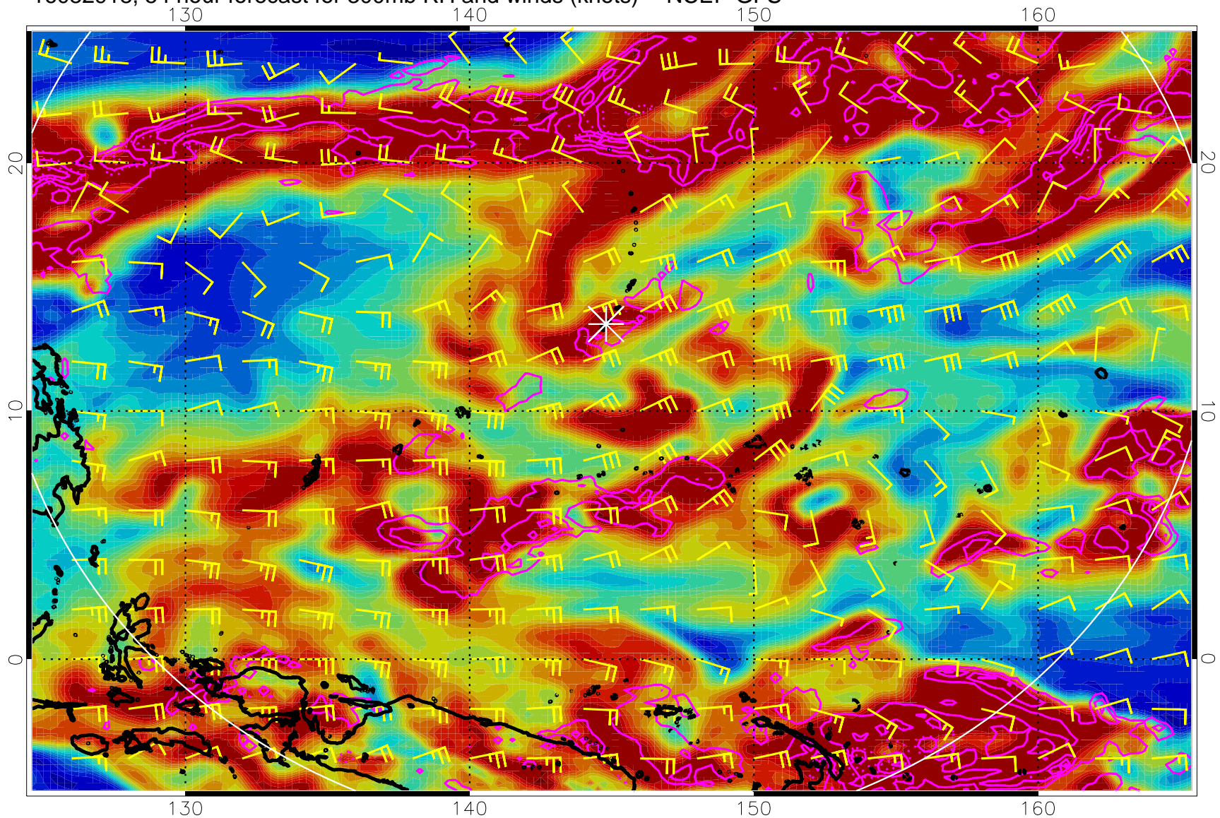
16082918, 54 hour forecast for 300mb RH and winds (knots) -- NCEP GFS
