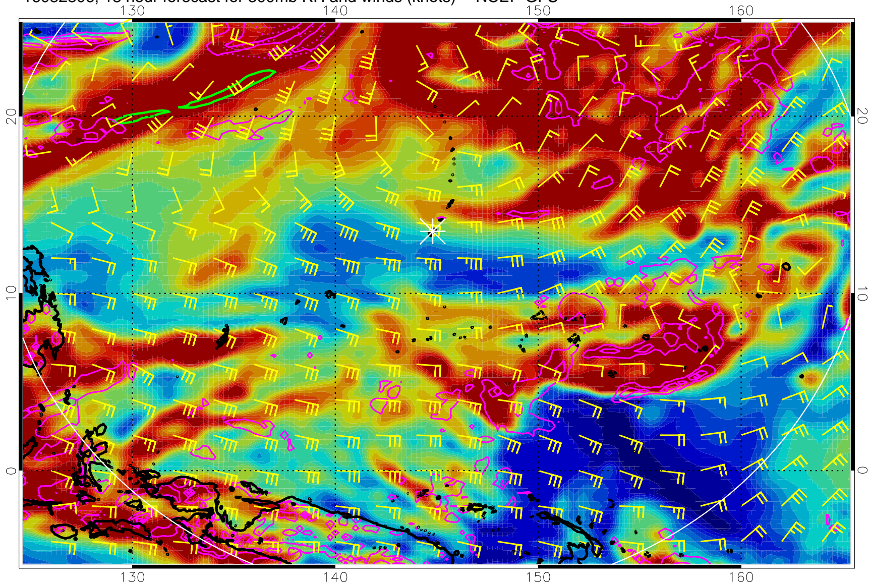
16082806, 18 hour forecast for 300mb RH and winds (knots) -- NCEP GFS
