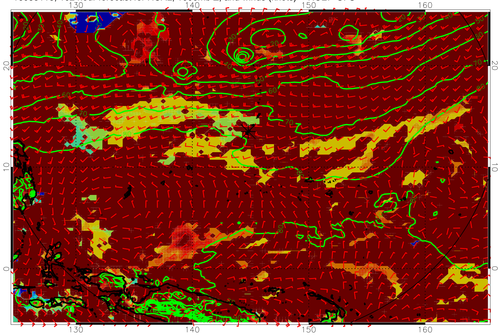
16083118, 102 hour forecast for HCAL, 1000mb Z, and winds (knots) -- NCEP GFS
