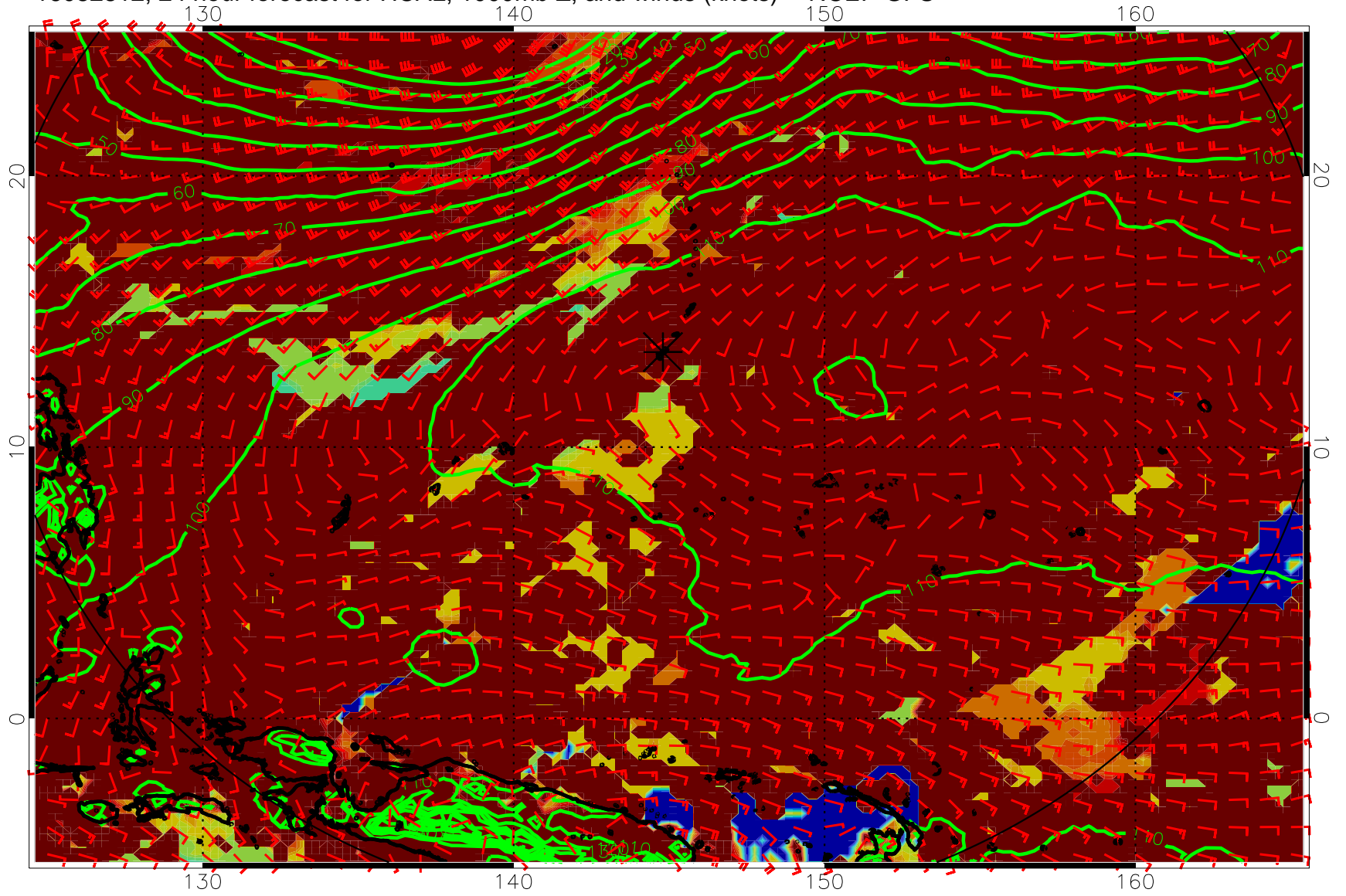
16082812, 24 hour forecast for HCAL, 1000mb Z, and winds (knots) -- NCEP GFS
