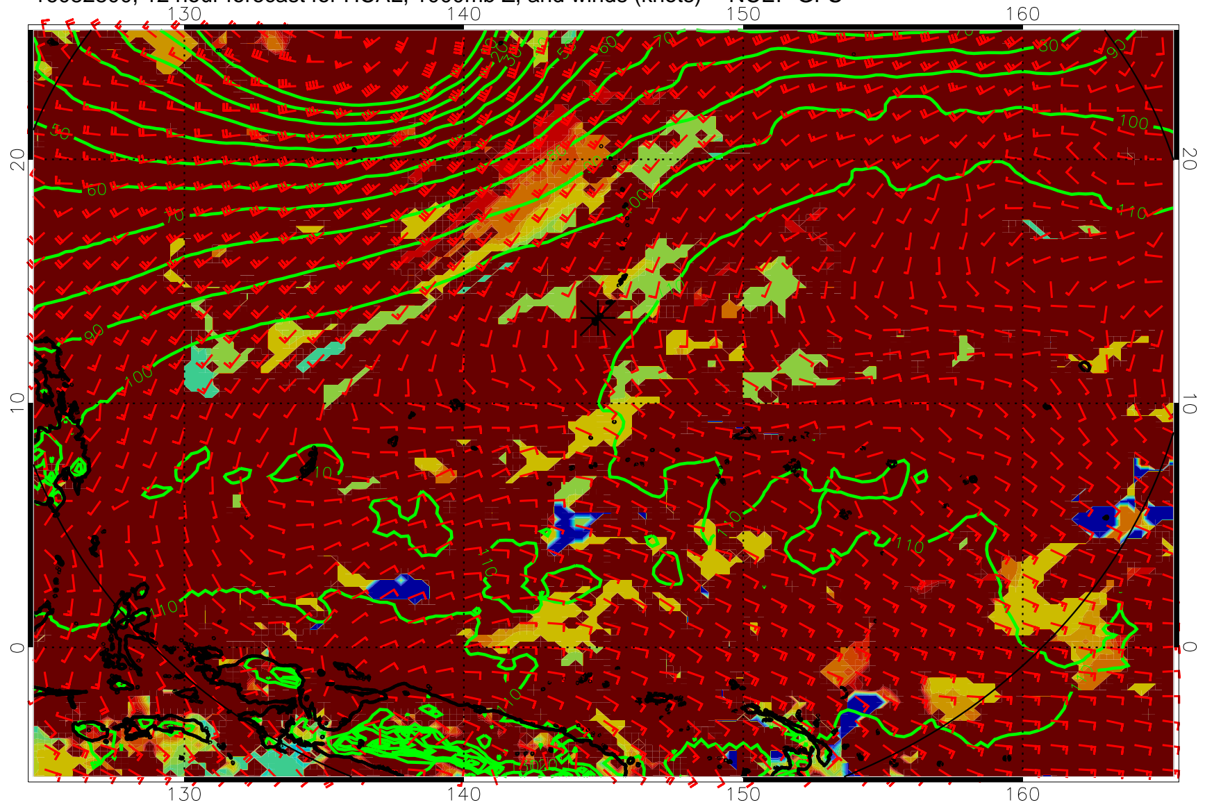
16082800, 12 hour forecast for HCAL, 1000mb Z, and winds (knots) -- NCEP GFS
