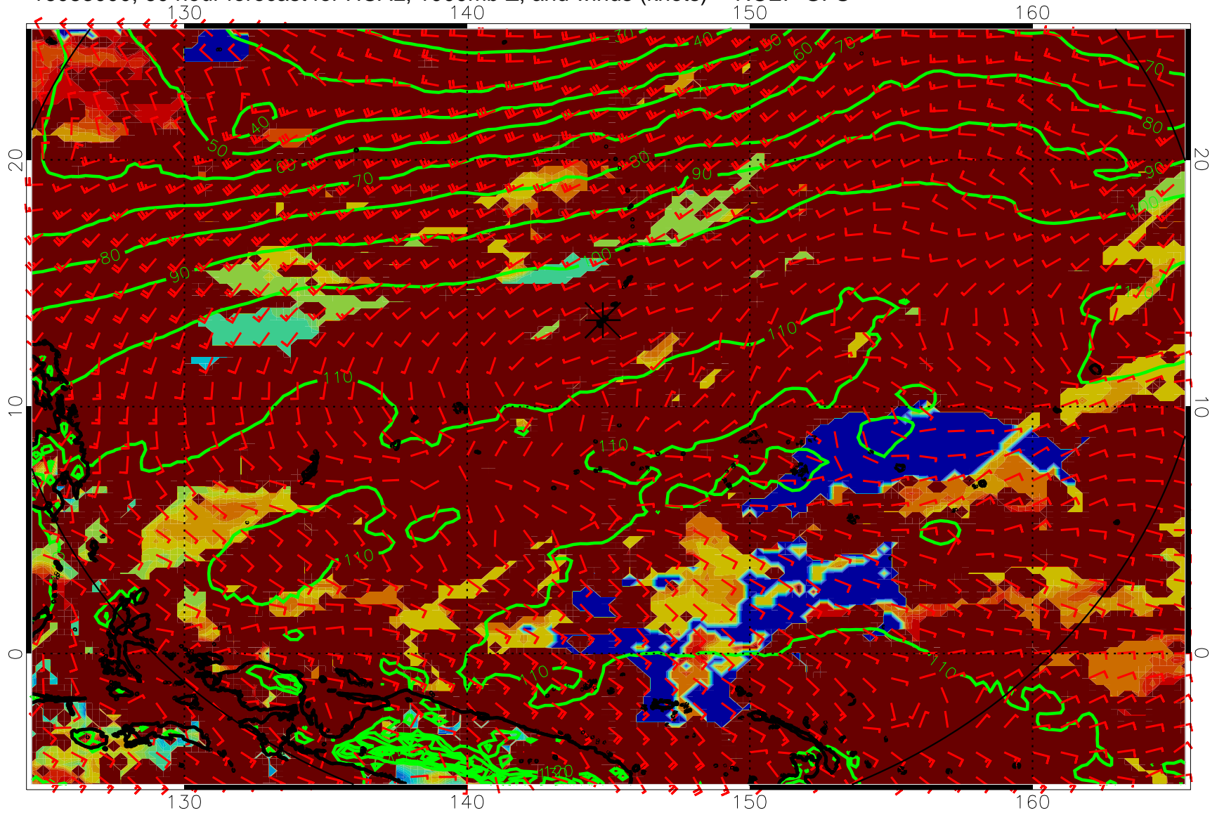
16083000, 60 hour forecast for HCAL, 1000mb Z, and winds (knots) -- NCEP GFS
