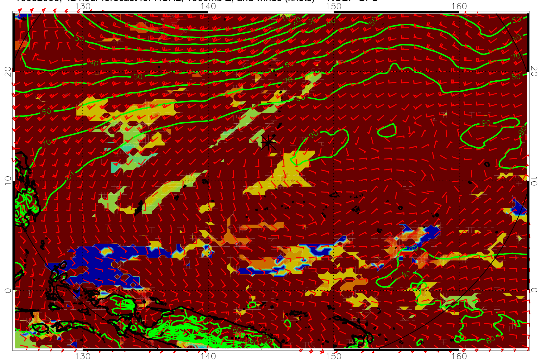
16082906, 42 hour forecast for HCAL, 1000mb Z, and winds (knots) -- NCEP GFS
