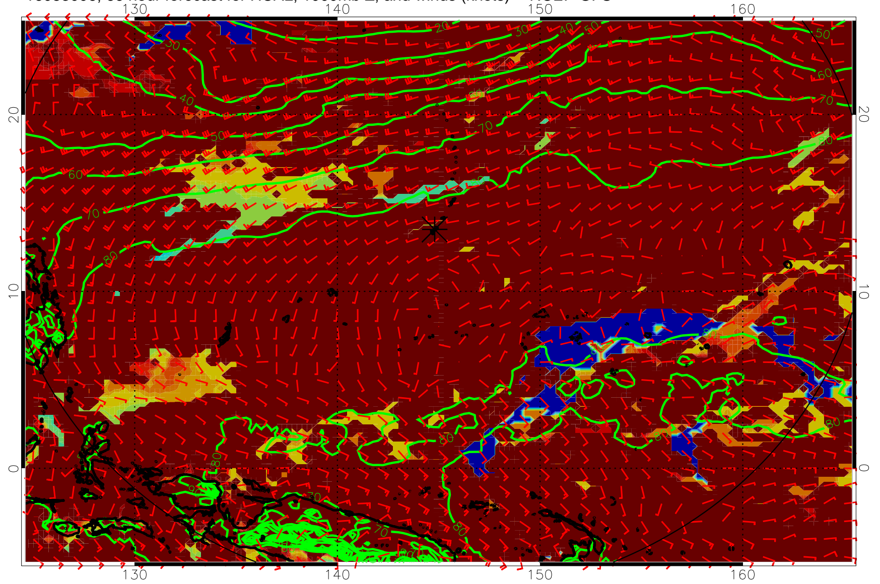
16083006, 66 hour forecast for HCAL, 1000mb Z, and winds (knots) -- NCEP GFS
