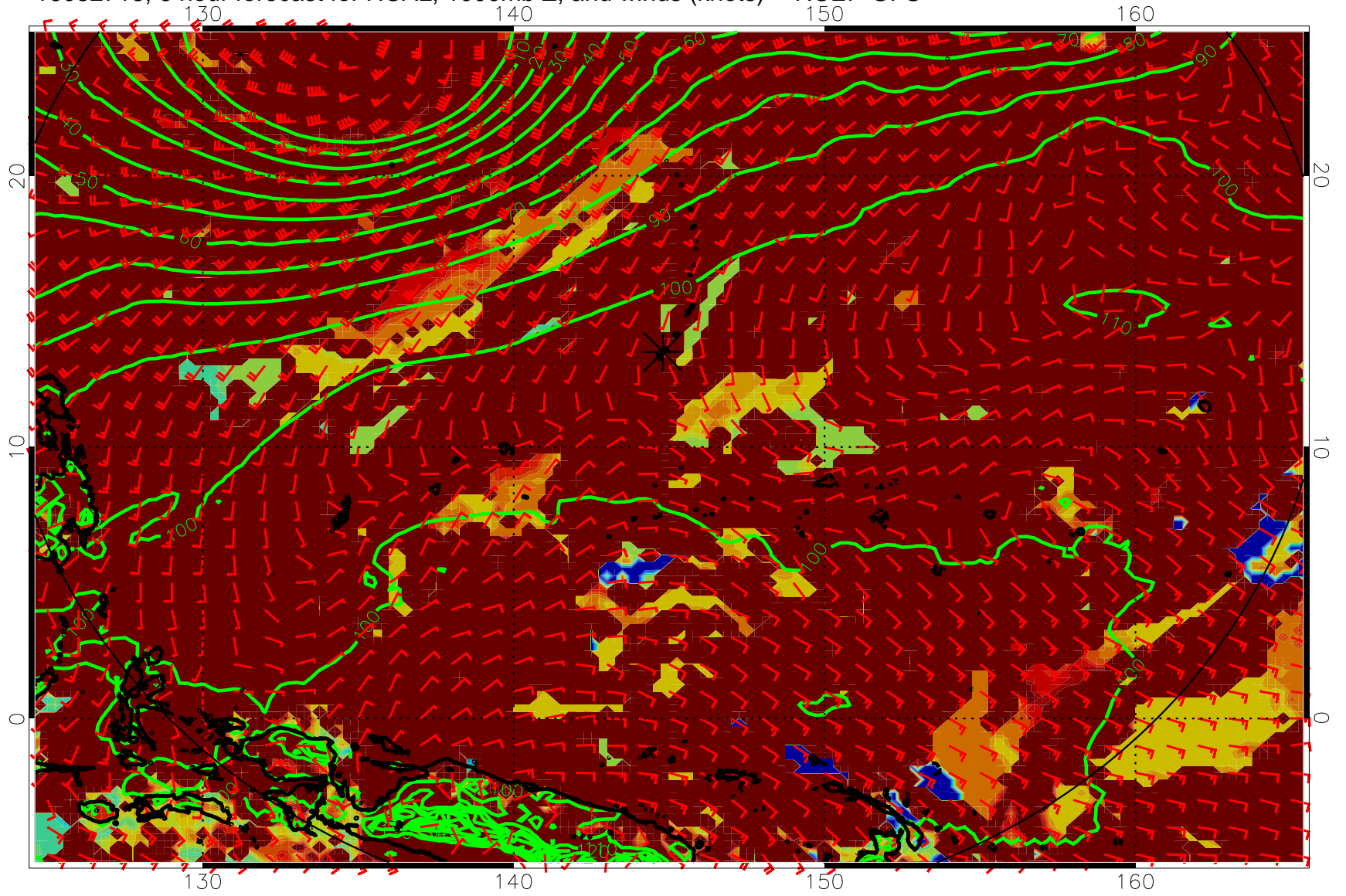
16082718, 6 hour forecast for HCAL, 1000mb Z, and winds (knots) -- NCEP GFS
