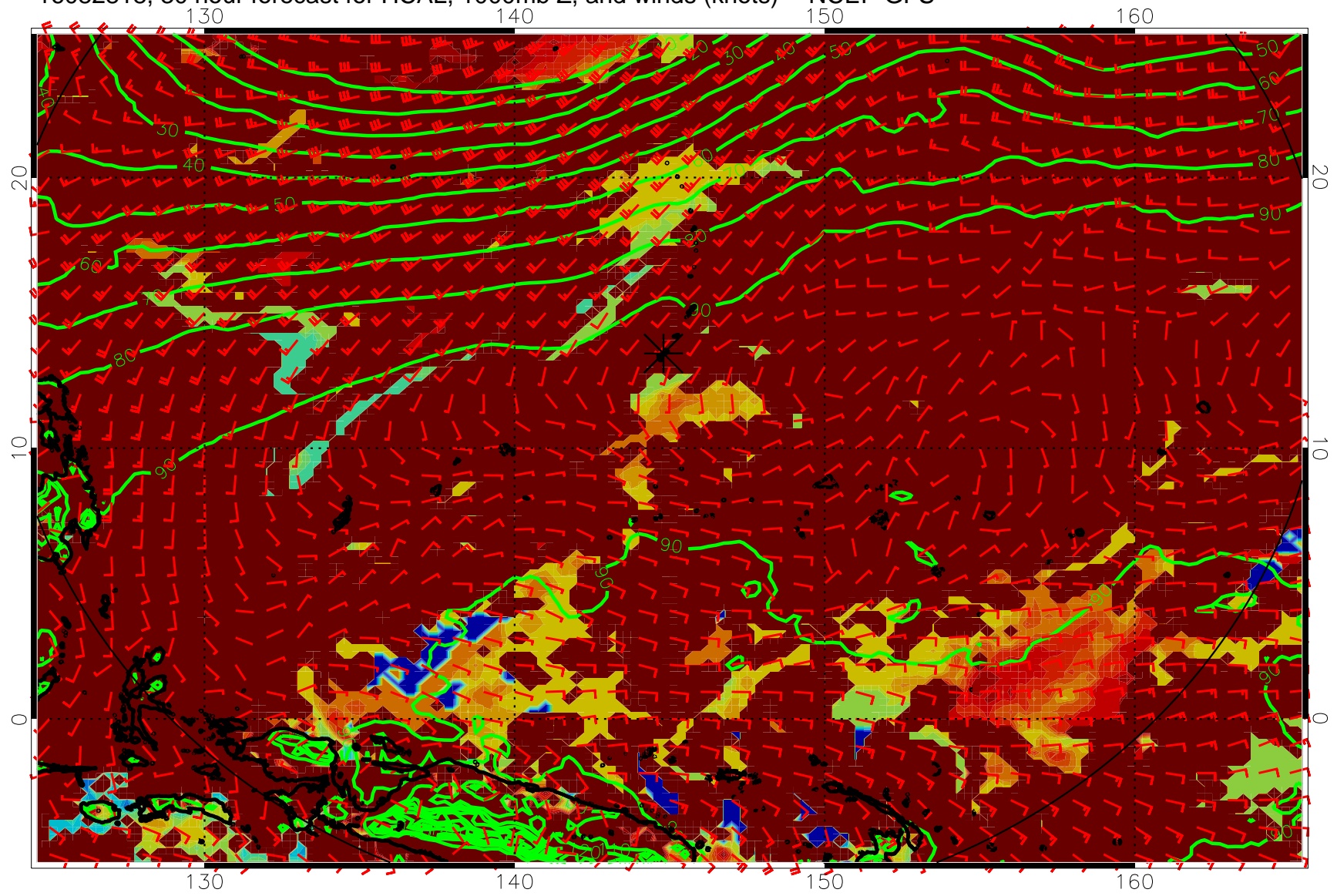
16082818, 30 hour forecast for HCAL, 1000mb Z, and winds (knots) -- NCEP GFS
