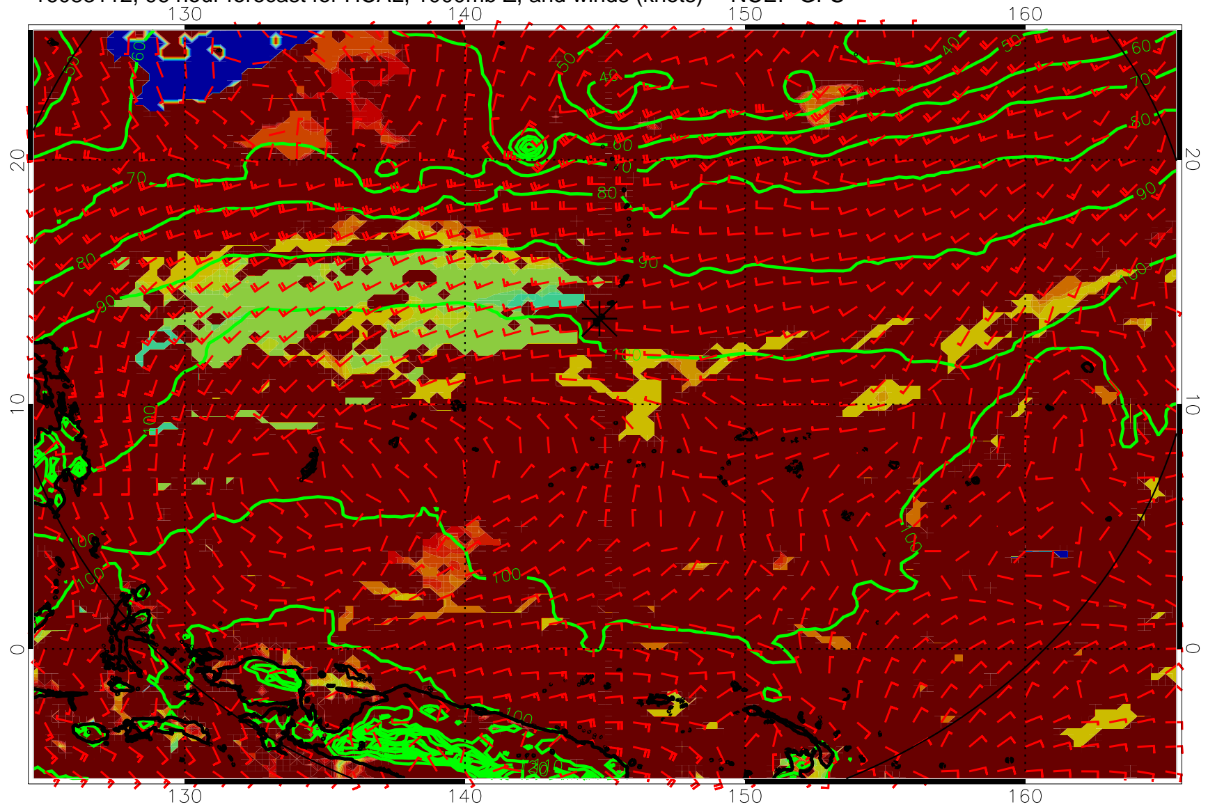
16083112, 96 hour forecast for HCAL, 1000mb Z, and winds (knots) -- NCEP GFS
