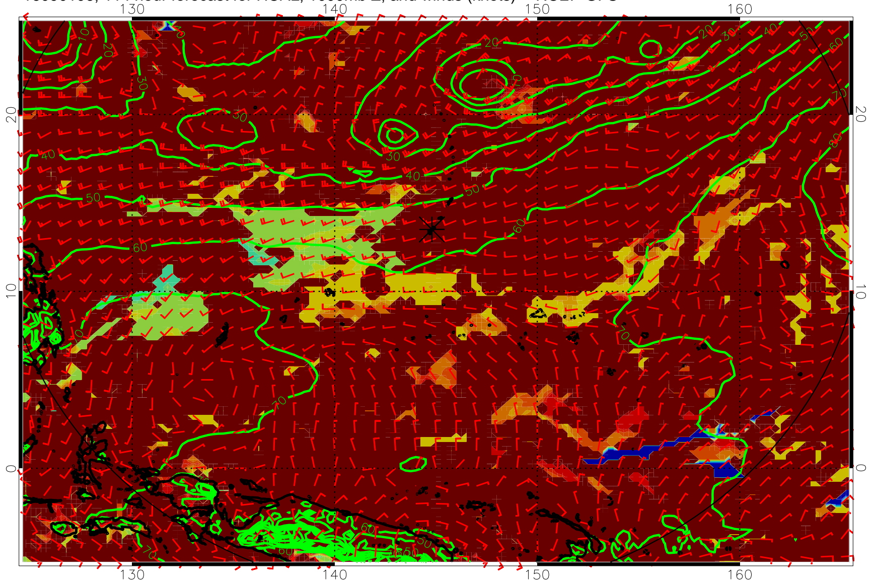
16090106, 114 hour forecast for HCAL, 1000mb Z, and winds (knots) -- NCEP GFS
