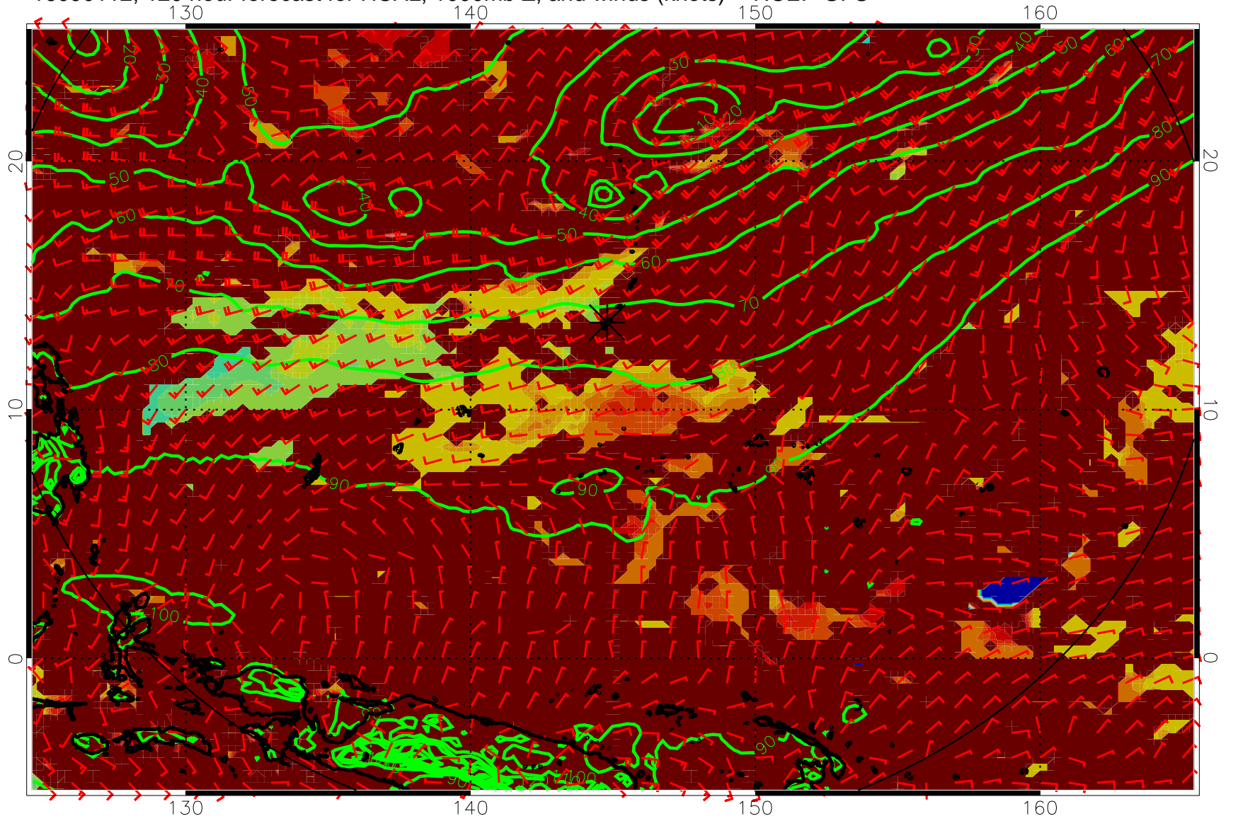
16090112, 120 hour forecast for HCAL, 1000mb Z, and winds (knots) -- NCEP GFS
