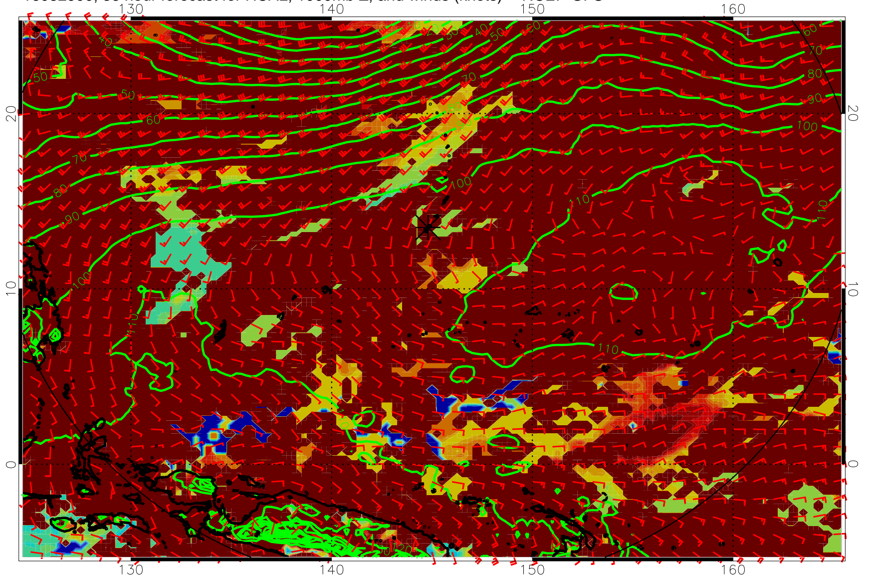
16082900, 36 hour forecast for HCAL, 1000mb Z, and winds (knots) -- NCEP GFS
