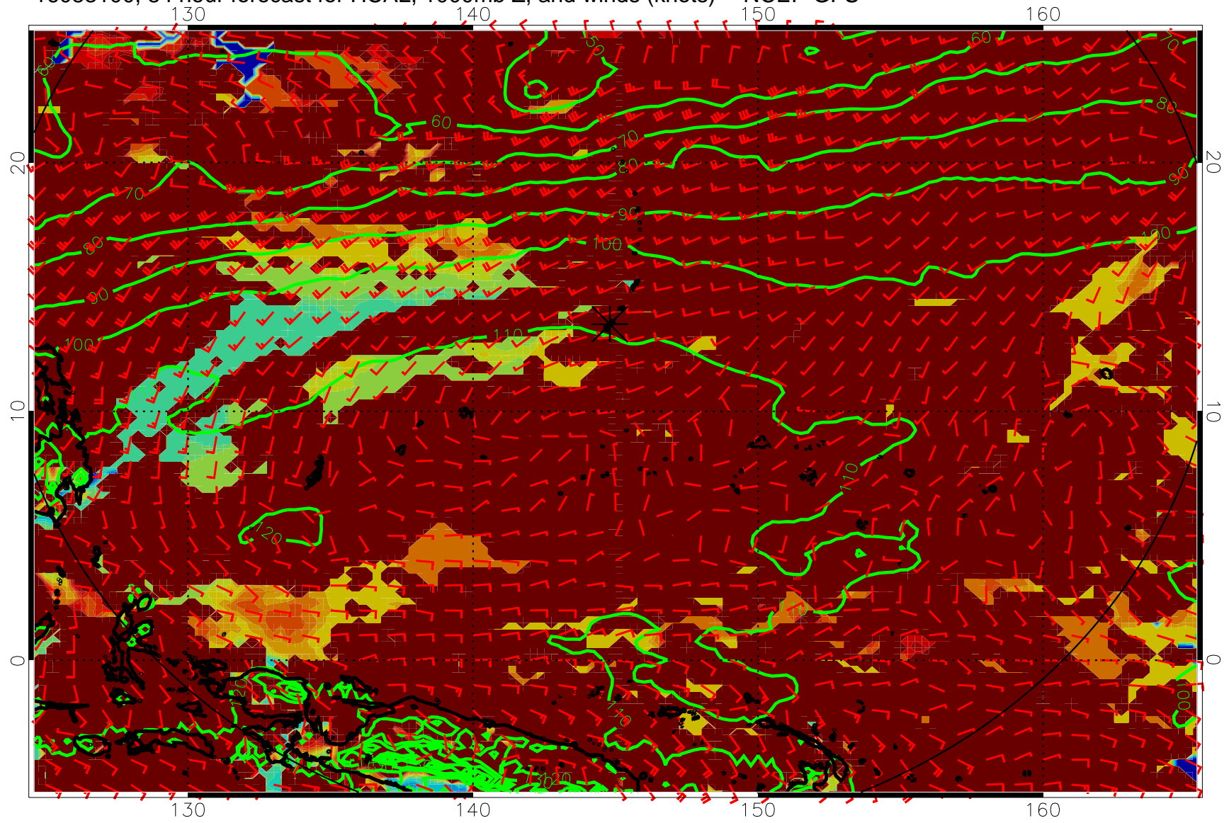
16083100, 84 hour forecast for HCAL, 1000mb Z, and winds (knots) -- NCEP GFS
