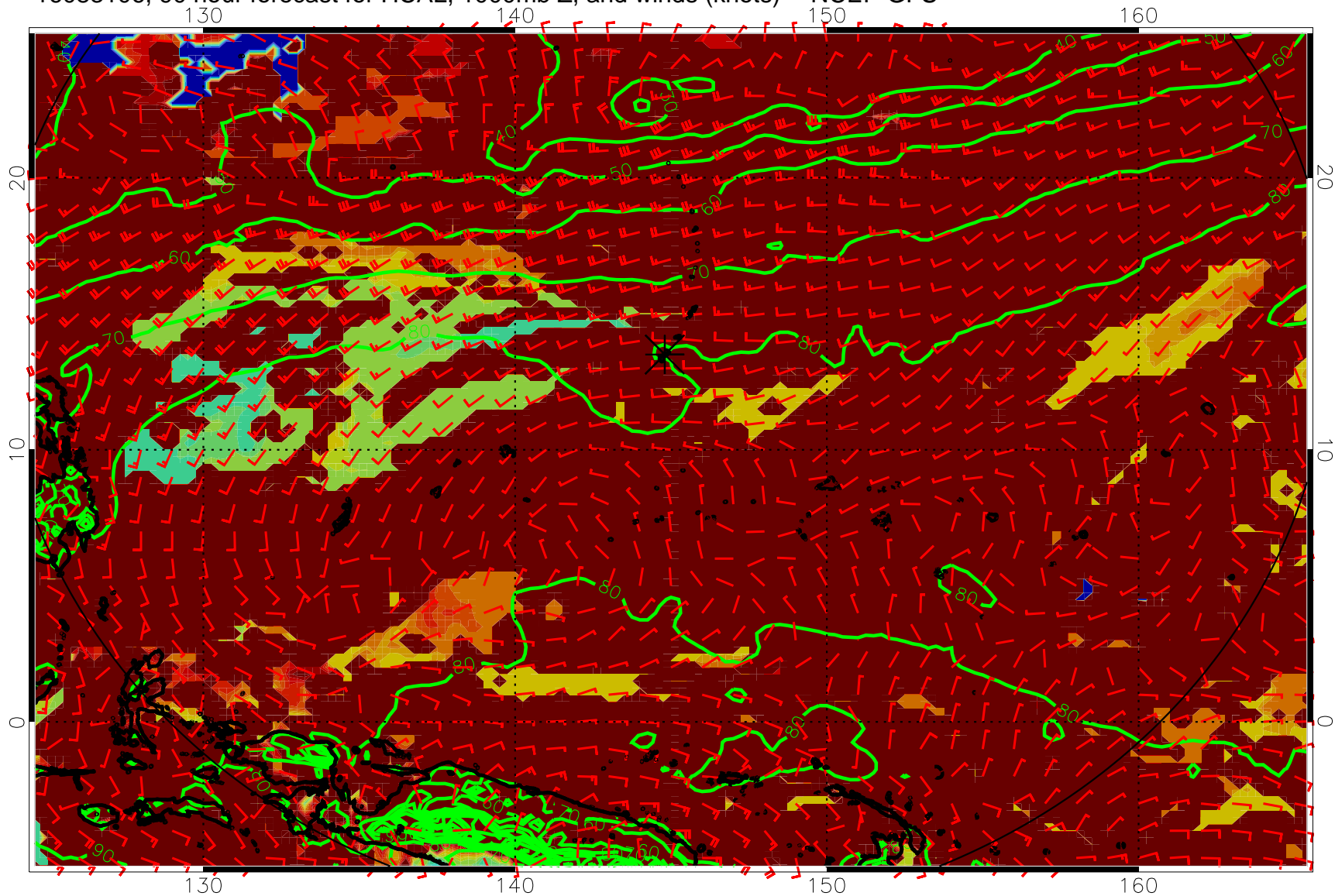
16083106, 90 hour forecast for HCAL, 1000mb Z, and winds (knots) -- NCEP GFS
