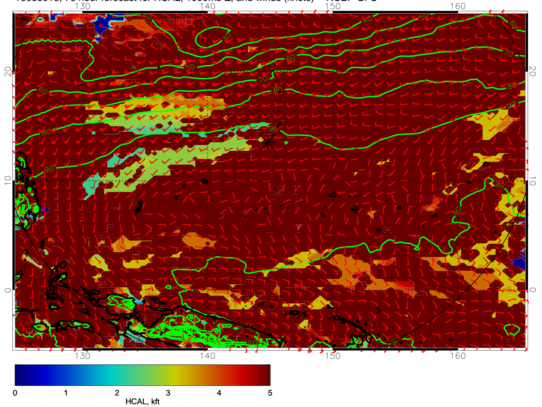
16083018, 78 hour forecast for HCAL, 1000mb Z, and winds (knots) -- NCEP GFS
