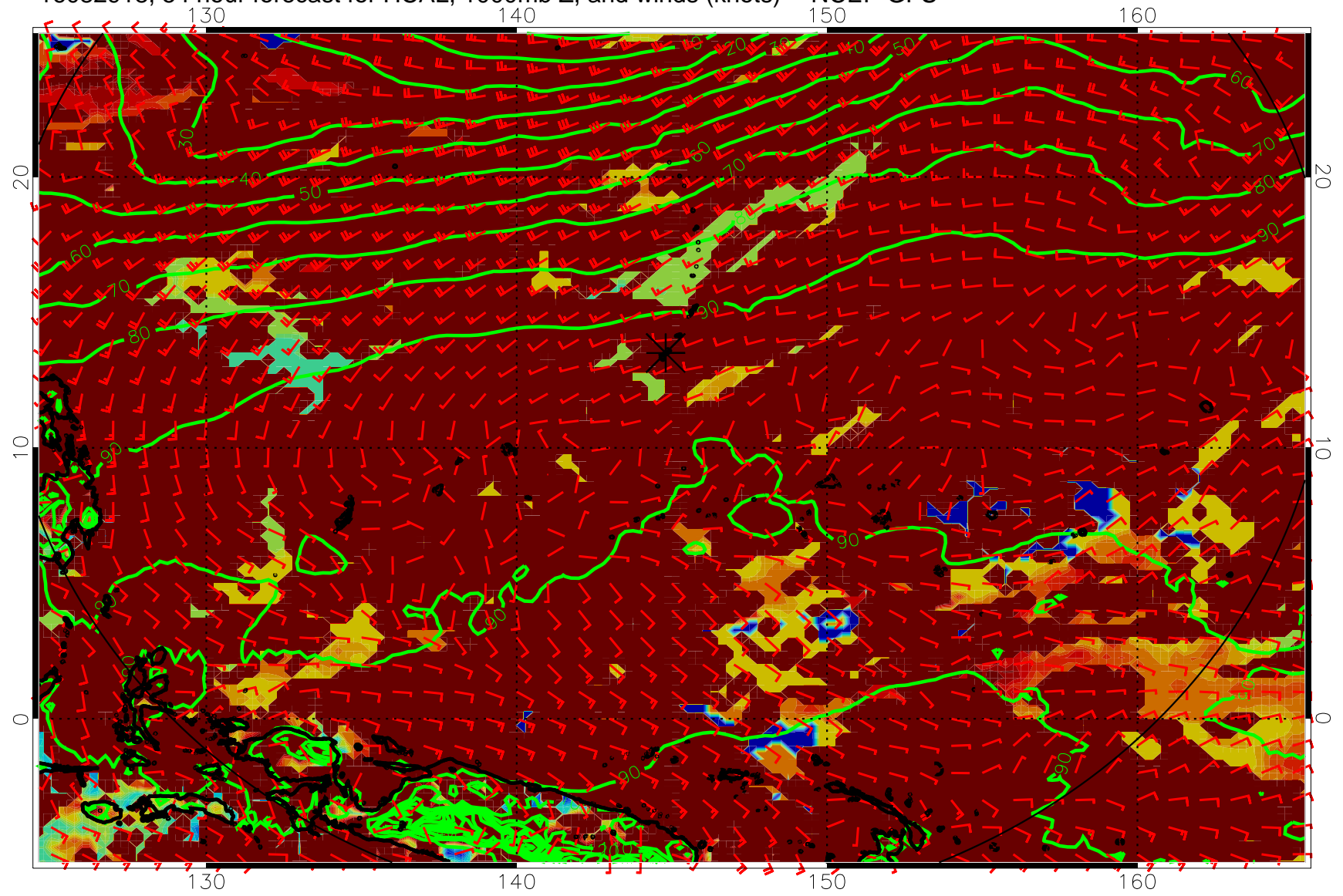
16082918, 54 hour forecast for HCAL, 1000mb Z, and winds (knots) -- NCEP GFS
