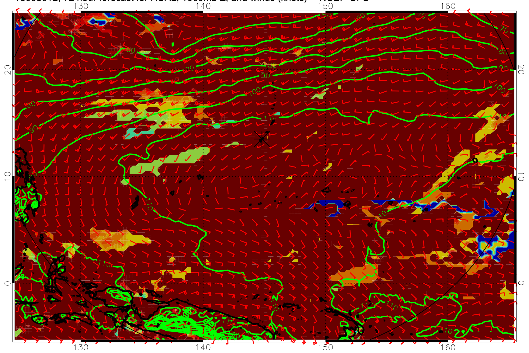
16083012, 72 hour forecast for HCAL, 1000mb Z, and winds (knots) -- NCEP GFS
