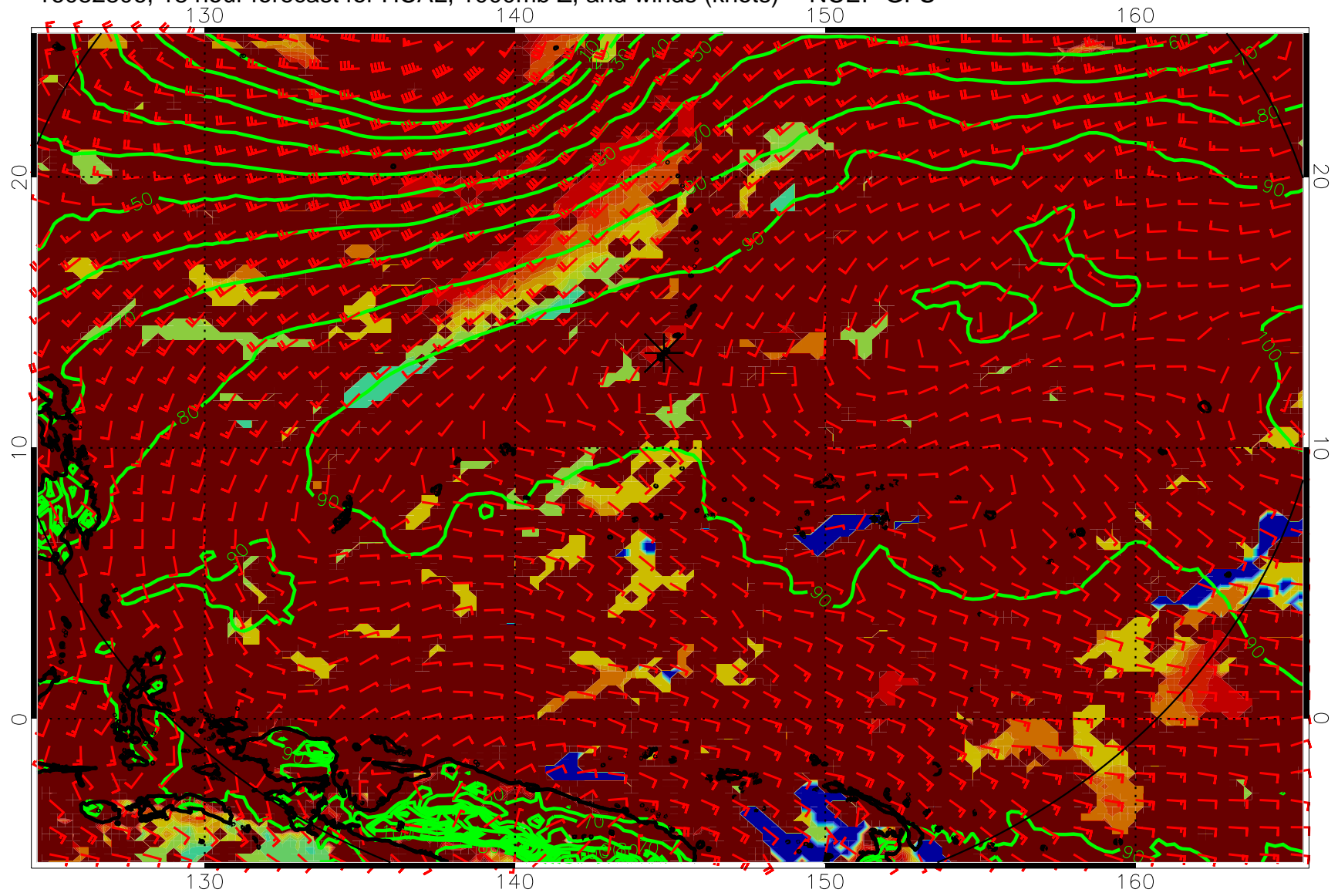
16082806, 18 hour forecast for HCAL, 1000mb Z, and winds (knots) -- NCEP GFS
