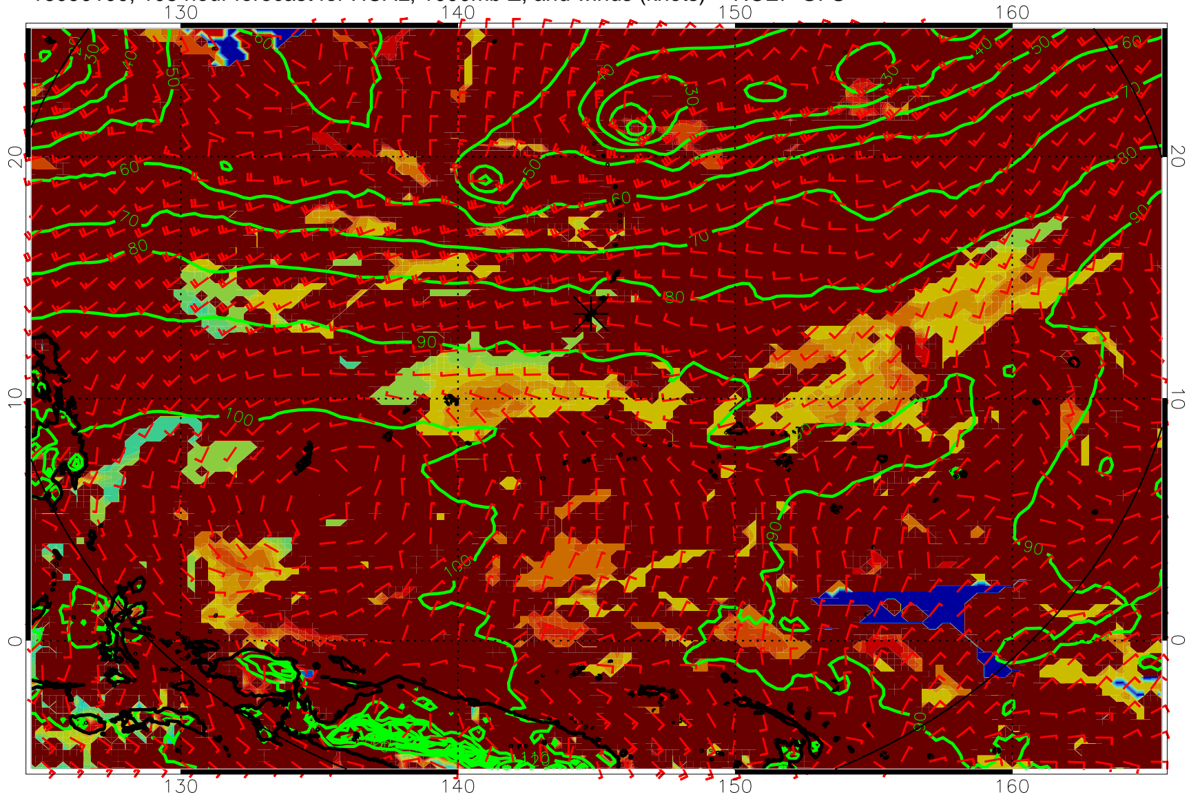
16090100, 108 hour forecast for HCAL, 1000mb Z, and winds (knots) -- NCEP GFS
