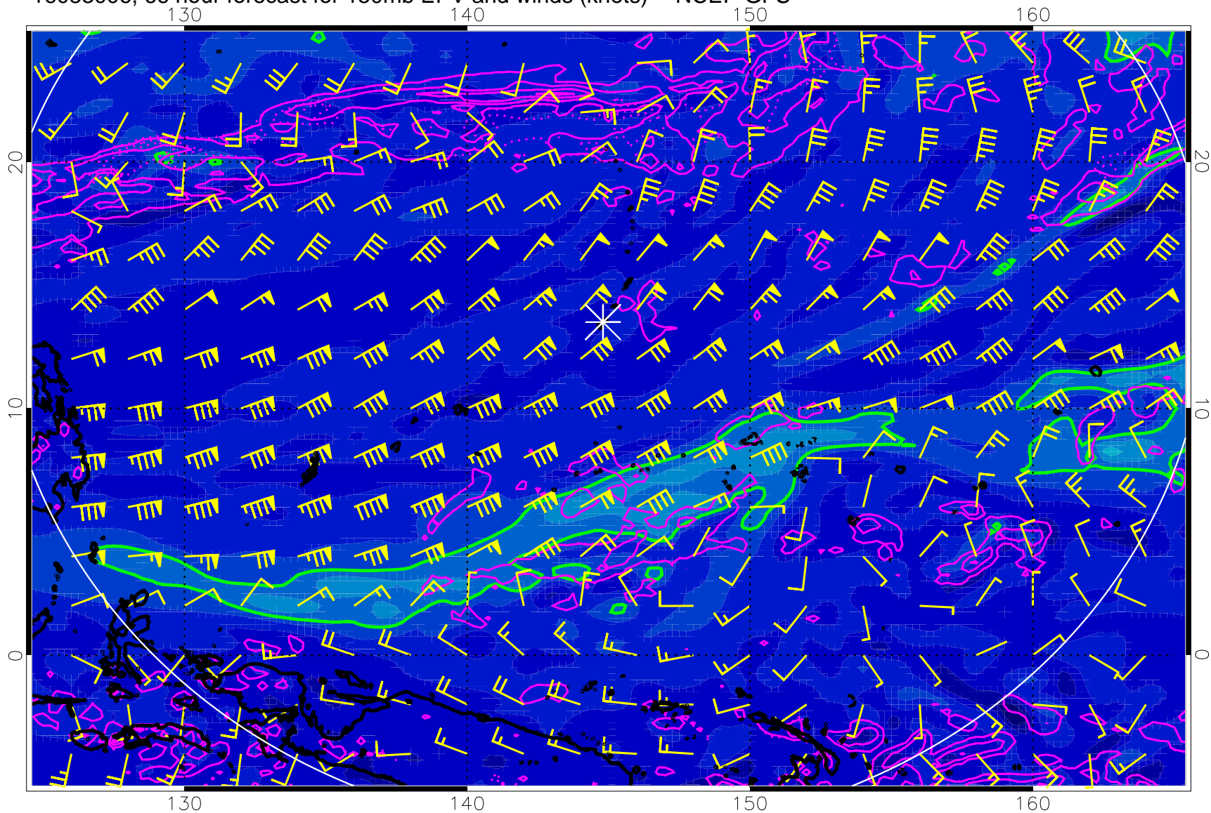
16083006, 66 hour forecast for 150mb EPV and winds (knots) -- NCEP GFS
