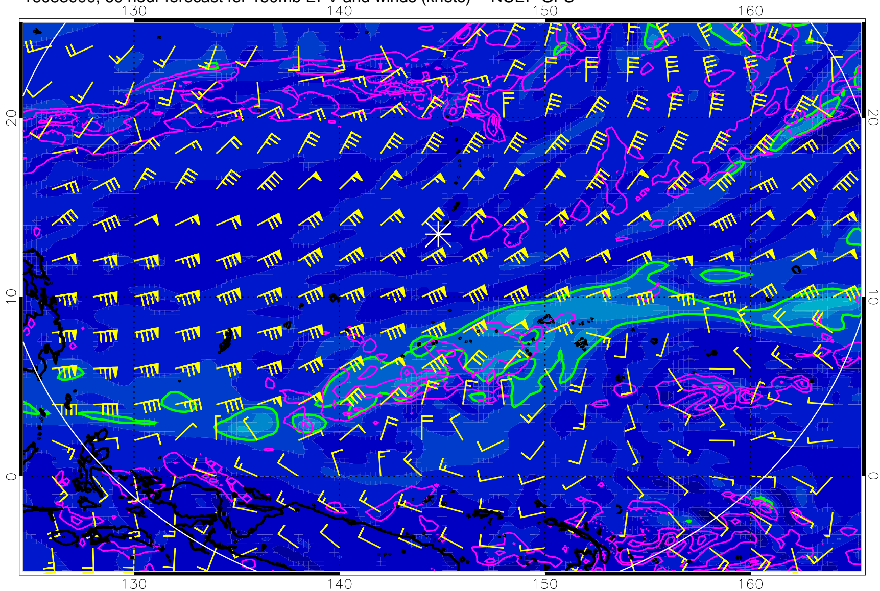
16083000, 60 hour forecast for 150mb EPV and winds (knots) -- NCEP GFS
