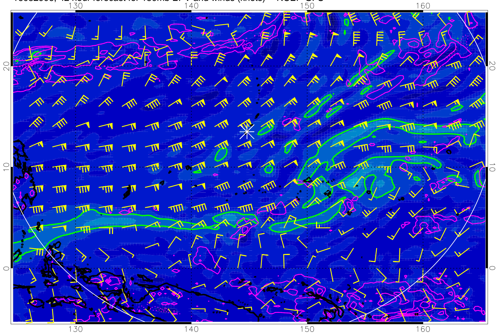
16082906, 42 hour forecast for 150mb EPV and winds (knots) -- NCEP GFS
