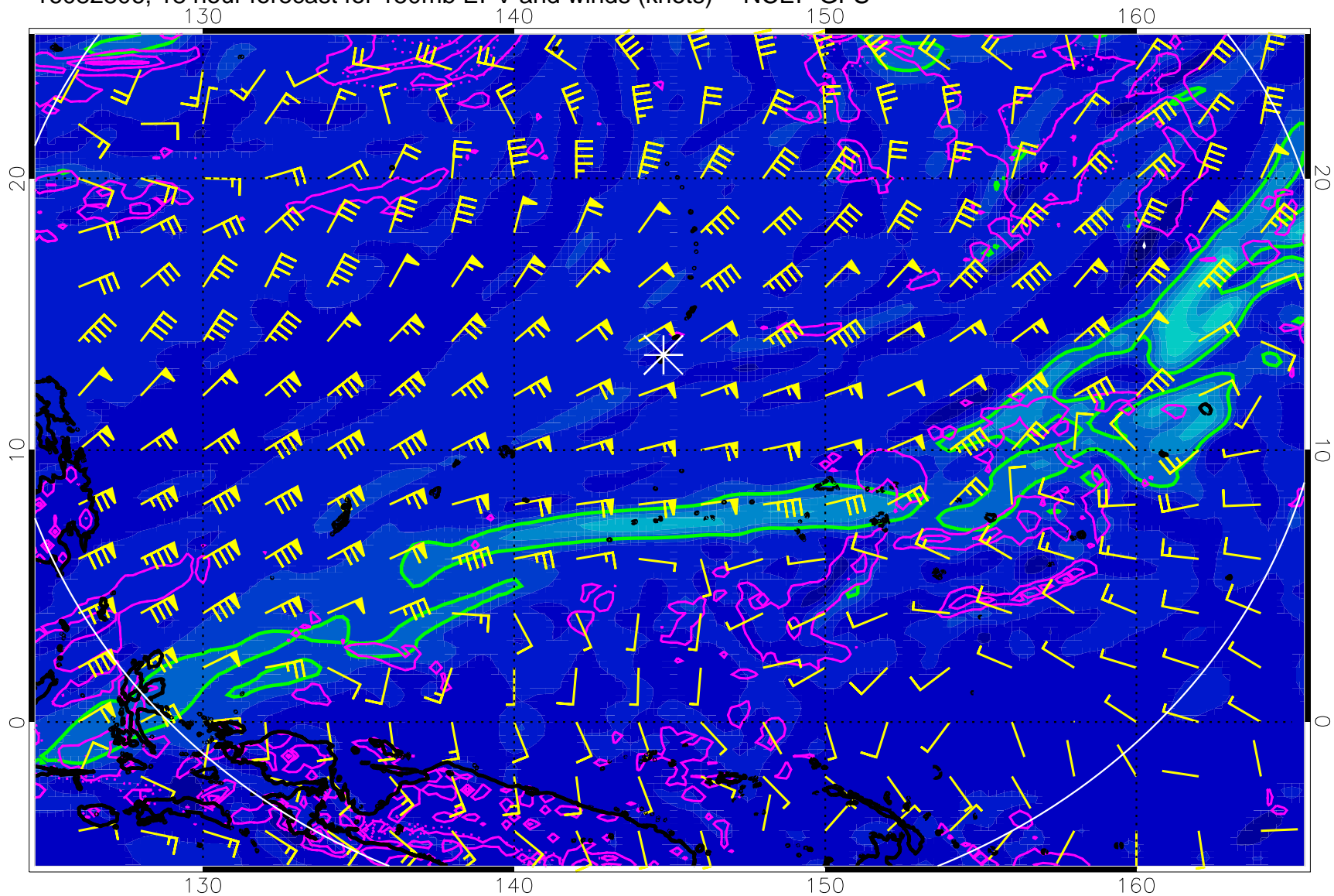
16082806, 18 hour forecast for 150mb EPV and winds (knots) -- NCEP GFS
