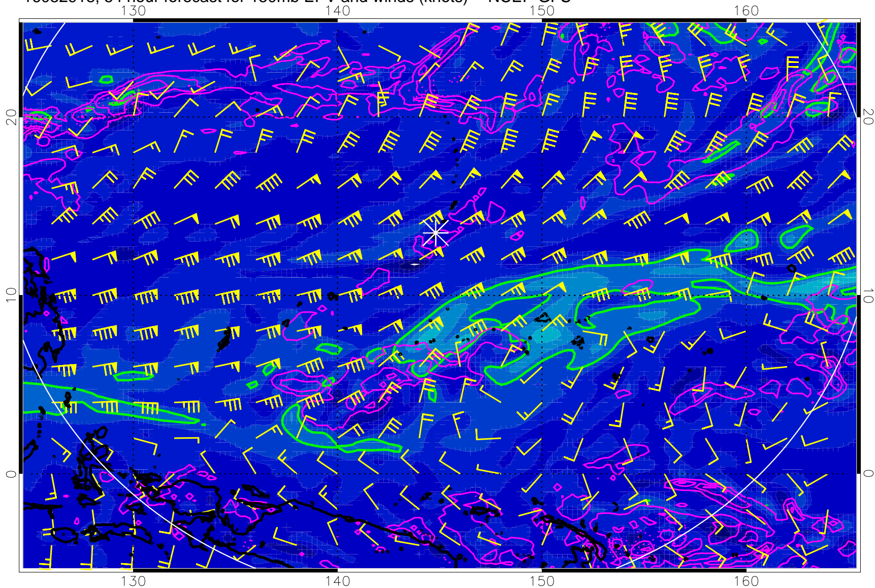
16082918, 54 hour forecast for 150mb EPV and winds (knots) -- NCEP GFS
