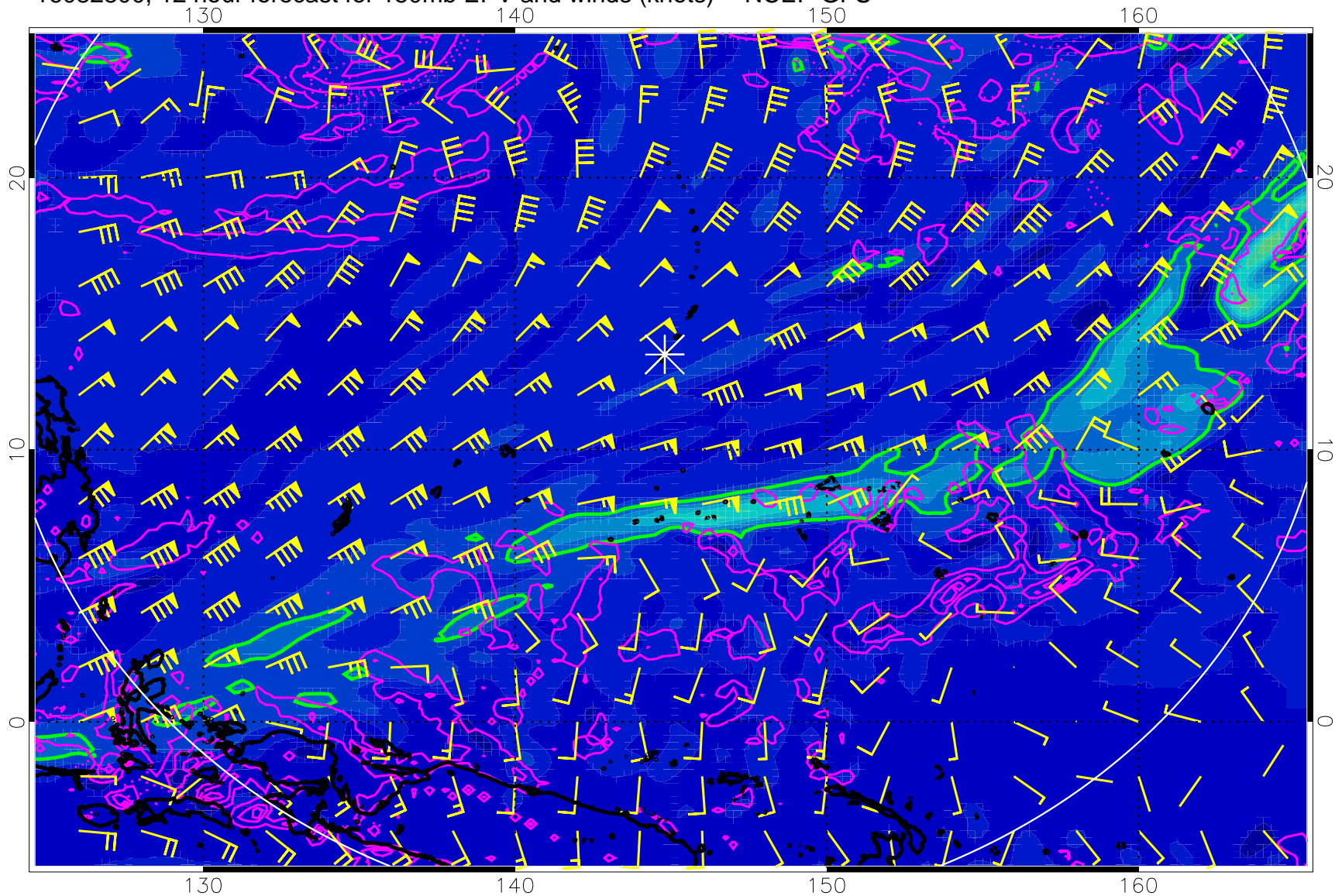
16082800, 12 hour forecast for 150mb EPV and winds (knots) -- NCEP GFS
