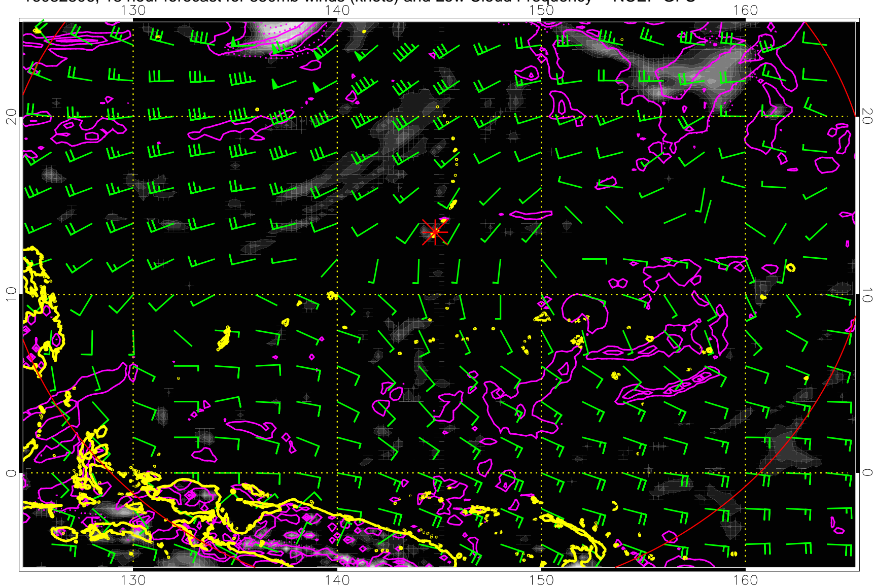
16082806, 18 hour forecast for 850mb winds (knots) and Low Cloud Frequency -- NCEP GFS
