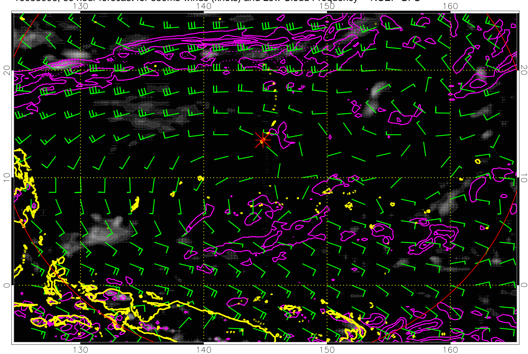
16083006, 66 hour forecast for 850mb winds (knots) and Low Cloud Frequency -- NCEP GFS
