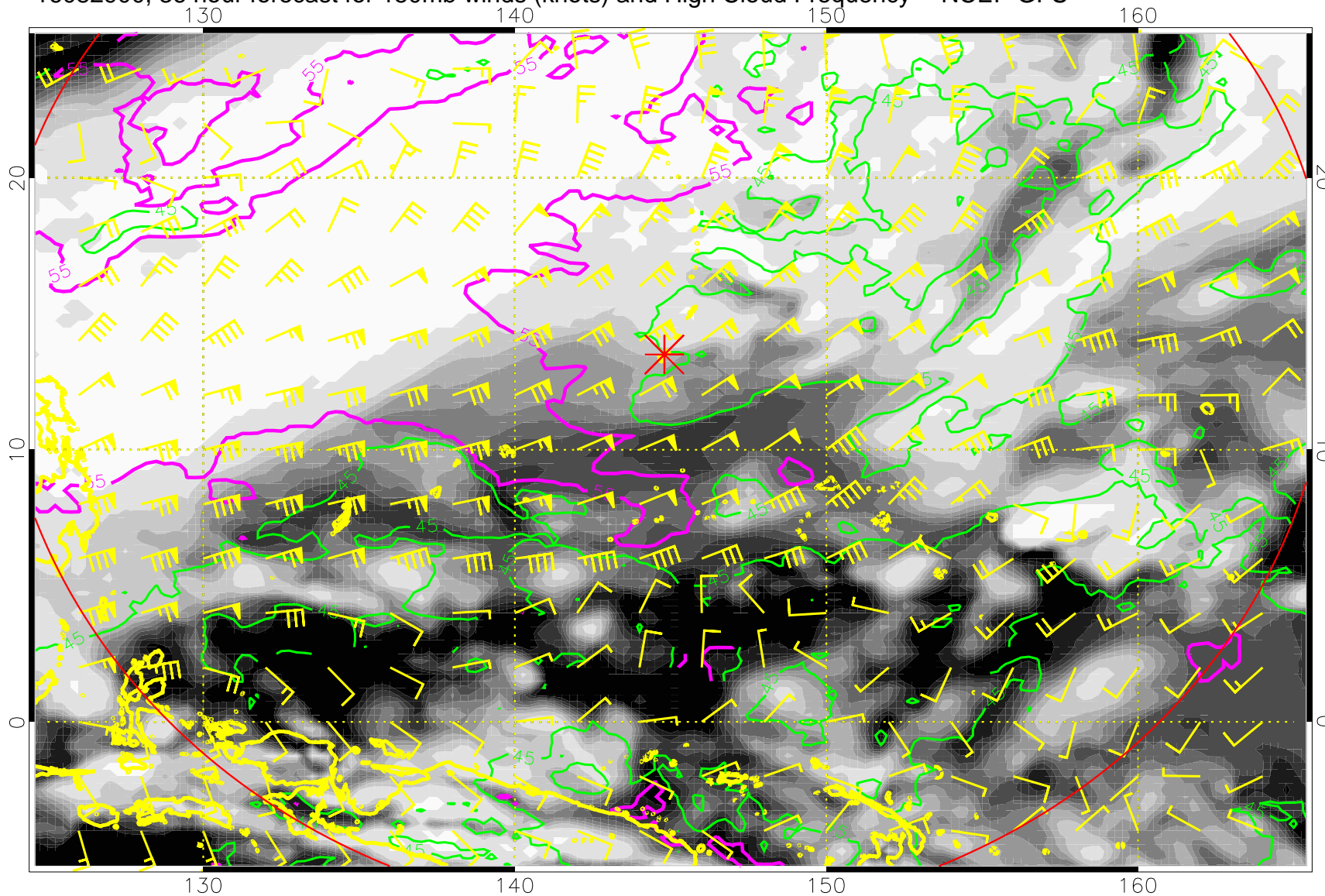
16082900, 36 hour forecast for 150mb winds (knots) and High Cloud Frequency -- NCEP GFS
