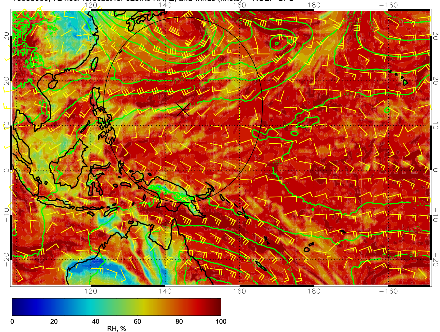
16083000, 72 hour forecast for 925mb RH, Z, and winds (knots) -- NCEP GFS
