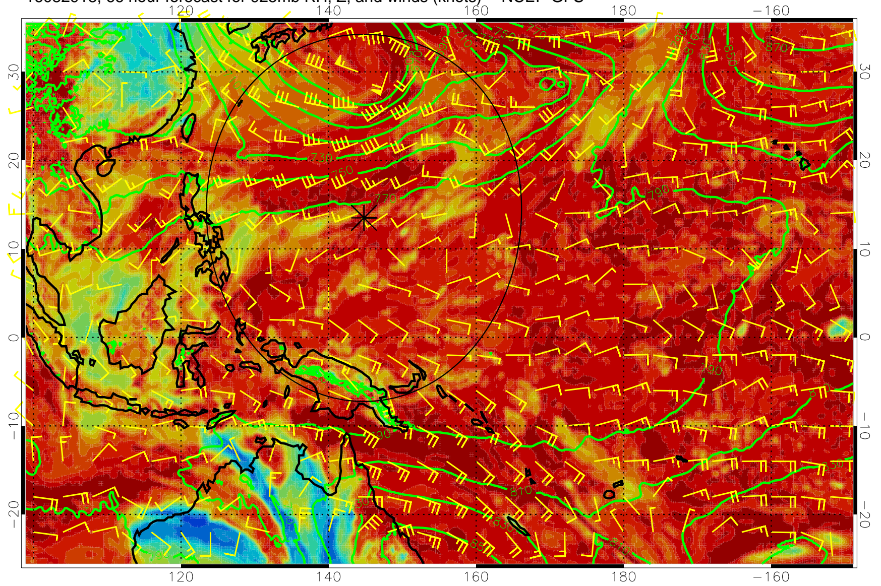
16082918, 66 hour forecast for 925mb RH, Z, and winds (knots) -- NCEP GFS
