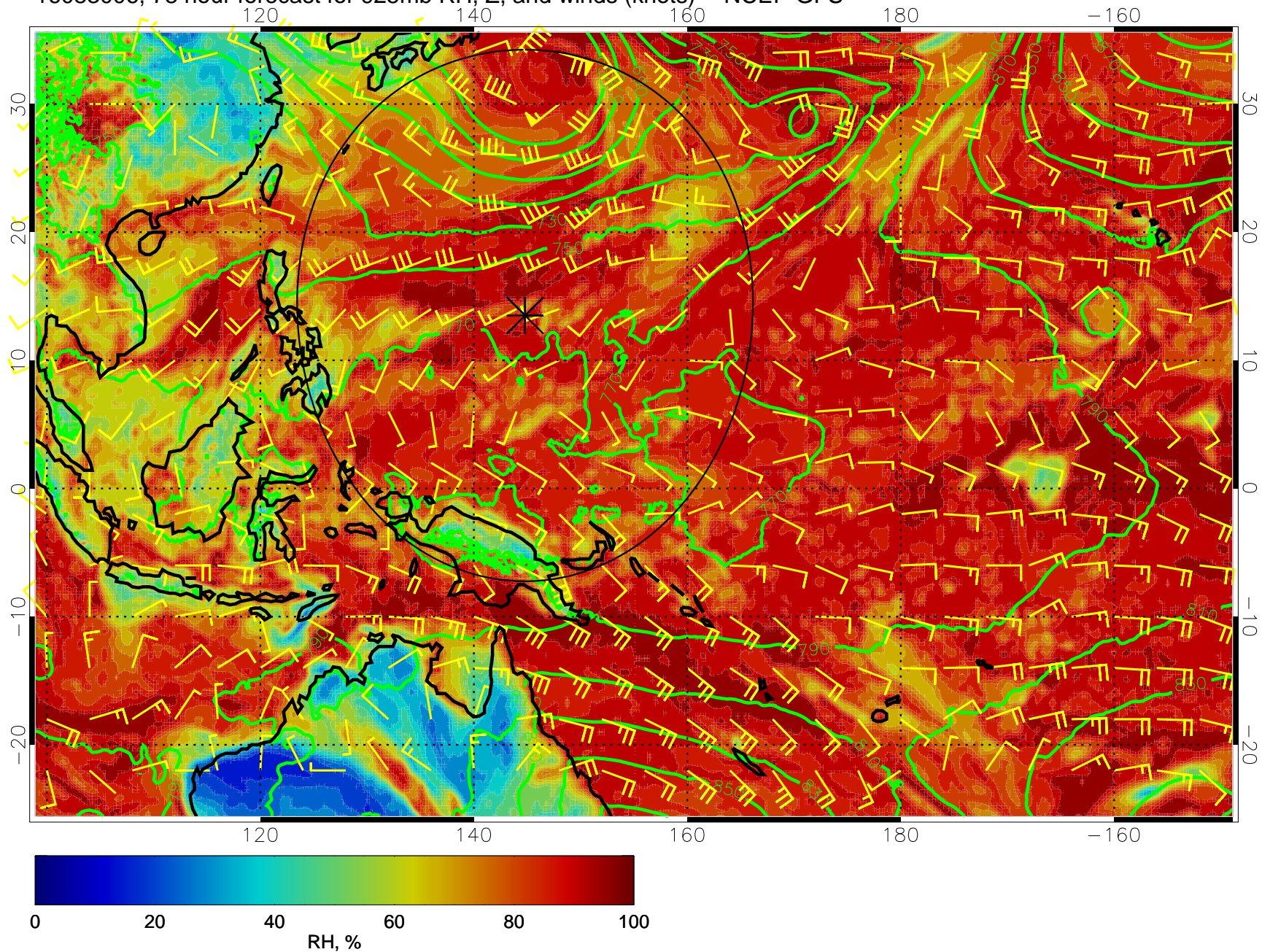
16083006, 78 hour forecast for 925mb RH, Z, and winds (knots) -- NCEP GFS
