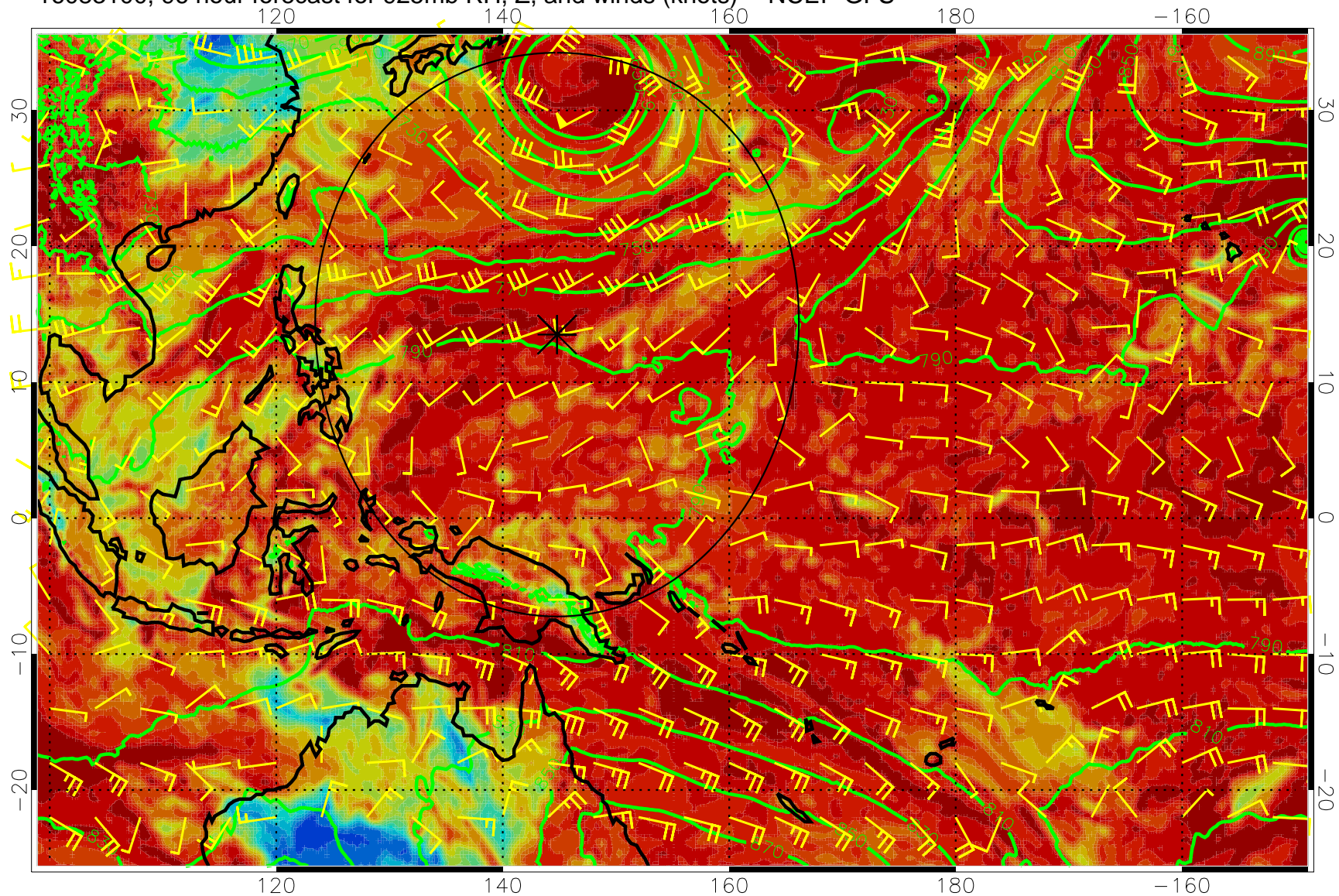
16083100, 96 hour forecast for 925mb RH, Z, and winds (knots) -- NCEP GFS
