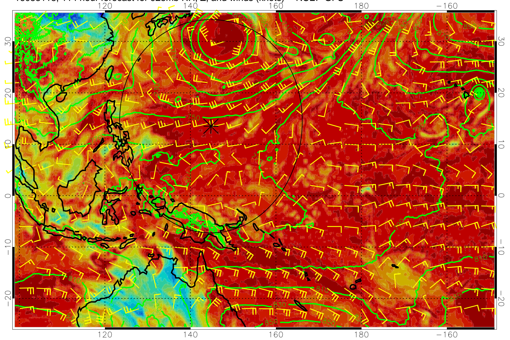
16083118, 114 hour forecast for 925mb RH, Z, and winds (knots) -- NCEP GFS
