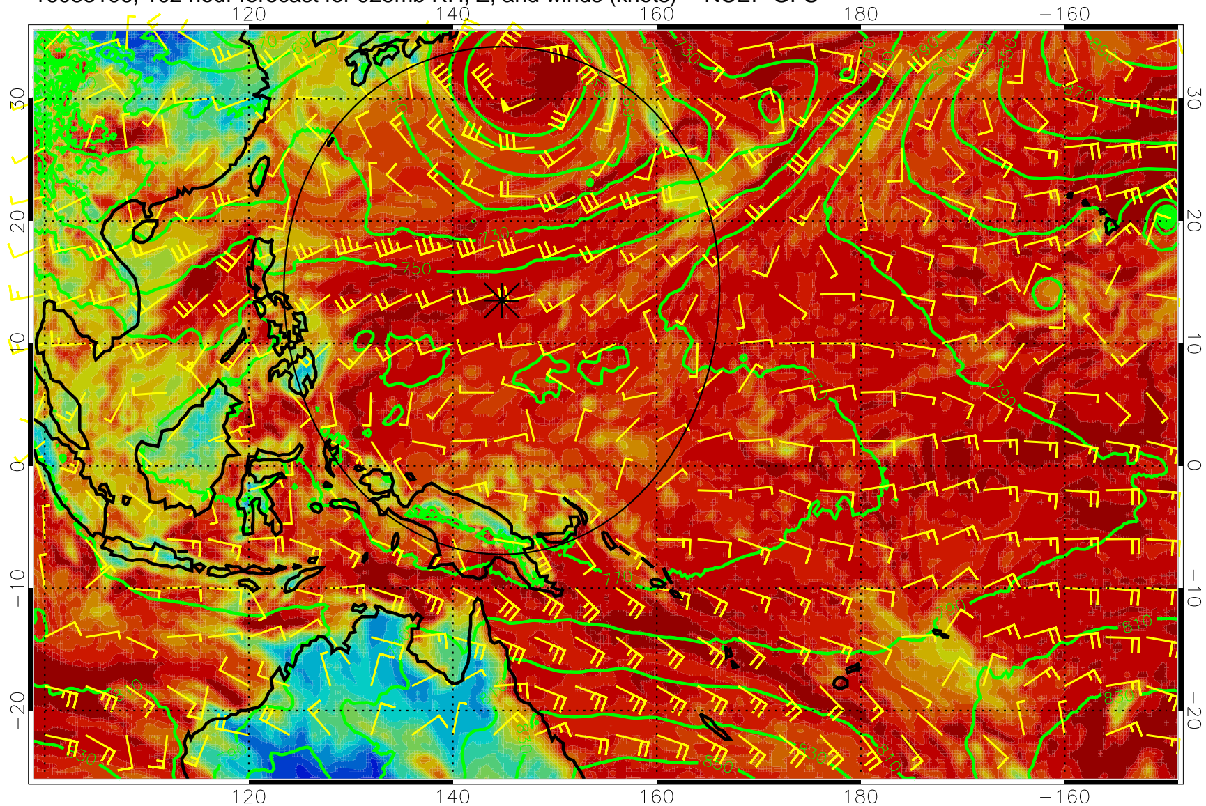
16083106, 102 hour forecast for 925mb RH, Z, and winds (knots) -- NCEP GFS
