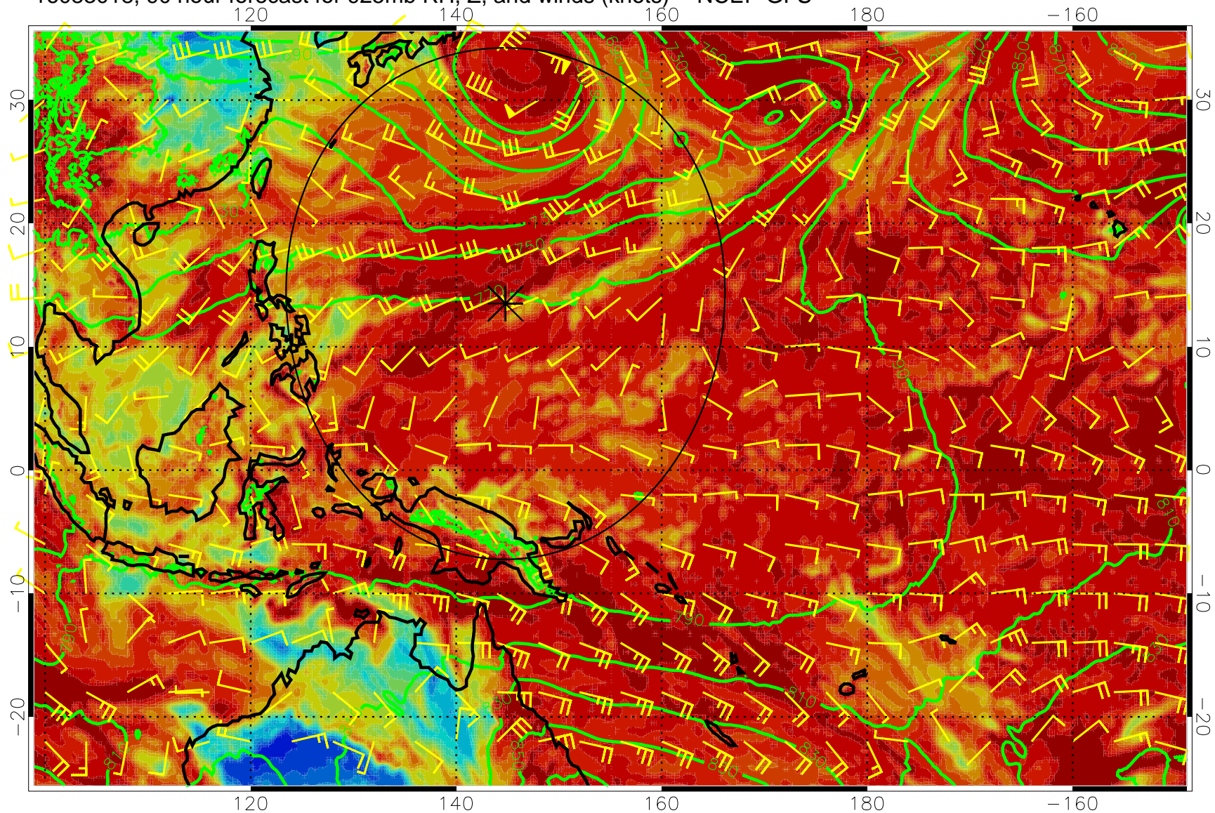
16083018, 90 hour forecast for 925mb RH, Z, and winds (knots) -- NCEP GFS
