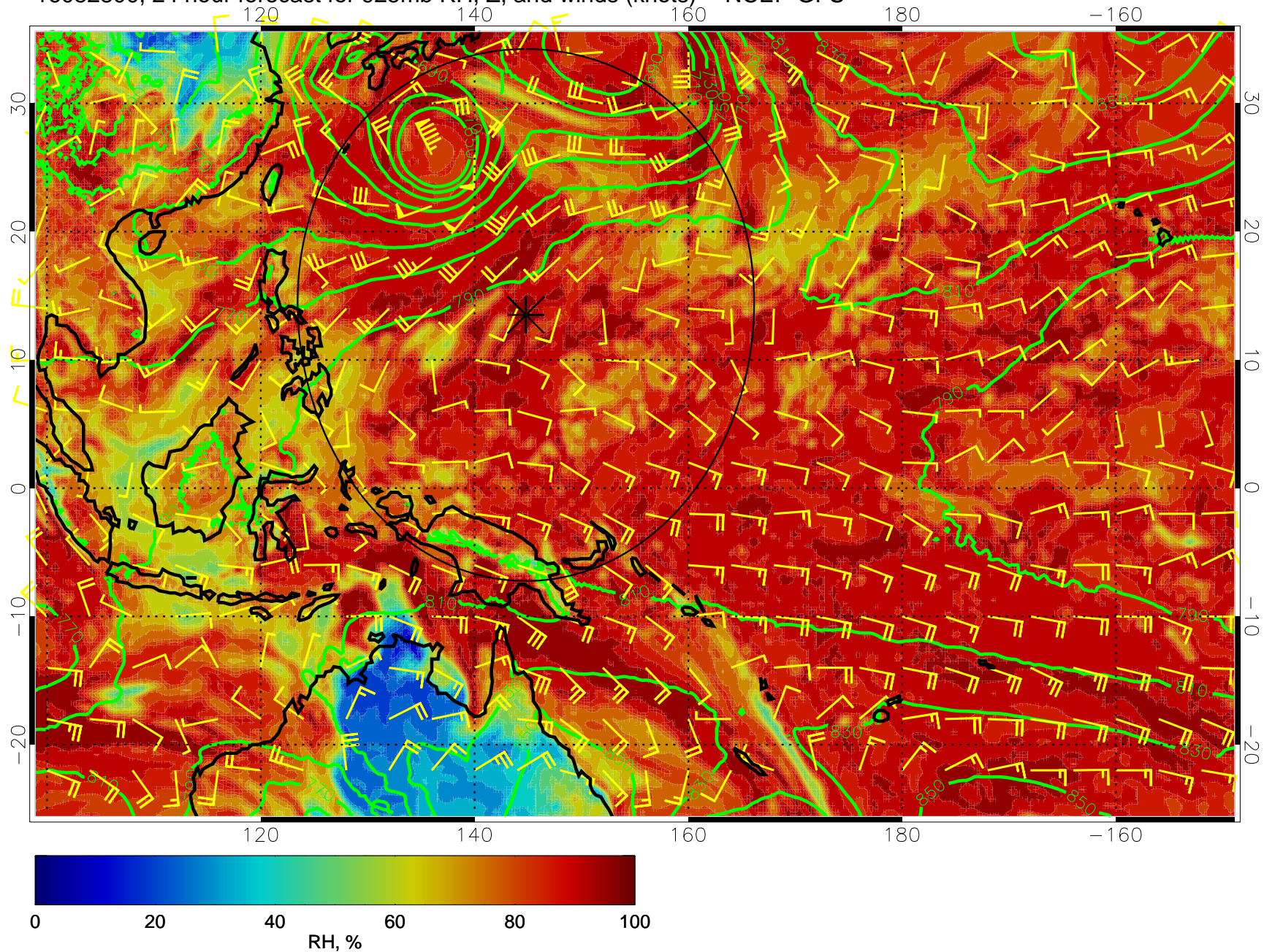
16082800, 24 hour forecast for 925mb RH, Z, and winds (knots) -- NCEP GFS
