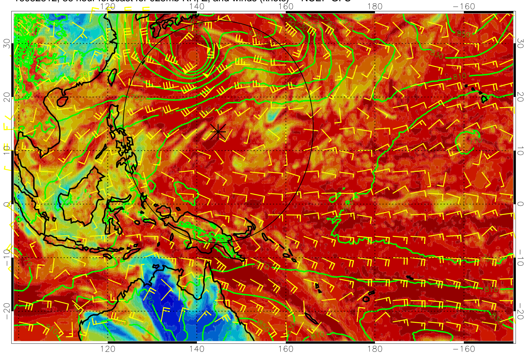
16082812, 36 hour forecast for 925mb RH, Z, and winds (knots) -- NCEP GFS
