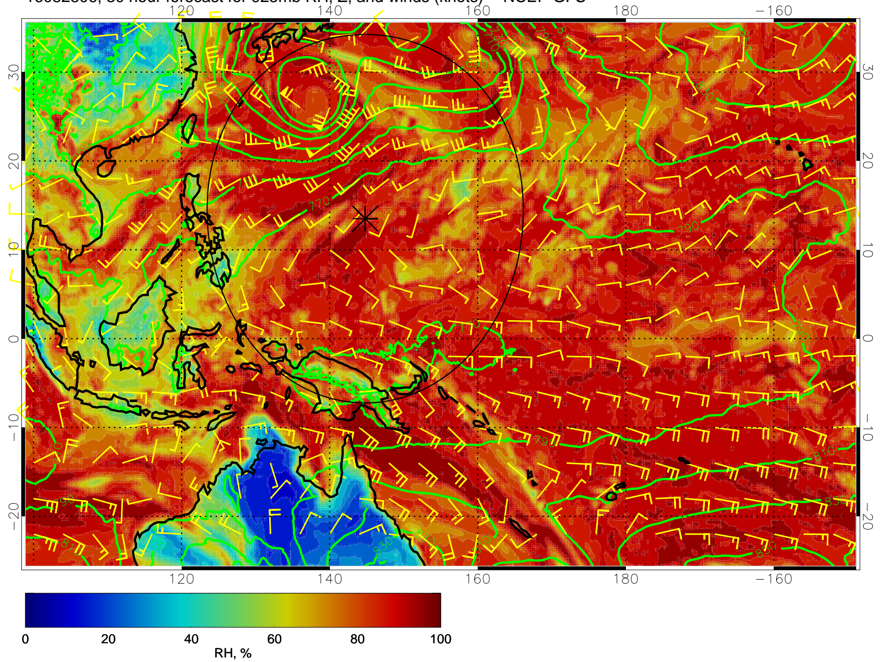
16082806, 30 hour forecast for 925mb RH, Z, and winds (knots) -- NCEP GFS
