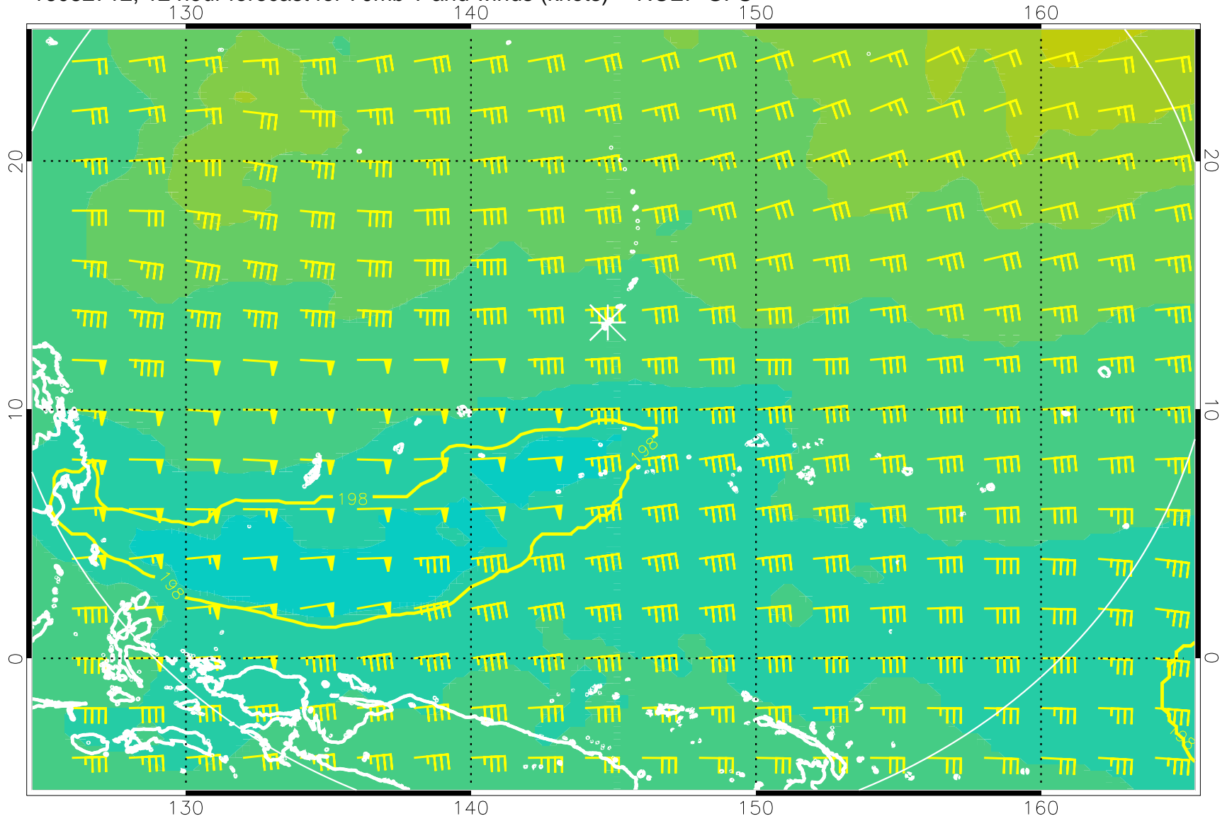
16082712, 12 hour forecast for 70mb T and winds (knots) -- NCEP GFS
