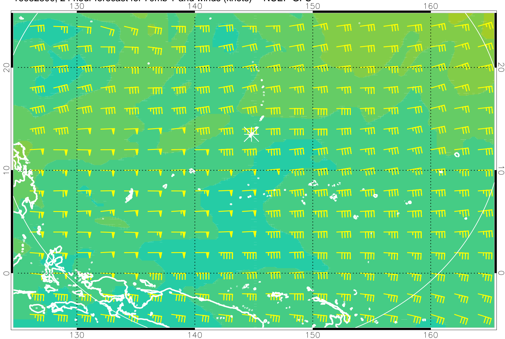
16082800, 24 hour forecast for 70mb T and winds (knots) -- NCEP GFS
