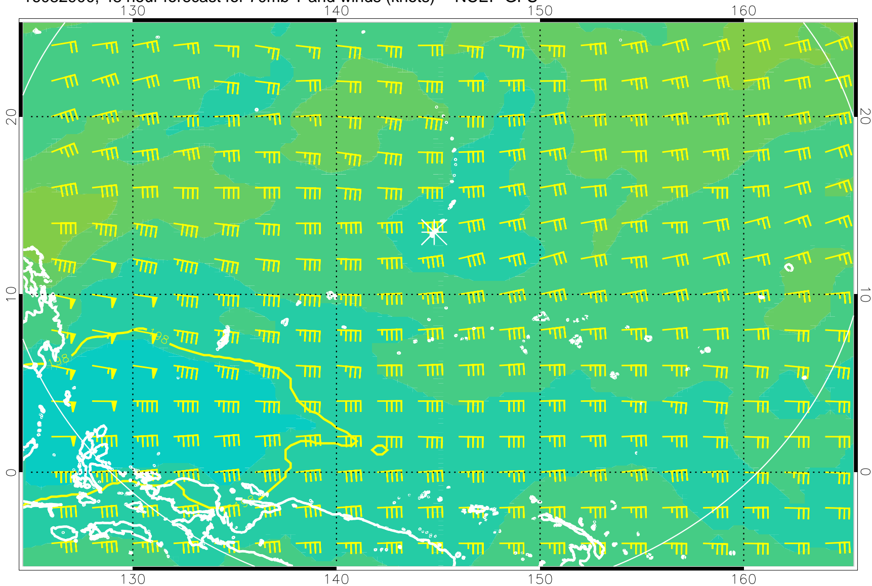
16082900, 48 hour forecast for 70mb T and winds (knots) -- NCEP GFS
