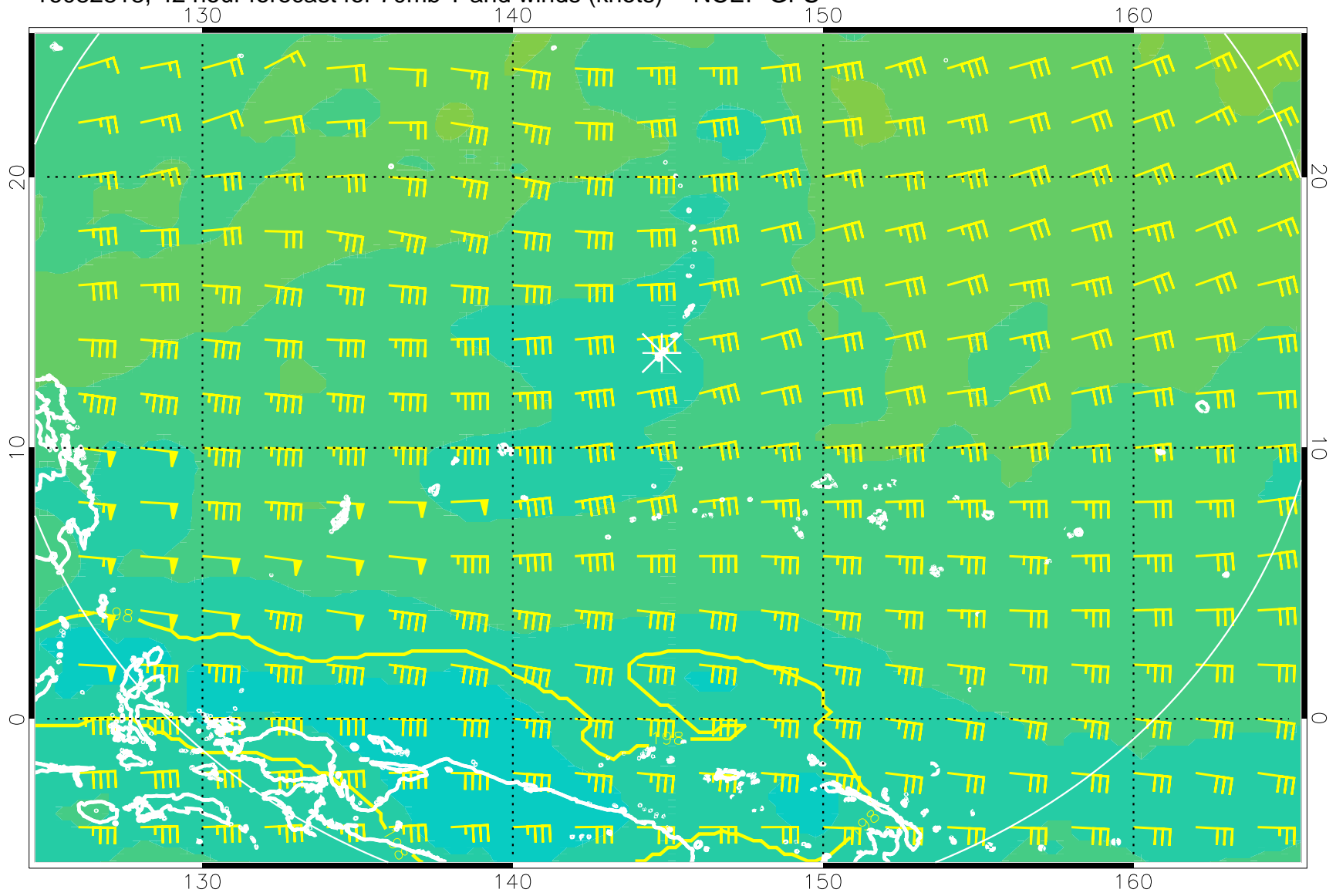
16082818, 42 hour forecast for 70mb T and winds (knots) -- NCEP GFS
