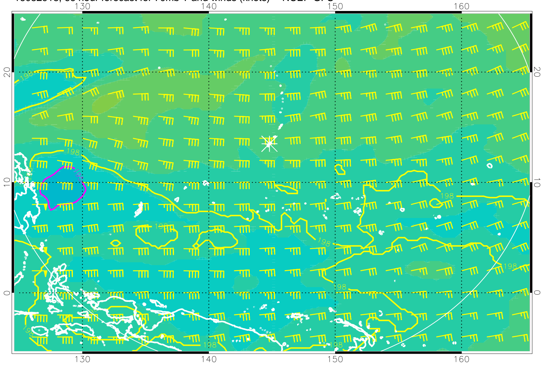
16082918, 66 hour forecast for 70mb T and winds (knots) -- NCEP GFS
