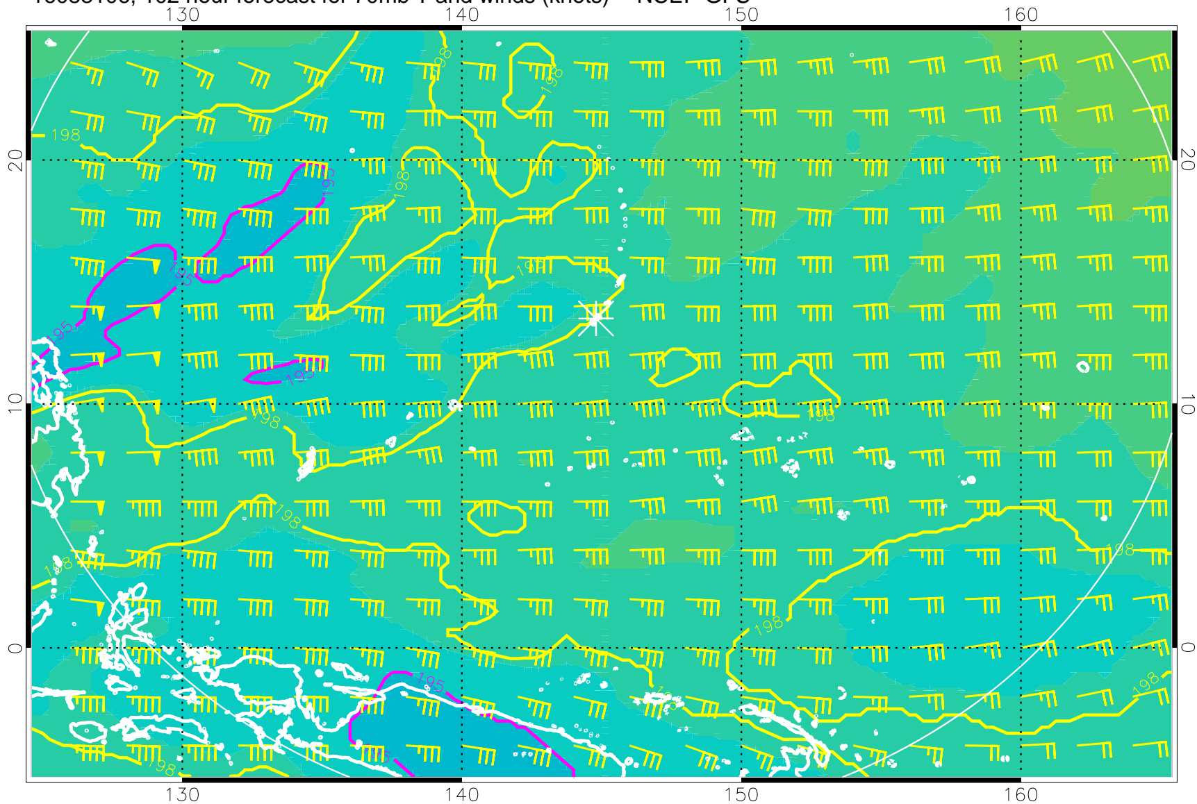
16083106, 102 hour forecast for 70mb T and winds (knots) -- NCEP GFS
