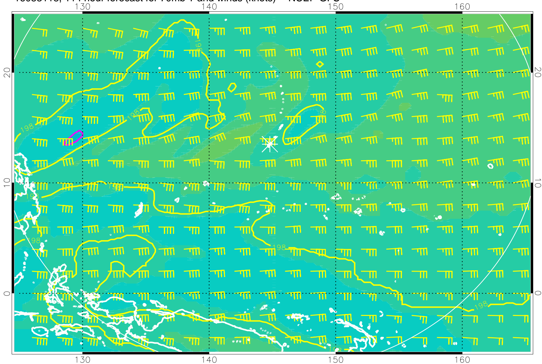
16083118, 114 hour forecast for 70mb T and winds (knots) -- NCEP GFS
