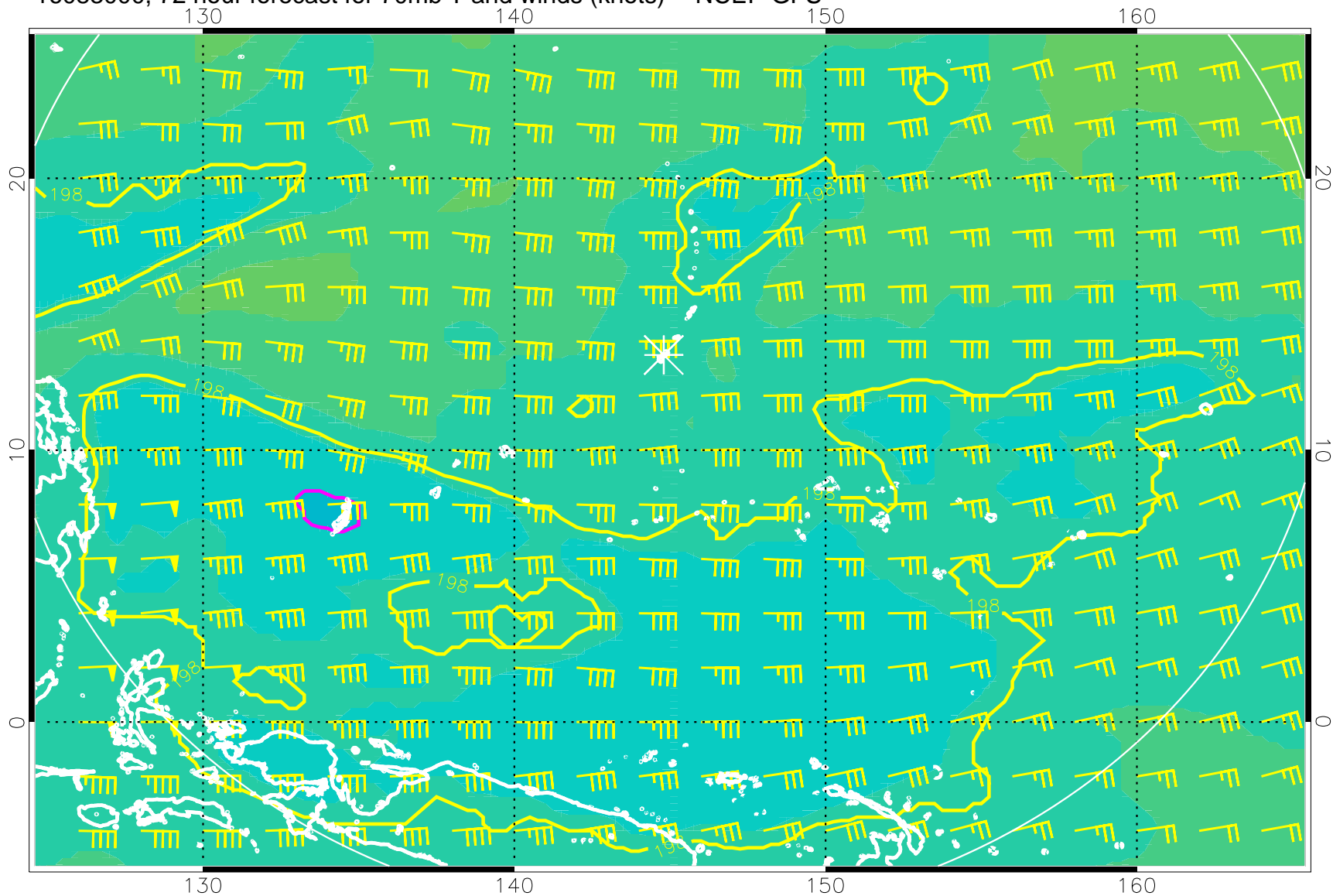
16083000, 72 hour forecast for 70mb T and winds (knots) -- NCEP GFS
