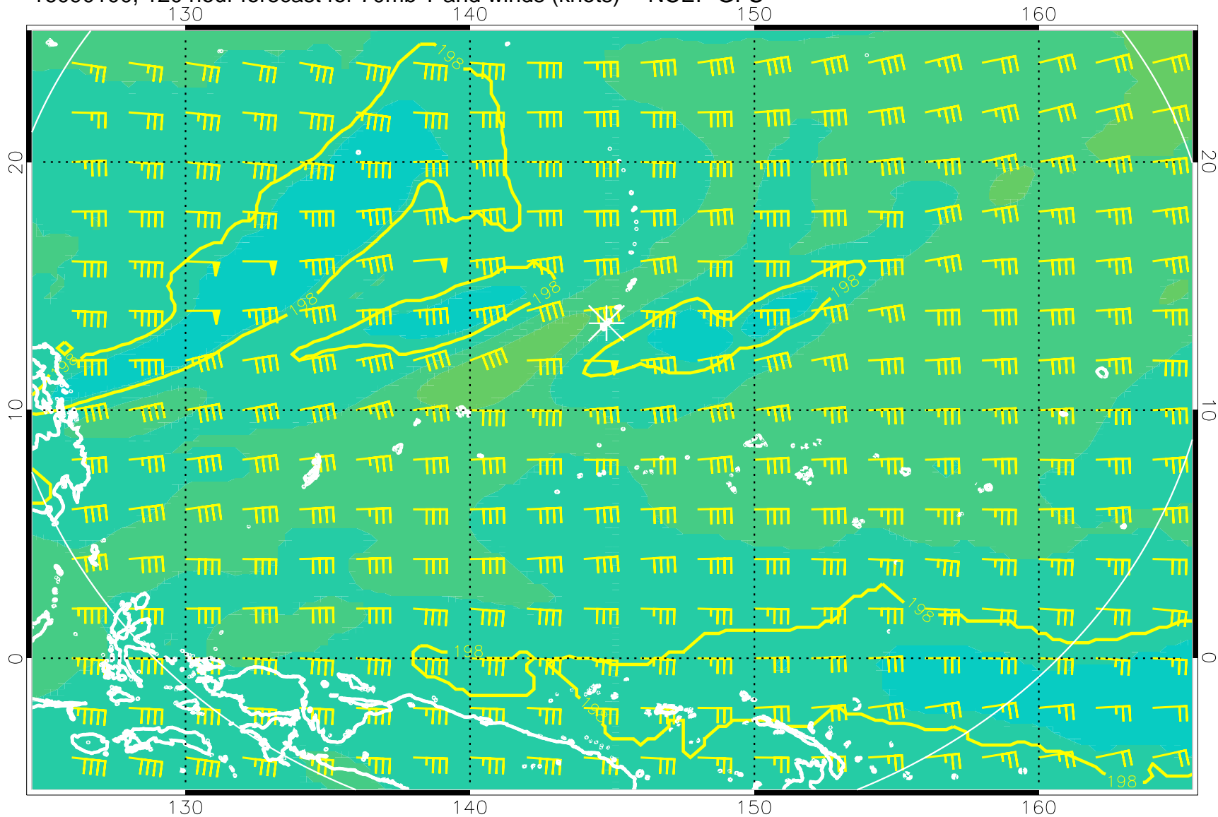
16090100, 120 hour forecast for 70mb T and winds (knots) -- NCEP GFS
