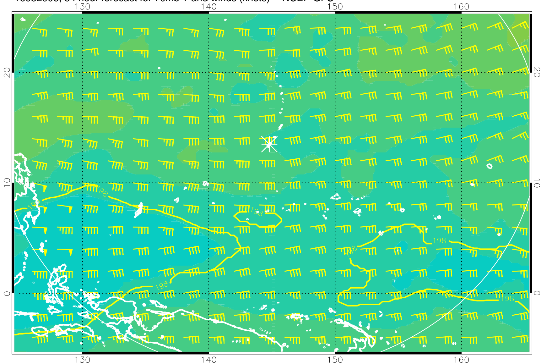
16082906, 54 hour forecast for 70mb T and winds (knots) -- NCEP GFS
