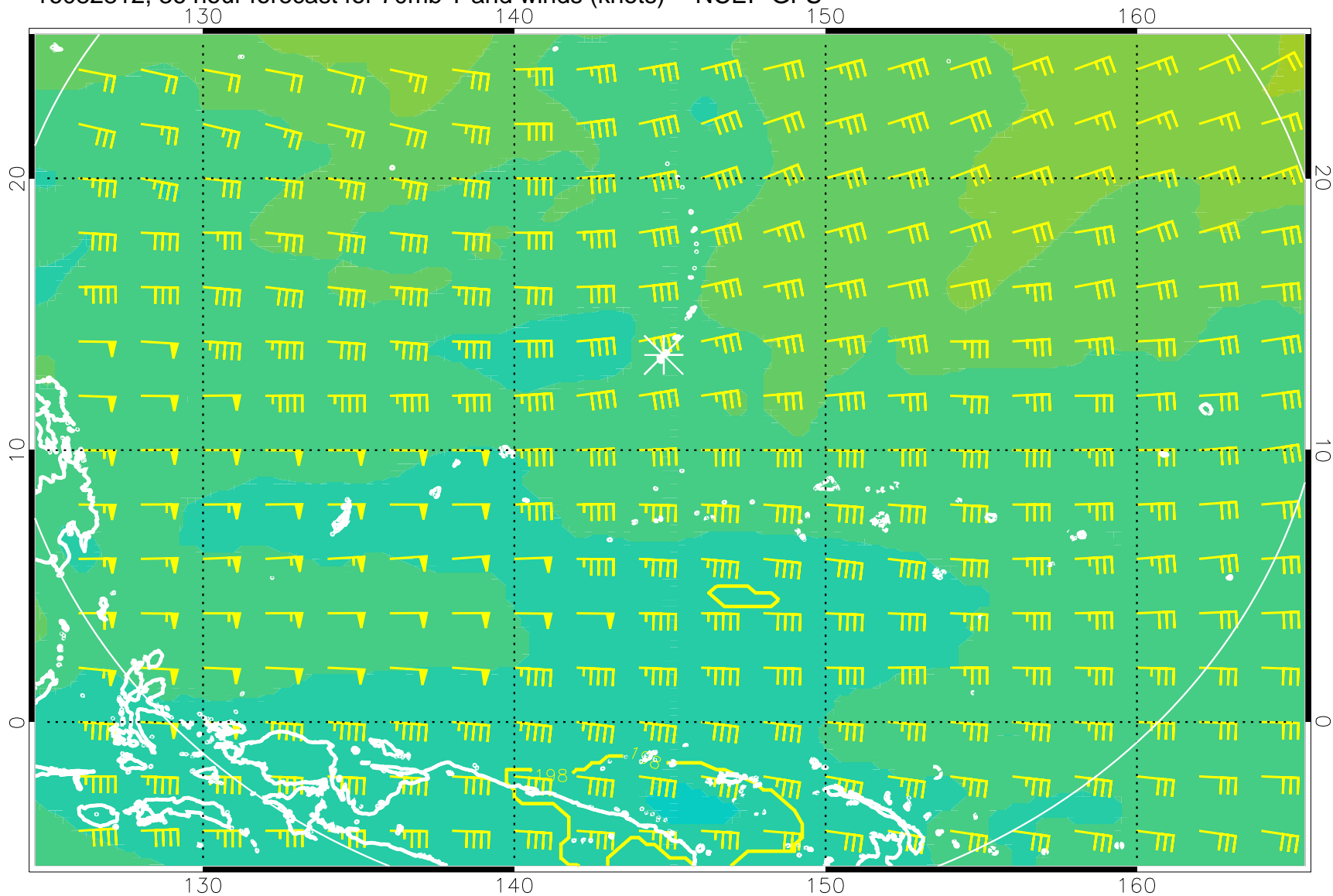
16082812, 36 hour forecast for 70mb T and winds (knots) -- NCEP GFS
