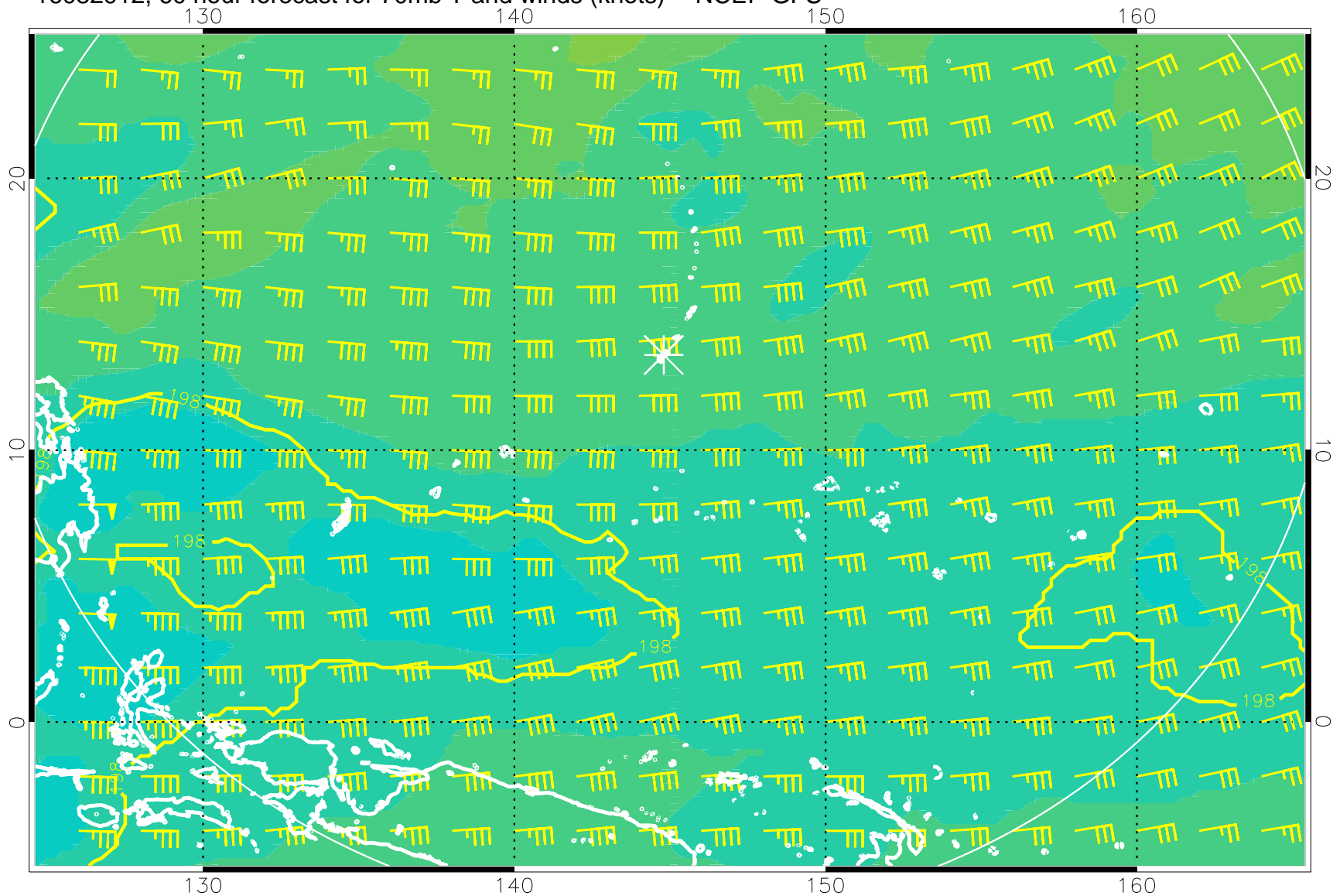
16082912, 60 hour forecast for 70mb T and winds (knots) -- NCEP GFS
