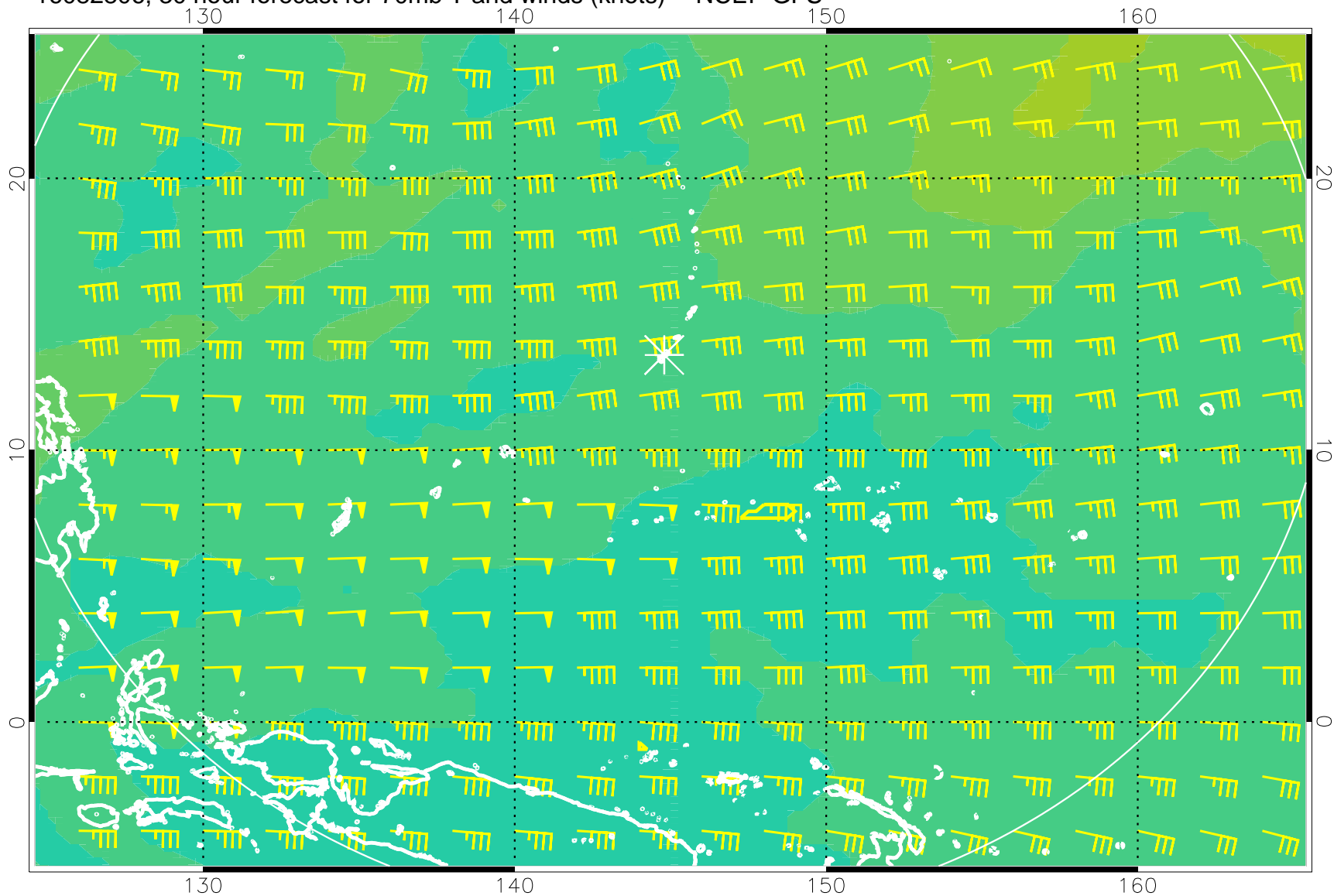
16082806, 30 hour forecast for 70mb T and winds (knots) -- NCEP GFS
