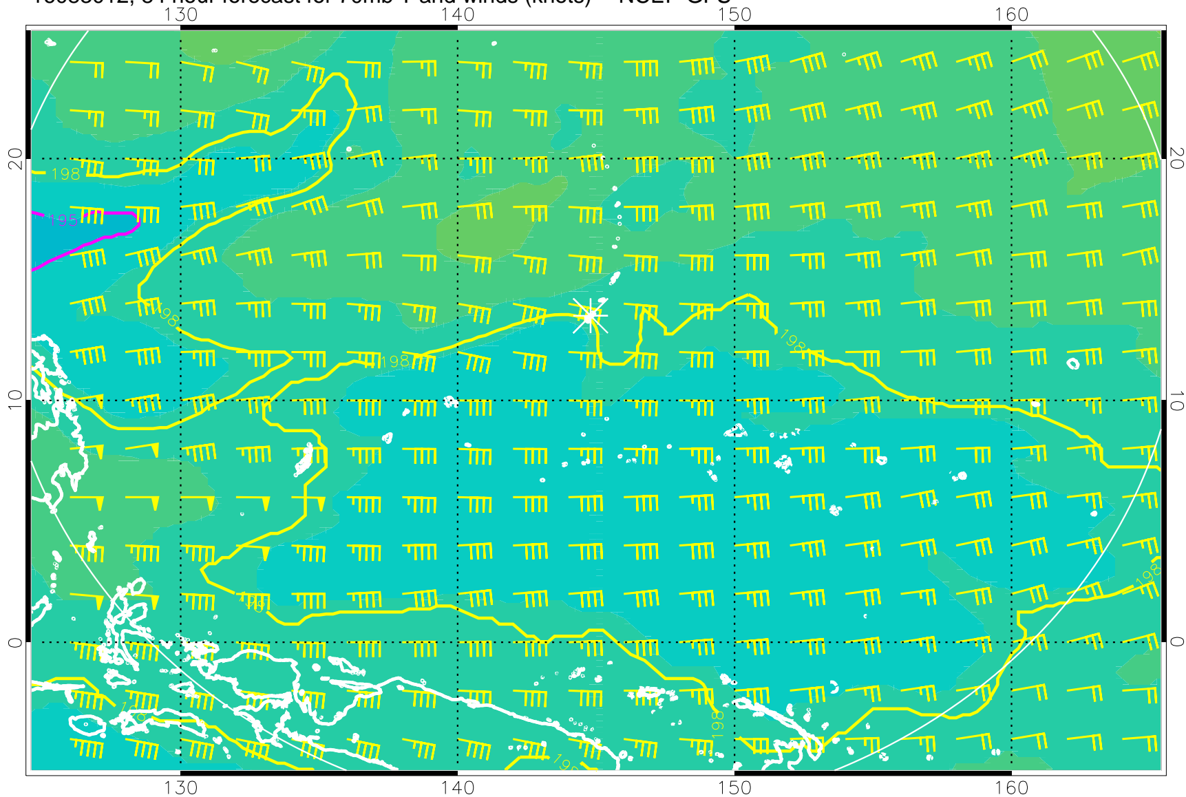
16083012, 84 hour forecast for 70mb T and winds (knots) -- NCEP GFS
