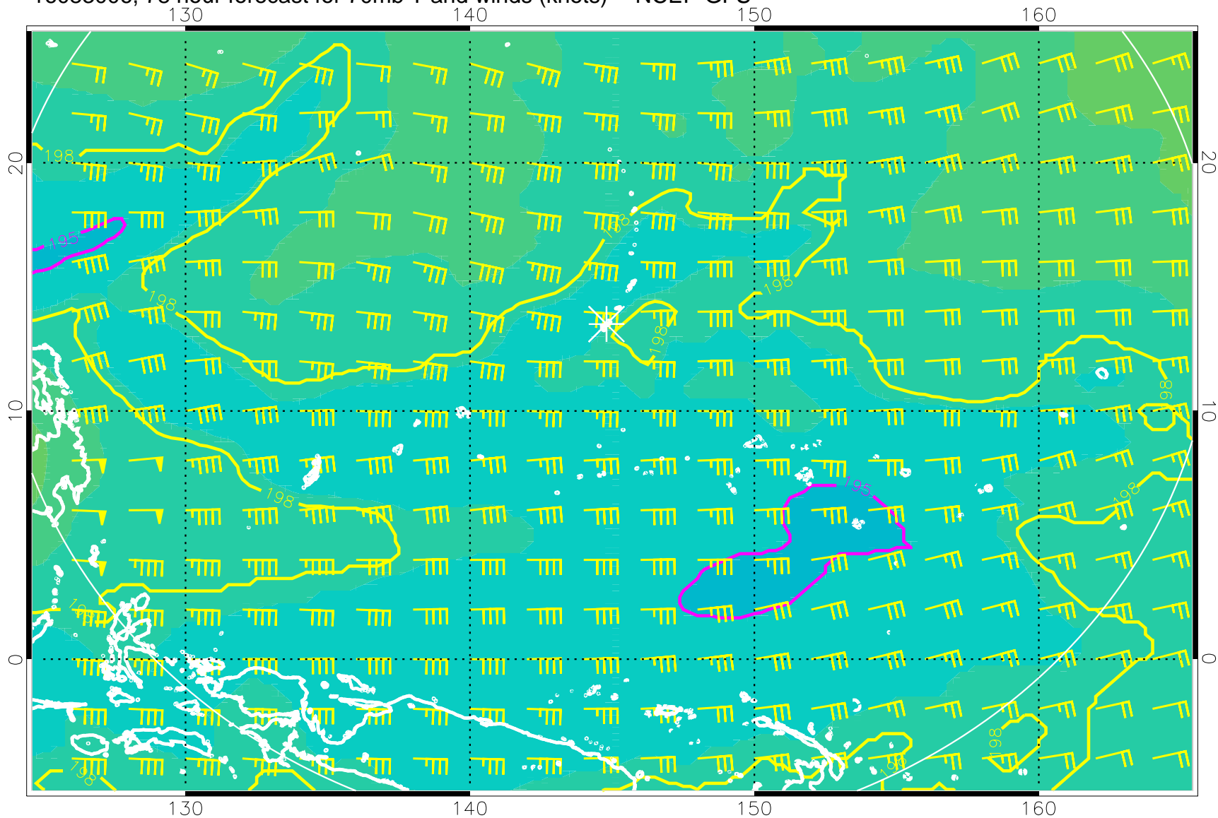
16083006, 78 hour forecast for 70mb T and winds (knots) -- NCEP GFS
