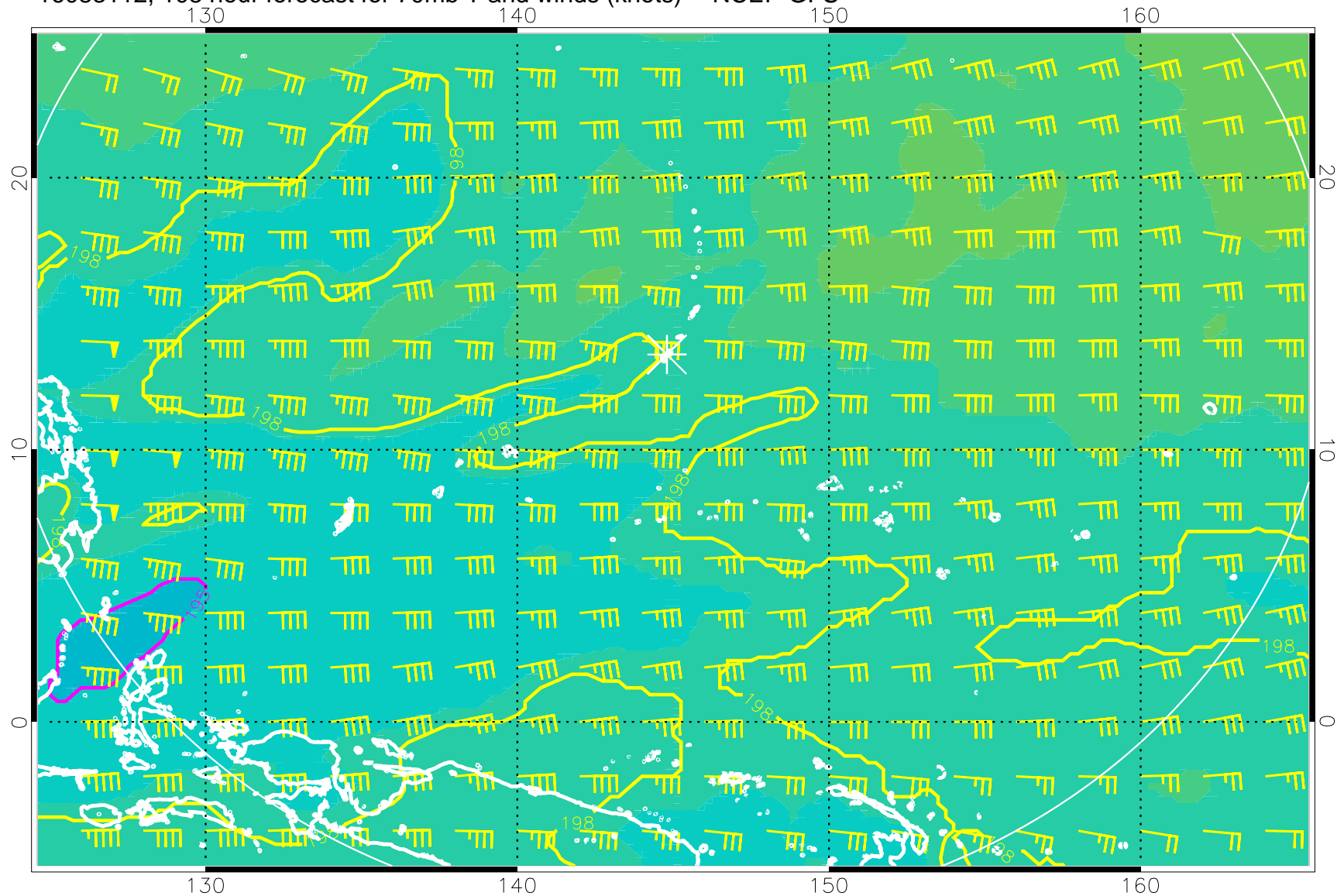
16083112, 108 hour forecast for 70mb T and winds (knots) -- NCEP GFS
