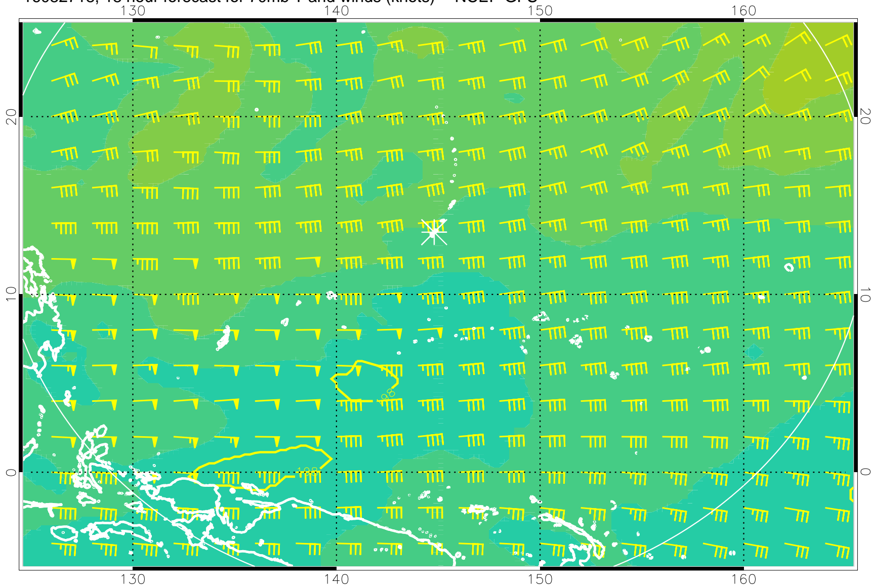
16082718, 18 hour forecast for 70mb T and winds (knots) -- NCEP GFS
