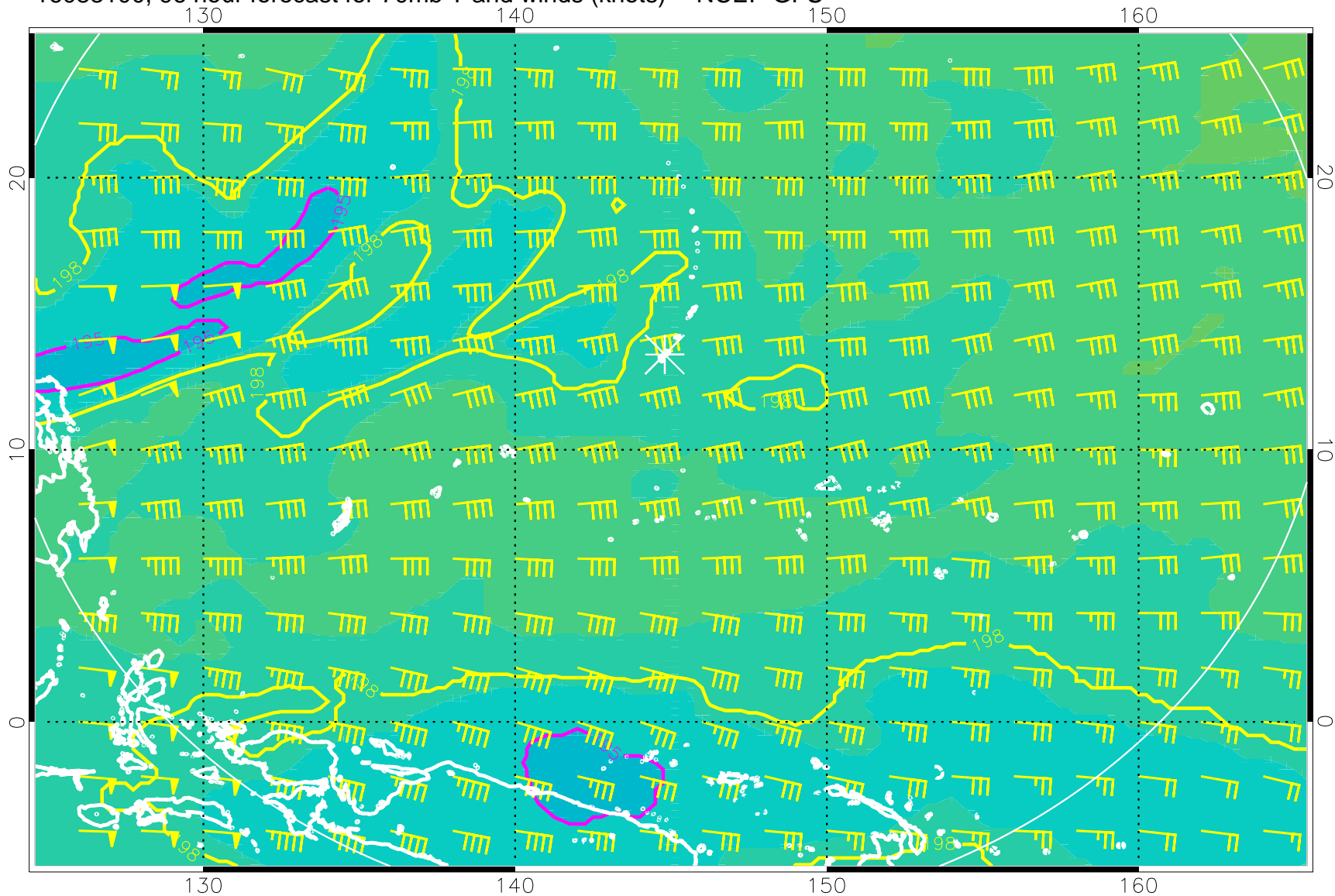
16083100, 96 hour forecast for 70mb T and winds (knots) -- NCEP GFS
