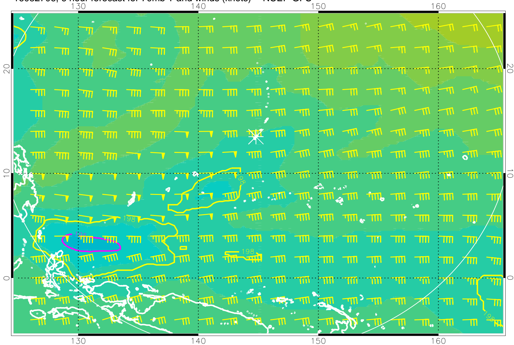
16082706, 6 hour forecast for 70mb T and winds (knots) -- NCEP GFS
