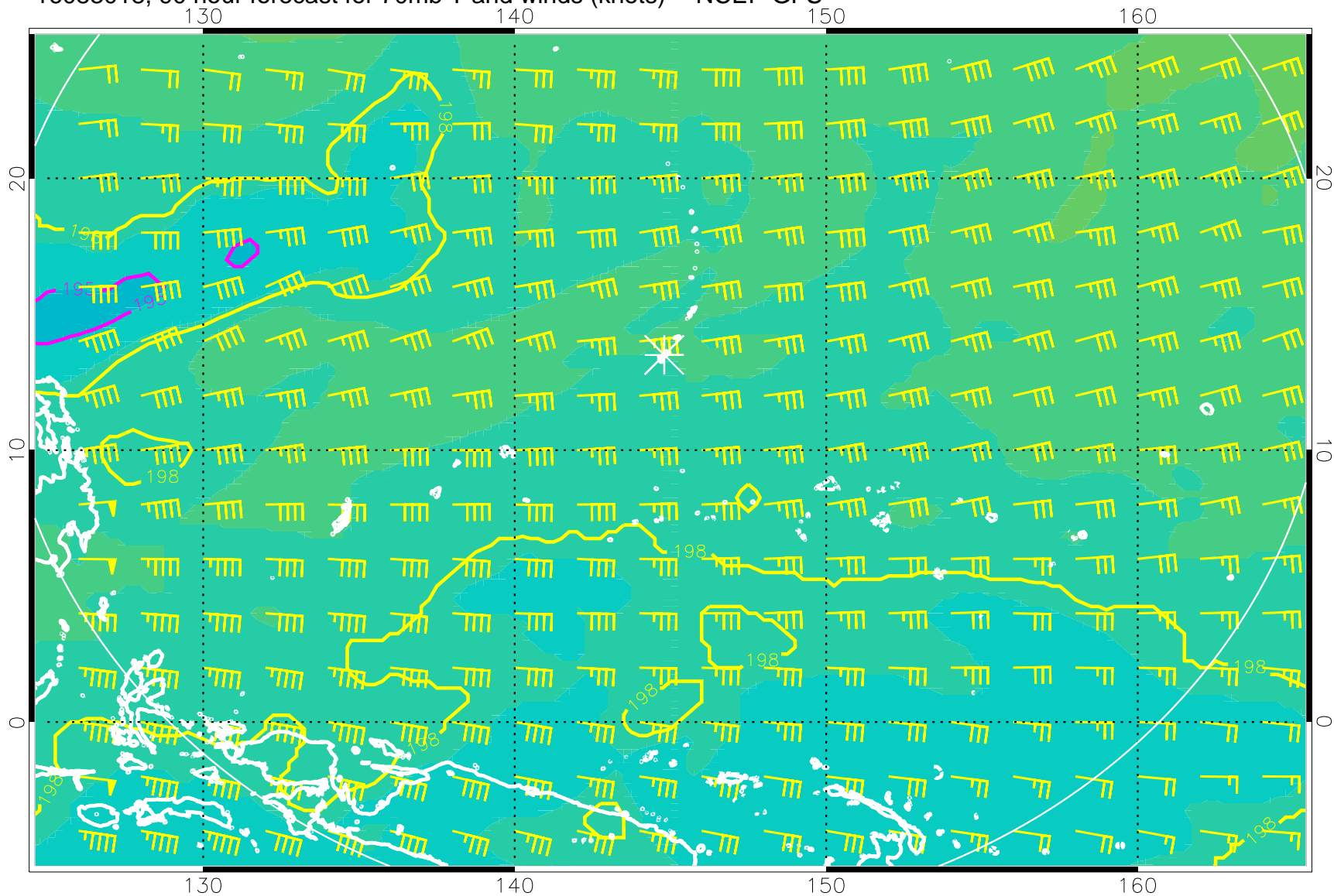
16083018, 90 hour forecast for 70mb T and winds (knots) -- NCEP GFS
