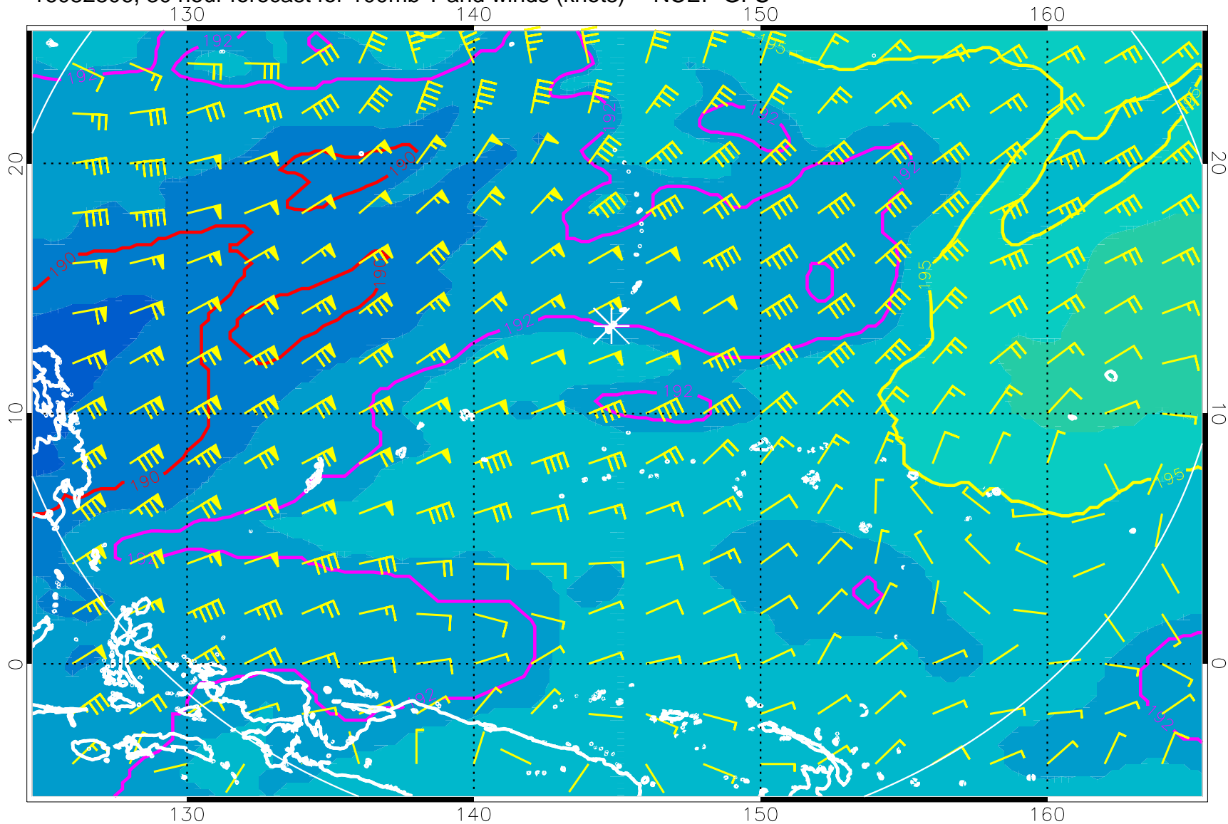
16082806, 30 hour forecast for 100mb T and winds (knots) -- NCEP GFS
