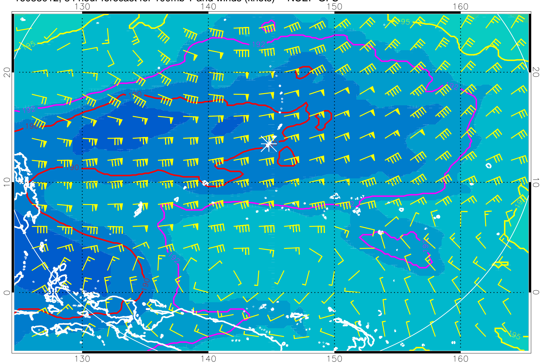
16083012, 84 hour forecast for 100mb T and winds (knots) -- NCEP GFS
