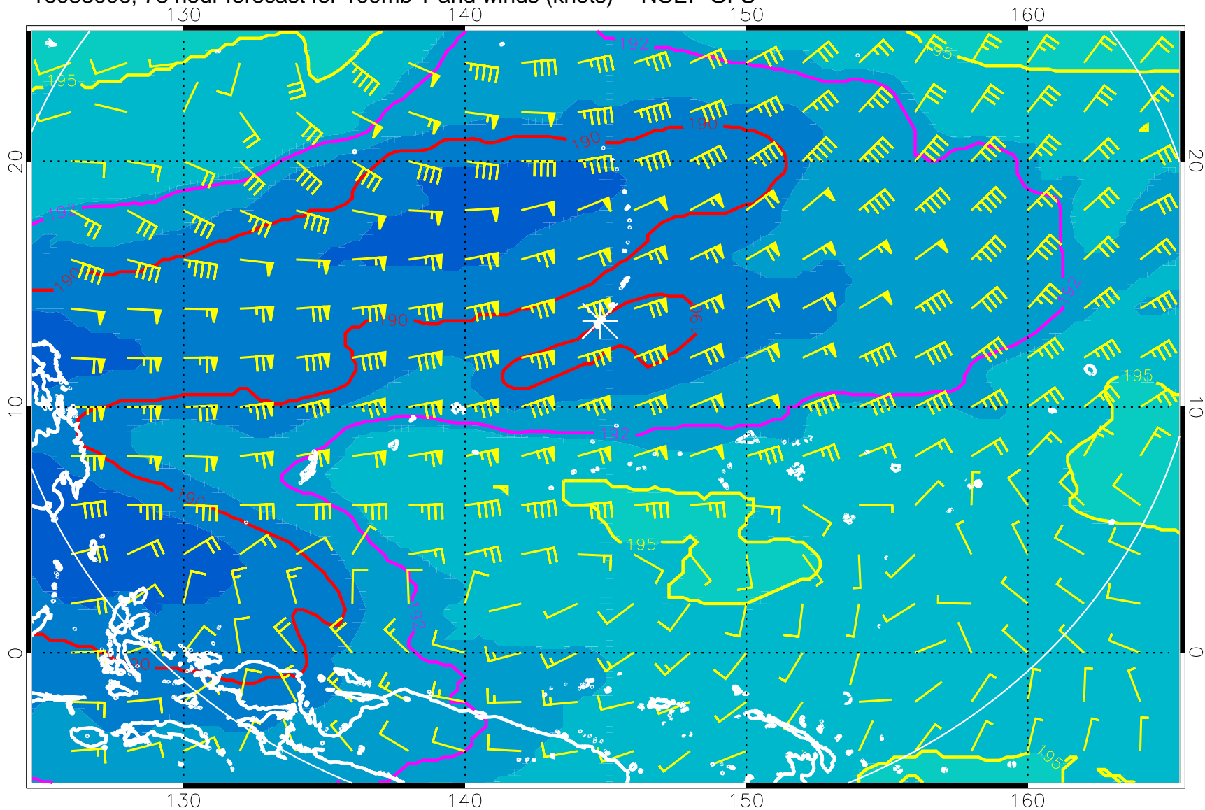
16083006, 78 hour forecast for 100mb T and winds (knots) -- NCEP GFS
