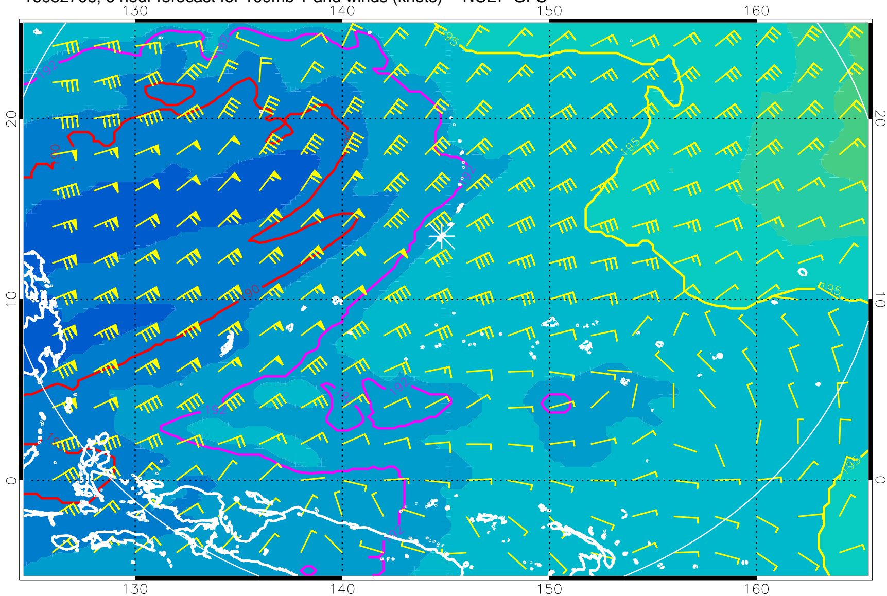
16082706, 6 hour forecast for 100mb T and winds (knots) -- NCEP GFS
