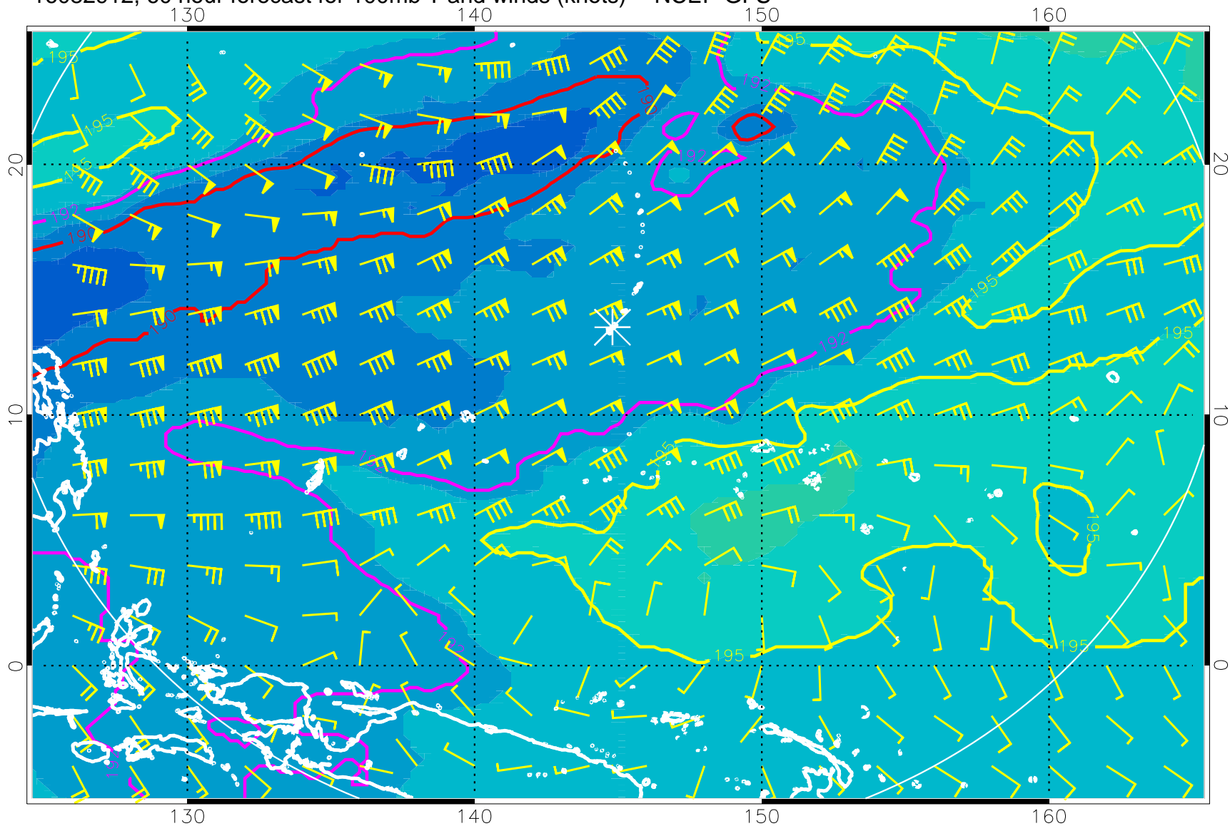
16082912, 60 hour forecast for 100mb T and winds (knots) -- NCEP GFS
