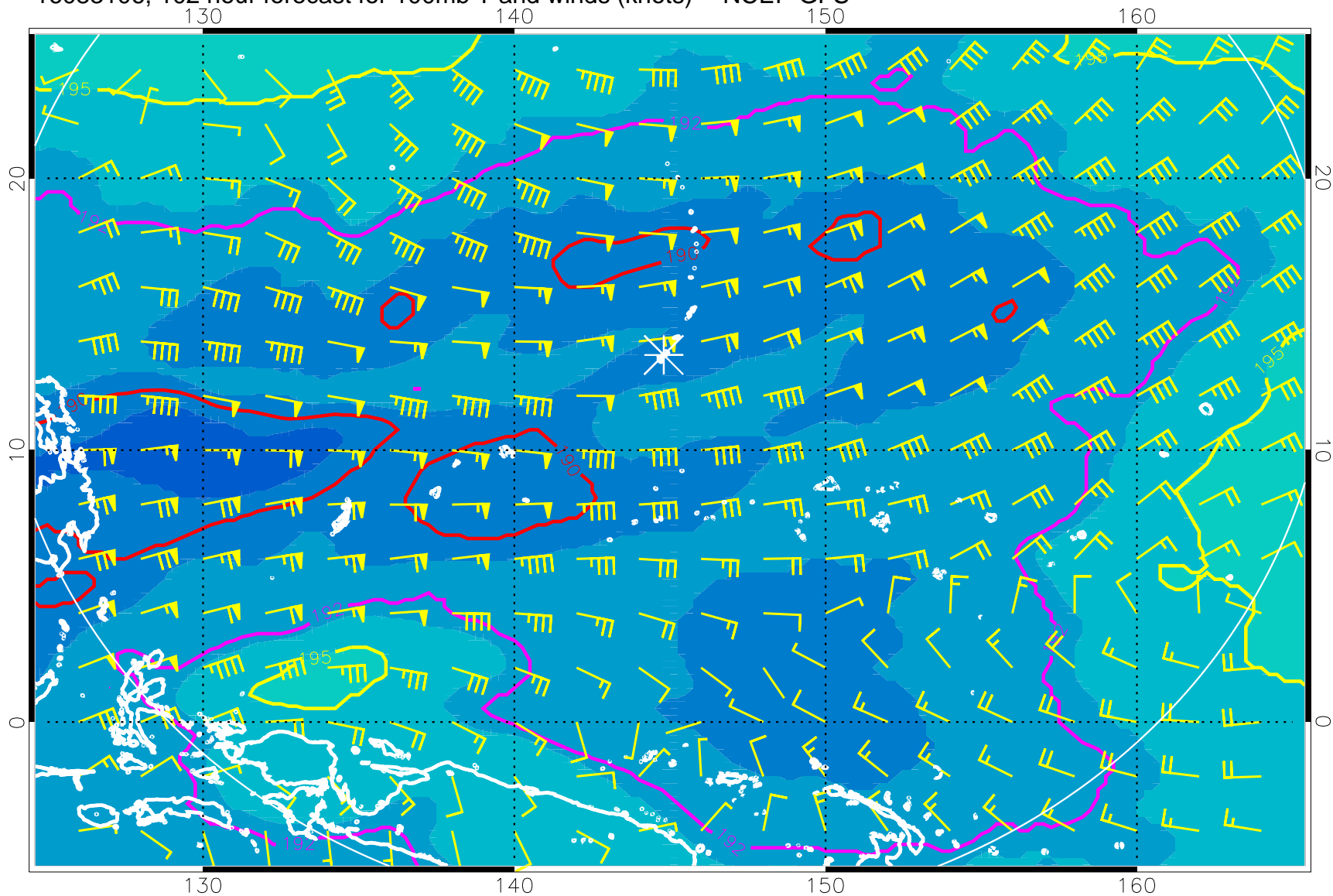
16083106, 102 hour forecast for 100mb T and winds (knots) -- NCEP GFS
