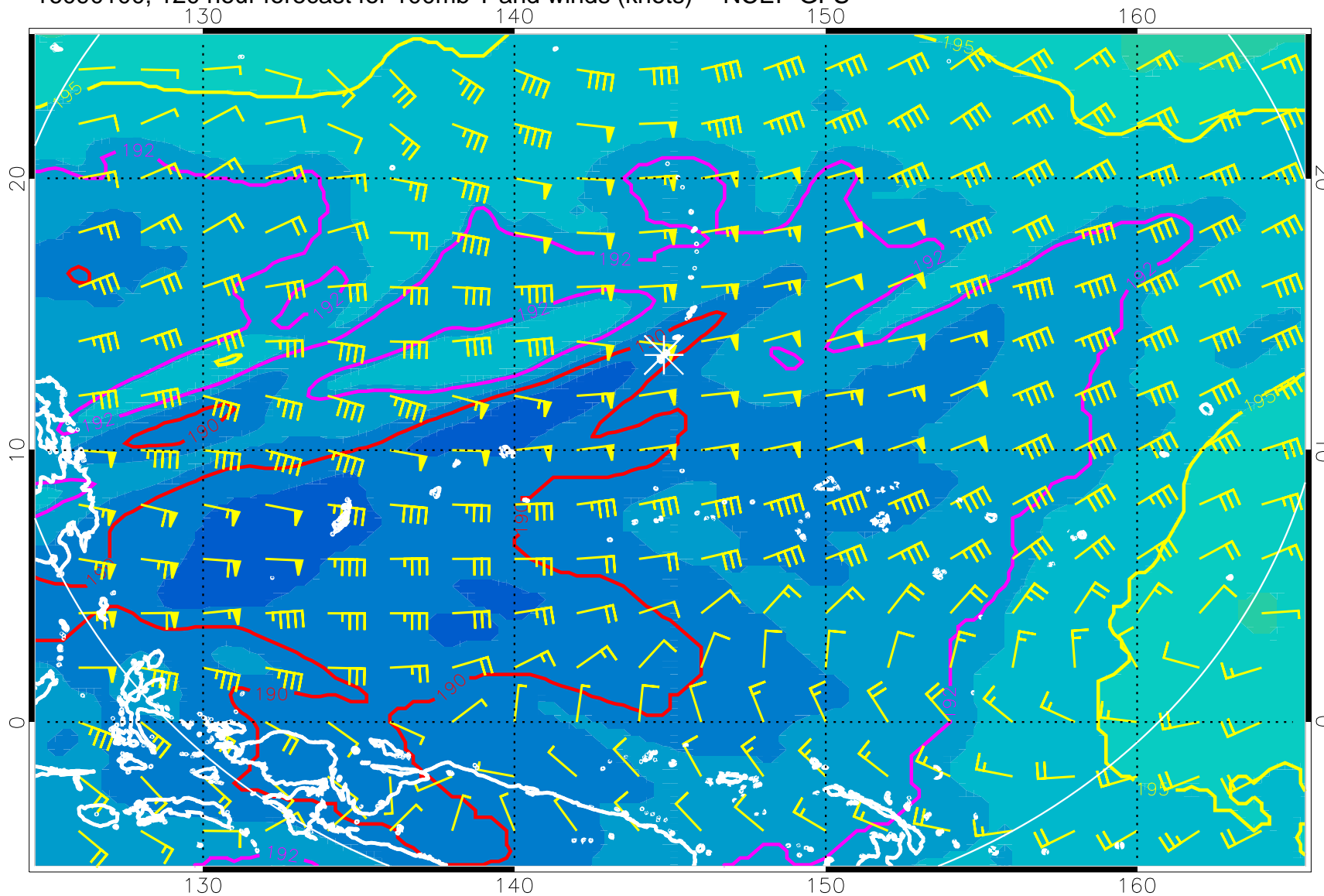
16090100, 120 hour forecast for 100mb T and winds (knots) -- NCEP GFS
