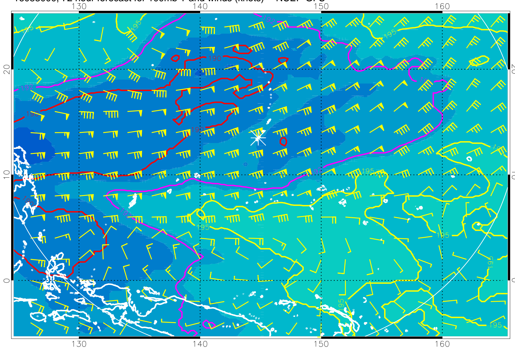
16083000, 72 hour forecast for 100mb T and winds (knots) -- NCEP GFS
