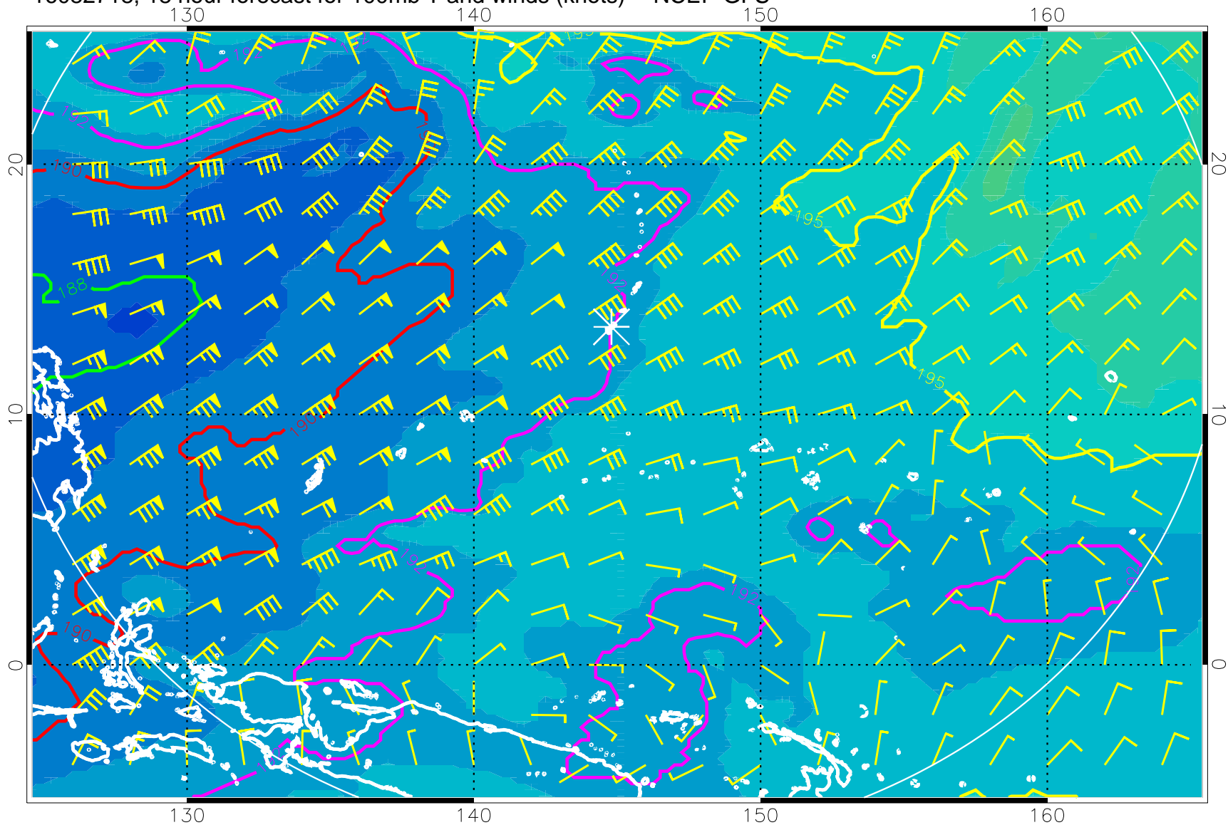
16082718, 18 hour forecast for 100mb T and winds (knots) -- NCEP GFS
