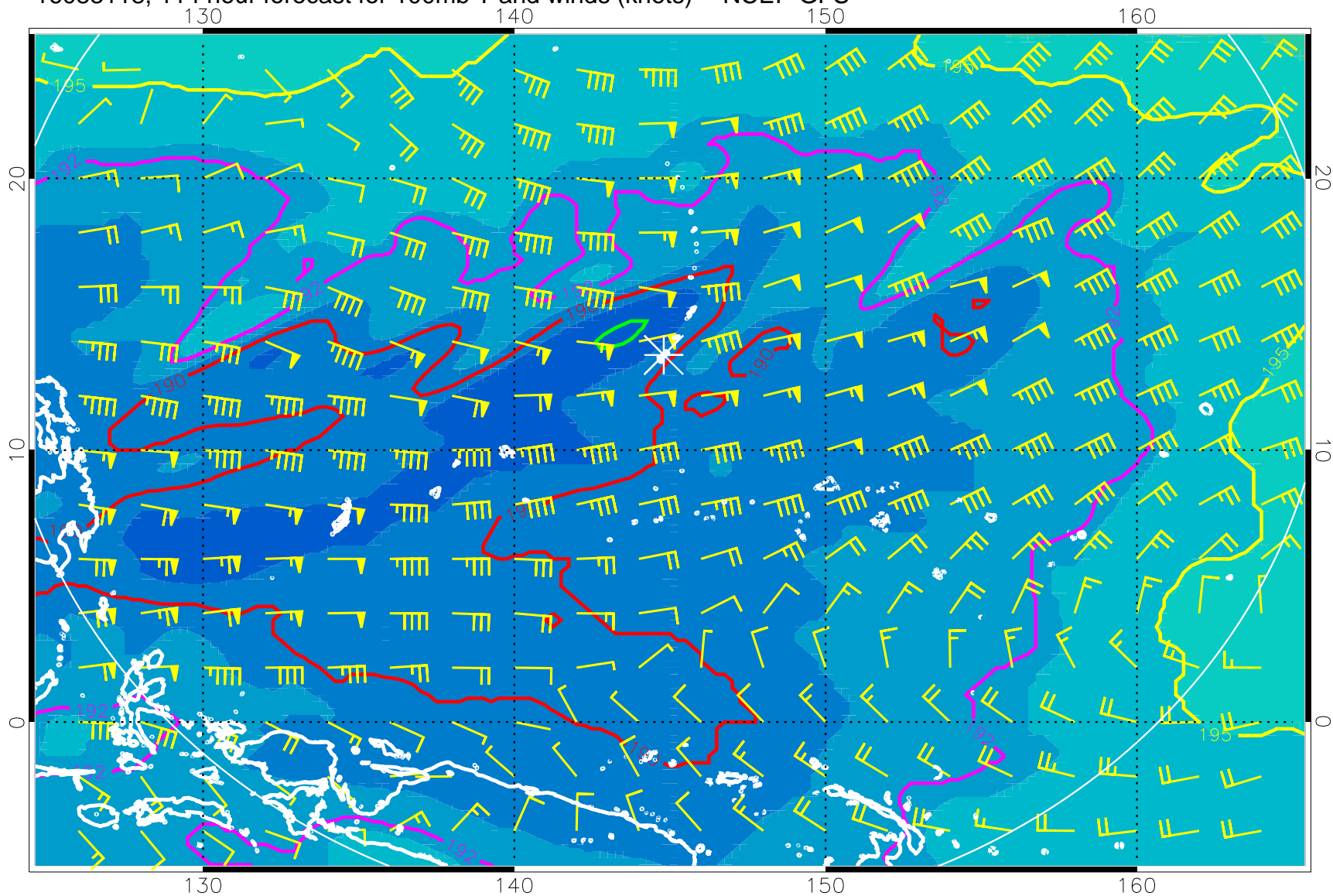
16083118, 114 hour forecast for 100mb T and winds (knots) -- NCEP GFS
