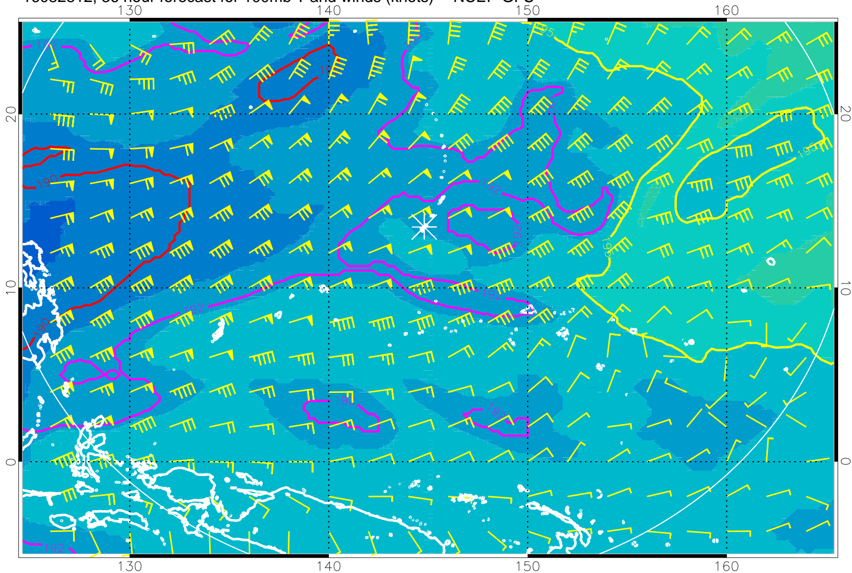
16082812, 36 hour forecast for 100mb T and winds (knots) -- NCEP GFS
