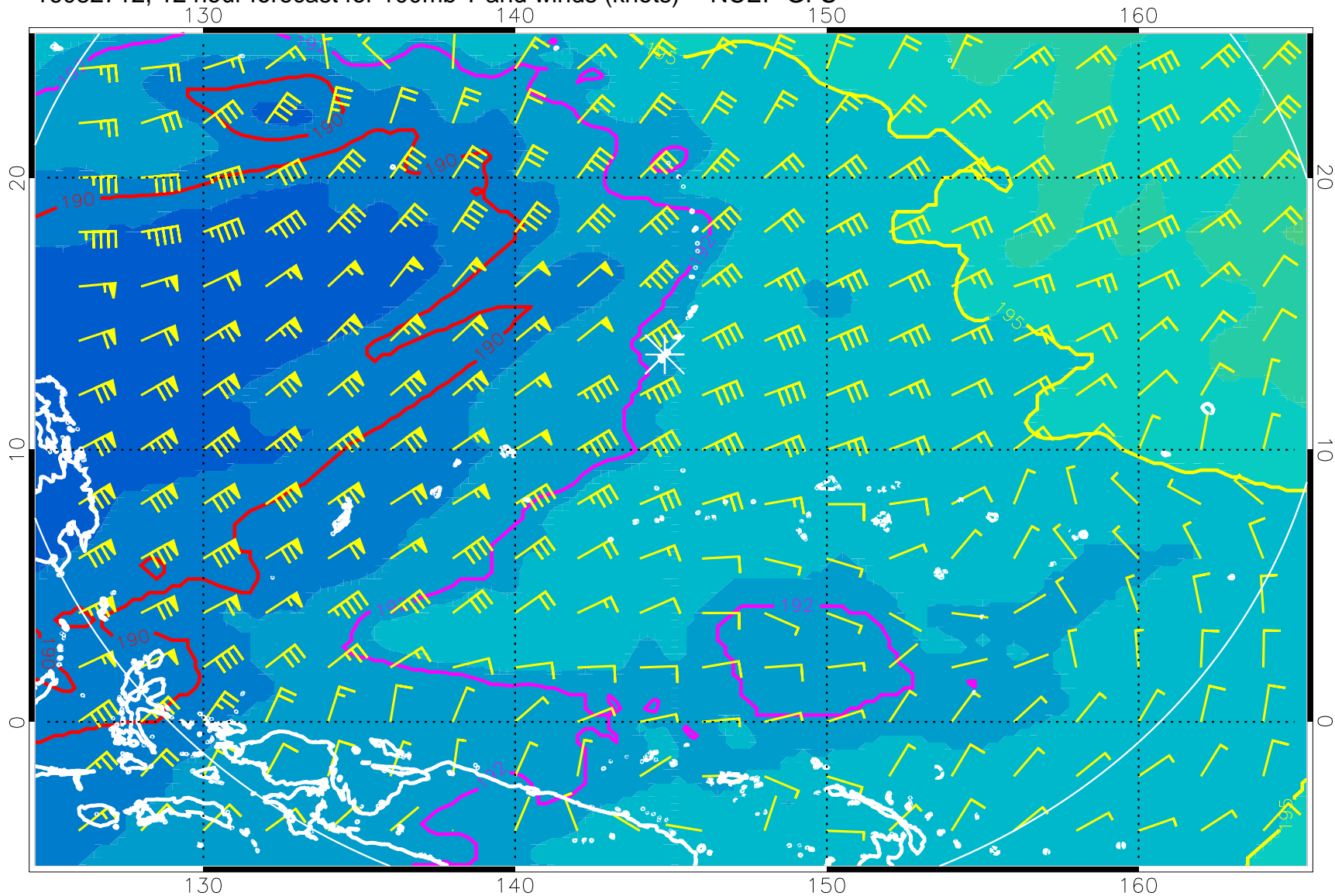
16082712, 12 hour forecast for 100mb T and winds (knots) -- NCEP GFS
