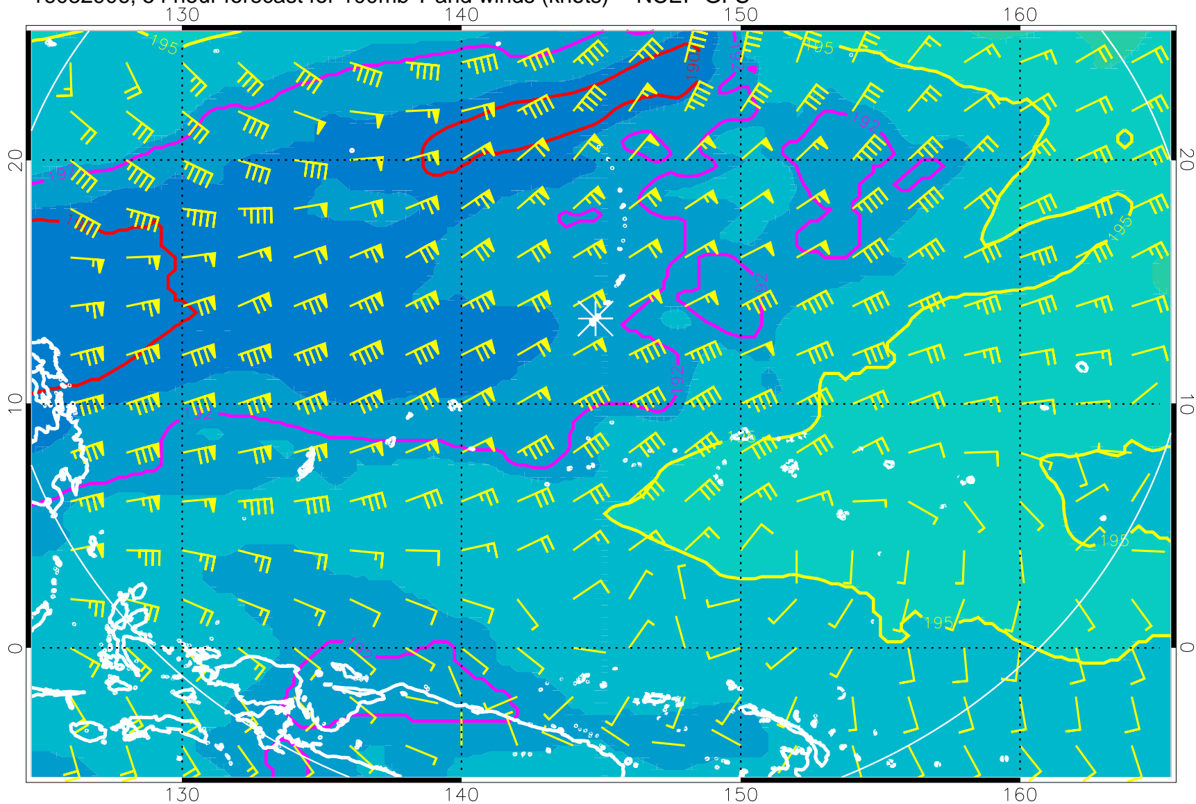
16082906, 54 hour forecast for 100mb T and winds (knots) -- NCEP GFS
