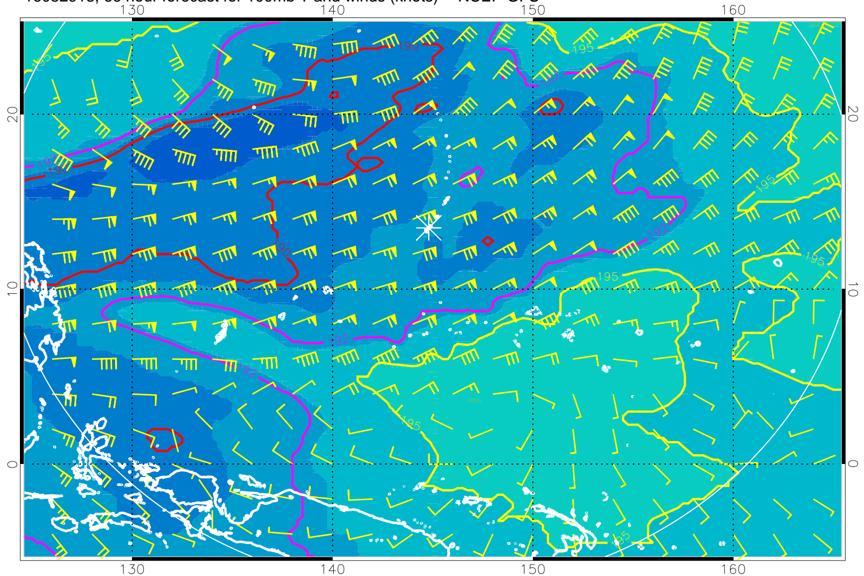
16082918, 66 hour forecast for 100mb T and winds (knots) -- NCEP GFS
