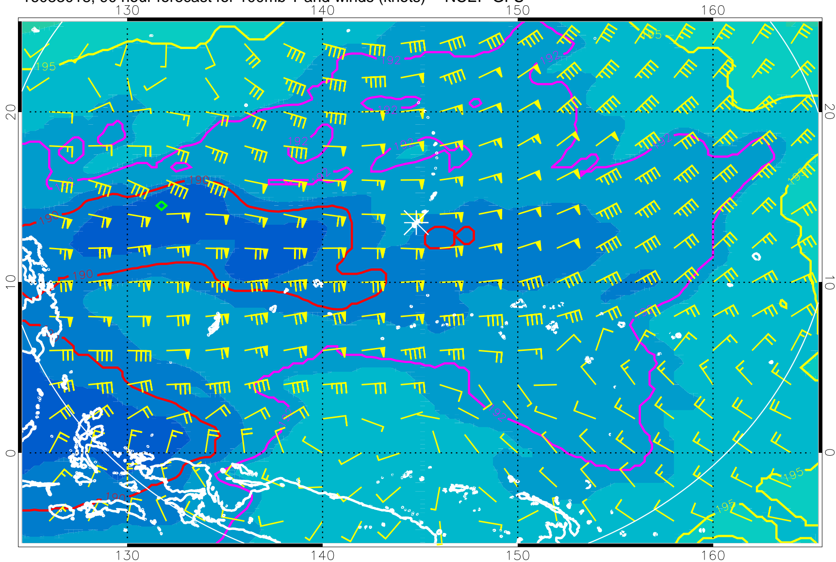
16083018, 90 hour forecast for 100mb T and winds (knots) -- NCEP GFS
