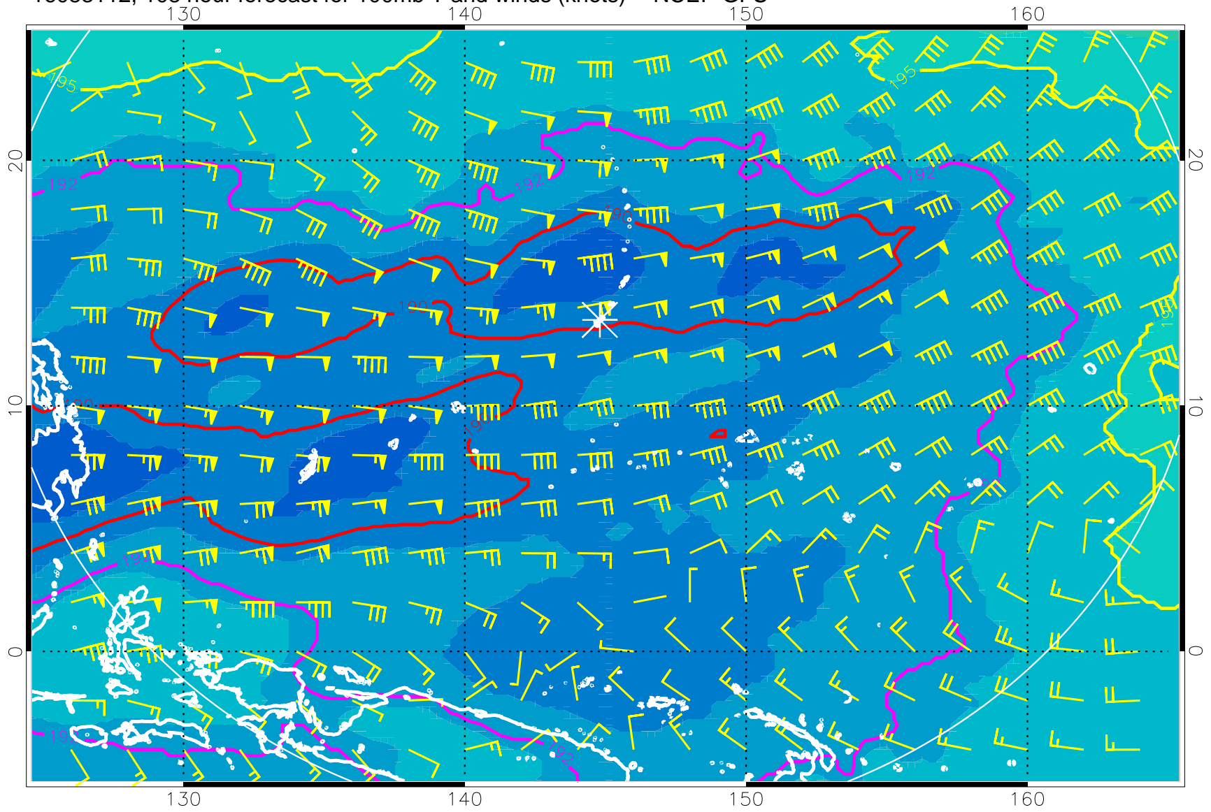
16083112, 108 hour forecast for 100mb T and winds (knots) -- NCEP GFS
