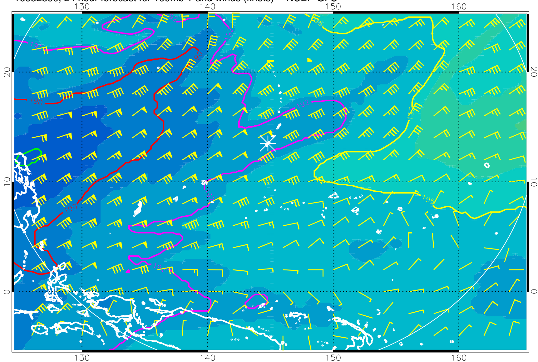
16082800, 24 hour forecast for 100mb T and winds (knots) -- NCEP GFS
