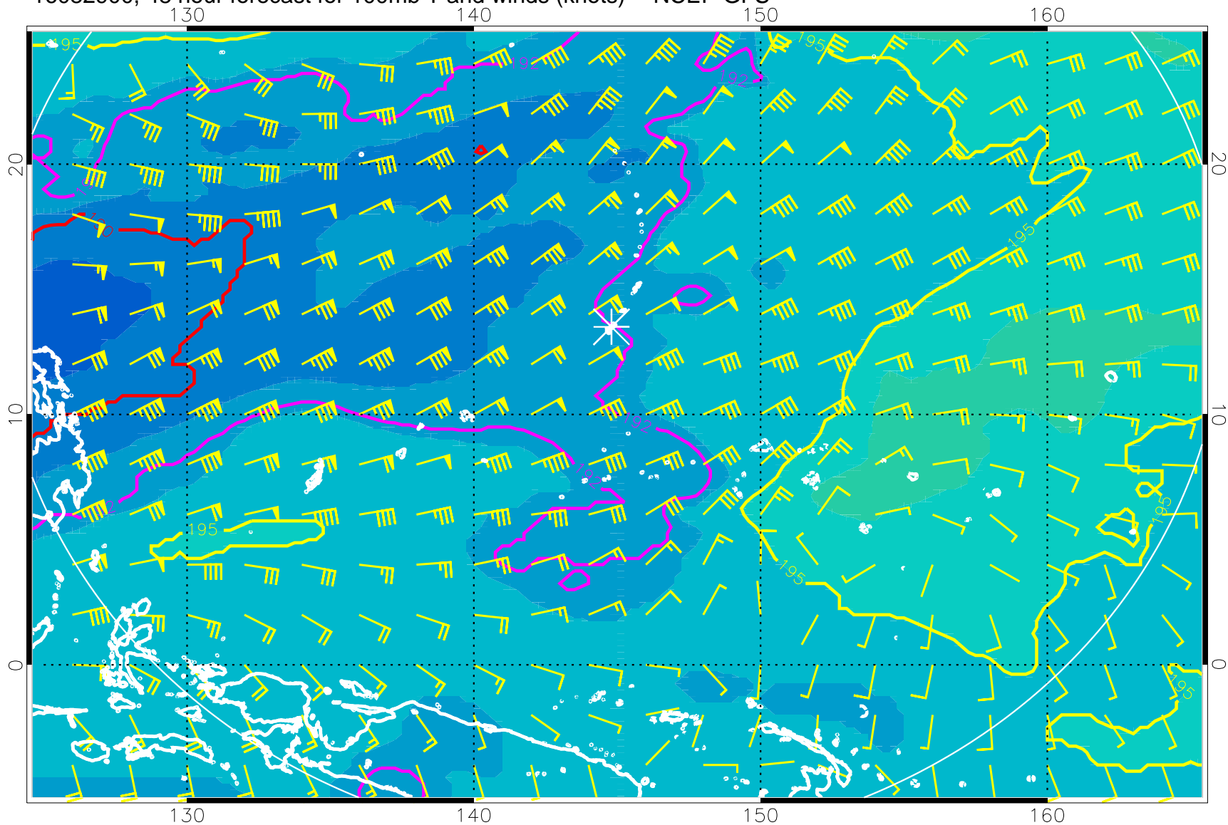
16082900, 48 hour forecast for 100mb T and winds (knots) -- NCEP GFS
