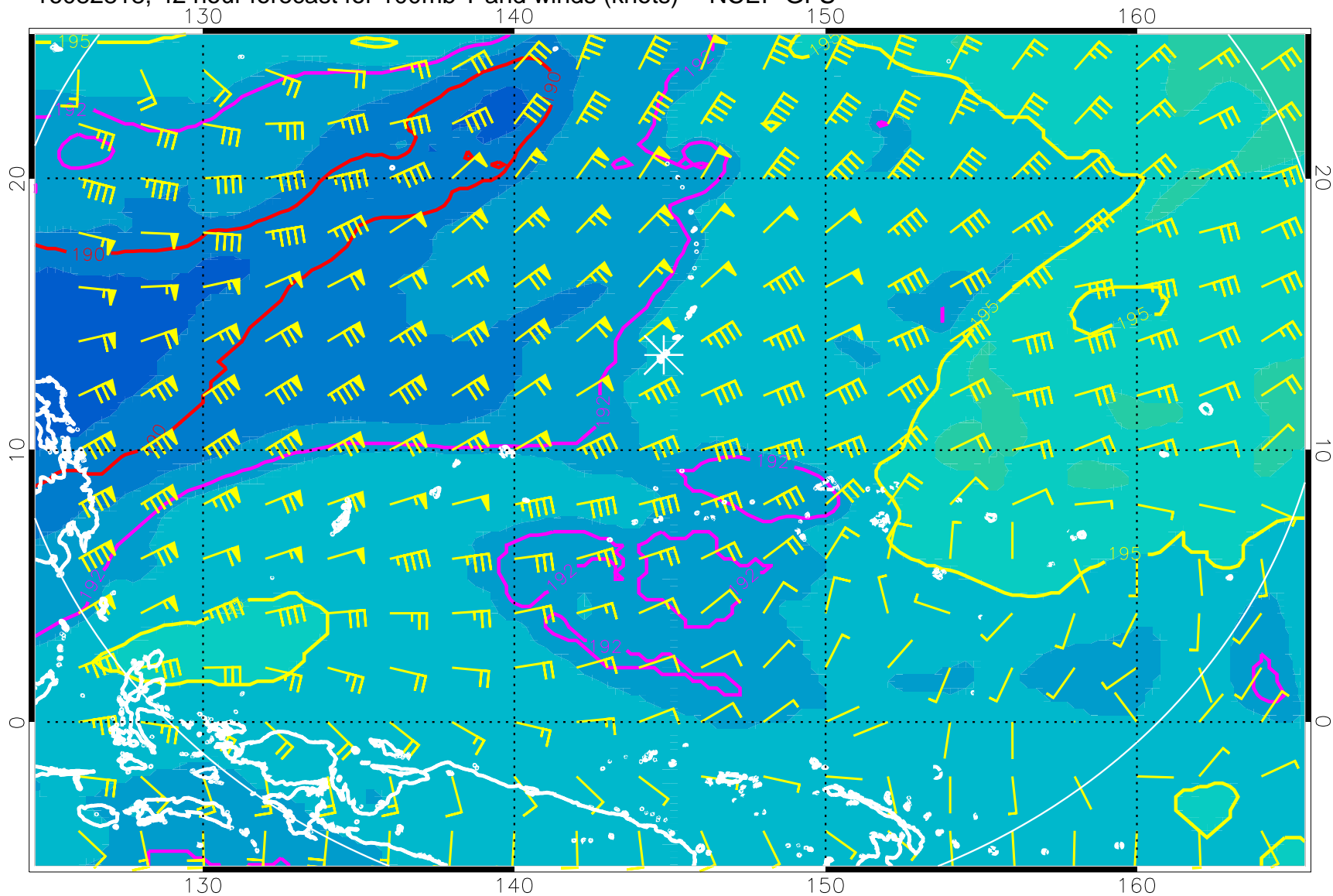
16082818, 42 hour forecast for 100mb T and winds (knots) -- NCEP GFS
