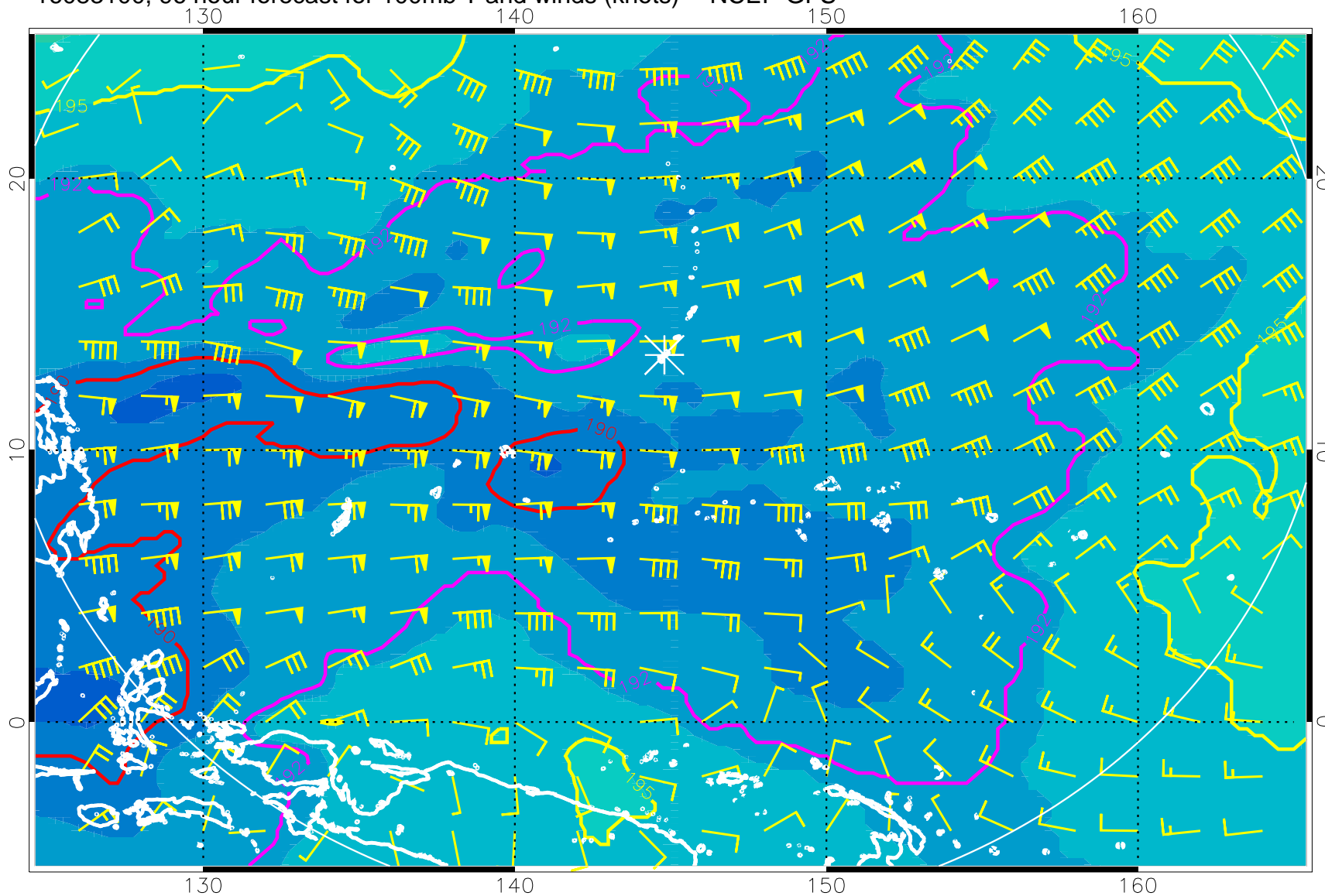
16083100, 96 hour forecast for 100mb T and winds (knots) -- NCEP GFS
