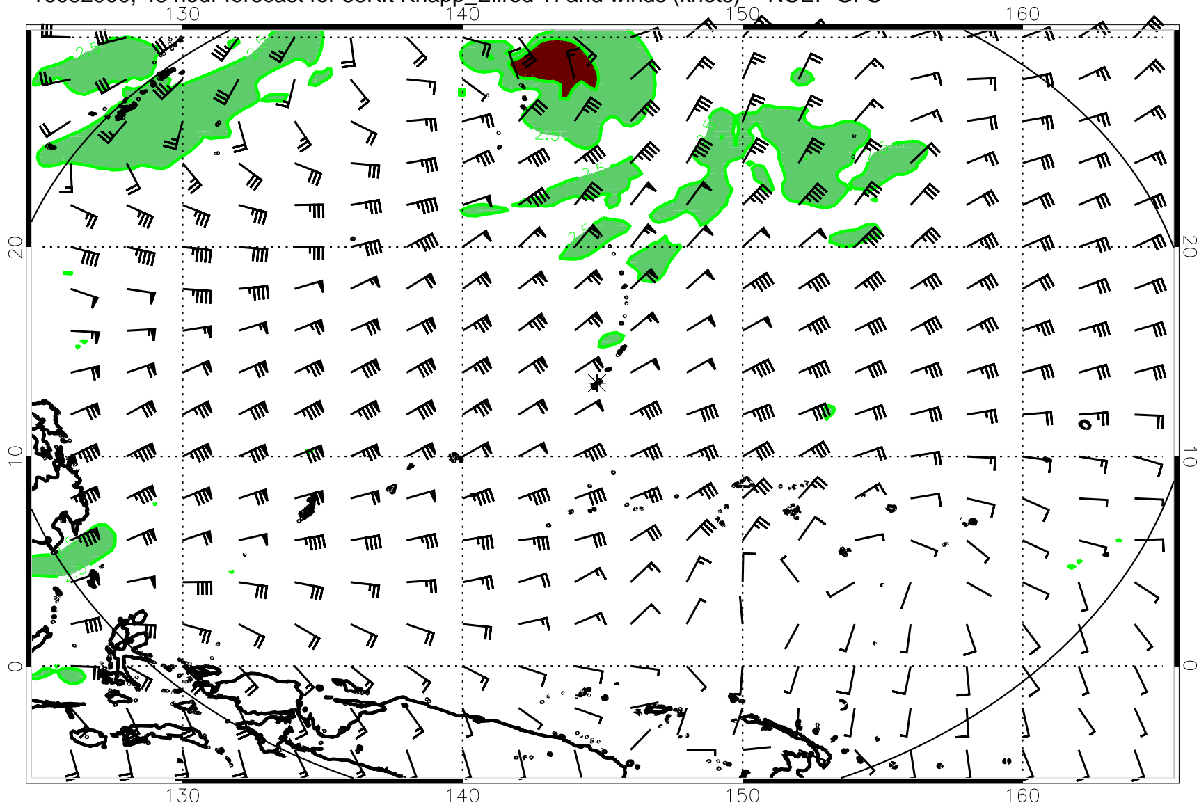
16082900, 48 hour forecast for 53Kft Knapp_Ellrod TI and winds (knots) -- NCEP GFS
