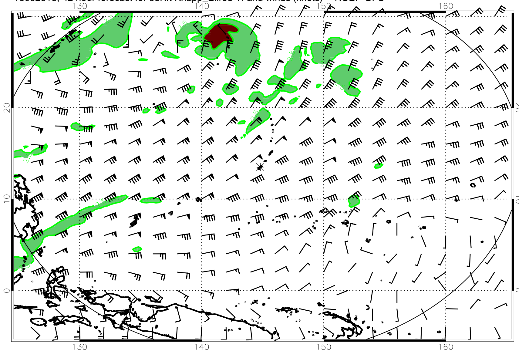
16082818, 42 hour forecast for 53Kft Knapp_Ellrod TI and winds (knots) -- NCEP GFS
