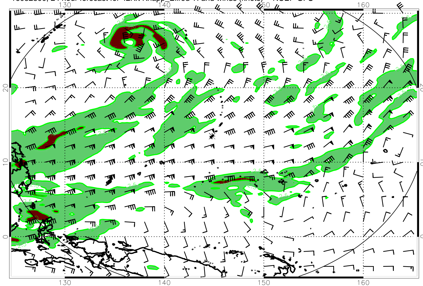
16082800, 24 hour forecast for 42Kft Knapp_Ellrod TI and winds (knots) -- NCEP GFS
