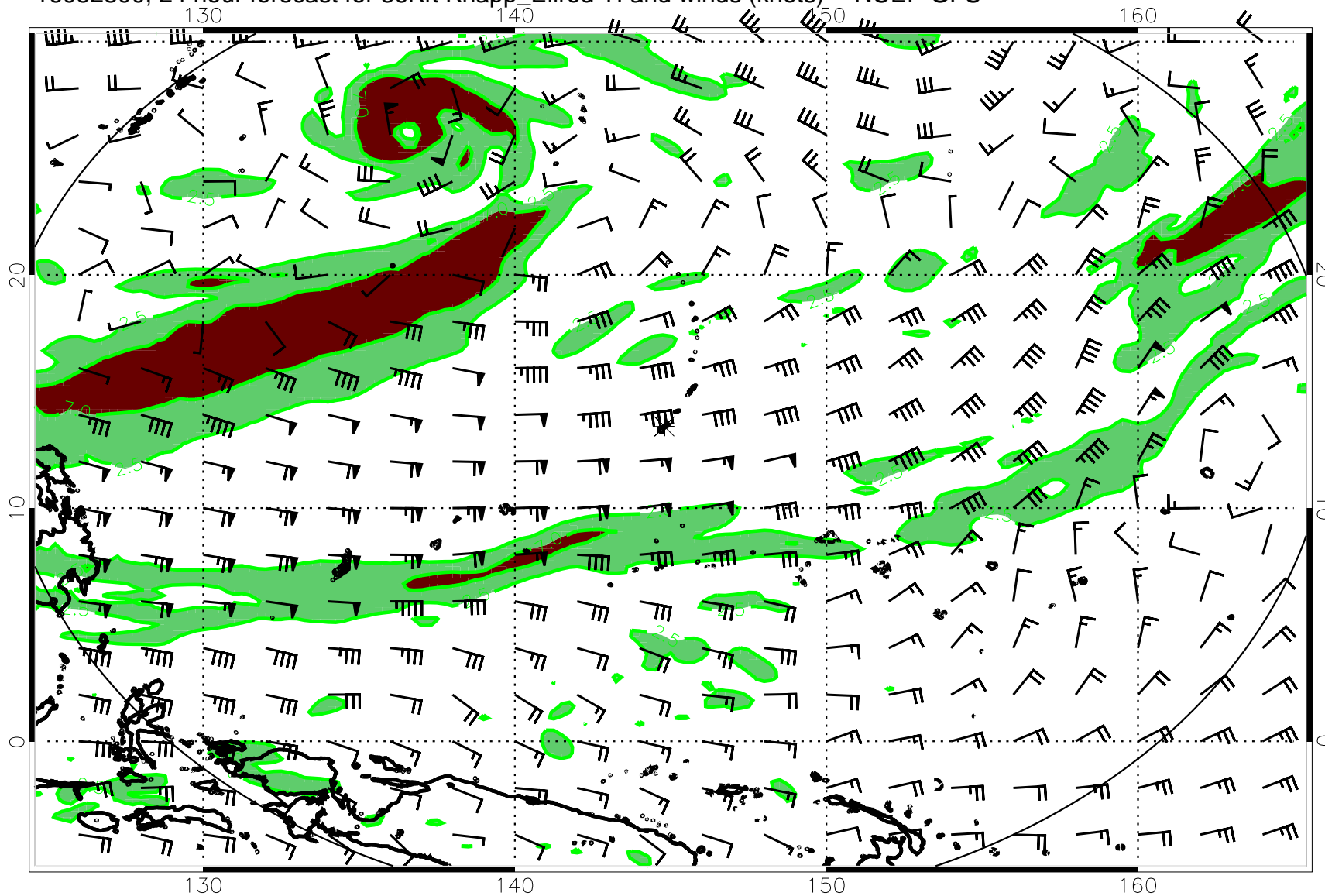
16082800, 24 hour forecast for 36Kft Knapp_Ellrod TI and winds (knots) -- NCEP GFS
