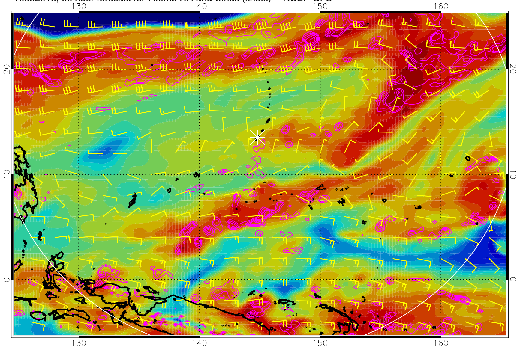
16082918, 66 hour forecast for 700mb RH and winds (knots) -- NCEP GFS
