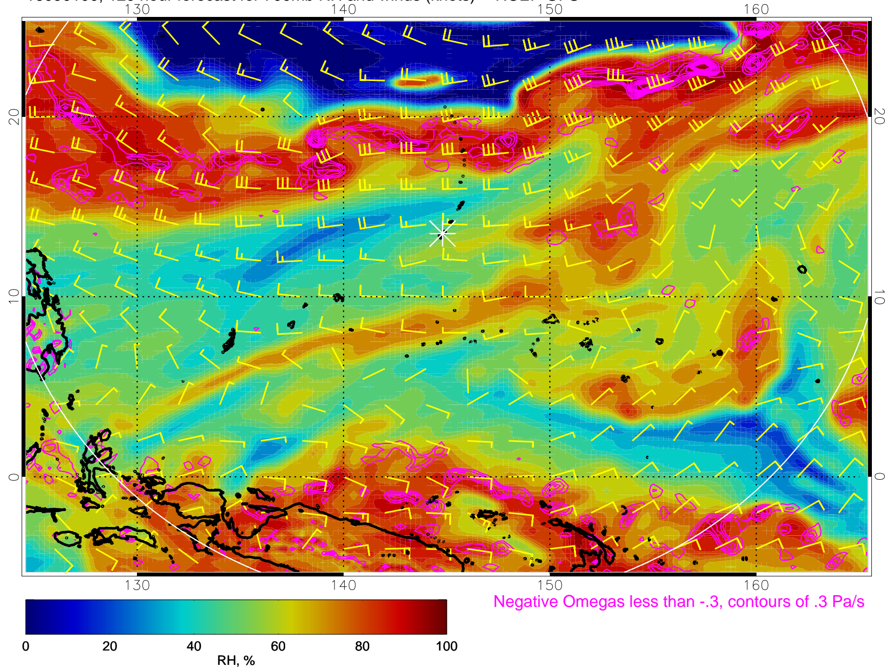
16090100, 120 hour forecast for 700mb RH and winds (knots) -- NCEP GFS
