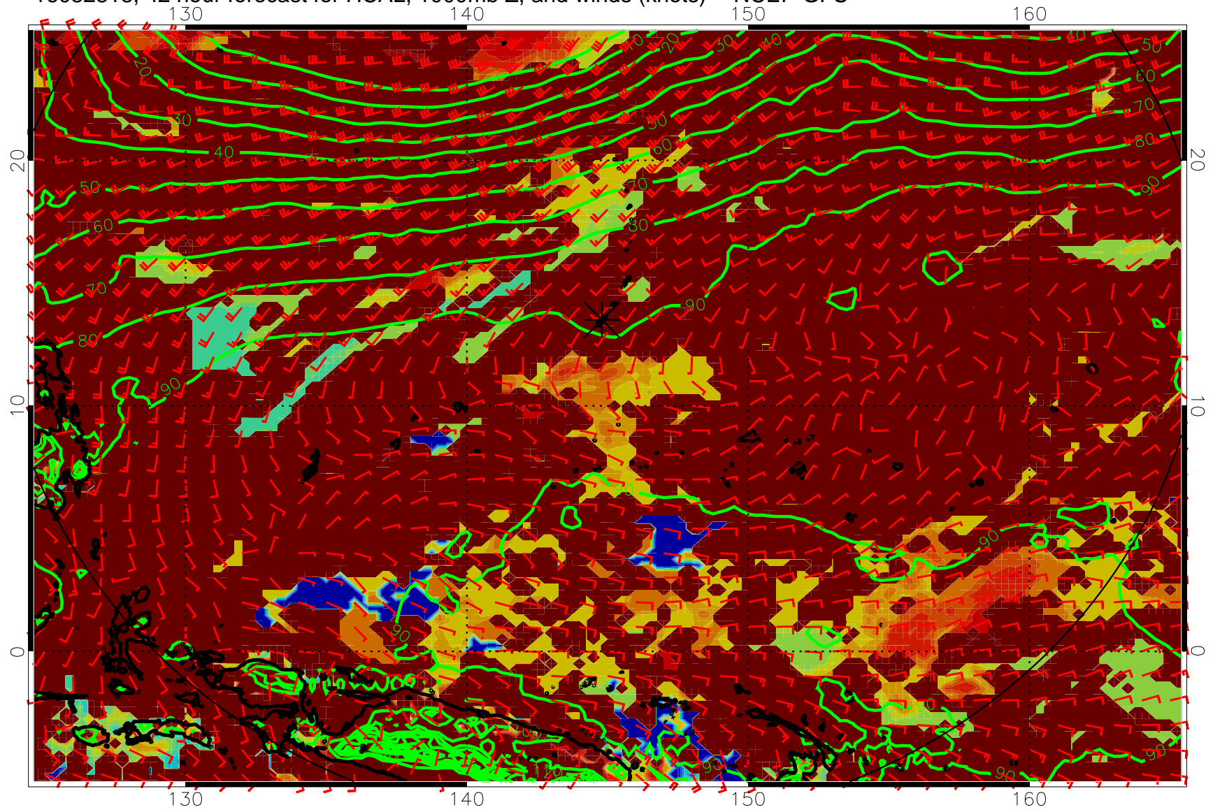
16082818, 42 hour forecast for HCAL, 1000mb Z, and winds (knots) -- NCEP GFS
