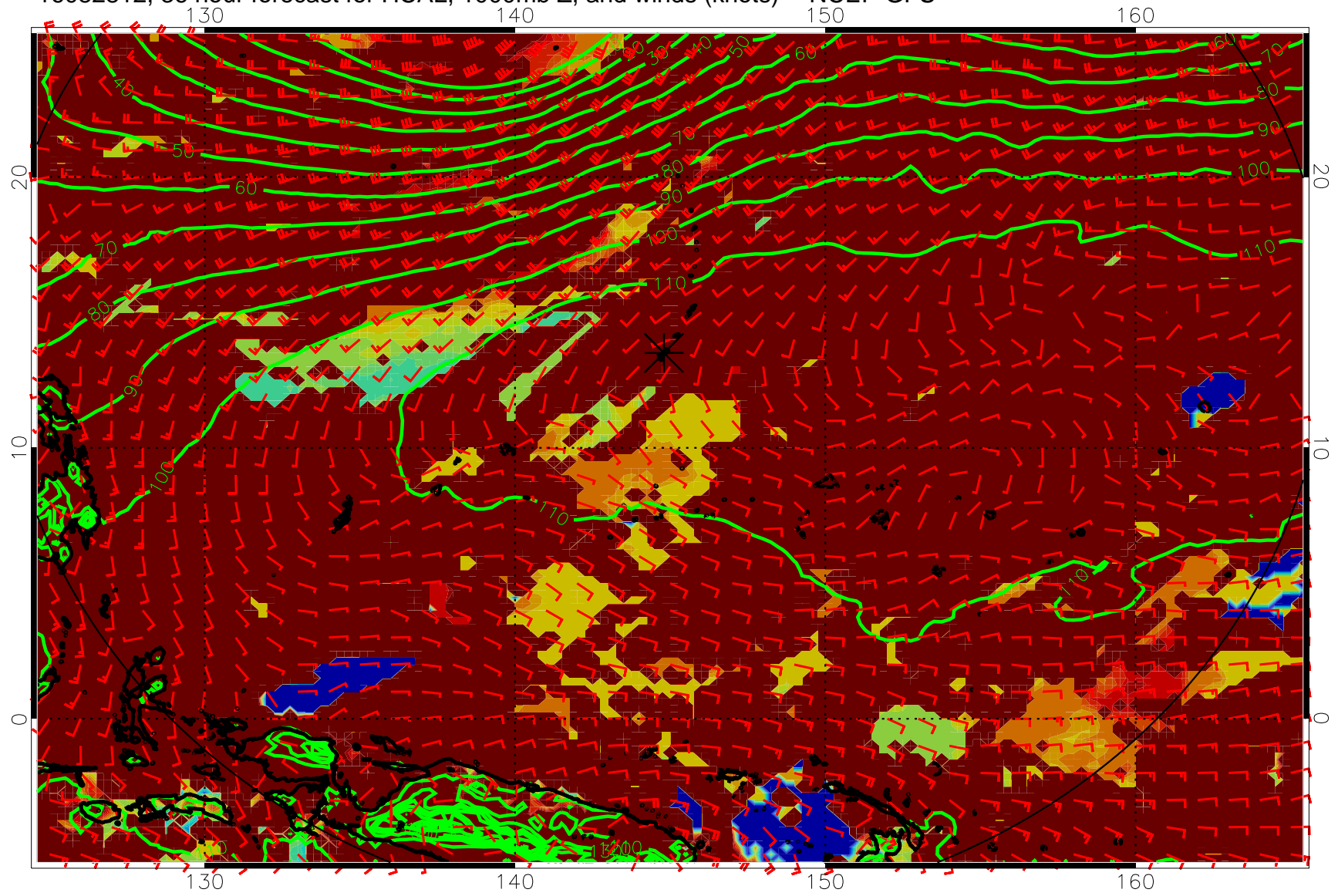
16082812, 36 hour forecast for HCAL, 1000mb Z, and winds (knots) -- NCEP GFS
