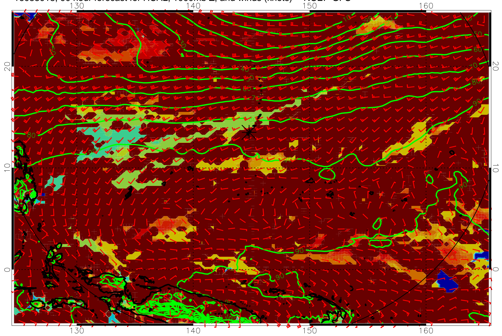
16083018, 90 hour forecast for HCAL, 1000mb Z, and winds (knots) -- NCEP GFS
