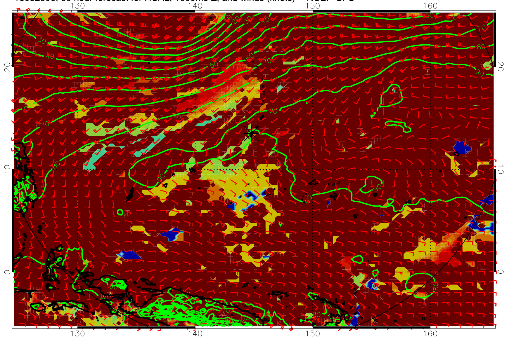
16082806, 30 hour forecast for HCAL, 1000mb Z, and winds (knots) -- NCEP GFS
