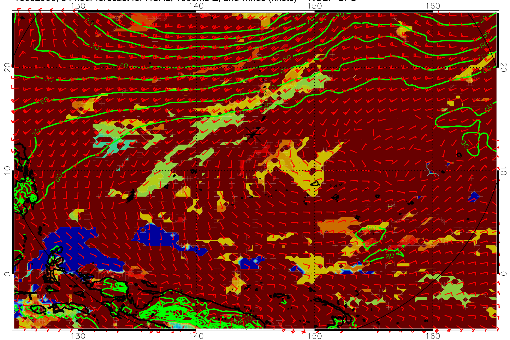
16082906, 54 hour forecast for HCAL, 1000mb Z, and winds (knots) -- NCEP GFS
