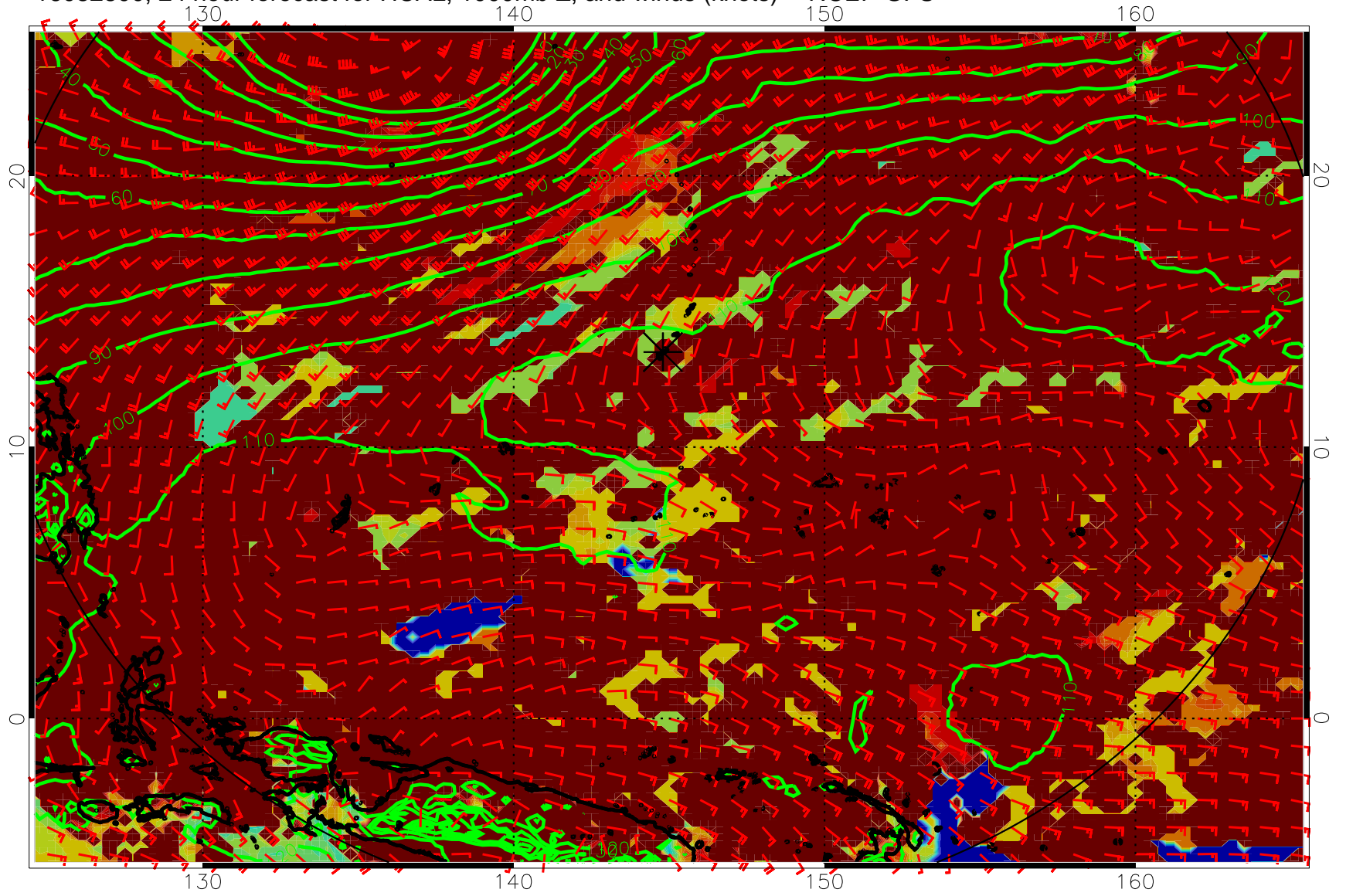
16082800, 24 hour forecast for HCAL, 1000mb Z, and winds (knots) -- NCEP GFS
