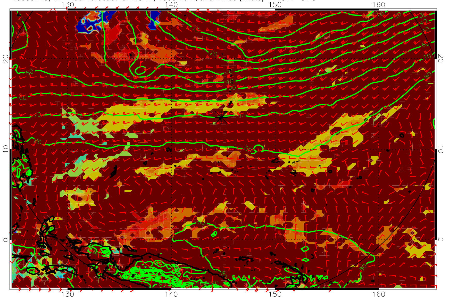
16083118, 114 hour forecast for HCAL, 1000mb Z, and winds (knots) -- NCEP GFS
