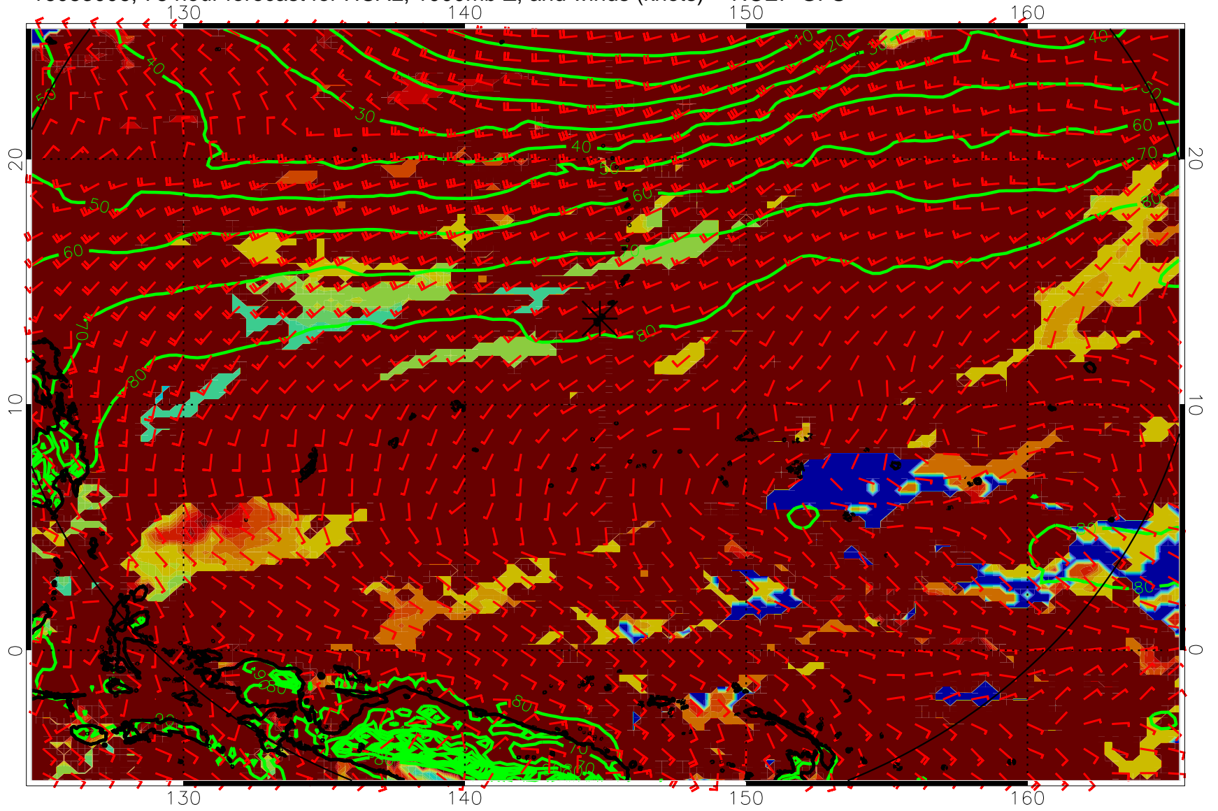
16083006, 78 hour forecast for HCAL, 1000mb Z, and winds (knots) -- NCEP GFS
