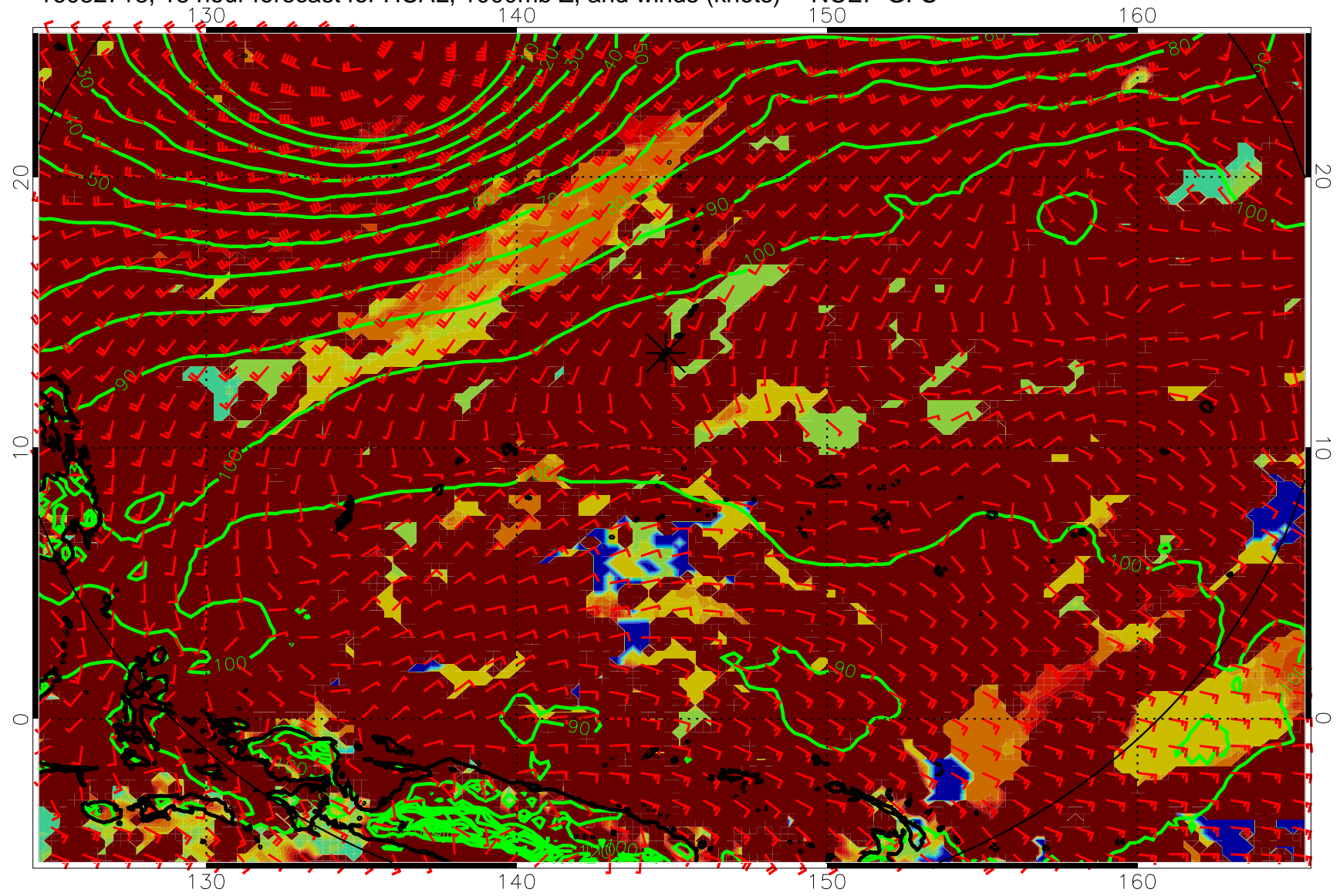
16082718, 18 hour forecast for HCAL, 1000mb Z, and winds (knots) -- NCEP GFS
