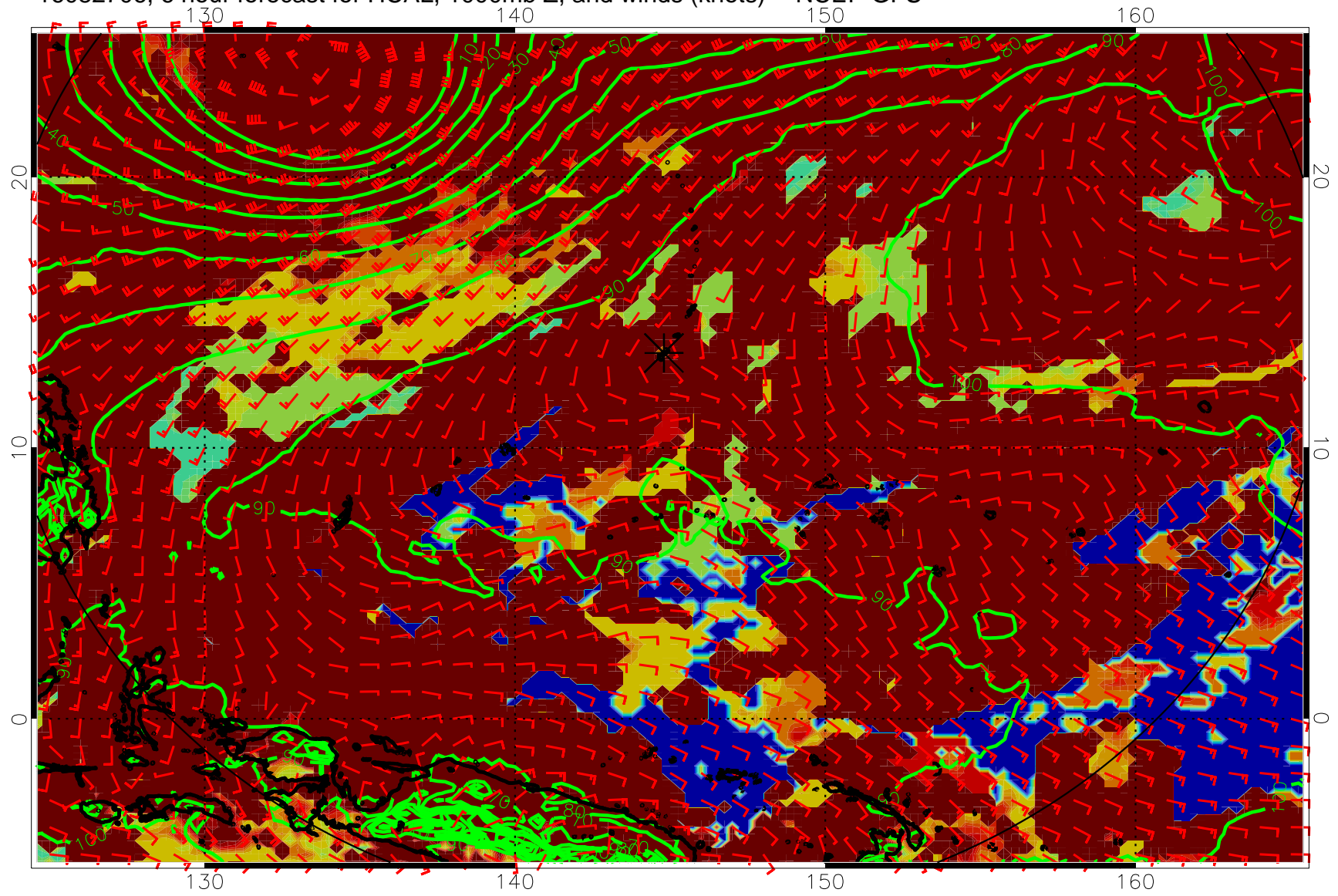
16082706, 6 hour forecast for HCAL, 1000mb Z, and winds (knots) -- NCEP GFS
