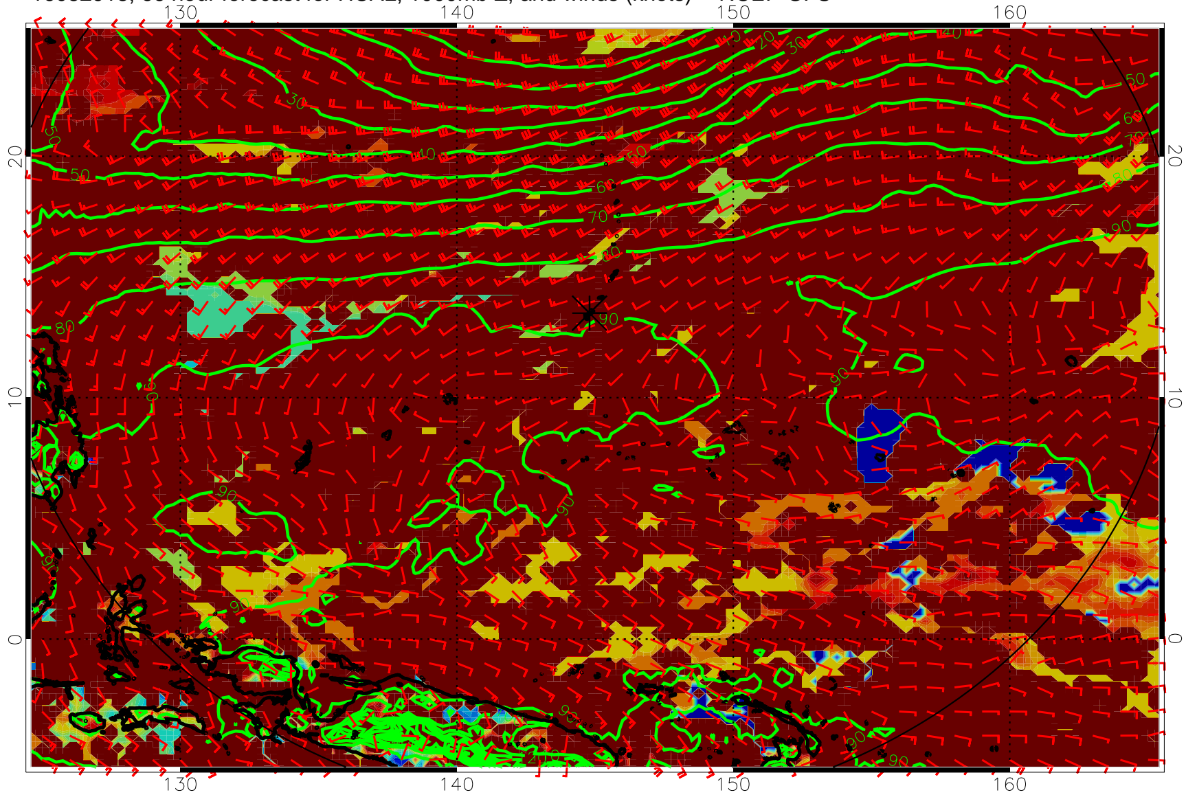
16082918, 66 hour forecast for HCAL, 1000mb Z, and winds (knots) -- NCEP GFS
