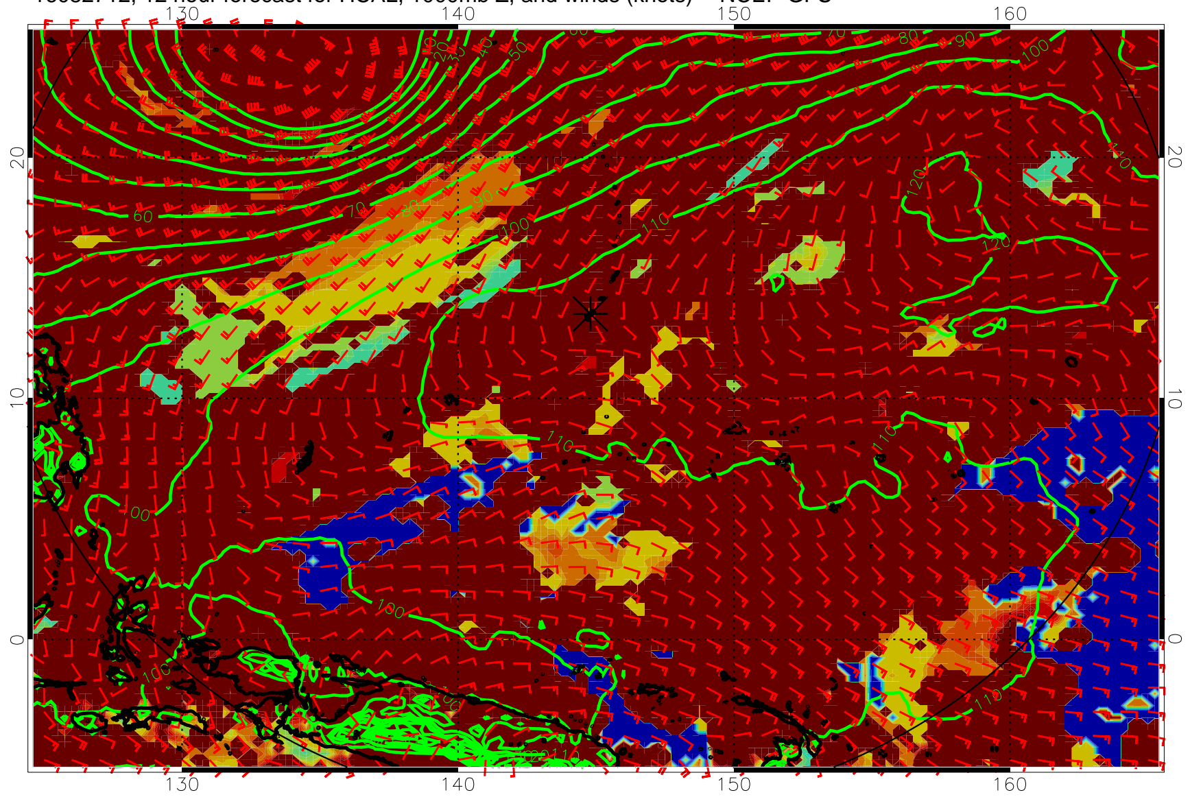
16082712, 12 hour forecast for HCAL, 1000mb Z, and winds (knots) -- NCEP GFS
