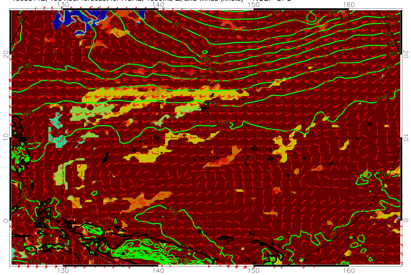
16083112, 108 hour forecast for HCAL, 1000mb Z, and winds (knots) -- NCEP GFS
