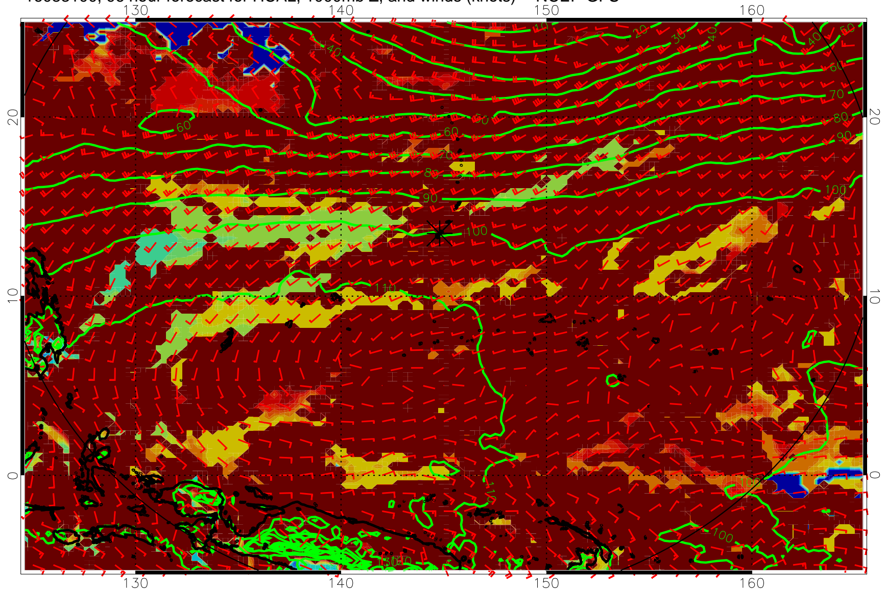
16083100, 96 hour forecast for HCAL, 1000mb Z, and winds (knots) -- NCEP GFS
