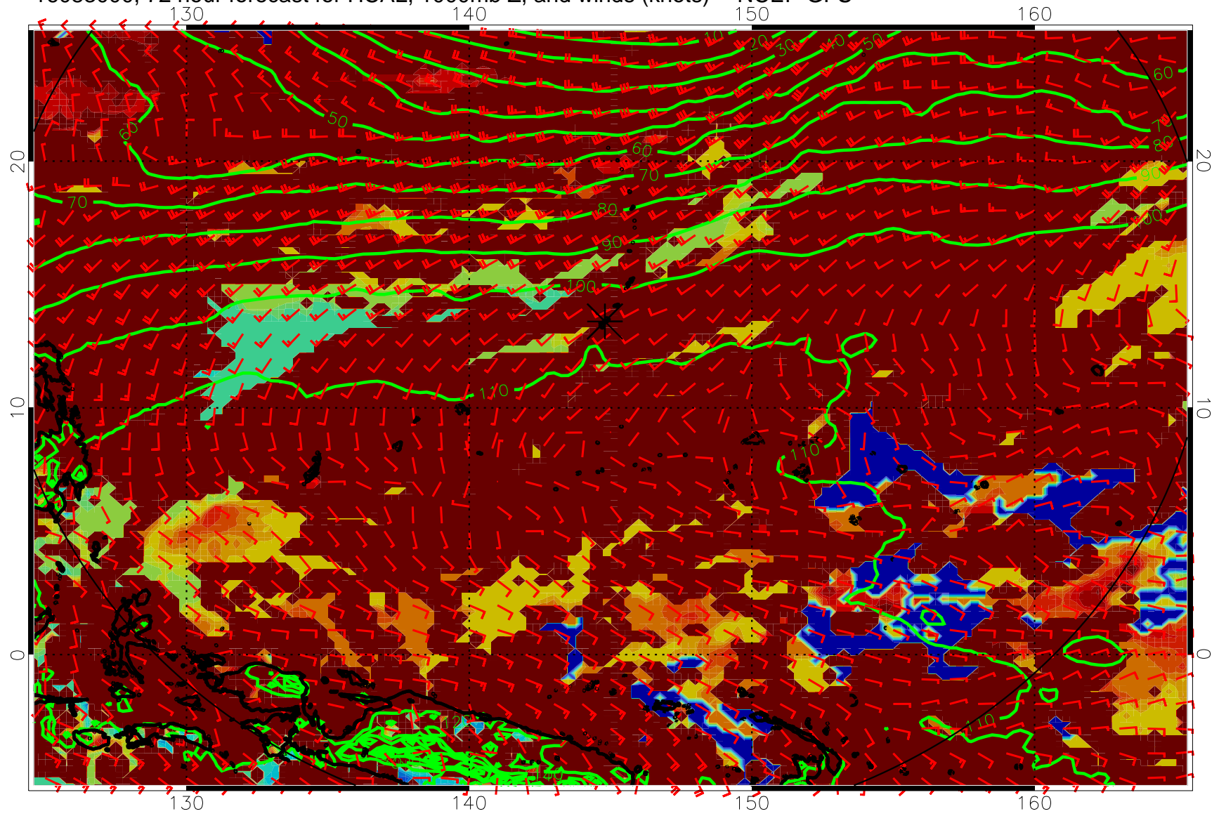
16083000, 72 hour forecast for HCAL, 1000mb Z, and winds (knots) -- NCEP GFS
