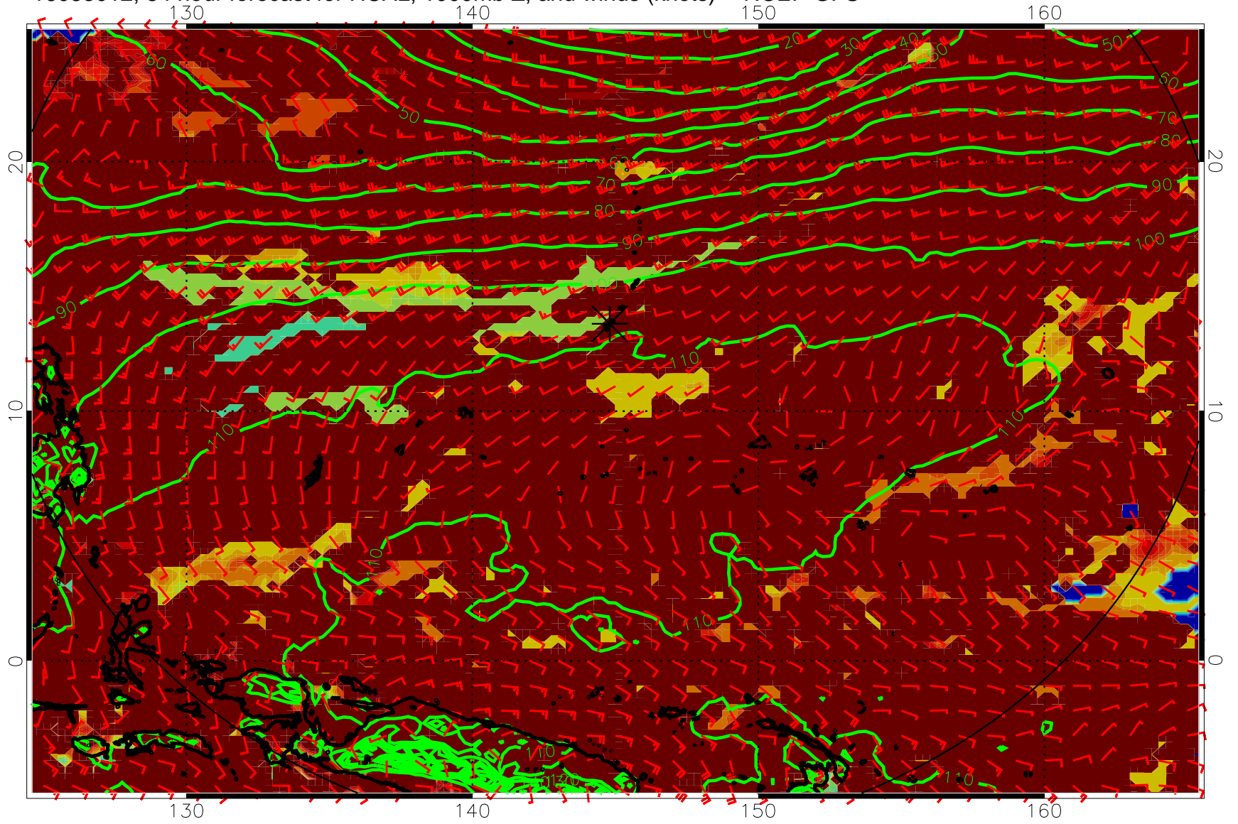
16083012, 84 hour forecast for HCAL, 1000mb Z, and winds (knots) -- NCEP GFS
