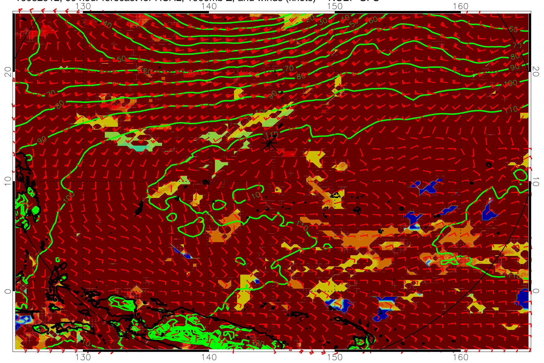
16082912, 60 hour forecast for HCAL, 1000mb Z, and winds (knots) -- NCEP GFS
