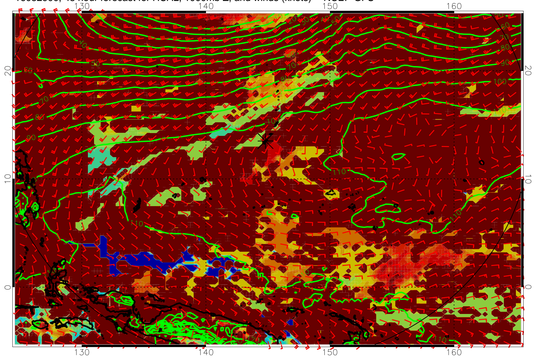
16082900, 48 hour forecast for HCAL, 1000mb Z, and winds (knots) -- NCEP GFS
