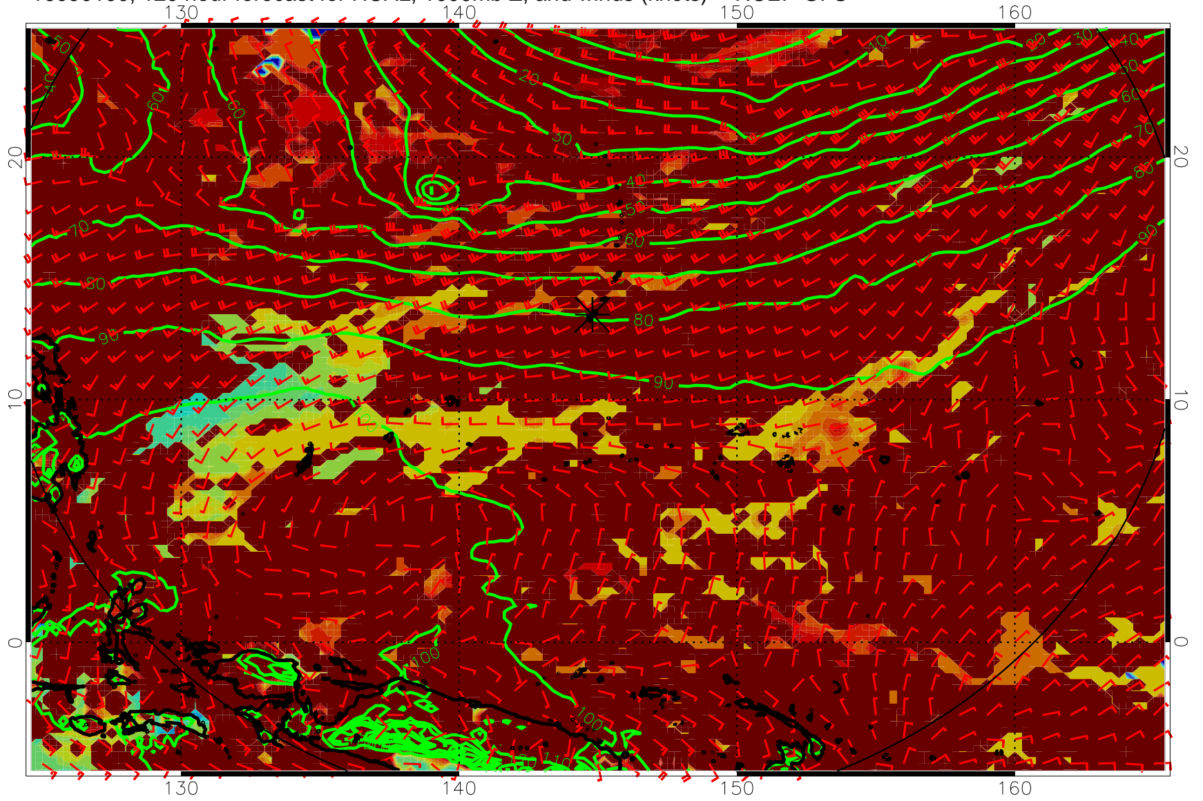
16090100, 120 hour forecast for HCAL, 1000mb Z, and winds (knots) -- NCEP GFS
