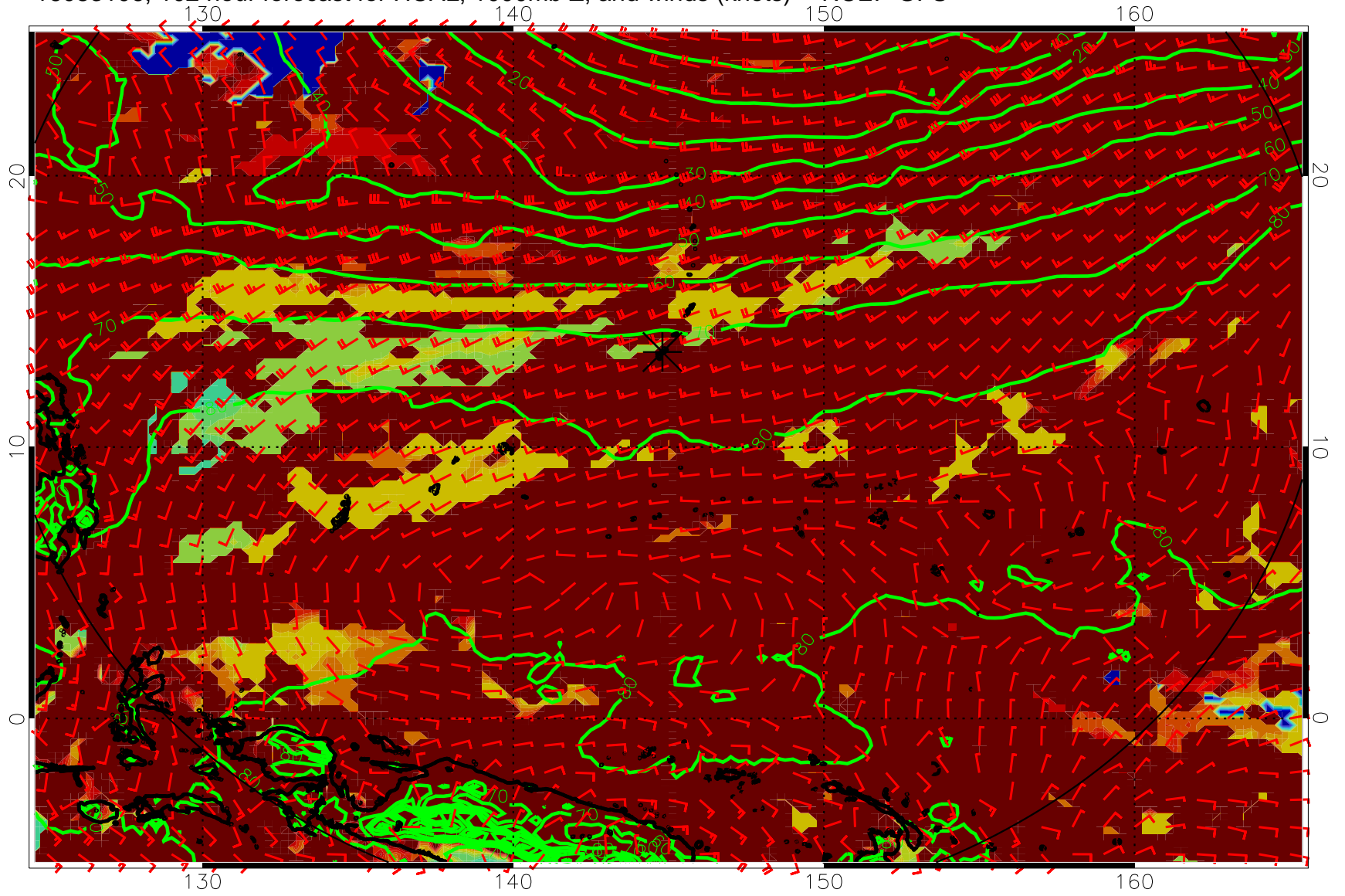
16083106, 102 hour forecast for HCAL, 1000mb Z, and winds (knots) -- NCEP GFS
