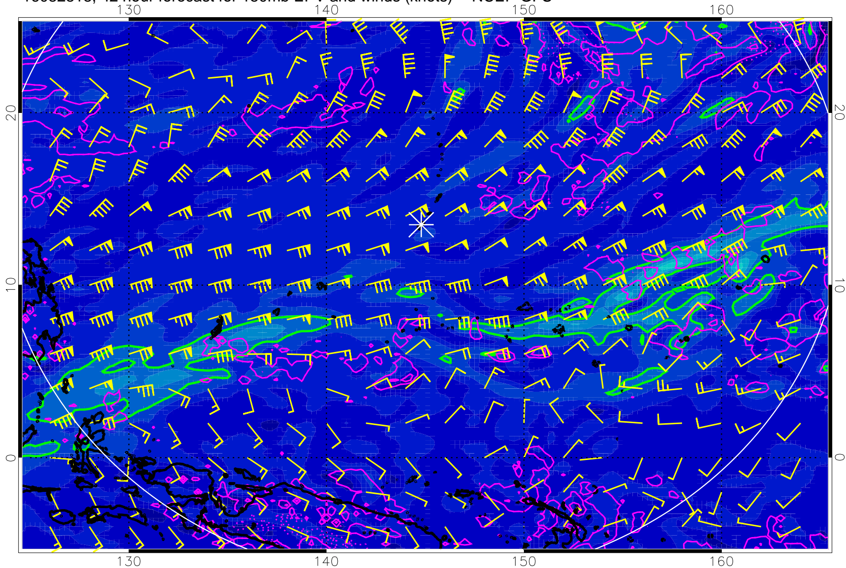
16082818, 42 hour forecast for 150mb EPV and winds (knots) -- NCEP GFS
