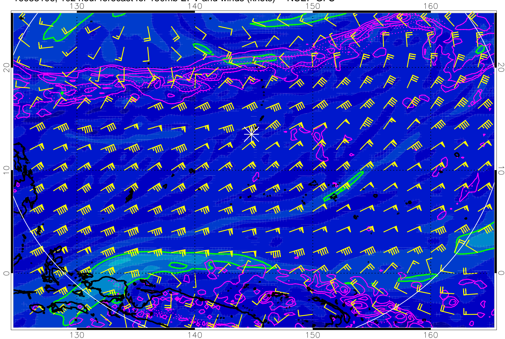
16083106, 102 hour forecast for 150mb EPV and winds (knots) -- NCEP GFS
