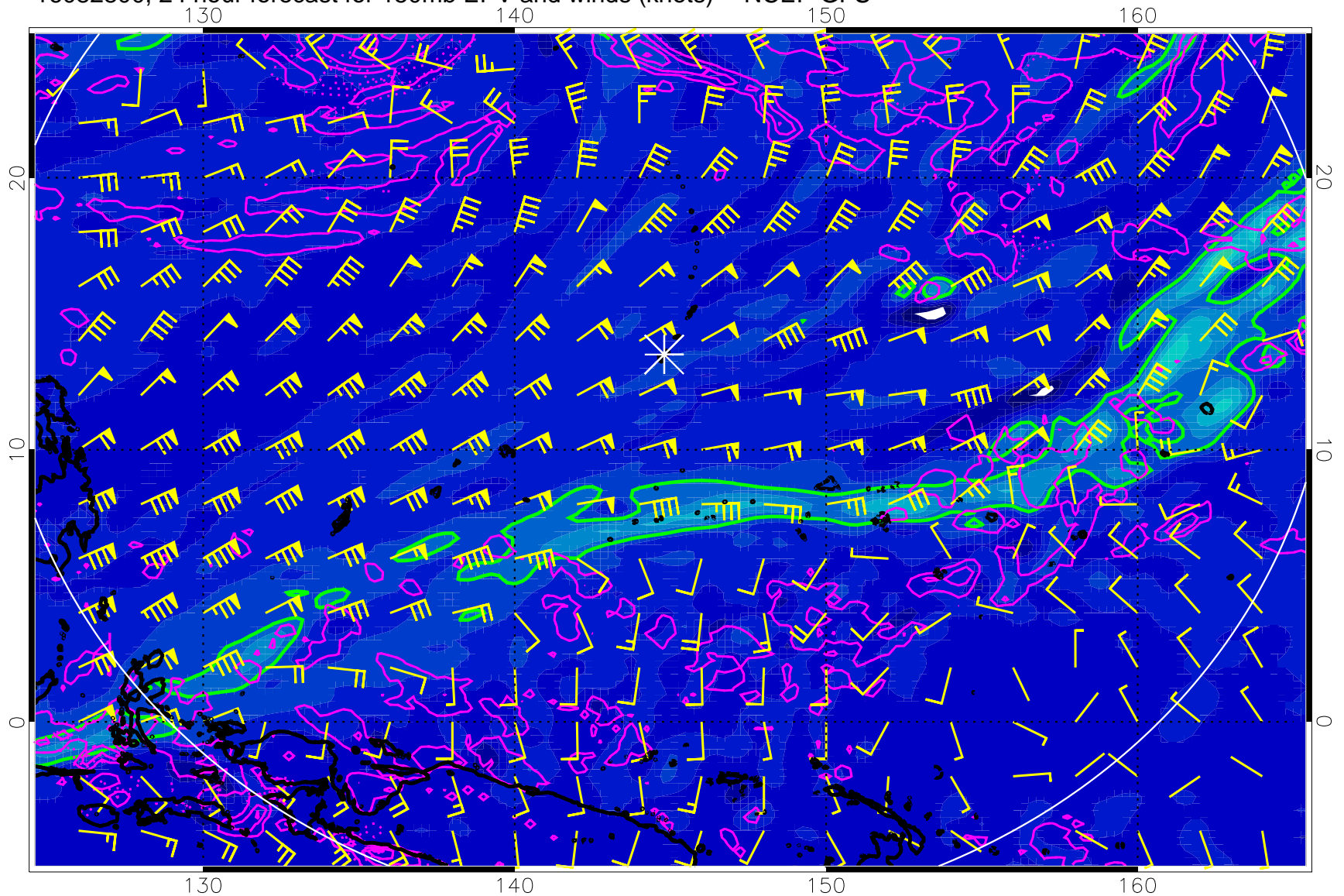
16082800, 24 hour forecast for 150mb EPV and winds (knots) -- NCEP GFS
