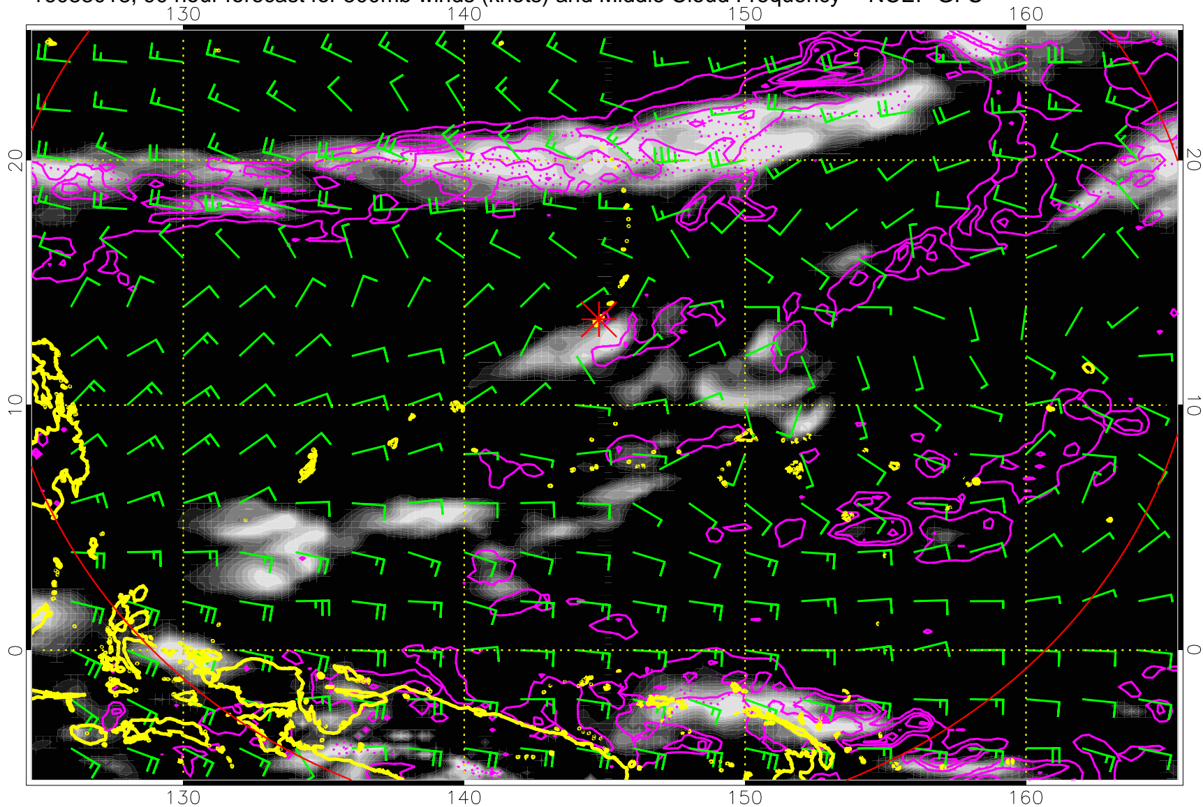
16083018, 90 hour forecast for 500mb winds (knots) and Middle Cloud Frequency -- NCEP GFS
