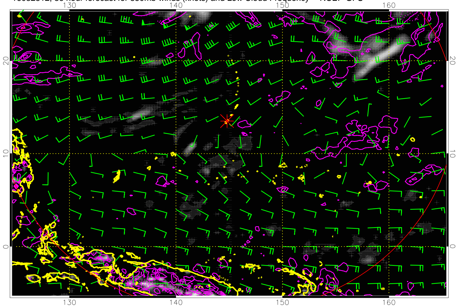
16082812, 36 hour forecast for 850mb winds (knots) and Low Cloud Frequency -- NCEP GFS
