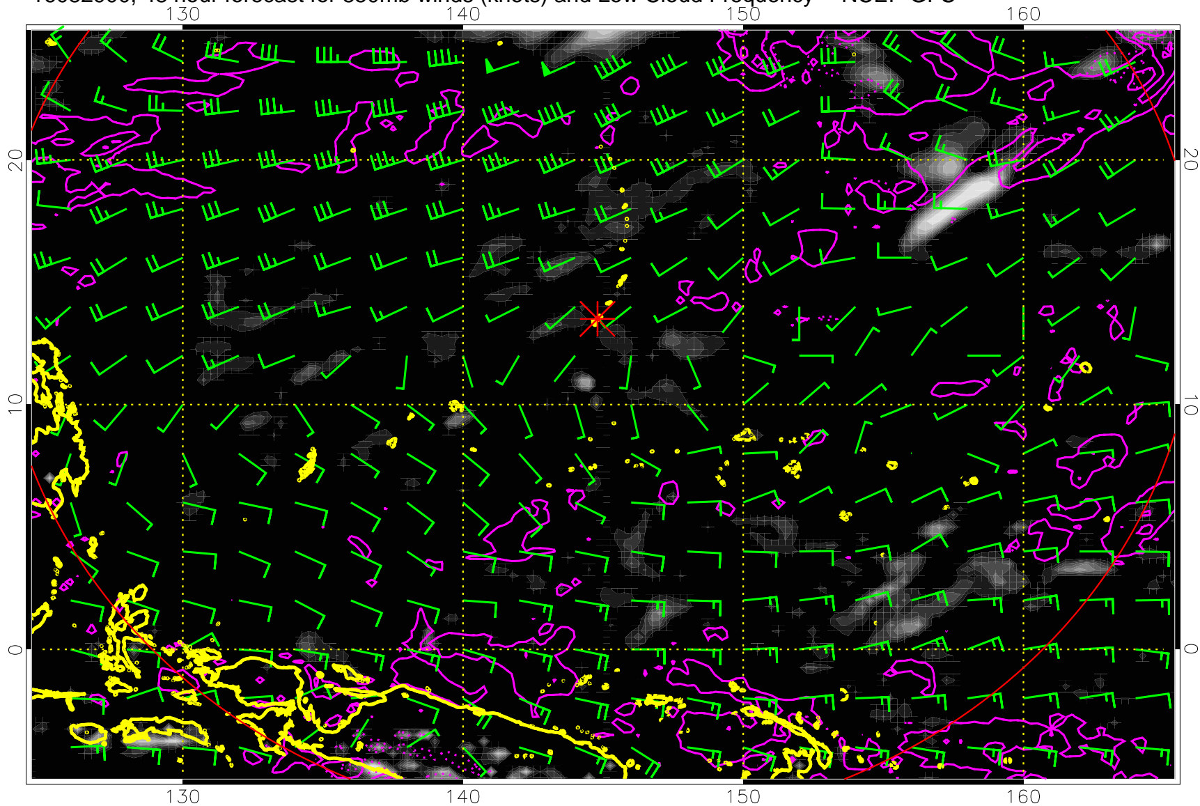
16082900, 48 hour forecast for 850mb winds (knots) and Low Cloud Frequency -- NCEP GFS
