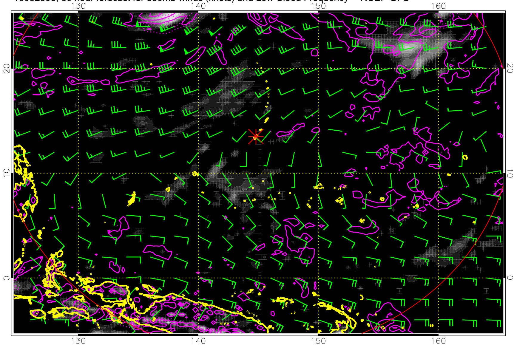
16082806, 30 hour forecast for 850mb winds (knots) and Low Cloud Frequency -- NCEP GFS
