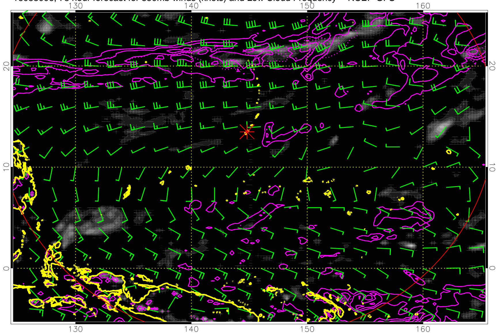
16083006, 78 hour forecast for 850mb winds (knots) and Low Cloud Frequency -- NCEP GFS
