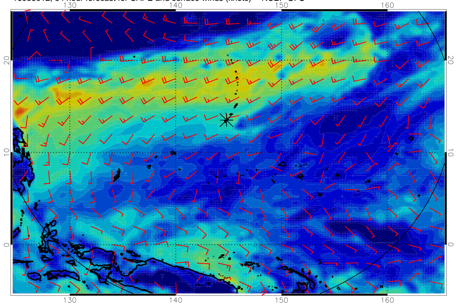
16083012, 84 hour forecast for CAPE and surface winds (knots) -- NCEP GFS
