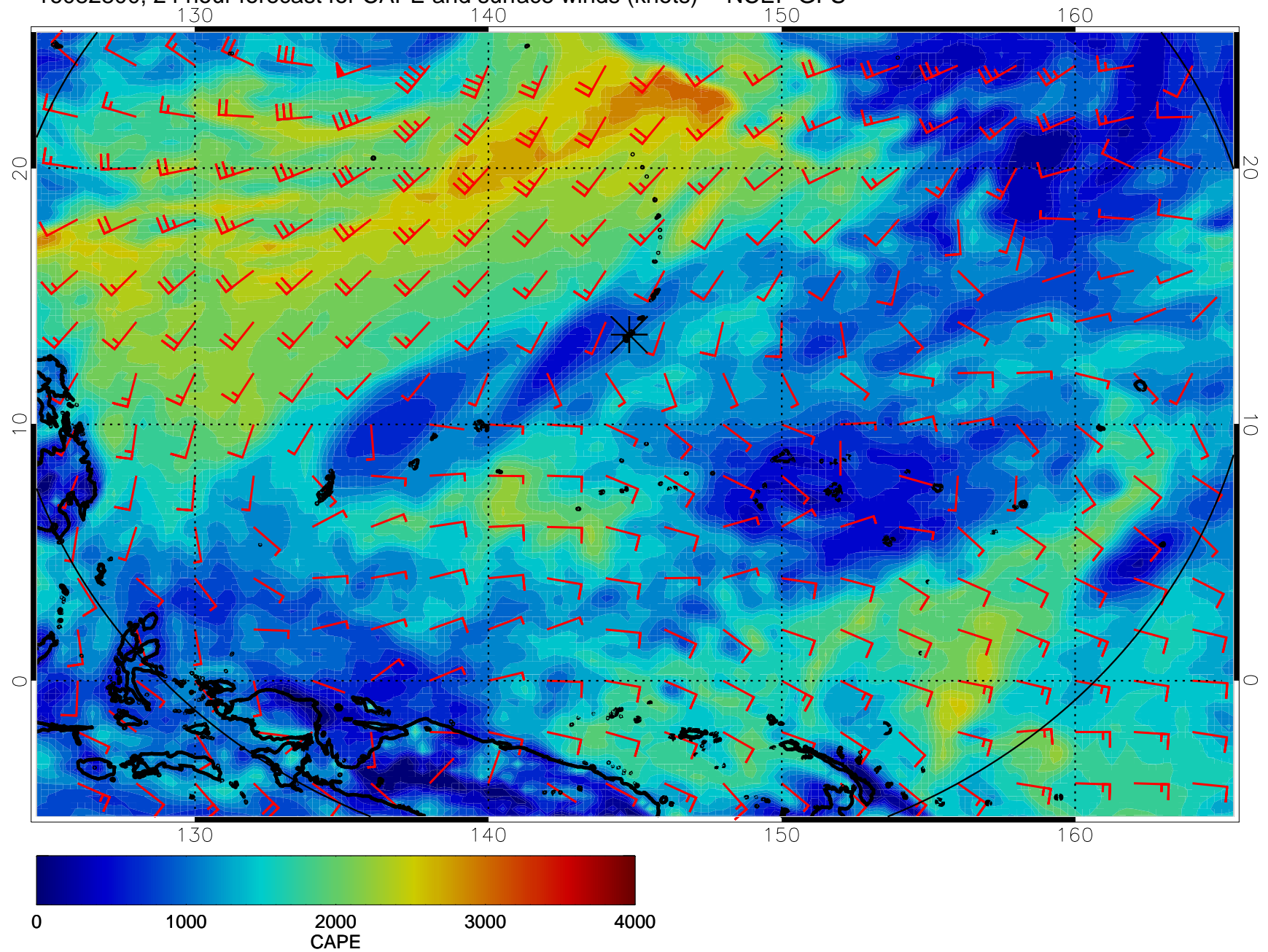
16082800, 24 hour forecast for CAPE and surface winds (knots) -- NCEP GFS
