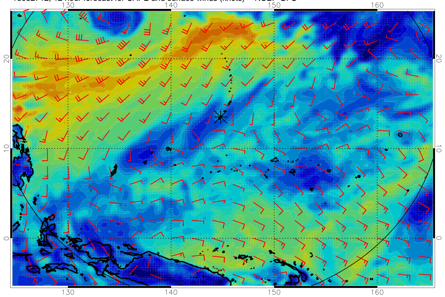
16082712, 12 hour forecast for CAPE and surface winds (knots) -- NCEP GFS
