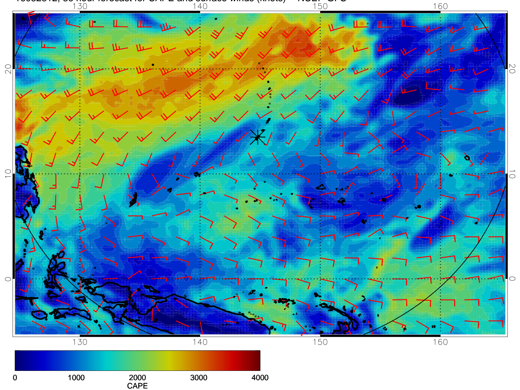
16082812, 36 hour forecast for CAPE and surface winds (knots) -- NCEP GFS
