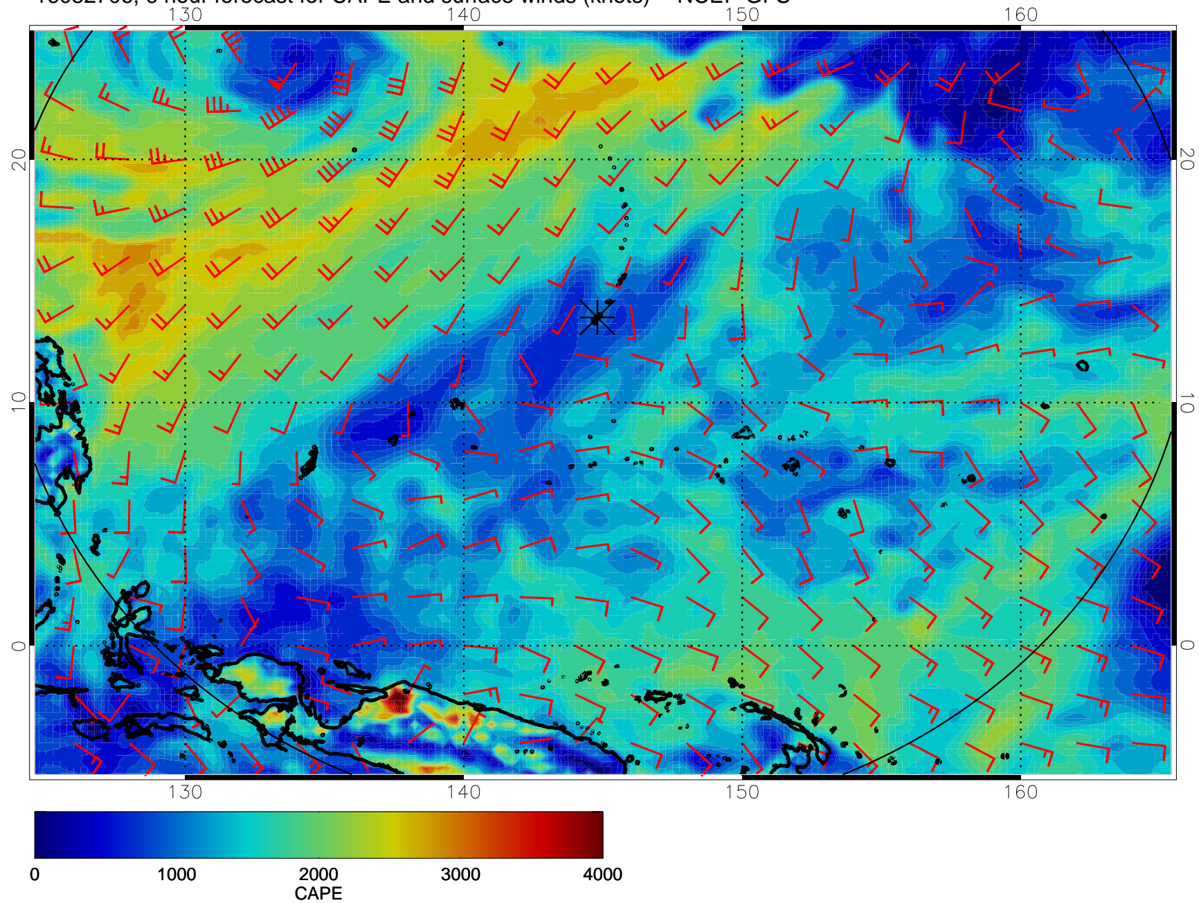
16082706, 6 hour forecast for CAPE and surface winds (knots) -- NCEP GFS
