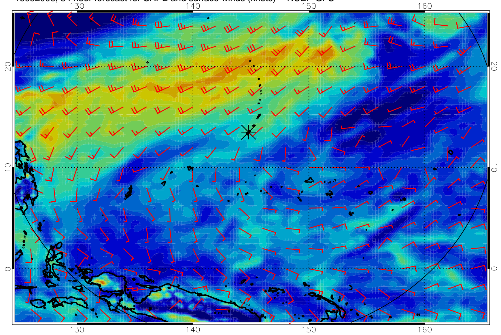
16082906, 54 hour forecast for CAPE and surface winds (knots) -- NCEP GFS
