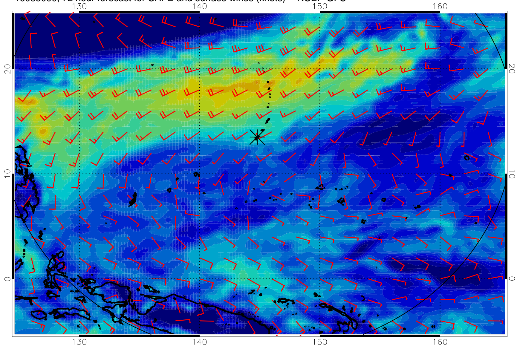
16083000, 72 hour forecast for CAPE and surface winds (knots) -- NCEP GFS
