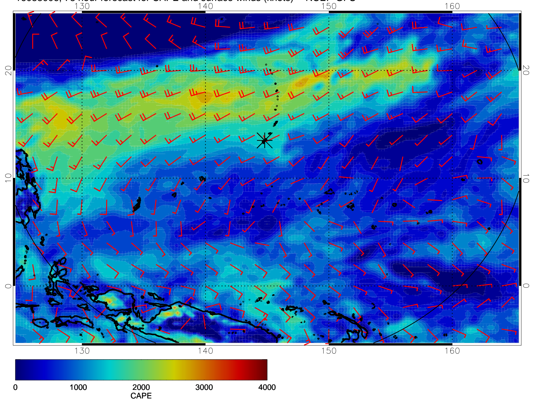
16083006, 78 hour forecast for CAPE and surface winds (knots) -- NCEP GFS
