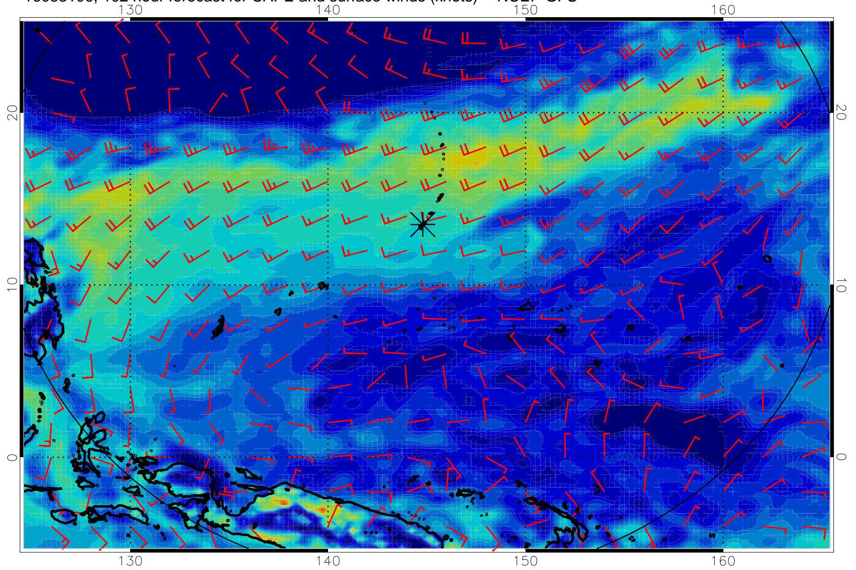
16083106, 102 hour forecast for CAPE and surface winds (knots) -- NCEP GFS
