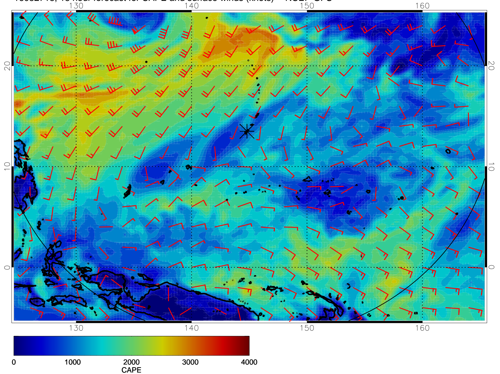
16082718, 18 hour forecast for CAPE and surface winds (knots) -- NCEP GFS
