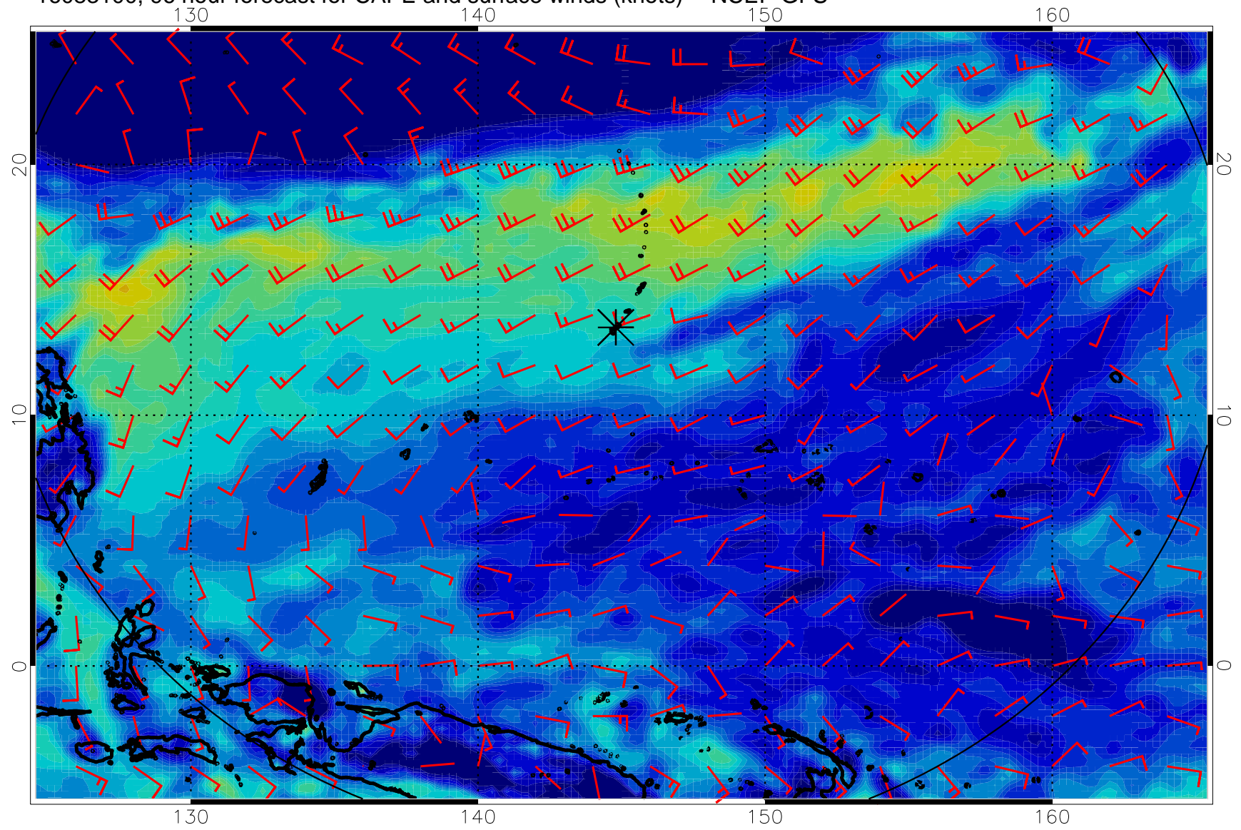
16083100, 96 hour forecast for CAPE and surface winds (knots) -- NCEP GFS
