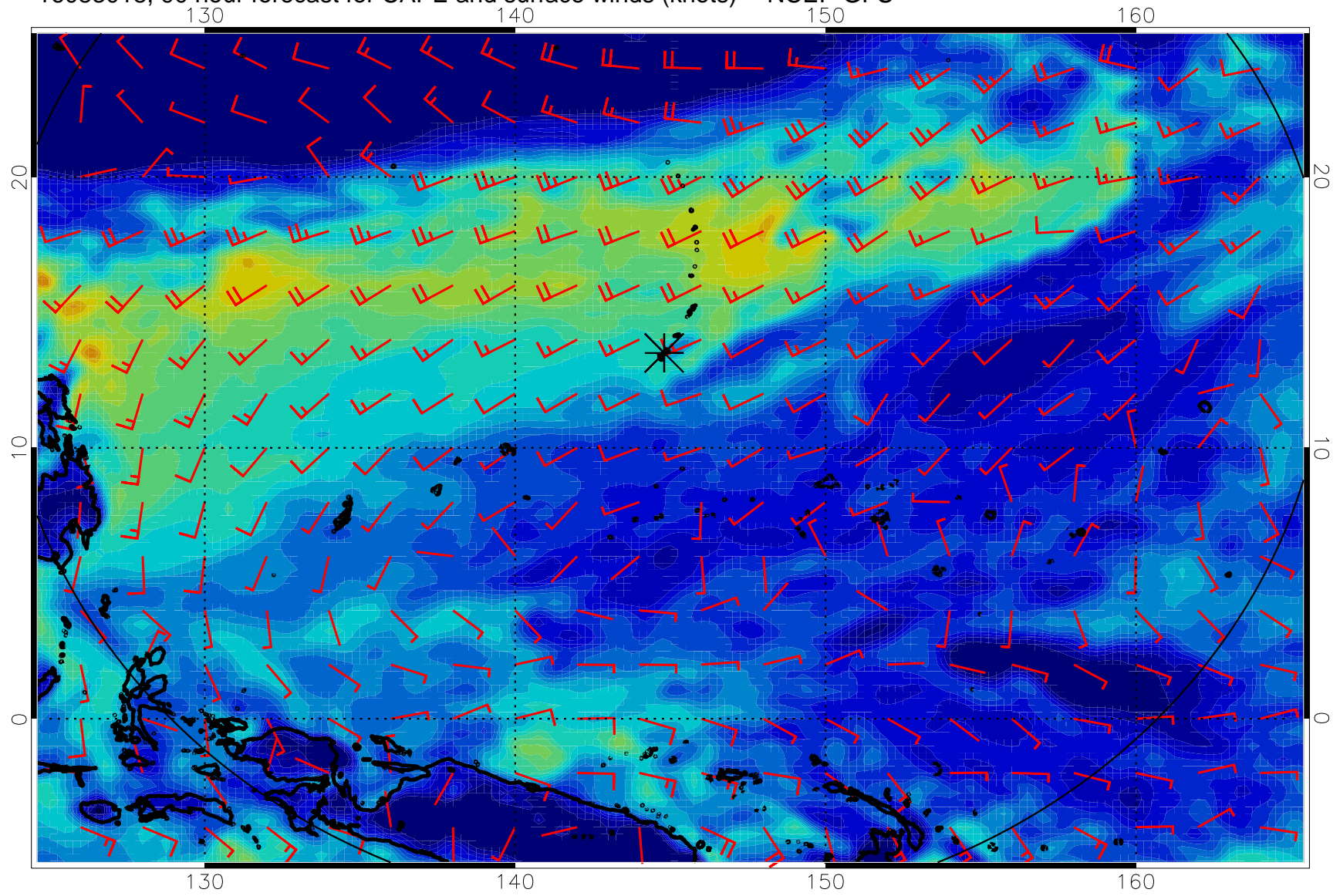
16083018, 90 hour forecast for CAPE and surface winds (knots) -- NCEP GFS
