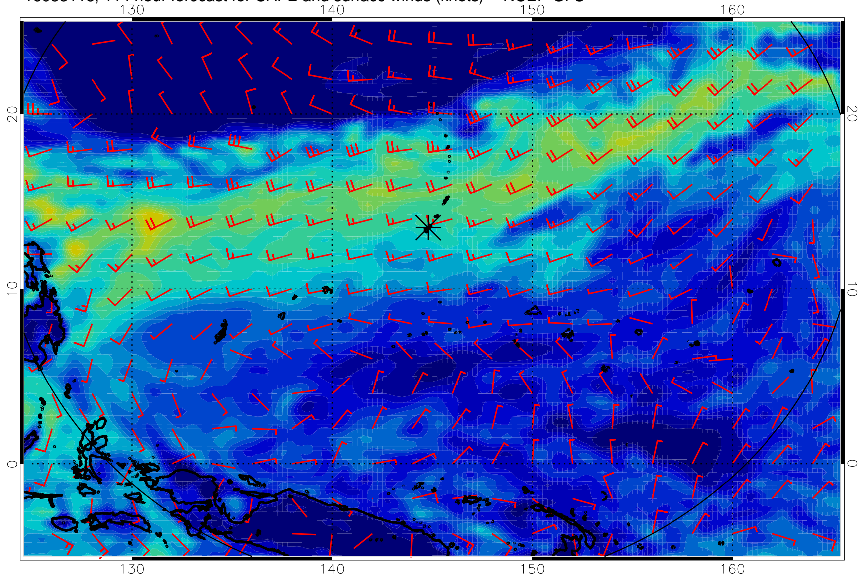
16083118, 114 hour forecast for CAPE and surface winds (knots) -- NCEP GFS
