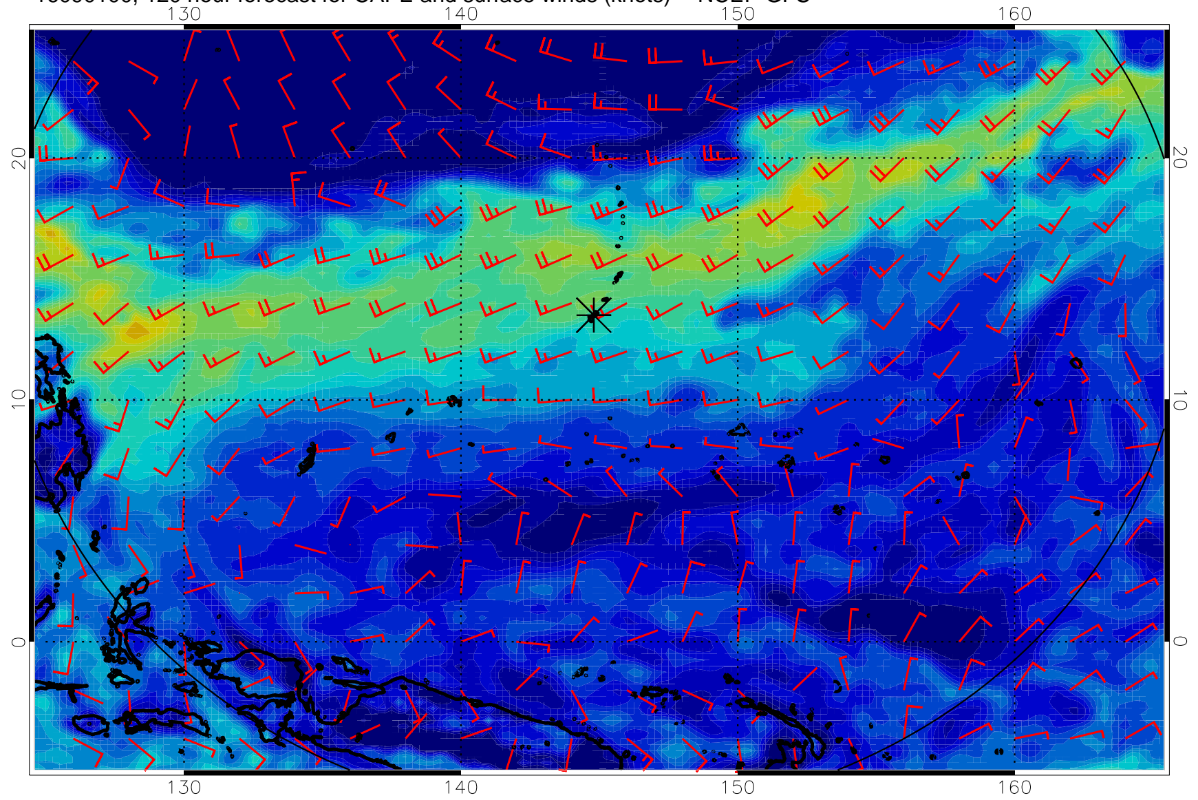
16090100, 120 hour forecast for CAPE and surface winds (knots) -- NCEP GFS
