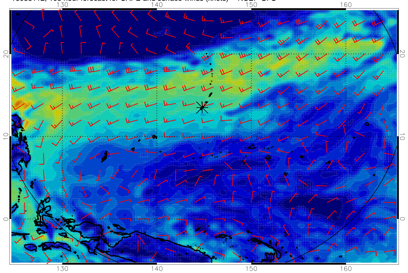
16083112, 108 hour forecast for CAPE and surface winds (knots) -- NCEP GFS
