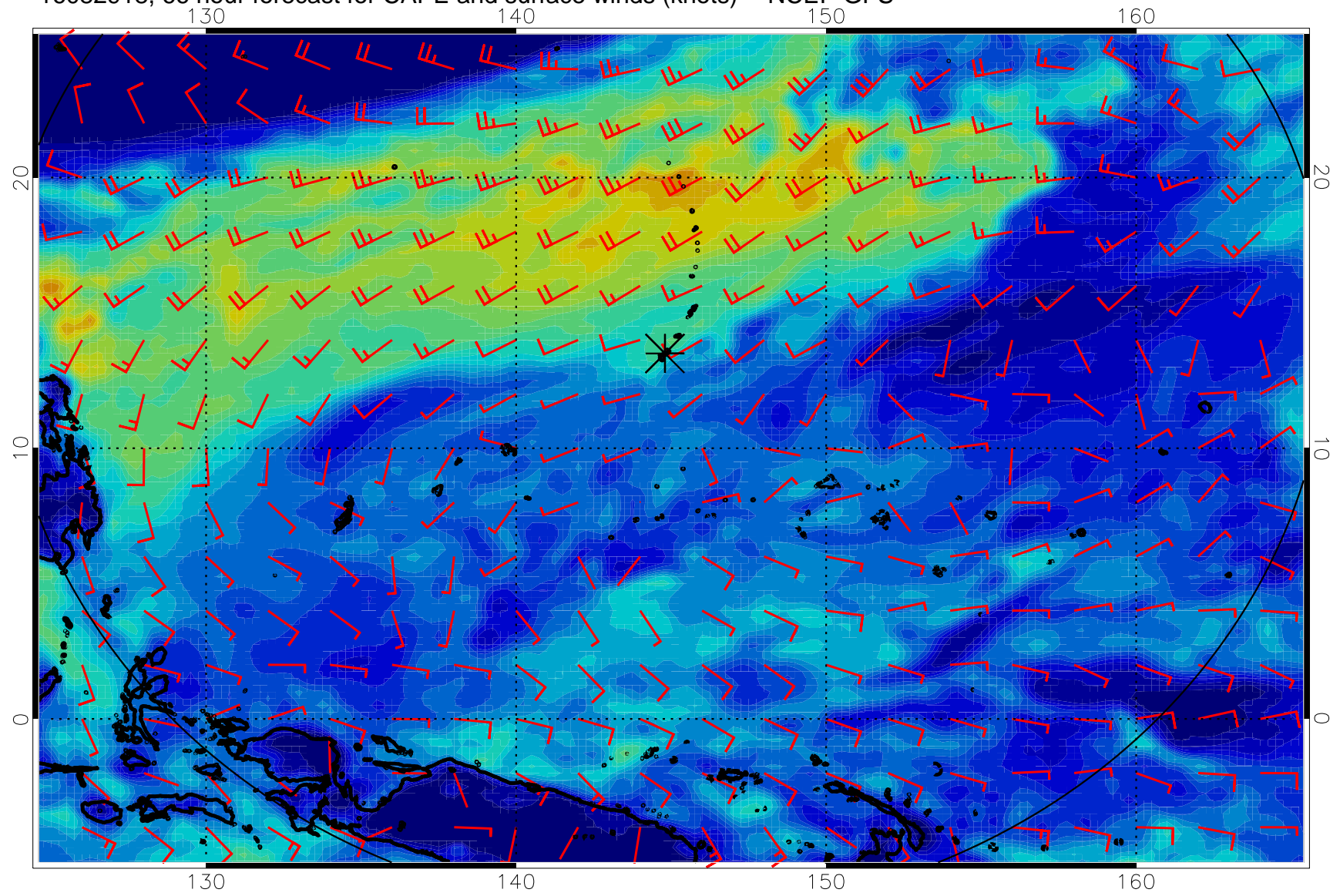
16082918, 66 hour forecast for CAPE and surface winds (knots) -- NCEP GFS
