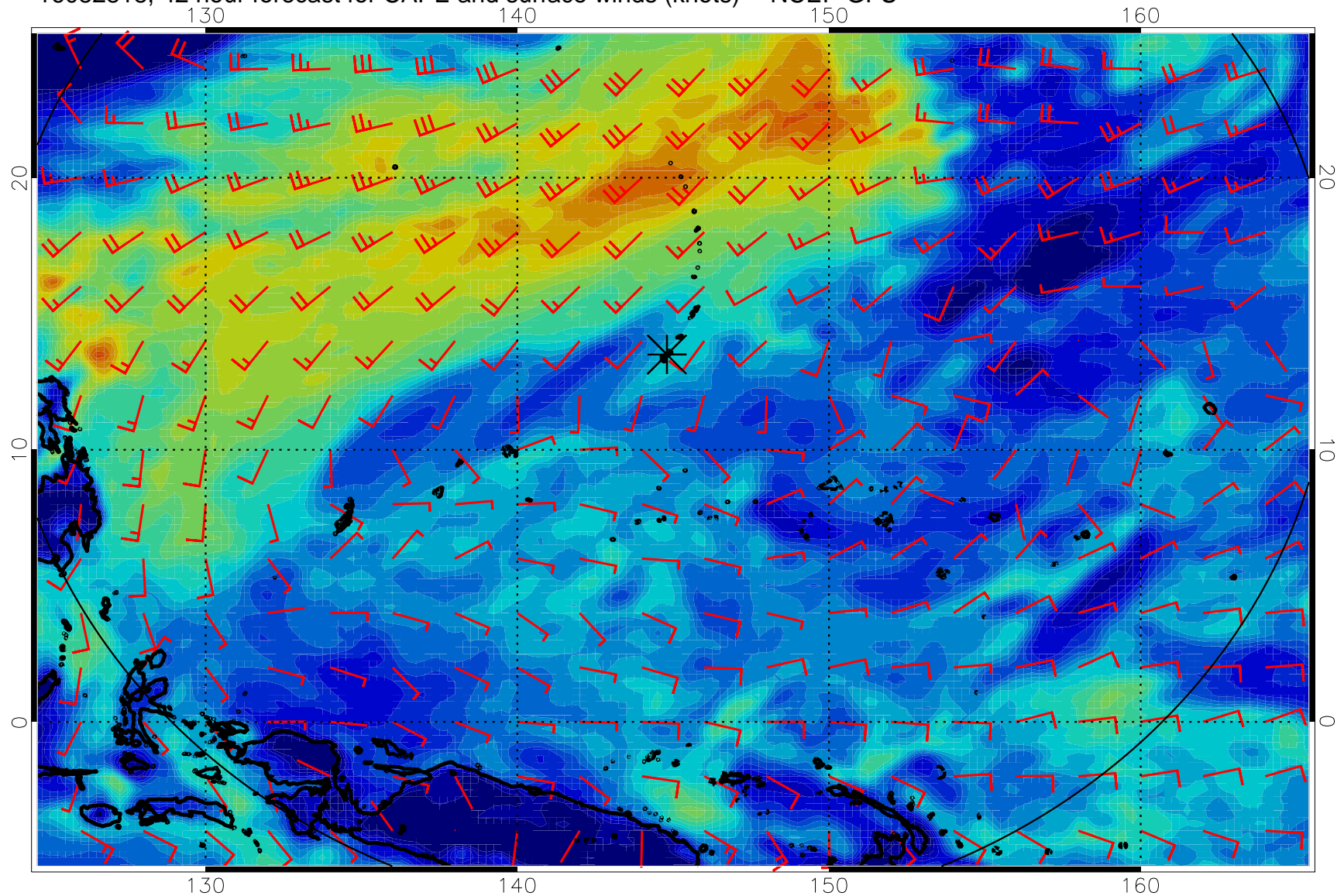
16082818, 42 hour forecast for CAPE and surface winds (knots) -- NCEP GFS
