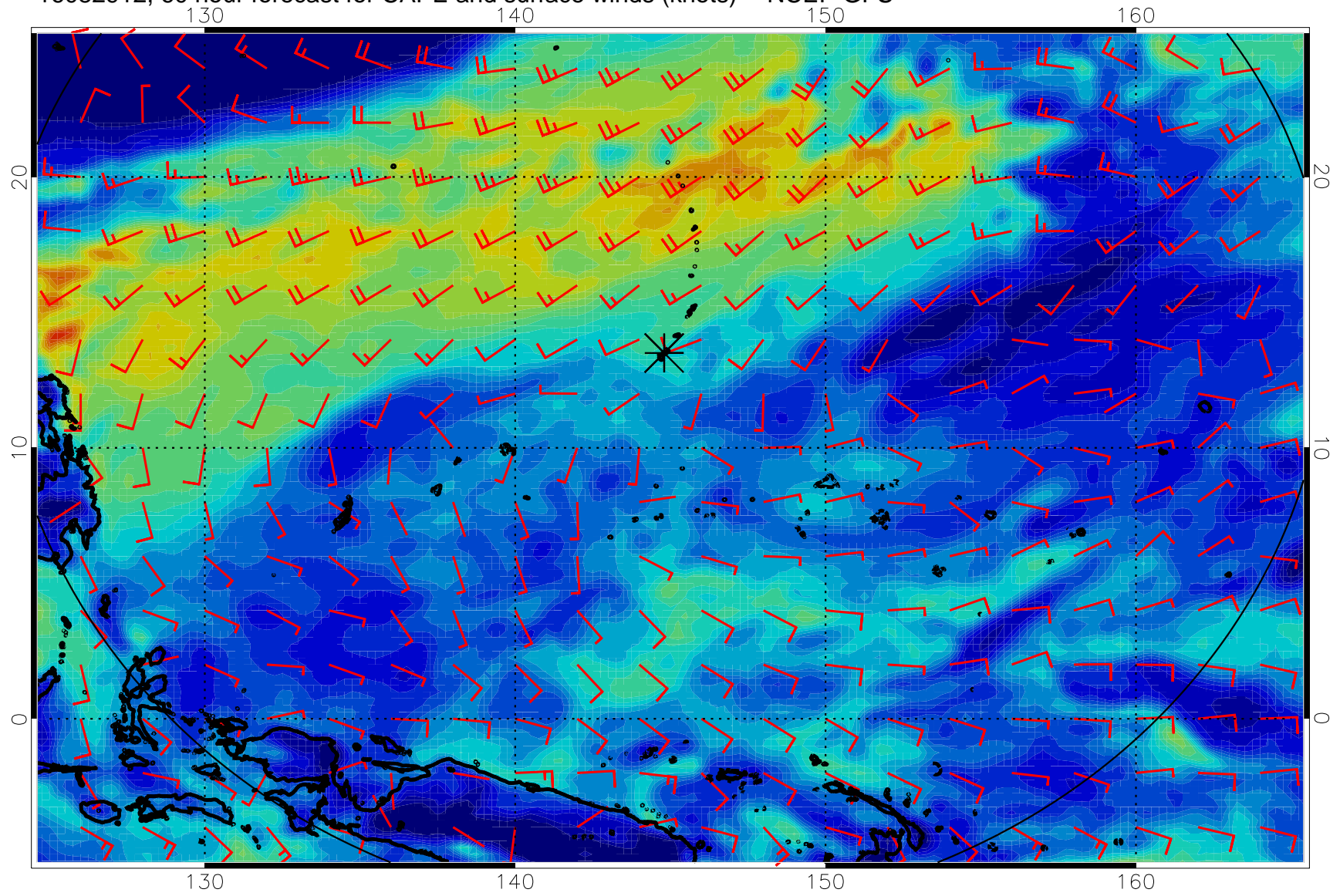
16082912, 60 hour forecast for CAPE and surface winds (knots) -- NCEP GFS
