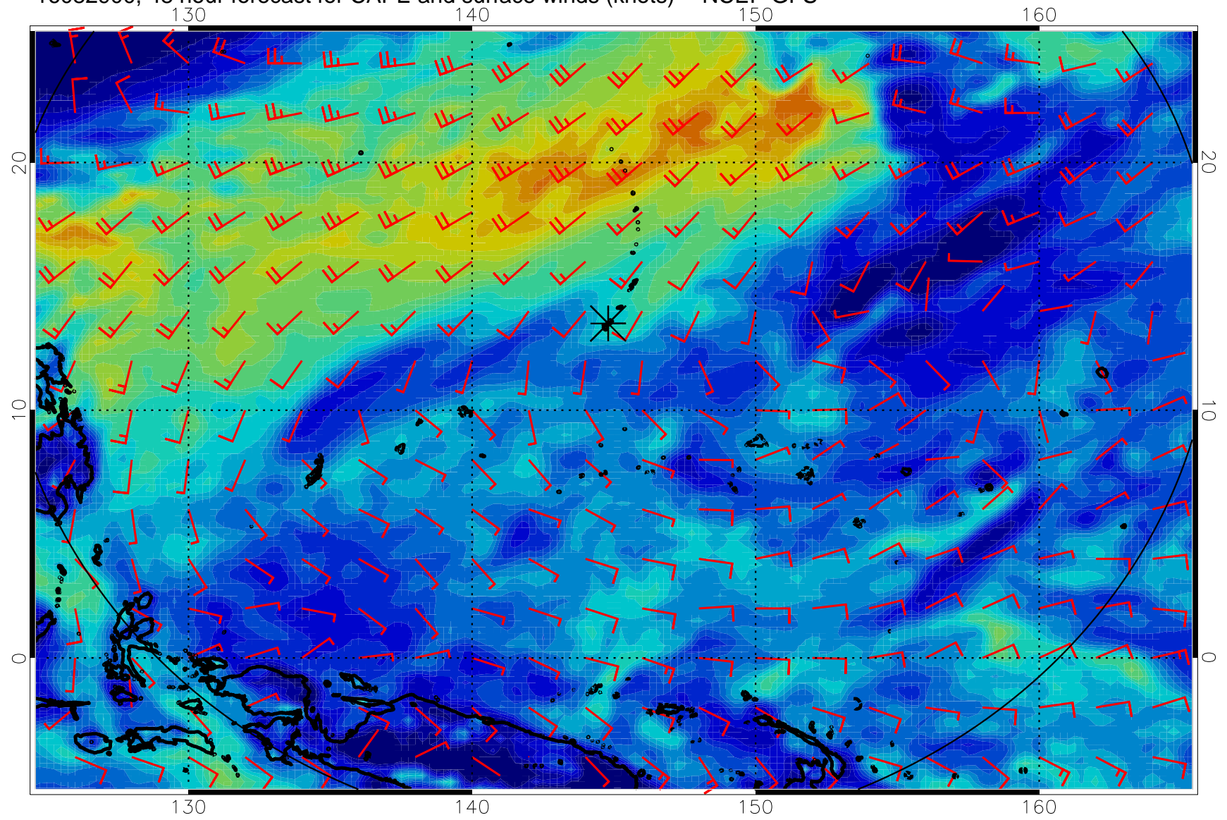
16082900, 48 hour forecast for CAPE and surface winds (knots) -- NCEP GFS
